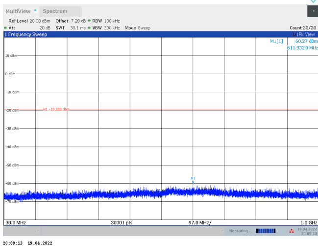
11AX40SISO_Ant1_2437_242Tone_RU61_30~1000
