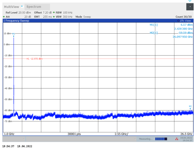
11AX20SISO_Ant1_2437_106Tone_RU53_1000~26500
