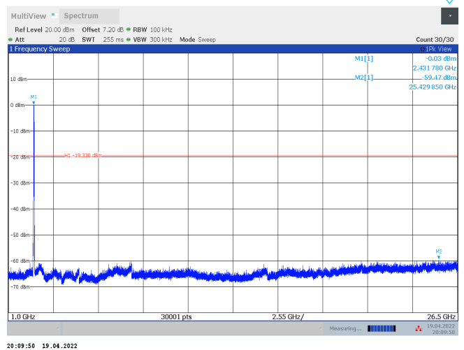
11AX40SISO_Ant1_2437_242Tone_RU61_1000~26500
