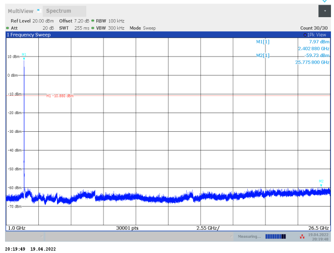
11AX20SISO_Ant2_2412_106Tone_RU53_1000~26500
