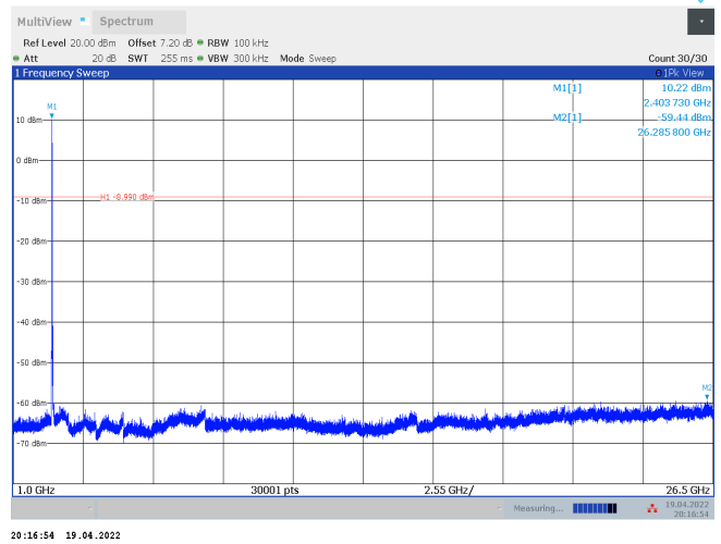
11AX20SISO_Ant2_2412_52Tone_RU37_1000~26500
