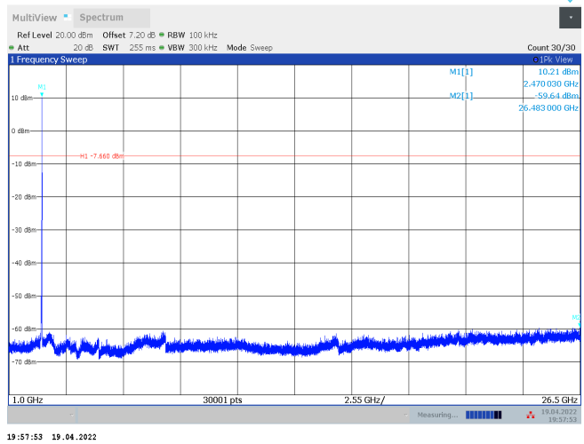
11AX20SISO_Ant1_2462_52Tone_RU37_1000~26500
