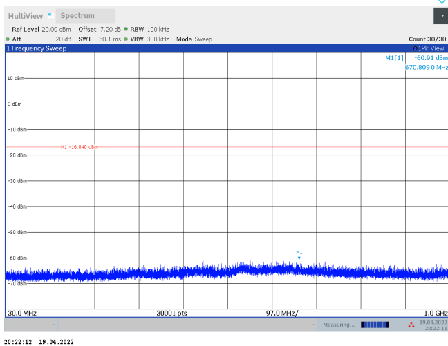
11AX20SISO_Ant2_2412_106Tone_RU53_30~1000
