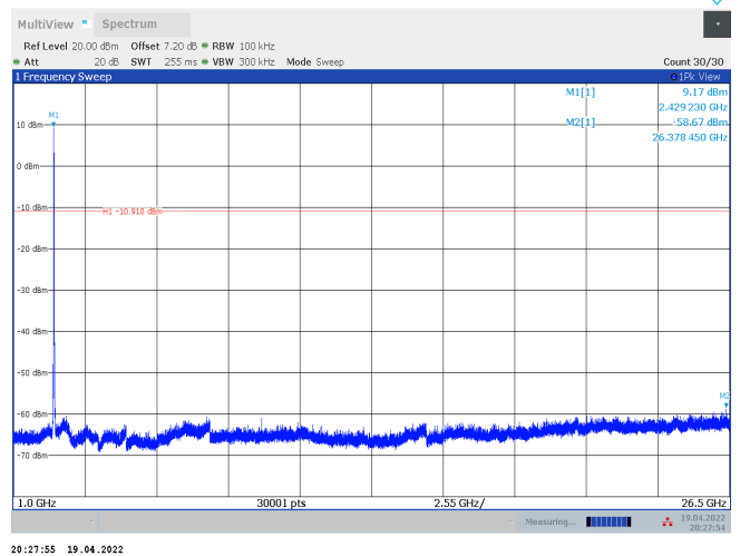
11AX20SISO_Ant2_2437_106Tone_RU53_1000~26500
