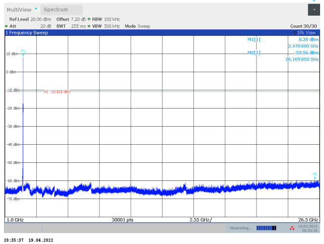
11AX20SISO_Ant2_2462_106Tone_RU53_1000~26500
