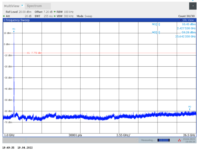
11AX20SISO_Ant1_2437_52Tone_RU37_1000~26500
