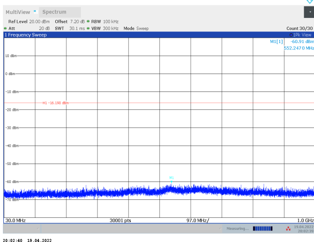
11AX20SISO_Ant1_2462_106Tone_RU53_30~1000
