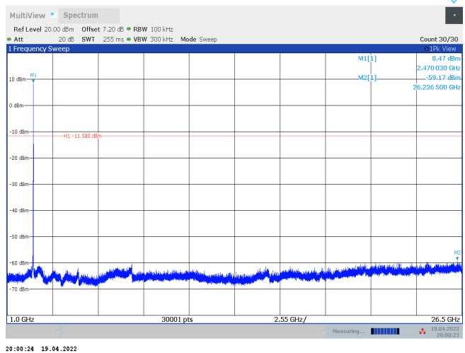
11AX20SISO_Ant1_2462_106Tone_RU53_1000~26500
