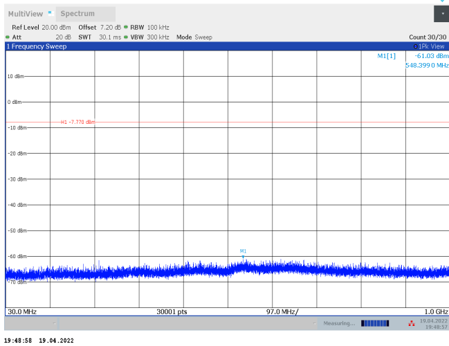
11AX20SISO_Ant1_2437_52Tone_RU37_30~1000
