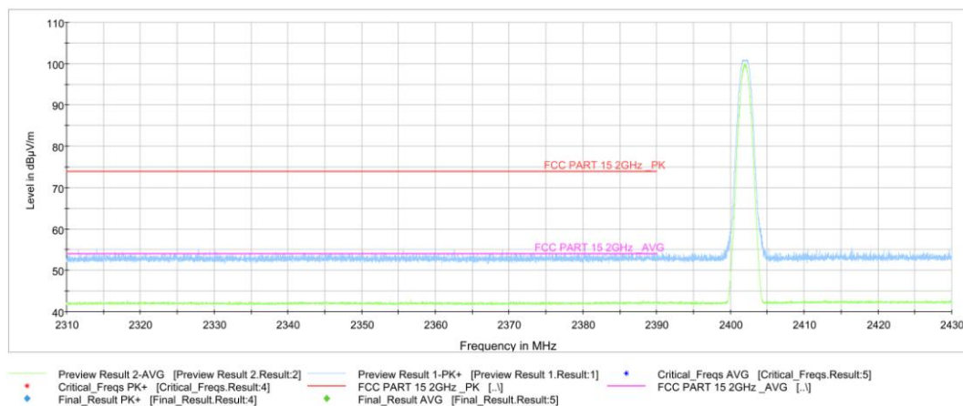
Fig.1. Frequency Band Edges: GFSK, 2402 MHz, 2.31 GHz – 2.43GHz
