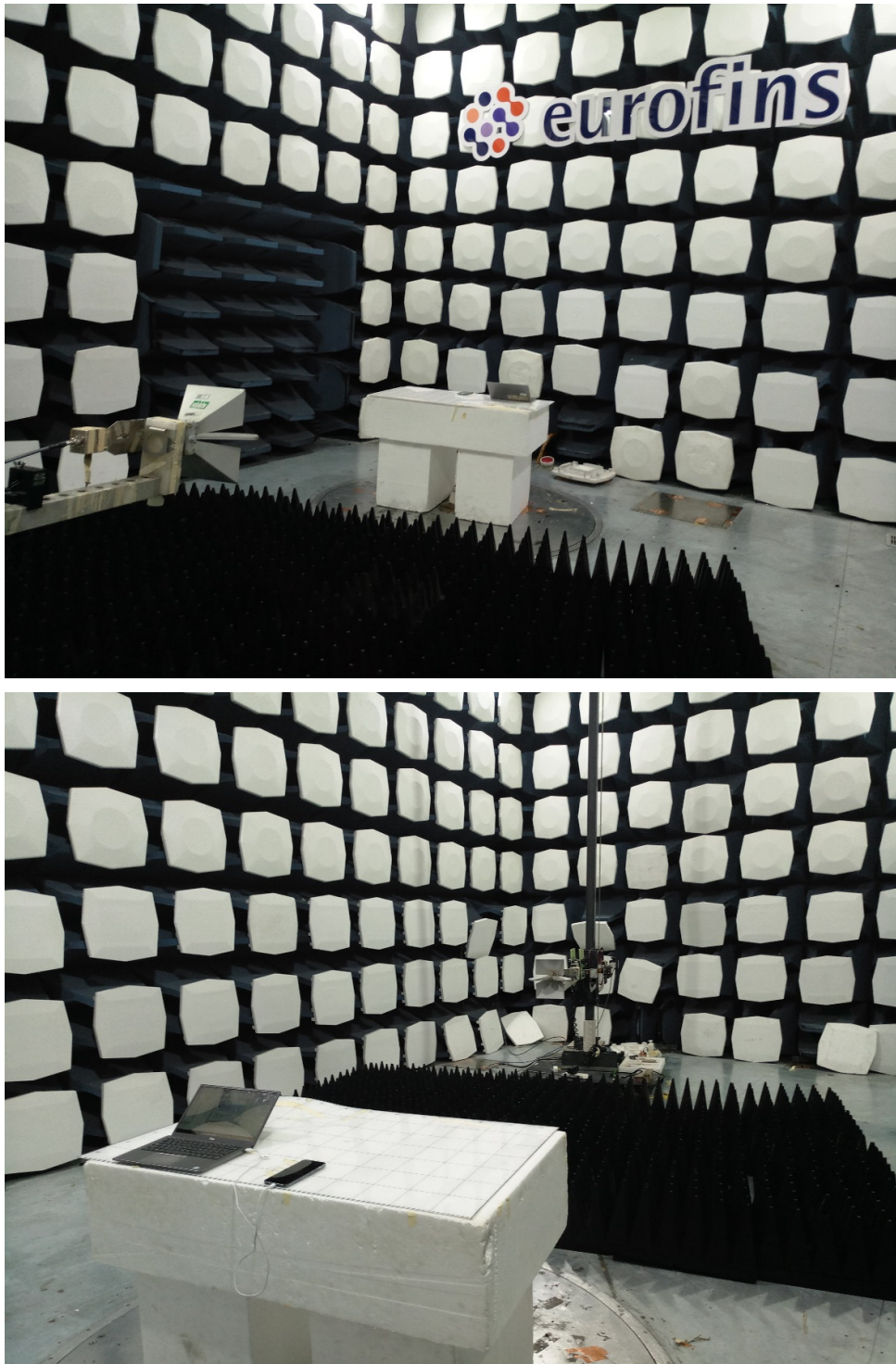
Picture 1: Radiated Emission Test Setup
