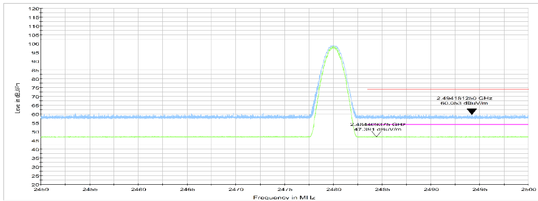
Fig.14. Frequency Band Edges: GFSK, Channel 78, ch11, 2.45 GHz - 2.50GHz
