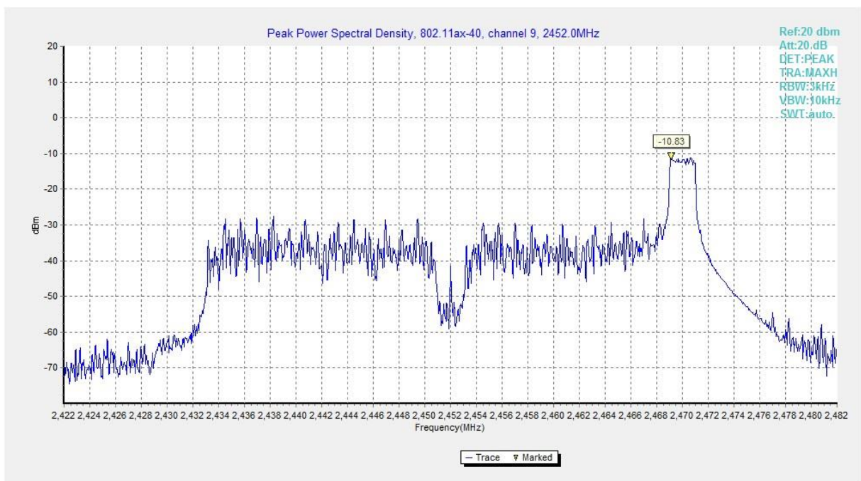
Fig.A.3.57 Power Spectral Density (802.11ax-HE40-RU26- right, Ch 9)
