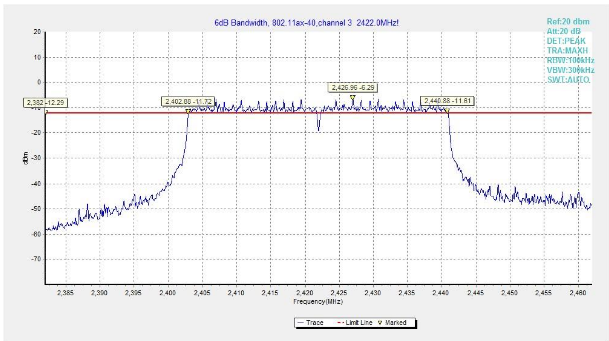
Fig.A.4.16 Occupied 6dB Bandwidth (802.11ax-HE40MHz-RU484, Ch 3)
