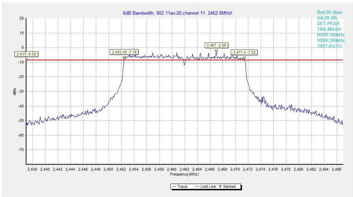
Fig.A.4.30 Occupied 6dB Bandwidth (802.11ax-HE20MHz-RU242, Ch 11)
