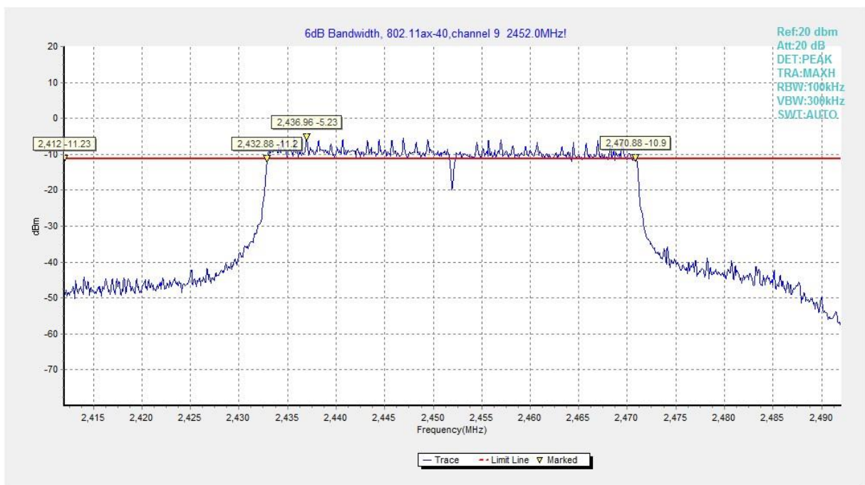
Fig.A.4.33 Occupied 6dB Bandwidth (802.11ax-HE40MHz-RU484, Ch 9)
