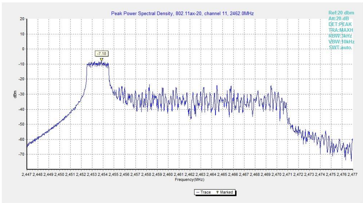
Fig.A.3.48 Power Spectral Density (802.11ax-HE20-RU26-left, Ch 11)
