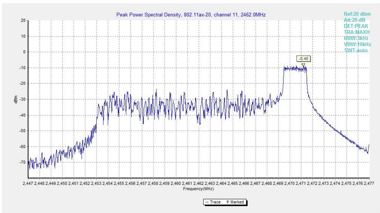
Fig.A.3.51 Power Spectral Density (802.11ax-HE20-RU26-right, Ch 11)
