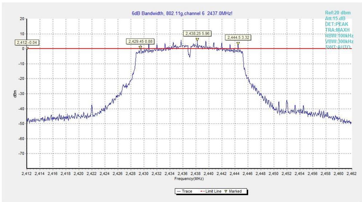
Fig.A.4.20 Occupied 6dB Bandwidth (802.11g, Ch 6)
