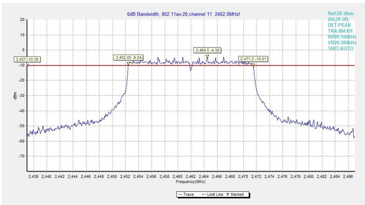
Fig.A.4.15 Occupied 6dB Bandwidth (802.11ax-HE20MHz-RU242, Ch 11)
