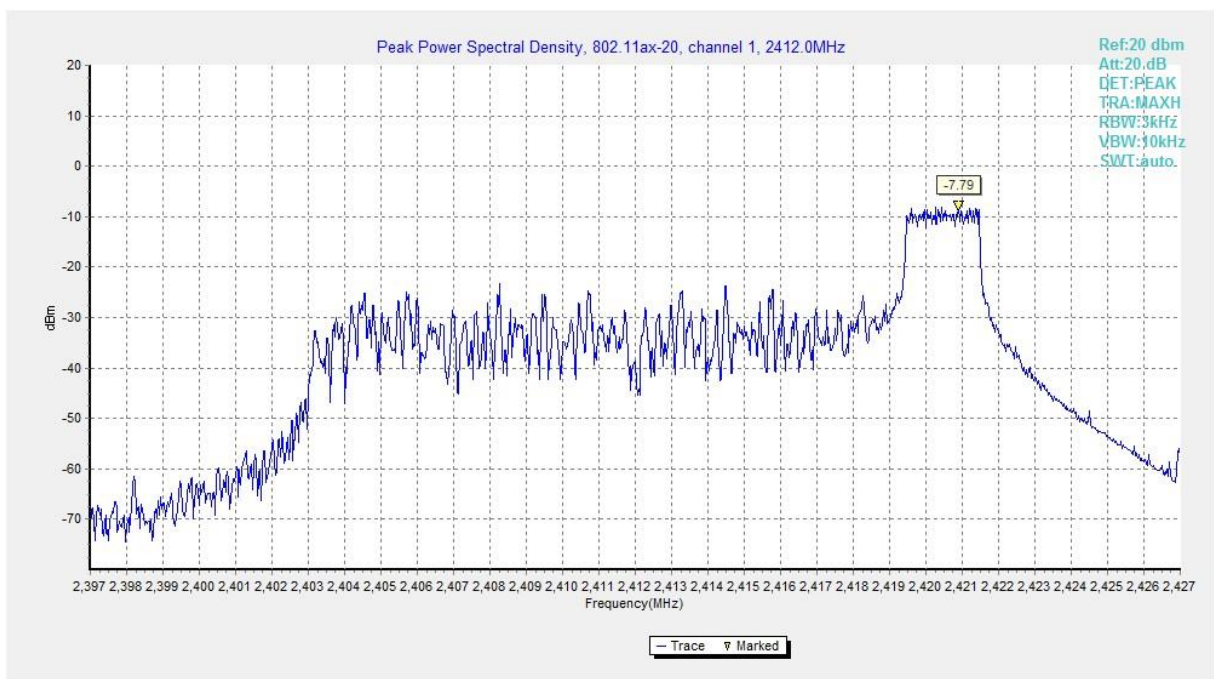
Fig.A.3.49 Power Spectral Density (802.11ax-HE20-RU26-right, Ch 1)
