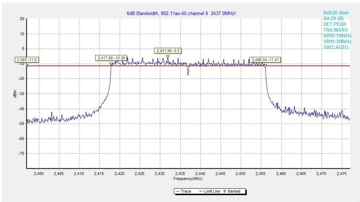
Fig.A.4.32 Occupied 6dB Bandwidth (802.11ax-HE40MHz-RU484, Ch 6)
