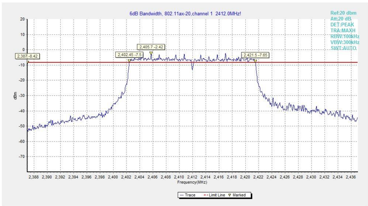
Fig.A.4.28 Occupied 6dB Bandwidth (802.11ax-HE20MHz-RU242, Ch 1)
