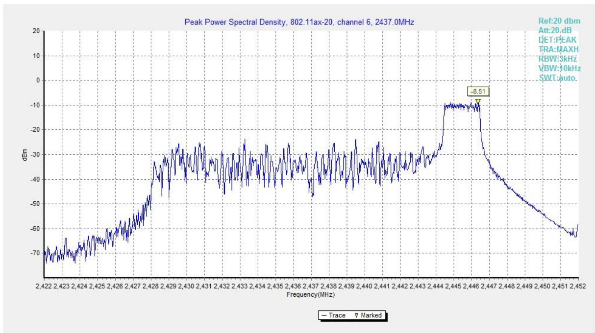
Fig.A.3.50 Power Spectral Density (802.11ax-HE20-RU26-right, Ch 6)
