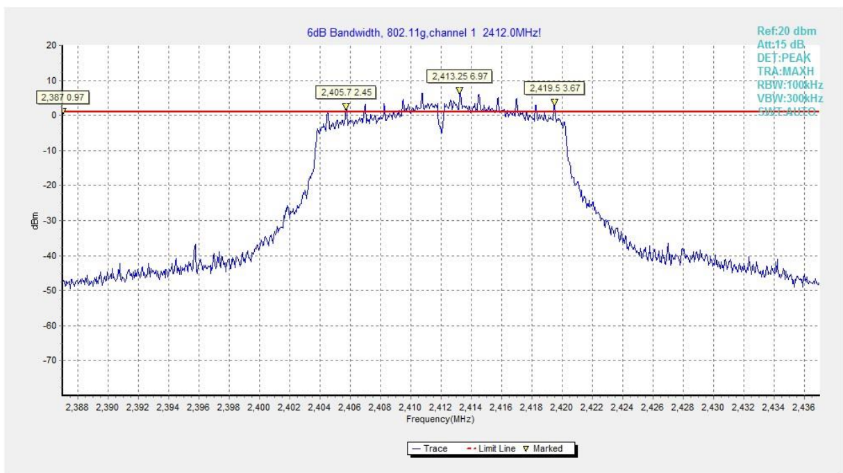
Fig.A.4.19 Occupied 6dB Bandwidth (802.11g, Ch 1)
