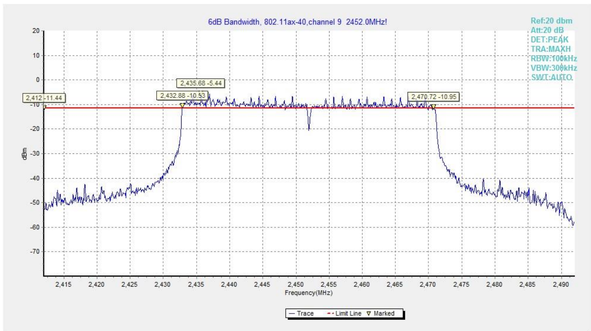
Fig.A.4.18 Occupied 6dB Bandwidth (802.11ax-HE40MHz-RU484, Ch 9)
