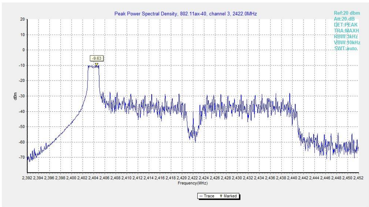
Fig.A.3.52 Power Spectral Density (802.11ax-HE40-RU26-left, Ch 3)
