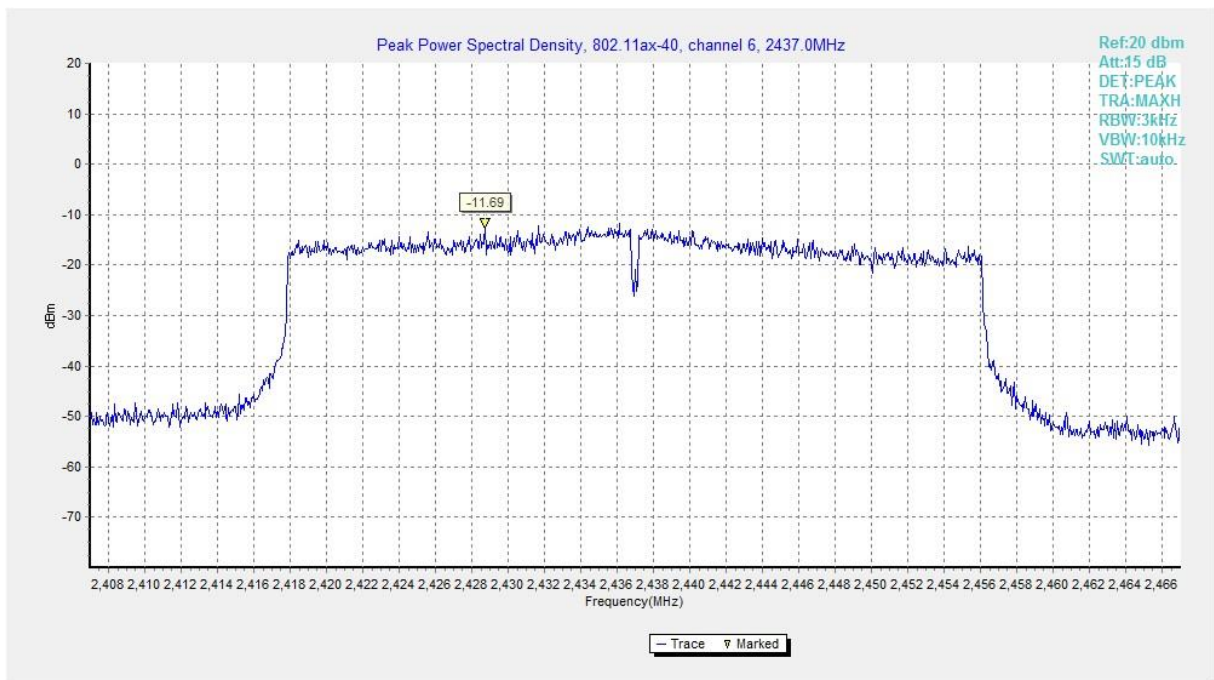
Fig.A.3.44 Power Spectral Density (802.11ax-HE40, Ch 6)
