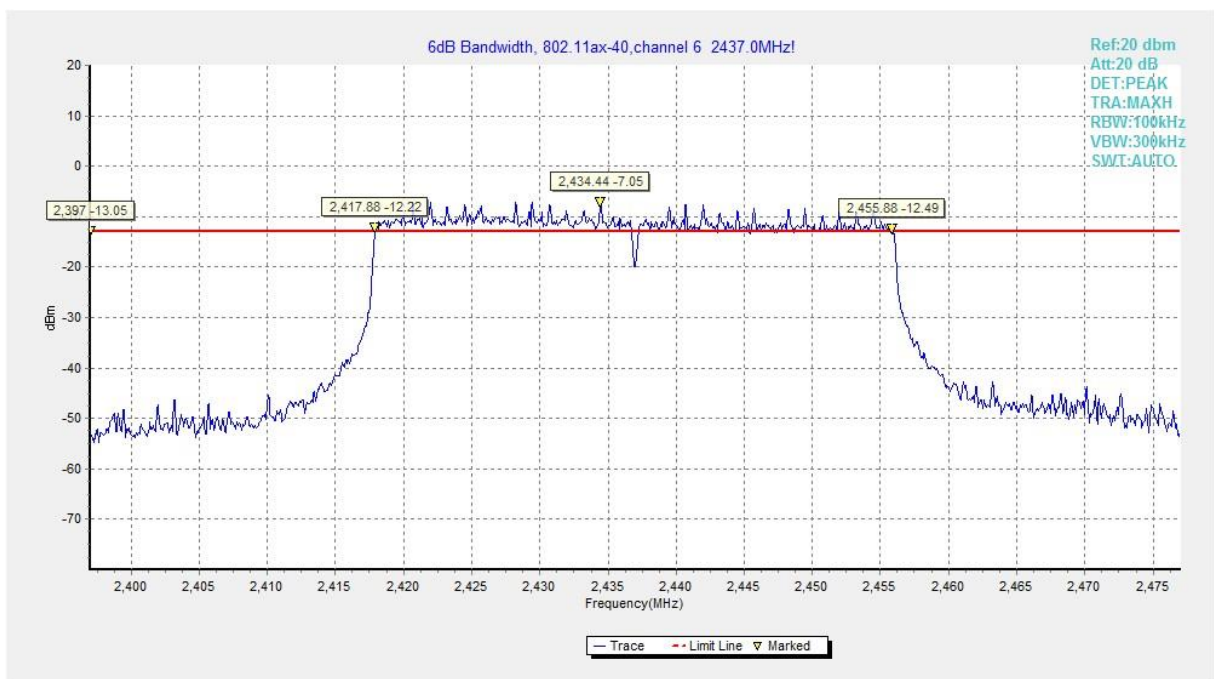
Fig.A.4.17 Occupied 6dB Bandwidth (802.11ax-HE40MHz-RU484, Ch 6)
