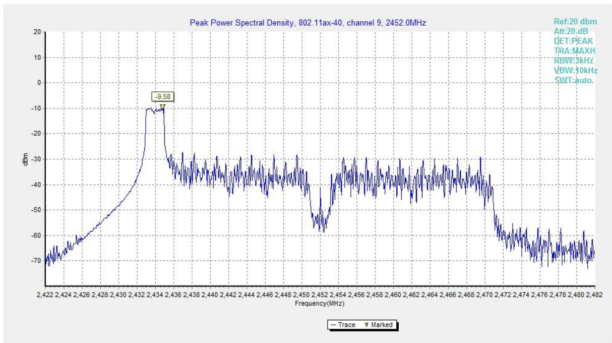
Fig.A.3.54 Power Spectral Density (802.11ax-HE40-RU26-left, Ch 9)
