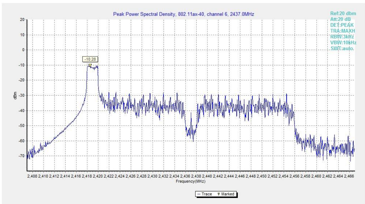
Fig.A.3.53 Power Spectral Density (802.11ax-HE40-RU26-left, Ch 6)
