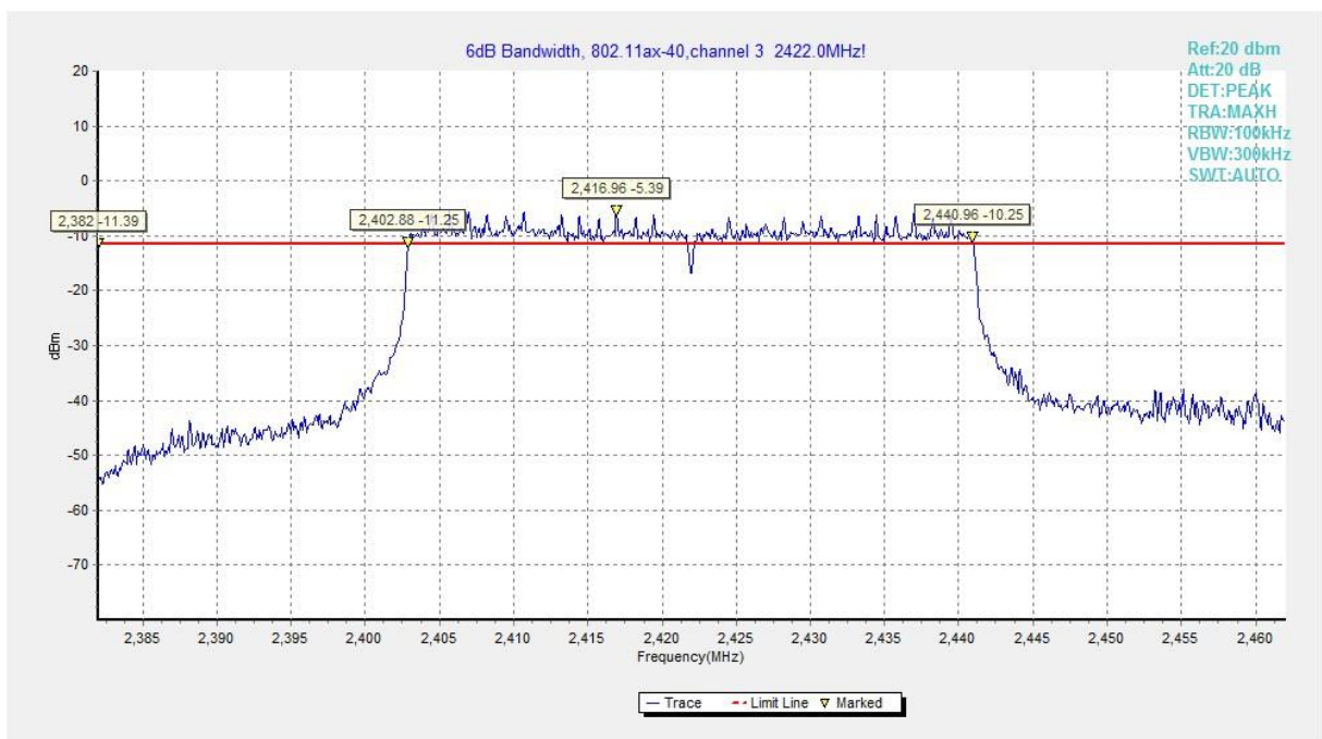
Fig.A.4.31 Occupied 6dB Bandwidth (802.11ax-HE40MHz-RU484, Ch 3)
