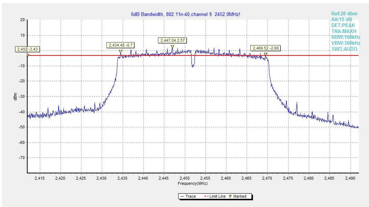
Fig.A.4.27 Occupied 6dB Bandwidth (802.11n-HT40, Ch 9)
