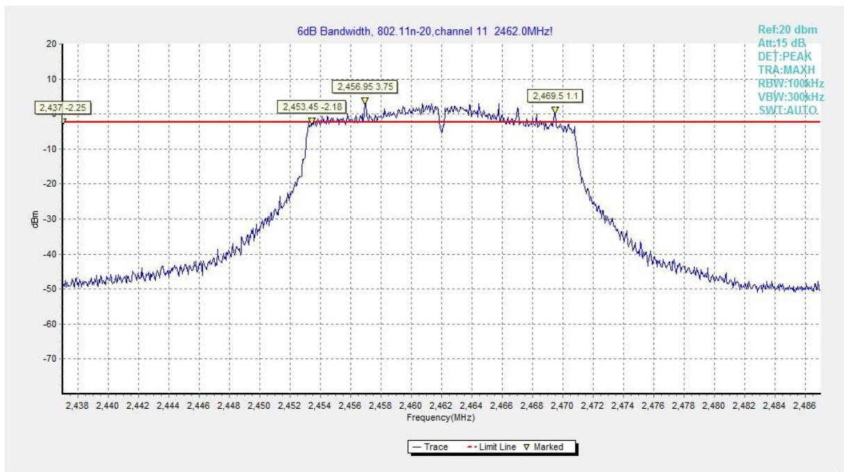
Fig.A.4.24 Occupied 6dB Bandwidth (802.11n-HT20, Ch 11)
