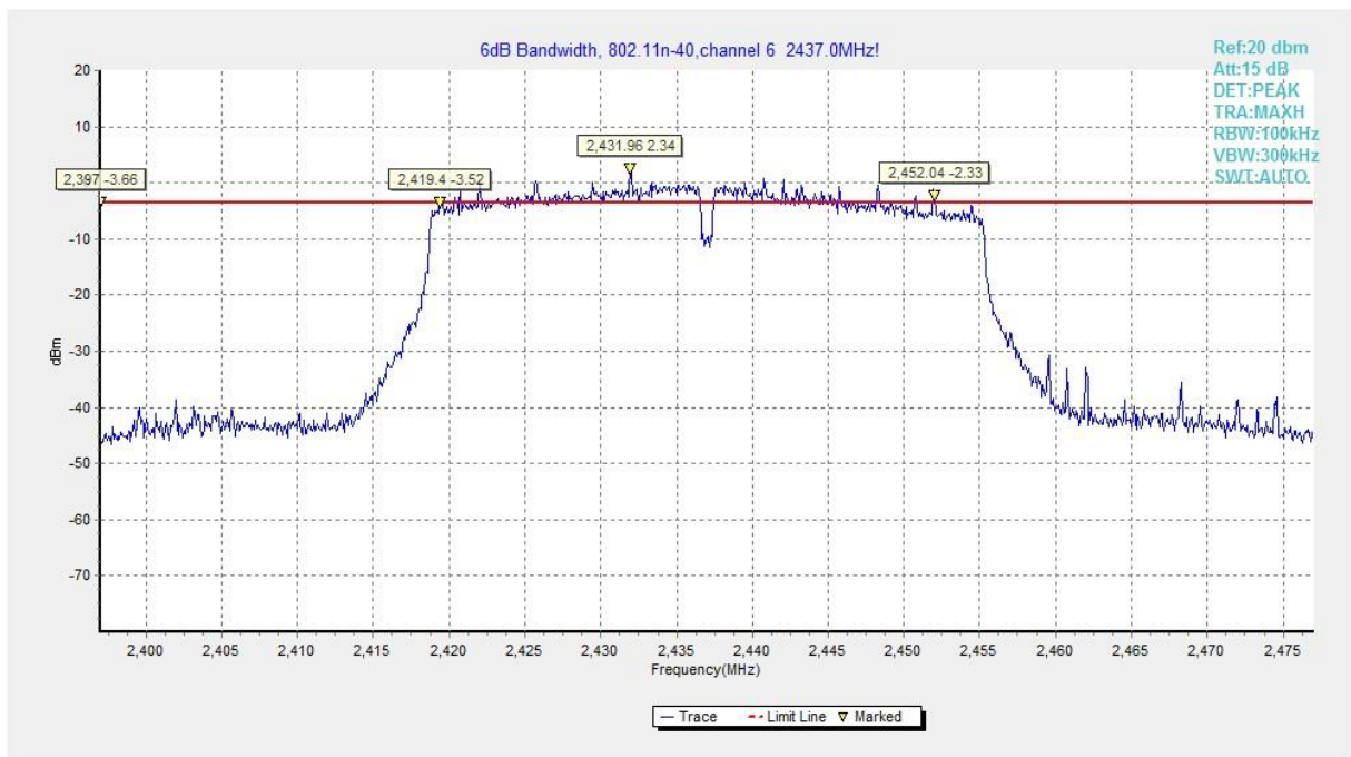
Fig.A.4.26 Occupied 6dB Bandwidth (802.11n-HT40, Ch 6)
