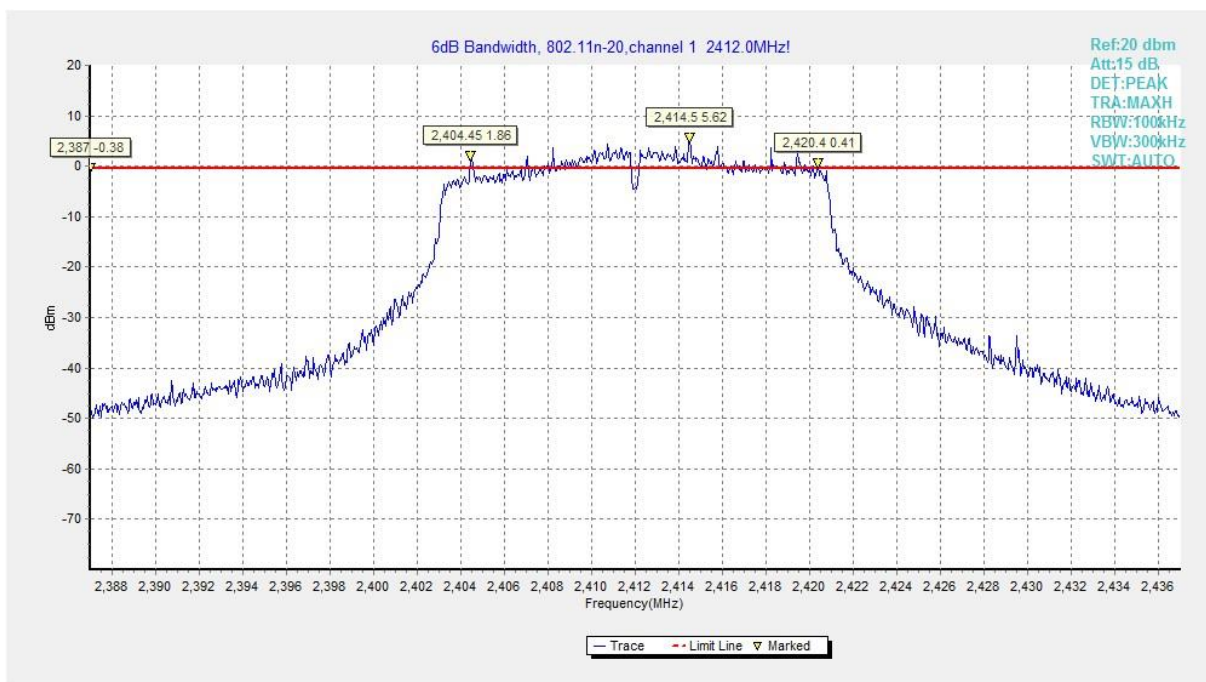
Fig.A.4.22 Occupied 6dB Bandwidth (802.11n-20MHz, Ch 1)
