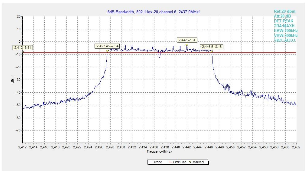
Fig.A.4.29 Occupied 6dB Bandwidth (802.11ax-HE20MHz-RU242, Ch 6)
