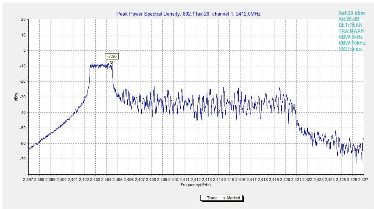
Fig.A.3.46 Power Spectral Density (802.11ax-HE20-RU26-left, Ch 1)
