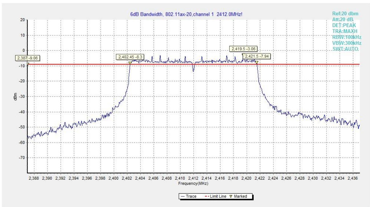
Fig.A.4.13 Occupied 6dB Bandwidth (802.11ax-HE20MHz-RU242, Ch 1)
