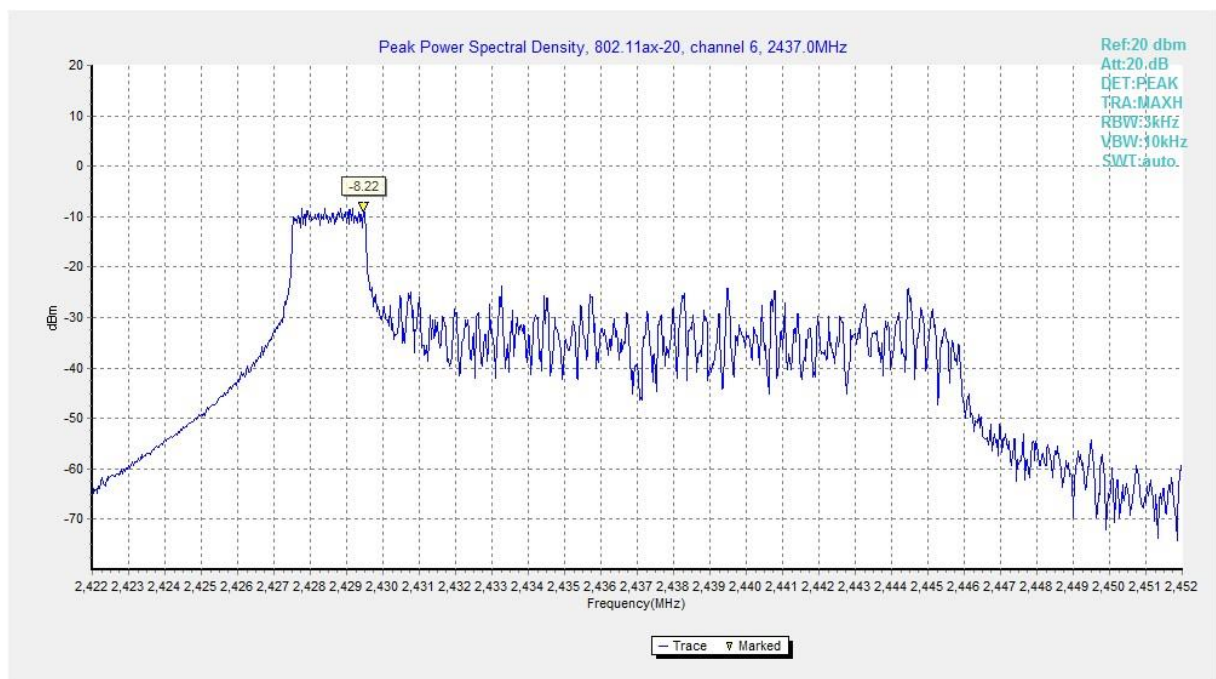
Fig.A.3.47 Power Spectral Density (802.11ax-HE20-RU26-left, Ch 6)
