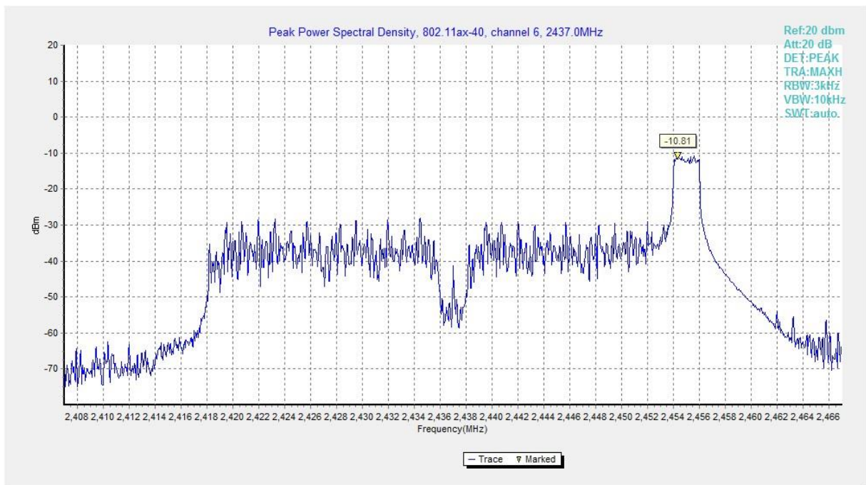
Fig.A.3.56 Power Spectral Density (802.11ax-HE40-RU26- right, Ch 6)
