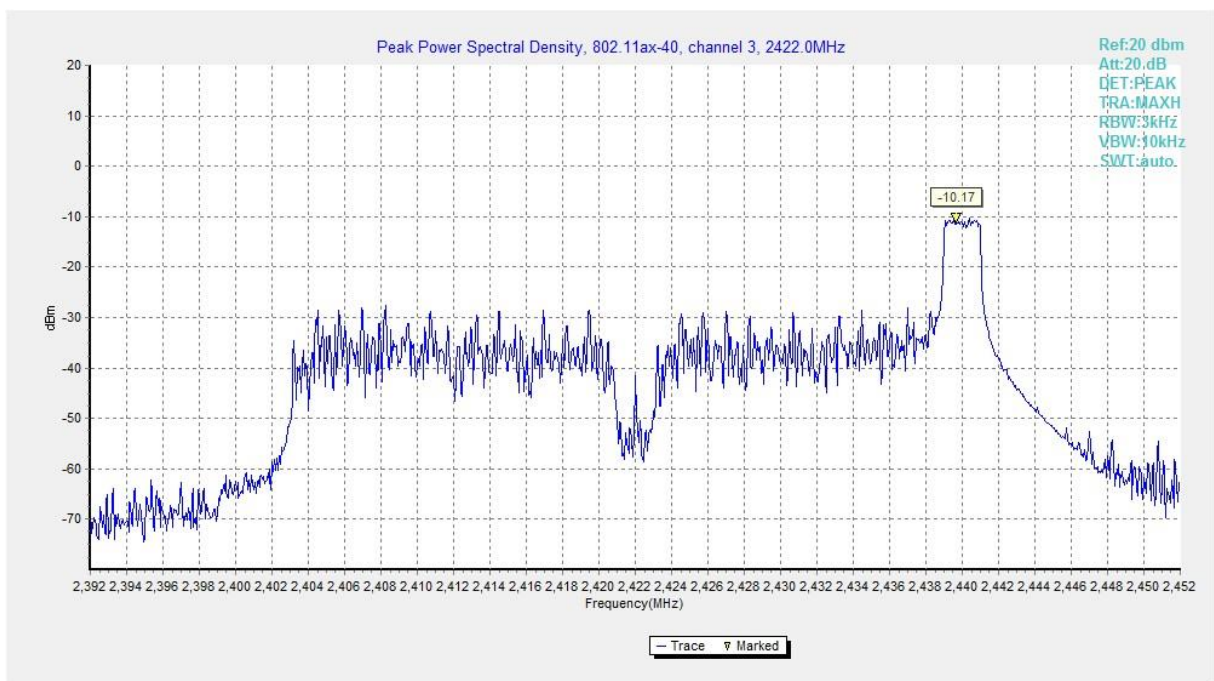
Fig.A.3.55 Power Spectral Density (802.11ax-HE40-RU26-right, Ch 3)
