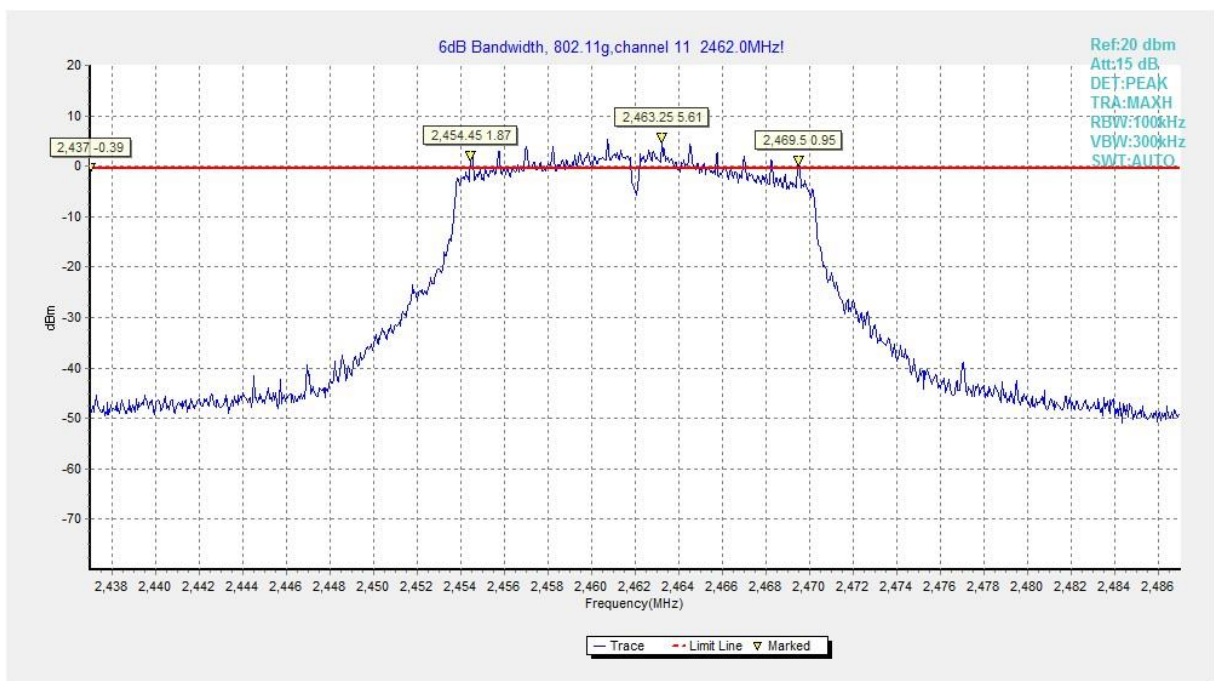
Fig.A.4.21 Occupied 6dB Bandwidth (802.11g, Ch 11)
