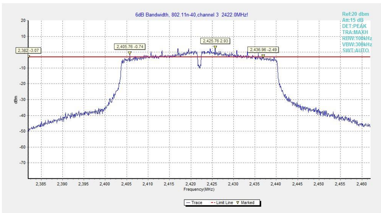
Fig.A.4.25 Occupied 6dB Bandwidth (802.11n-40MHz, Ch 3)
