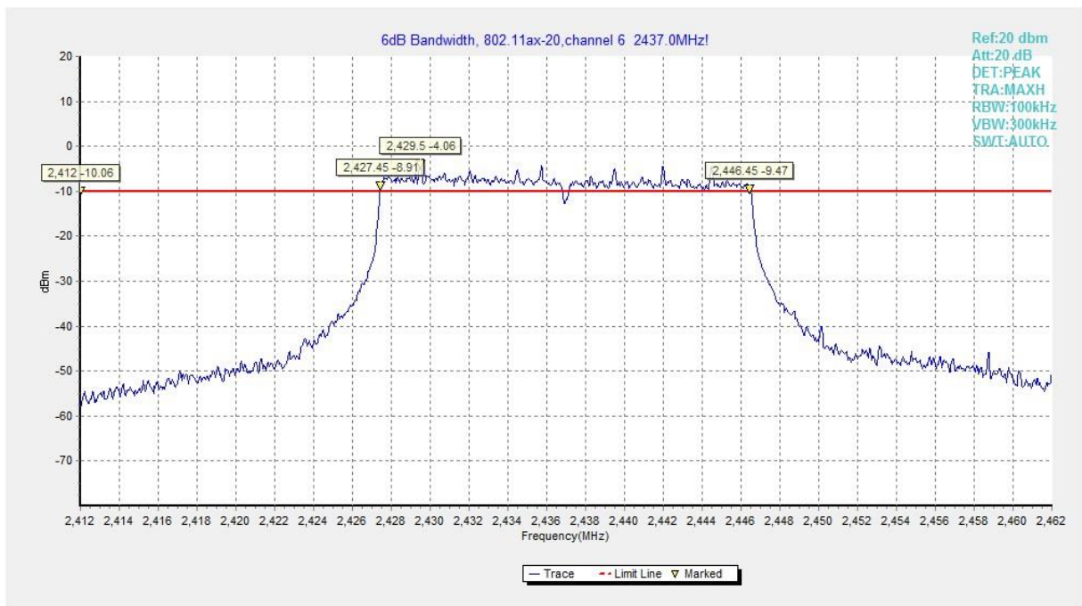
Fig.A.4.14 Occupied 6dB Bandwidth (802.11ax-HE20MHz-RU242, Ch 6)
