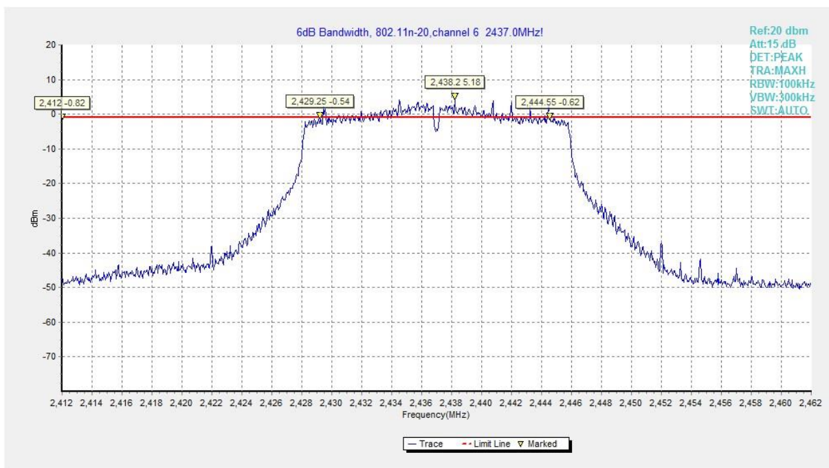
Fig.A.4.23 Occupied 6dB Bandwidth (802.11n-HT20, Ch 6)
