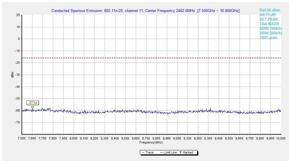
Fig.A.6.1.405 Transmitter Spurious Emission - Conducted (802.11n-HT20, Ch11, 7.5 GHz-10 GHz)
