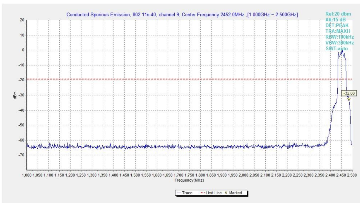
Fig.A.6.1.427 Transmitter Spurious Emission - Conducted (802.11n-HT40, Ch9, 1 GHz-2.5 GHz)
