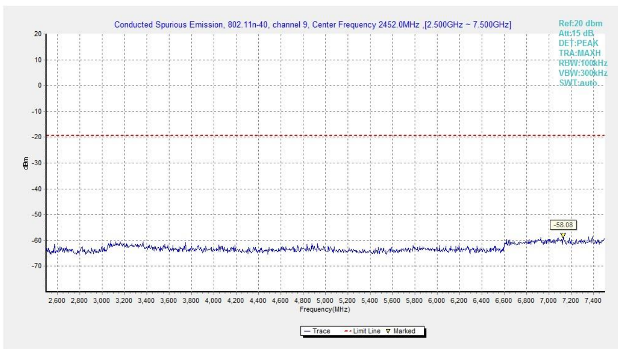
Fig.A.6.1.428 Transmitter Spurious Emission - Conducted (802.11n-HT40, Ch9, 2.5 GHz-7.5 GHz)
