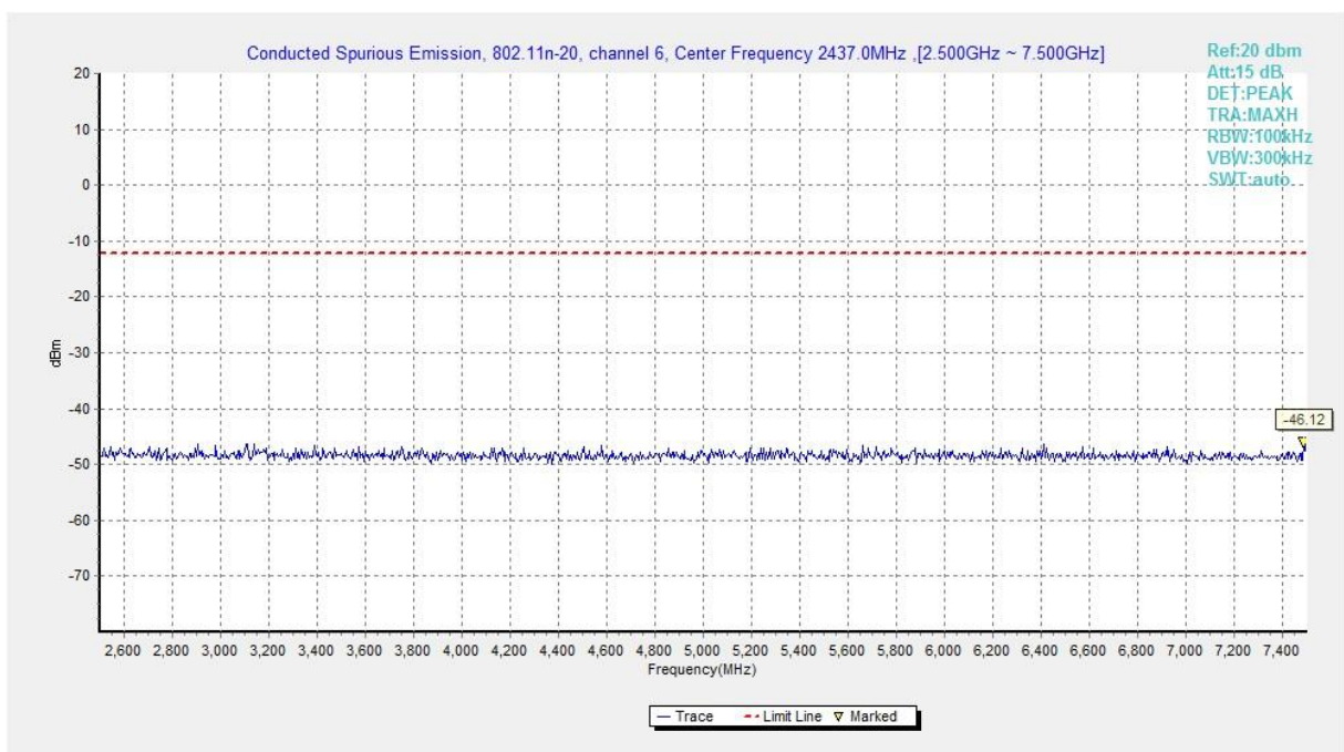
Fig.A.6.1.396 Transmitter Spurious Emission - Conducted (802.11n-HT20, Ch6, 2.5 GHz-7.5 GHz)
