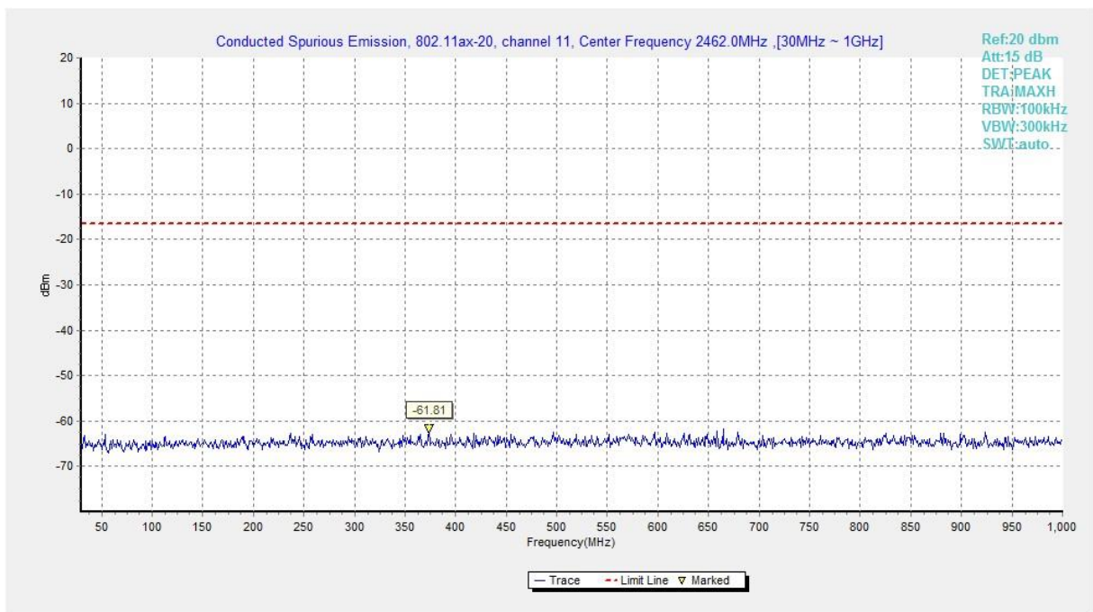
Fig.A.6.1.450 Transmitter Spurious Emission - Conducted (802.11ax-HE20, Ch11, 30 MHz-1 GHz)
