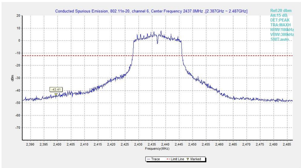
Fig.A.6.1.393 Transmitter Spurious Emission - Conducted (802.11n-HT20, Ch6, Center Frequency)
