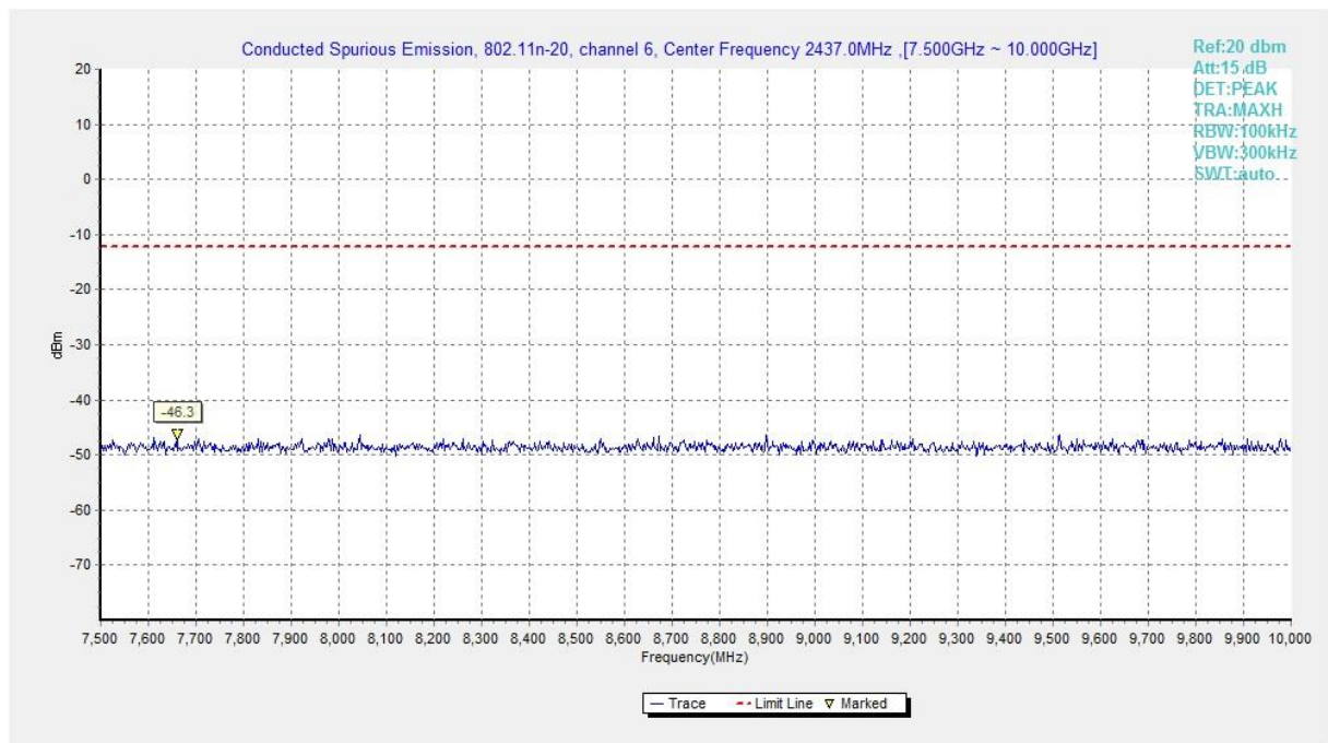
Fig.A.6.1.397 Transmitter Spurious Emission - Conducted (802.11n-HT20, Ch6, 7.5 GHz-10 GHz)
