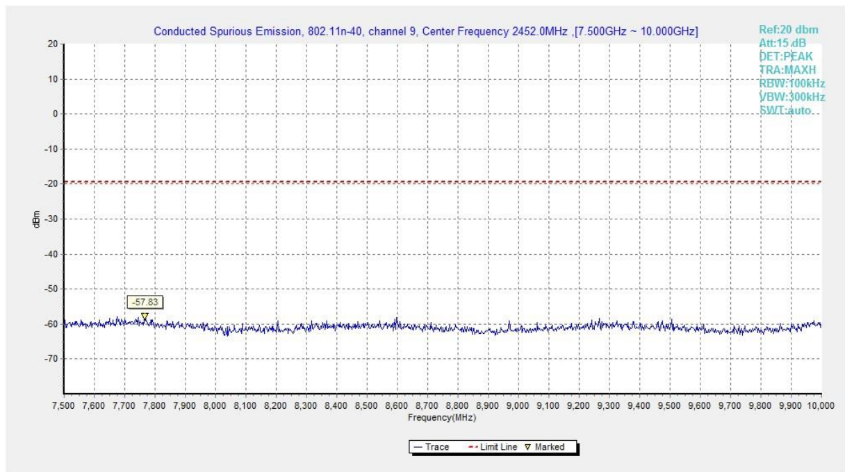
Fig.A.6.1.429 Transmitter Spurious Emission - Conducted (802.11n-HT40, Ch9, 7.5 GHz-10 GHz)
