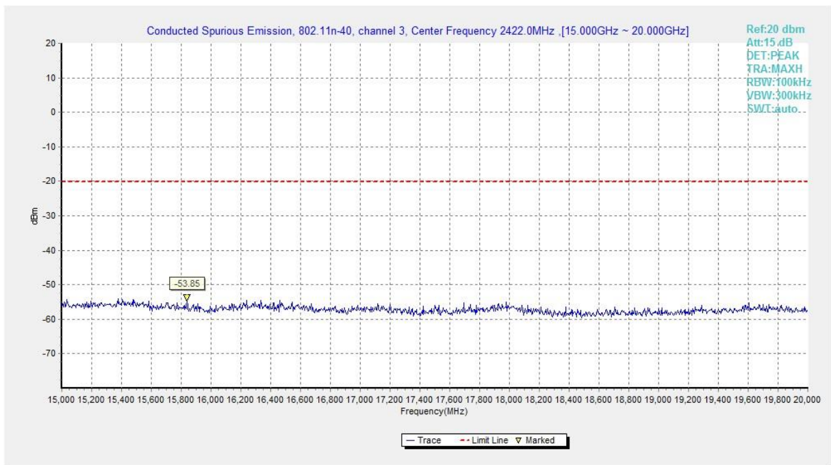
Fig.A.6.1.415 Transmitter Spurious Emission - Conducted (802.11n-HT40, Ch3, 15 GHz-20 GHz)
