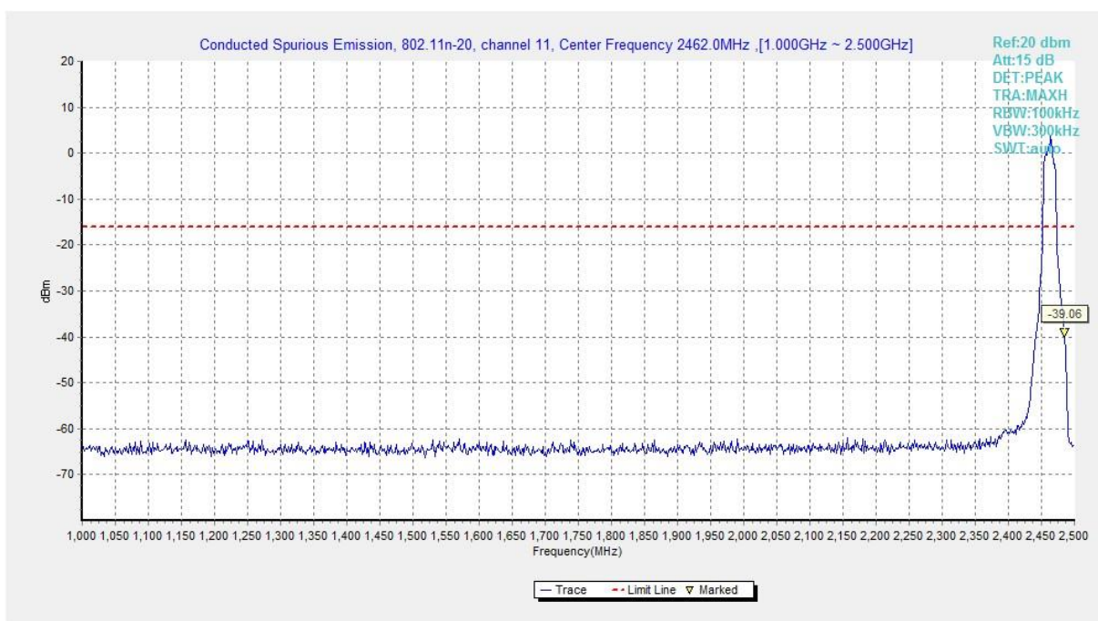
Fig.A.6.1.403 Transmitter Spurious Emission - Conducted (802.11n-HT20, Ch11, 1 GHz-2.5 GHz)
