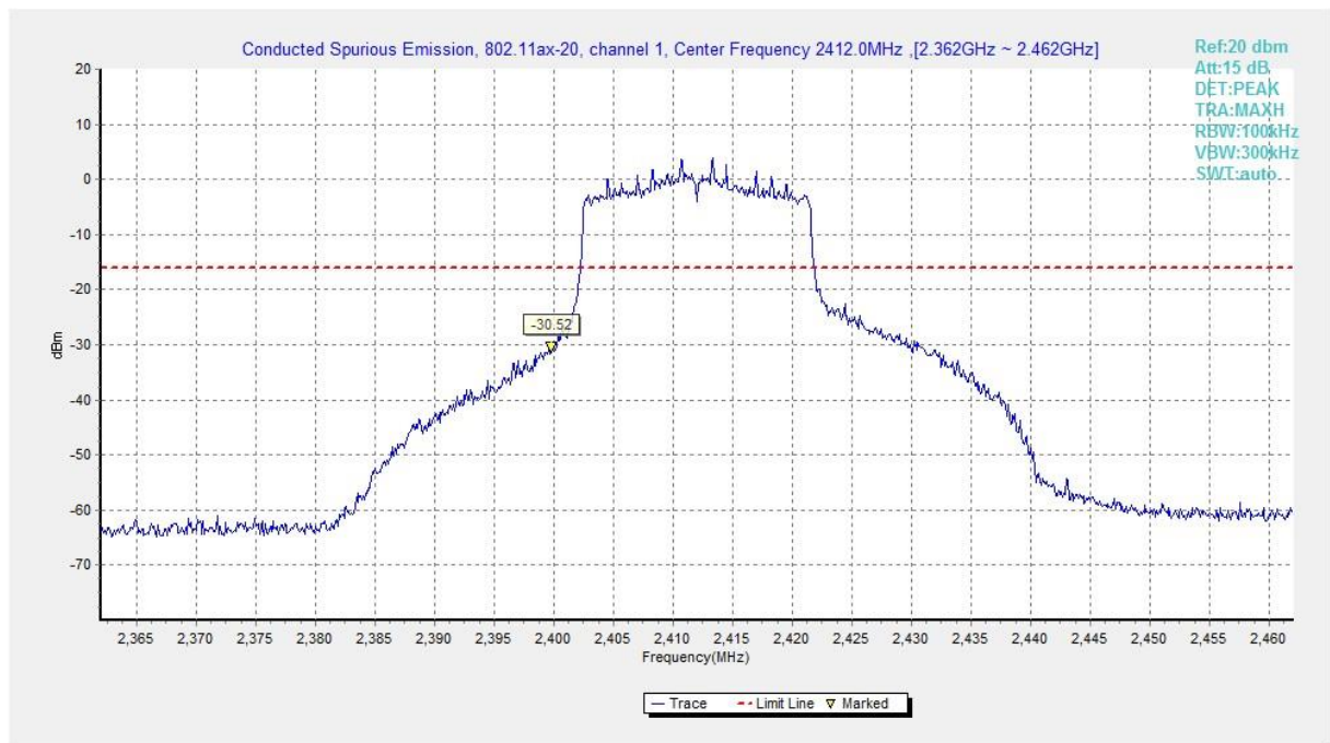
Fig.A.6.1.433 Transmitter Spurious Emission - Conducted (802.11ax-HE20, Ch1, Center Frequency)
