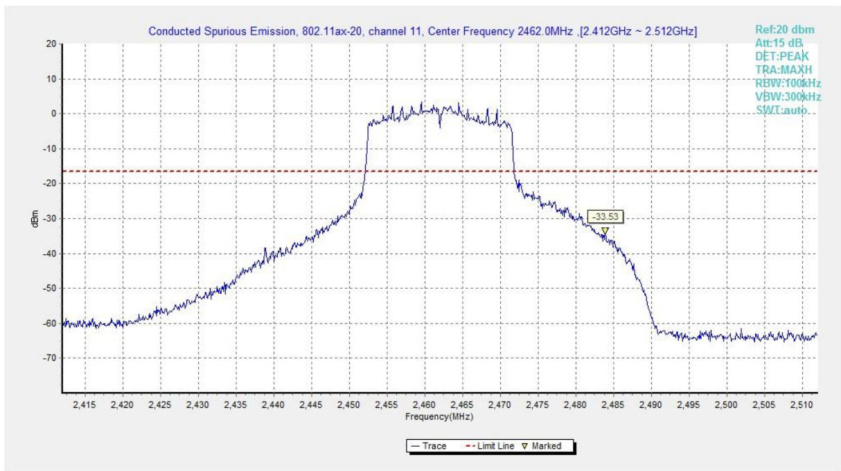
Fig.A.6.1.449 Transmitter Spurious Emission - Conducted (802.11ax-HE20, Ch11, Center Frequency)
