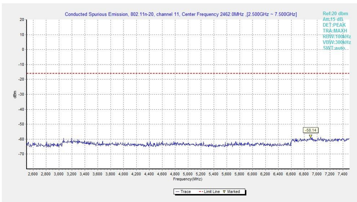
Fig.A.6.1.404 Transmitter Spurious Emission - Conducted (802.11n-HT20, Ch11, 2.5 GHz-7.5 GHz)
