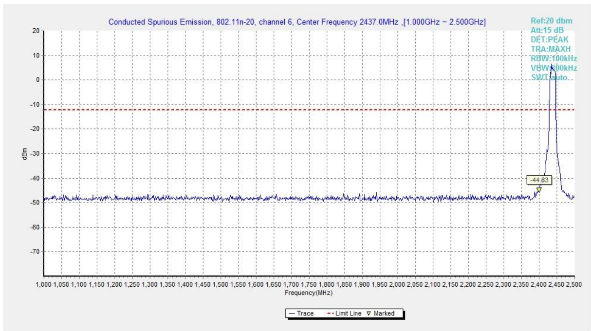
Fig.A.6.1.395 Transmitter Spurious Emission - Conducted (802.11n-HT20, Ch6, 1 GHz-2.5 GHz)
