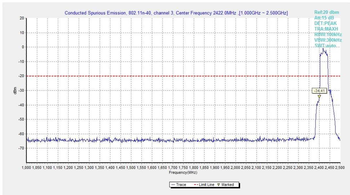
Fig.A.6.1.411 Transmitter Spurious Emission - Conducted (802.11n-HT40, Ch3, 1 GHz-2.5 GHz)
