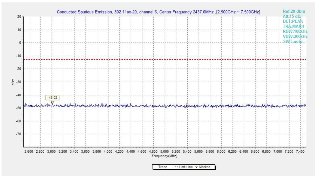
Fig.A.6.1.444 Transmitter Spurious Emission - Conducted (802.11ax-HE20, Ch6, 2.5 GHz-7.5 GHz)
