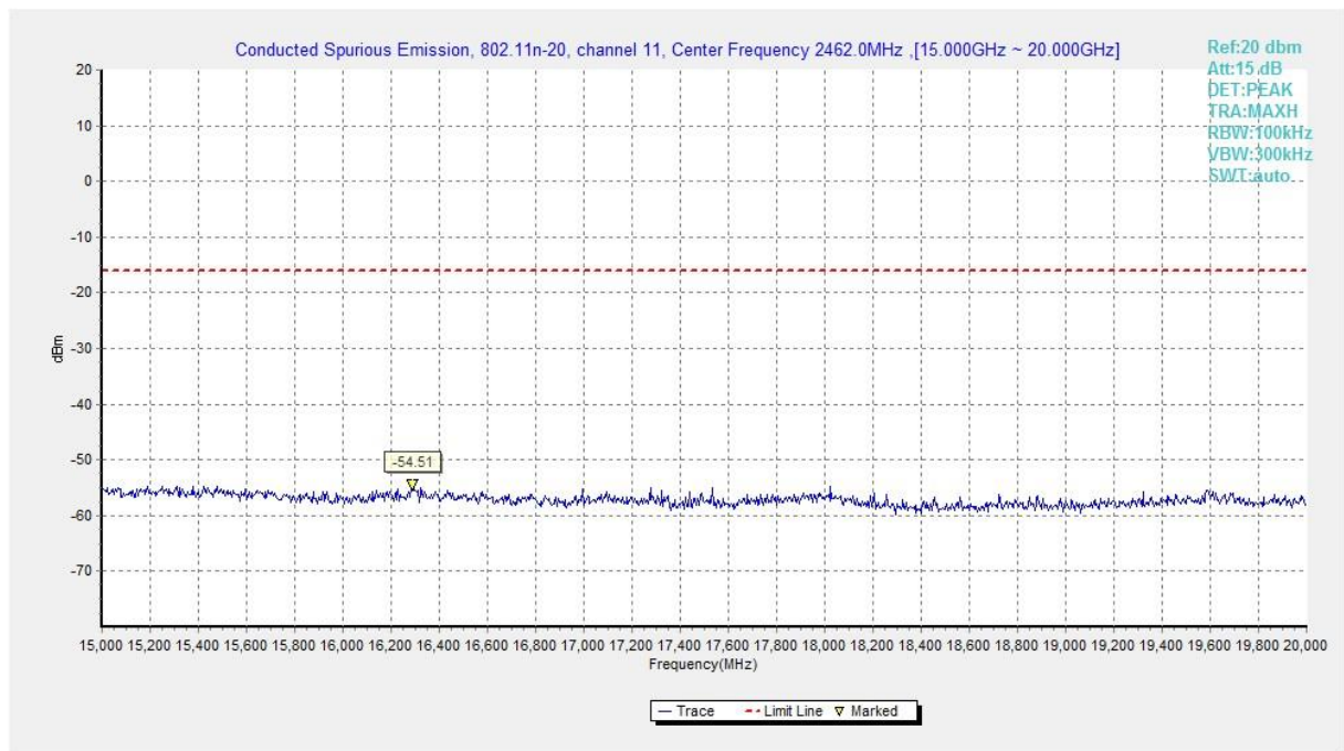
Fig.A.6.1.407 Transmitter Spurious Emission - Conducted (802.11n-HT20, Ch11, 15 GHz-20 GHz)
