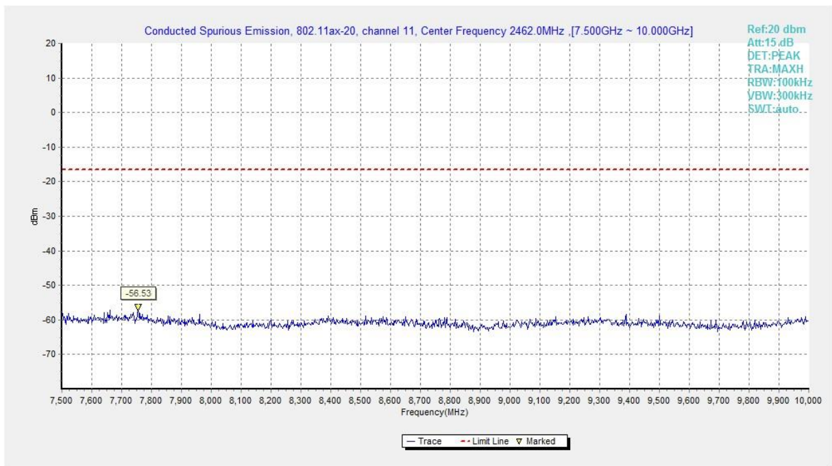
Fig.A.6.1.453 Transmitter Spurious Emission - Conducted (802.11ax-HE20, Ch11, 7.5 GHz-10 GHz)
