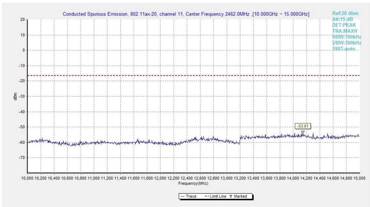
Fig.A.6.1.454 Transmitter Spurious Emission - Conducted (802.11ax-HE20, Ch11, 10 GHz-15 GHz)
