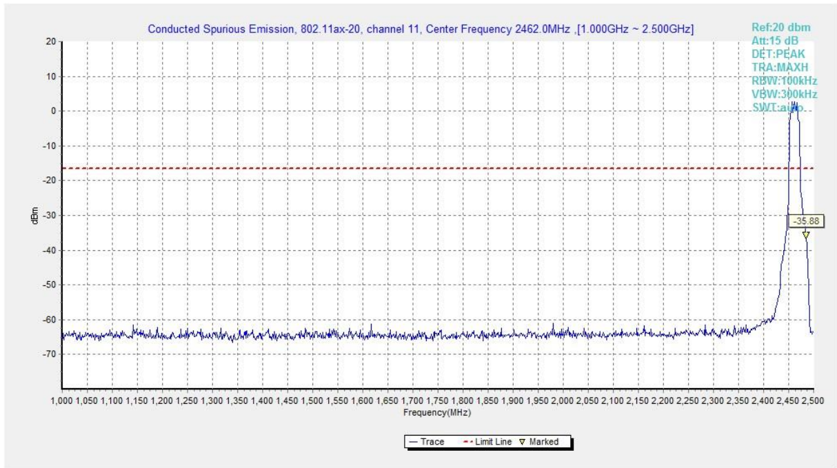
Fig.A.6.1.451 Transmitter Spurious Emission - Conducted (802.11ax-HE20, Ch11, 1 GHz-2.5 GHz)
