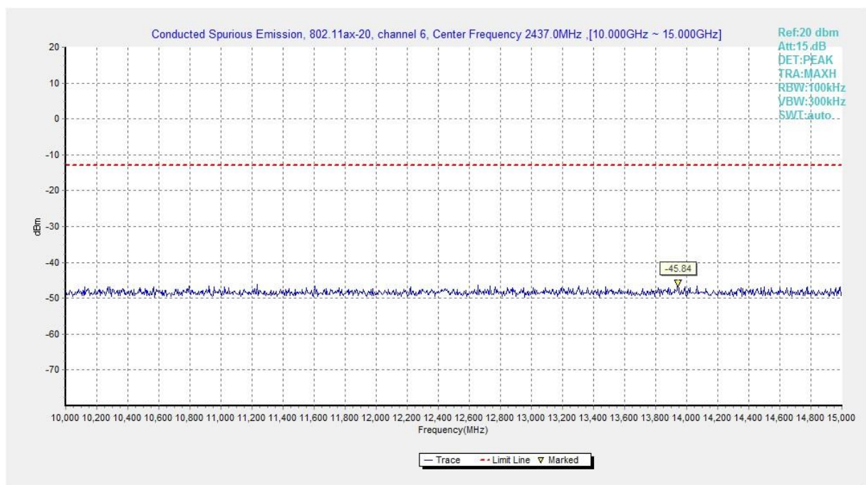
Fig.A.6.1.446 Transmitter Spurious Emission - Conducted (802.11ax-HE20, Ch6, 10 GHz-15 GHz)
