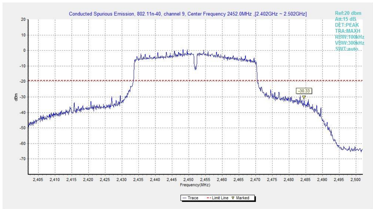
Fig.A.6.1.425 Transmitter Spurious Emission - Conducted (802.11n-HT40, Ch9, Center Frequency)
