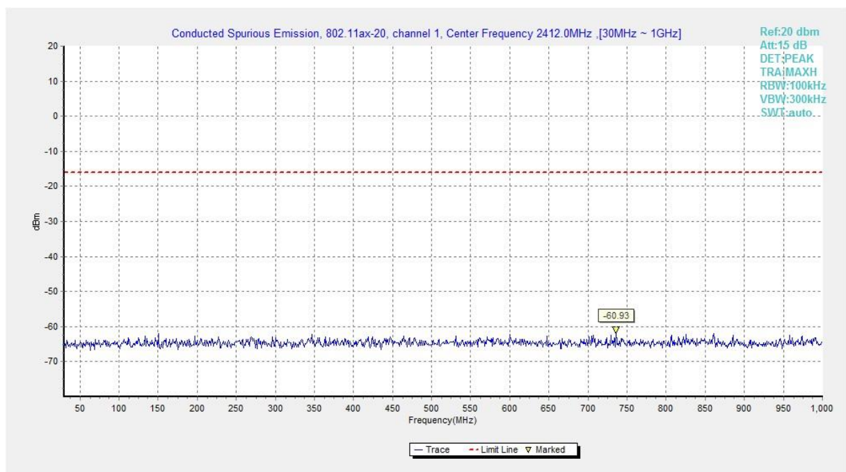
Fig.A.6.1.434 Transmitter Spurious Emission - Conducted (802.11ax-HE20, Ch1, 30 MHz-1 GHz)
