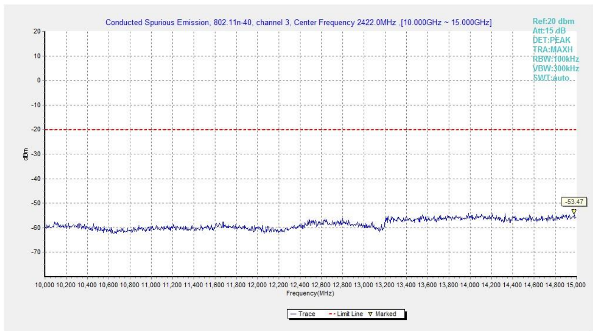
Fig.A.6.1.414 Transmitter Spurious Emission - Conducted (802.11n-HT40, Ch3, 10 GHz-15 GHz)
