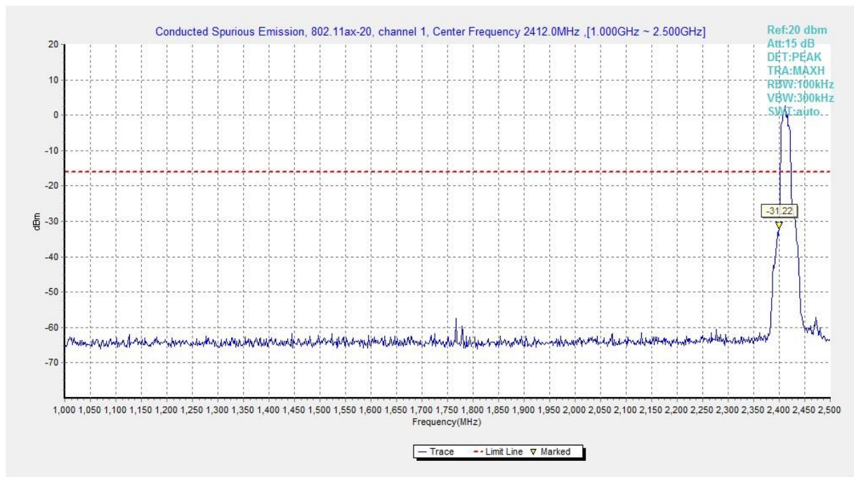
Fig.A.6.1.435 Transmitter Spurious Emission - Conducted (802.11ax-HE20, Ch1, 1 GHz-2.5 GHz)
