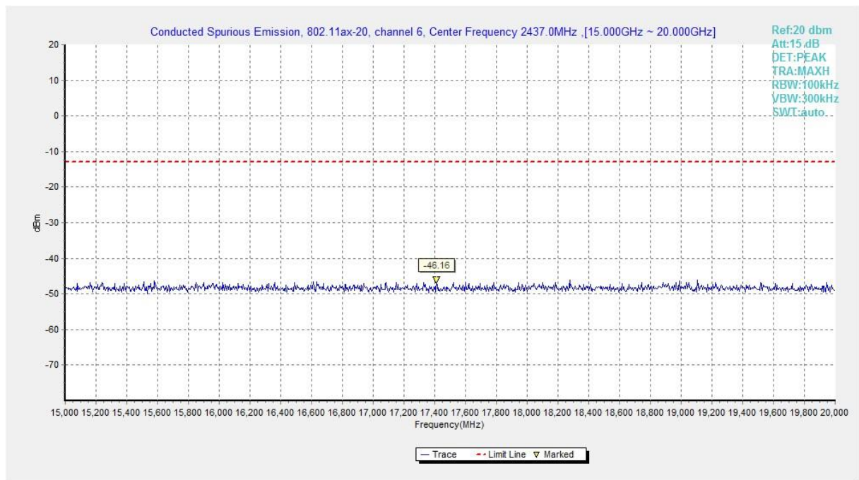
Fig.A.6.1.447 Transmitter Spurious Emission - Conducted (802.11ax-HE20, Ch6, 15 GHz-20 GHz)
