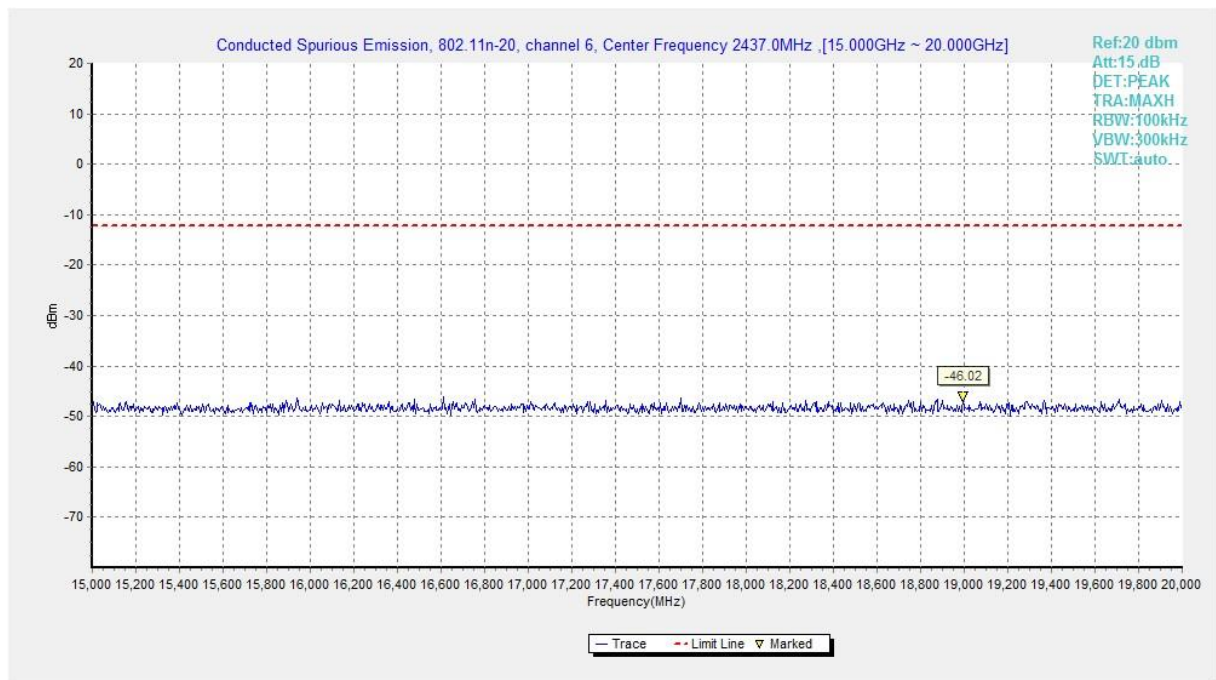
Fig.A.6.1.399 Transmitter Spurious Emission - Conducted (802.11n-HT20, Ch6, 15 GHz-20 GHz)
