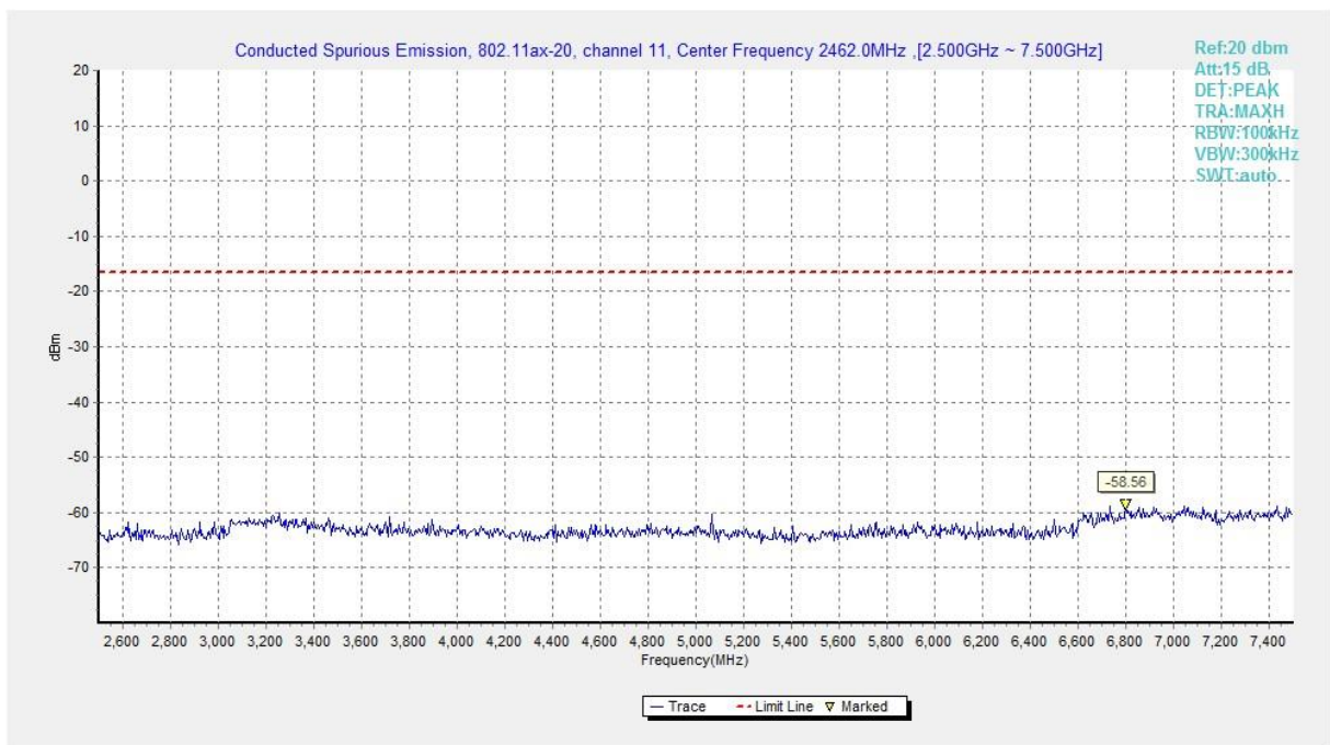
Fig.A.6.1.452 Transmitter Spurious Emission - Conducted (802.11ax-HE20, Ch11, 2.5 GHz-7.5 GHz)
