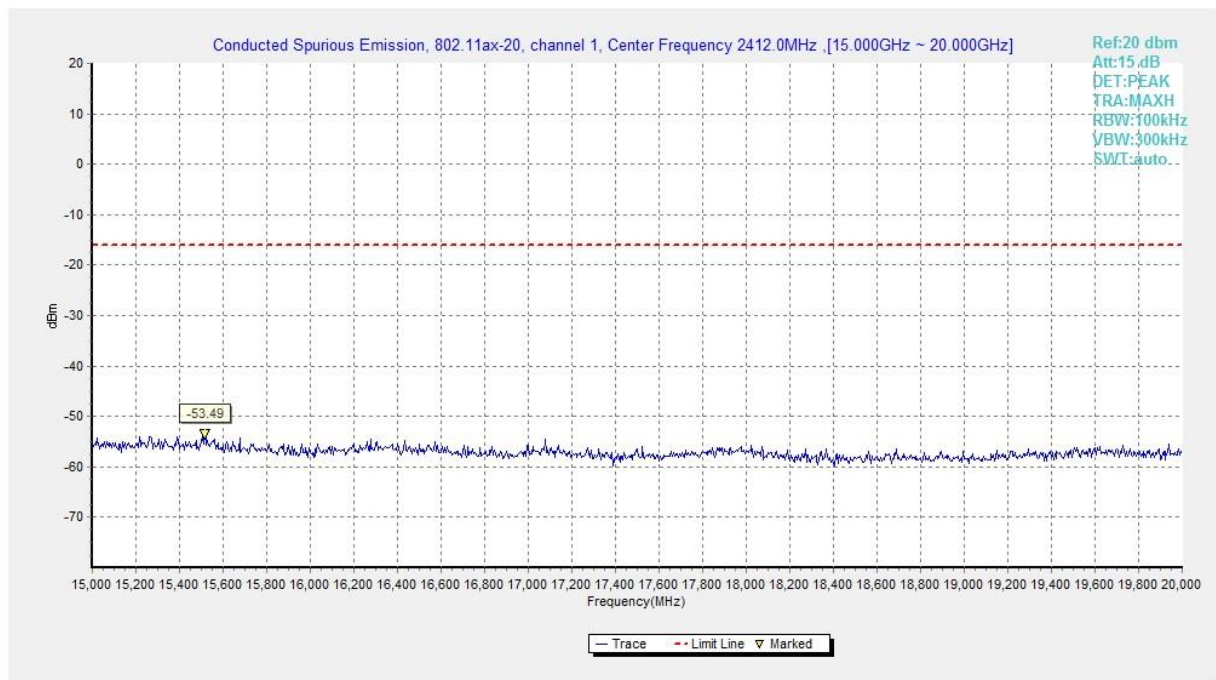
Fig.A.6.1.439 Transmitter Spurious Emission - Conducted (802.11ax-HE20, Ch1, 15 GHz-20 GHz)
