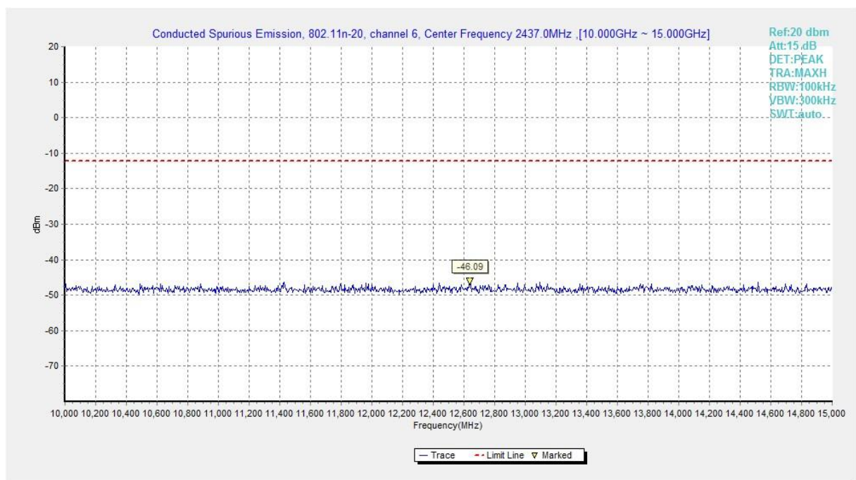
Fig.A.6.1.398 Transmitter Spurious Emission - Conducted (802.11n-HT20, Ch6, 10 GHz-15 GHz)
