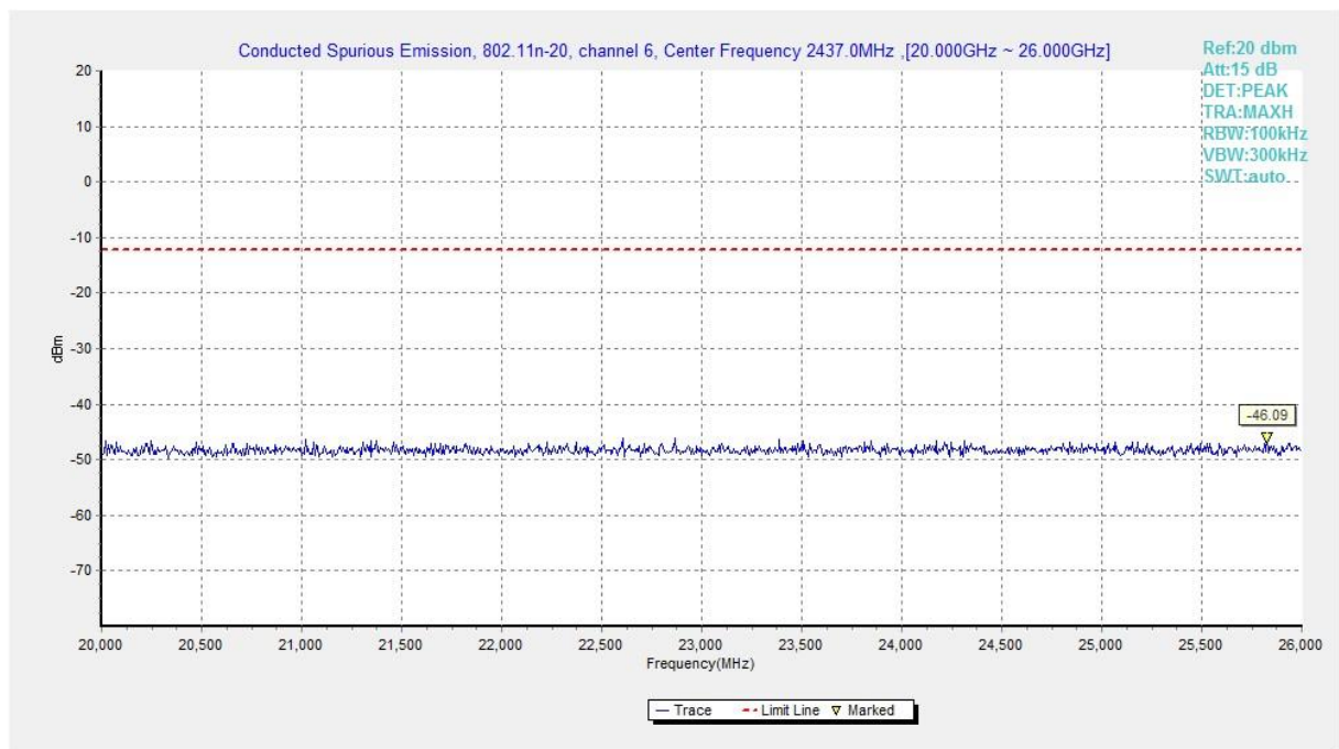
Fig.A.6.1.400 Transmitter Spurious Emission - Conducted (802.11n-HT20, Ch6, 20 GHz-26 GHz)
