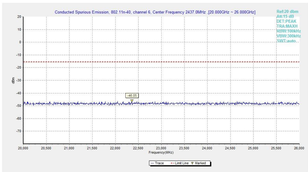
Fig.A.6.1.424 Transmitter Spurious Emission - Conducted (802.11n-HT40, Ch6, 20 GHz-26 GHz)
