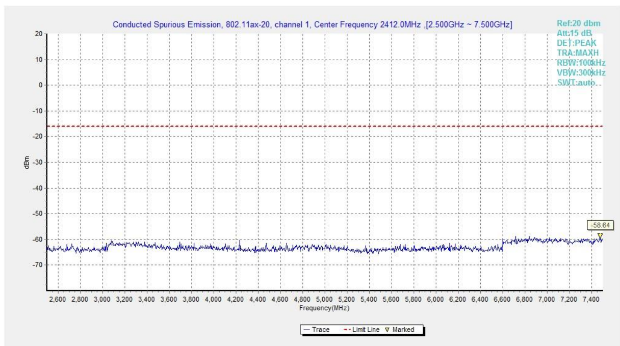
Fig.A.6.1.436 Transmitter Spurious Emission - Conducted (802.11ax-HE20, Ch1, 2.5 GHz-7.5 GHz)
