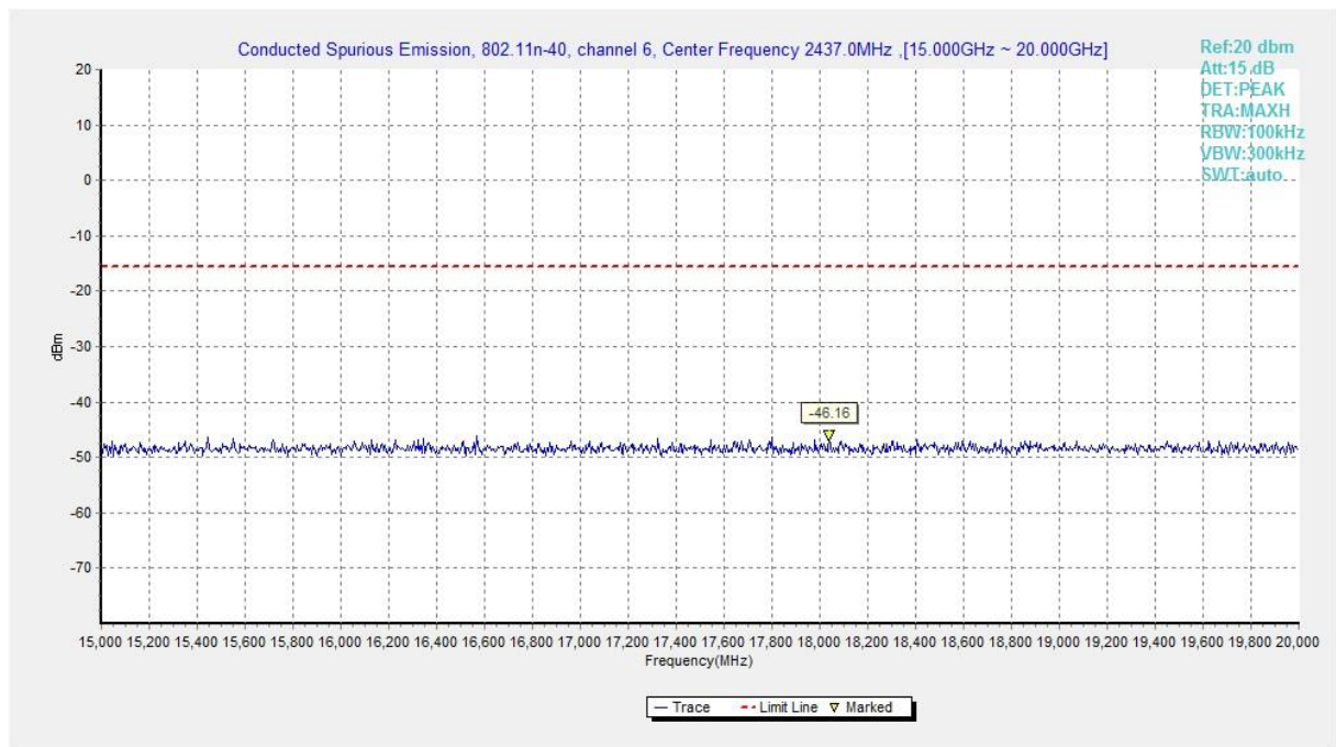
Fig.A.6.1.423 Transmitter Spurious Emission - Conducted (802.11n-HT40, Ch6, 15 GHz-20 GHz)
