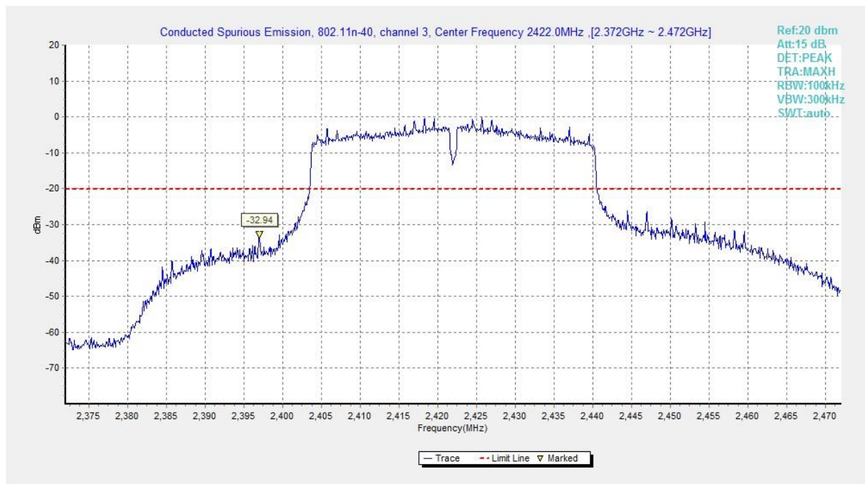
Fig.A.6.1.409 Transmitter Spurious Emission - Conducted (802.11n-HT40, Ch3, Center Frequency)
