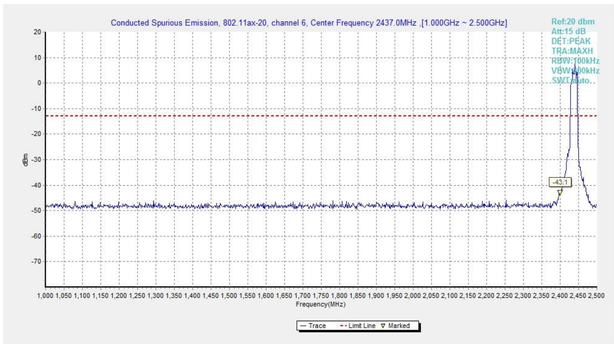
Fig.A.6.1.443 Transmitter Spurious Emission - Conducted (802.11ax-HE20, Ch6, 1 GHz-2.5 GHz)
