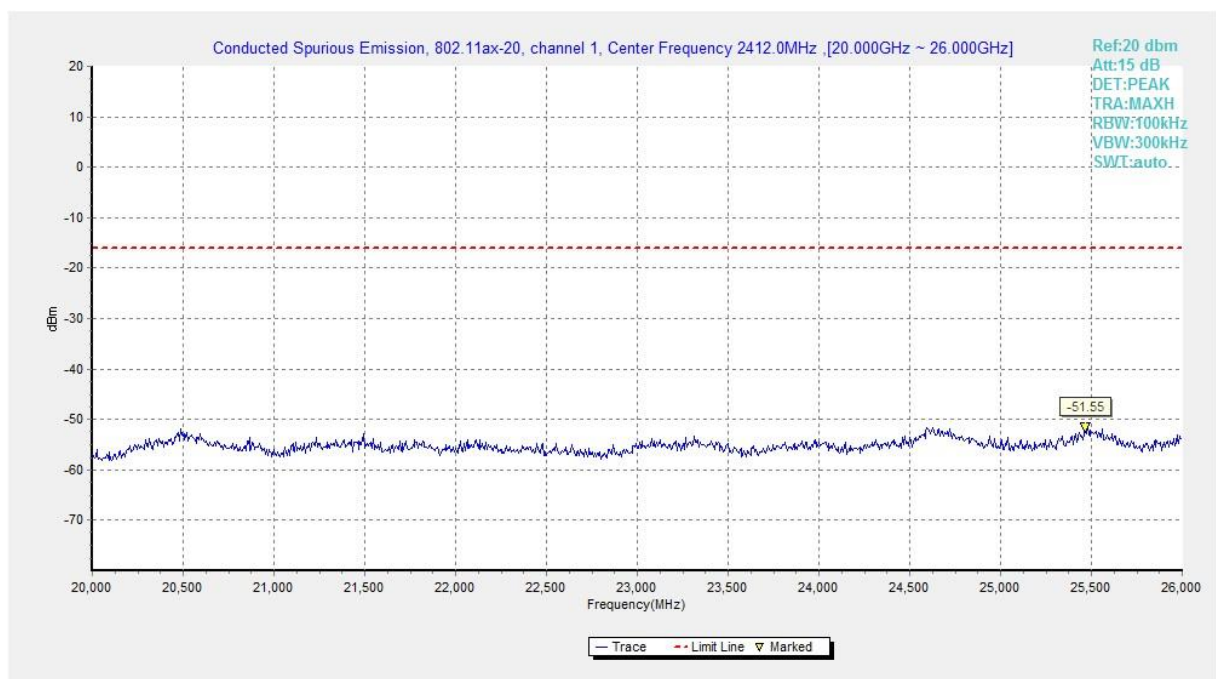
Fig.A.6.1.440 Transmitter Spurious Emission - Conducted (802.11ax-HE20, Ch1, 20 GHz-26 GHz)
