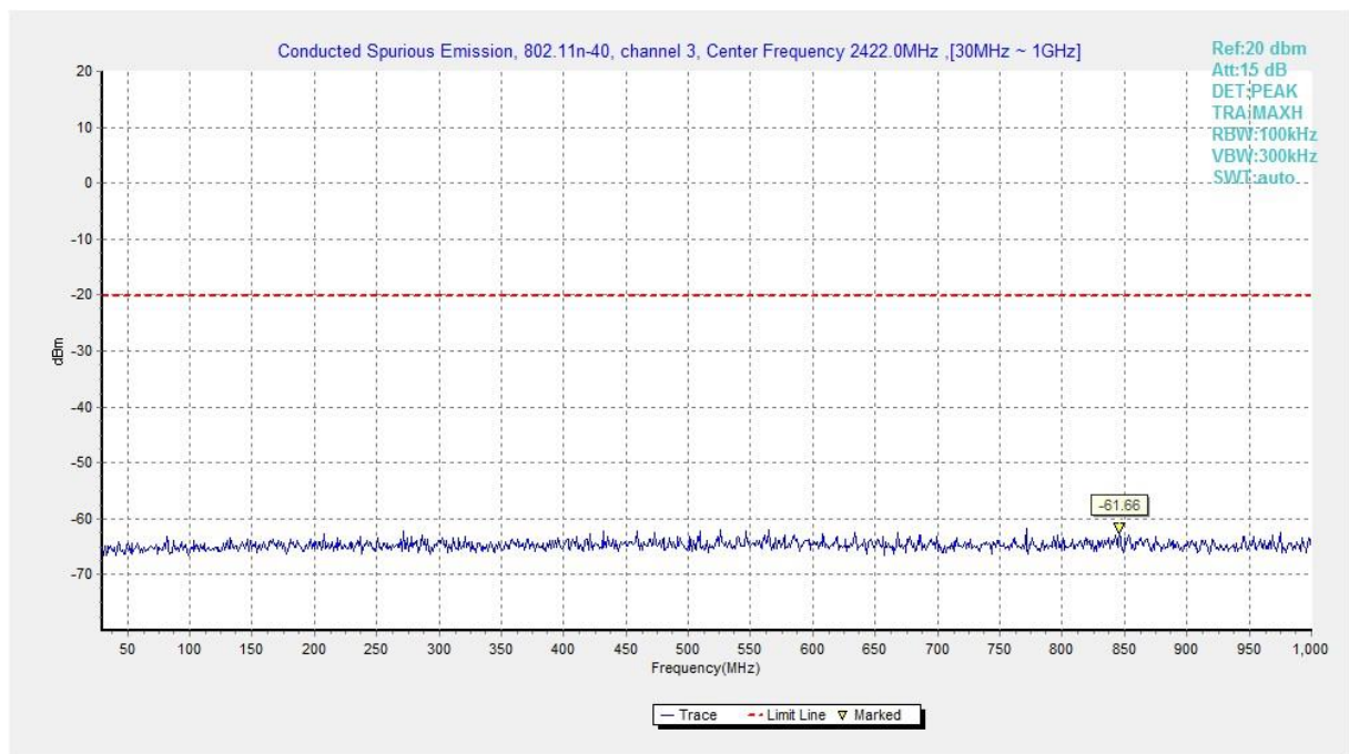
Fig.A.6.1.410 Transmitter Spurious Emission - Conducted (802.11n-HT40, Ch3, 30 MHz-1 GHz)
