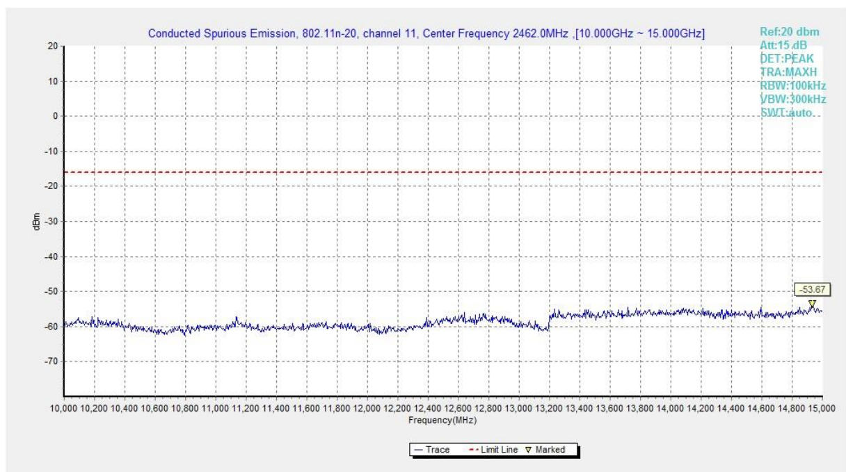
Fig.A.6.1.406 Transmitter Spurious Emission - Conducted (802.11n-HT20, Ch11, 10 GHz-15 GHz)
