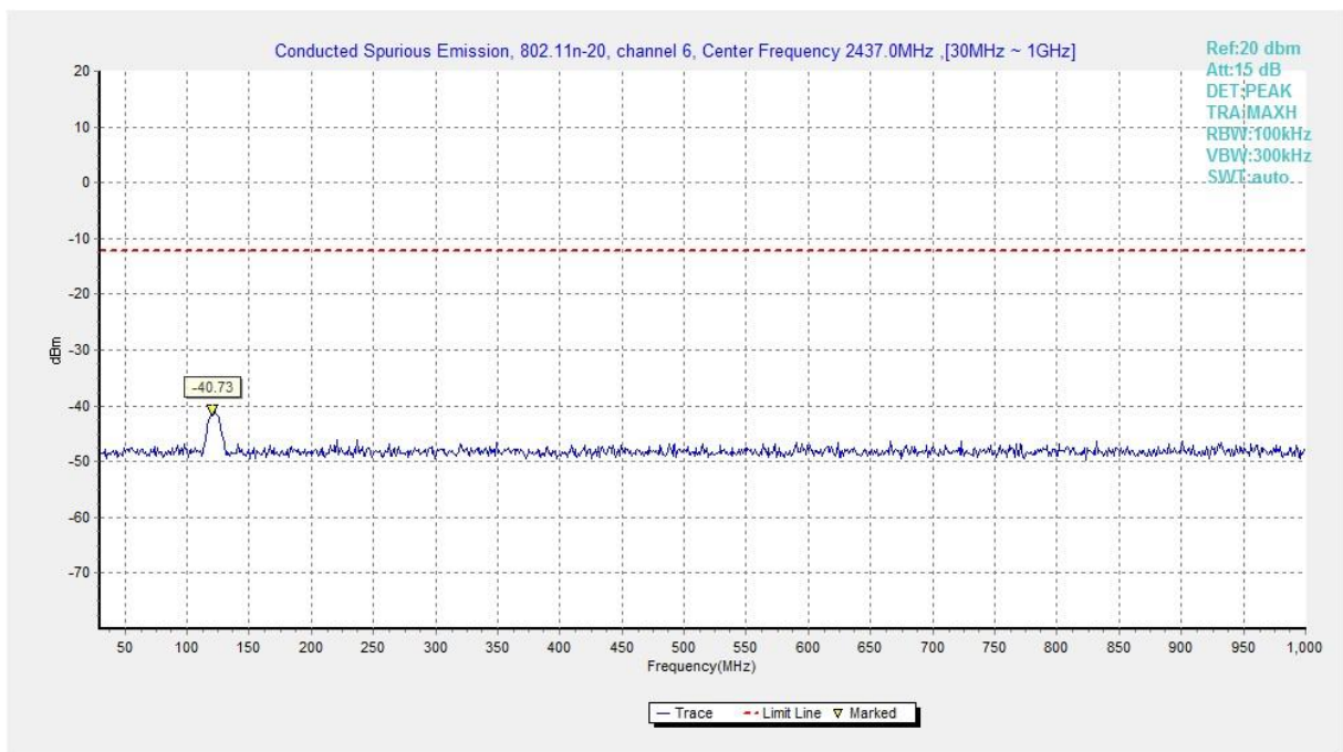
Fig.A.6.1.394 Transmitter Spurious Emission - Conducted (802.11n-HT20, Ch6, 30 MHz-1 GHz)
