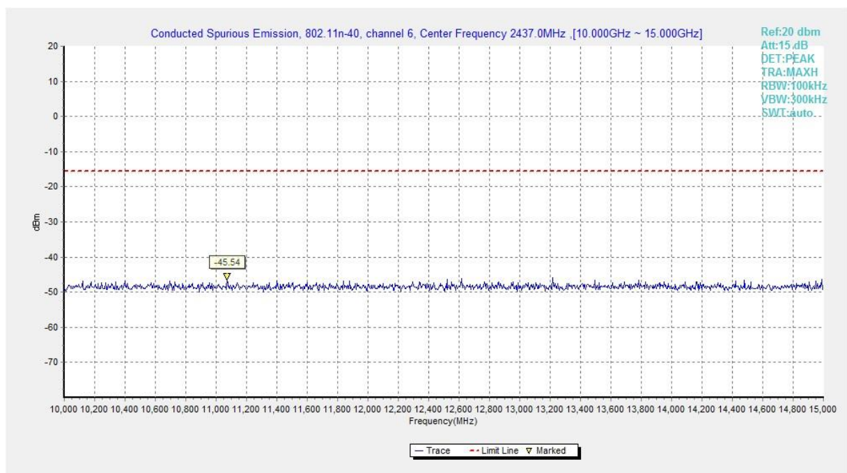
Fig.A.6.1.422 Transmitter Spurious Emission - Conducted (802.11n-HT40, Ch6, 10 GHz-15 GHz)
