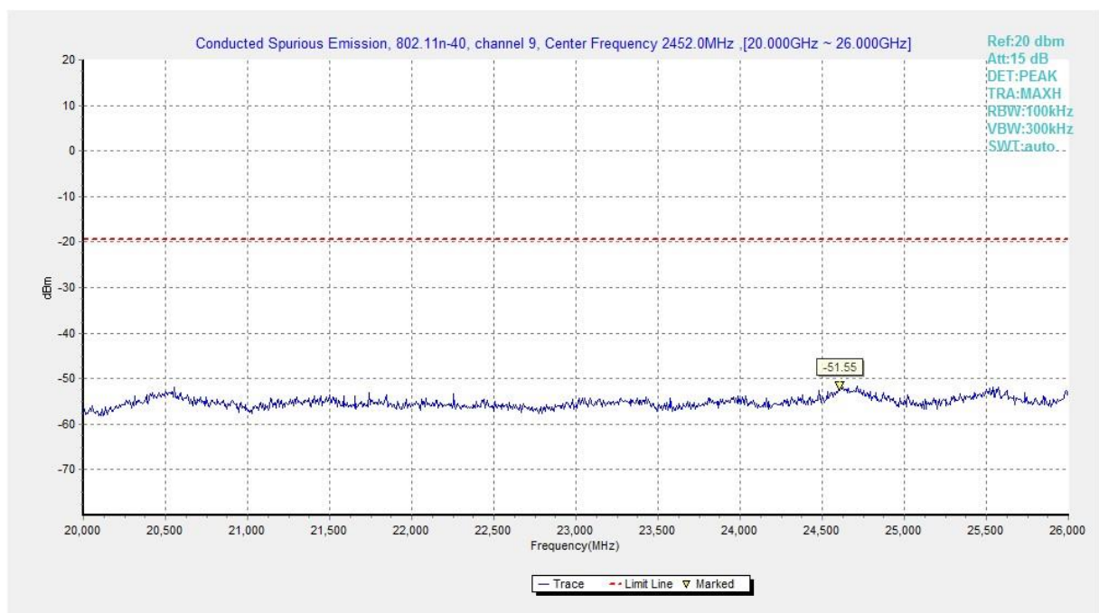
Fig.A.6.1.432 Transmitter Spurious Emission - Conducted (802.11n-HT40, Ch9, 20 GHz-26 GHz)
