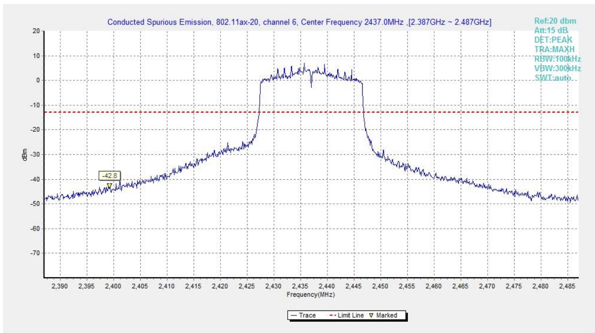
Fig.A.6.1.441 Transmitter Spurious Emission - Conducted (802.11ax-HE20, Ch6, Center Frequency)
