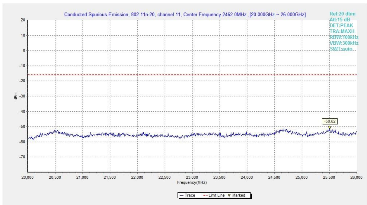
Fig.A.6.1.408 Transmitter Spurious Emission - Conducted (802.11n-HT20, Ch11, 20 GHz-26 GHz)
