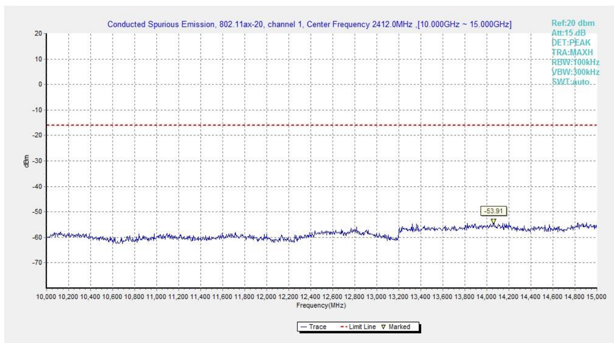
Fig.A.6.1.438 Transmitter Spurious Emission - Conducted (802.11ax-HE20, Ch1, 10 GHz-15 GHz)
