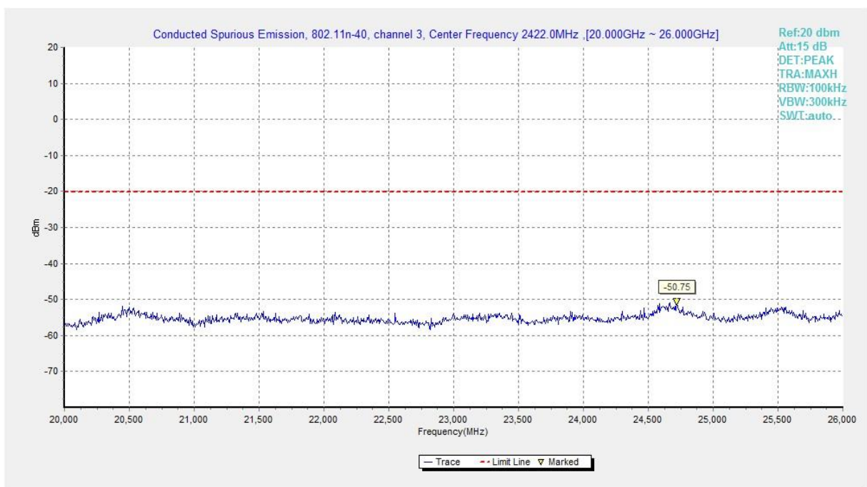
Fig.A.6.1.416 Transmitter Spurious Emission - Conducted (802.11n-HT40, Ch3, 20 GHz-26 GHz)
