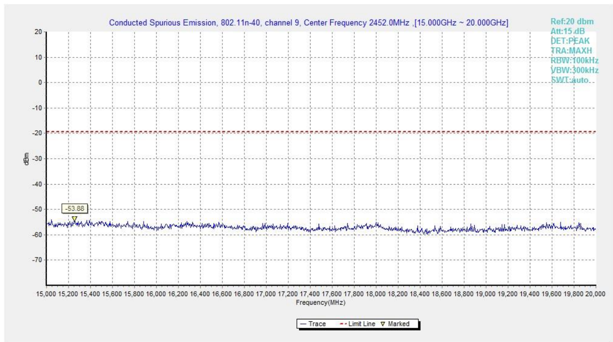
Fig.A.6.1.431 Transmitter Spurious Emission - Conducted (802.11n-HT40, Ch9, 15 GHz-20 GHz)
