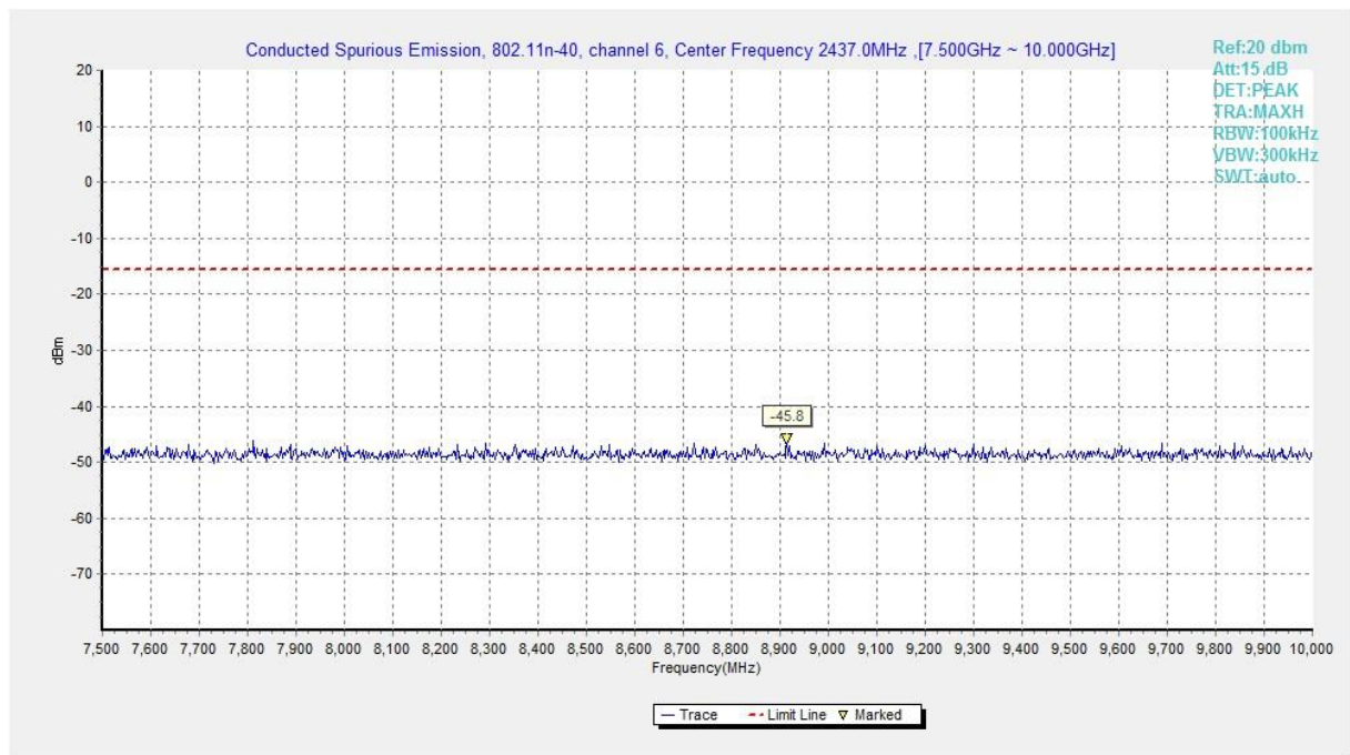
Fig.A.6.1.421 Transmitter Spurious Emission - Conducted (802.11n-HT40, Ch6, 7.5 GHz-10 GHz)
