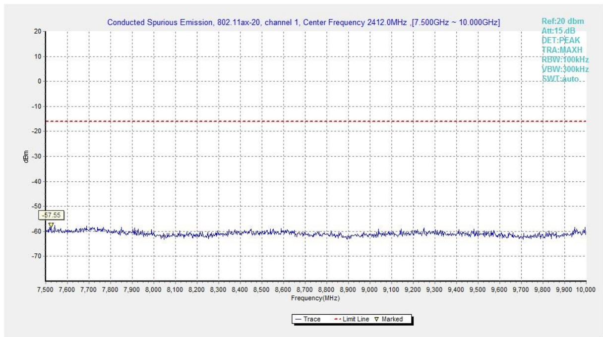
Fig.A.6.1.437 Transmitter Spurious Emission - Conducted (802.11ax-HE20, Ch1, 7.5 GHz-10 GHz)
