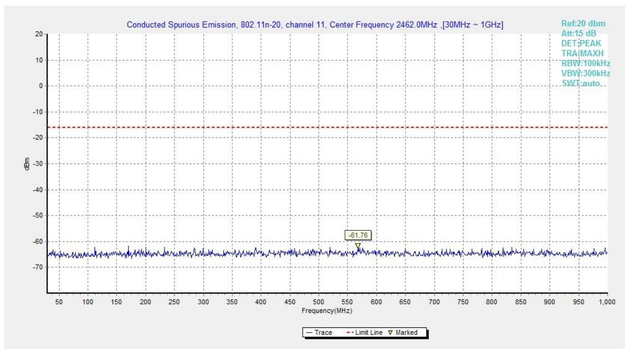
Fig.A.6.1.402 Transmitter Spurious Emission - Conducted (802.11n-HT20, Ch11, 30 MHz-1 GHz)
