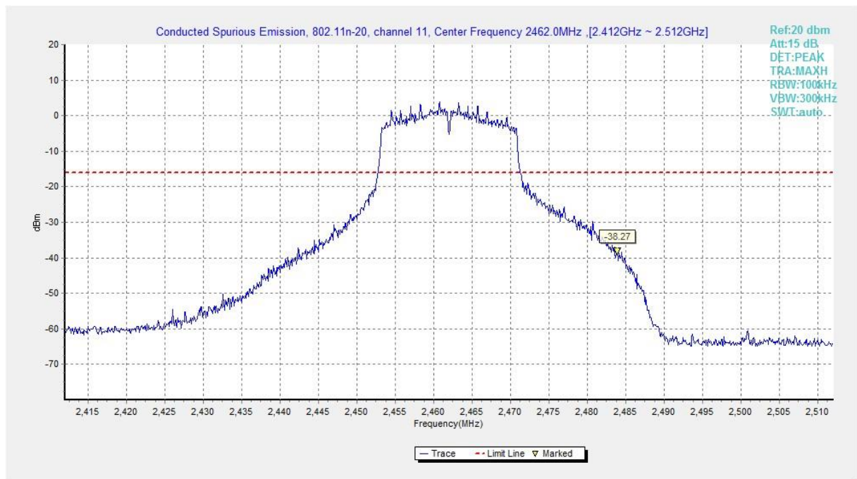
Fig.A.6.1.401 Transmitter Spurious Emission - Conducted (802.11n-HT20, Ch11, Center Frequency)
