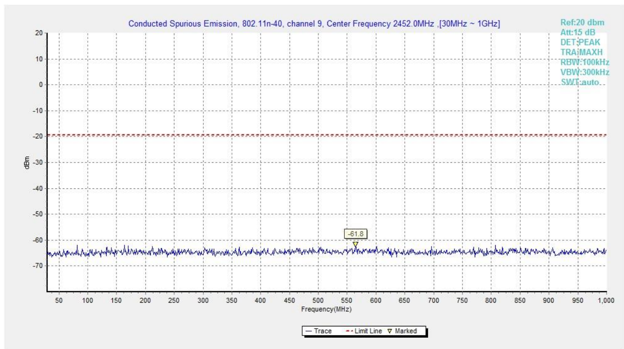
Fig.A.6.1.426 Transmitter Spurious Emission - Conducted (802.11n-HT40, Ch9, 30 MHz-1 GHz)
