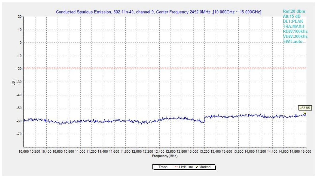
Fig.A.6.1.430 Transmitter Spurious Emission - Conducted (802.11n-HT40, Ch9, 10 GHz-15 GHz)
