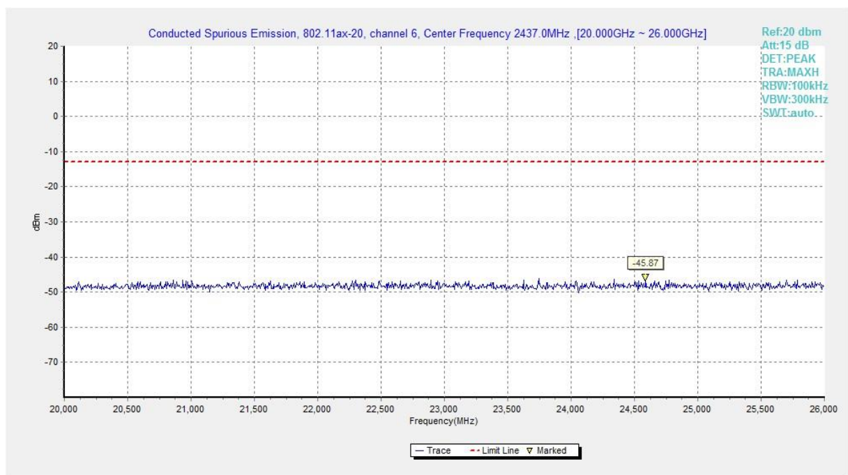
Fig.A.6.1.448 Transmitter Spurious Emission - Conducted (802.11ax-HE20, Ch6, 20 GHz-26 GHz)
