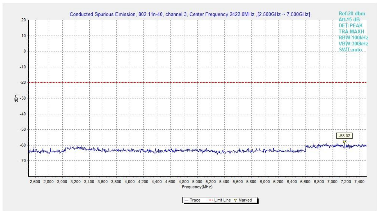
Fig.A.6.1.412 Transmitter Spurious Emission - Conducted (802.11n-HT40, Ch3, 2.5 GHz-7.5 GHz)
