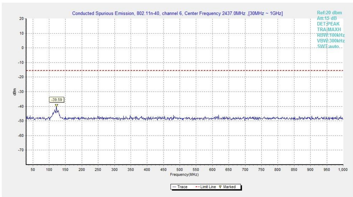
Fig.A.6.1.418 Transmitter Spurious Emission - Conducted (802.11n-HT40, Ch6, 30 MHz-1 GHz)
