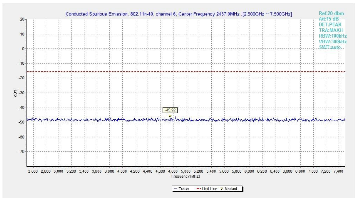
Fig.A.6.1.420 Transmitter Spurious Emission - Conducted (802.11n-HT40, Ch6, 2.5 GHz-7.5 GHz)
