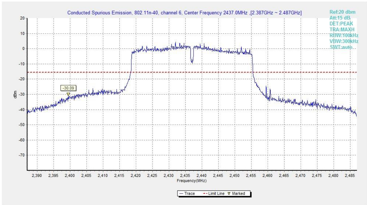
Fig.A.6.1.417 Transmitter Spurious Emission - Conducted (802.11n-HT40, Ch6, Center Frequency)
