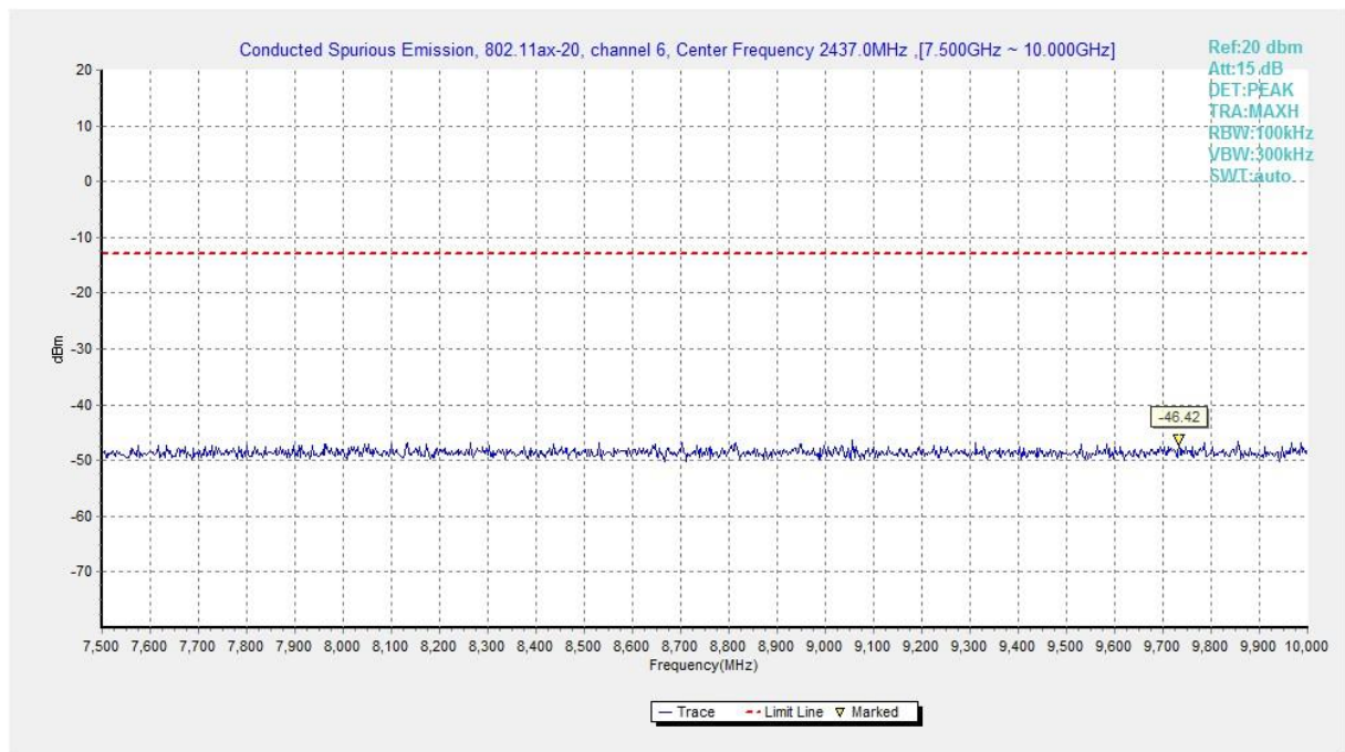
Fig.A.6.1.445 Transmitter Spurious Emission - Conducted (802.11ax-HE20, Ch6, 7.5 GHz-10 GHz)
