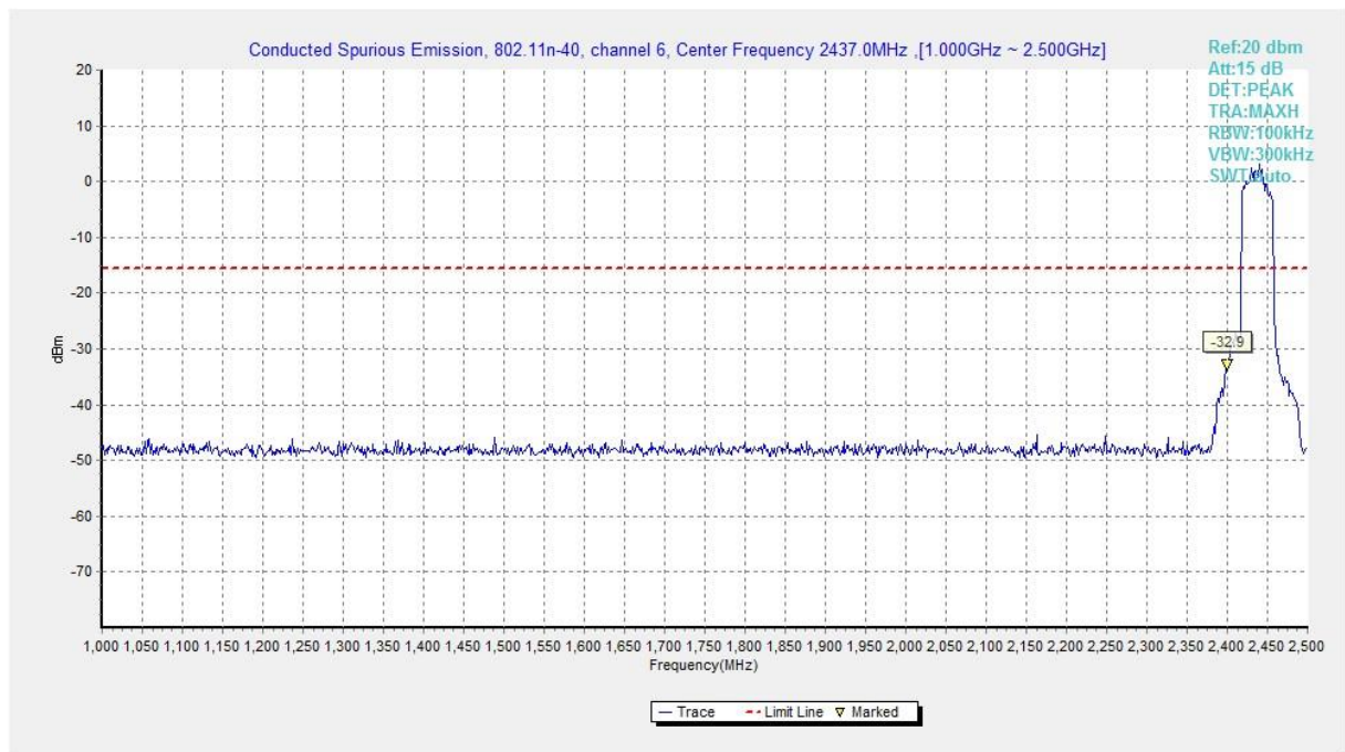
Fig.A.6.1.419 Transmitter Spurious Emission - Conducted (802.11n-HT40, Ch6, 1 GHz-2.5 GHz)
