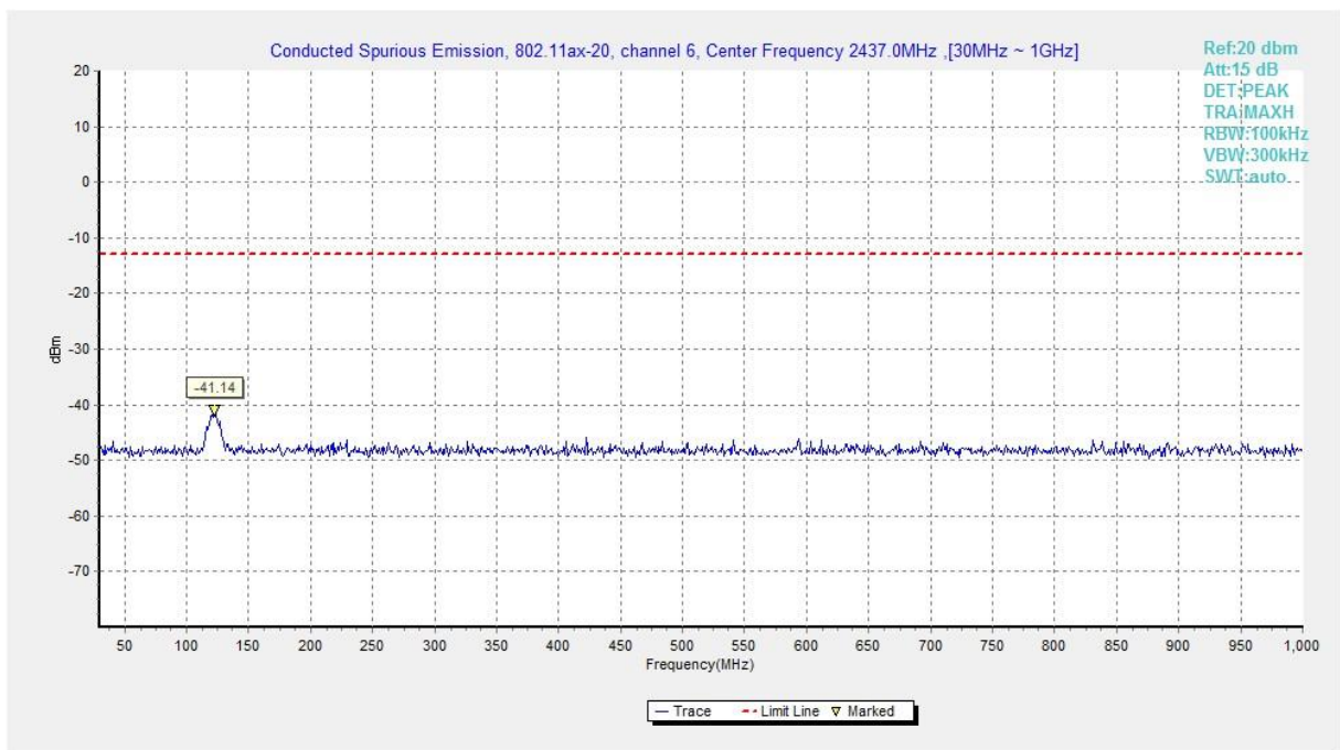
Fig.A.6.1.442 Transmitter Spurious Emission - Conducted (802.11ax-HE20, Ch6, 30 MHz-1 GHz)
