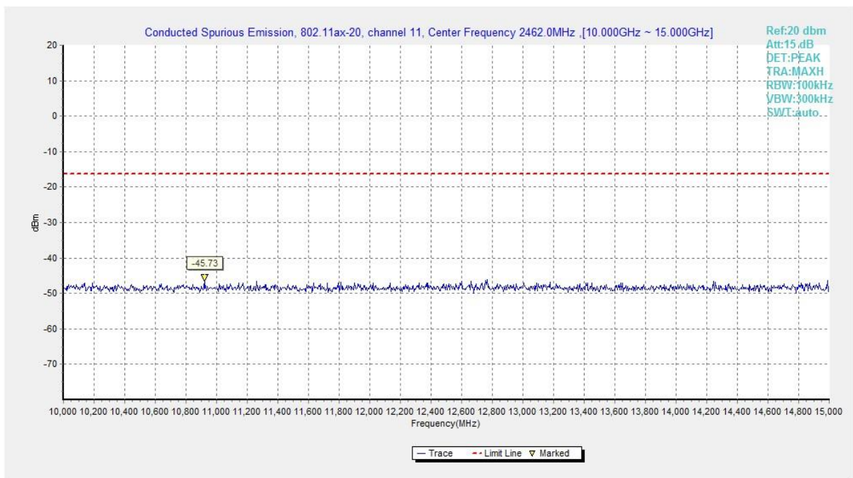
Fig.A.6.1.502 Transmitter Spurious Emission - Conducted (802.11ax-HE20-RU52-right, Ch11, 10 GHz-15 GHz)
