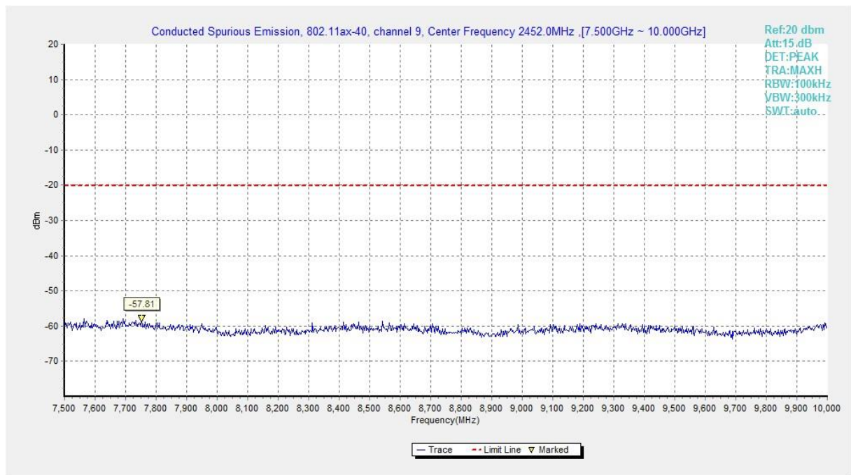
Fig.A.6.1.477 Transmitter Spurious Emission - Conducted (802.11ax-HE40, Ch9, 7.5 GHz-10 GHz)
