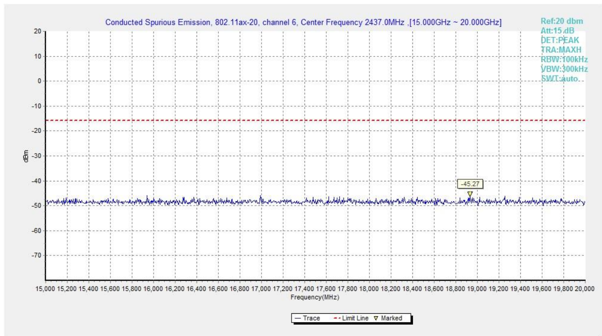
Fig.A.6.1.495 Transmitter Spurious Emission - Conducted (802.11ax-HE20-RU52-right, Ch6, 15 GHz-20 GHz)
