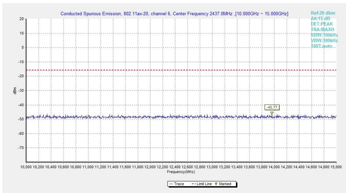
Fig.A.6.1.494 Transmitter Spurious Emission – Conducted (802.11ax-HE20-RU52-right, Ch6, 10 GHz-15 GHz)
