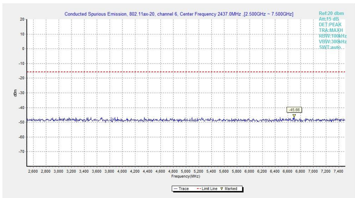
Fig.A.6.1.492 Transmitter Spurious Emission - Conducted (802.11ax-HE20-RU52-right, Ch6, 2.5 GHz-7.5 GHz)
