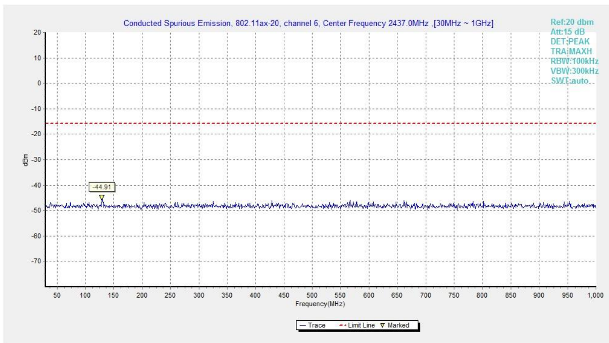
Fig.A.6.1.490 Transmitter Spurious Emission - Conducted (802.11ax-HE20-RU52-right, Ch6, 30 MHz-1 GHz)
