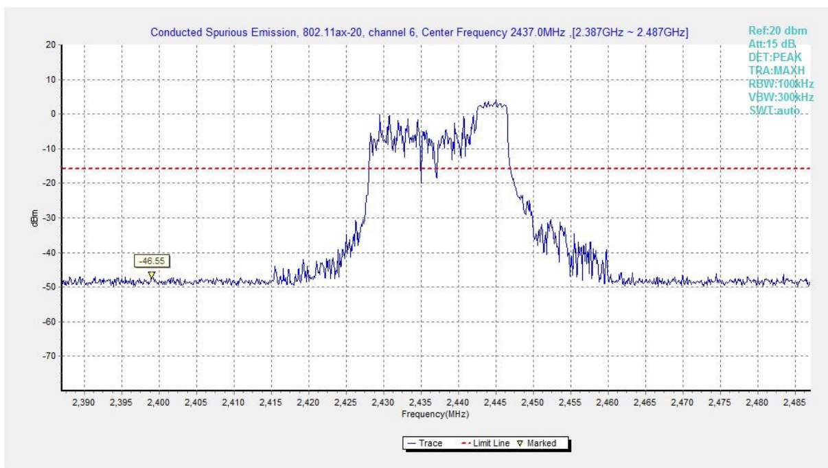
Fig.A.6.1.489 Transmitter Spurious Emission - Conducted (802.11ax-HE20-RU52-right, Ch6, Center Frequency)
