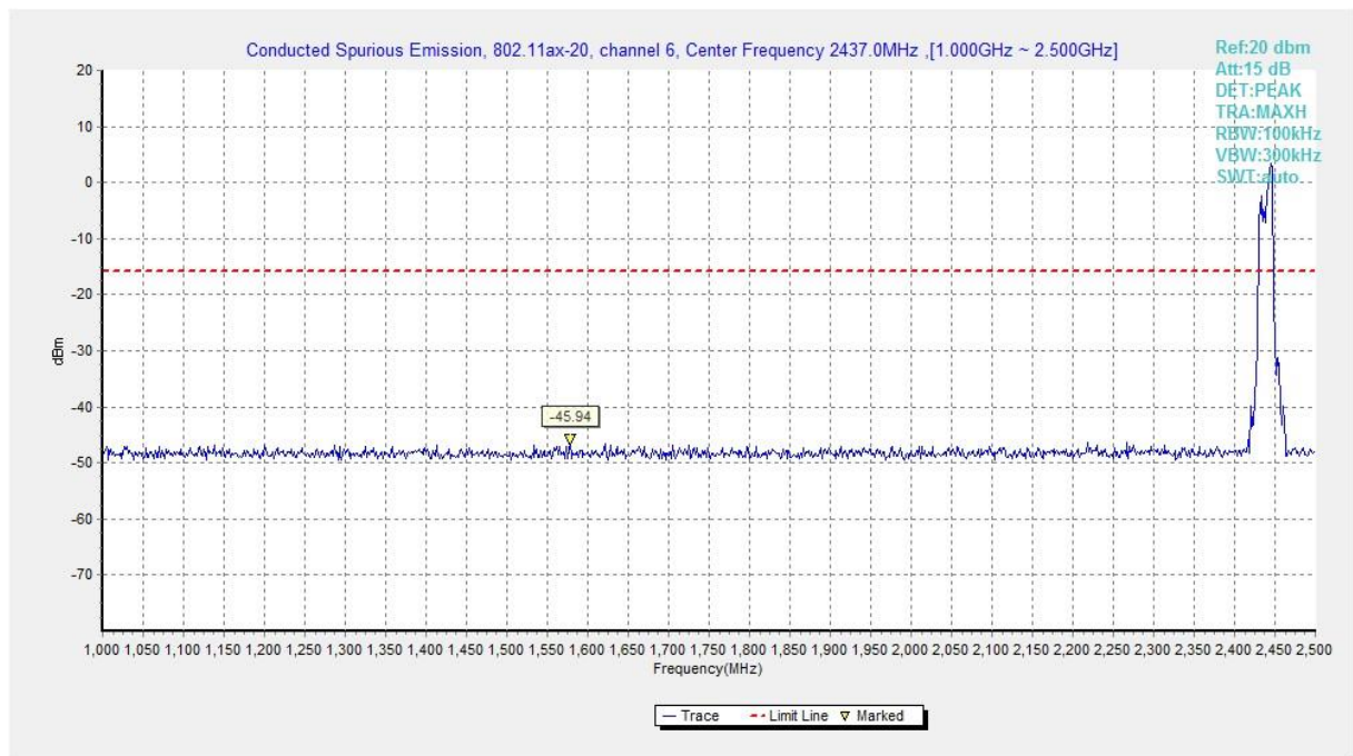
Fig.A.6.1.491 Transmitter Spurious Emission - Conducted (802.11ax-HE20-RU52-right, Ch6, 1 GHz-2.5 GHz)
