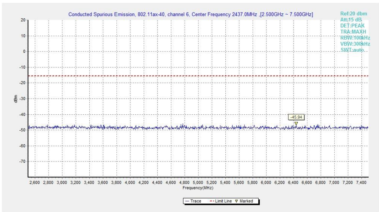
Fig.A.6.1.468 Transmitter Spurious Emission - Conducted (802.11ax-HE40, Ch6, 2.5 GHz-7.5 GHz)
