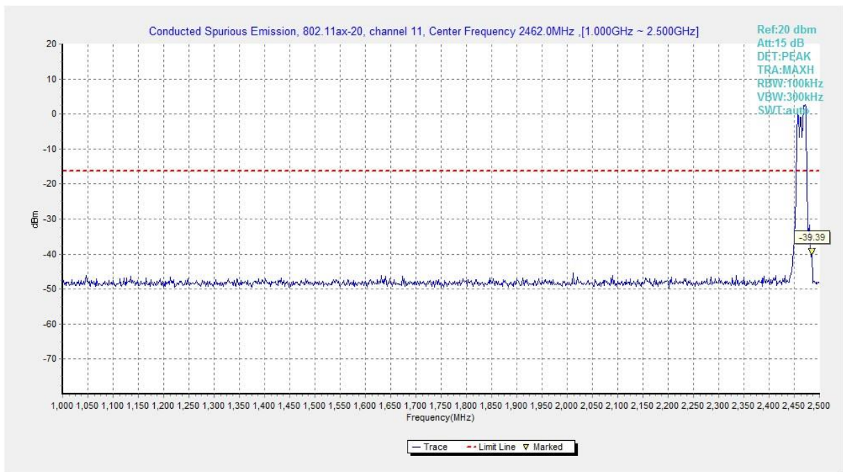
Fig.A.6.1.499 Transmitter Spurious Emission - Conducted (802.11ax-HE20-RU52-right, Ch11, 1 GHz-2.5 GHz)
