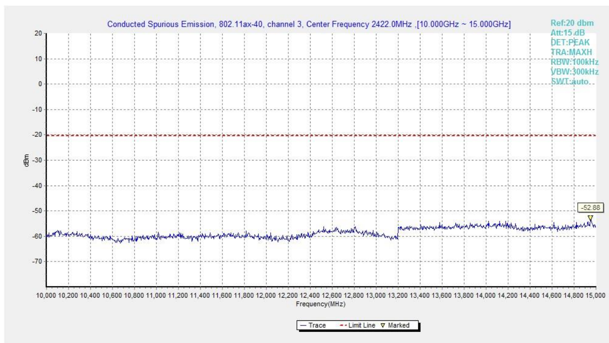
Fig.A.6.1.462 Transmitter Spurious Emission - Conducted (802.11ax-HE40, Ch3, 10 GHz-15 GHz)
