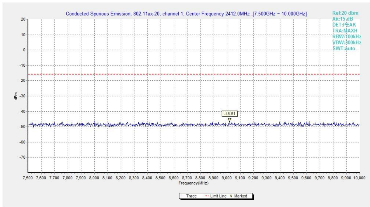
Fig.A.6.1.485 Transmitter Spurious Emission - Conducted (802.11ax-HE20-RU52-right, Ch1, 7.5 GHz-10 GHz)
