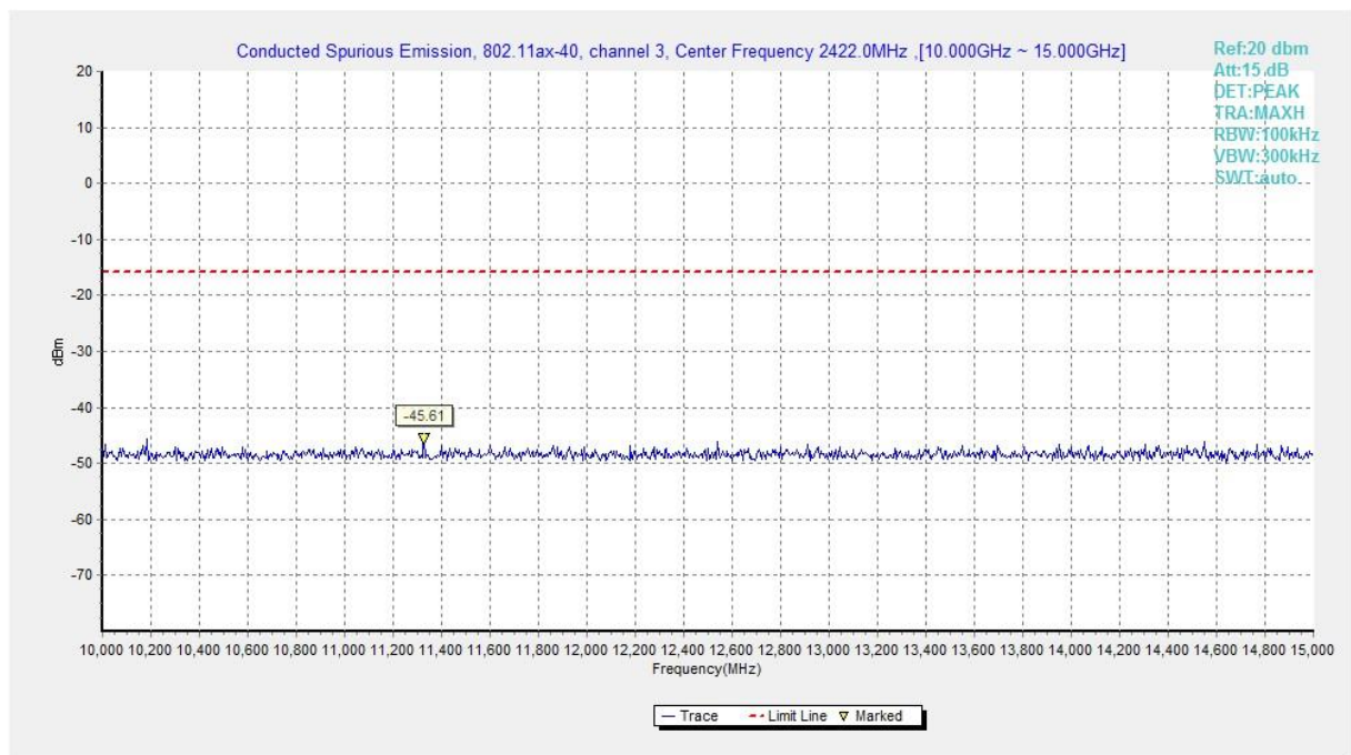
Fig.A.6.1.510 Transmitter Spurious Emission – Conducted (802.11ax-HE40-RU52-left, Ch3, 10 GHz-15 GHz)
