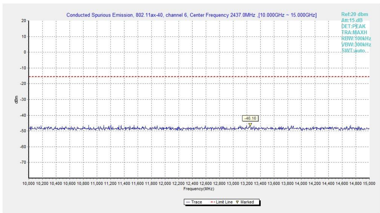
Fig.A.6.1.470 Transmitter Spurious Emission - Conducted (802.11ax-HE40, Ch6, 10 GHz-15 GHz)
