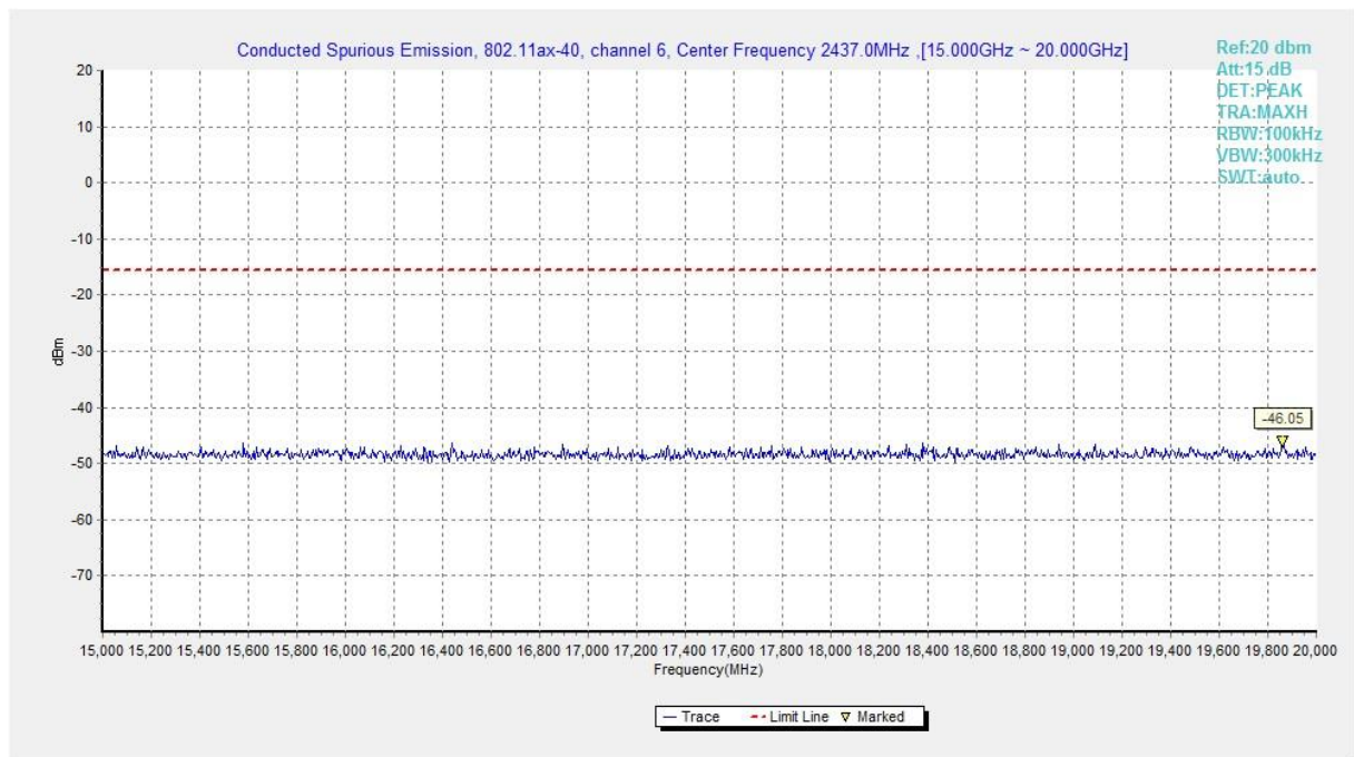
Fig.A.6.1.471 Transmitter Spurious Emission - Conducted (802.11ax-HE40, Ch6, 15 GHz-20 GHz)
