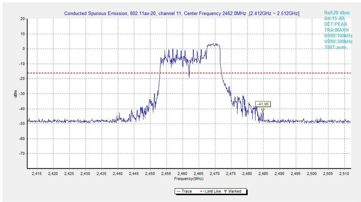
Fig.A.6.1.497 Transmitter Spurious Emission - Conducted (802.11ax-HE20-RU52-right, Ch11, Center Frequency)
