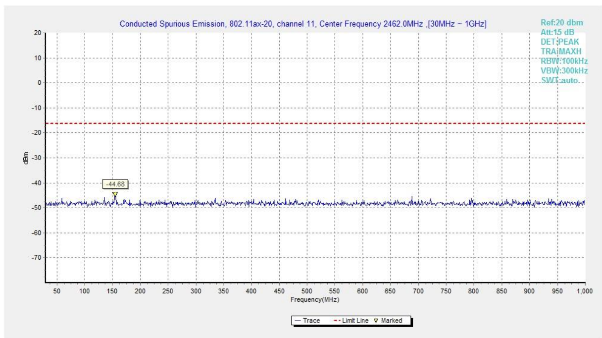
Fig.A.6.1.498 Transmitter Spurious Emission - Conducted (802.11ax-HE20-RU52-right, Ch11, 30 MHz-1 GHz)
