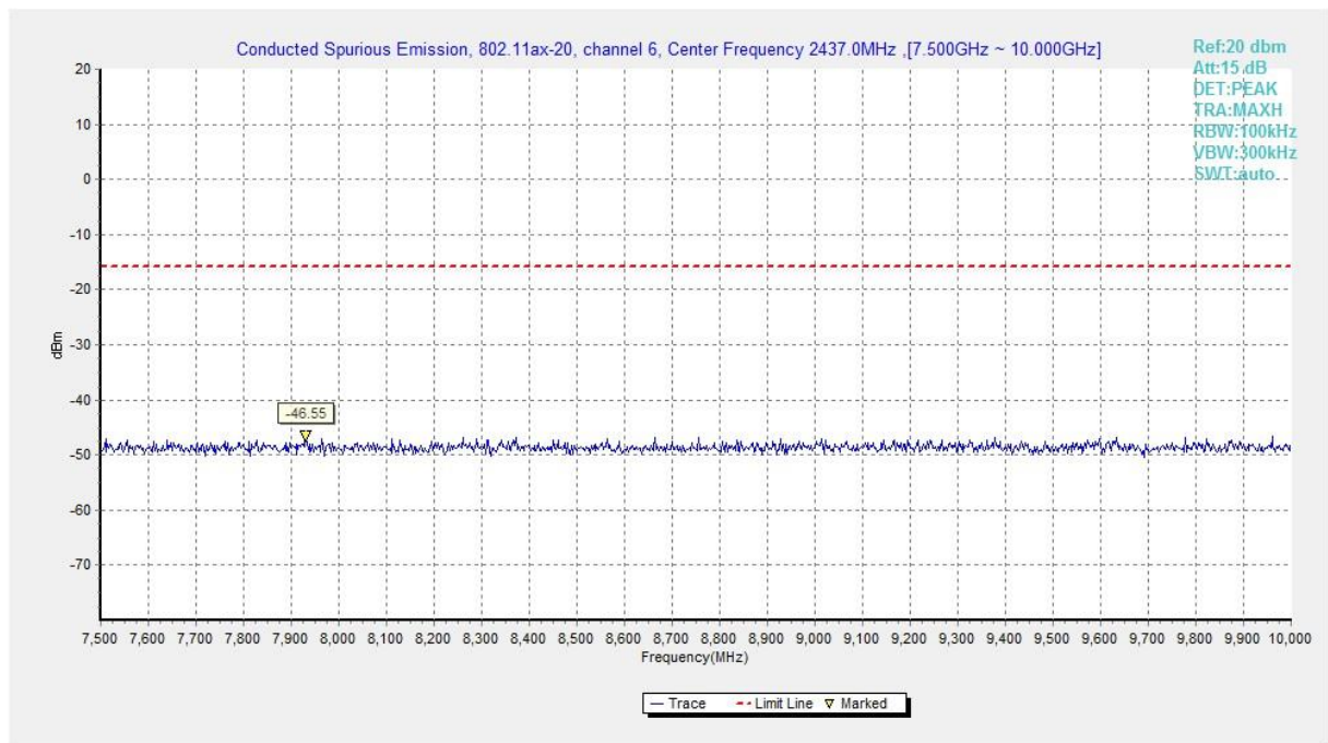
Fig.A.6.1.493 Transmitter Spurious Emission - Conducted (802.11ax-HE20-RU52-right, Ch6, 7.5 GHz-10 GHz)
