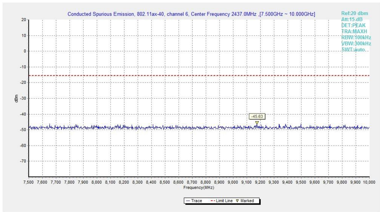
Fig.A.6.1.469 Transmitter Spurious Emission - Conducted (802.11ax-HE40, Ch6, 7.5 GHz-10 GHz)
