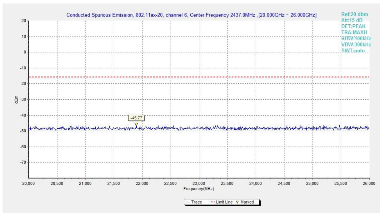
Fig.A.6.1.496 Transmitter Spurious Emission - Conducted (802.11ax-HE20-RU52-right, Ch6, 20 GHz-26 GHz)
