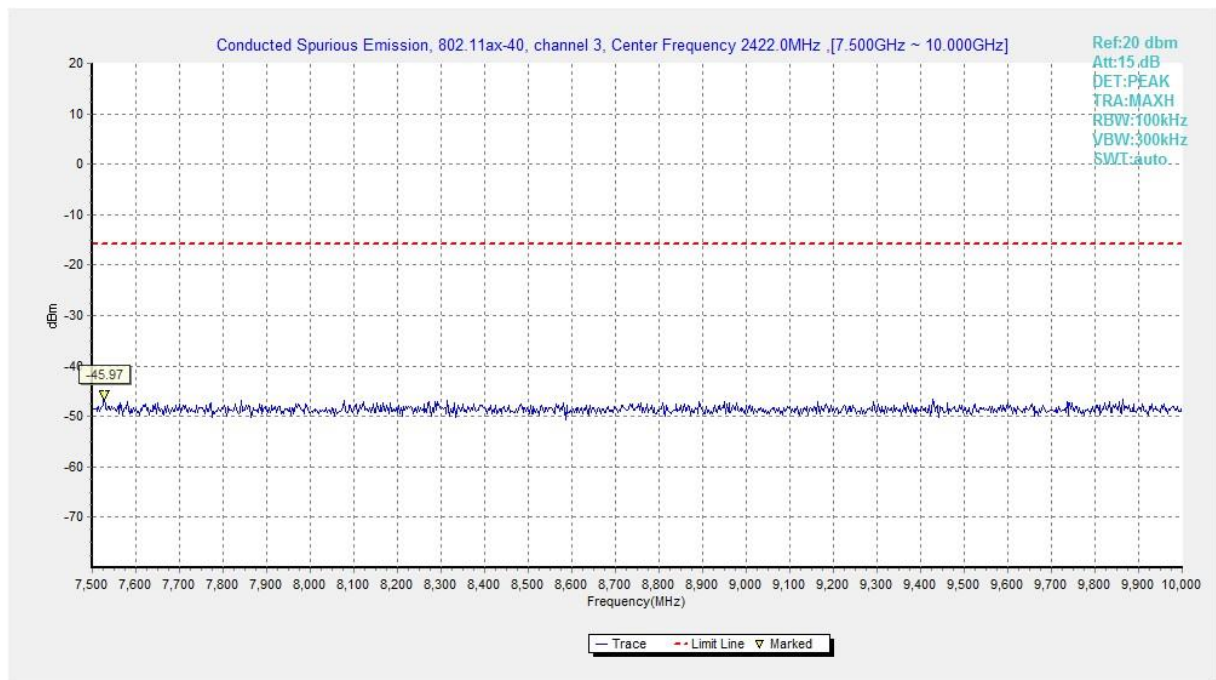
Fig.A.6.1.509 Transmitter Spurious Emission - Conducted (802.11ax-HE40-RU52-left, Ch3, 7.5 GHz-10 GHz)
