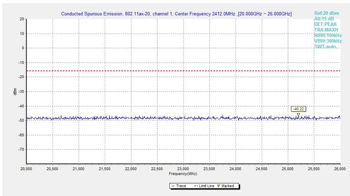
Fig.A.6.1.488 Transmitter Spurious Emission - Conducted (802.11ax-HE20-RU52-right, Ch1, 20 GHz-26 GHz)
