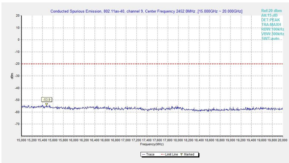
Fig.A.6.1.479 Transmitter Spurious Emission - Conducted (802.11ax-HE40, Ch9, 15 GHz-20 GHz)
