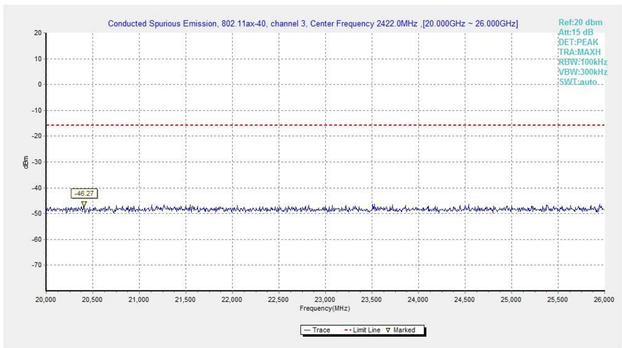
Fig.A.6.1.512 Transmitter Spurious Emission - Conducted (802.11ax-HE40-RU52-left, Ch3, 20 GHz-26 GHz)
