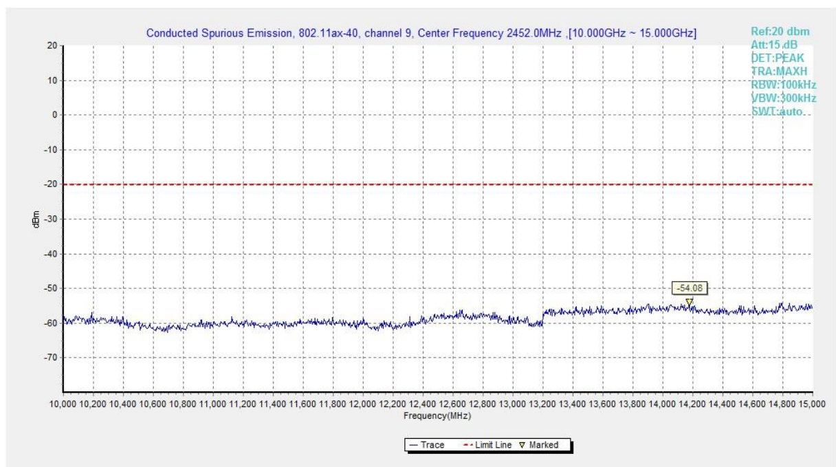
Fig.A.6.1.478 Transmitter Spurious Emission - Conducted (802.11ax-HE40, Ch9, 10 GHz-15 GHz)
