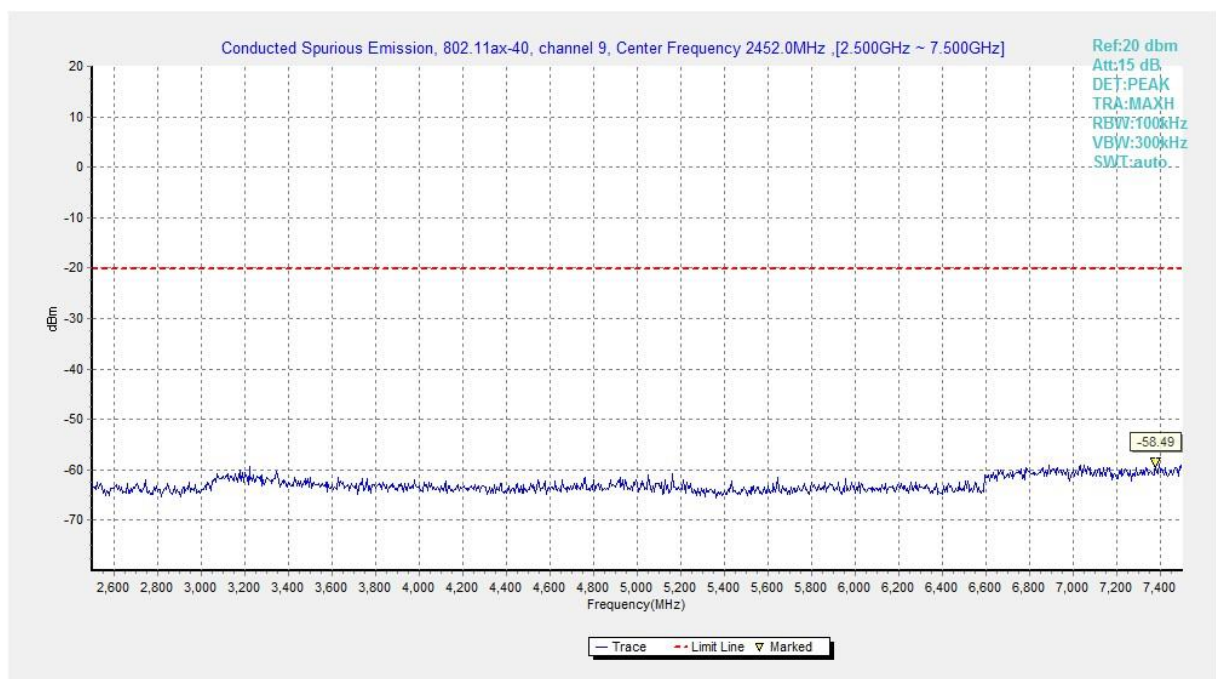
Fig.A.6.1.476 Transmitter Spurious Emission - Conducted (802.11ax-HE40, Ch9, 2.5 GHz-7.5 GHz)
