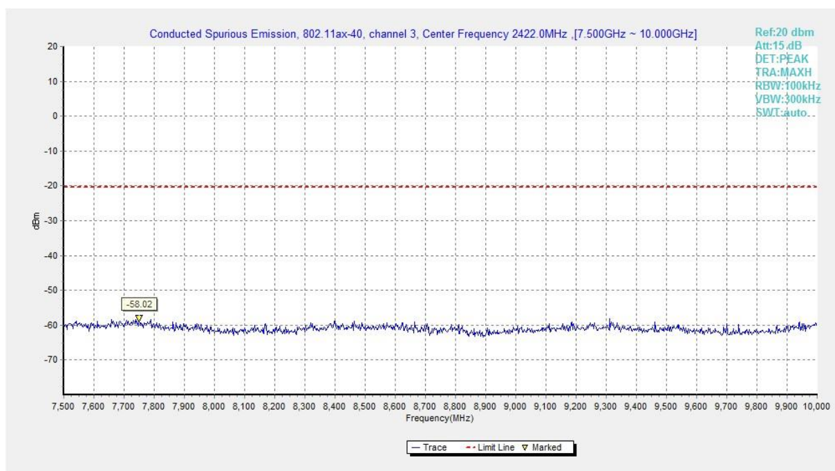
Fig.A.6.1.461 Transmitter Spurious Emission - Conducted (802.11ax-HE40, Ch3, 7.5 GHz-10 GHz)
