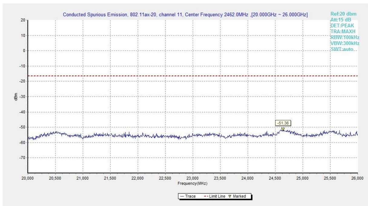
Fig.A.6.1.456 Transmitter Spurious Emission - Conducted (802.11ax-HE20, Ch11, 20 GHz-26 GHz)
