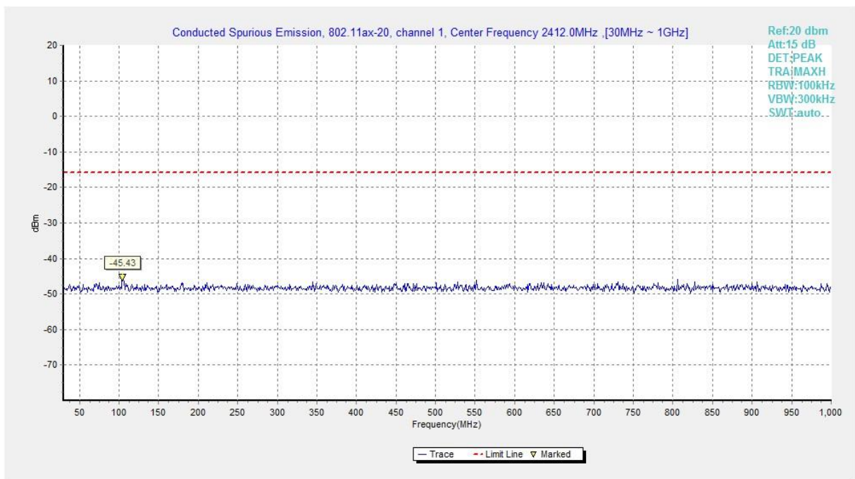
Fig.A.6.1.482 Transmitter Spurious Emission - Conducted (802.11ax-HE20-RU52-right, Ch1, 30 MHz-1 GHz)
