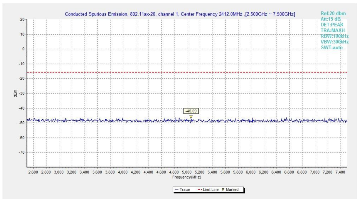
Fig.A.6.1.484 Transmitter Spurious Emission - Conducted (802.11ax-HE20-RU52-right, 2.5 GHz-7.5 GHz)
