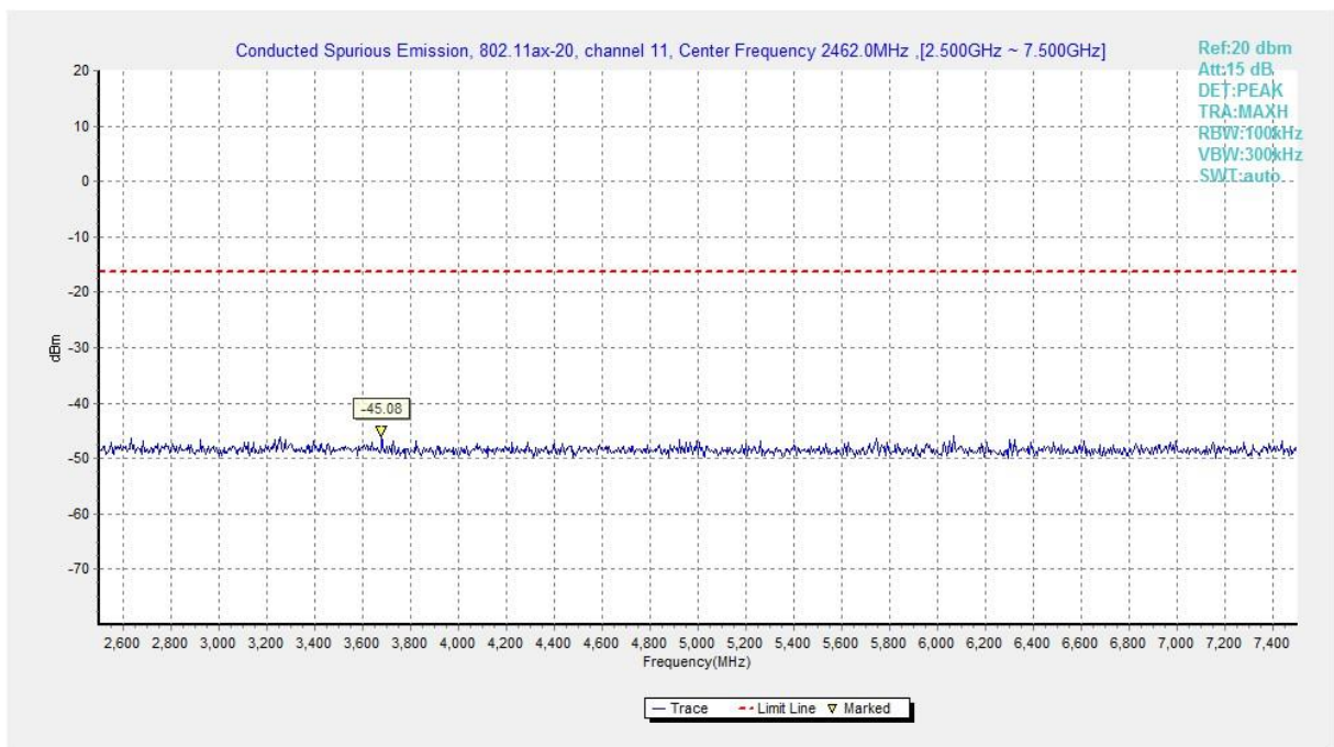
Fig.A.6.1.500 Transmitter Spurious Emission - Conducted (802.11ax-HE20-RU52-right, Ch11, 2.5 GHz-7.5 GHz)
