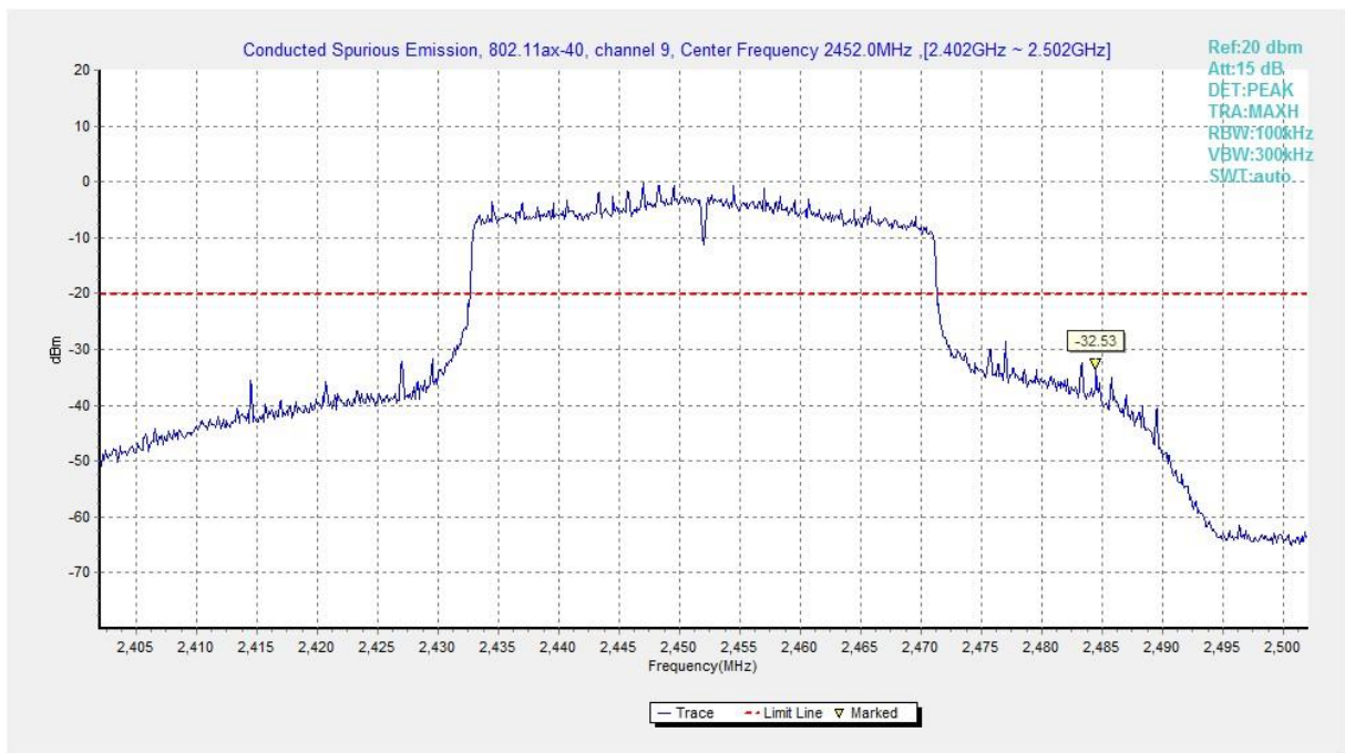
Fig.A.6.1.473 Transmitter Spurious Emission - Conducted (802.11ax-HE40, Ch9, Center Frequency)
