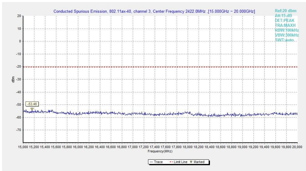
Fig.A.6.1.463 Transmitter Spurious Emission - Conducted (802.11ax-HE40, Ch3, 15 GHz-20 GHz)
