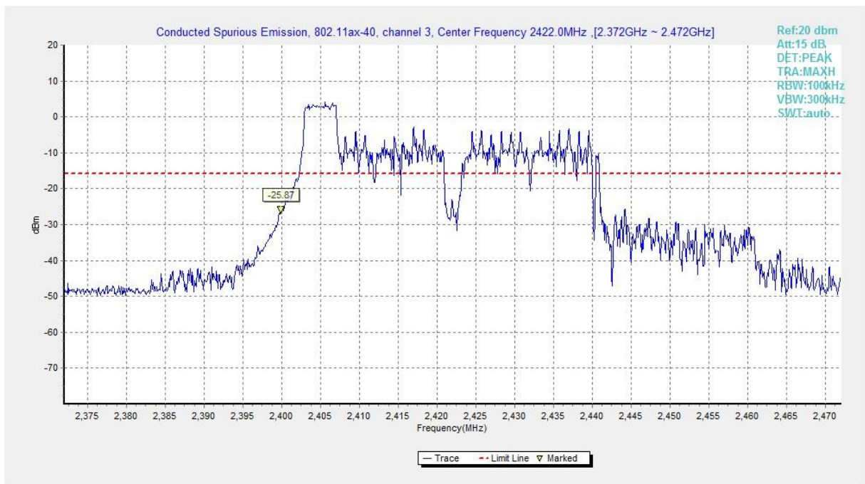
Fig.A.6.1.505 Transmitter Spurious Emission – Conducted (802.11ax-HE40-RU52-left, Ch3, Center Frequency)
