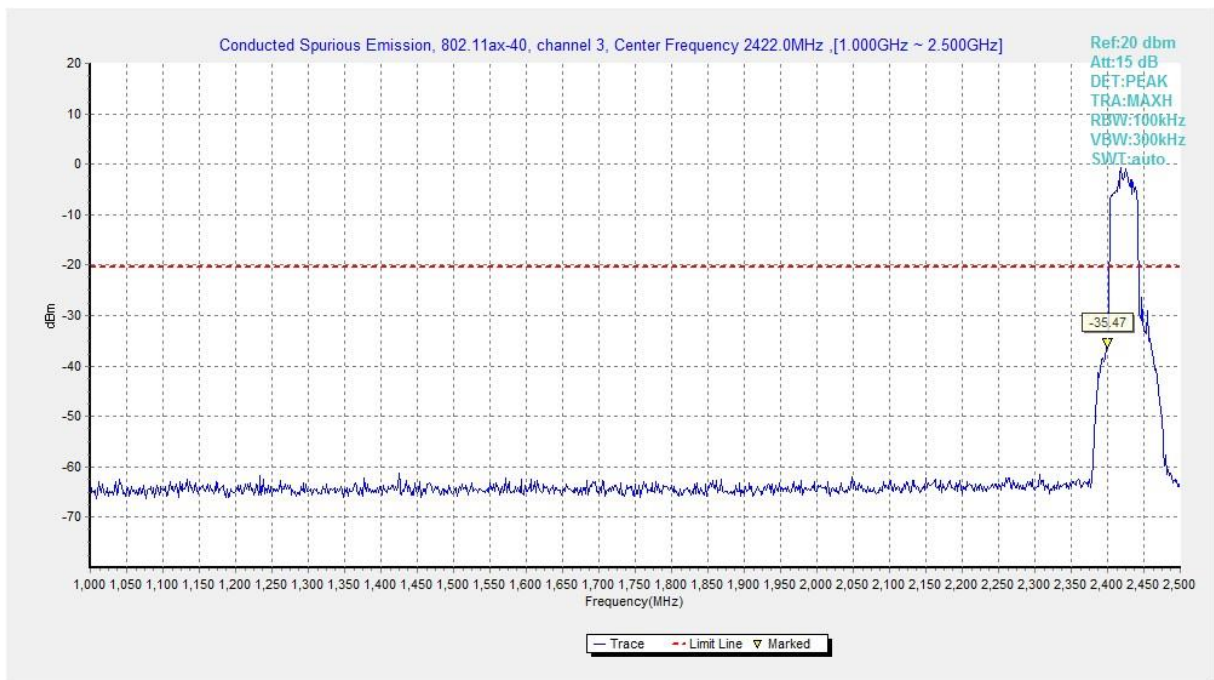
Fig.A.6.1.459 Transmitter Spurious Emission - Conducted (802.11ax-HE40, Ch3, 1 GHz-2.5 GHz)
