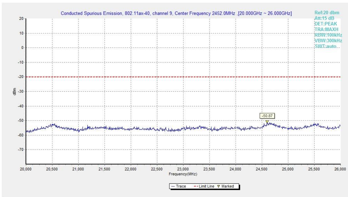
Fig.A.6.1.480 Transmitter Spurious Emission - Conducted (802.11ax-HE40, Ch9, 20 GHz-26 GHz)
