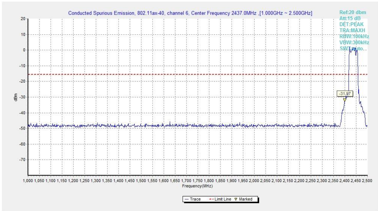
Fig.A.6.1.467 Transmitter Spurious Emission - Conducted (802.11ax-HE40, Ch6, 1 GHz-2.5 GHz)
