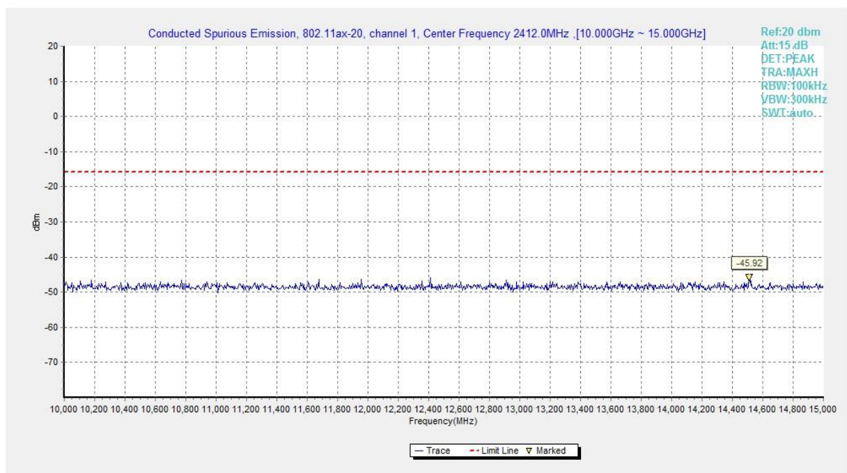
Fig.A.6.1.486 Transmitter Spurious Emission - Conducted (802.11ax-HE20-RU52-right, Ch1, 10 GHz-15 GHz)
