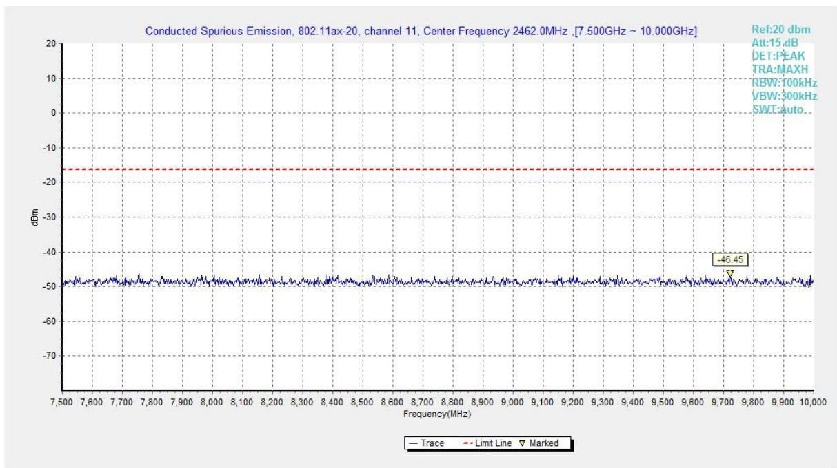
Fig.A.6.1.501 Transmitter Spurious Emission - Conducted (802.11ax-HE20-RU52-right, Ch11, 7.5 GHz-10 GHz)
