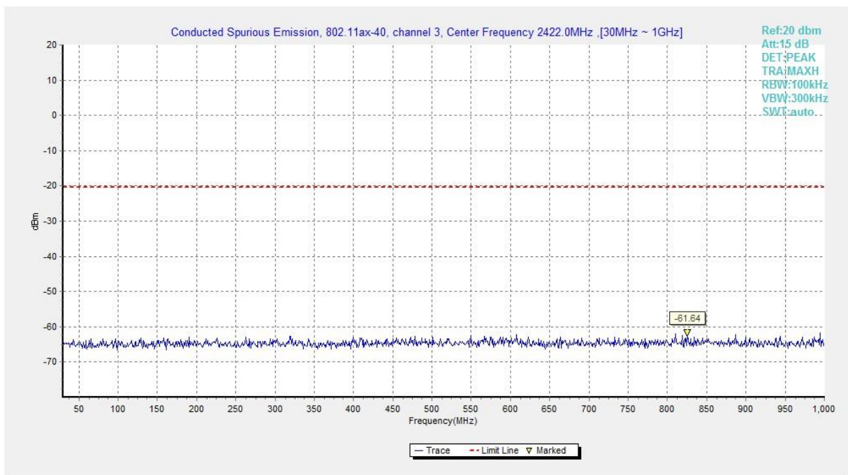
Fig.A.6.1.458 Transmitter Spurious Emission - Conducted (802.11ax-HE40, Ch3, 30 MHz-1 GHz)
