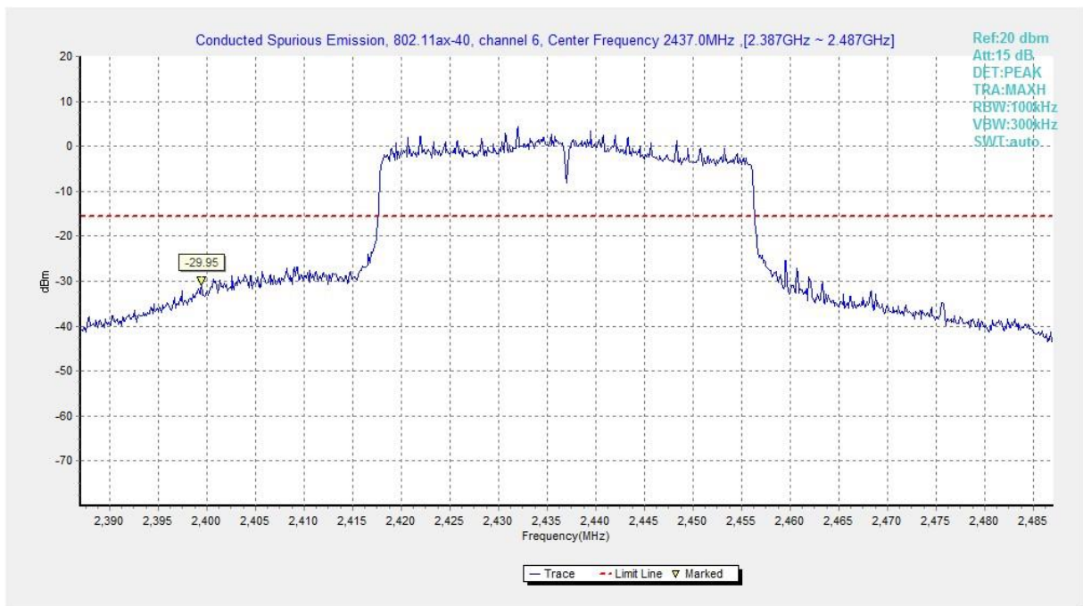
Fig.A.6.1.465 Transmitter Spurious Emission - Conducted (802.11ax-HE40, Ch6, Center Frequency)
