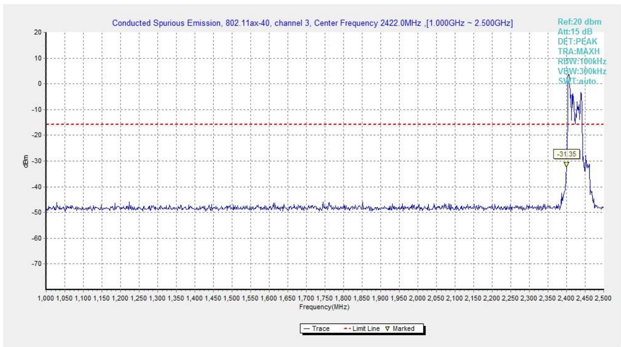
Fig.A.6.1.507 Transmitter Spurious Emission - Conducted (802.11ax-HE40-RU52-left, Ch3, 1 GHz-2.5 GHz)
