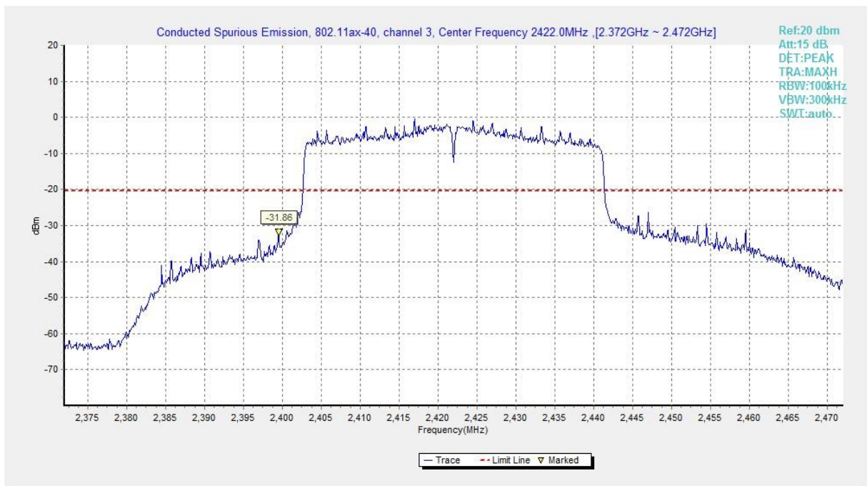
Fig.A.6.1.457 Transmitter Spurious Emission - Conducted (802.11ax-HE40, Ch3, Center Frequency)
