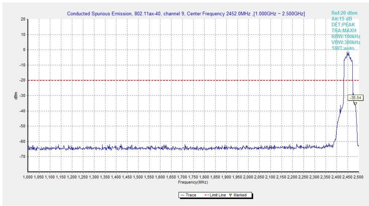
Fig.A.6.1.475 Transmitter Spurious Emission - Conducted (802.11ax-HE40, Ch9, 1 GHz-2.5 GHz)
