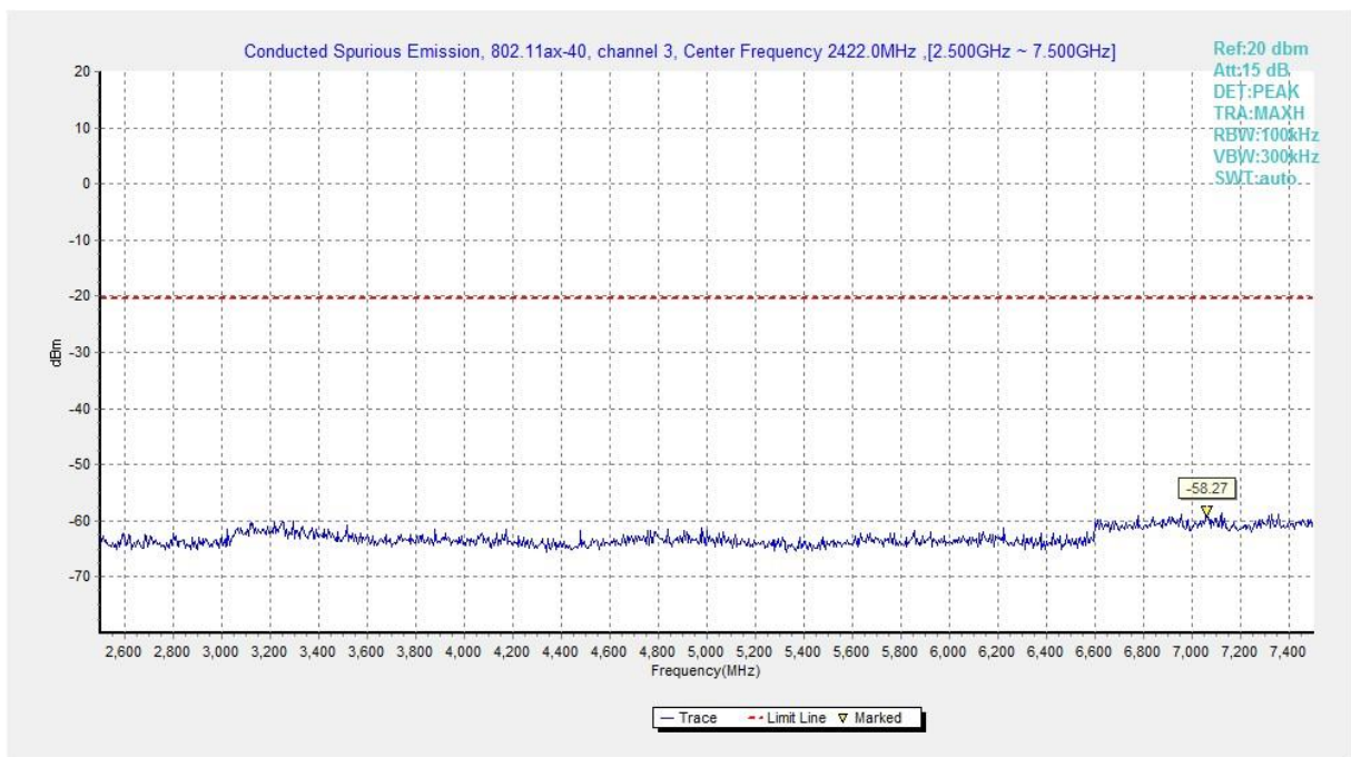
Fig.A.6.1.460 Transmitter Spurious Emission - Conducted (802.11ax-HE40, Ch3, 2.5 GHz-7.5 GHz)
