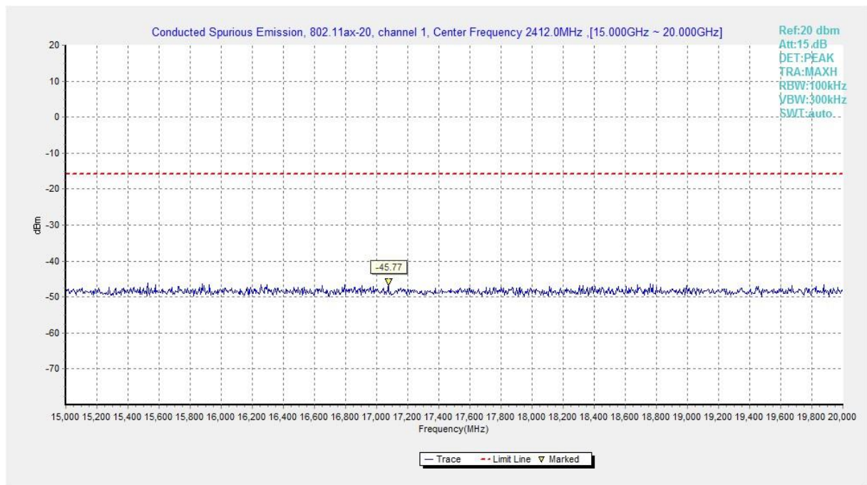
Fig.A.6.1.487 Transmitter Spurious Emission - Conducted (802.11ax-HE20-RU52-right, Ch1, 15 GHz-20 GHz)
