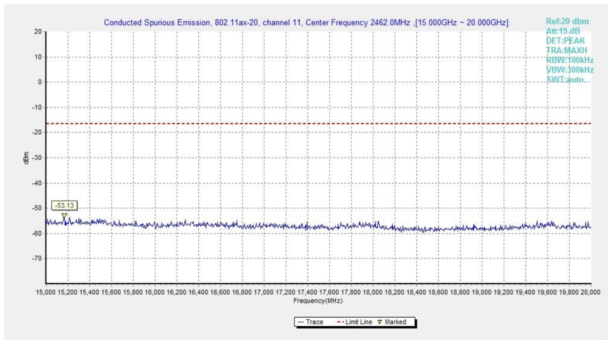
Fig.A.6.1.455 Transmitter Spurious Emission - Conducted (802.11ax-HE20, Ch11, 15 GHz-20 GHz)
