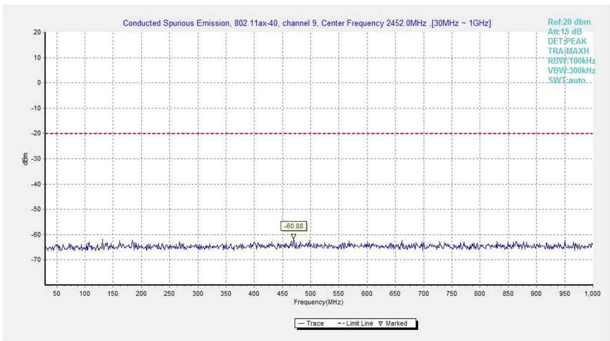
Fig.A.6.1.474 Transmitter Spurious Emission - Conducted (802.11ax-HE40, Ch9, 30 MHz-1 GHz)
