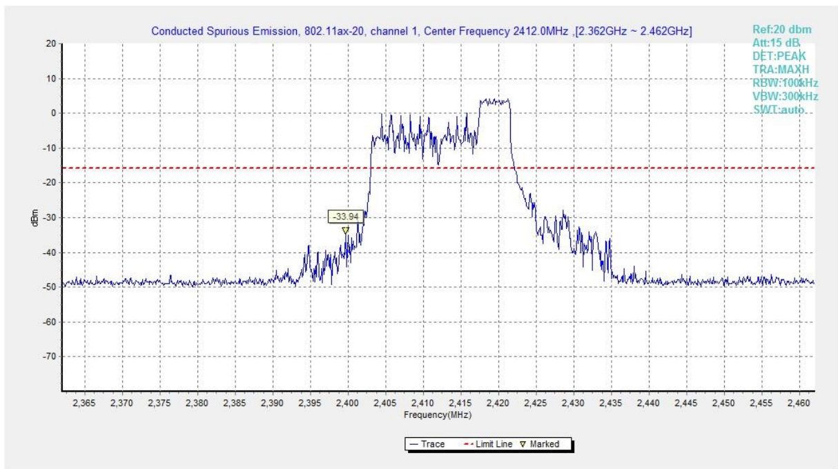
Fig.A.6.1.481 Transmitter Spurious Emission - Conducted (802.11ax-HE20-RU52-right, Ch1, Center Frequency)
