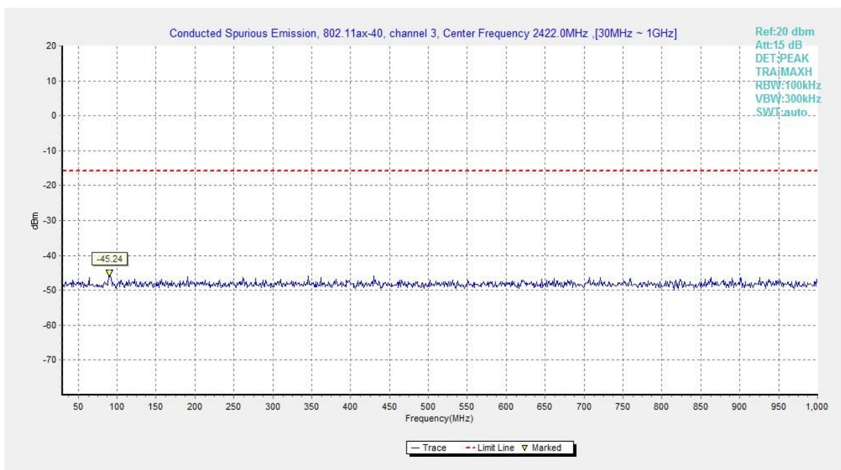
Fig.A.6.1.506 Transmitter Spurious Emission - Conducted (802.11ax-HE40-RU52-left, Ch3, 30 MHz-1 GHz)
