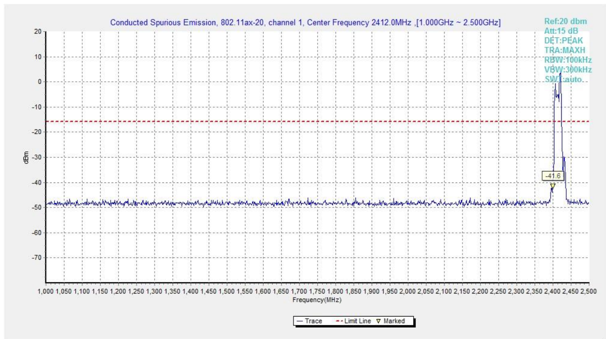
Fig.A.6.1.483 Transmitter Spurious Emission - Conducted (802.11ax-HE20-RU52-right, Ch1, 1 GHz-2.5 GHz)
