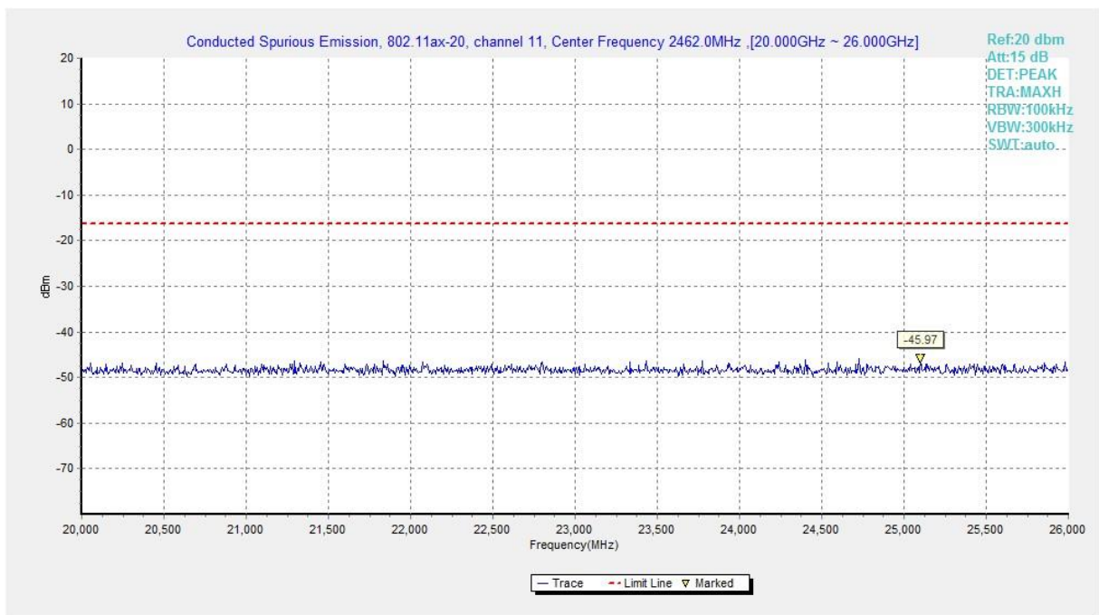
Fig.A.6.1.504 Transmitter Spurious Emission - Conducted (802.11ax-HE20-RU52-right, Ch11, 20 GHz-26 GHz)
