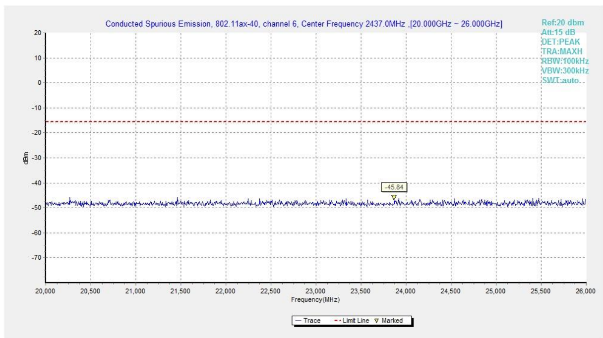
Fig.A.6.1.472 Transmitter Spurious Emission - Conducted (802.11ax-HE40, Ch6, 20 GHz-26 GHz)
