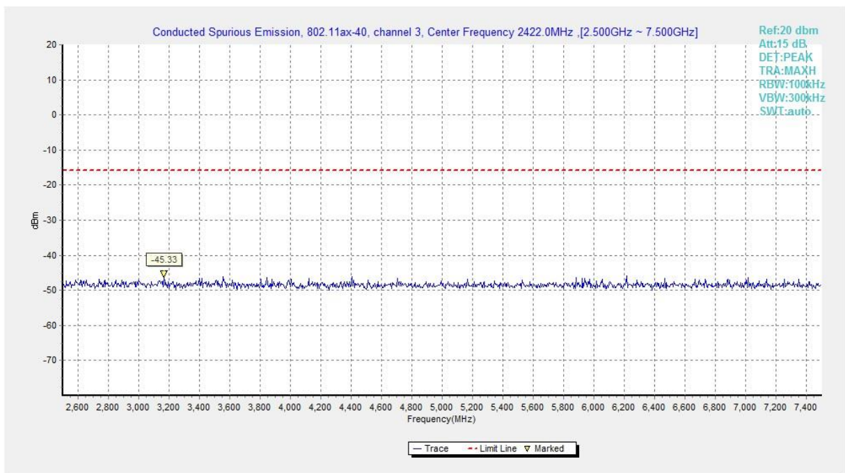
Fig.A.6.1.508 Transmitter Spurious Emission - Conducted (802.11ax-HE40-RU52-left, Ch3, 2.5 GHz-7.5 GHz)
