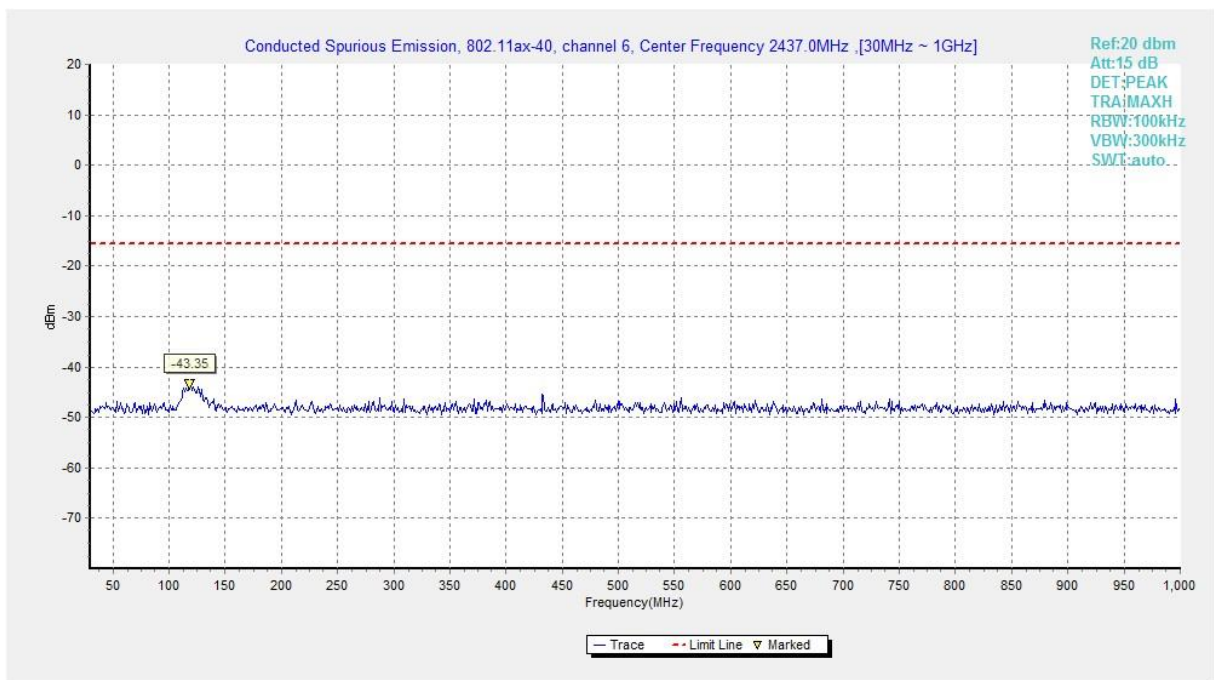
Fig.A.6.1.466 Transmitter Spurious Emission - Conducted (802.11ax-HE40, Ch6, 30 MHz-1 GHz)
