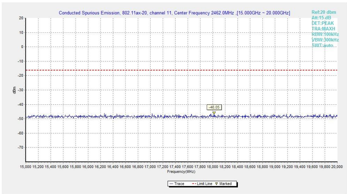
Fig.A.6.1.503 Transmitter Spurious Emission - Conducted (802.11ax-HE20-RU52-right, Ch11, 15 GHz-20 GHz)
