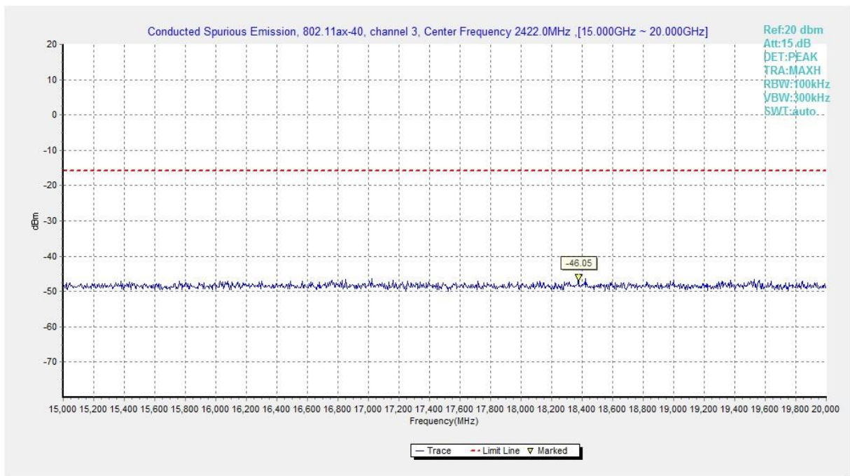
Fig.A.6.1.511 Transmitter Spurious Emission - Conducted (802.11ax-HE40-RU52-left, Ch3, 15 GHz-20 GHz)
