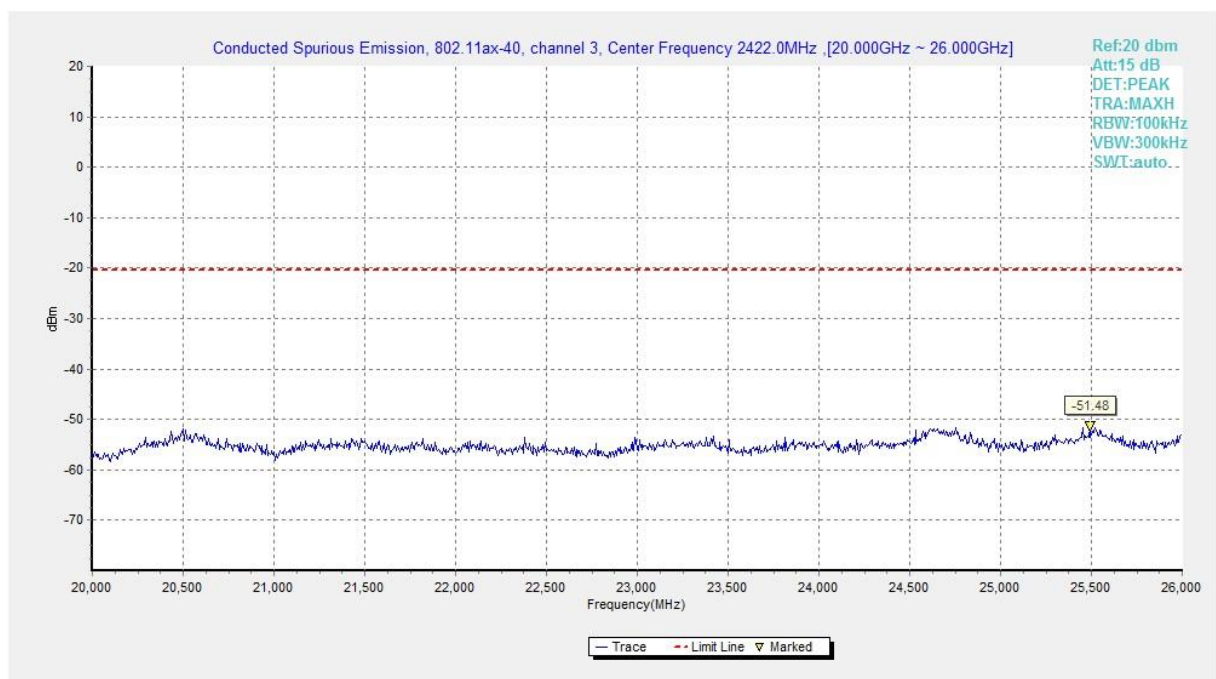
Fig.A.6.1.464 Transmitter Spurious Emission - Conducted (802.11ax-HE40, Ch3, 20 GHz-26 GHz)
