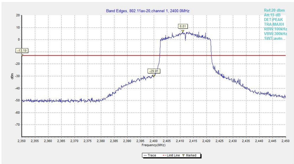
Fig.A.5.9 Band Edges (802.11ax-HE20, Ch 1)
