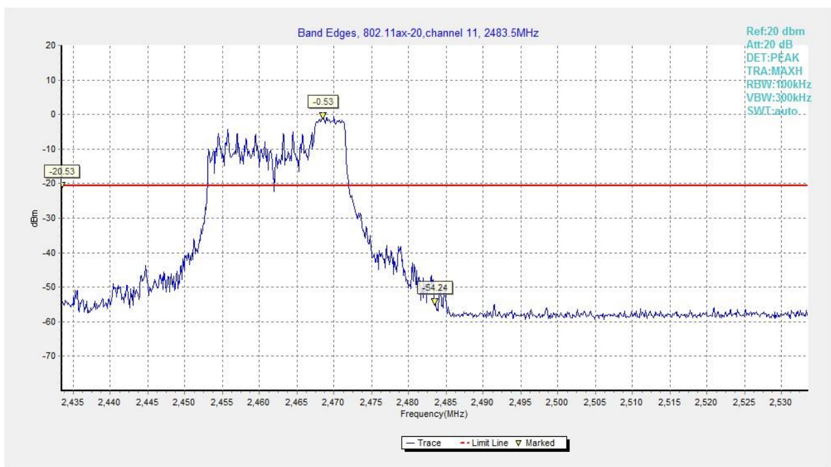
Fig.A.5.42 Band Edges (802.11ax-HE20-RU52-right, Ch 11)
