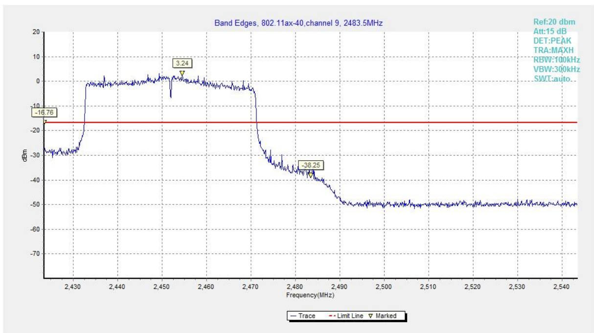
Fig.A.5.26 Band Edges (802.11ax-HE40, Ch 9)
