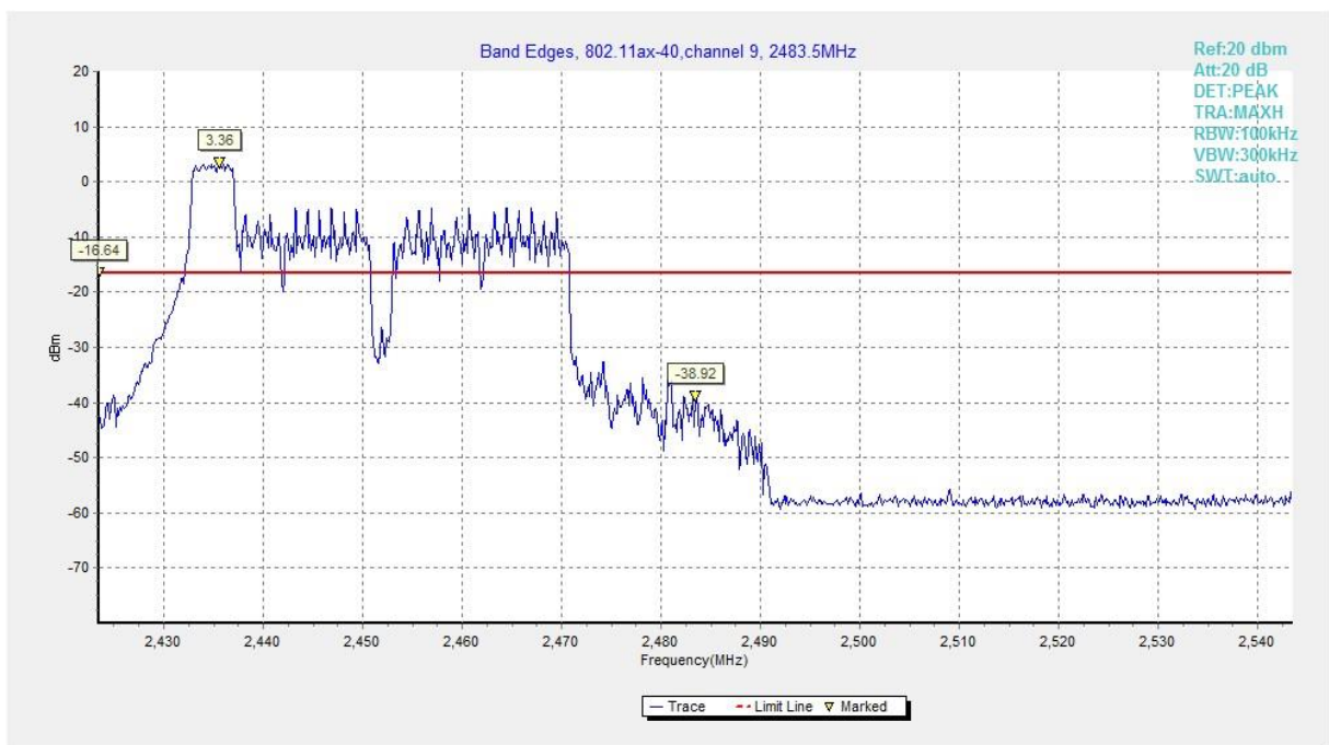
Fig.A.5.16 Band Edges (802.11ax-HE40-RU52-left, Ch 9)
