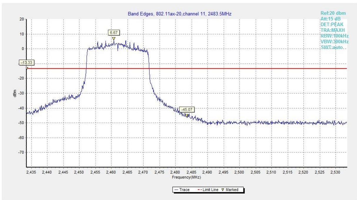
Fig.A.5.24 Band Edges (802.11ax-HE20, Ch 11)
