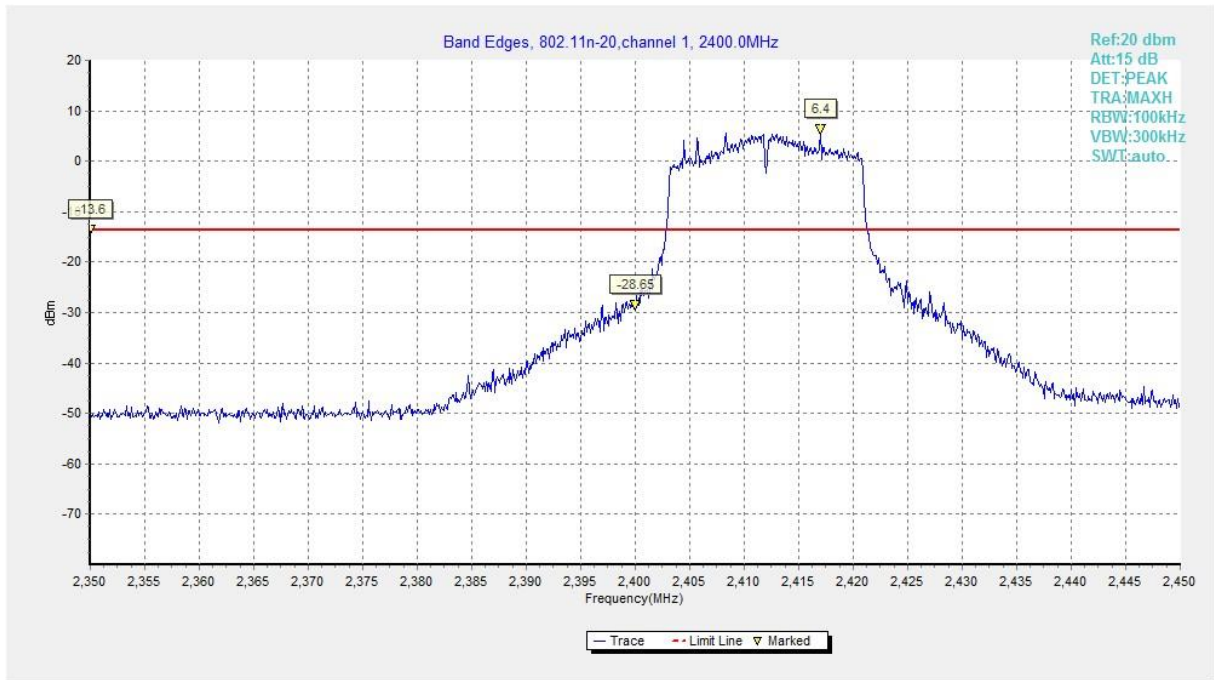
Fig.A.5.19 Band Edges (802.11n-HT20, Ch 1)
