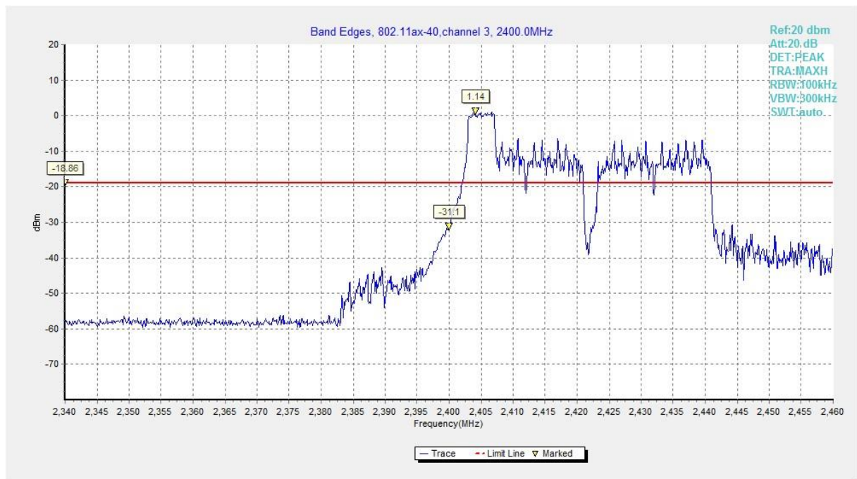
Fig.A.5.43 Band Edges (802.11ax-HE40-RU52-left, Ch 3)
