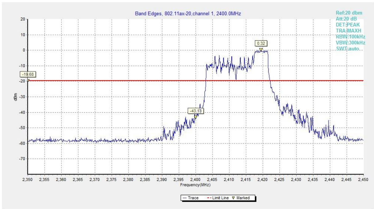
Fig.A.5.41 Band Edges (802.11ax-HE20-RU52-right, Ch 1)
