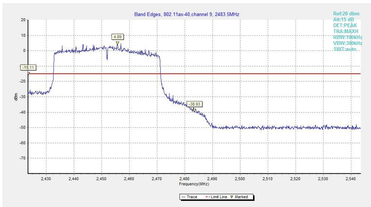
Fig.A.5.12 Band Edges (802.11ax-HE40, Ch 9)
