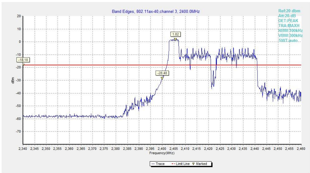
Fig.A.5.15 Band Edges (802.11ax-HE40-RU52-left, Ch 3)
