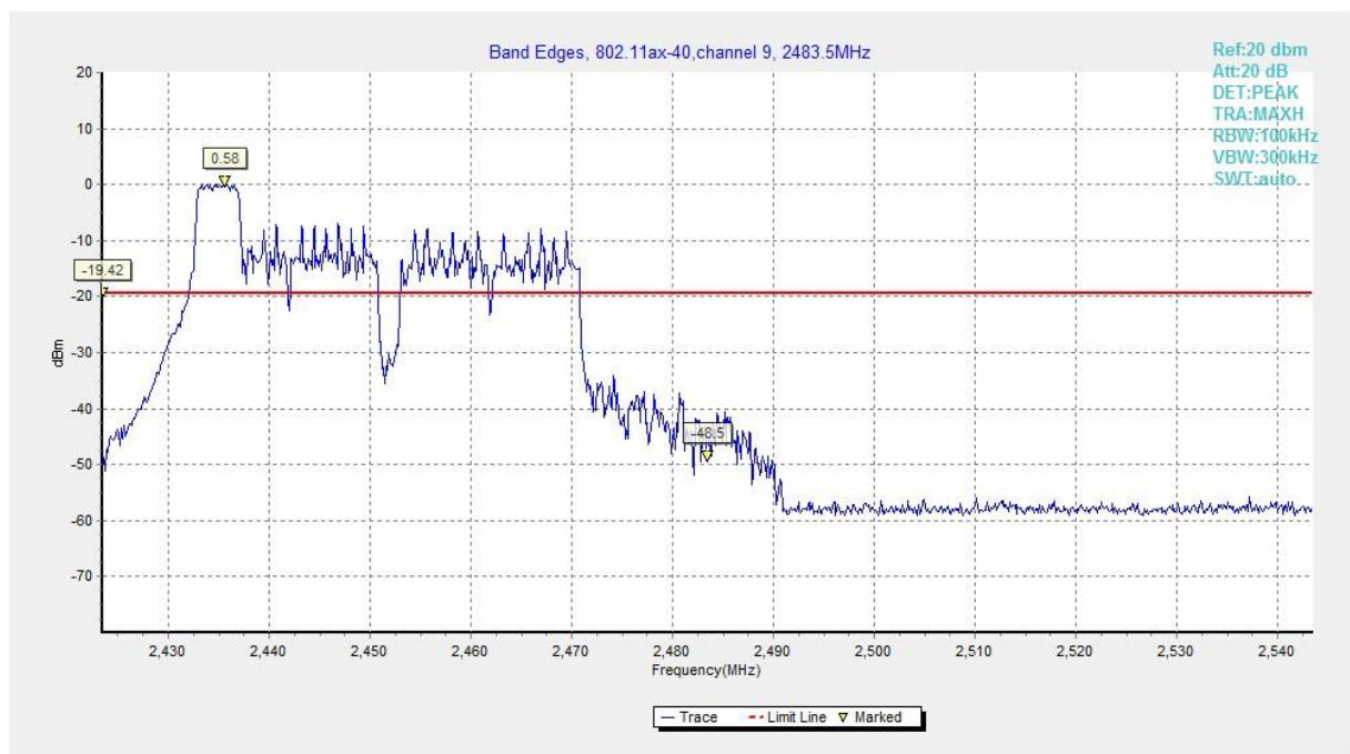
Fig.A.5.44 Band Edges (802.11ax-HE40-RU52-left, Ch 9)
