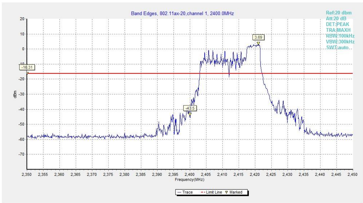
Fig.A.5.27 Band Edges (802.11ax-HE20-RU52-right, Ch 1)
