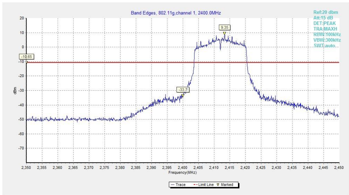
Fig.A.5.17 Band Edges (802.11g, Ch 1)
