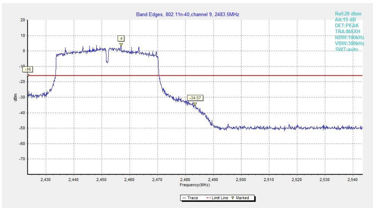
Fig.A.5.22 Band Edges (802.11n-HT40, Ch 9)
