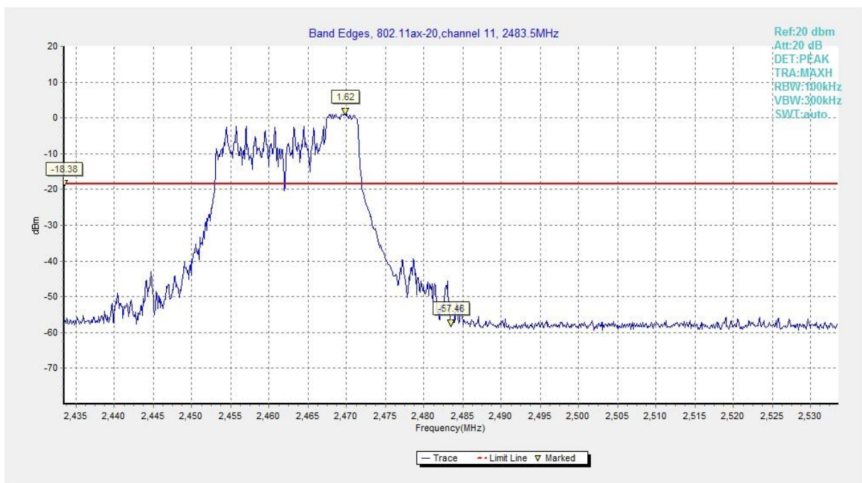
Fig.A.5.14 Band Edges (802.11ax-HE20-RU52-right, Ch 11)
