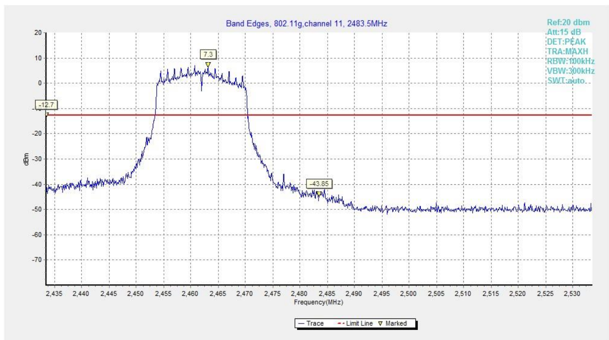
Fig.A.5.18 Band Edges (802.11g, Ch 11)
