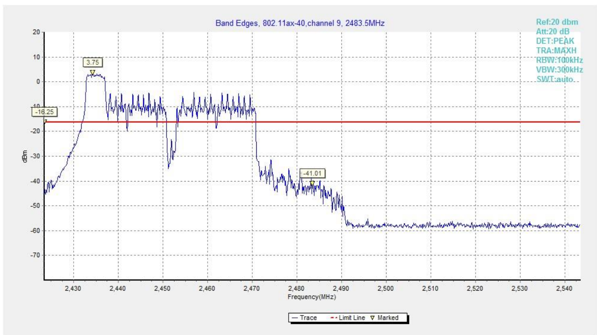
Fig.A.5.30 Band Edges (802.11ax-HE40-RU52-left, Ch 9)
