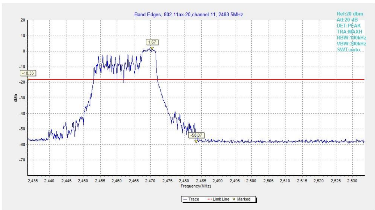
Fig.A.5.28 Band Edges (802.11ax-HE20-RU52-right, Ch 11)
