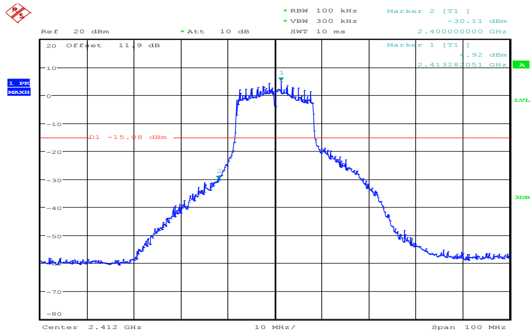
Fig.A.5.31 Band Edges (802.11g, Ch 1)
