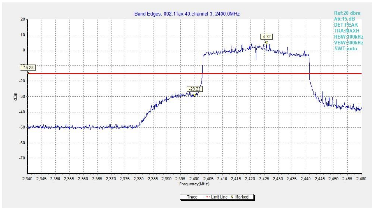
Fig.A.5.25 Band Edges (802.11ax-HE40, Ch 3)
