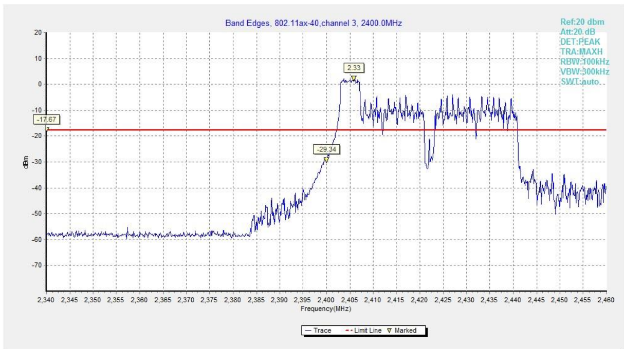
Fig.A.5.29 Band Edges (802.11ax-HE40-RU52-left, Ch 3)
