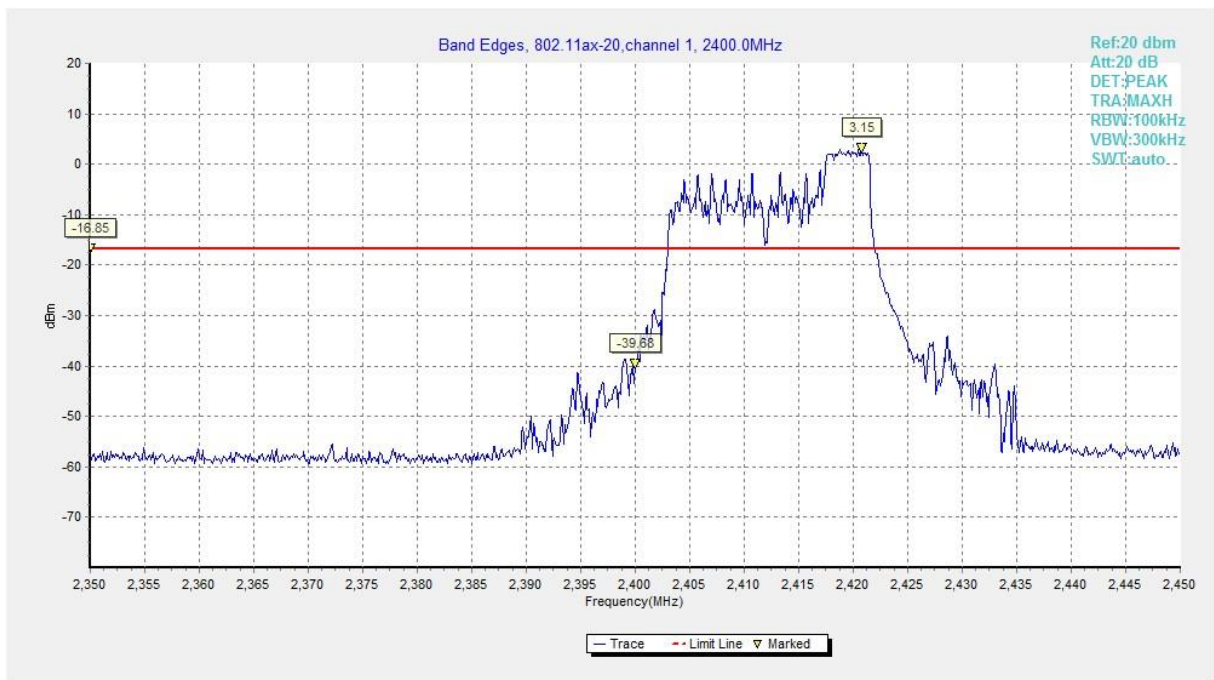
Fig.A.5.13 Band Edges (802.11ax-HE20-RU52-right, Ch 1)
