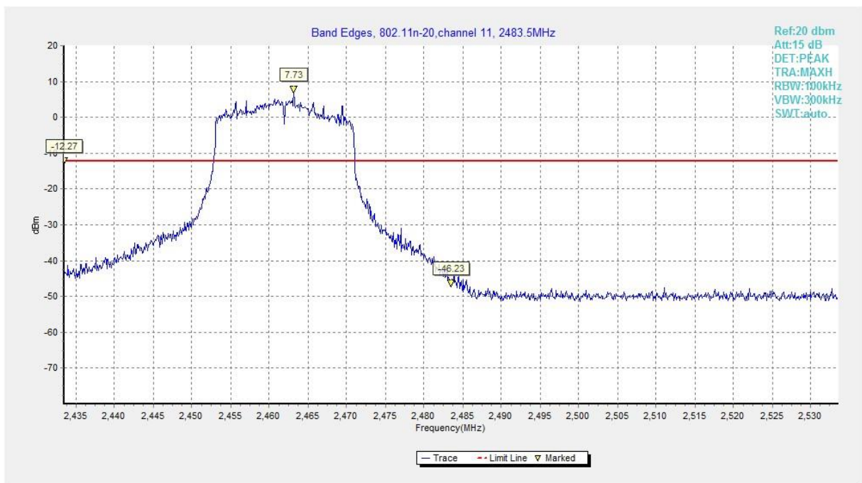
Fig.A.5.20 Band Edges (802.11n-HT20, Ch 11)
