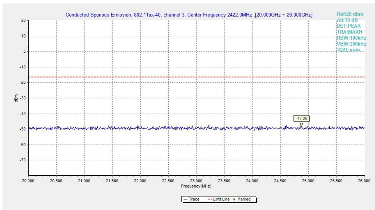
Fig.A.6.1.176 Transmitter Spurious Emission - Conducted (802.11ax-HE40-RU52-left, Ch3, 20 GHz-26 GHz)
