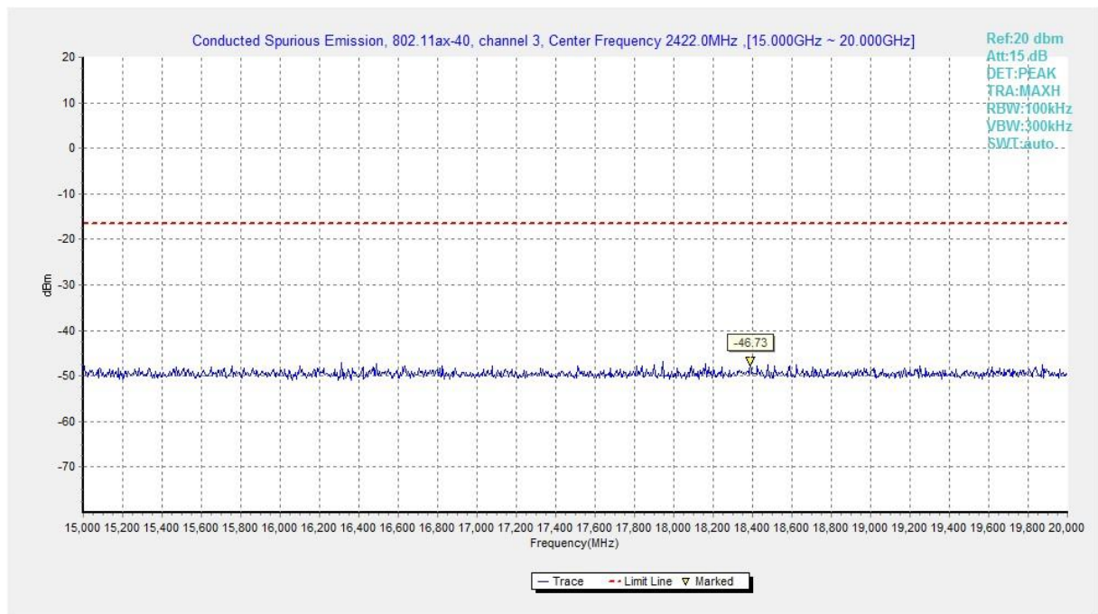
Fig.A.6.1.175 Transmitter Spurious Emission - Conducted (802.11ax-HE40-RU52-left, Ch3, 15 GHz-20 GHz)
