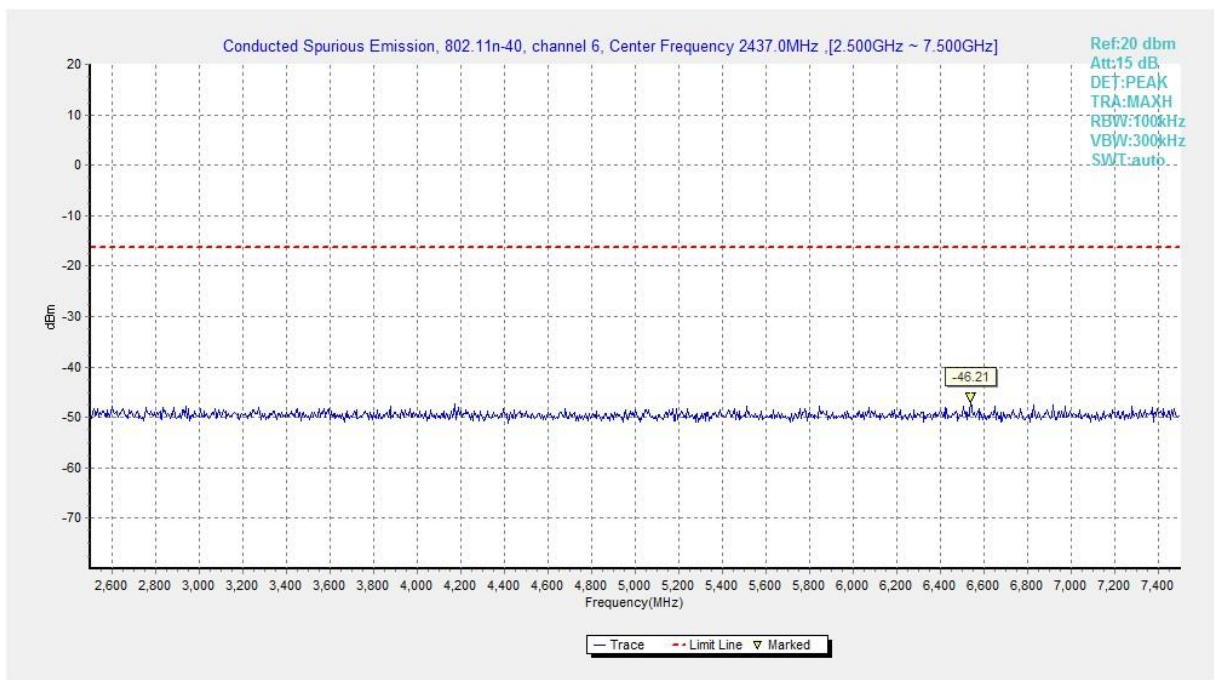
Fig.A.6.1.252 Transmitter Spurious Emission - Conducted (802.11n-HT40, Ch6, 2.5 GHz-7.5 GHz)
