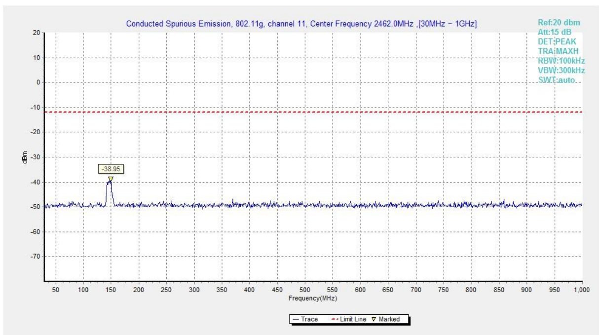
Fig.A.6.1.210 Transmitter Spurious Emission - Conducted (802.11g, Ch11, 30 MHz-1 GHz)
