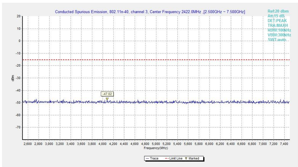
Fig.A.6.1.244 Transmitter Spurious Emission - Conducted (802.11n-HT40, Ch3, 2.5 GHz-7.5 GHz)
