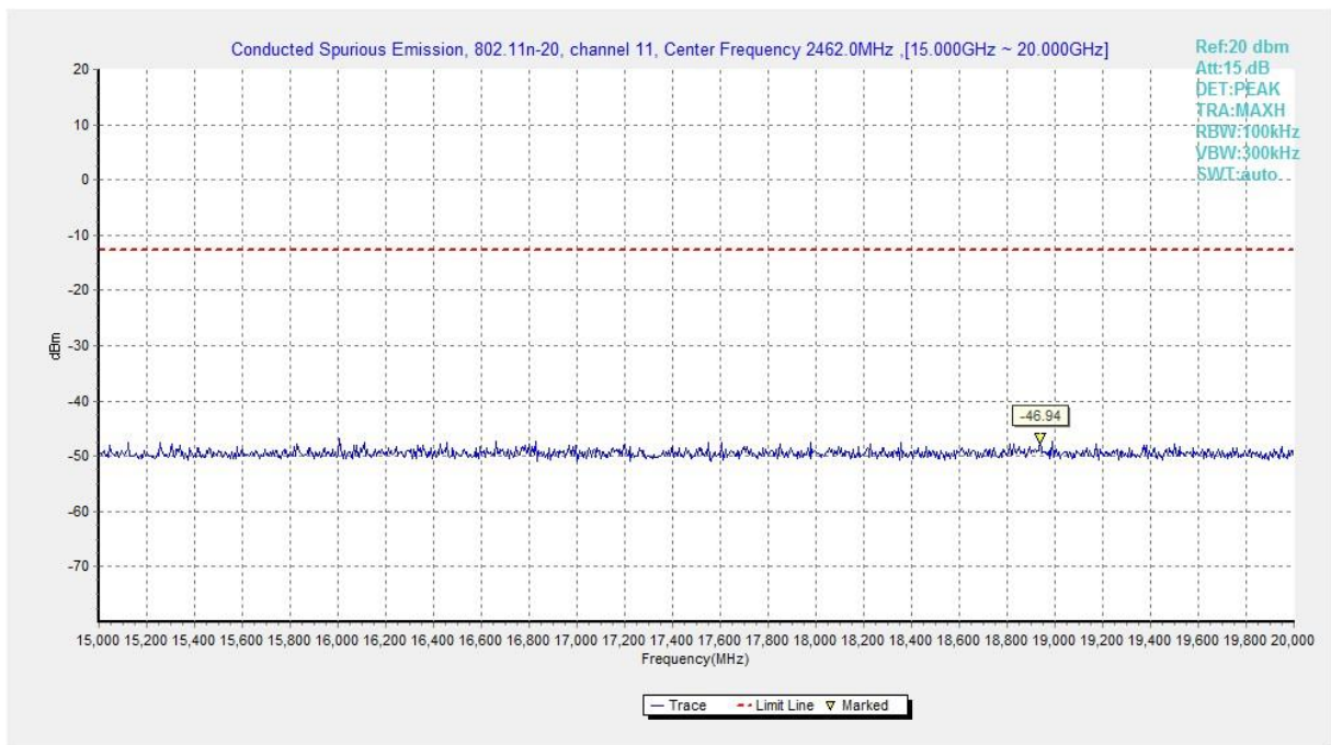
Fig.A.6.1.239 Transmitter Spurious Emission - Conducted (802.11n-HT20, Ch11, 15 GHz-20 GHz)
