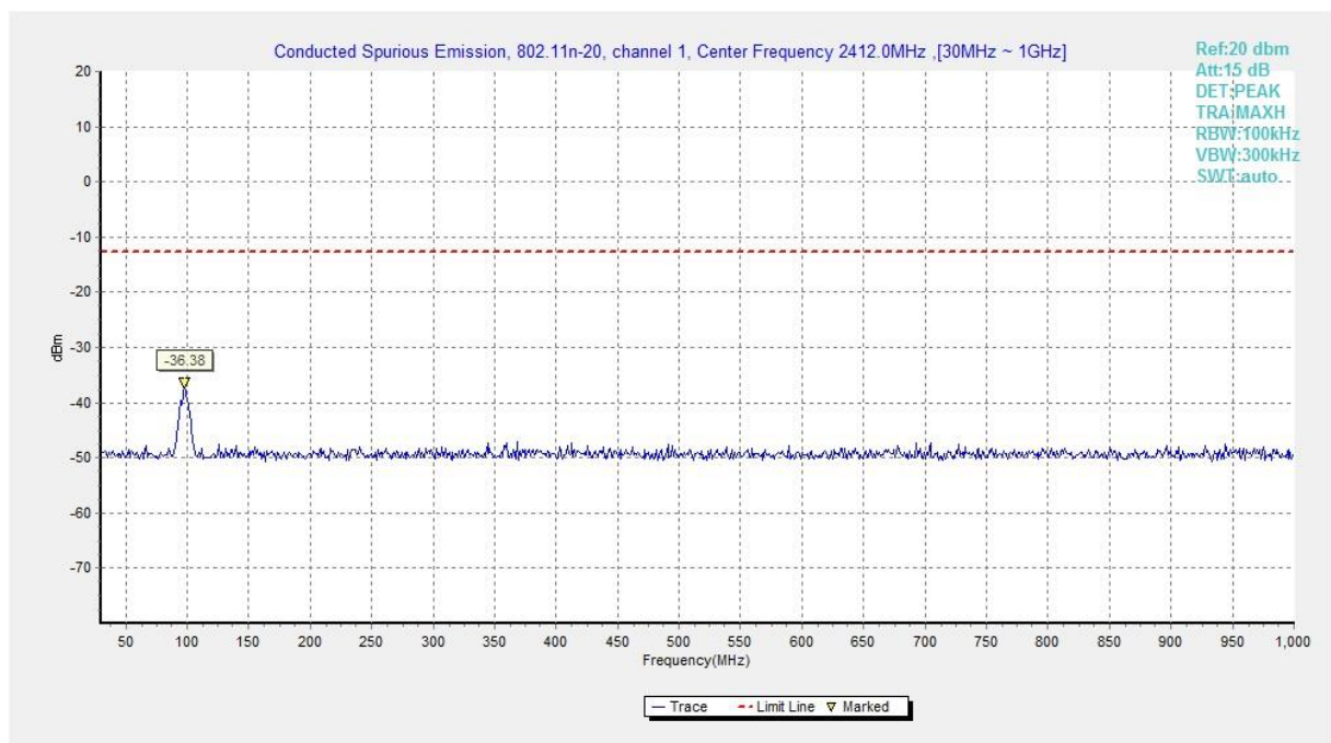
Fig.A.6.1.218 Transmitter Spurious Emission - Conducted (802.11n-HT20, Ch1, 30 MHz-1 GHz)
