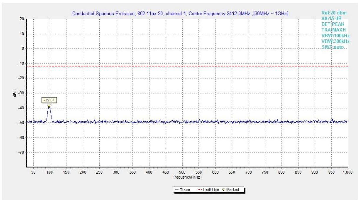
Fig.A.6.1.266 Transmitter Spurious Emission - Conducted (802.11ax-HE20, Ch1, 30 MHz-1 GHz)
