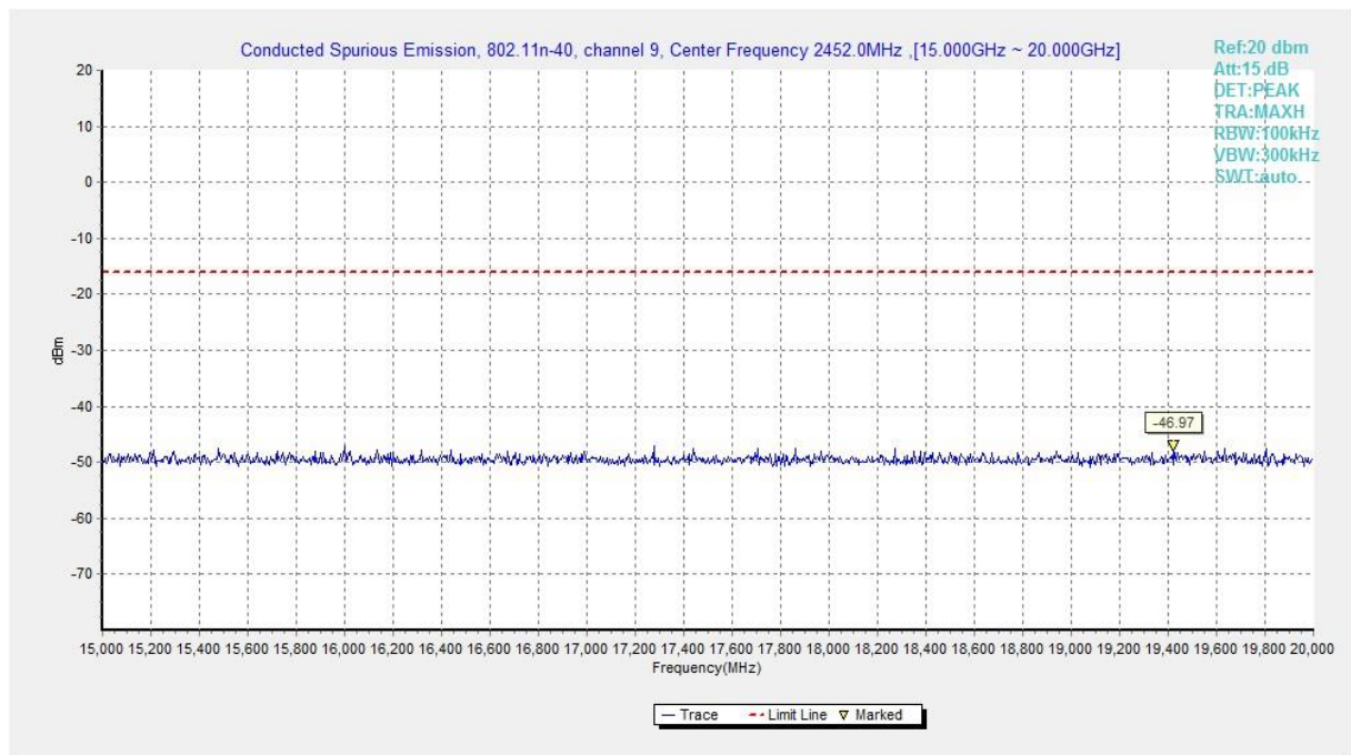
Fig.A.6.1.263 Transmitter Spurious Emission - Conducted (802.11n-HT40, Ch9, 15 GHz-20 GHz)
