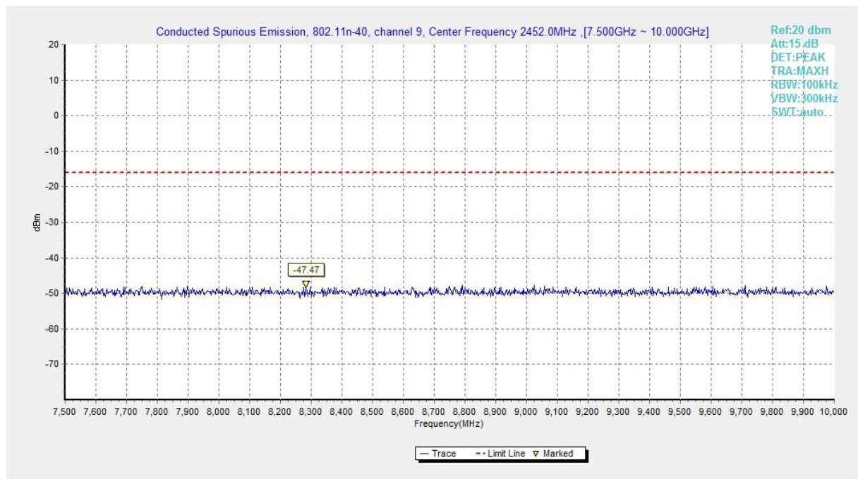
Fig.A.6.1.261 Transmitter Spurious Emission - Conducted (802.11n-HT40, Ch9, 7.5 GHz-10 GHz)
