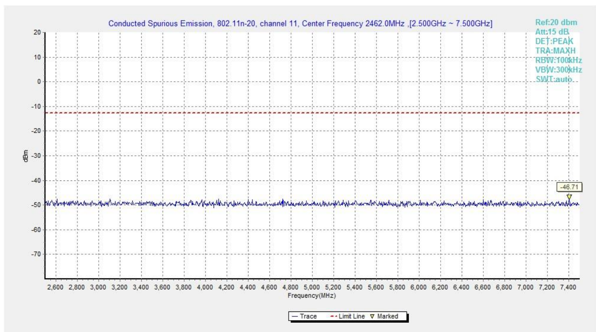
Fig.A.6.1.236 Transmitter Spurious Emission - Conducted (802.11n-HT20, Ch11, 2.5 GHz-7.5 GHz)
