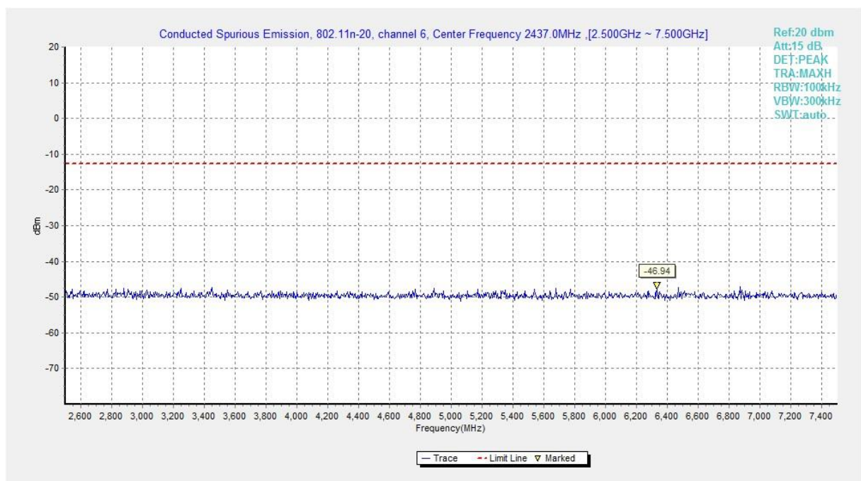
Fig.A.6.1.228 Transmitter Spurious Emission - Conducted (802.11n-HT20, Ch6, 2.5 GHz-7.5 GHz)
