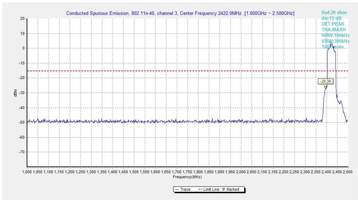
Fig.A.6.1.243 Transmitter Spurious Emission - Conducted (802.11n-HT40, Ch3, 1 GHz-2.5 GHz)
