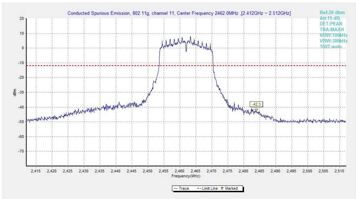
Fig.A.6.1.209 Transmitter Spurious Emission - Conducted (802.11g, Ch11, Center Frequency)
