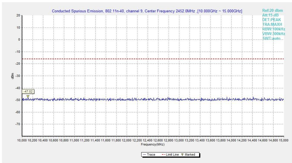
Fig.A.6.1.262 Transmitter Spurious Emission - Conducted (802.11n-HT40, Ch9, 10 GHz-15 GHz)
