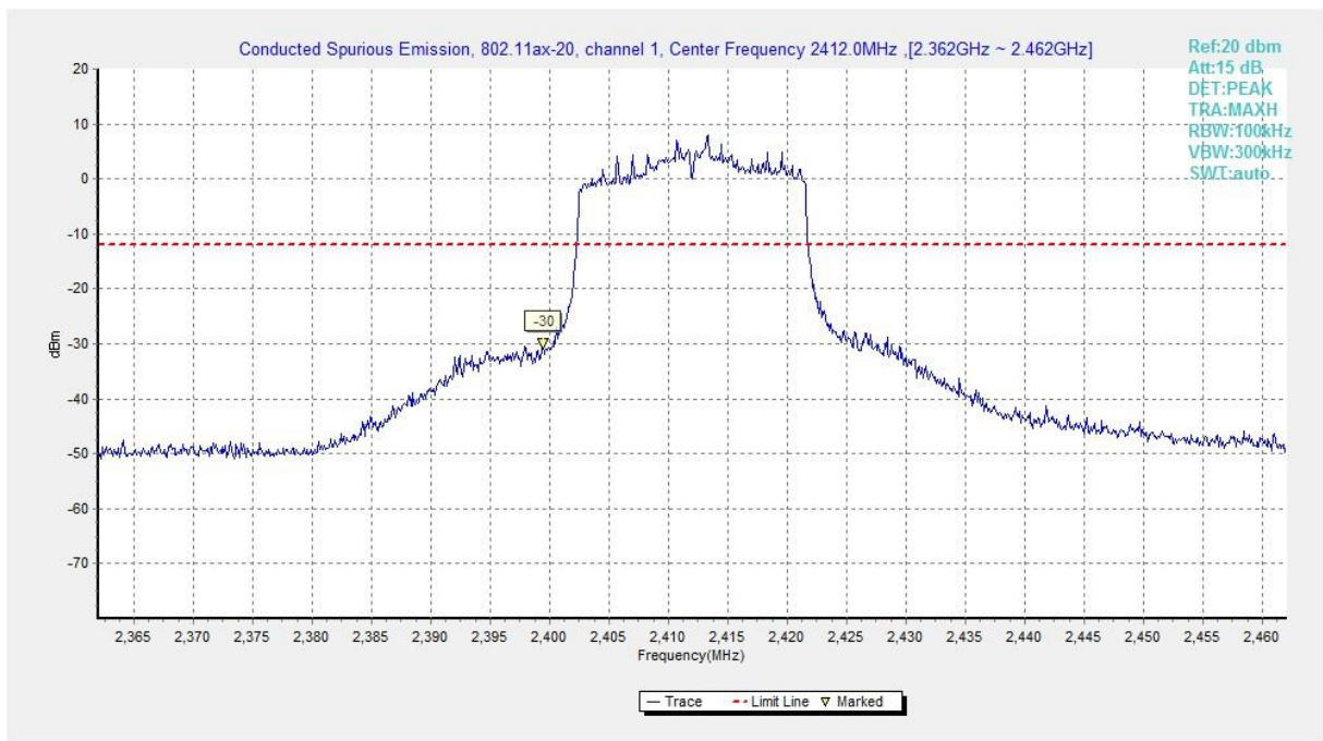
Fig.A.6.1.265 Transmitter Spurious Emission - Conducted (802.11ax-HE20, Ch1, Center Frequency)
