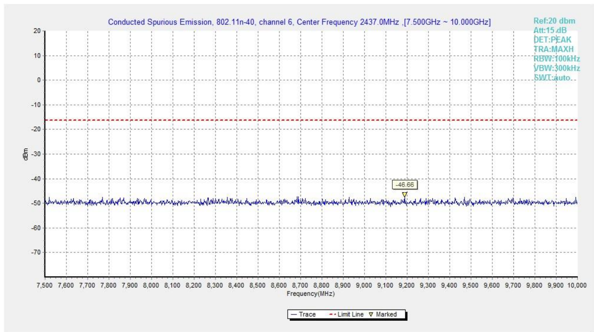
Fig.A.6.1.253 Transmitter Spurious Emission - Conducted (802.11n-HT40, Ch6, 7.5 GHz-10 GHz)
