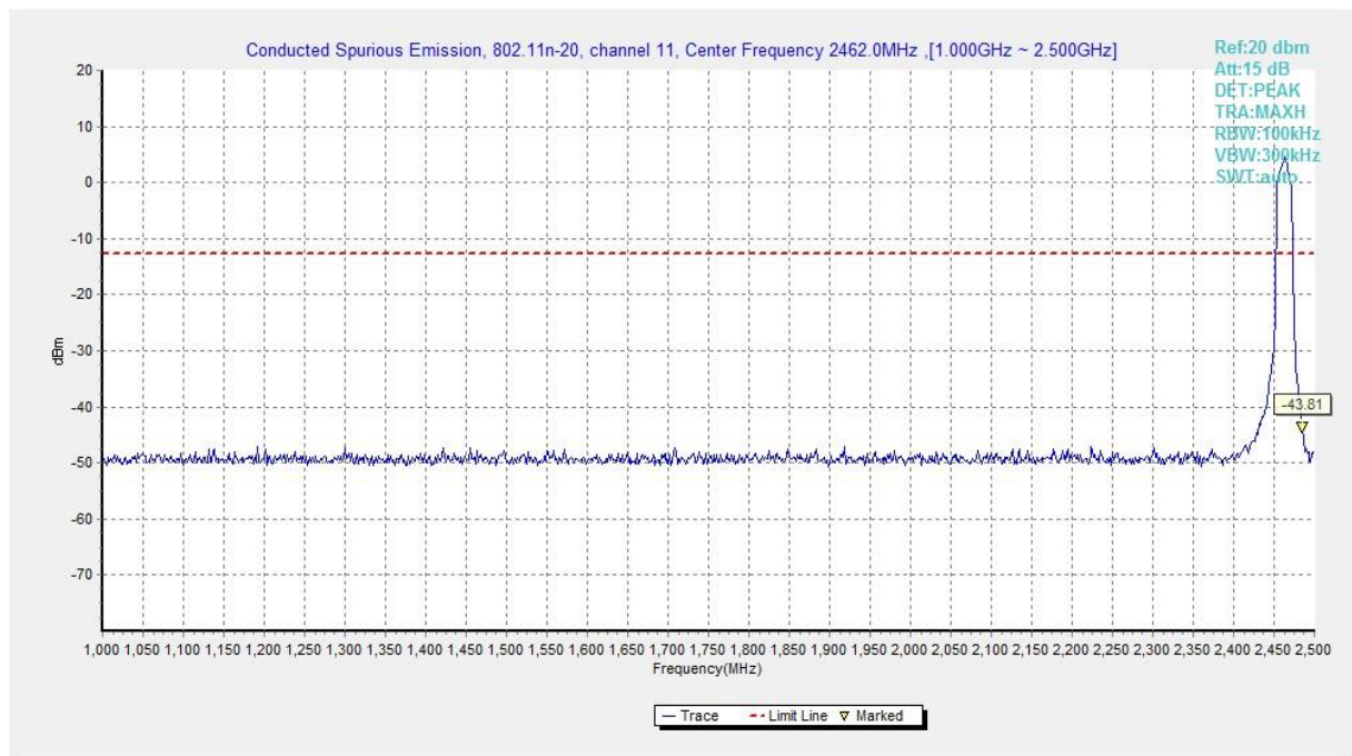
Fig.A.6.1.235 Transmitter Spurious Emission - Conducted (802.11n-HT20, Ch11, 1 GHz-2.5 GHz)
