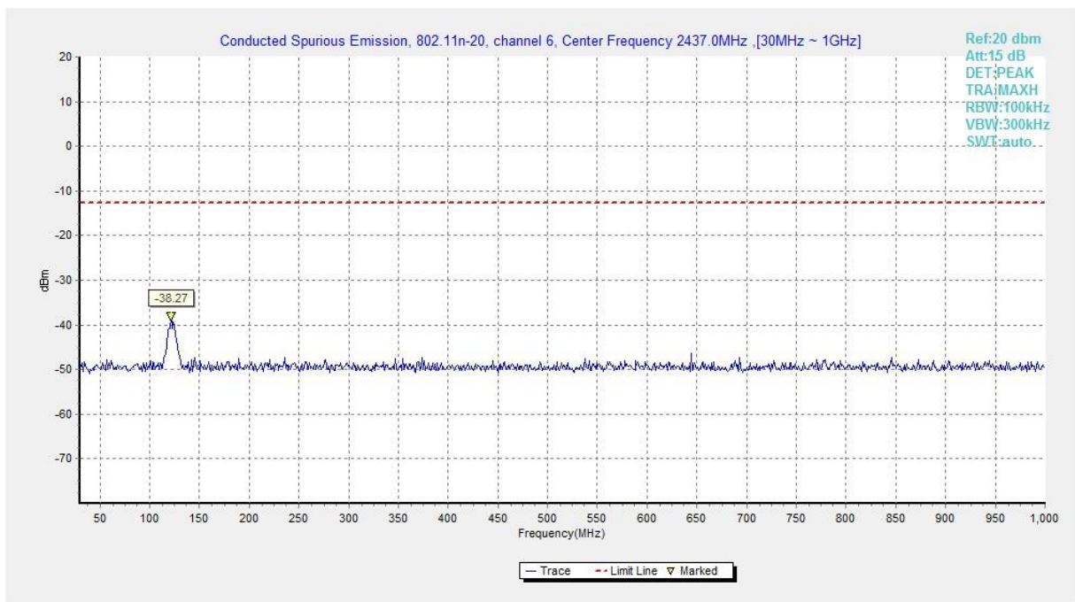
Fig.A.6.1.226 Transmitter Spurious Emission - Conducted (802.11n-HT20, Ch6, 30 MHz-1 GHz)
