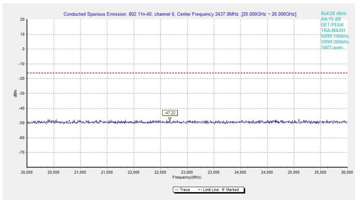
Fig.A.6.1.256 Transmitter Spurious Emission - Conducted (802.11n-HT40, Ch6, 20 GHz-26 GHz)
