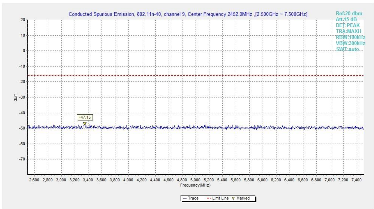
Fig.A.6.1.260 Transmitter Spurious Emission - Conducted (802.11n-HT40, Ch9, 2.5 GHz-7.5 GHz)
