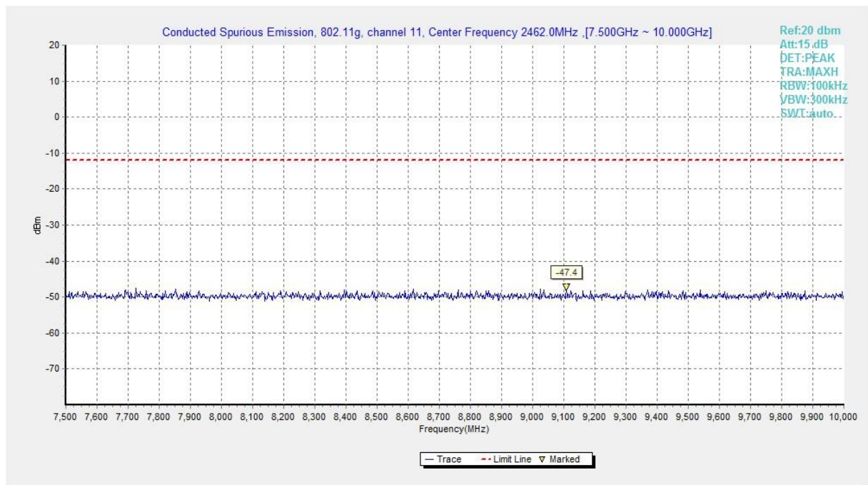
Fig.A.6.1.213 Transmitter Spurious Emission - Conducted (802.11g, Ch11, 7.5 GHz-10 GHz)
