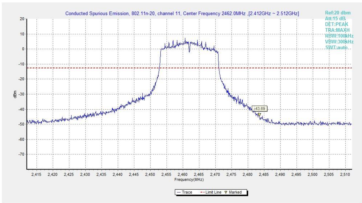
Fig.A.6.1.233 Transmitter Spurious Emission - Conducted (802.11n-HT20, Ch11, Center Frequency)
