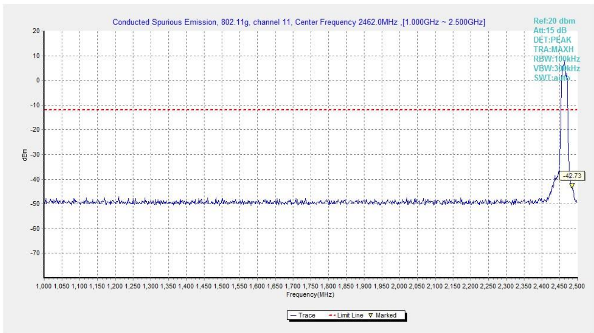
Fig.A.6.1.211 Transmitter Spurious Emission - Conducted (802.11g, Ch11, 1 GHz-2.5 GHz)
