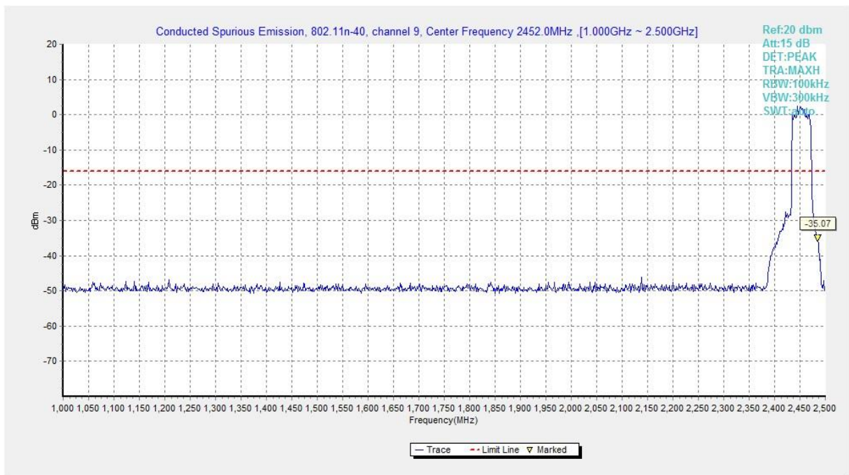
Fig.A.6.1.259 Transmitter Spurious Emission - Conducted (802.11n-HT40, Ch9, 1 GHz-2.5 GHz)
