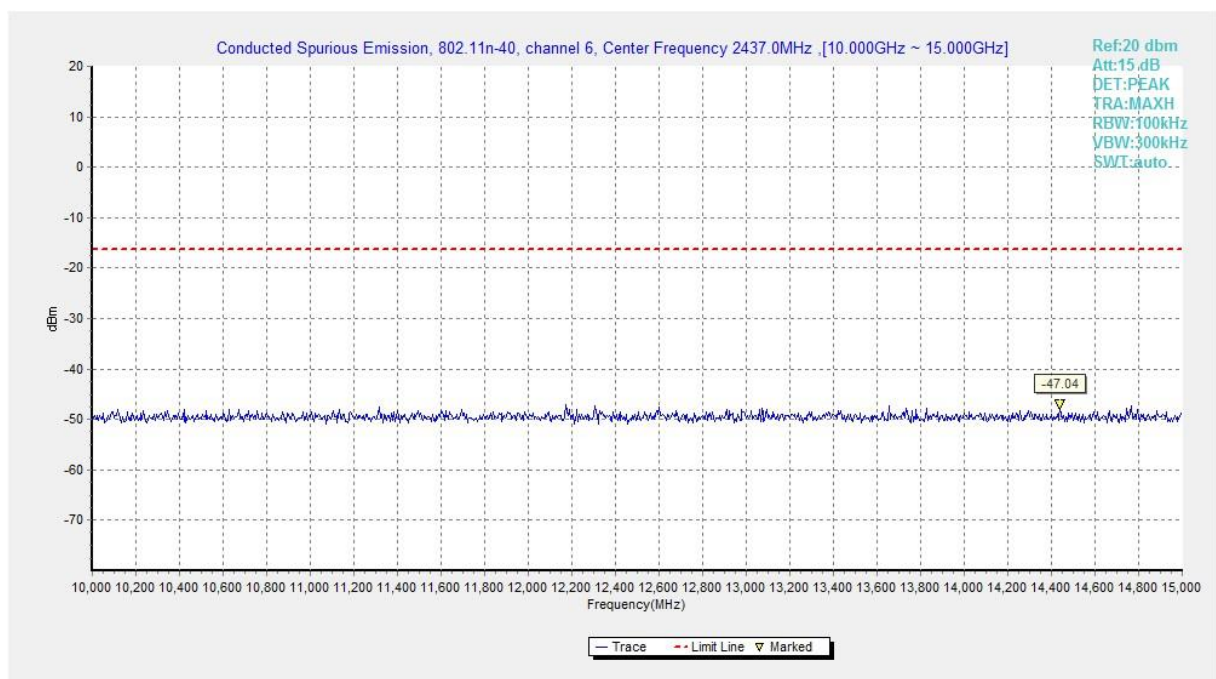
Fig.A.6.1.254 Transmitter Spurious Emission - Conducted (802.11n-HT40, Ch6, 10 GHz-15 GHz)
