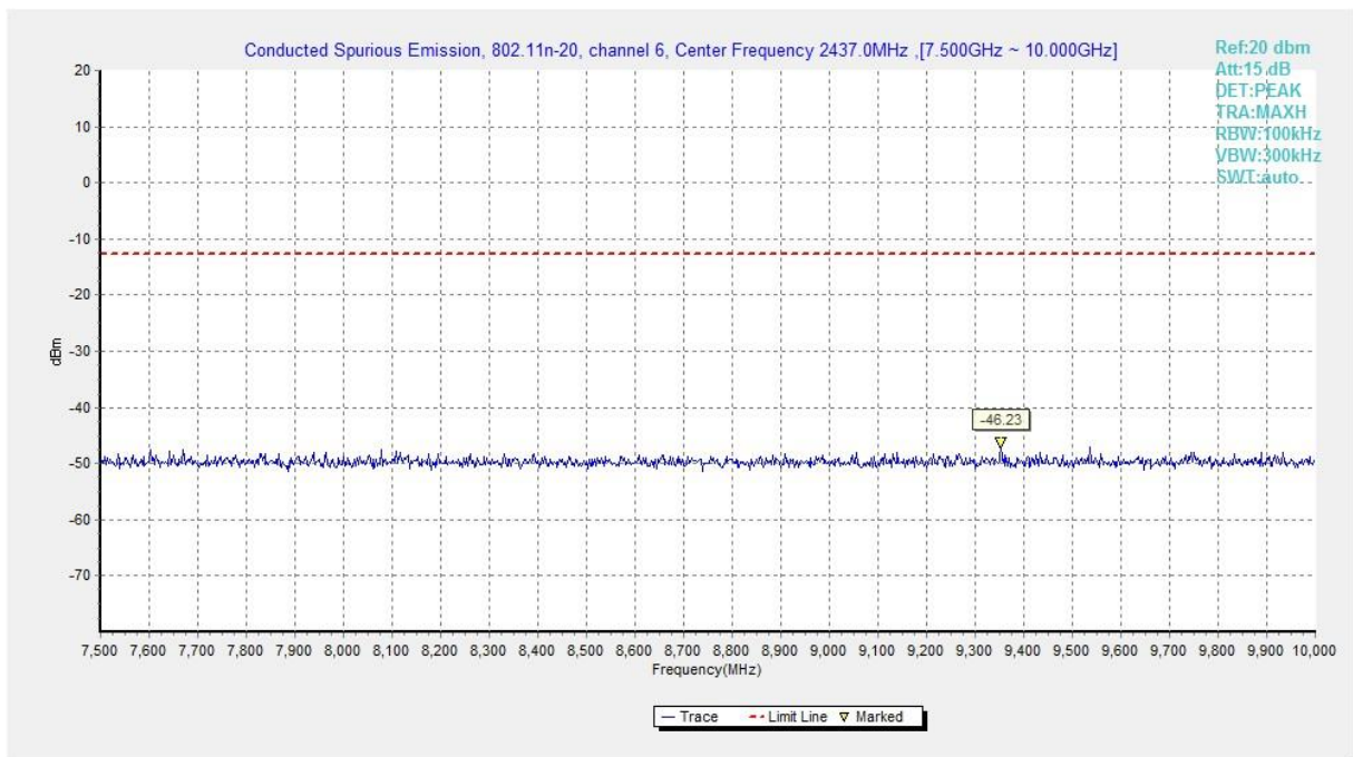
Fig.A.6.1.229 Transmitter Spurious Emission - Conducted (802.11n-HT20, Ch6, 7.5 GHz-10 GHz)
