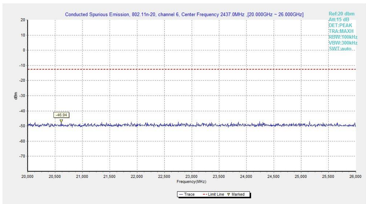
Fig.A.6.1.232 Transmitter Spurious Emission - Conducted (802.11n-HT20, Ch6, 20 GHz-26 GHz)
