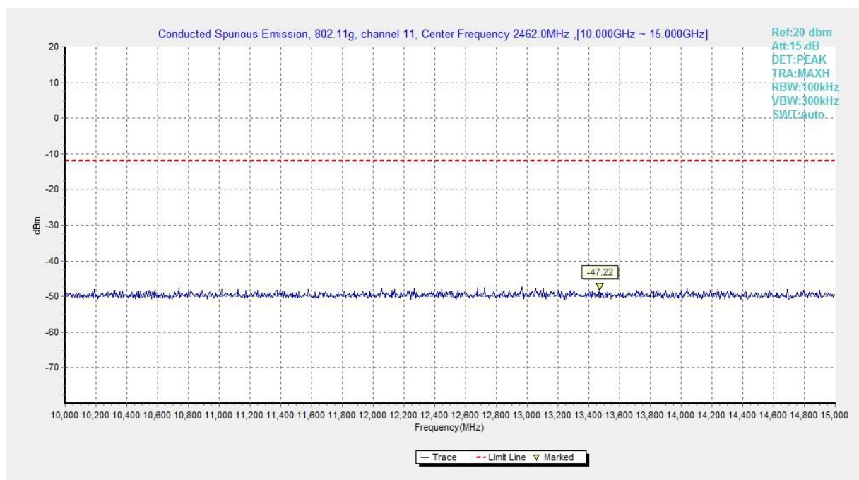
Fig.A.6.1.214 Transmitter Spurious Emission - Conducted (802.11g, Ch11, 10 GHz-15 GHz)
