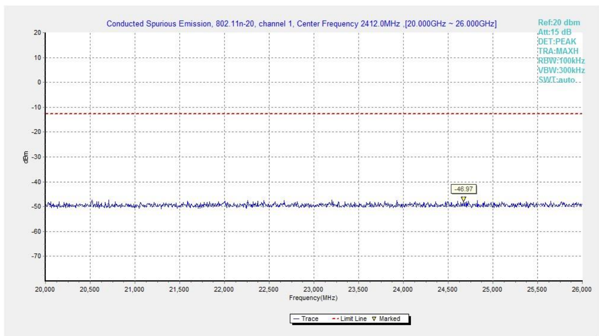
Fig.A.6.1.224 Transmitter Spurious Emission - Conducted (802.11n-HT20, Ch1, 20 GHz-26 GHz)
