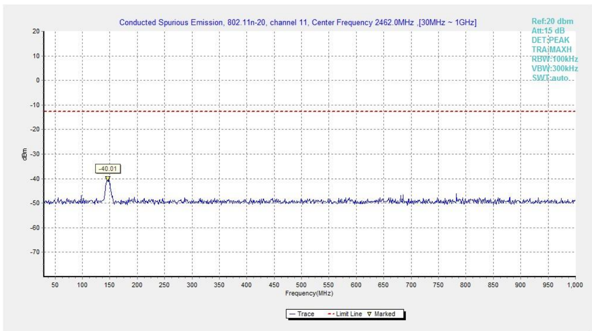
Fig.A.6.1.234 Transmitter Spurious Emission - Conducted (802.11n-HT20, Ch11, 30 MHz-1 GHz)
