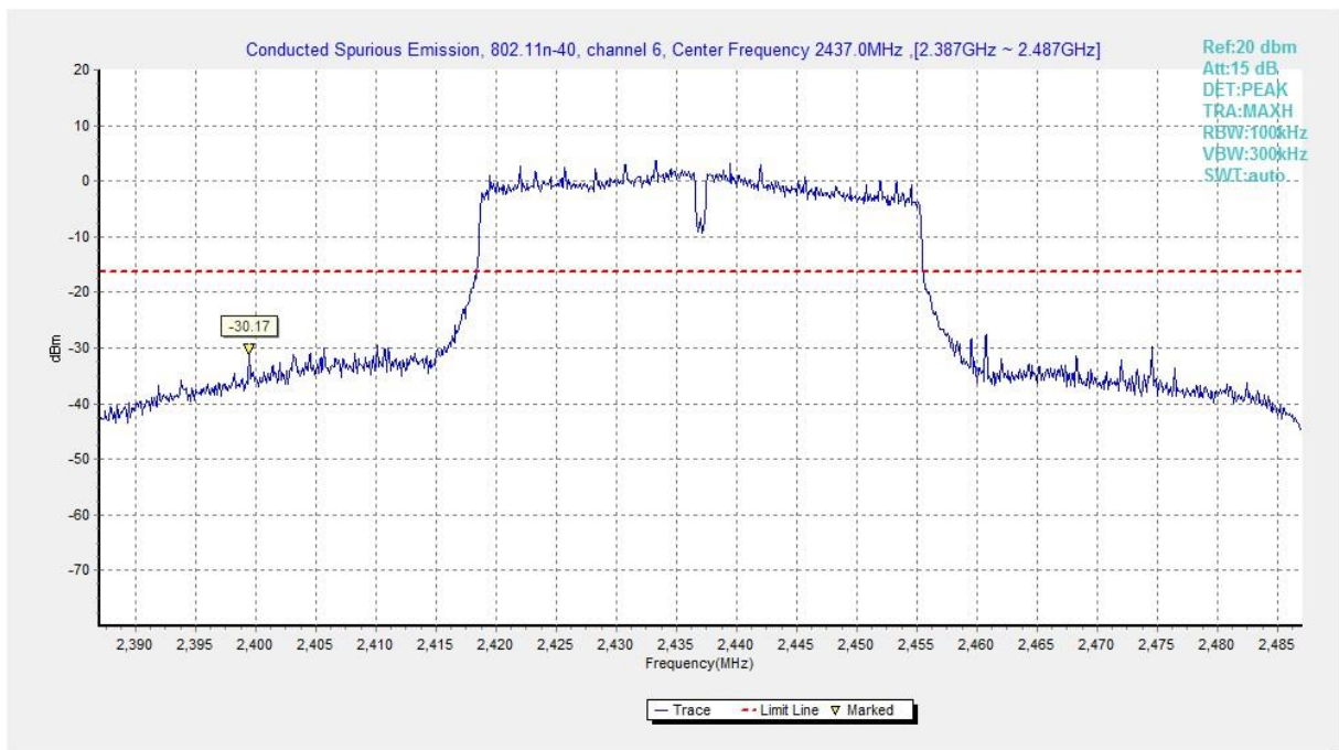
Fig.A.6.1.249 Transmitter Spurious Emission - Conducted (802.11n-HT40, Ch6, Center Frequency)
