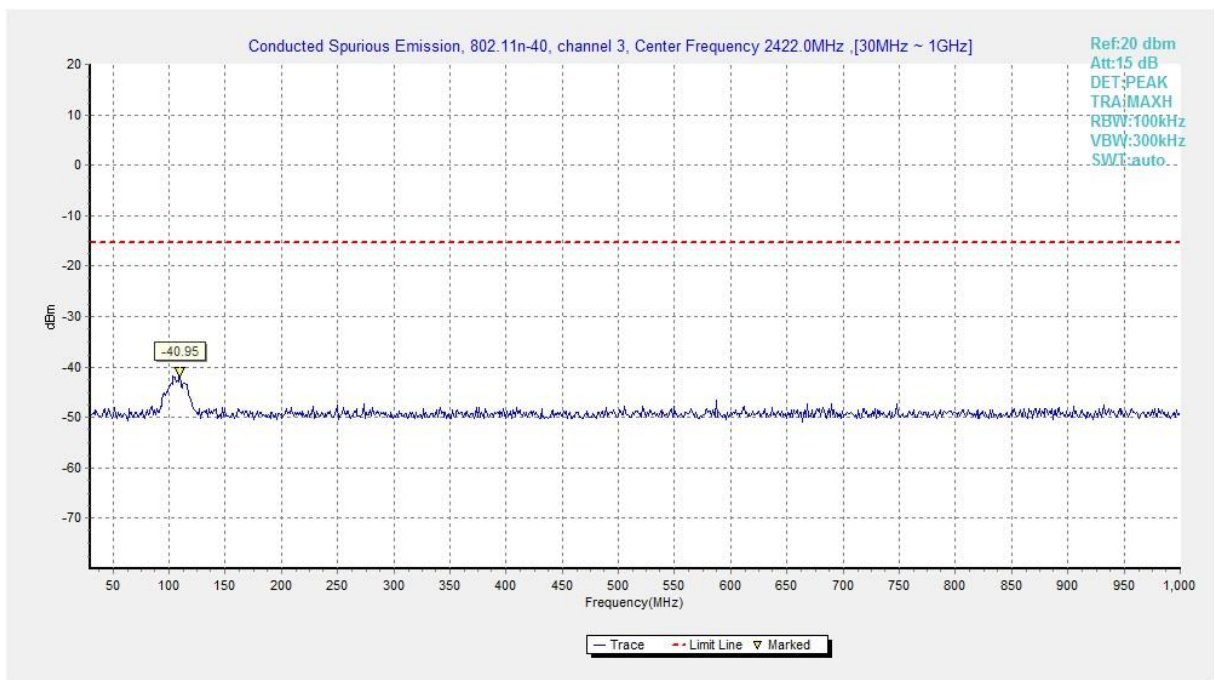
Fig.A.6.1.242 Transmitter Spurious Emission - Conducted (802.11n-HT40, Ch3, 30 MHz-1 GHz)
