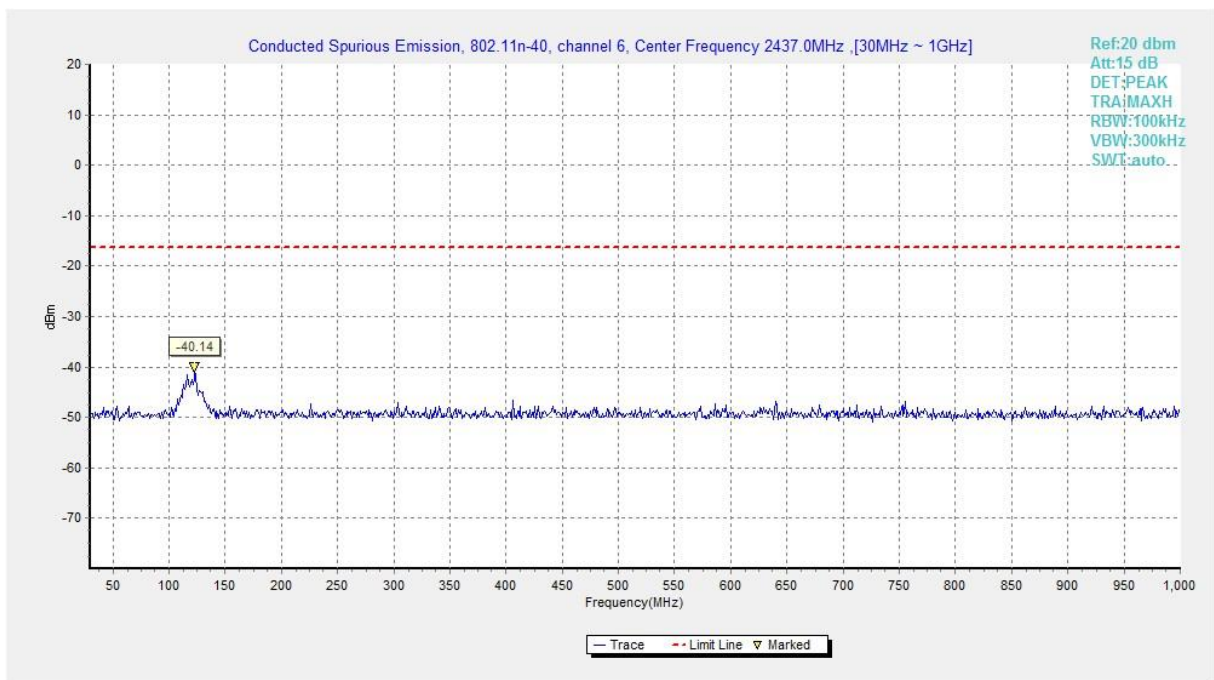
Fig.A.6.1.250 Transmitter Spurious Emission - Conducted (802.11n-HT40, Ch6, 30 MHz-1 GHz)
