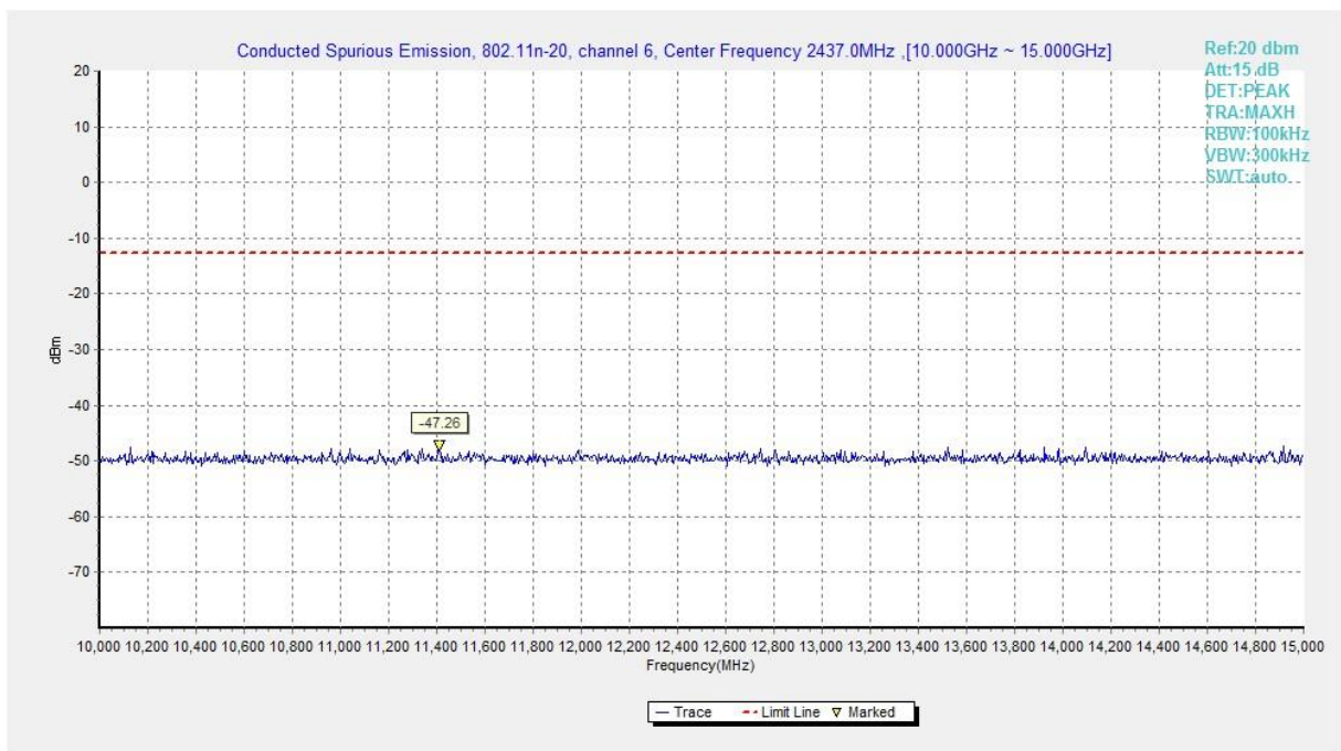
Fig.A.6.1.230 Transmitter Spurious Emission - Conducted (802.11n-HT20, Ch6, 10 GHz-15 GHz)
