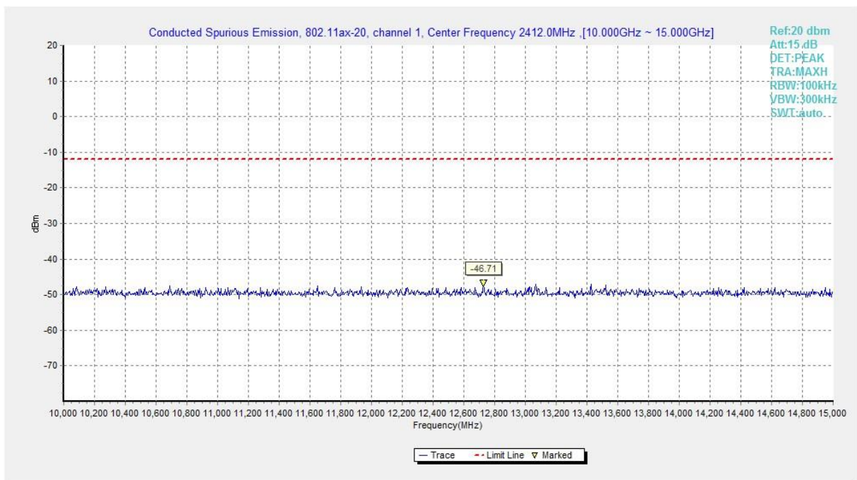
Fig.A.6.1.270 Transmitter Spurious Emission - Conducted (802.11ax-HE20, Ch1, 10 GHz-15 GHz)
