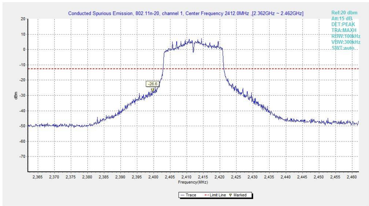
Fig.A.6.1.217 Transmitter Spurious Emission - Conducted (802.11n-HT20, Ch1, Center Frequency)
