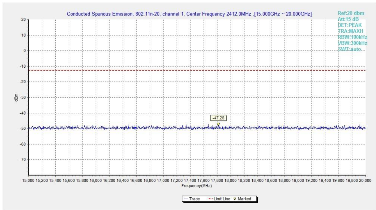
Fig.A.6.1.223 Transmitter Spurious Emission - Conducted (802.11n-HT20, Ch1, 15 GHz-20 GHz)
