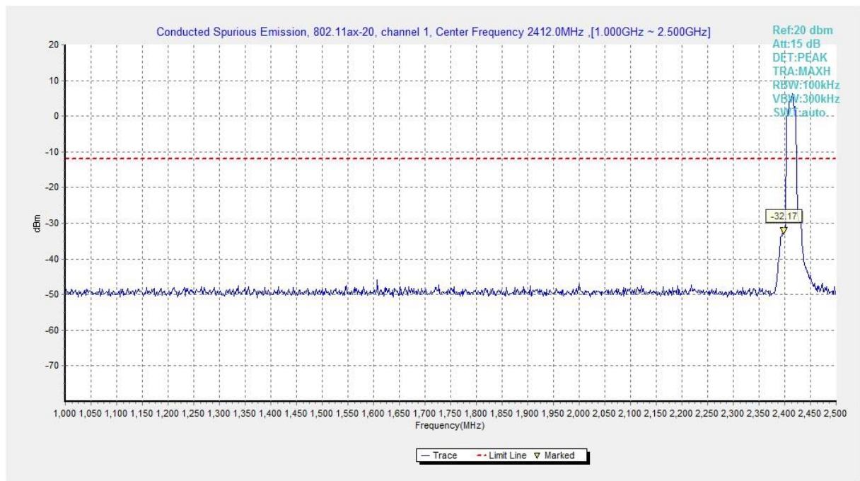
Fig.A.6.1.267 Transmitter Spurious Emission - Conducted (802.11ax-HE20, Ch1, 1 GHz-2.5 GHz)
