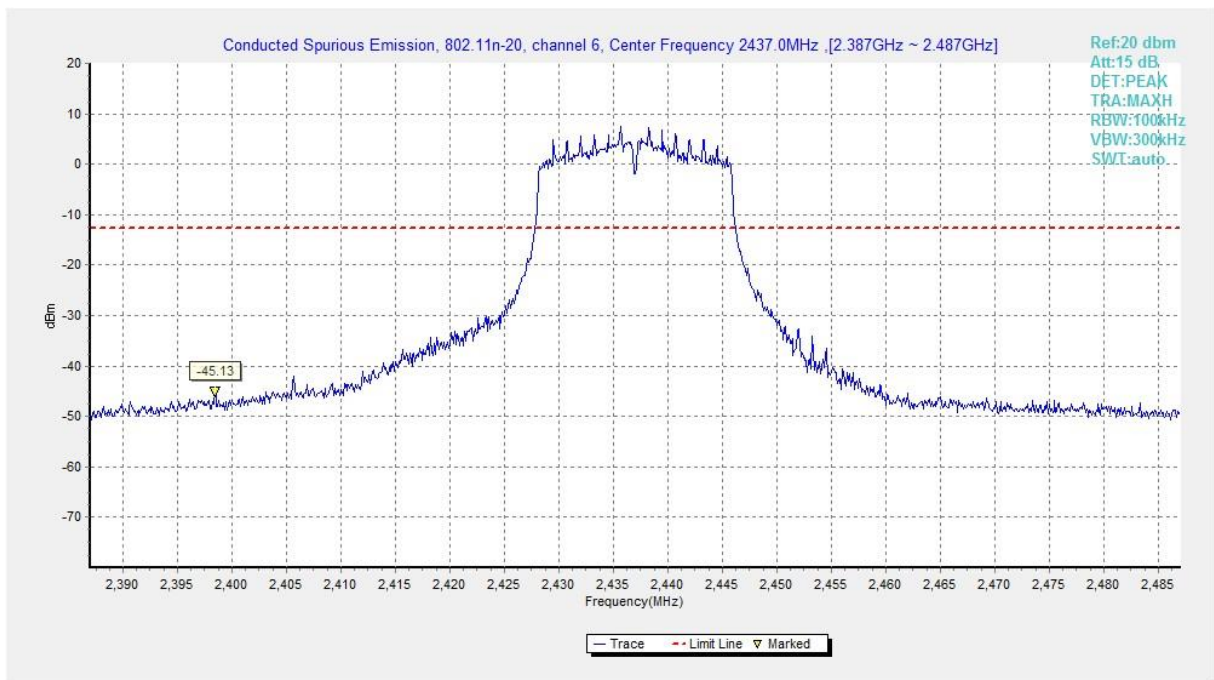
Fig.A.6.1.225 Transmitter Spurious Emission - Conducted (802.11n-HT20, Ch6, Center Frequency)
