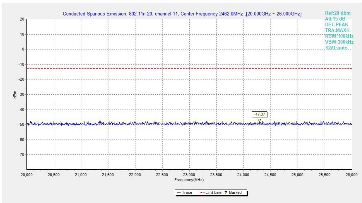
Fig.A.6.1.240 Transmitter Spurious Emission - Conducted (802.11n-HT20, Ch11, 20 GHz-26 GHz)
