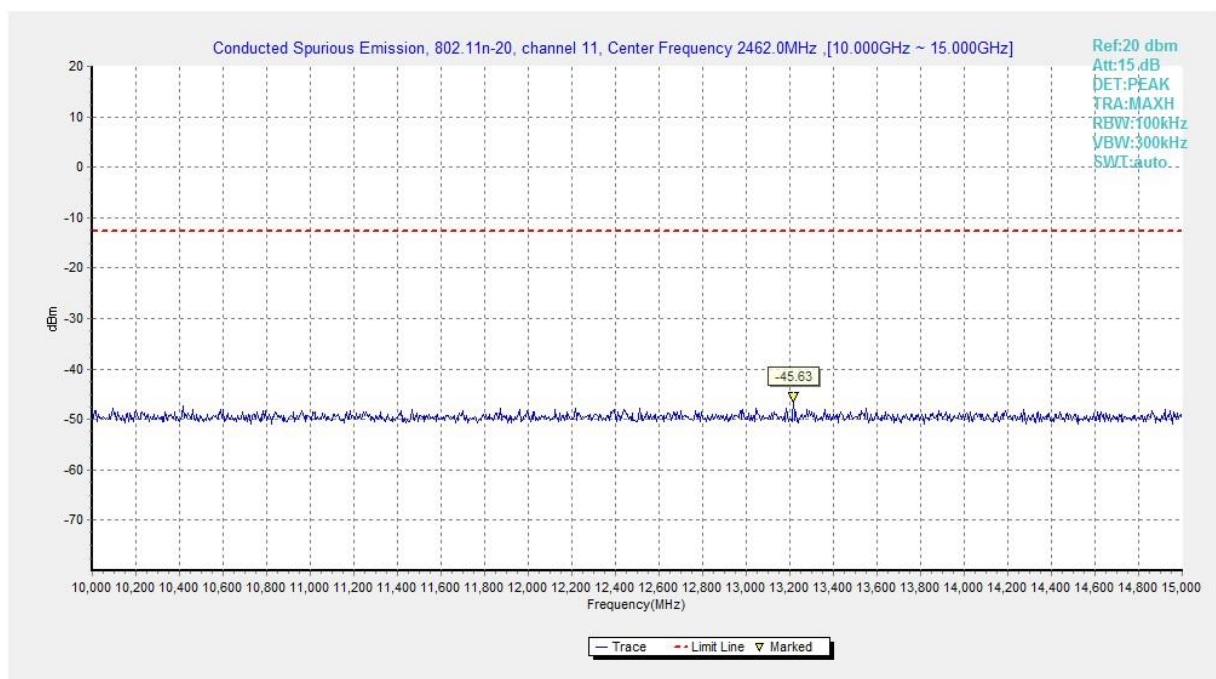
Fig.A.6.1.238 Transmitter Spurious Emission - Conducted (802.11n-HT20, Ch11, 10 GHz-15 GHz)
