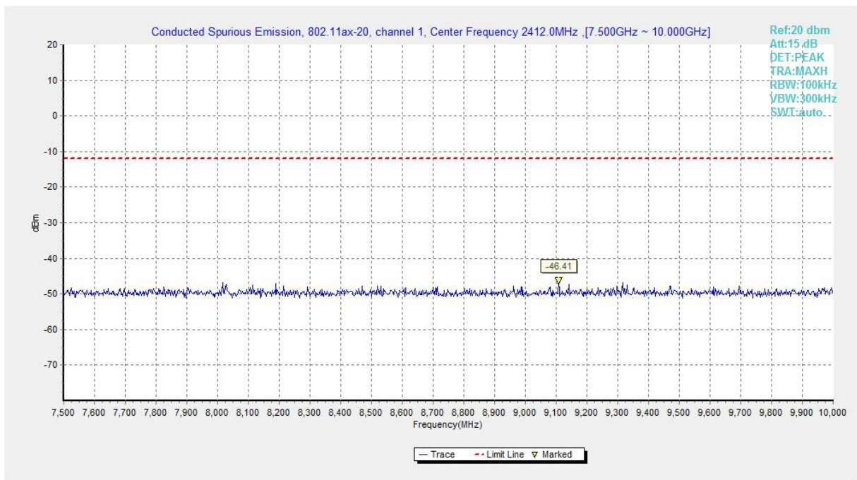
Fig.A.6.1.269 Transmitter Spurious Emission - Conducted (802.11ax-HE20, Ch1, 7.5 GHz-10 GHz)
