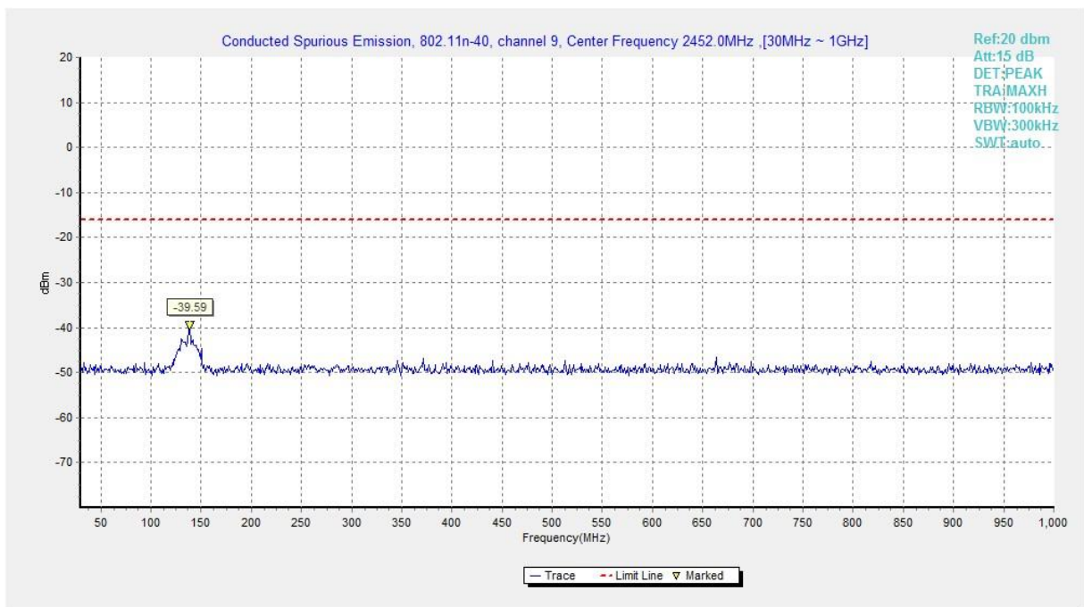
Fig.A.6.1.258 Transmitter Spurious Emission - Conducted (802.11n-HT40, Ch9, 30 MHz-1 GHz)
