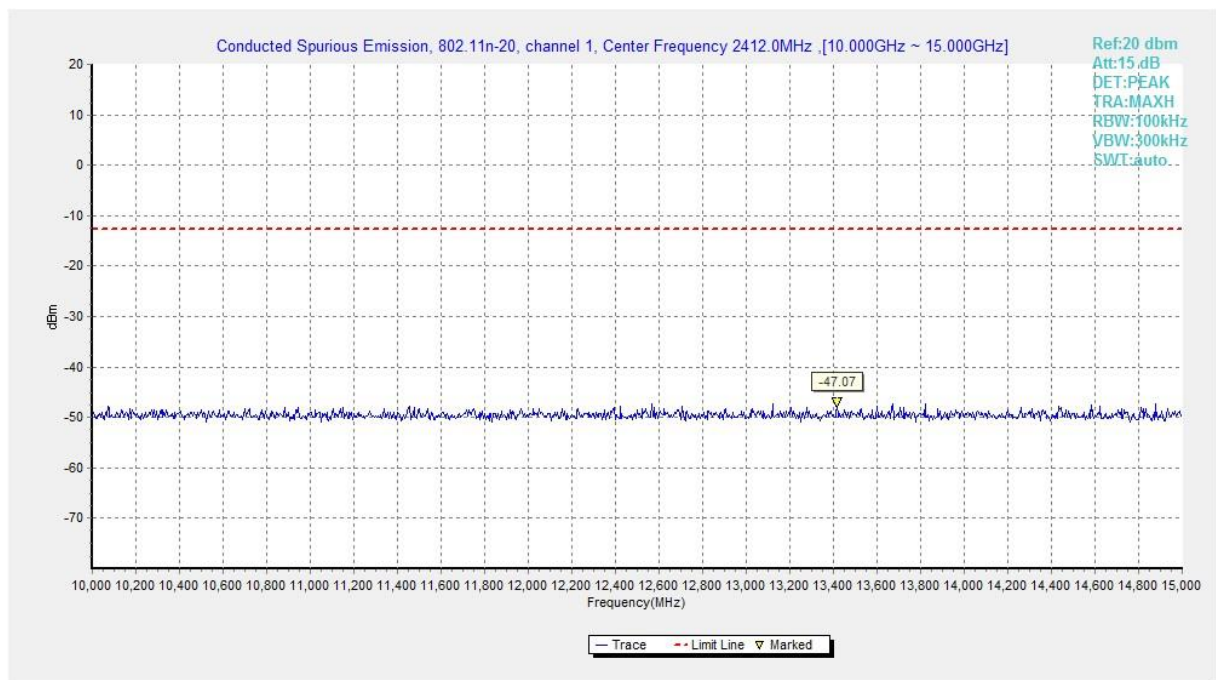
Fig.A.6.1.222 Transmitter Spurious Emission - Conducted (802.11n-HT20, Ch1, 10 GHz-15 GHz)
