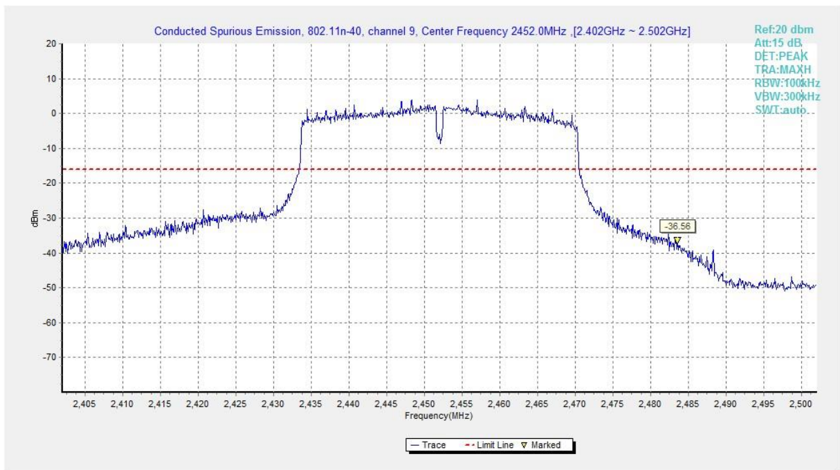
Fig.A.6.1.257 Transmitter Spurious Emission - Conducted (802.11n-HT40, Ch9, Center Frequency)
