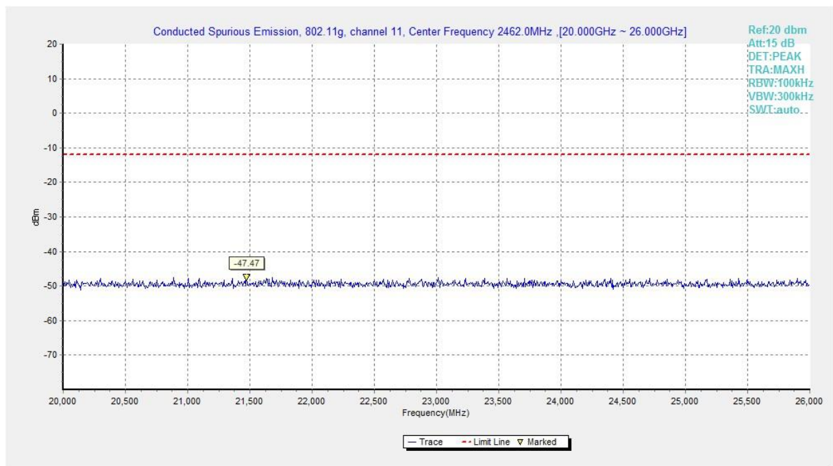
Fig.A.6.1.216 Transmitter Spurious Emission - Conducted (802.11g, Ch11, 20 GHz-26 GHz)
