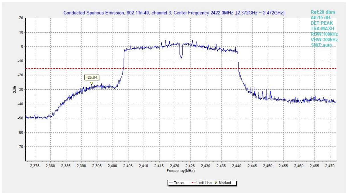
Fig.A.6.1.241 Transmitter Spurious Emission - Conducted (802.11n-HT40, Ch3, Center Frequency)
