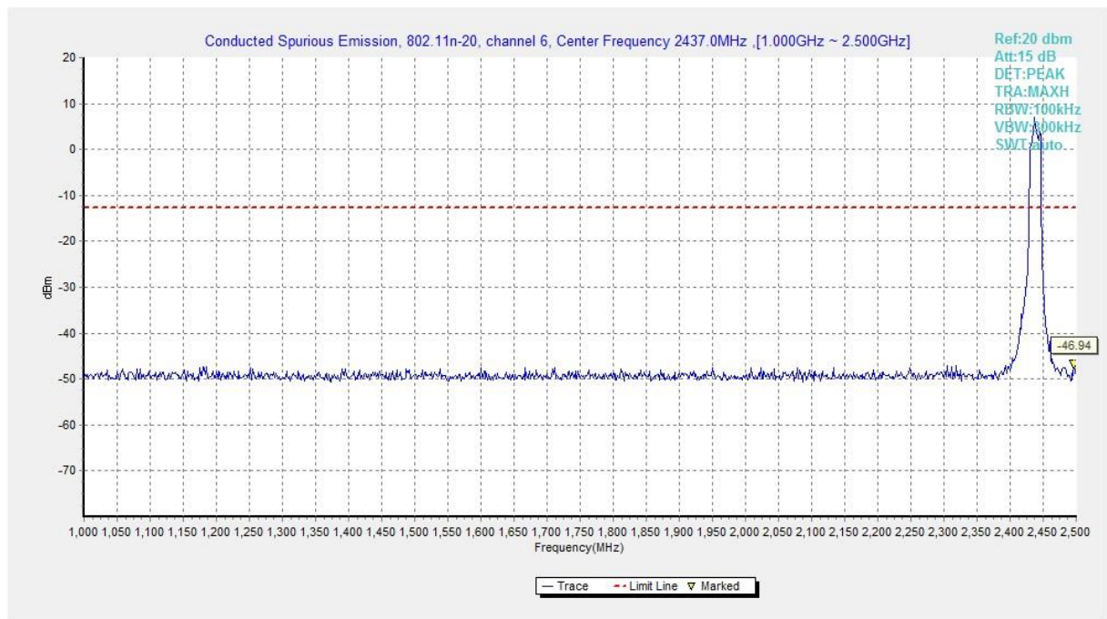
Fig.A.6.1.227 Transmitter Spurious Emission - Conducted (802.11n-HT20, Ch6, 1 GHz-2.5 GHz)
