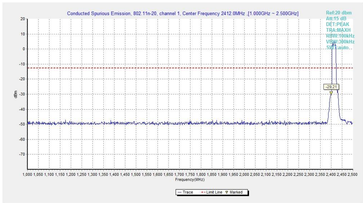
Fig.A.6.1.219 Transmitter Spurious Emission - Conducted (802.11n-HT20, Ch1, 1 GHz-2.5 GHz)
