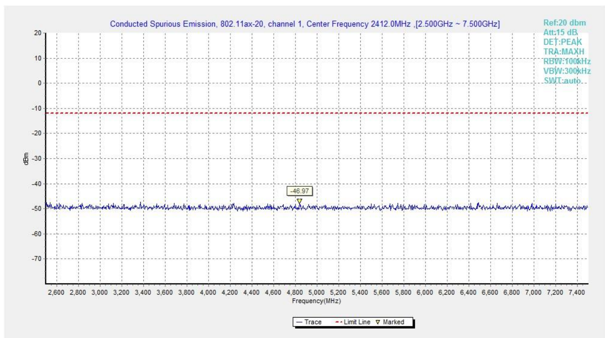
Fig.A.6.1.268 Transmitter Spurious Emission - Conducted (802.11ax-HE20, Ch1, 2.5 GHz-7.5 GHz)
