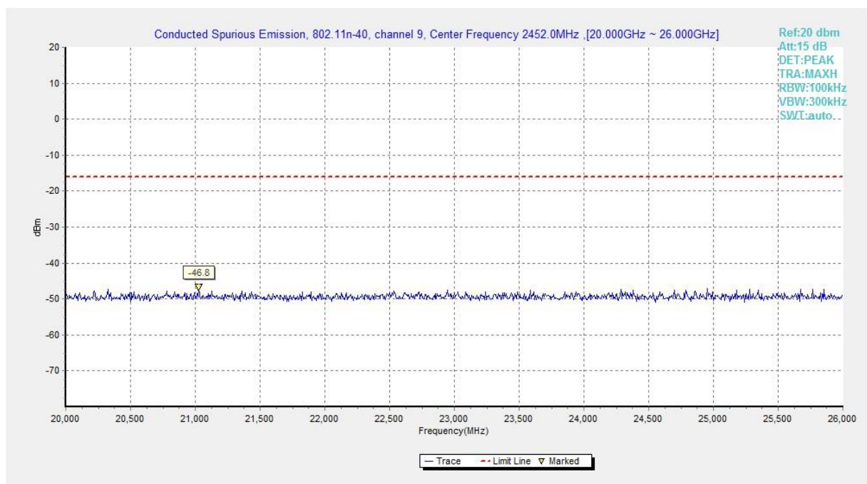
Fig.A.6.1.264 Transmitter Spurious Emission - Conducted (802.11n-HT40, Ch9, 20 GHz-26 GHz)
