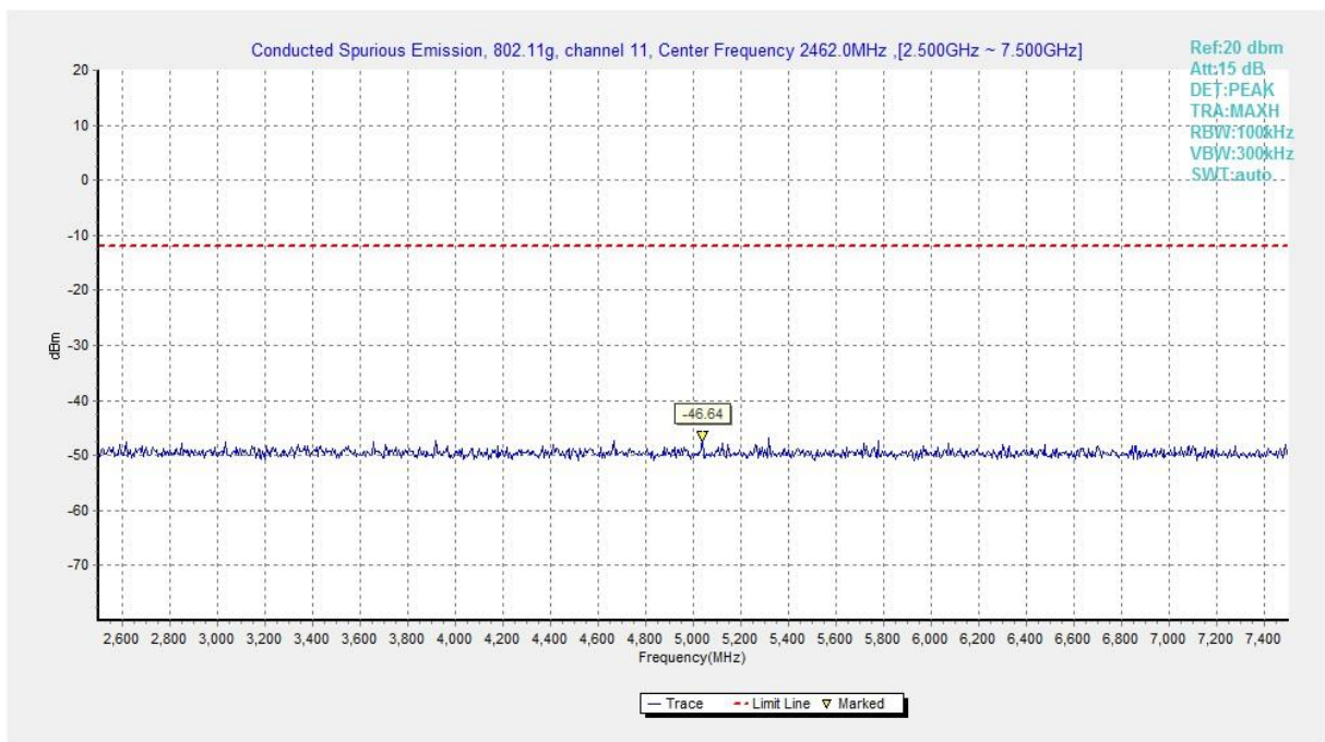
Fig.A.6.1.212 Transmitter Spurious Emission - Conducted (802.11g, Ch11, 2.5 GHz-7.5 GHz)
