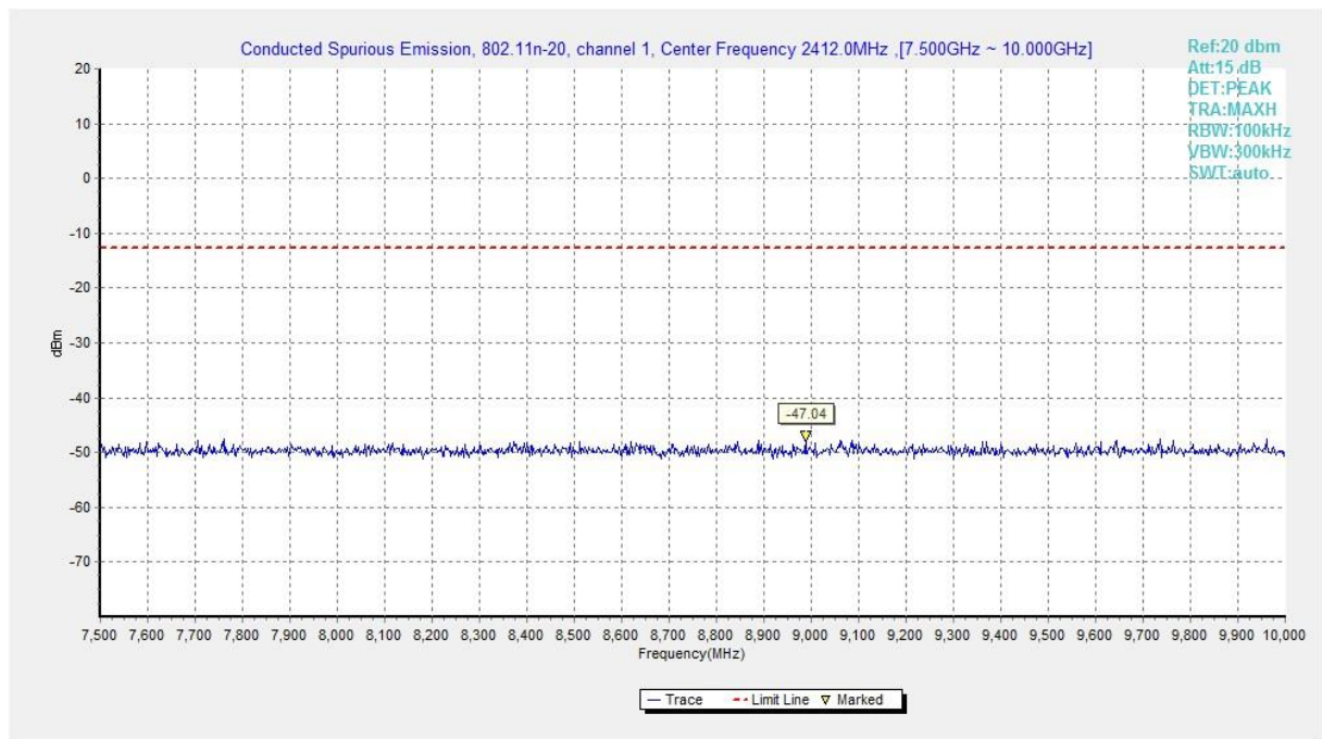
Fig.A.6.1.221 Transmitter Spurious Emission - Conducted (802.11n-HT20, Ch1, 7.5 GHz-10 GHz)
