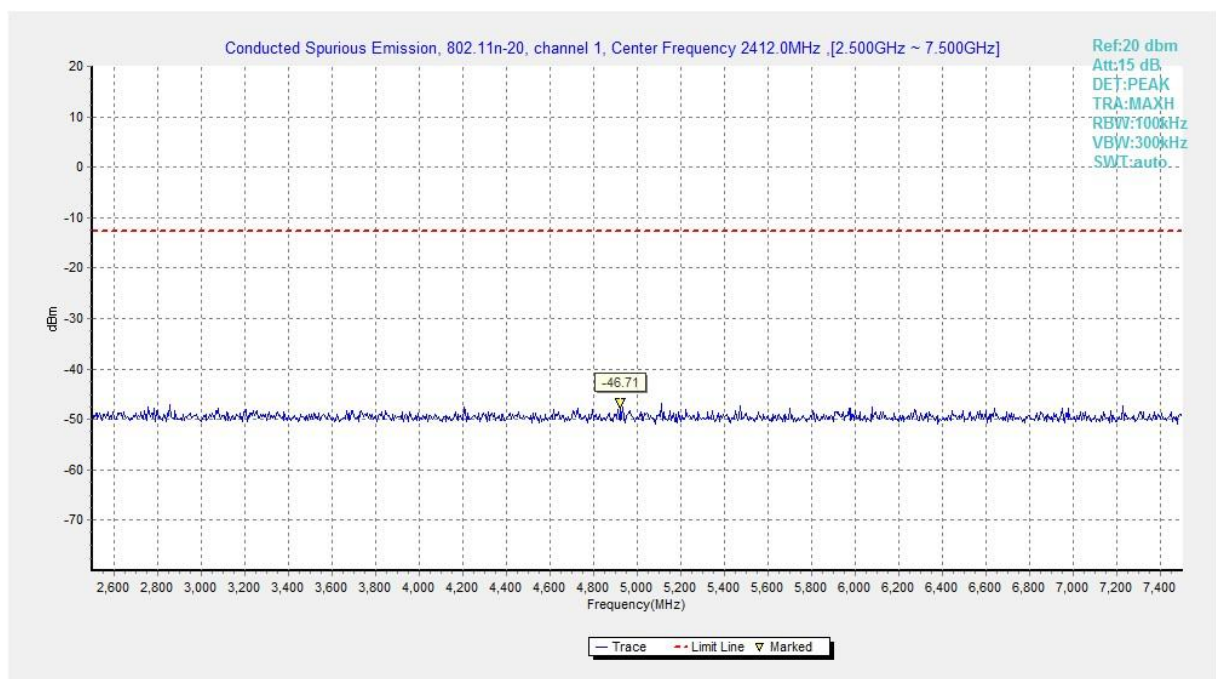
Fig.A.6.1.220 Transmitter Spurious Emission - Conducted (802.11n-HT20, Ch1, 2.5 GHz-7.5 GHz)
