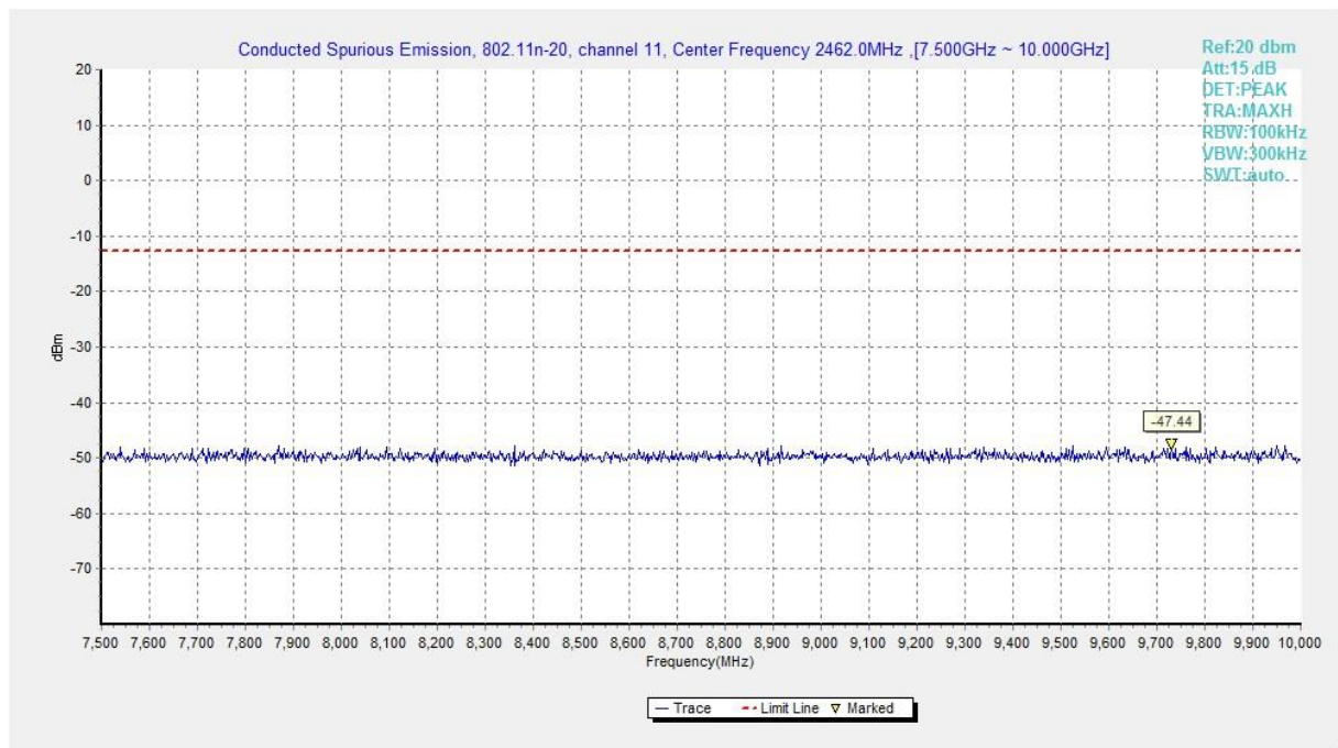
Fig.A.6.1.237 Transmitter Spurious Emission - Conducted (802.11n-HT20, Ch11, 7.5 GHz-10 GHz)
