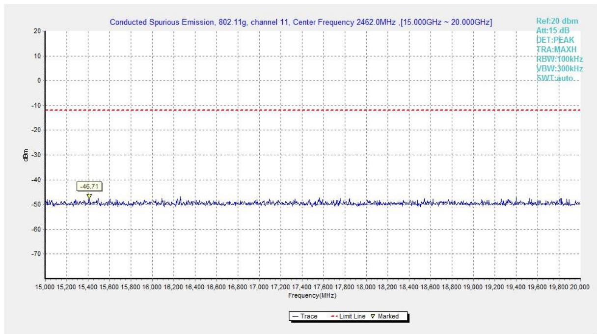
Fig.A.6.1.215 Transmitter Spurious Emission - Conducted (802.11g, Ch11, 15 GHz-20 GHz)
