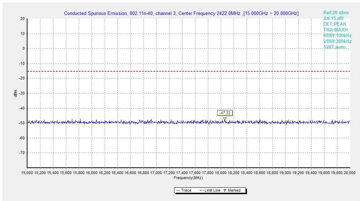
Fig.A.6.1.247 Transmitter Spurious Emission - Conducted (802.11n-HT40, Ch3, 15 GHz-20 GHz)
