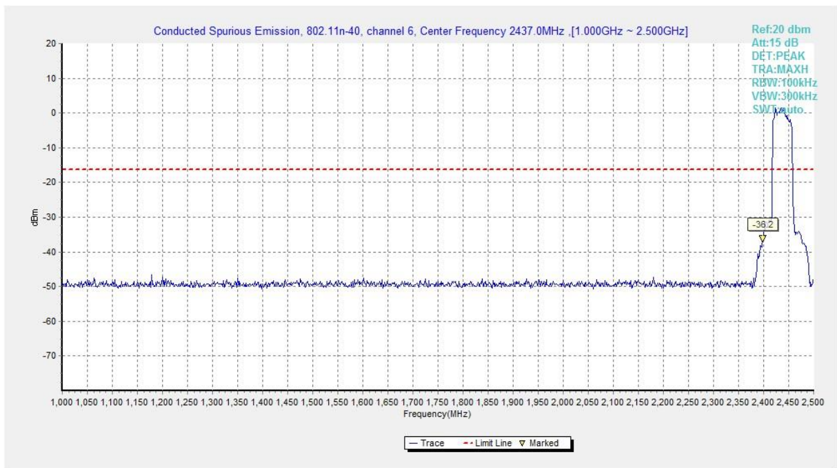
Fig.A.6.1.251 Transmitter Spurious Emission - Conducted (802.11n-HT40, Ch6, 1 GHz-2.5 GHz)
