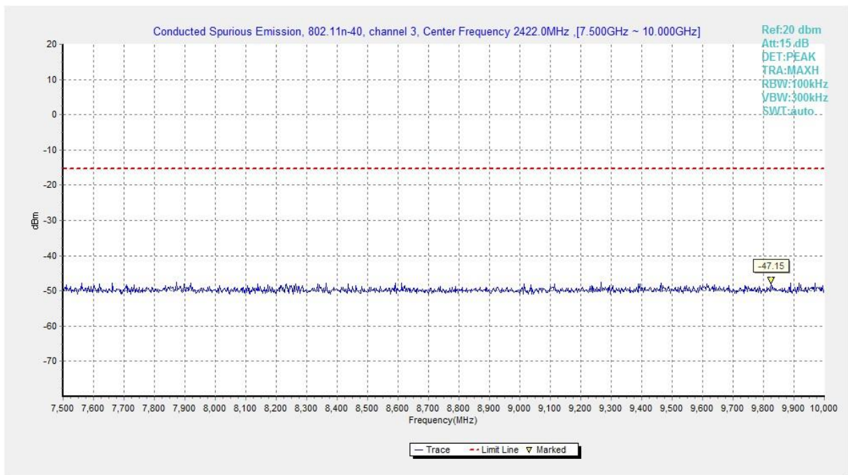
Fig.A.6.1.245 Transmitter Spurious Emission - Conducted (802.11n-HT40, Ch3, 7.5 GHz-10 GHz)
