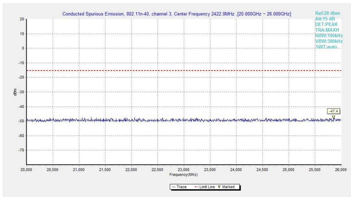
Fig.A.6.1.248 Transmitter Spurious Emission - Conducted (802.11n-HT40, Ch3, 20 GHz-26 GHz)
