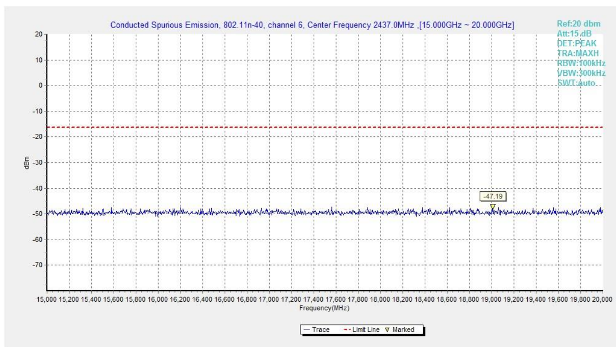
Fig.A.6.1.255 Transmitter Spurious Emission - Conducted (802.11n-HT40, Ch6, 15 GHz-20 GHz)
