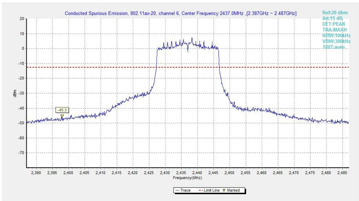
Fig.A.6.1.273 Transmitter Spurious Emission - Conducted (802.11ax-HE20, Ch6, Center Frequency)
