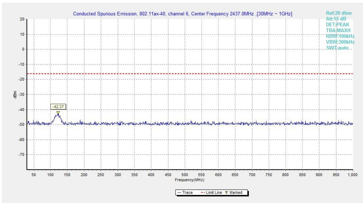
Fig.A.6.1.298 Transmitter Spurious Emission - Conducted (802.11ax-HE40, Ch6, 30 MHz-1 GHz)
