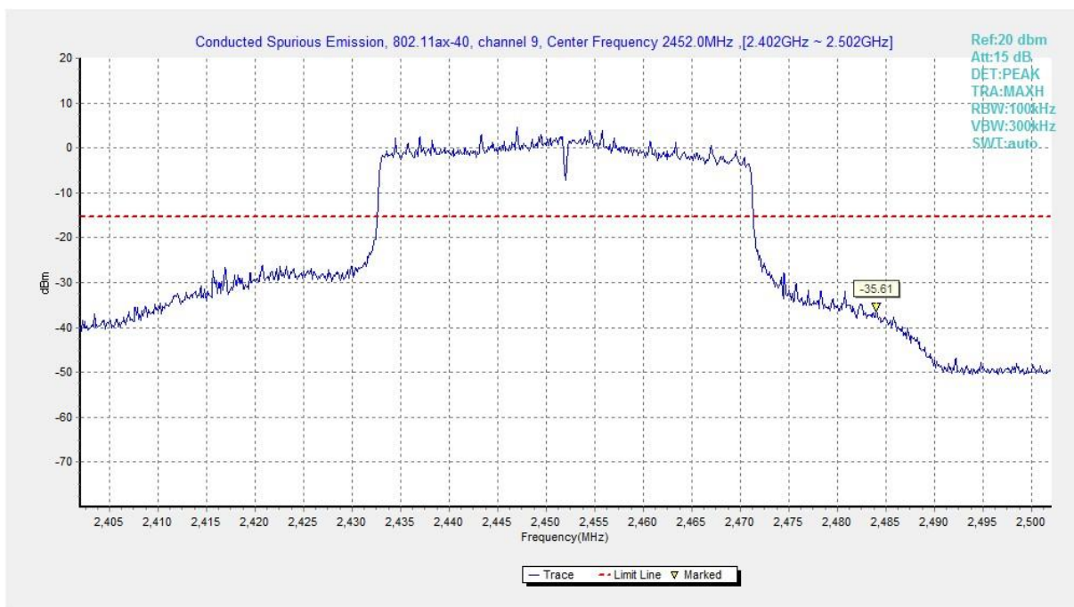
Fig.A.6.1.305 Transmitter Spurious Emission - Conducted (802.11ax-HE40, Ch9, Center Frequency)
