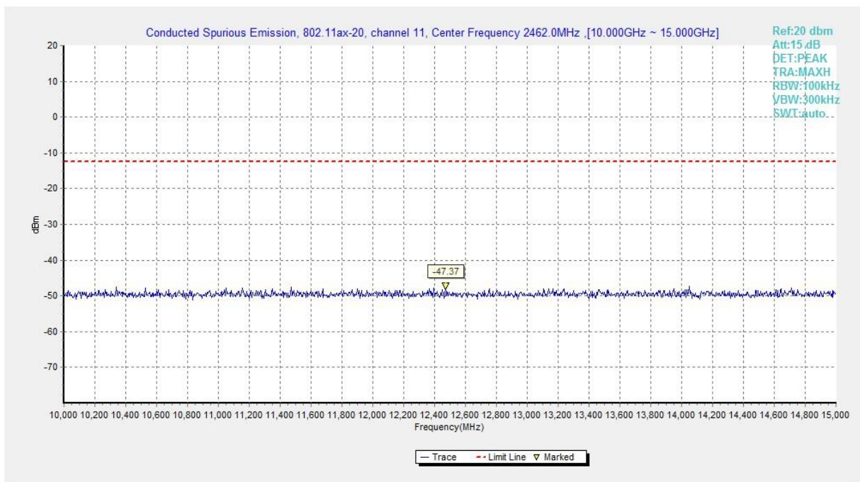
Fig.A.6.1.286 Transmitter Spurious Emission - Conducted (802.11ax-HE20, Ch11, 10 GHz-15 GHz)
