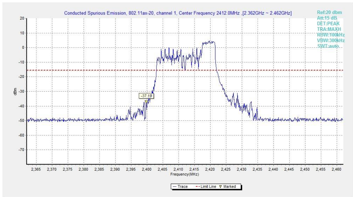
Fig.A.6.1.313 Transmitter Spurious Emission - Conducted (802.11ax-HE20-RU52-right, Ch1, Center Frequency)
