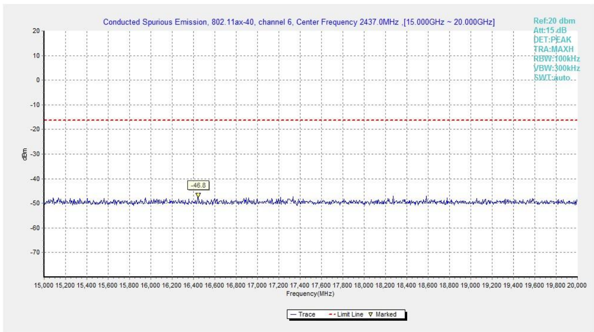
Fig.A.6.1.303 Transmitter Spurious Emission - Conducted (802.11ax-HE40, Ch6, 15 GHz-20 GHz)
