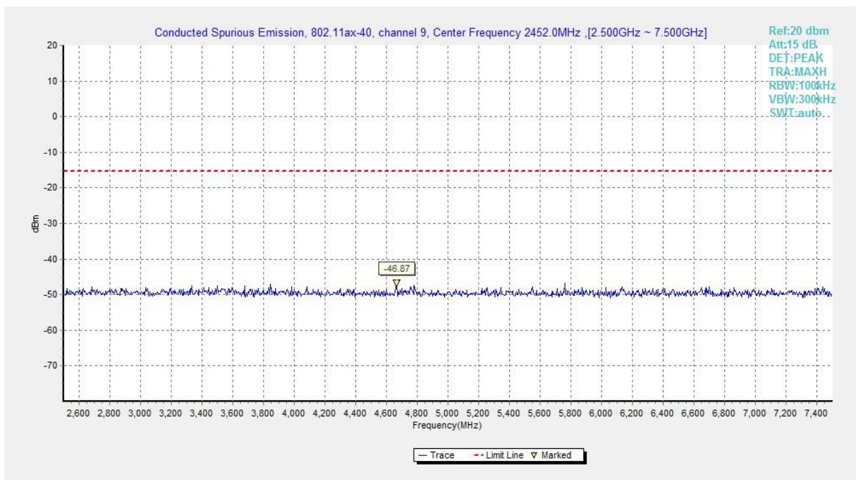
Fig.A.6.1.308 Transmitter Spurious Emission - Conducted (802.11ax-HE40, Ch9, 2.5 GHz-7.5 GHz)
