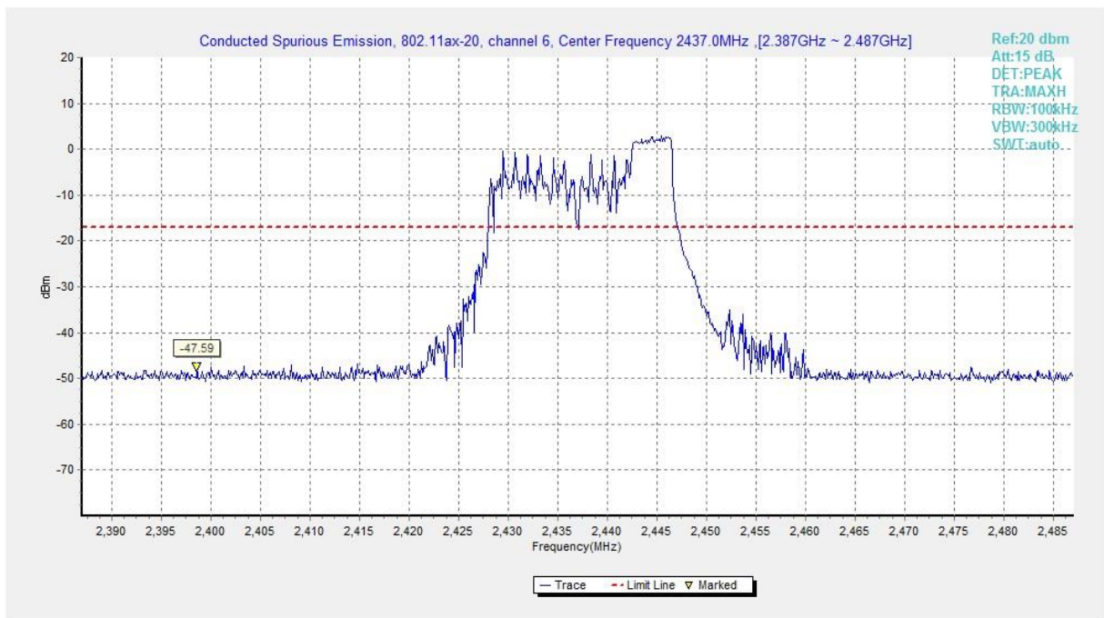
Fig.A.6.1.321 Transmitter Spurious Emission - Conducted (802.11ax-HE20-RU52-right, Ch6, Center Frequency)
