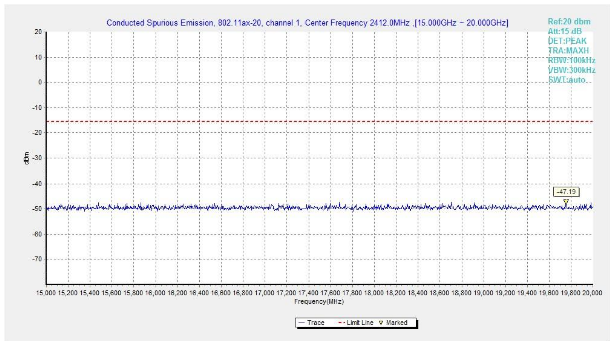
Fig.A.6.1.319 Transmitter Spurious Emission - Conducted (802.11ax-HE20-RU52-right, Ch1, 15 GHz-20 GHz)
