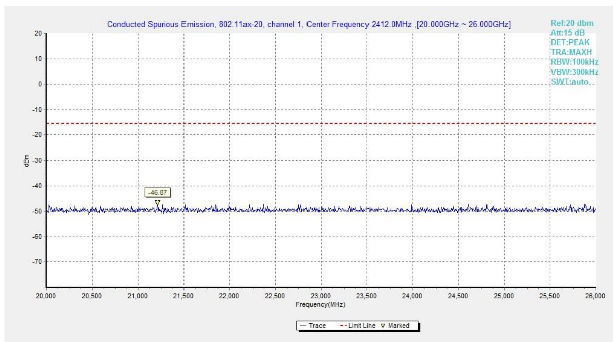
Fig.A.6.1.320 Transmitter Spurious Emission - Conducted (802.11ax-HE20-RU52-right, Ch1, 20 GHz-26 GHz)
