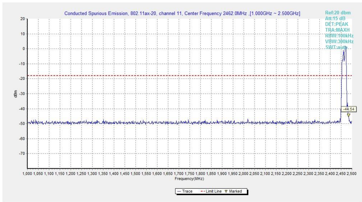
Fig.A.6.1.331 Transmitter Spurious Emission - Conducted (802.11ax-HE20-RU52-right, Ch11, 1 GHz-2.5 GHz)
