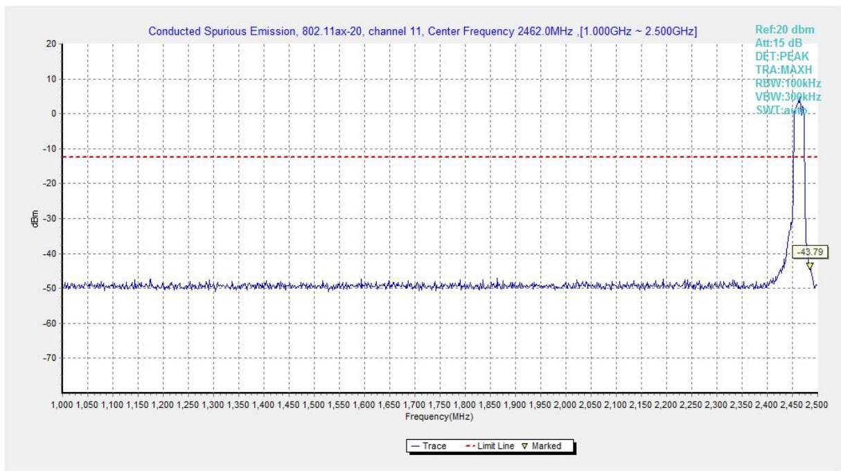
Fig.A.6.1.283 Transmitter Spurious Emission - Conducted (802.11ax-HE20, Ch11, 1 GHz-2.5 GHz)
