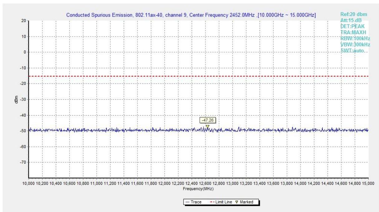
Fig.A.6.1.310 Transmitter Spurious Emission - Conducted (802.11ax-HE40, Ch9, 10 GHz-15 GHz)
