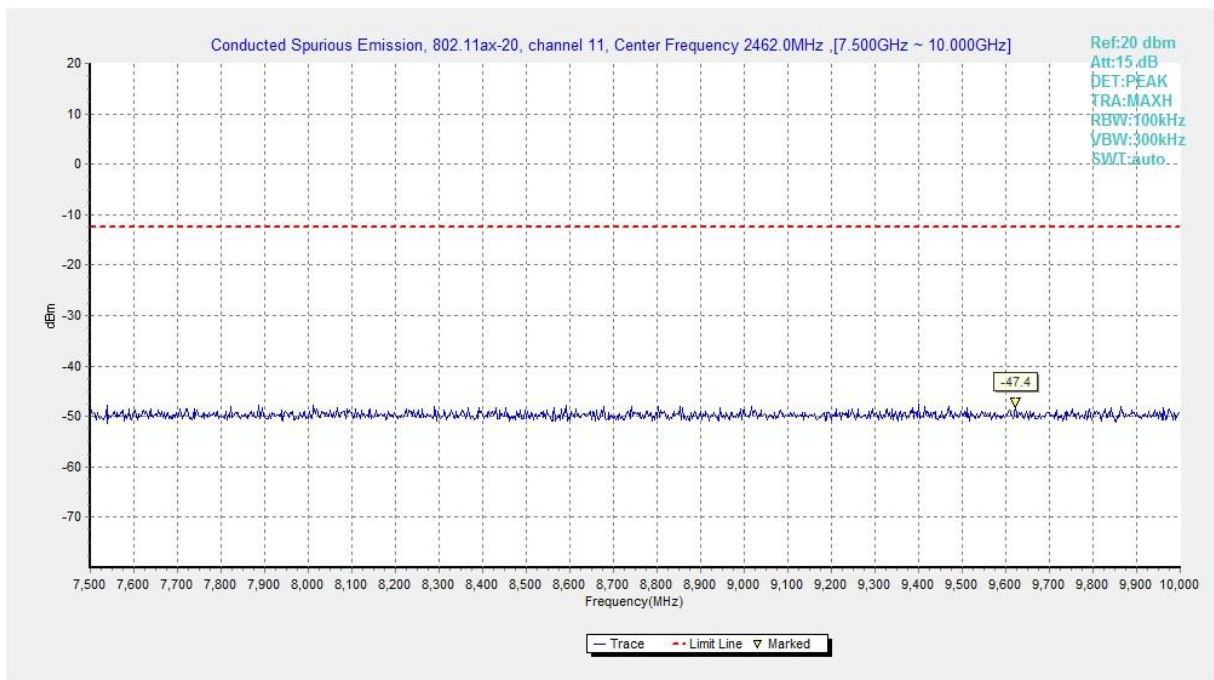
Fig.A.6.1.285 Transmitter Spurious Emission - Conducted (802.11ax-HE20, Ch11, 7.5 GHz-10 GHz)
