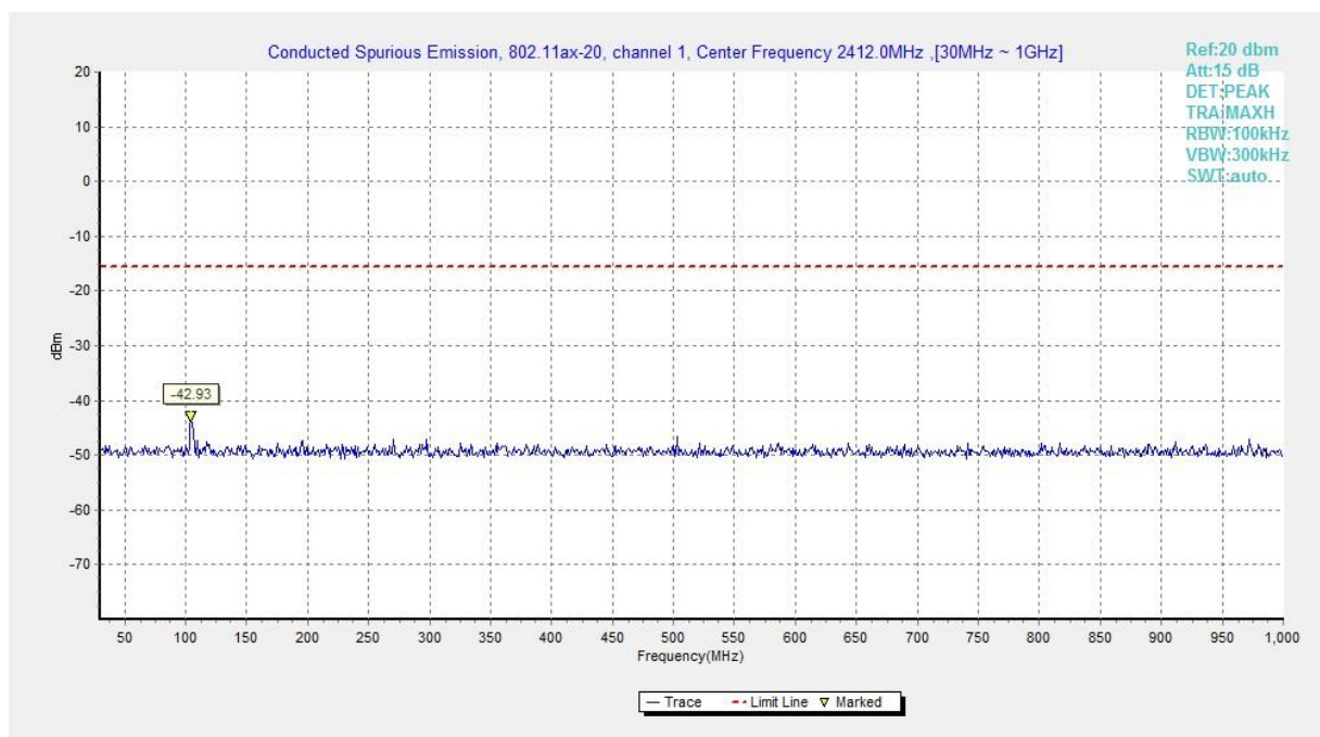
Fig.A.6.1.314 Transmitter Spurious Emission - Conducted (802.11ax-HE20-RU52-right, Ch1, 30 MHz-1 GHz)
