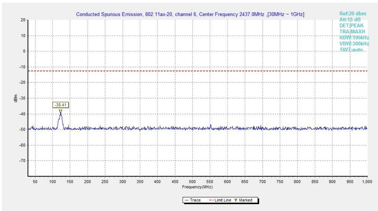
Fig.A.6.1.274 Transmitter Spurious Emission - Conducted (802.11ax-HE20, Ch6, 30 MHz-1 GHz)
