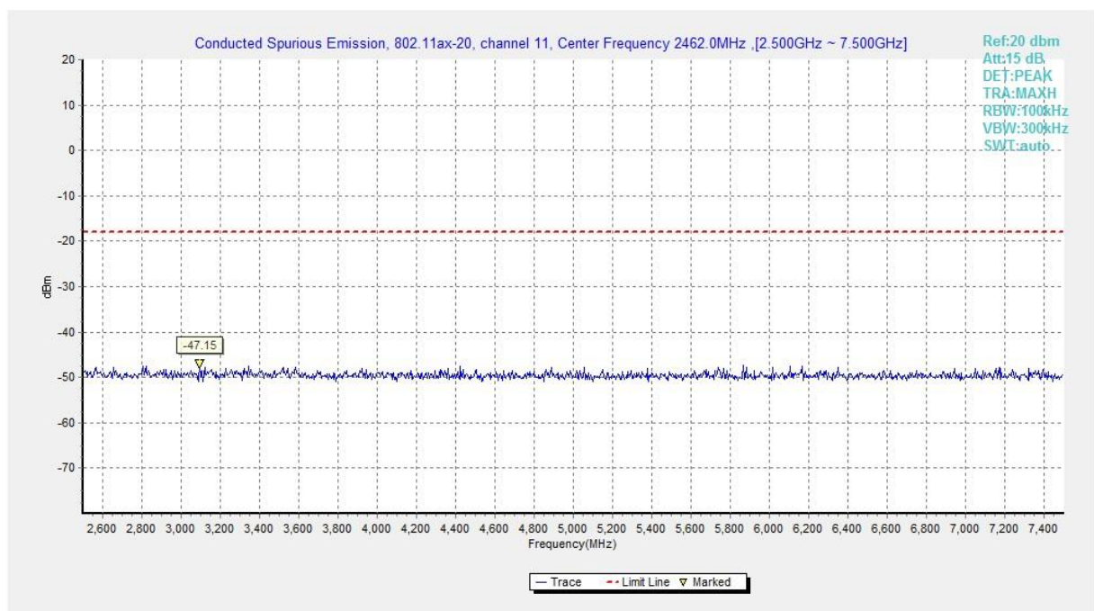
Fig.A.6.1.332 Transmitter Spurious Emission - Conducted (802.11ax-HE20-RU52-right, Ch11, 2.5 GHz-7.5 GHz)
