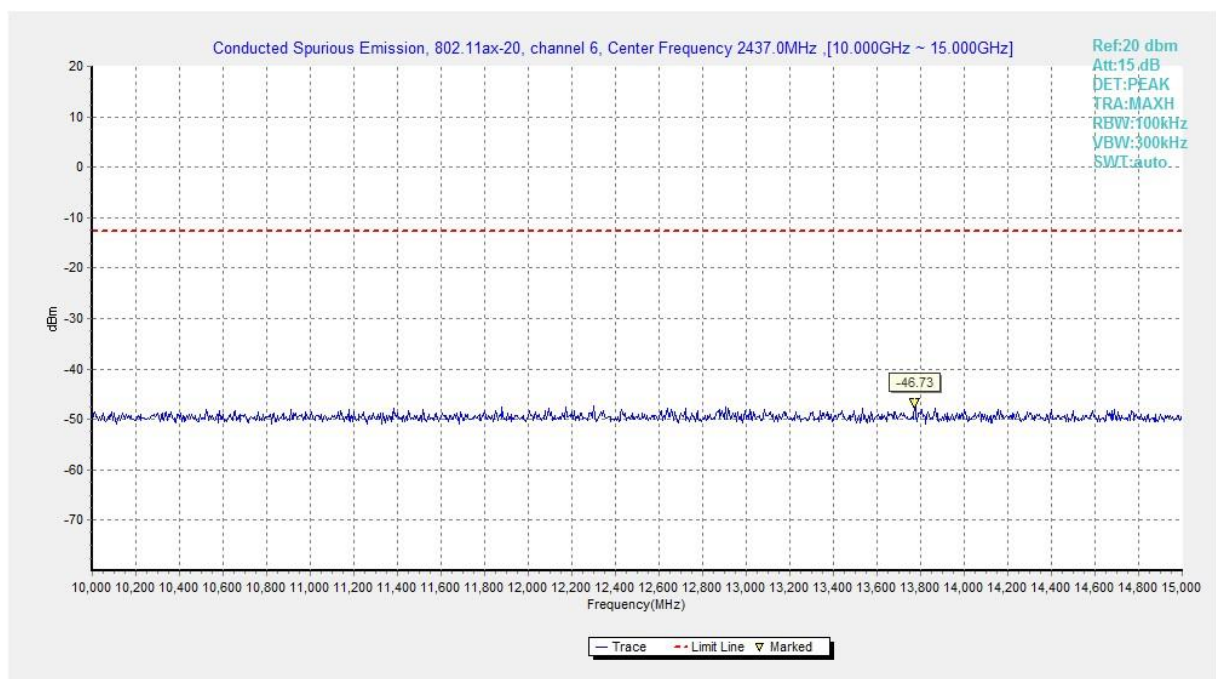
Fig.A.6.1.278 Transmitter Spurious Emission - Conducted (802.11ax-HE20, Ch6, 10 GHz-15 GHz)
