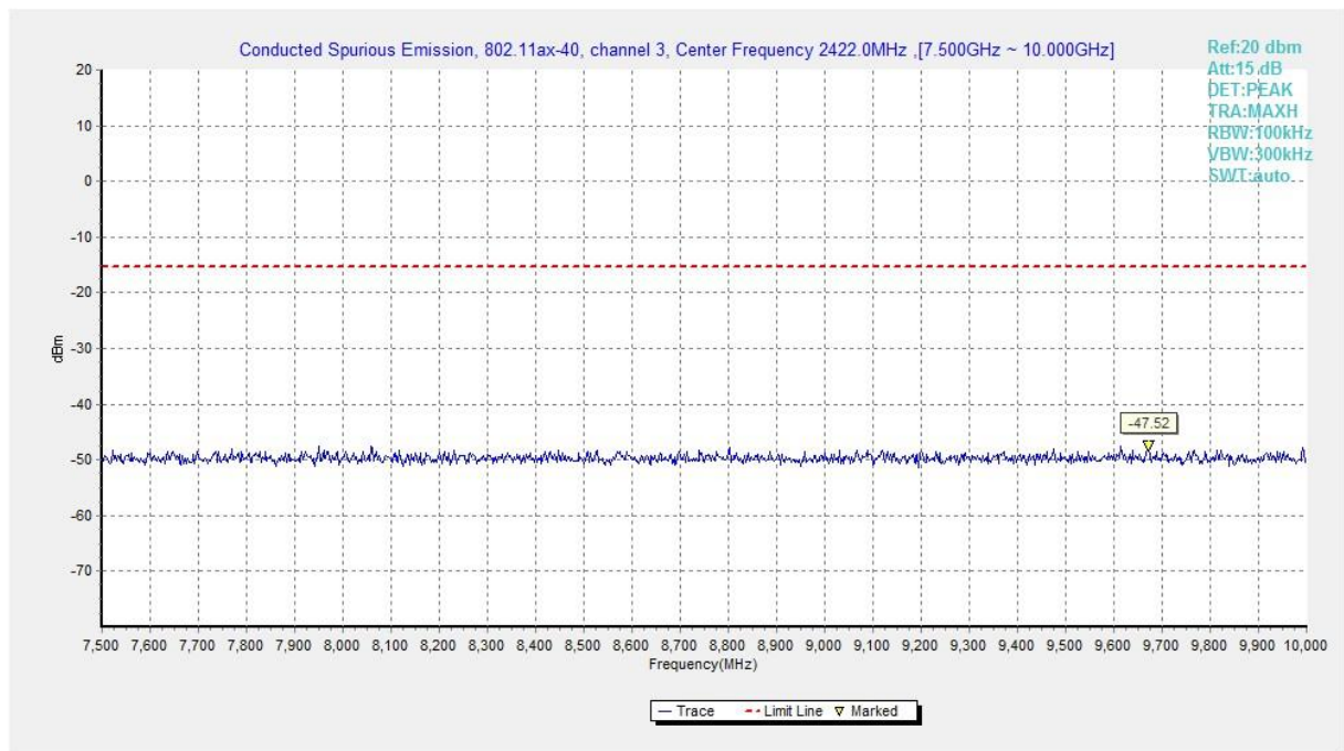
Fig.A.6.1.293 Transmitter Spurious Emission - Conducted (802.11ax-HE40, Ch3, 7.5 GHz-10 GHz)
