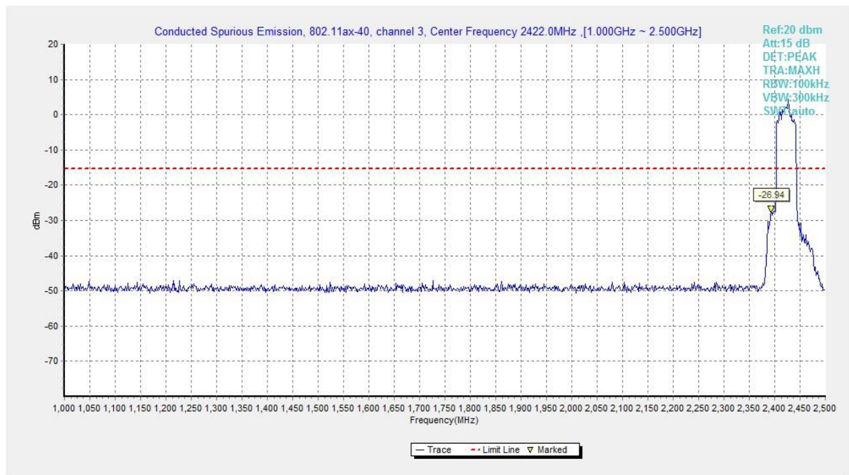
Fig.A.6.1.291 Transmitter Spurious Emission - Conducted (802.11ax-HE40, Ch3, 1 GHz-2.5 GHz)
