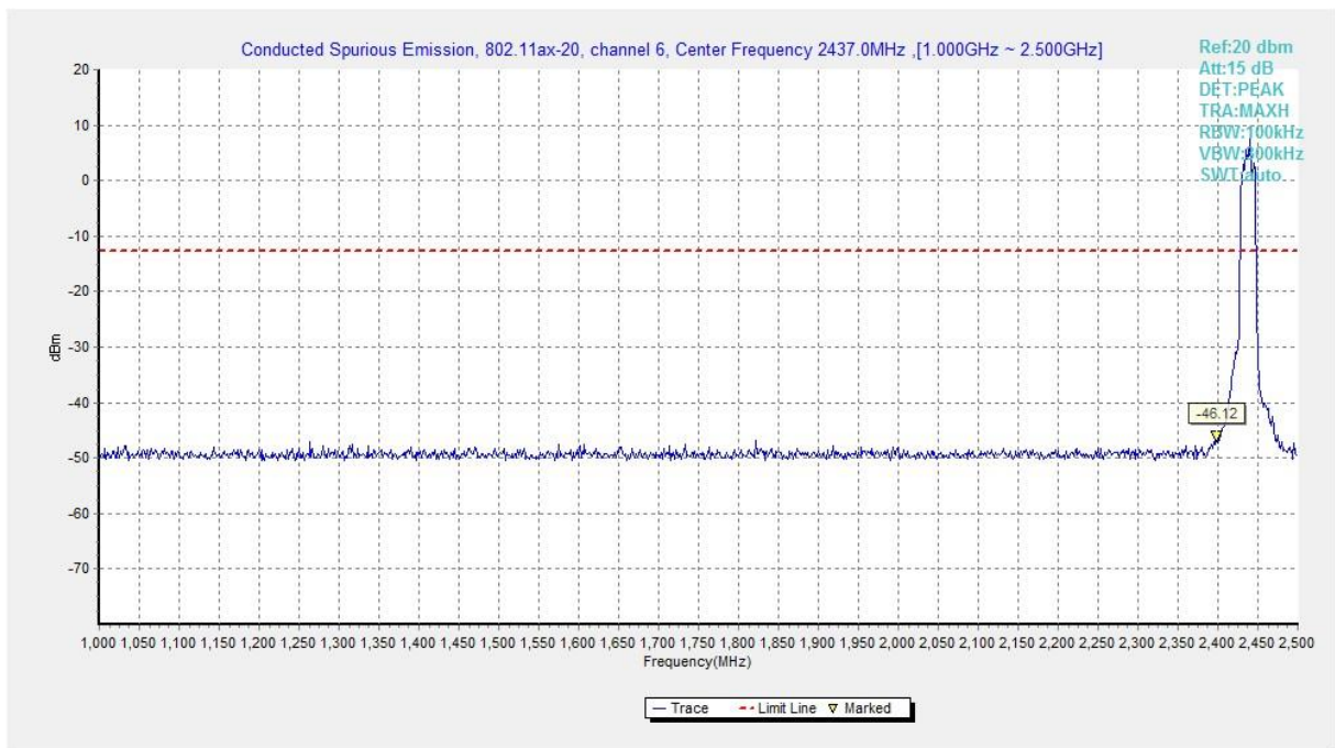
Fig.A.6.1.275 Transmitter Spurious Emission - Conducted (802.11ax-HE20, Ch6, 1 GHz-2.5 GHz)
