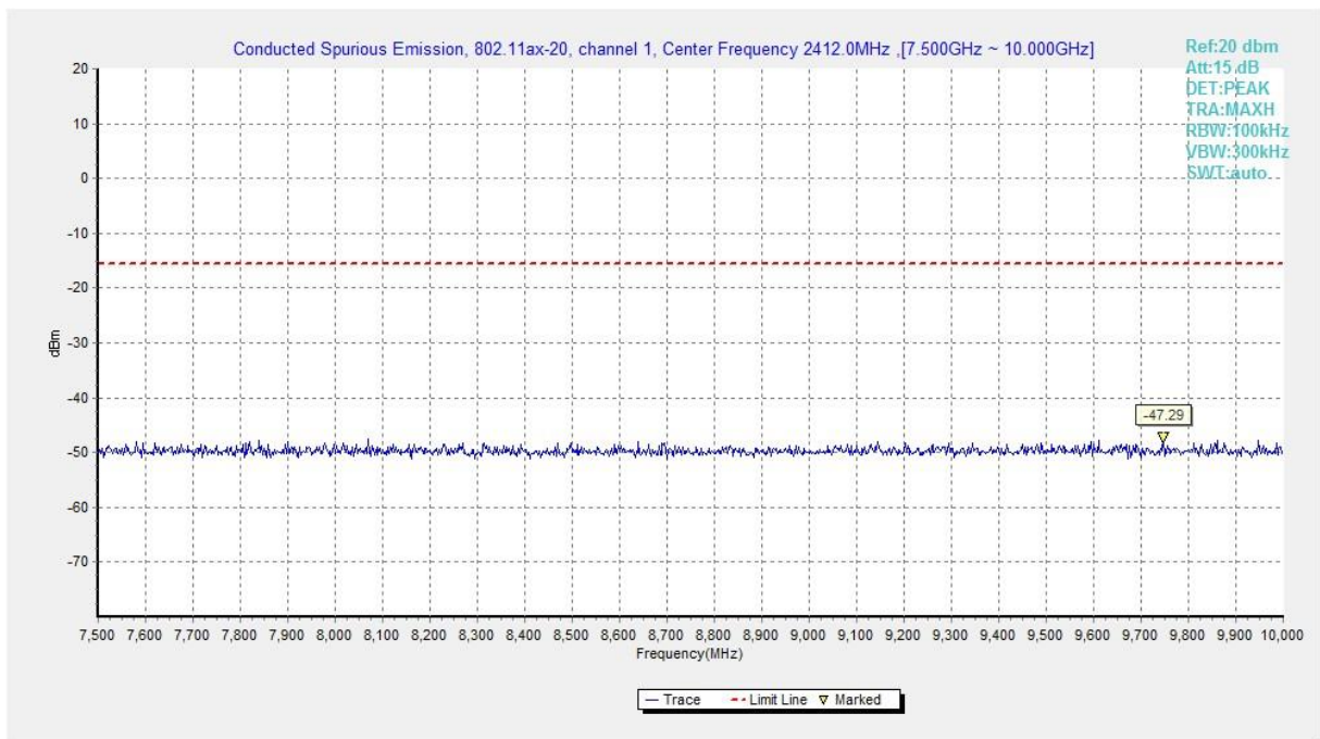
Fig.A.6.1.317 Transmitter Spurious Emission - Conducted (802.11ax-HE20-RU52-right, Ch1, 7.5 GHz-10 GHz)
