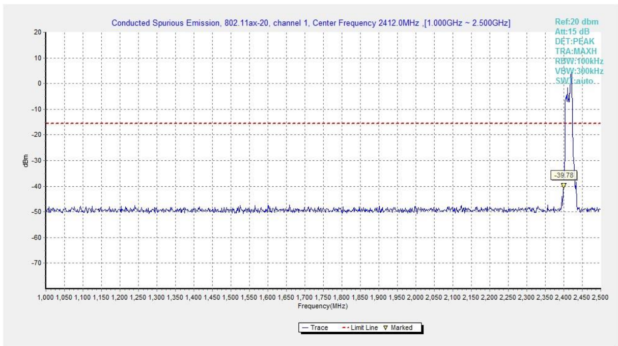
Fig.A.6.1.315 Transmitter Spurious Emission - Conducted (802.11ax-HE20-RU52-right, Ch1, 1 GHz-2.5 GHz)
