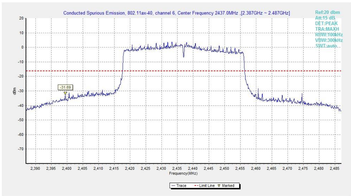
Fig.A.6.1.297 Transmitter Spurious Emission - Conducted (802.11ax-HE40, Ch6, Center Frequency)
