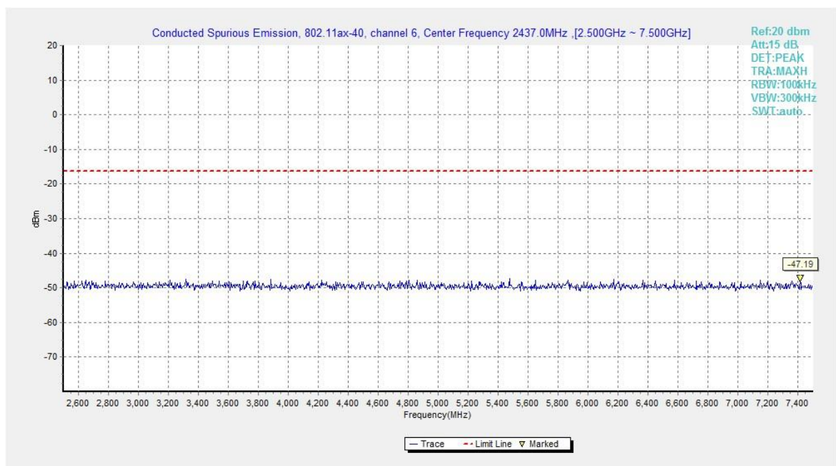
Fig.A.6.1.300 Transmitter Spurious Emission - Conducted (802.11ax-HE40, Ch6, 2.5 GHz-7.5 GHz)
