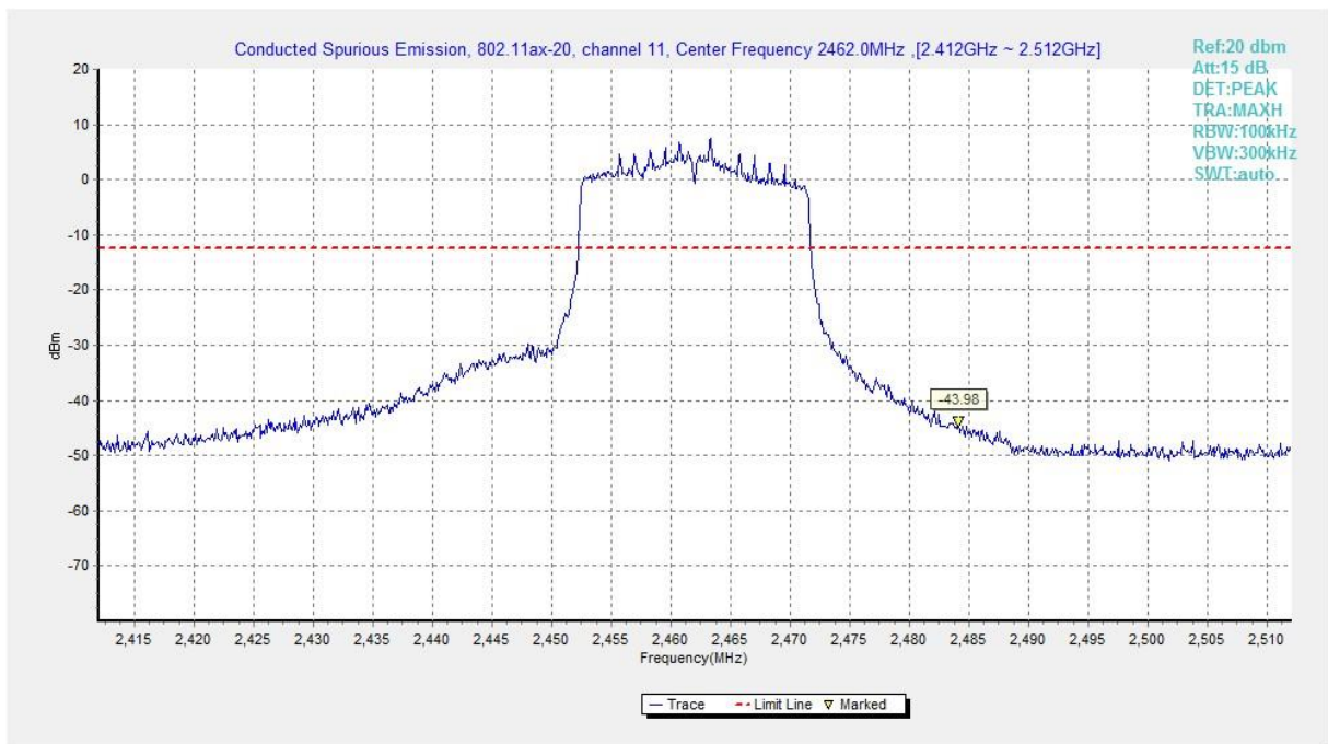
Fig.A.6.1.281 Transmitter Spurious Emission - Conducted (802.11ax-HE20, Ch11, Center Frequency)
