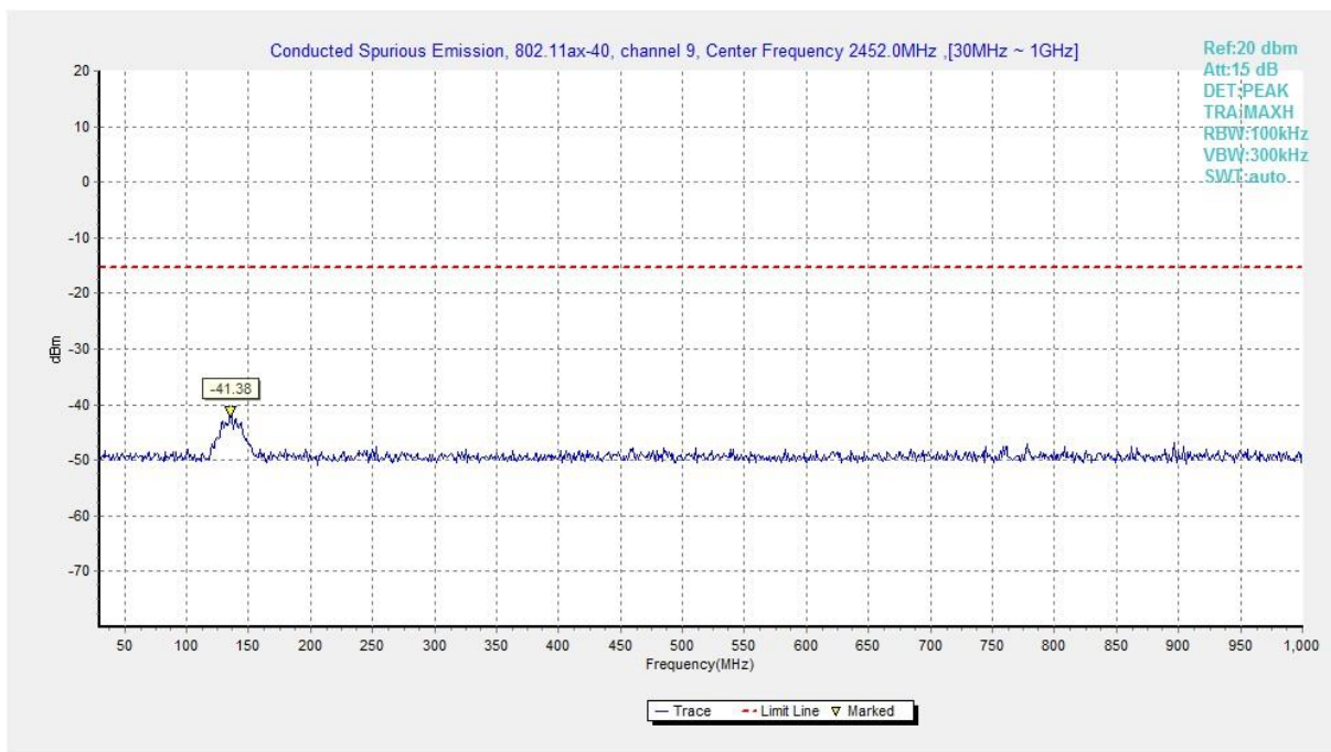
Fig.A.6.1.306 Transmitter Spurious Emission - Conducted (802.11ax-HE40, Ch9, 30 MHz-1 GHz)
