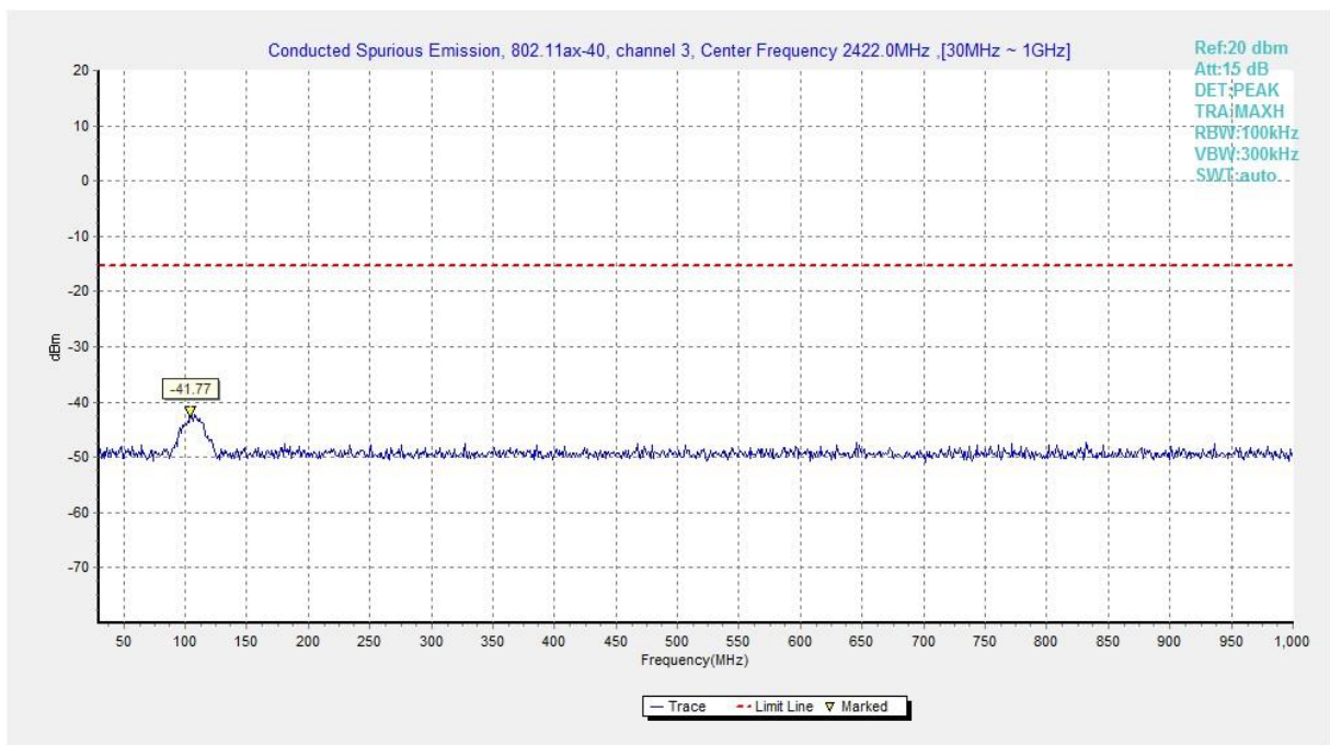
Fig.A.6.1.290 Transmitter Spurious Emission - Conducted (802.11ax-HE40, Ch3, 30 MHz-1 GHz)
