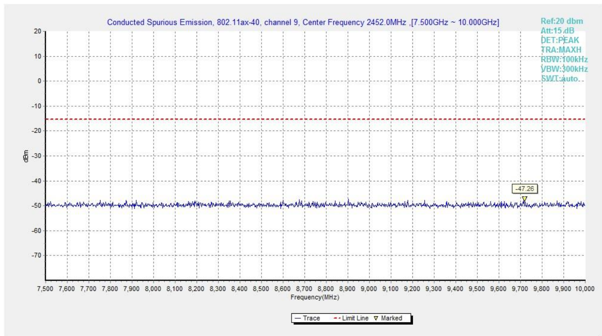
Fig.A.6.1.309 Transmitter Spurious Emission - Conducted (802.11ax-HE40, Ch9, 7.5 GHz-10 GHz)
