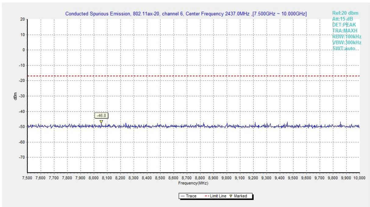
Fig.A.6.1.325 Transmitter Spurious Emission - Conducted (802.11ax-HE20-RU52-right, Ch6, 7.5 GHz-10 GHz)
