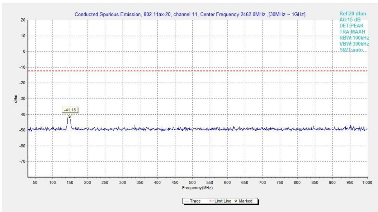
Fig.A.6.1.282 Transmitter Spurious Emission - Conducted (802.11ax-HE20, Ch11, 30 MHz-1 GHz)
