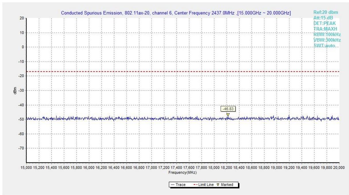
Fig.A.6.1.327 Transmitter Spurious Emission - Conducted (802.11ax-HE20-RU52-right, Ch6, 15 GHz-20 GHz)
