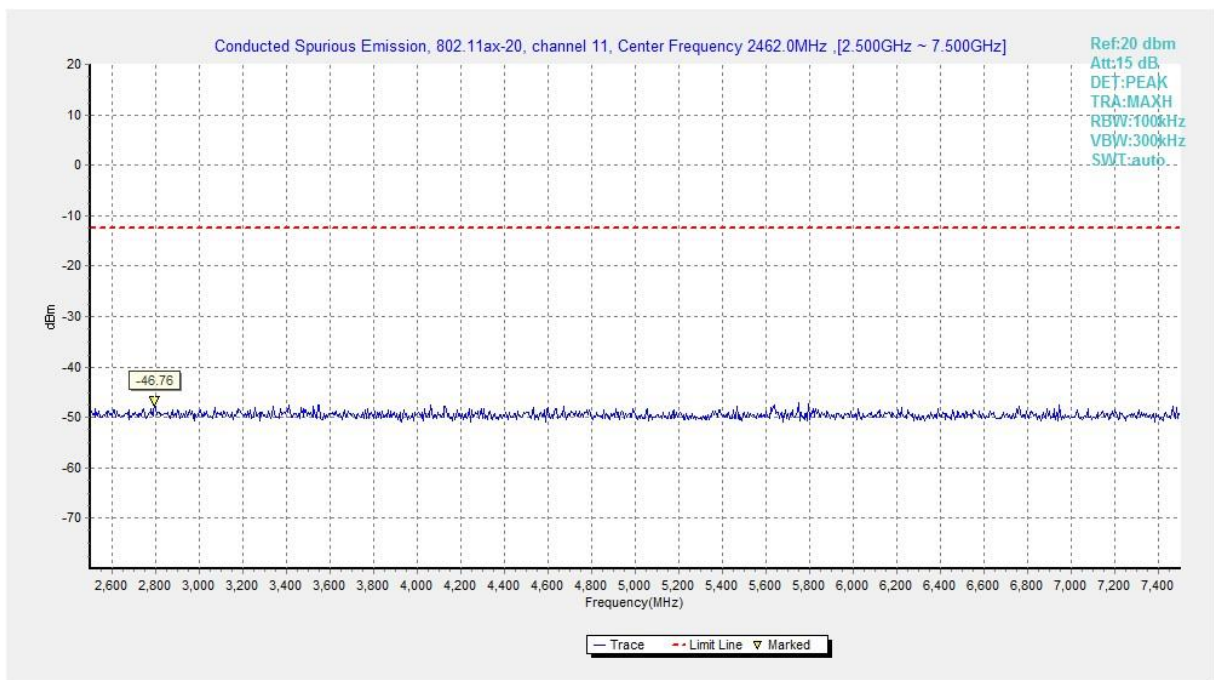
Fig.A.6.1.284 Transmitter Spurious Emission - Conducted (802.11ax-HE20, Ch11, 2.5 GHz-7.5 GHz)
