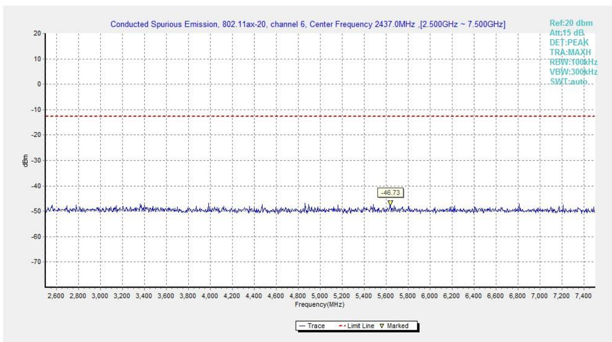
Fig.A.6.1.276 Transmitter Spurious Emission - Conducted (802.11ax-HE20, Ch6, 2.5 GHz-7.5 GHz)
