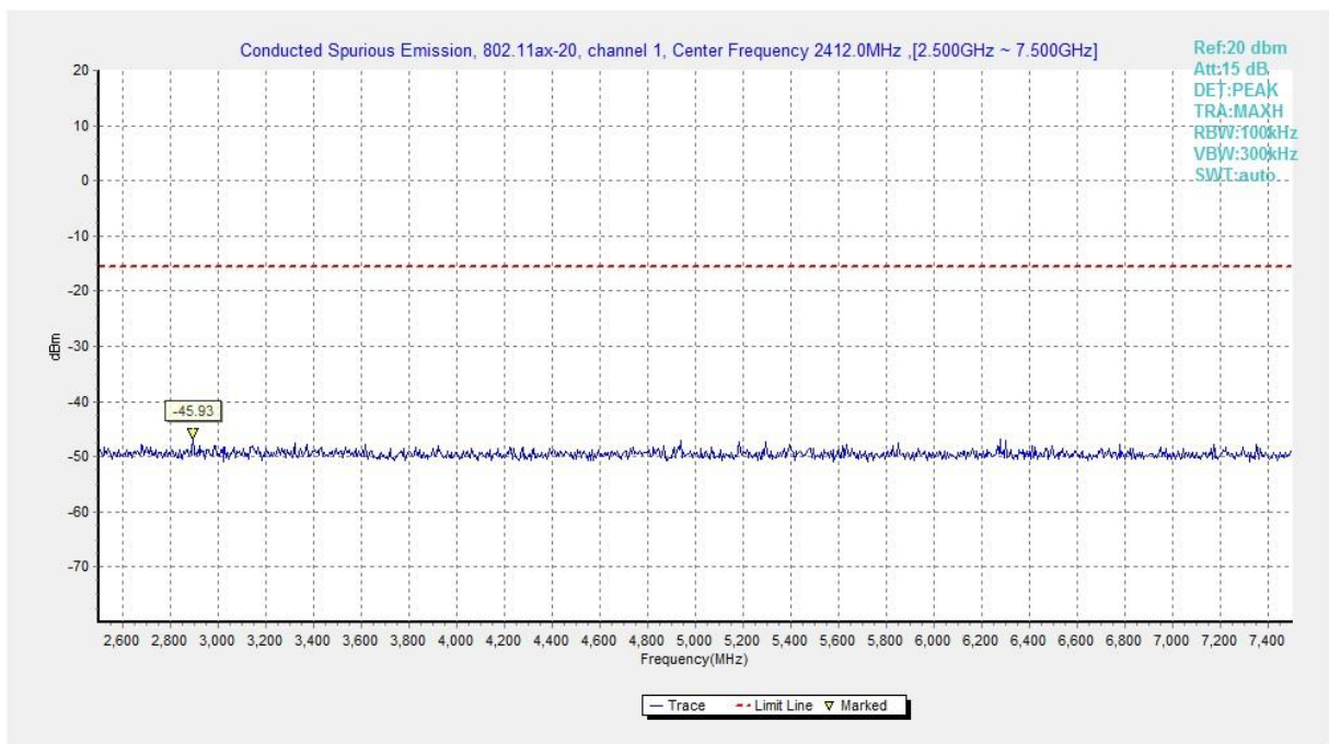
Fig.A.6.1.316 Transmitter Spurious Emission - Conducted (802.11ax-HE20-RU52-right, 2.5 GHz-7.5 GHz)
