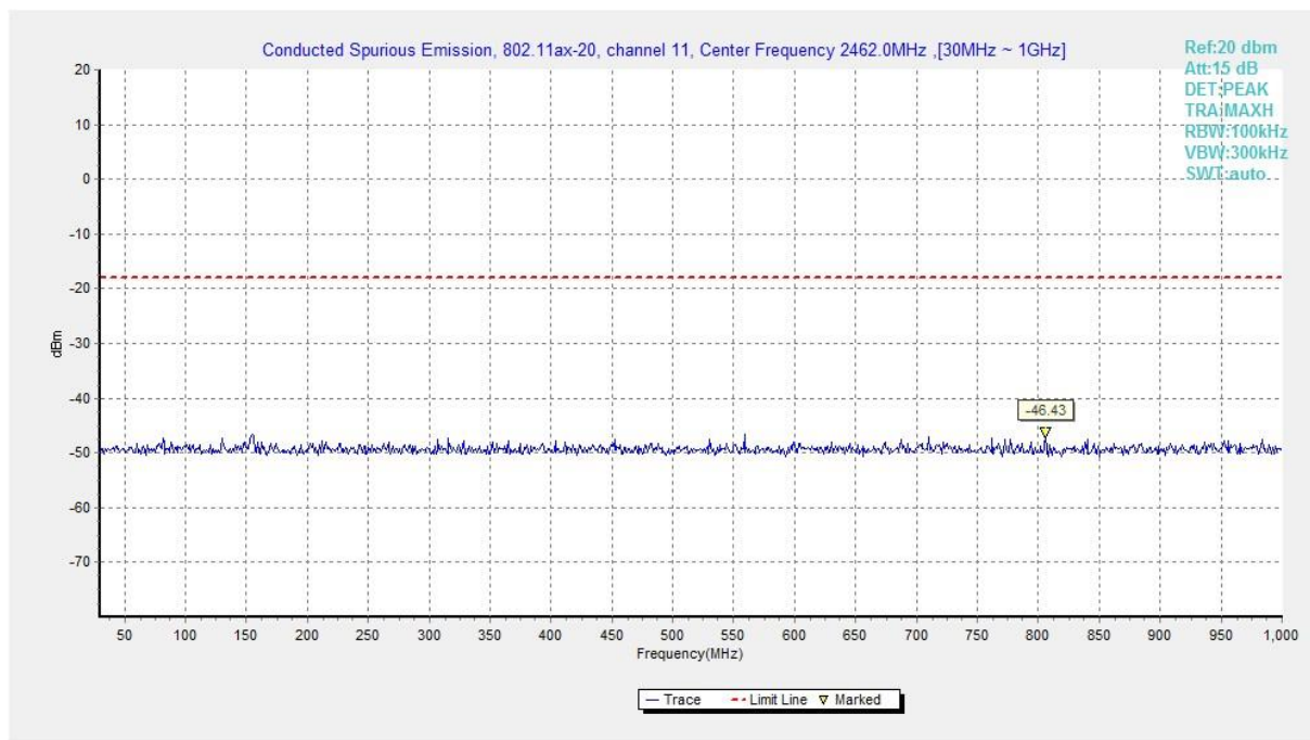
Fig.A.6.1.330 Transmitter Spurious Emission - Conducted (802.11ax-HE20-RU52-right, Ch11, 30 MHz-1 GHz)
