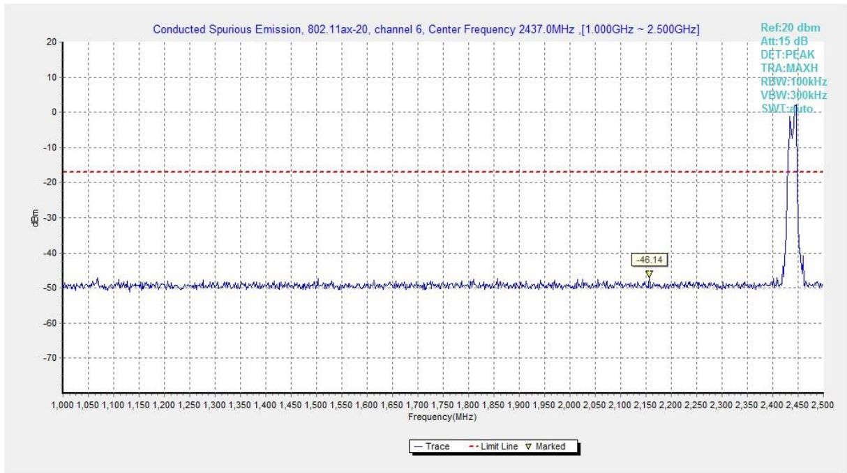
Fig.A.6.1.323 Transmitter Spurious Emission - Conducted (802.11ax-HE20-RU52-right, Ch6, 1 GHz-2.5 GHz)
