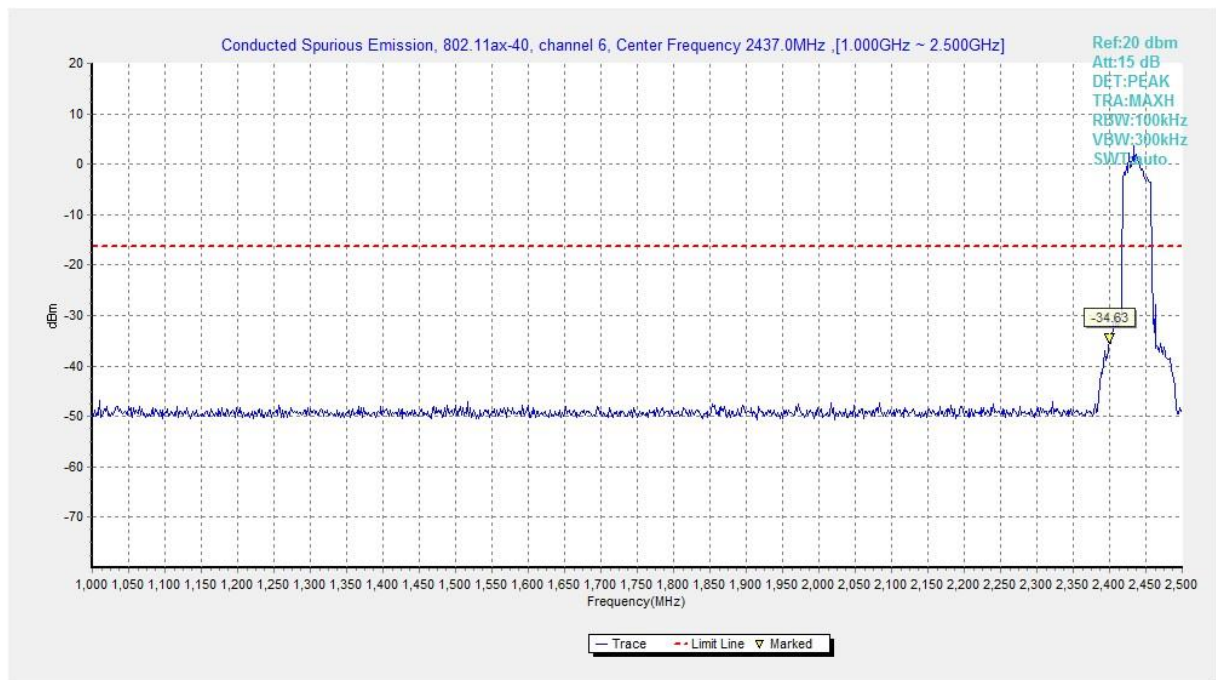
Fig.A.6.1.299 Transmitter Spurious Emission - Conducted (802.11ax-HE40, Ch6, 1 GHz-2.5 GHz)
