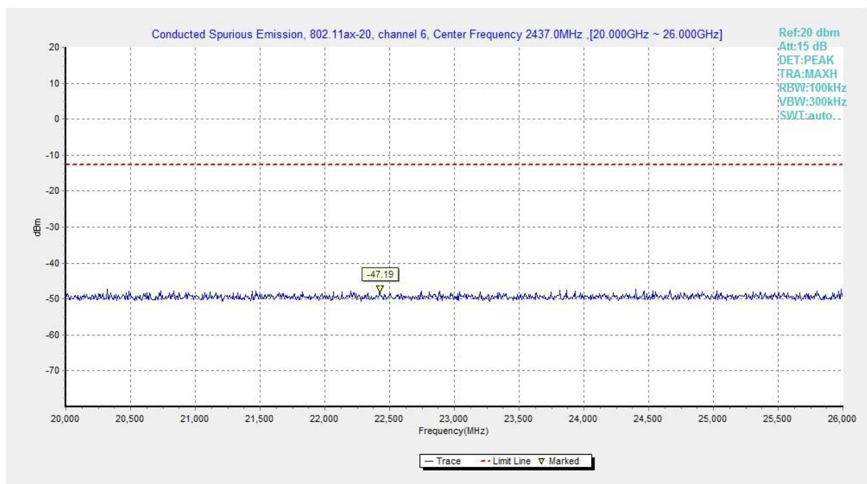
Fig.A.6.1.280 Transmitter Spurious Emission - Conducted (802.11ax-HE20, Ch6, 20 GHz-26 GHz)
