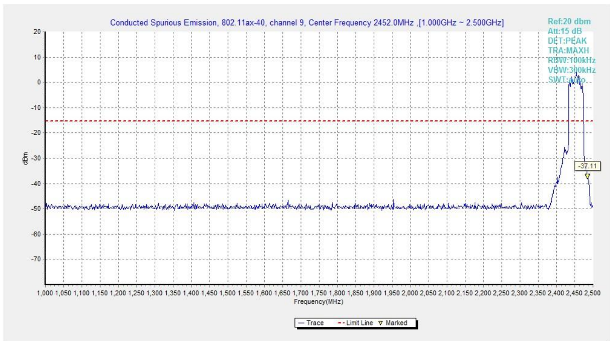
Fig.A.6.1.307 Transmitter Spurious Emission - Conducted (802.11ax-HE40, Ch9, 1 GHz-2.5 GHz)
