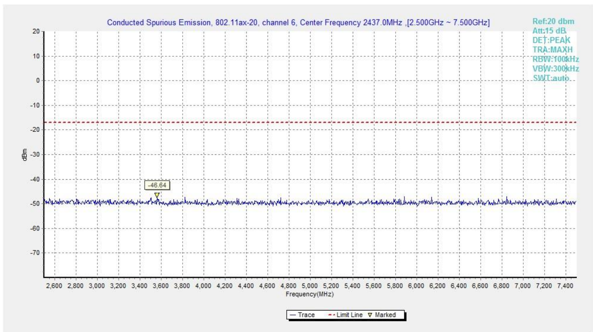
Fig.A.6.1.324 Transmitter Spurious Emission - Conducted (802.11ax-HE20-RU52-right, Ch6, 2.5 GHz-7.5 GHz)
