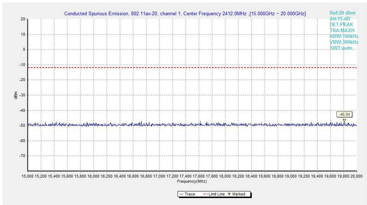
Fig.A.6.1.271 Transmitter Spurious Emission - Conducted (802.11ax-HE20, Ch1, 15 GHz-20 GHz)
