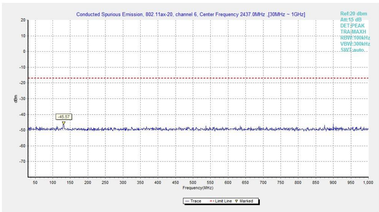
Fig.A.6.1.322 Transmitter Spurious Emission - Conducted (802.11ax-HE20-RU52-right, Ch6, 30 MHz-1 GHz)
