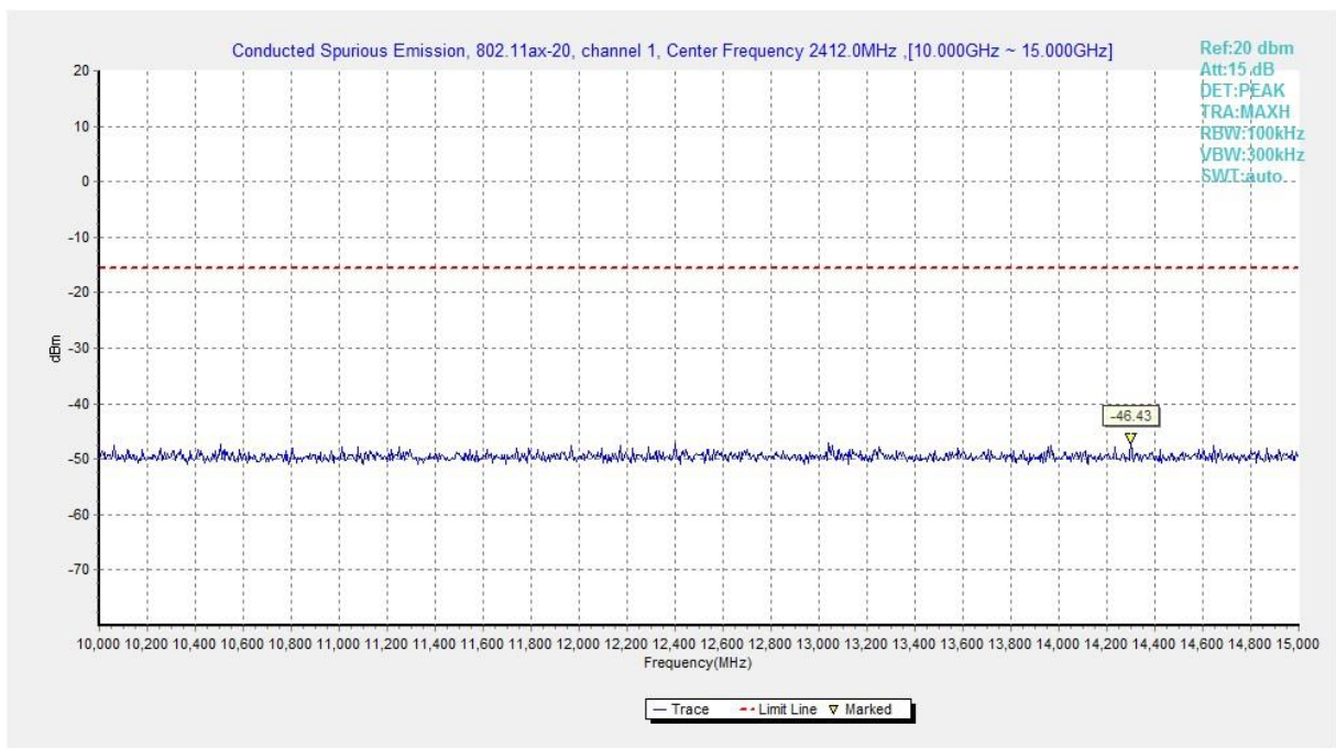
Fig.A.6.1.318 Transmitter Spurious Emission - Conducted (802.11ax-HE20-RU52-right, Ch1, 10 GHz-15 GHz)
