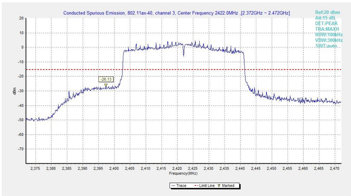
Fig.A.6.1.289 Transmitter Spurious Emission - Conducted (802.11ax-HE40, Ch3, Center Frequency)
