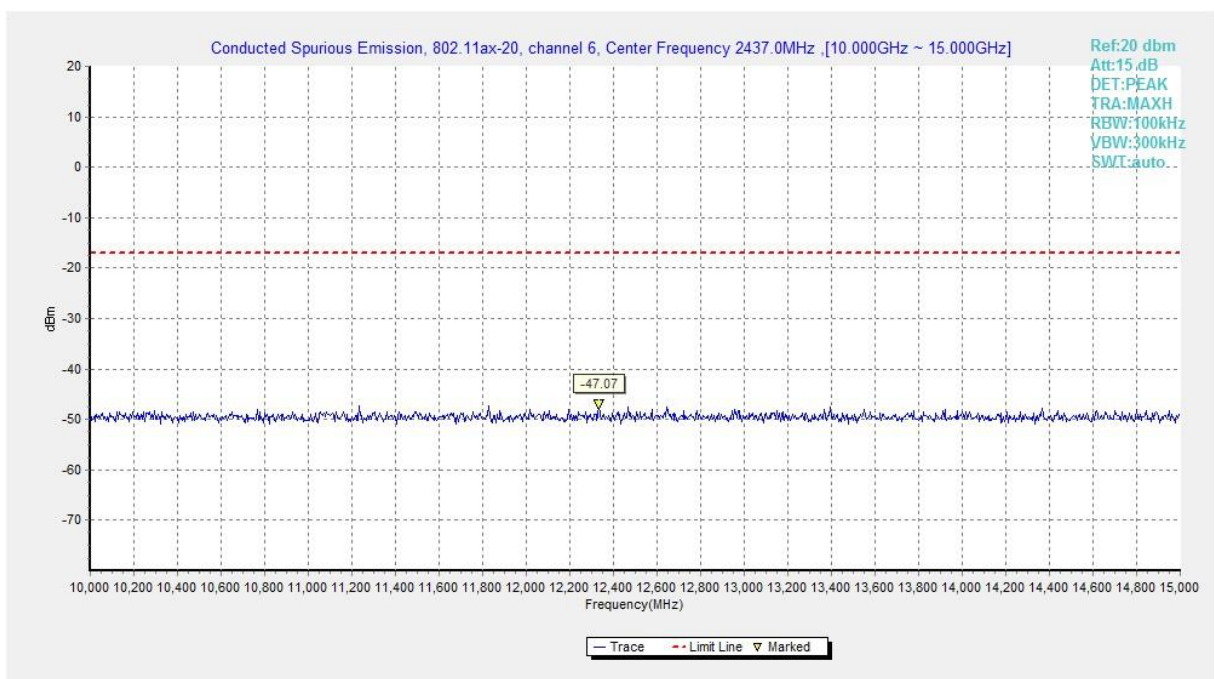
Fig.A.6.1.326 Transmitter Spurious Emission – Conducted (802.11ax-HE20-RU52-right, Ch6, 10 GHz-15 GHz)
