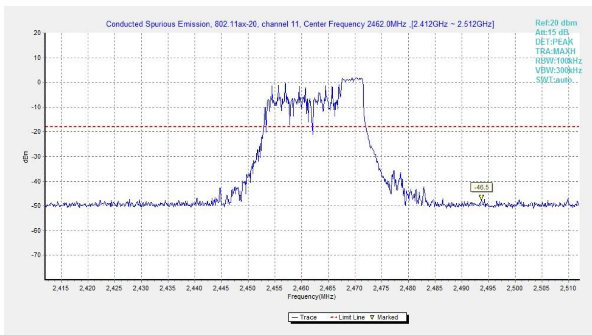
Fig.A.6.1.329 Transmitter Spurious Emission - Conducted (802.11ax-HE20-RU52-right, Ch11, Center Frequency)
