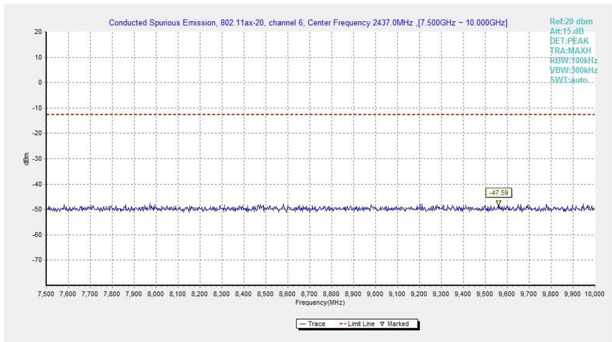
Fig.A.6.1.277 Transmitter Spurious Emission - Conducted (802.11ax-HE20, Ch6, 7.5 GHz-10 GHz)
