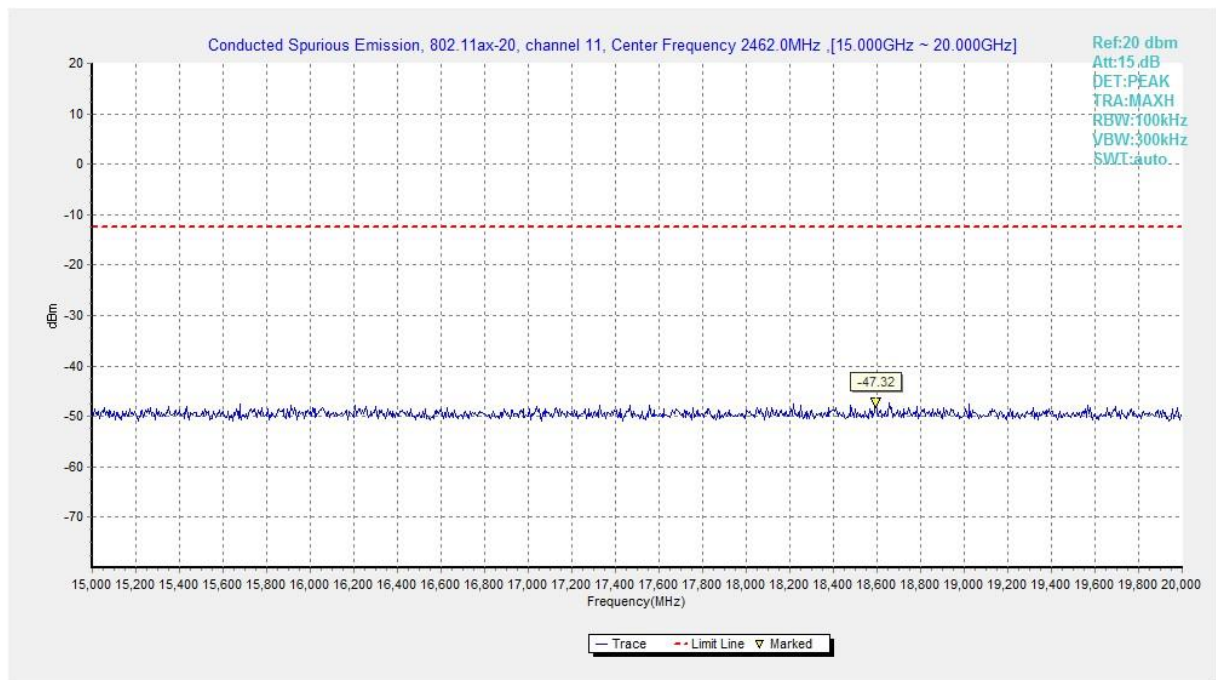
Fig.A.6.1.287 Transmitter Spurious Emission - Conducted (802.11ax-HE20, Ch11, 15 GHz-20 GHz)
