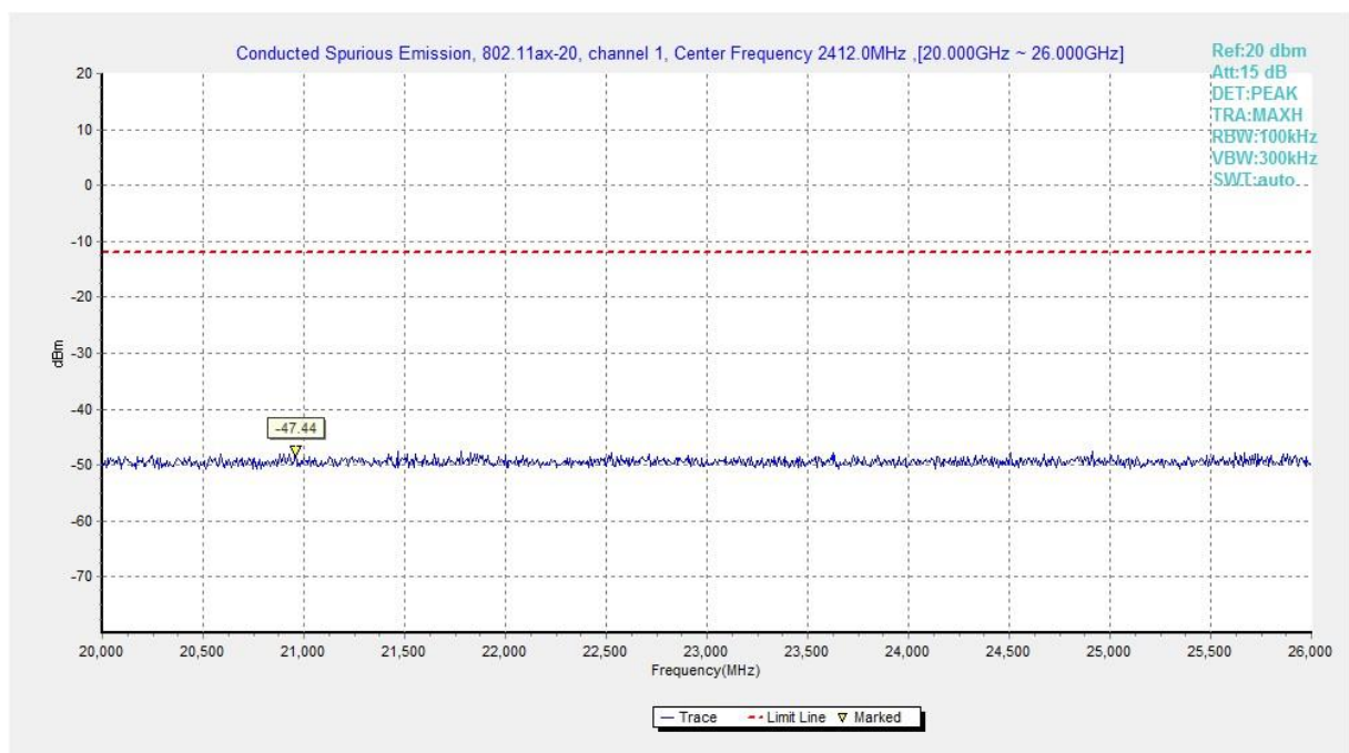
Fig.A.6.1.272 Transmitter Spurious Emission - Conducted (802.11ax-HE20, Ch1, 20 GHz-26 GHz)
