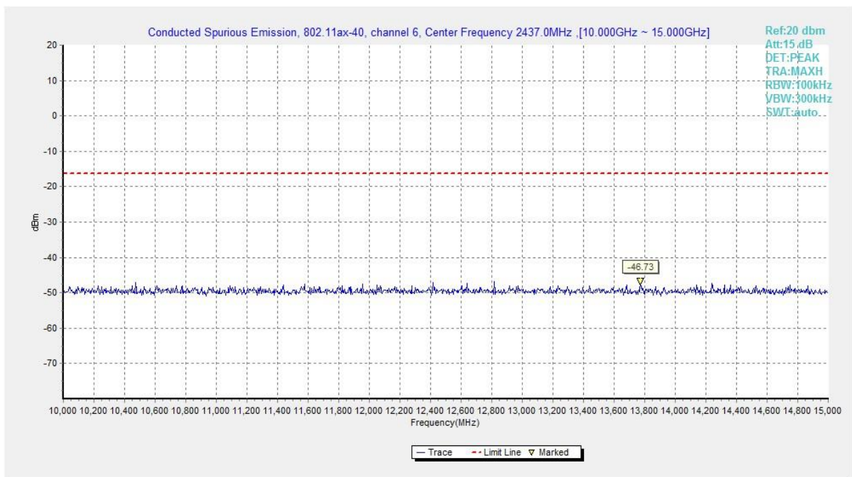
Fig.A.6.1.302 Transmitter Spurious Emission - Conducted (802.11ax-HE40, Ch6, 10 GHz-15 GHz)
