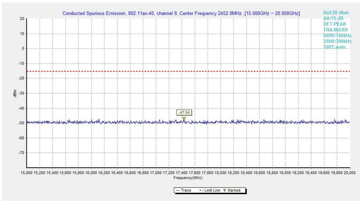
Fig.A.6.1.311 Transmitter Spurious Emission - Conducted (802.11ax-HE40, Ch9, 15 GHz-20 GHz)
