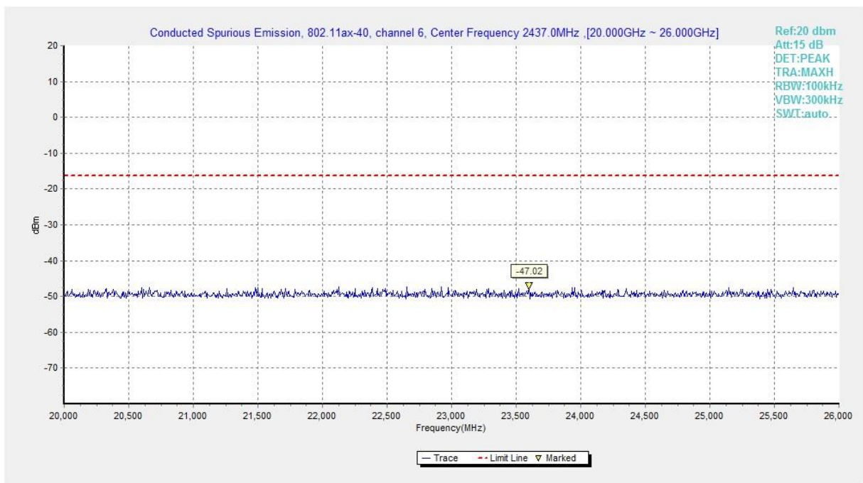
Fig.A.6.1.304 Transmitter Spurious Emission - Conducted (802.11ax-HE40, Ch6, 20 GHz-26 GHz)
