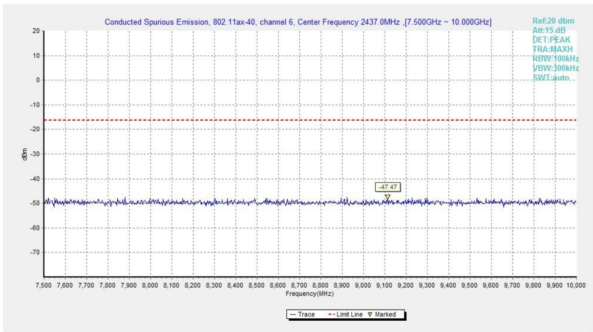
Fig.A.6.1.301 Transmitter Spurious Emission - Conducted (802.11ax-HE40, Ch6, 7.5 GHz-10 GHz)
