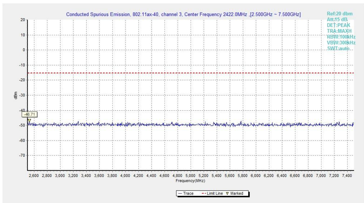
Fig.A.6.1.292 Transmitter Spurious Emission - Conducted (802.11ax-HE40, Ch3, 2.5 GHz-7.5 GHz)
