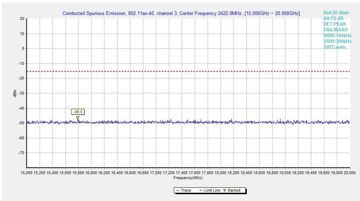
Fig.A.6.1.295 Transmitter Spurious Emission - Conducted (802.11ax-HE40, Ch3, 15 GHz-20 GHz)
