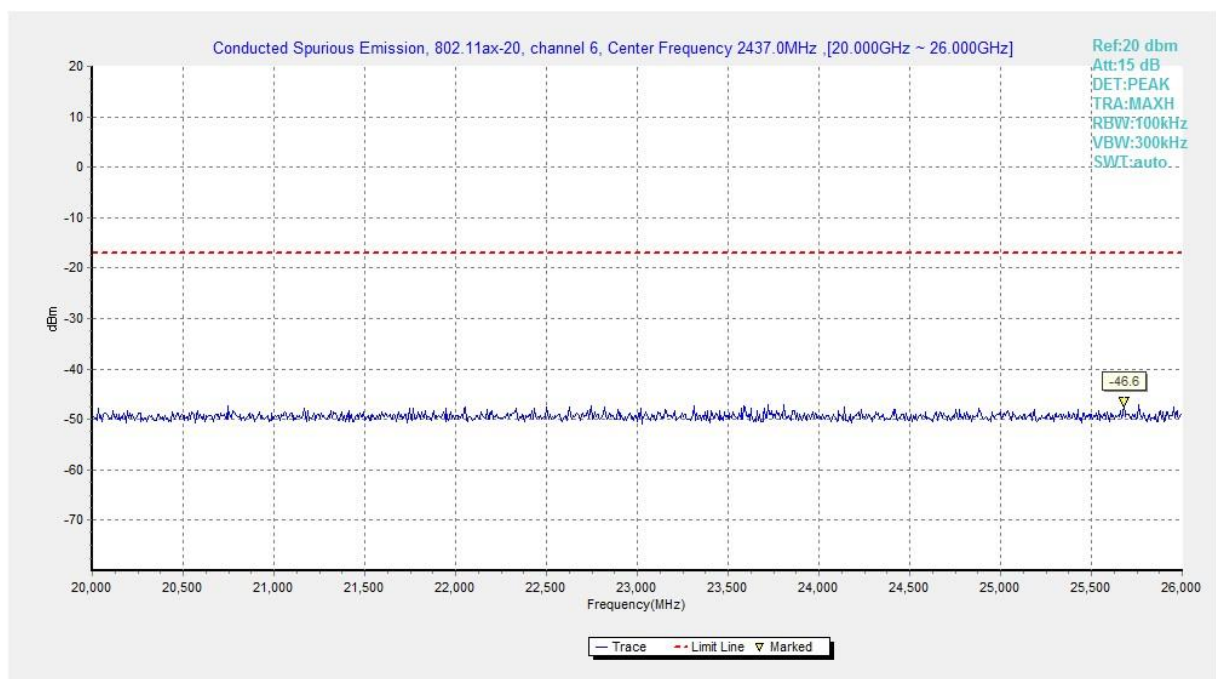
Fig.A.6.1.328 Transmitter Spurious Emission - Conducted (802.11ax-HE20-RU52-right, Ch6, 20 GHz-26 GHz)
