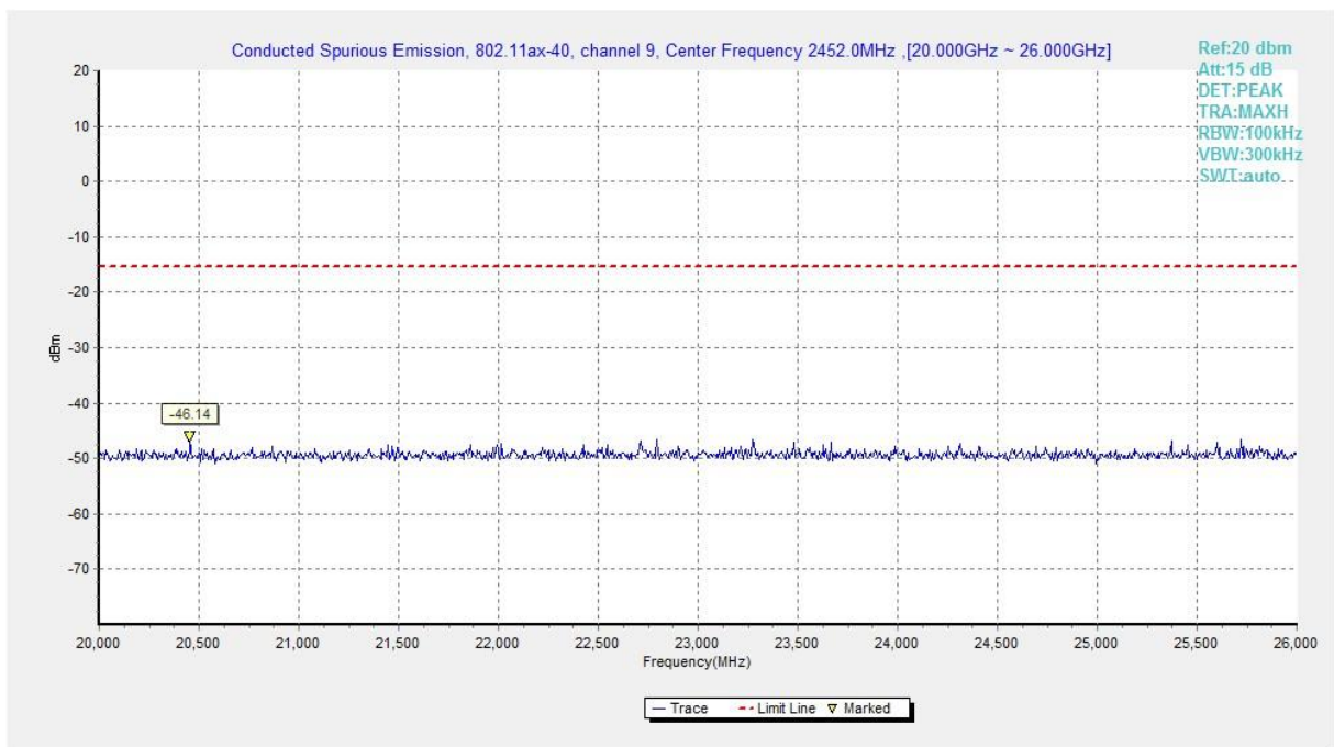
Fig.A.6.1.312 Transmitter Spurious Emission - Conducted (802.11ax-HE40, Ch9, 20 GHz-26 GHz)
