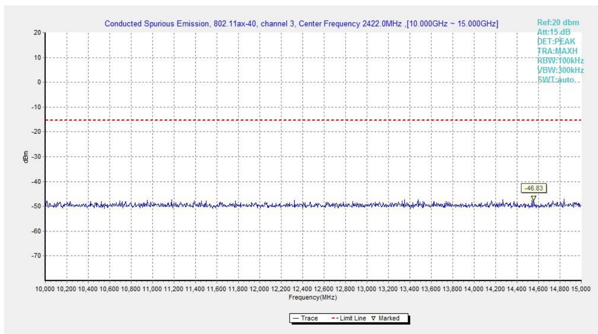
Fig.A.6.1.294 Transmitter Spurious Emission - Conducted (802.11ax-HE40, Ch3, 10 GHz-15 GHz)
