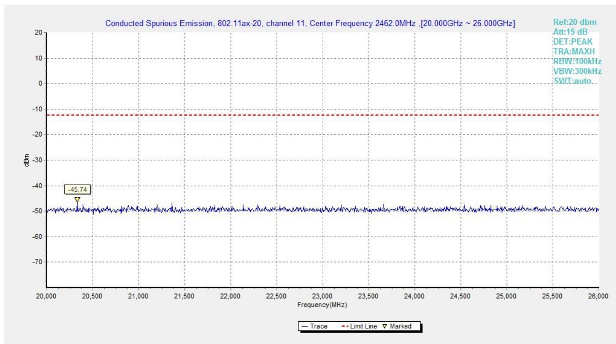
Fig.A.6.1.288 Transmitter Spurious Emission - Conducted (802.11ax-HE20, Ch11, 20 GHz-26 GHz)
