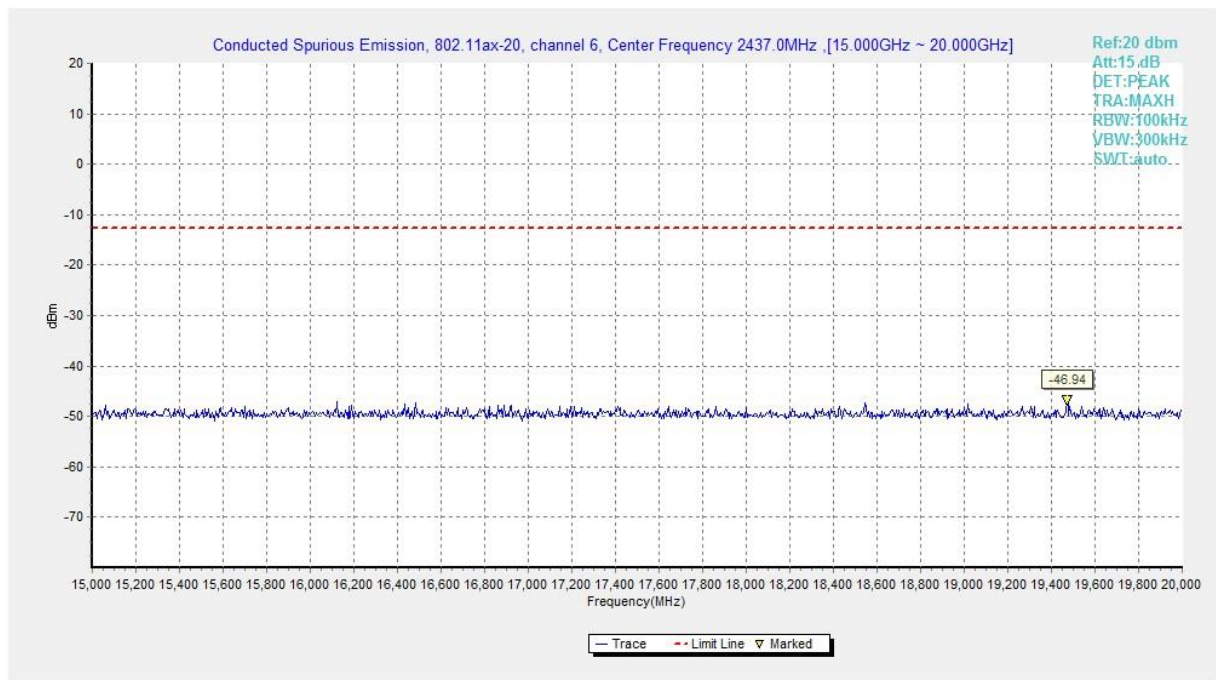
Fig.A.6.1.279 Transmitter Spurious Emission - Conducted (802.11ax-HE20, Ch6, 15 GHz-20 GHz)
