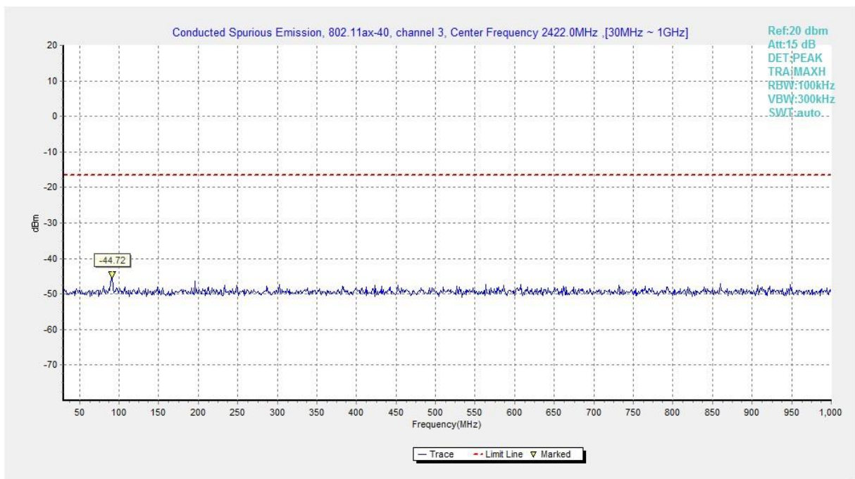
Fig.A.6.1.338 Transmitter Spurious Emission - Conducted (802.11ax-HE40-RU52-left, Ch3, 30 MHz-1 GHz)
