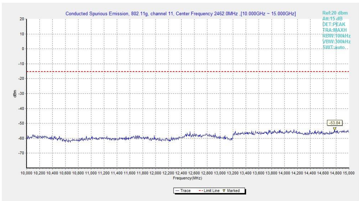
Fig.A.6.1.382 Transmitter Spurious Emission - Conducted (802.11g, Ch11, 10 GHz-15 GHz)
