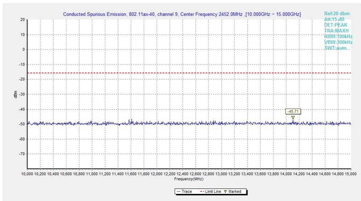
Fig.A.6.1.358 Transmitter Spurious Emission - Conducted(802.11ax-HE40-RU52-left, Ch9, 10 GHz-15 GHz)
