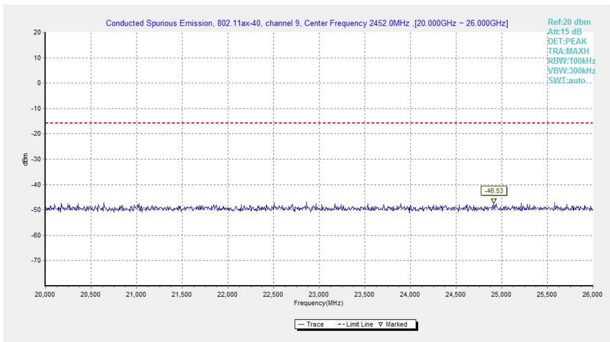
Fig.A.6.1.360 Transmitter Spurious Emission - Conducted (802.11ax-HE40-RU52-left, Ch9, 20 GHz-26 GHz)
