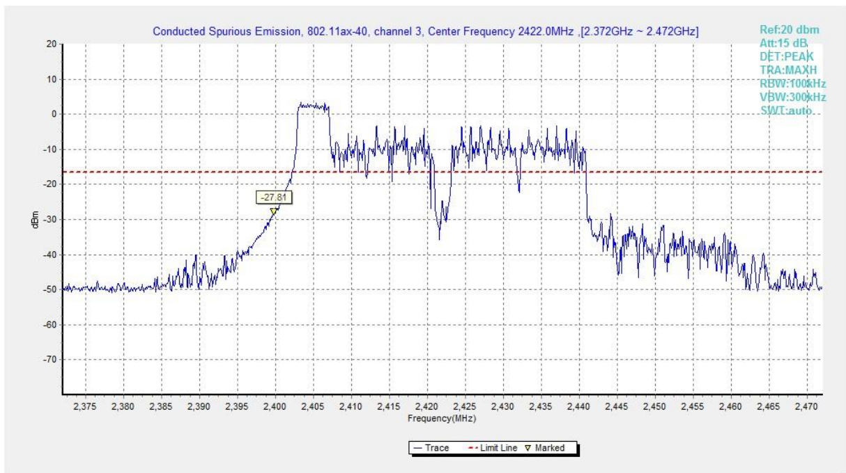
Fig.A.6.1.337 Transmitter Spurious Emission – Conducted (802.11ax-HE40-RU52-left, Ch3, Center Frequency)
