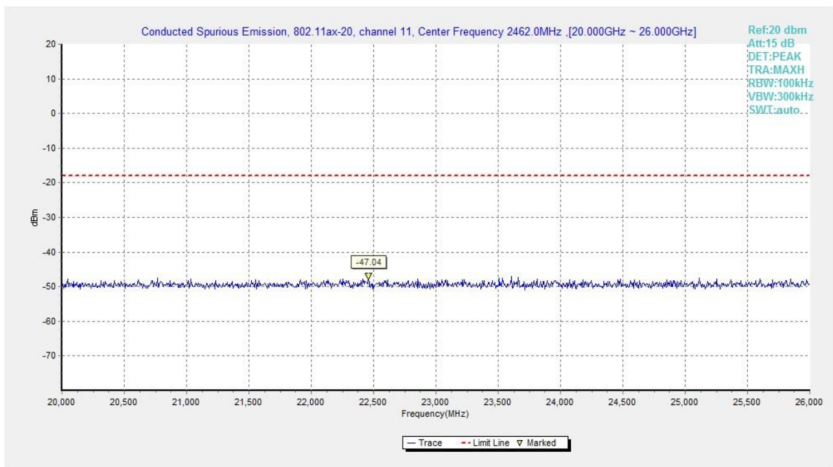
Fig.A.6.1.336 Transmitter Spurious Emission - Conducted (802.11ax-HE20-RU52-right, Ch11, 20 GHz-26 GHz)
