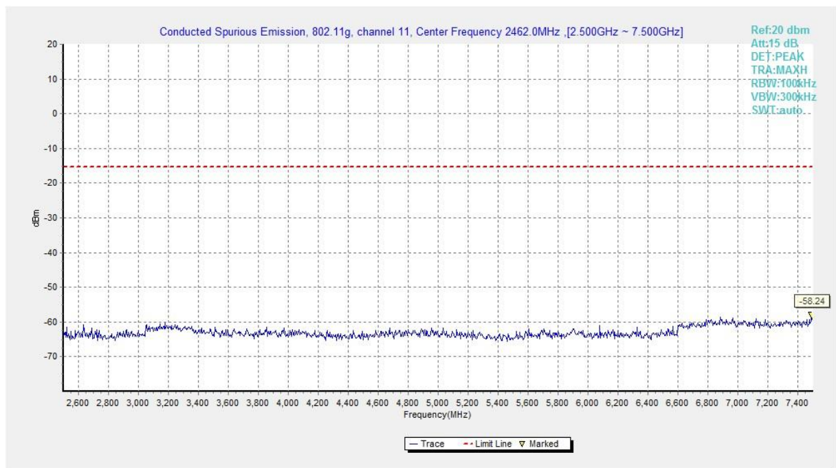
Fig.A.6.1.380 Transmitter Spurious Emission - Conducted (802.11g, Ch11, 2.5 GHz-7.5 GHz)
