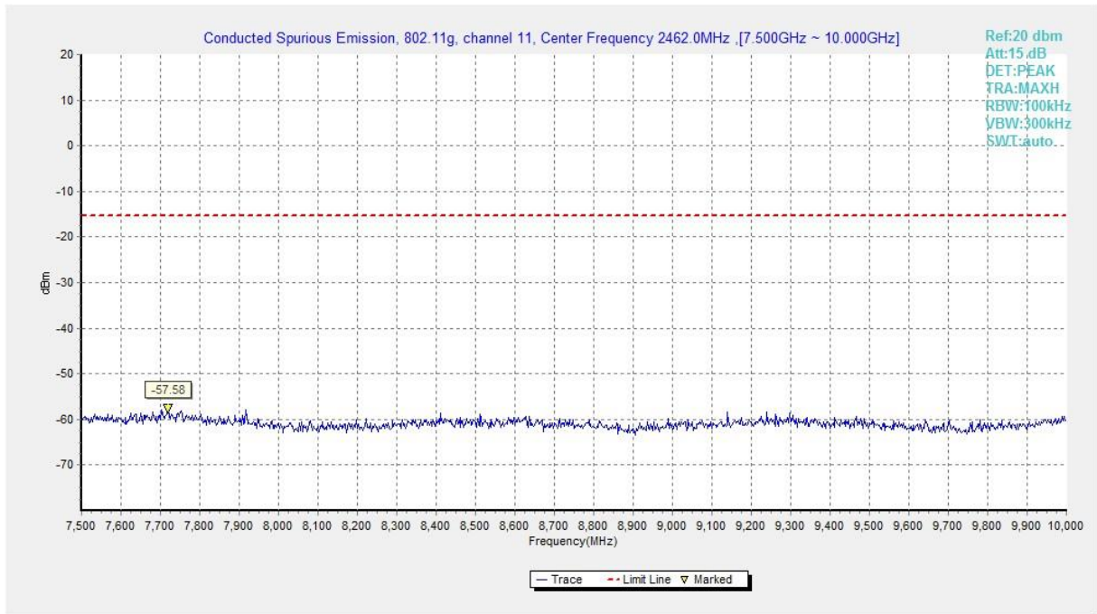
Fig.A.6.1.381 Transmitter Spurious Emission - Conducted (802.11g, Ch11, 7.5 GHz-10 GHz)
