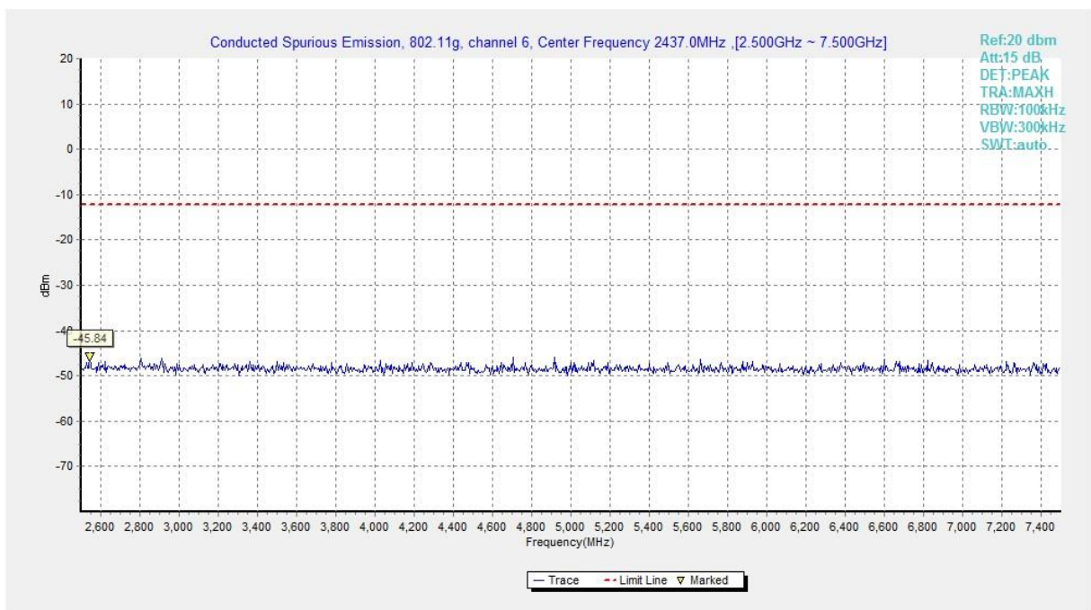
Fig.A.6.1.372 Transmitter Spurious Emission - Conducted (802.11g, Ch6, 2.5 GHz-7.5 GHz)
