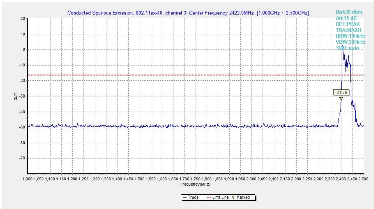
Fig.A.6.1.339 Transmitter Spurious Emission - Conducted (802.11ax-HE40-RU52-left, Ch3, 1 GHz-2.5 GHz)
