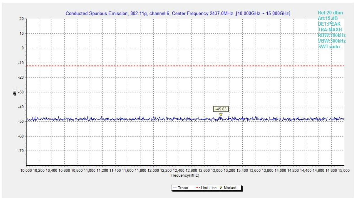
Fig.A.6.1.374 Transmitter Spurious Emission - Conducted (802.11g, Ch6, 10 GHz-15 GHz)
