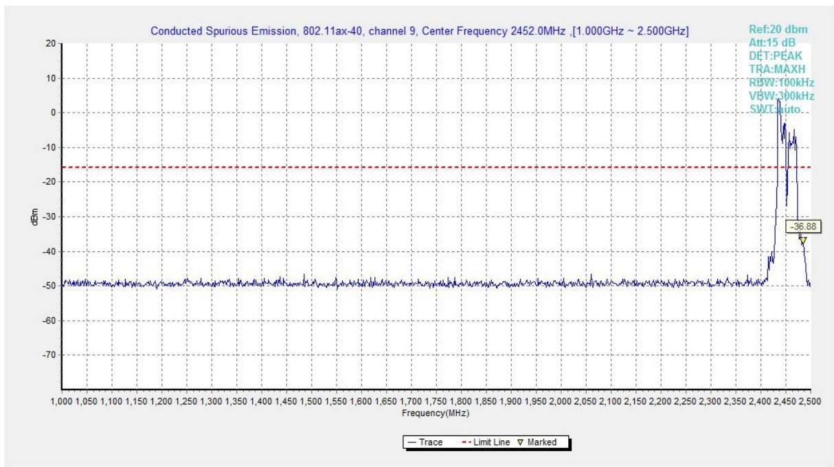
Fig.A.6.1.355 Transmitter Spurious Emission - Conducted (802.11ax-HE40-RU52-left, Ch9, 1 GHz-2.5 GHz)
