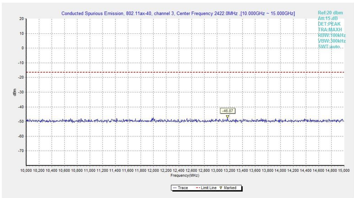
Fig.A.6.1.342 Transmitter Spurious Emission – Conducted (802.11ax-HE40-RU52-left, Ch3, 10 GHz-15 GHz)
