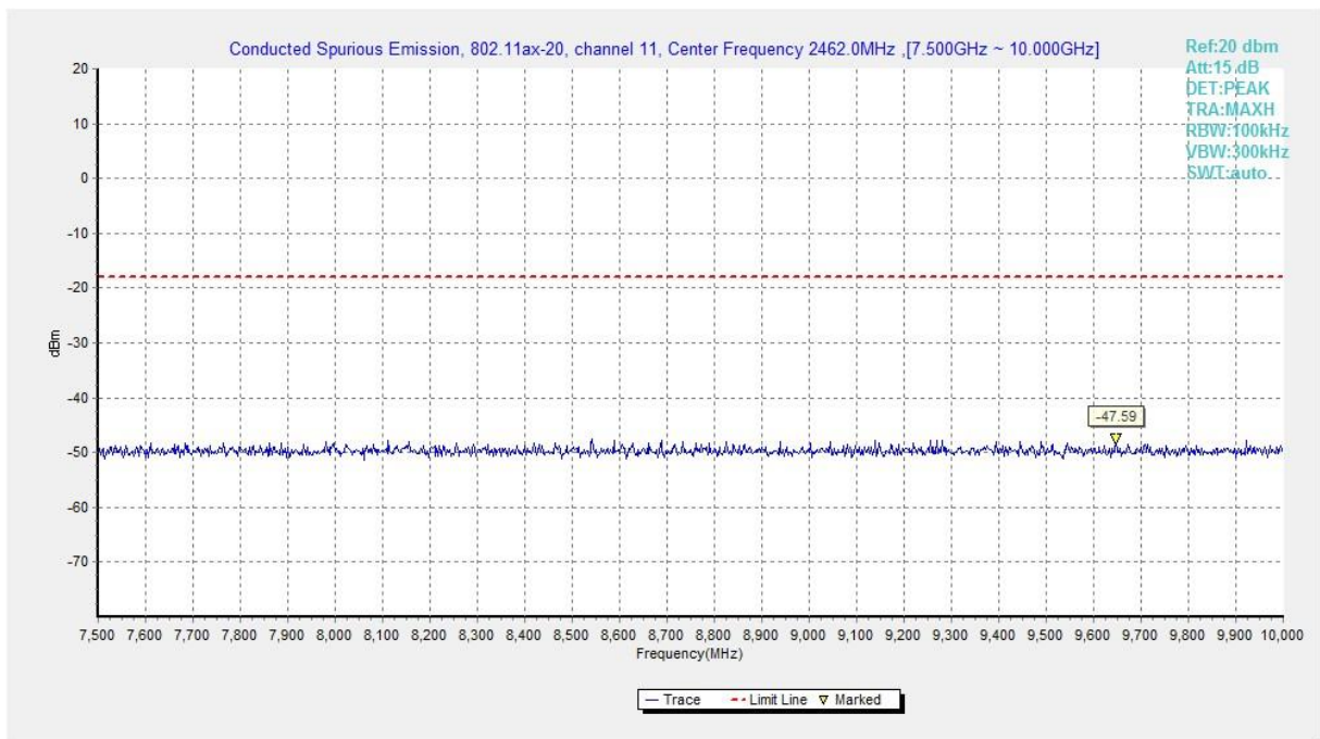
Fig.A.6.1.333 Transmitter Spurious Emission - Conducted (802.11ax-HE20-RU52-right, Ch11, 7.5 GHz-10 GHz)
