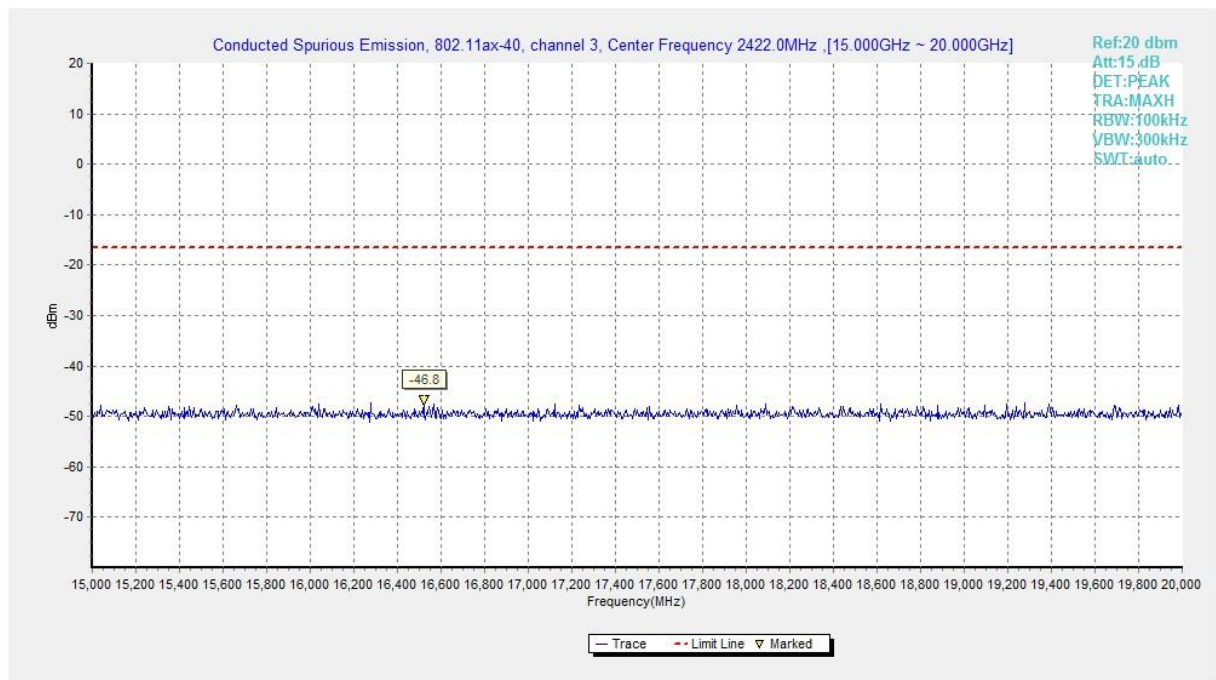
Fig.A.6.1.343 Transmitter Spurious Emission - Conducted (802.11ax-HE40-RU52-left, Ch3, 15 GHz-20 GHz)
