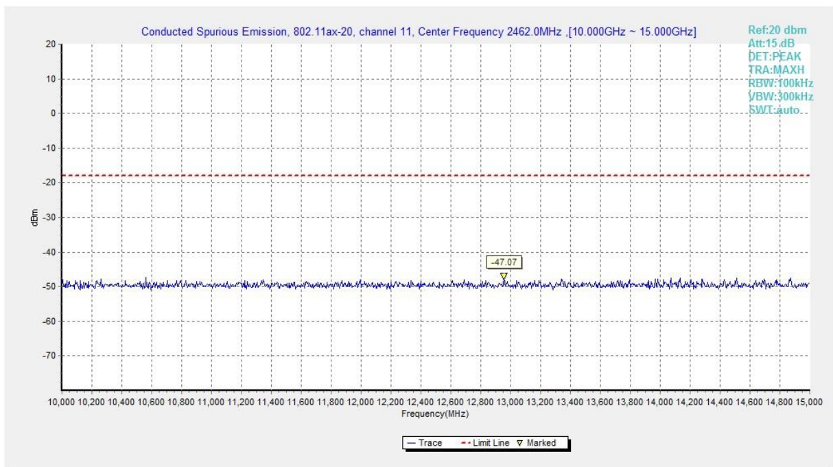
Fig.A.6.1.334 Transmitter Spurious Emission - Conducted (802.11ax-HE20-RU52-right, Ch11, 10 GHz-15 GHz)
