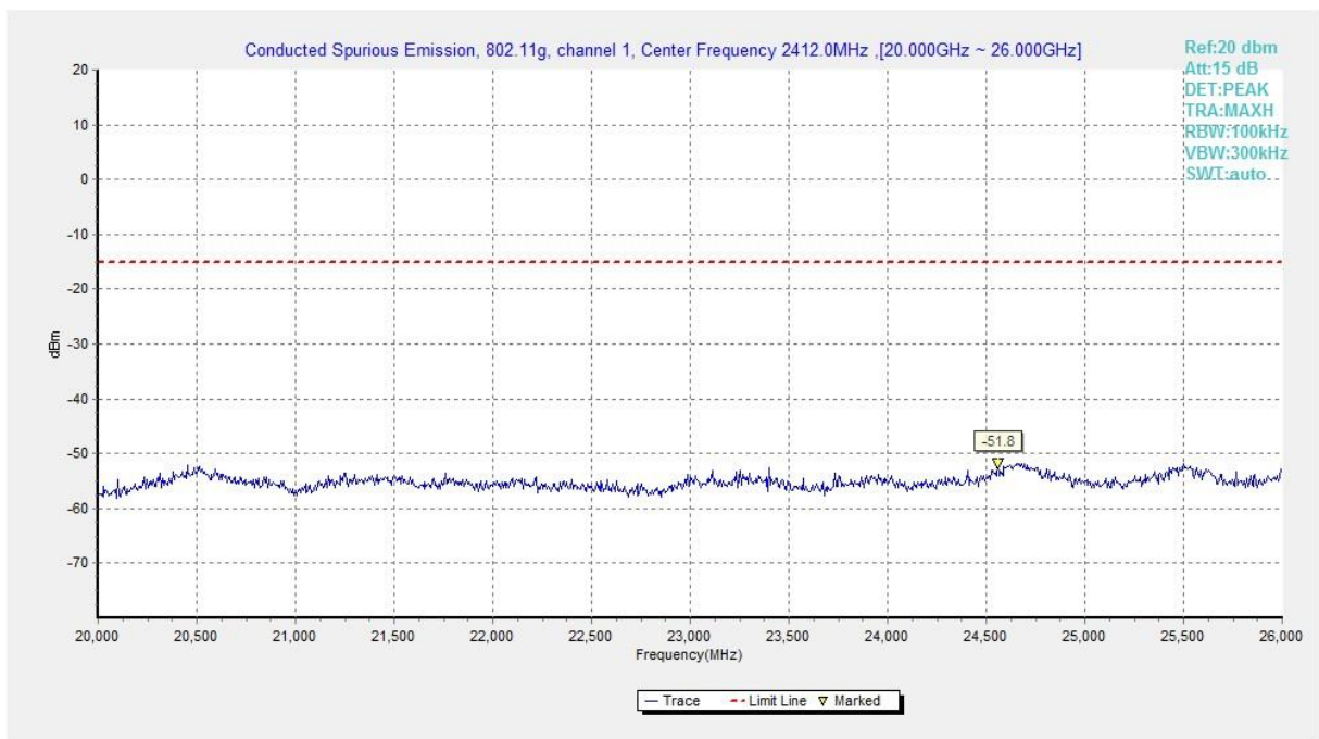
Fig.A.6.1.368 Transmitter Spurious Emission - Conducted (802.11g, Ch1, 20 GHz-26 GHz)
