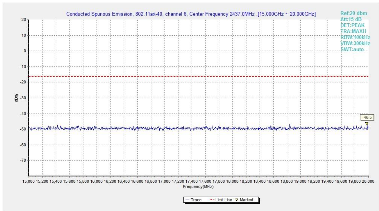
Fig.A.6.1.351 Transmitter Spurious Emission - Conducted (802.11ax-HE40-RU52-left, Ch6, 15 GHz-20 GHz)
