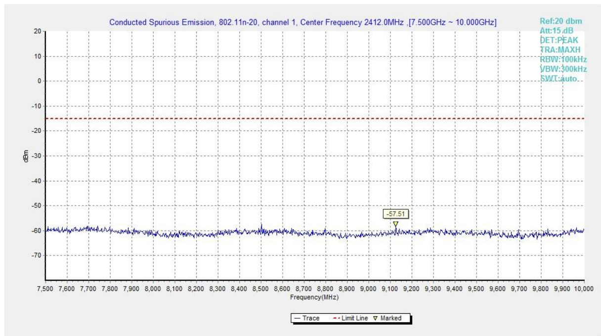
Fig.A.6.1.389 Transmitter Spurious Emission - Conducted (802.11n-HT20, Ch1, 7.5 GHz-10 GHz)
