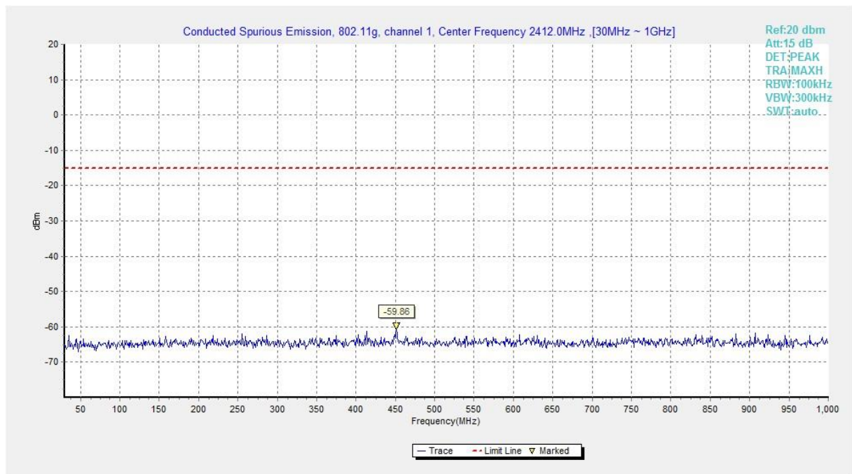
Fig.A.6.1.362 Transmitter Spurious Emission - Conducted (802.11g, Ch1, 30 MHz-1 GHz)
