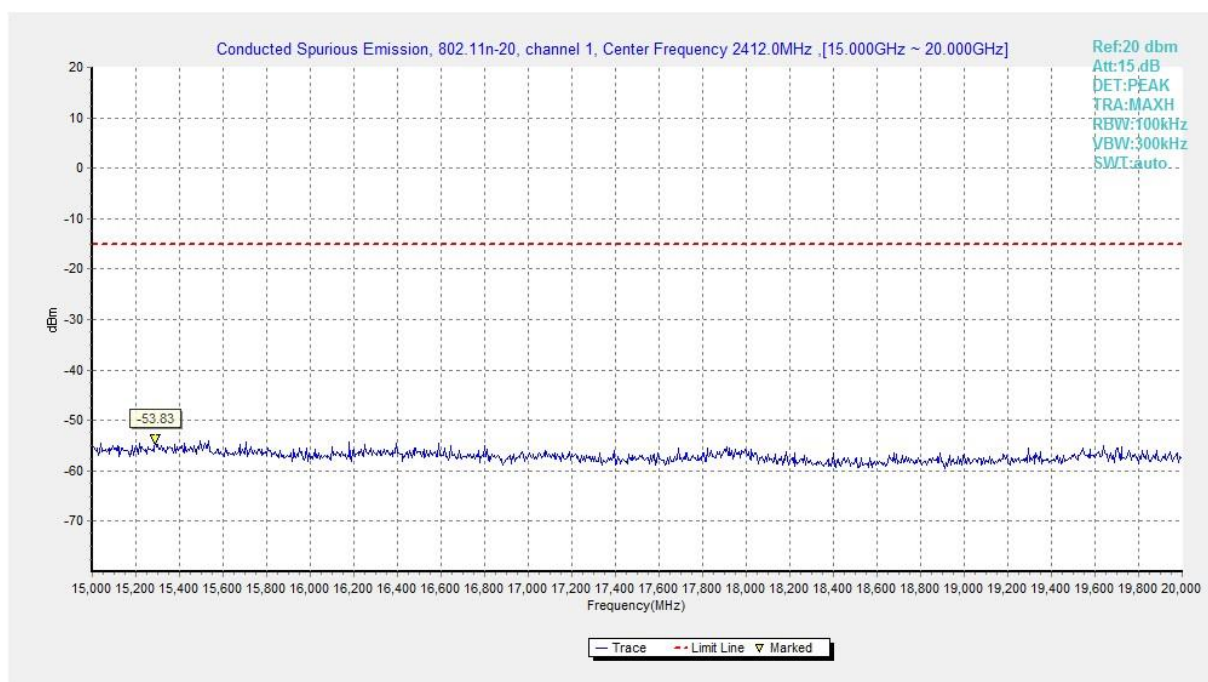
Fig.A.6.1.391 Transmitter Spurious Emission - Conducted (802.11n-HT20, Ch1, 15 GHz-20 GHz)
