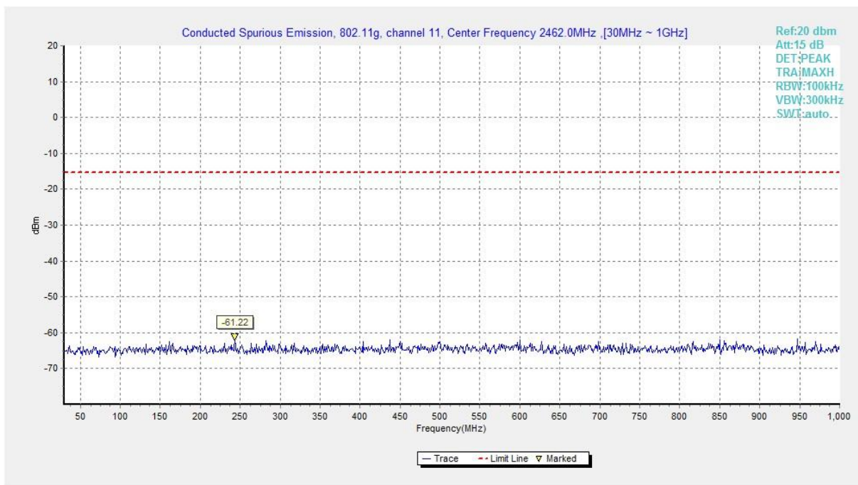
Fig.A.6.1.378 Transmitter Spurious Emission - Conducted (802.11g, Ch11, 30 MHz-1 GHz)
