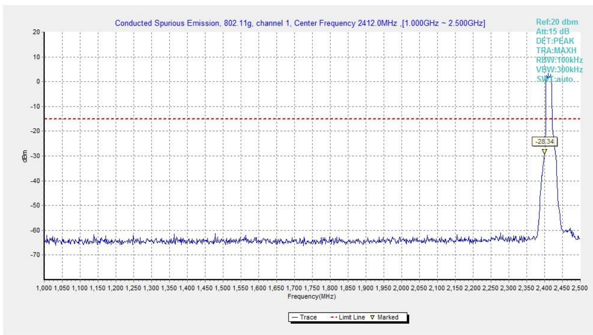
Fig.A.6.1.363 Transmitter Spurious Emission - Conducted (802.11g, Ch1, 1 GHz-2.5 GHz)
