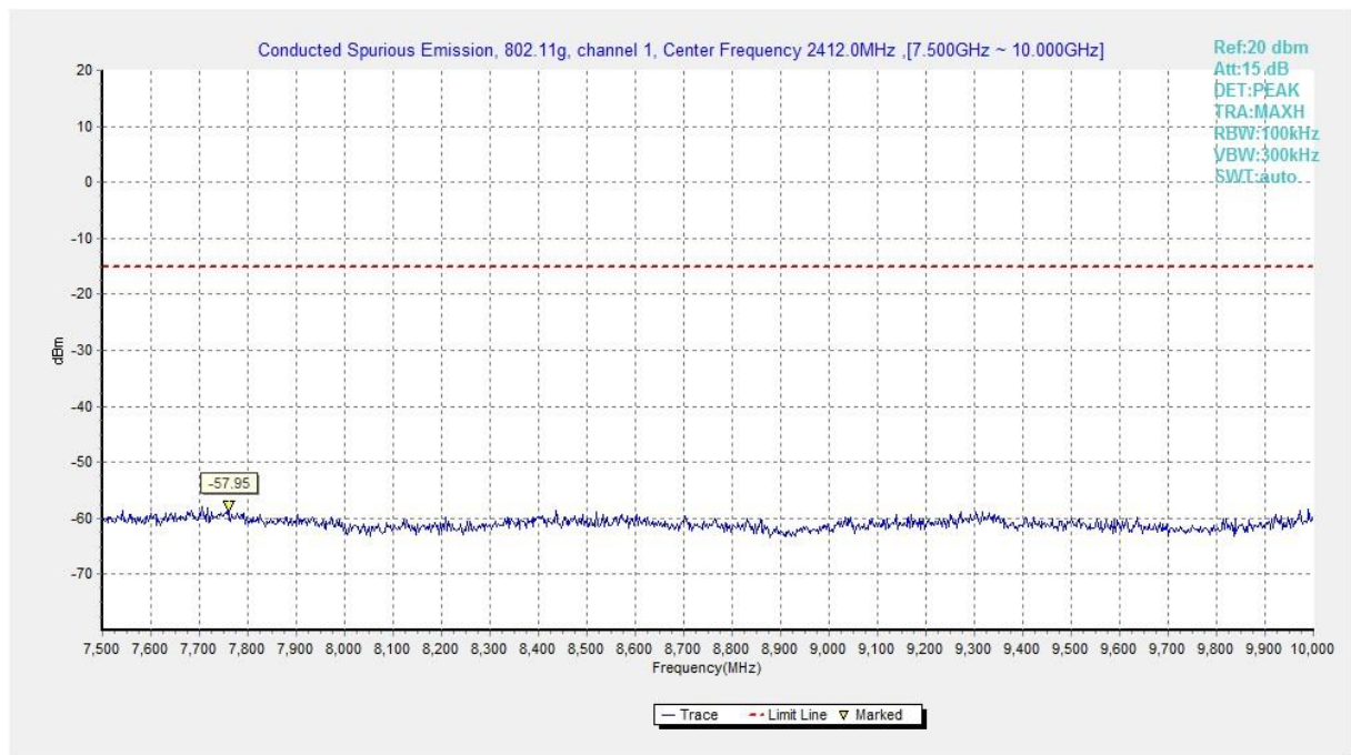
Fig.A.6.1.365 Transmitter Spurious Emission - Conducted (802.11g, Ch1, 7.5 GHz-10 GHz)
