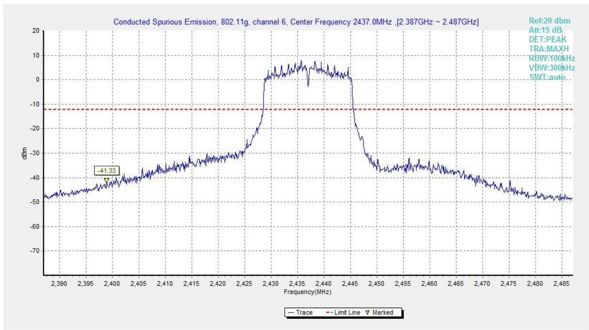
Fig.A.6.1.369 Transmitter Spurious Emission - Conducted (802.11g, Ch6, Center Frequency)
