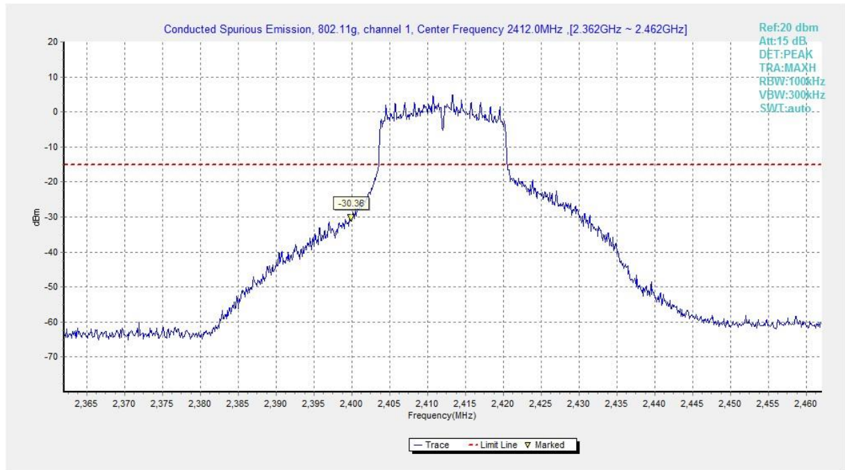
Fig.A.6.1.361 Transmitter Spurious Emission - Conducted (802.11g, Ch1, Center Frequency)
