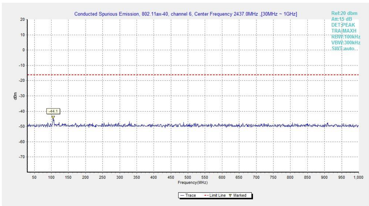
Fig.A.6.1.346 Transmitter Spurious Emission - Conducted(802.11ax-HE40-RU52-left, Ch6, 30 MHz-1 GHz)
