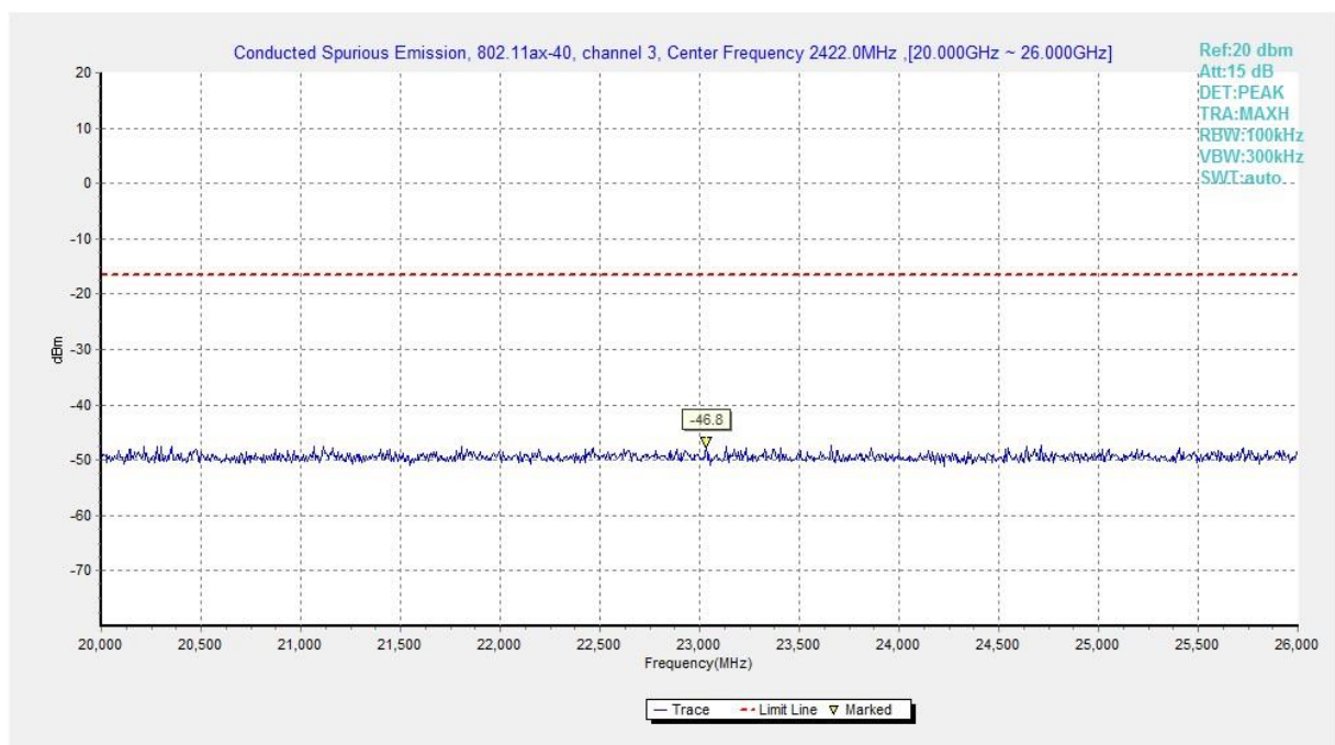
Fig.A.6.1.344 Transmitter Spurious Emission - Conducted (802.11ax-HE40-RU52-left, Ch3, 20 GHz-26 GHz)
