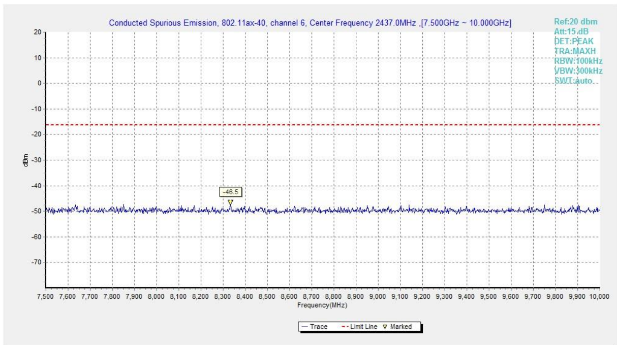
Fig.A.6.1.349 Transmitter Spurious Emission - Conducted (802.11ax-HE40-RU52-left, Ch6, 7.5 GHz-10 GHz)
