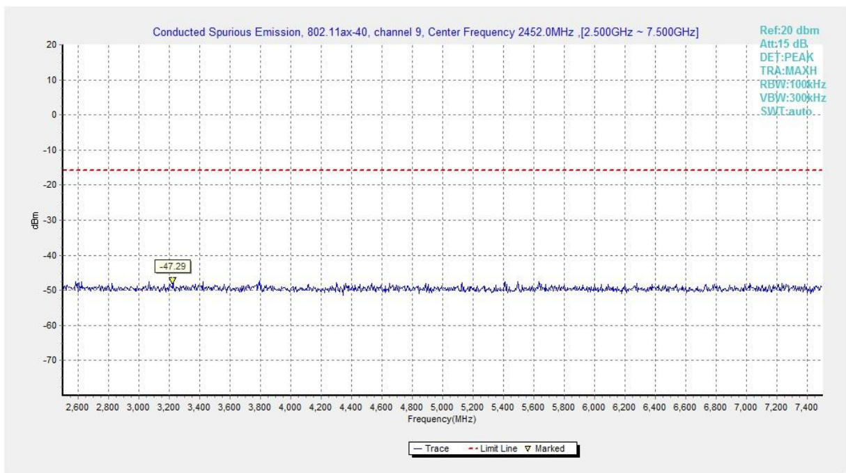
Fig.A.6.1.356 Transmitter Spurious Emission - Conducted (802.11ax-HE40-RU52-left, Ch9, 2.5 GHz-7.5 GHz)
