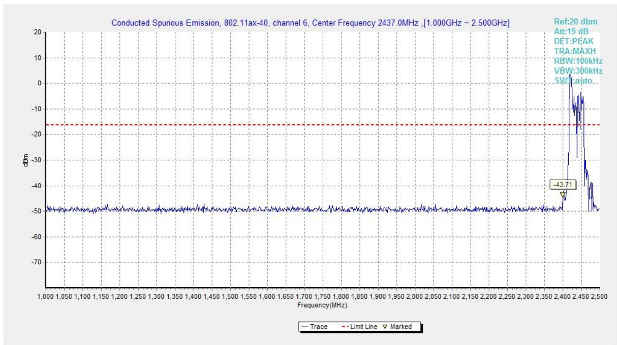
Fig.A.6.1.347 Transmitter Spurious Emission - Conducted (802.11ax-HE40-RU52-left, Ch6, 1 GHz-2.5 GHz)
