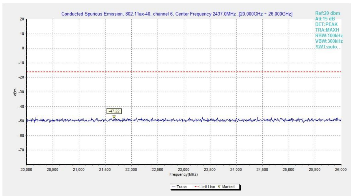
Fig.A.6.1.352 Transmitter Spurious Emission - Conducted (802.11ax-HE40-RU52-left, Ch6, 20 GHz-26 GHz)
