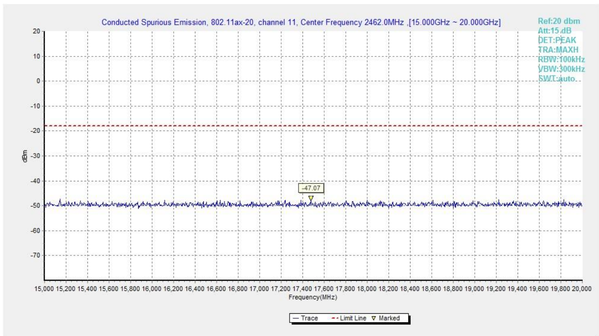
Fig.A.6.1.335 Transmitter Spurious Emission - Conducted (802.11ax-HE20-RU52-right, Ch11, 15 GHz-20 GHz)
