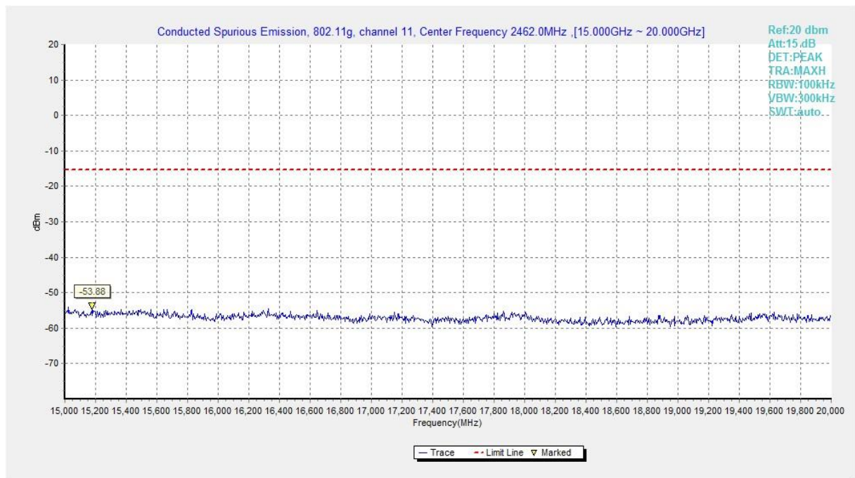
Fig.A.6.1.383 Transmitter Spurious Emission - Conducted (802.11g, Ch11, 15 GHz-20 GHz)
