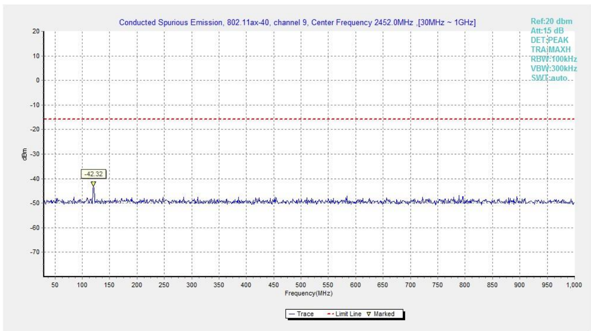
Fig.A.6.1.354 Transmitter Spurious Emission - Conducted(802.11ax-HE40-RU52-left, Ch9, 30 MHz-1 GHz)
