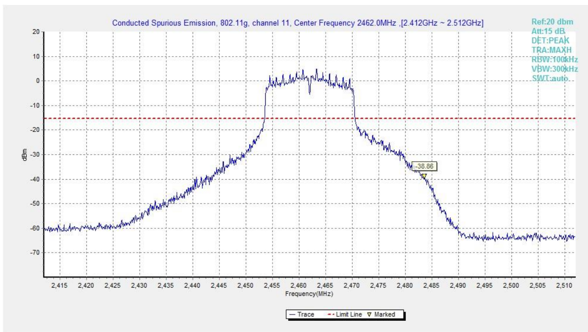
Fig.A.6.1.377 Transmitter Spurious Emission - Conducted (802.11g, Ch11, Center Frequency)
