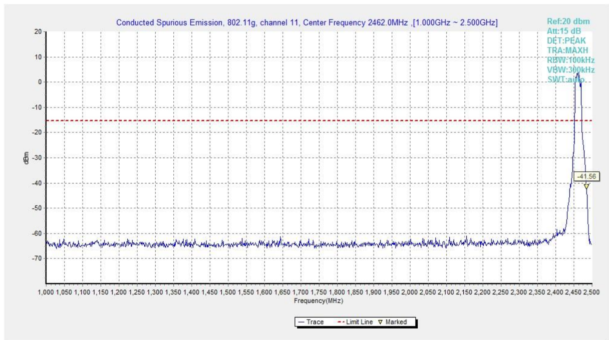
Fig.A.6.1.379 Transmitter Spurious Emission - Conducted (802.11g, Ch11, 1 GHz-2.5 GHz)
