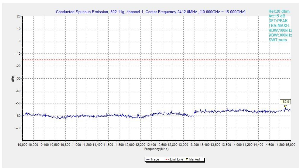
Fig.A.6.1.366 Transmitter Spurious Emission - Conducted (802.11g, Ch1, 10 GHz-15 GHz)
