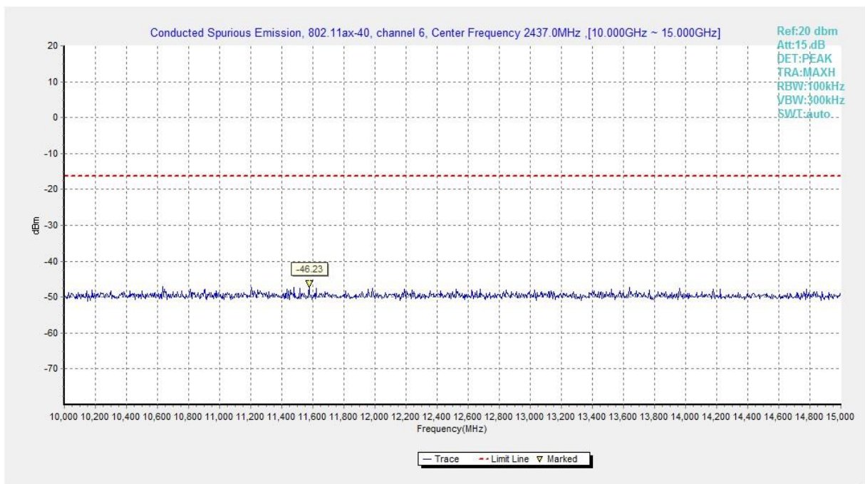
Fig.A.6.1.350 Transmitter Spurious Emission - Conducted (802.11ax-HE40-RU52-left, Ch6, 10 GHz-15 GHz)
