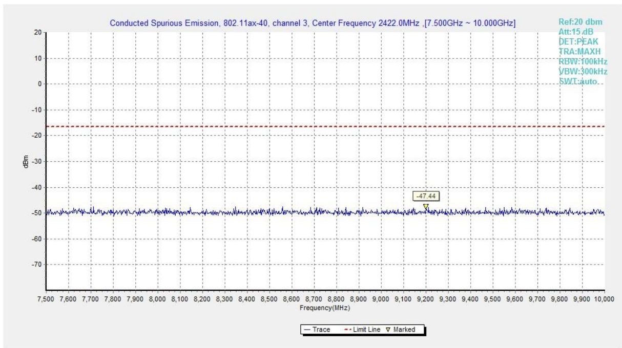
Fig.A.6.1.341 Transmitter Spurious Emission - Conducted (802.11ax-HE40-RU52-left, Ch3, 7.5 GHz-10 GHz)
