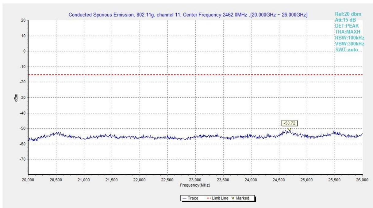
Fig.A.6.1.384 Transmitter Spurious Emission - Conducted (802.11g, Ch11, 20 GHz-26 GHz)
