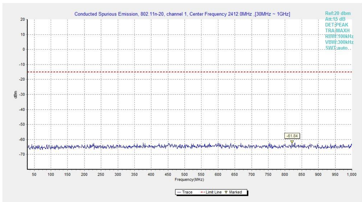
Fig.A.6.1.386 Transmitter Spurious Emission - Conducted (802.11n-HT20, Ch1, 30 MHz-1 GHz)
