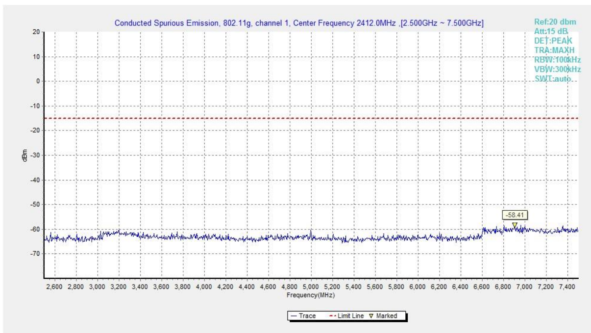
Fig.A.6.1.364 Transmitter Spurious Emission - Conducted (802.11g, Ch1, 2.5 GHz-7.5 GHz)
