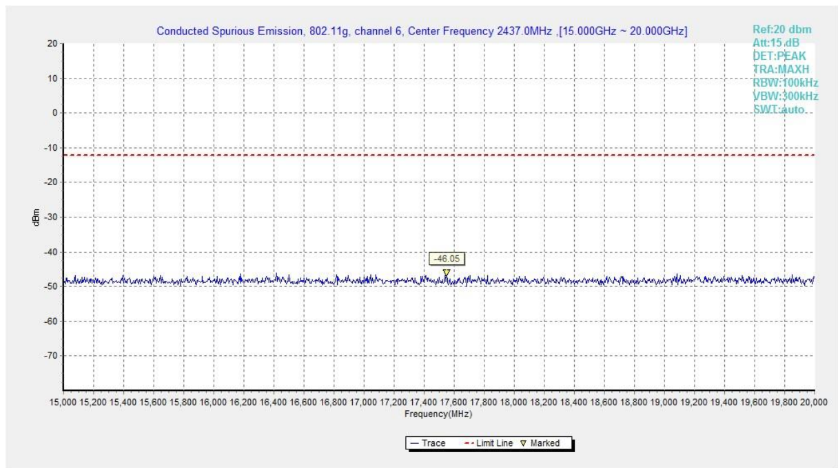
Fig.A.6.1.375 Transmitter Spurious Emission - Conducted (802.11g, Ch6, 15 GHz-20 GHz)
