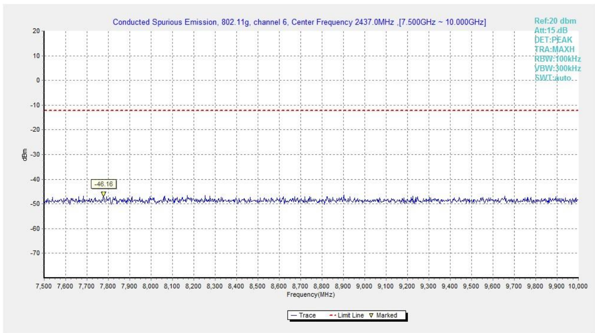
Fig.A.6.1.373 Transmitter Spurious Emission - Conducted (802.11g, Ch6, 7.5 GHz-10 GHz)
