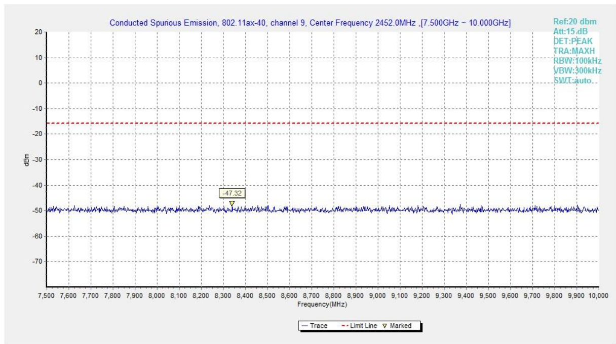
Fig.A.6.1.357 Transmitter Spurious Emission - Conducted(802.11ax-HE40-RU52-left, Ch9, 7.5 GHz-10 GHz)
