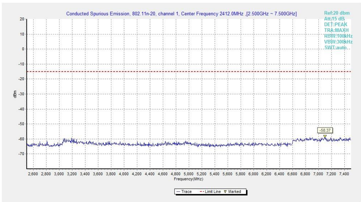
Fig.A.6.1.388 Transmitter Spurious Emission - Conducted (802.11n-HT20, Ch1, 2.5 GHz-7.5 GHz)
