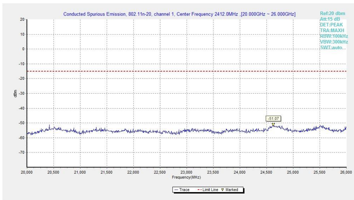
Fig.A.6.1.392 Transmitter Spurious Emission - Conducted (802.11n-HT20, Ch1, 20 GHz-26 GHz)
