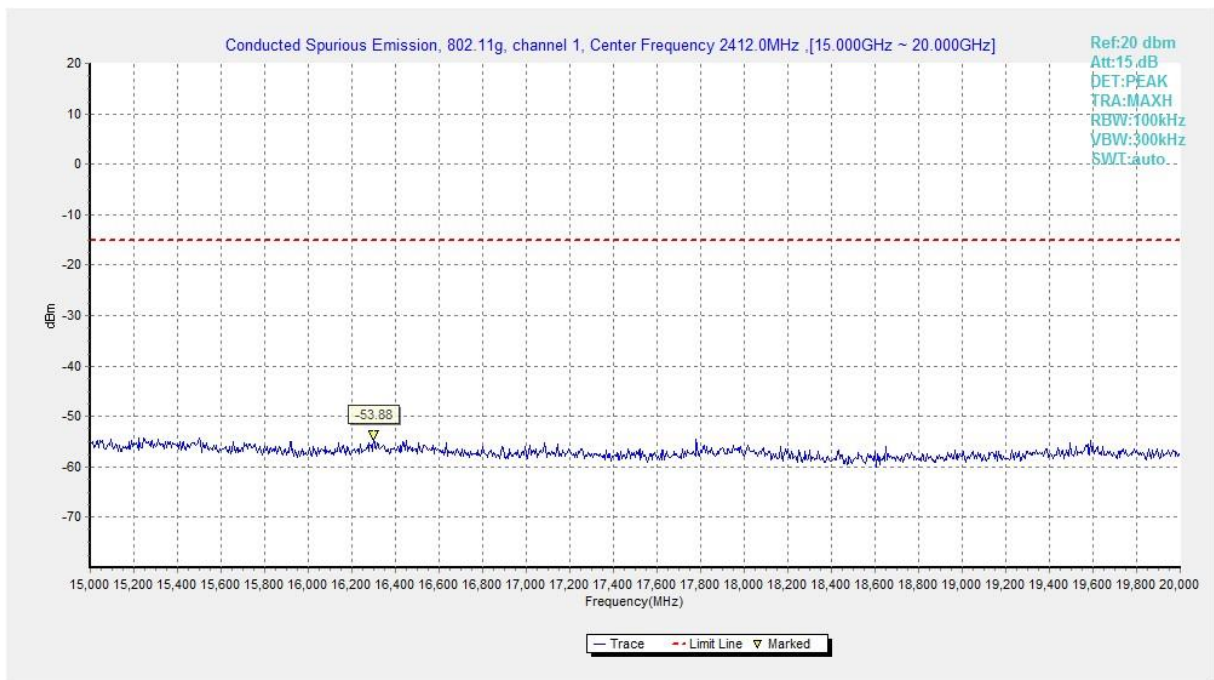
Fig.A.6.1.367 Transmitter Spurious Emission - Conducted (802.11g, Ch1, 15 GHz-20 GHz)
