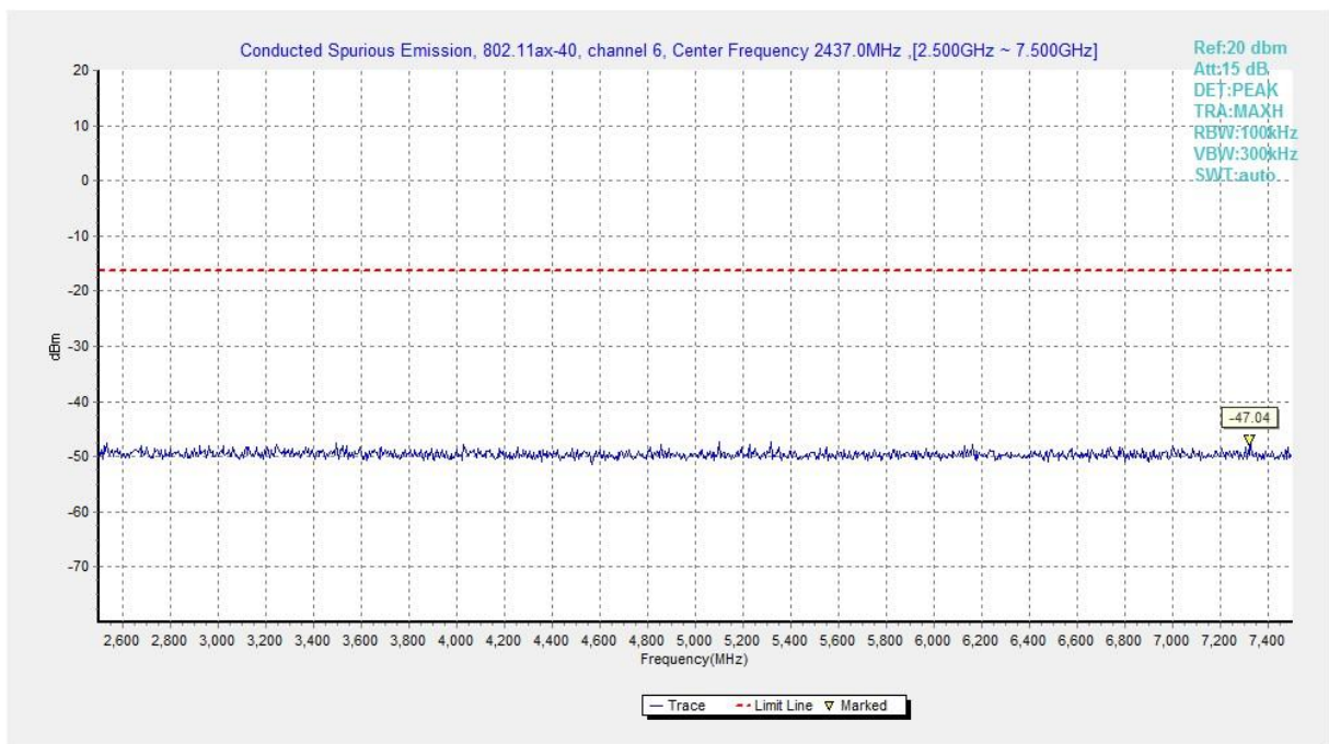
Fig.A.6.1.348 Transmitter Spurious Emission - Conducted (802.11ax-HE40-RU52-left, Ch6, 2.5 GHz-7.5 GHz)
