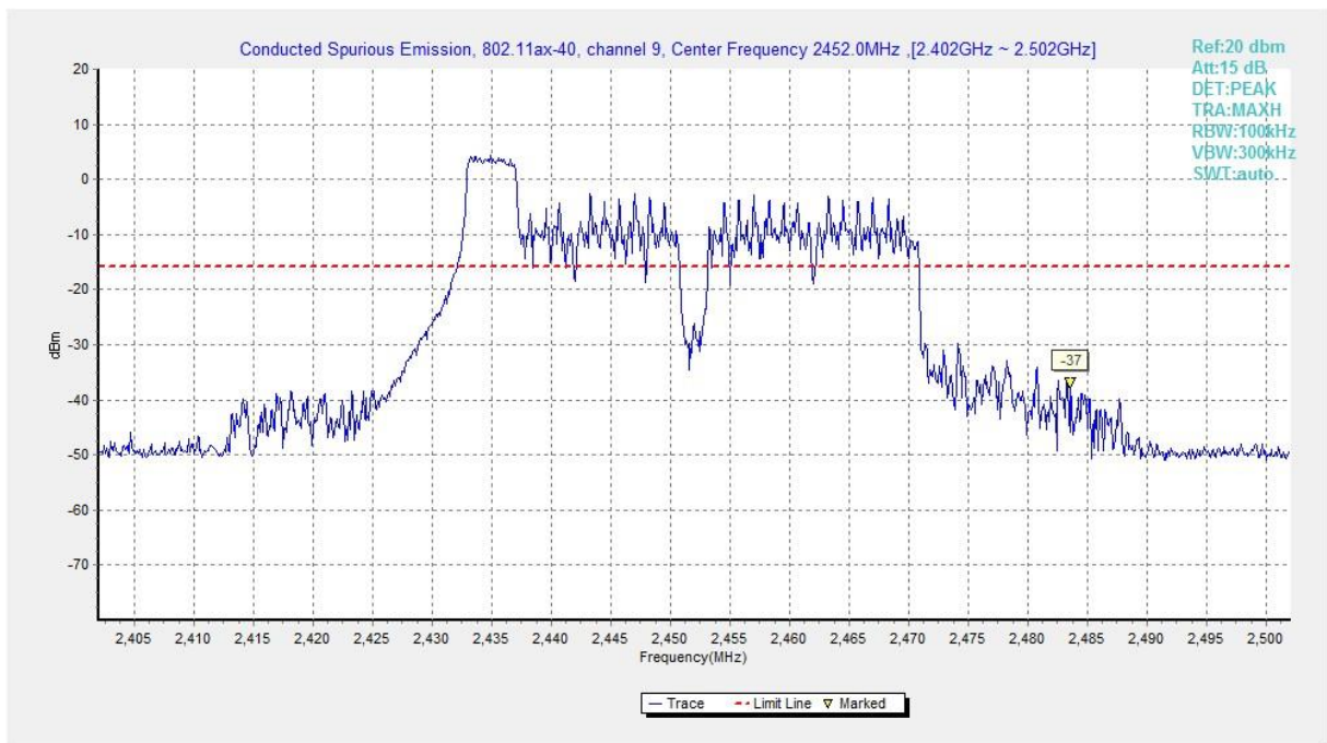
Fig.A.6.1.353 Transmitter Spurious Emission - Conducted(802.11ax-HE40-RU52-left,Ch9, Center Frequency)
