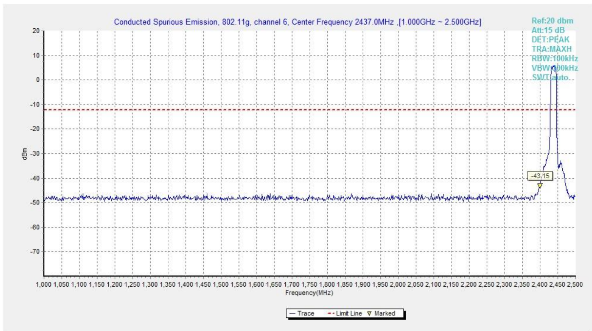
Fig.A.6.1.371 Transmitter Spurious Emission - Conducted (802.11g, Ch6, 1 GHz-2.5 GHz)
