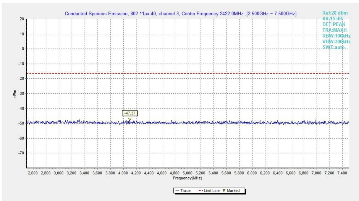
Fig.A.6.1.340 Transmitter Spurious Emission - Conducted (802.11ax-HE40-RU52-left, Ch3, 2.5 GHz-7.5 GHz)
