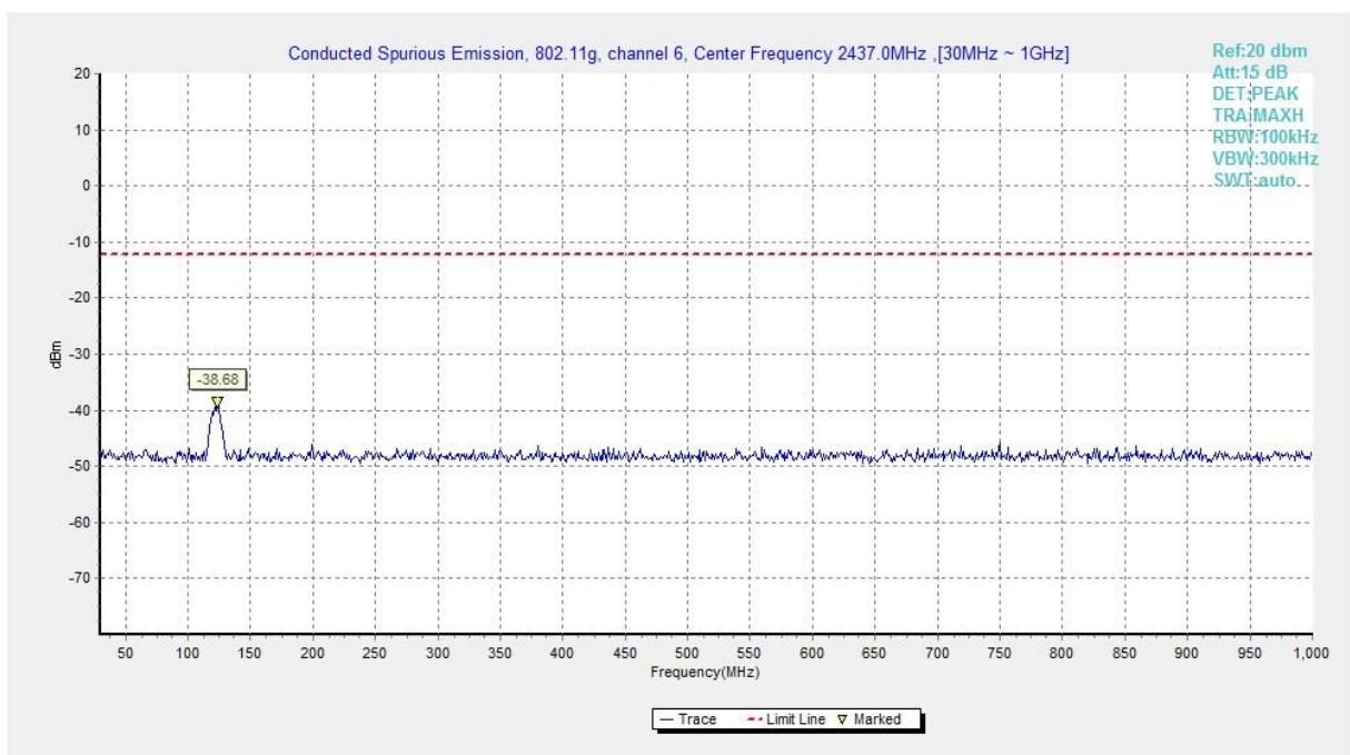
Fig.A.6.1.370 Transmitter Spurious Emission - Conducted (802.11g, Ch6, 30 MHz-1 GHz)
