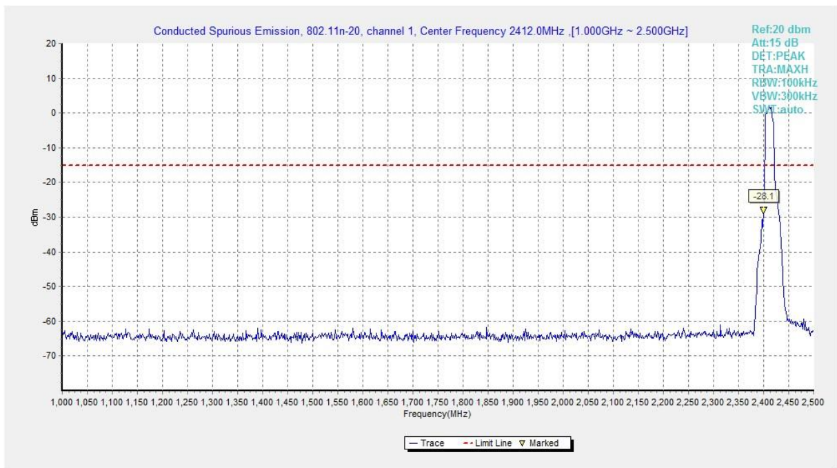
Fig.A.6.1.387 Transmitter Spurious Emission - Conducted (802.11n-HT20, Ch1, 1 GHz-2.5 GHz)
