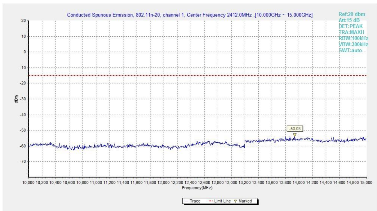
Fig.A.6.1.390 Transmitter Spurious Emission - Conducted (802.11n-HT20, Ch1, 10 GHz-15 GHz)
