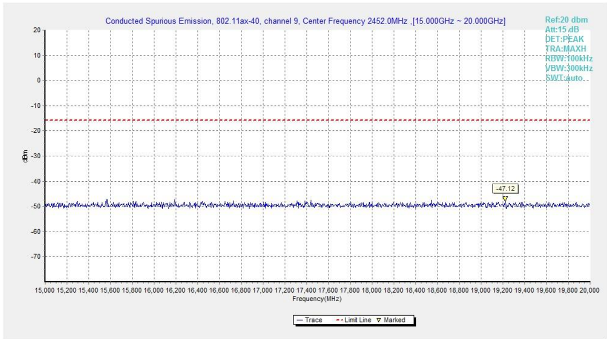
Fig.A.6.1.359 Transmitter Spurious Emission - Conducted (802.11ax-HE40-RU52-left, Ch9, 15 GHz-20 GHz)
