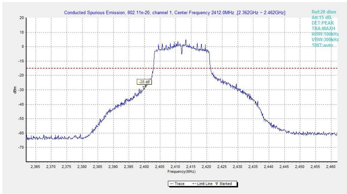
Fig.A.6.1.385 Transmitter Spurious Emission - Conducted (802.11n-HT20, Ch1, Center Frequency)
