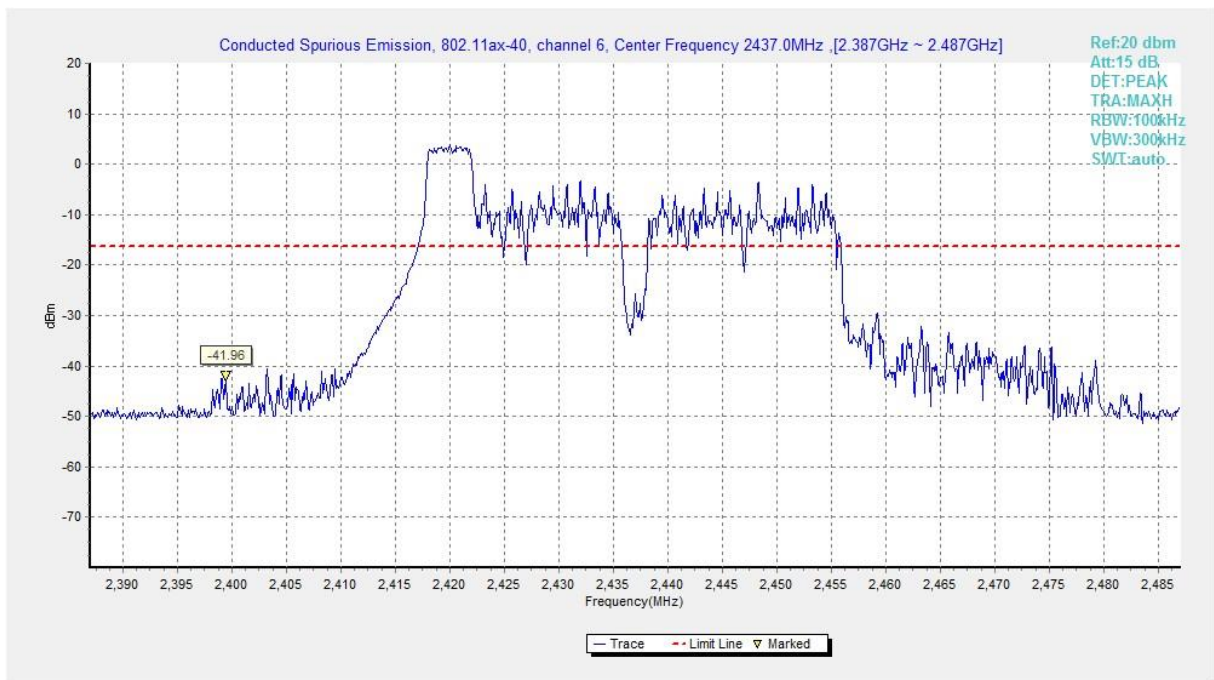
Fig.A.6.1.345 Transmitter Spurious Emission - Conducted (802.11ax-HE40-RU52-left, Ch6, Center Frequency)
