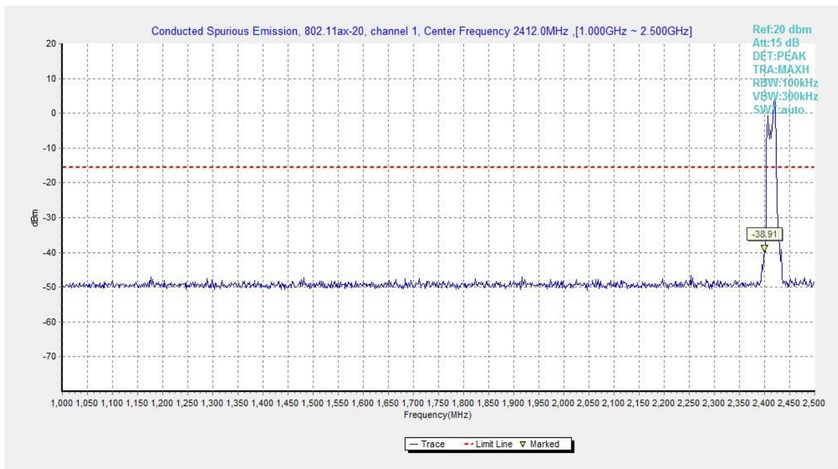
Fig.A.6.1.147 Transmitter Spurious Emission - Conducted (802.11ax-HE20-RU52-right, Ch1, 1 GHz-2.5 GHz)
