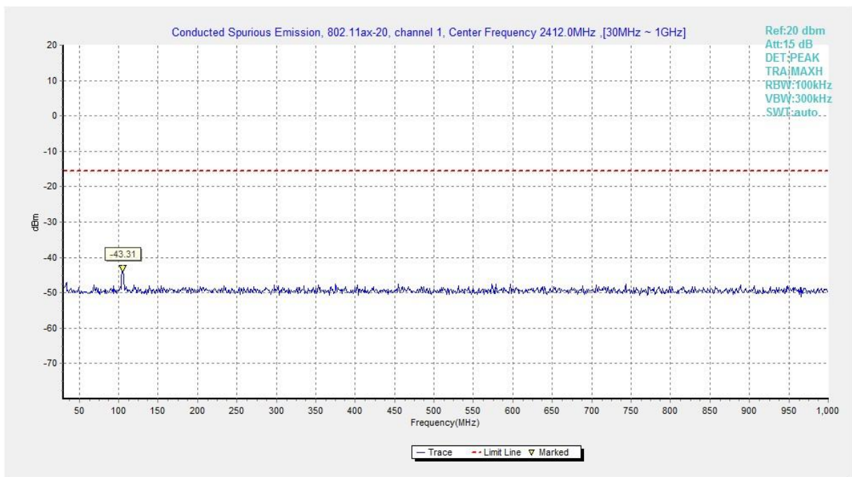
Fig.A.6.1.146 Transmitter Spurious Emission - Conducted (802.11ax-HE20-RU52-right, Ch1, 30 MHz-1 GHz)
