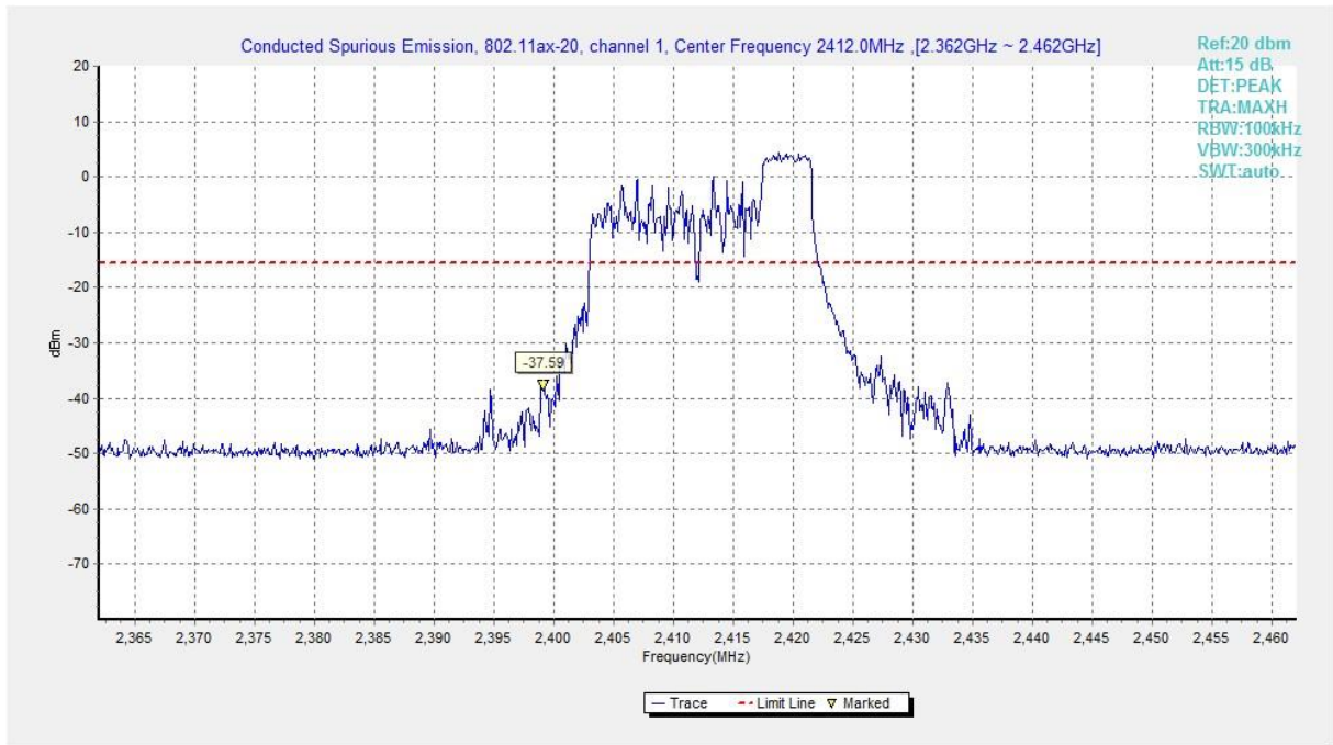
Fig.A.6.1.145 Transmitter Spurious Emission - Conducted (802.11ax-HE20-RU52-right, Ch1, Center Frequency)
