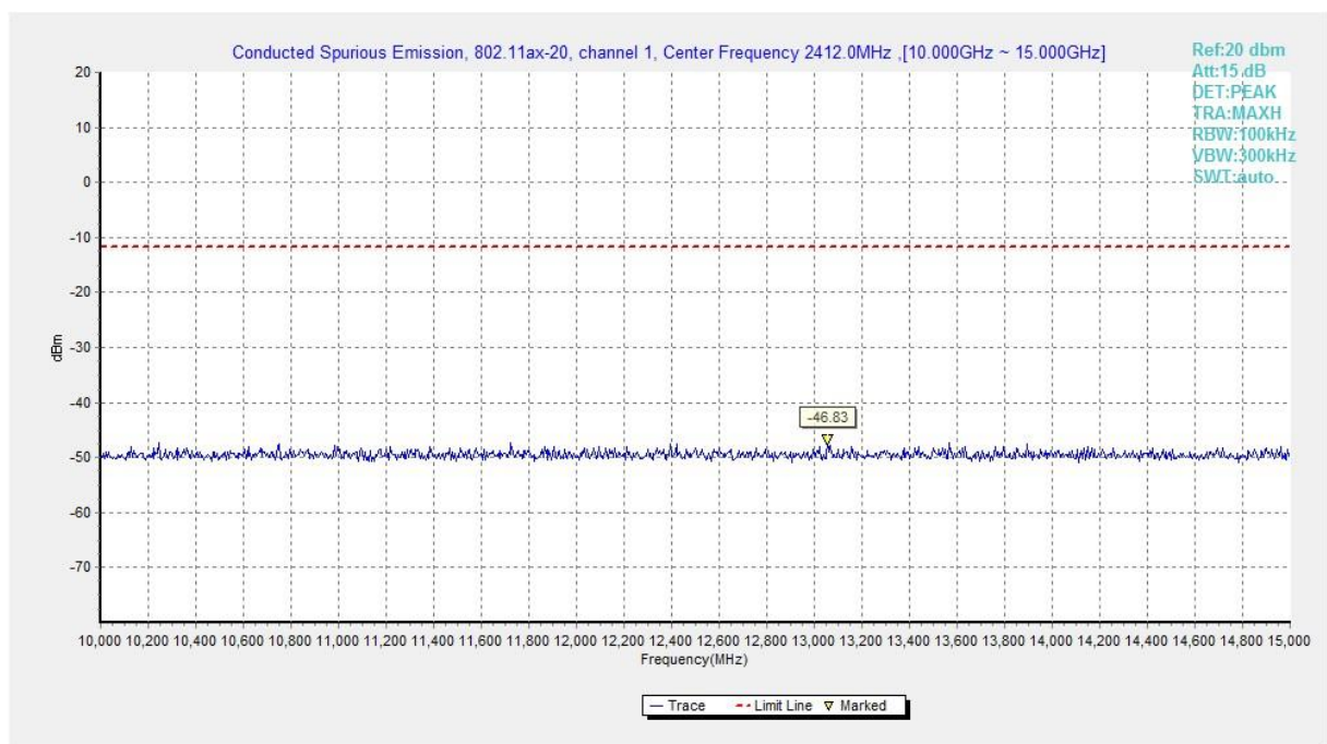
Fig.A.6.1.102 Transmitter Spurious Emission - Conducted (802.11ax-HE20, Ch1, 10 GHz-15 GHz)
