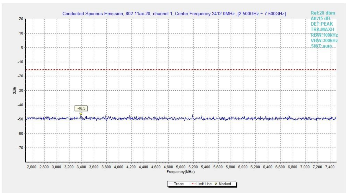
Fig.A.6.1.148 Transmitter Spurious Emission - Conducted (802.11ax-HE20-RU52-right, 2.5 GHz-7.5 GHz)
