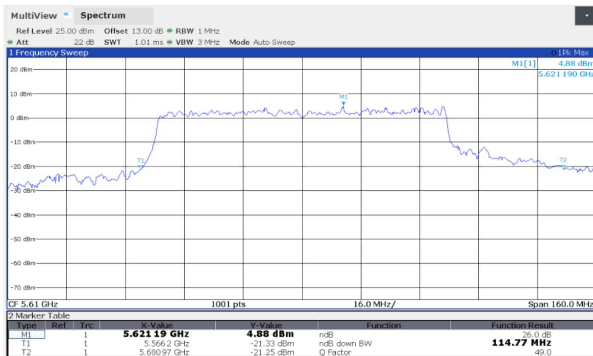
Fig.55 Occupied 26dB Bandwidth (802.11ax-HE80, 5610MHz)
