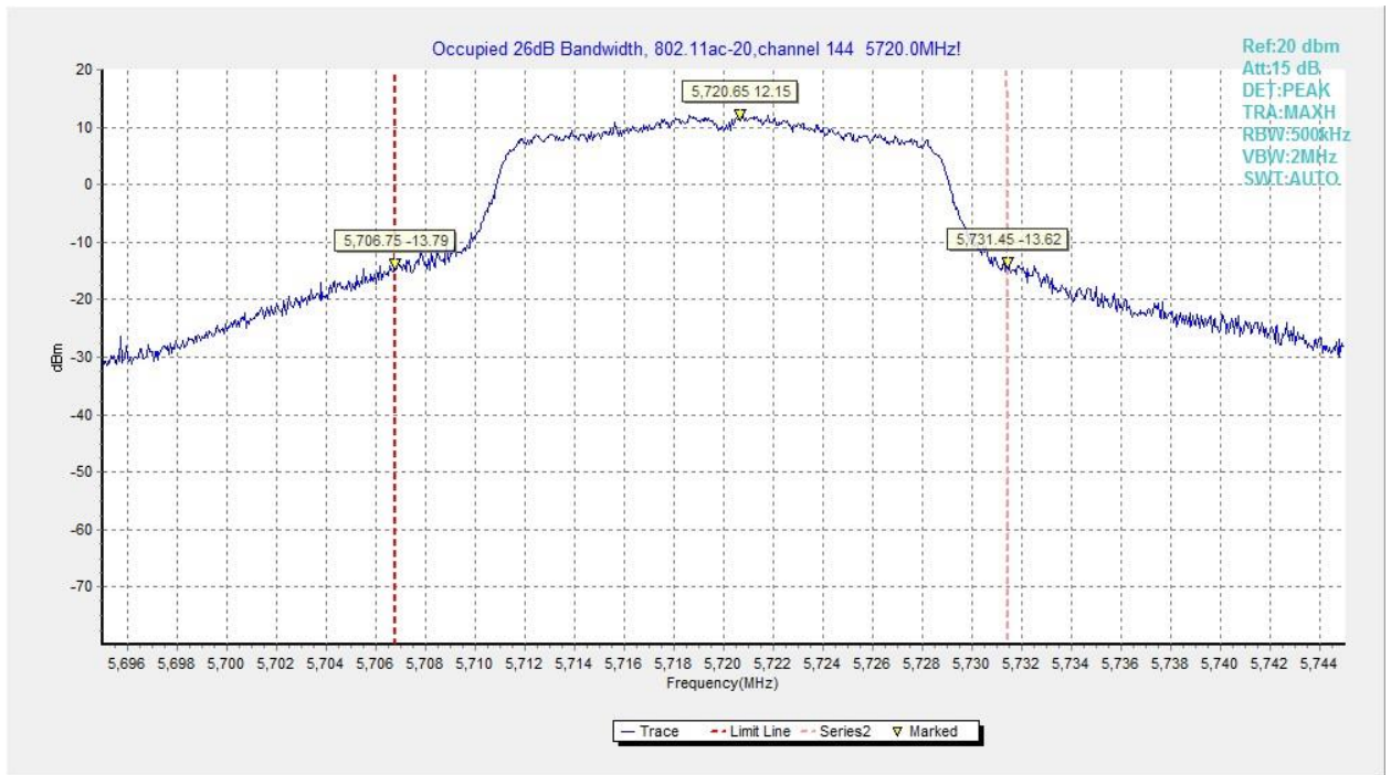
Fig.80 Occupied 26dB Bandwidth (802.11ac-VHT20, 5720MHz)
