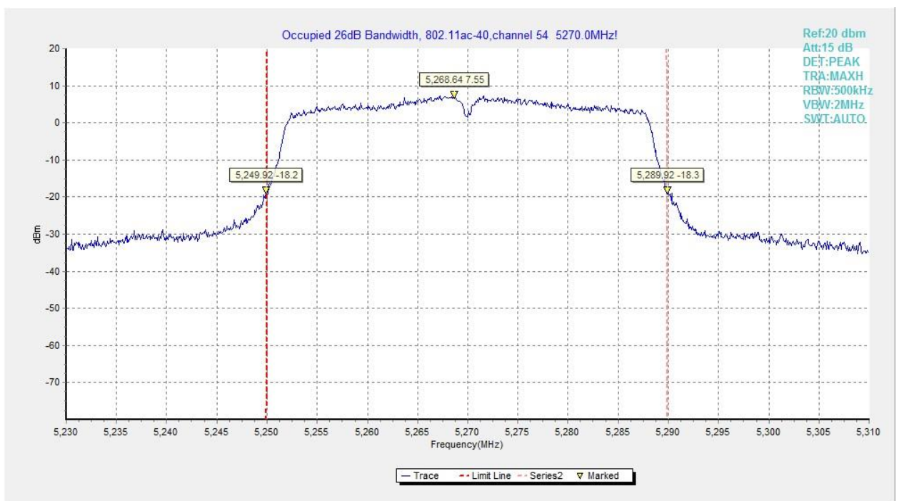
Fig.83 Occupied 26dB Bandwidth (802.11ac-VHT40, 5270MHz)
