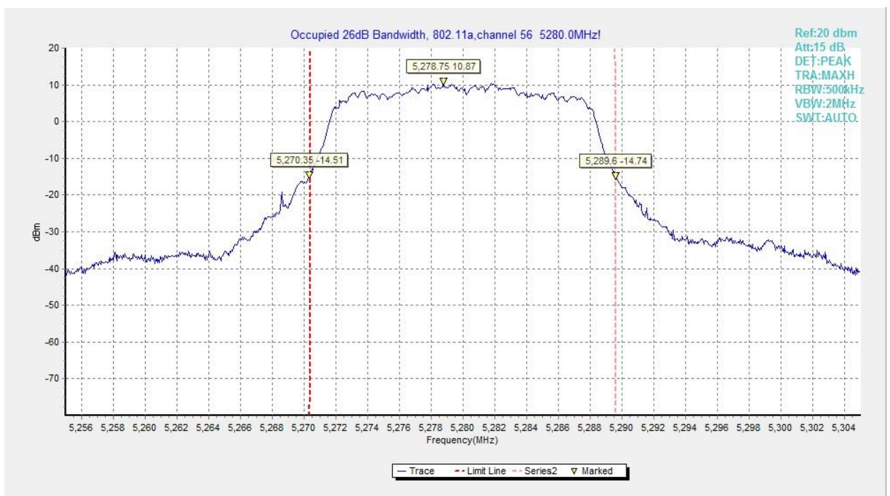
Fig.65 Occupied 26dB Bandwidth (802.11a, 5280MHz)
