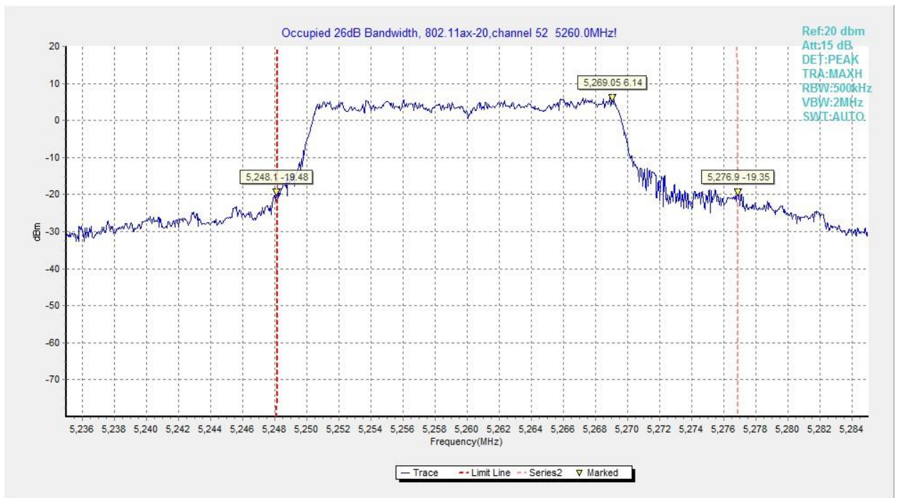
Fig.97 Occupied 26dB Bandwidth (802.11ax-HE20, 5260MHz)
