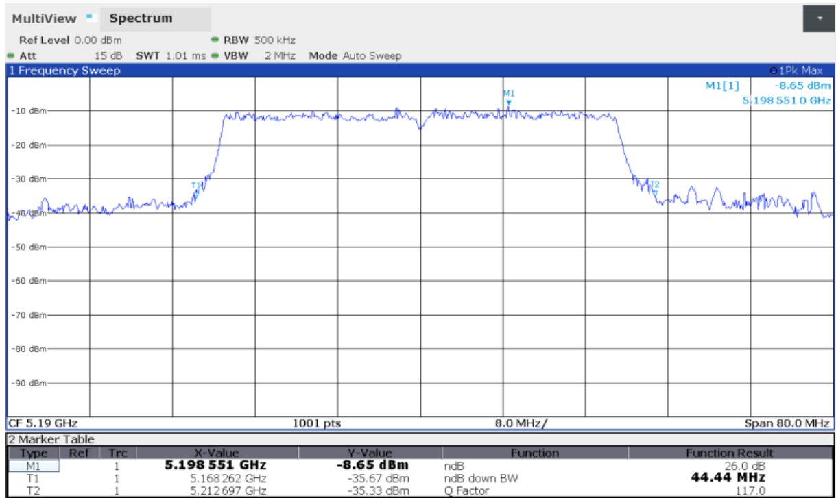
Fig.44 Occupied 26dB Bandwidth (802.11ax-HE40, 5190MHz)
