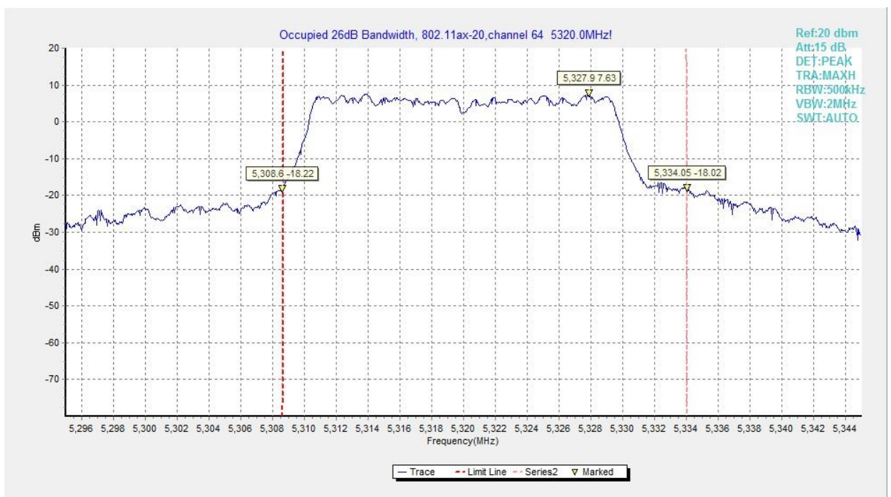
Fig.39 Occupied 26dB Bandwidth (802.11ax-HE20, 5320MHz)
