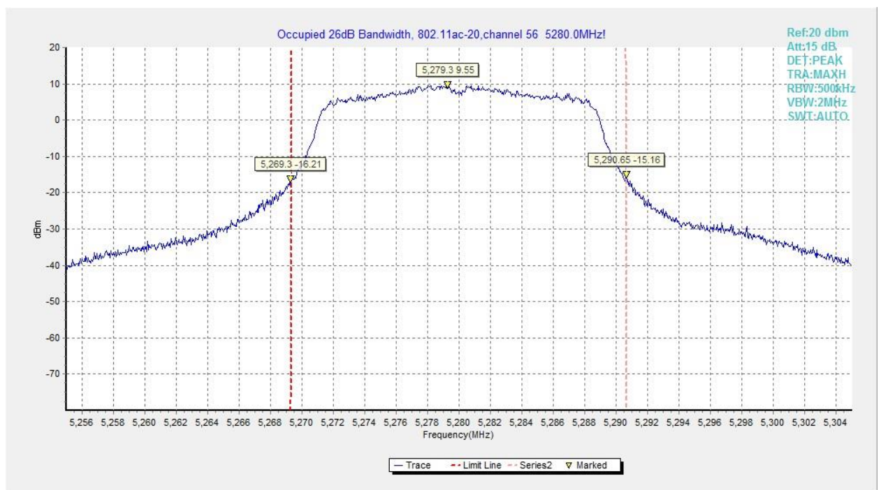
Fig.75 Occupied 26dB Bandwidth (802.11ac-VHT20, 5280MHz)
