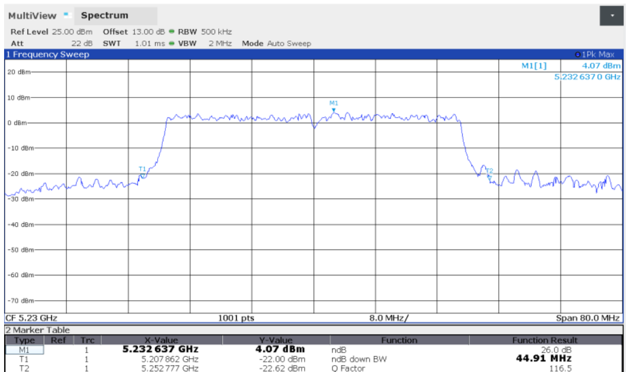
Fig.45 Occupied 26dB Bandwidth (802.11ax-HE40, 5230MHz)
