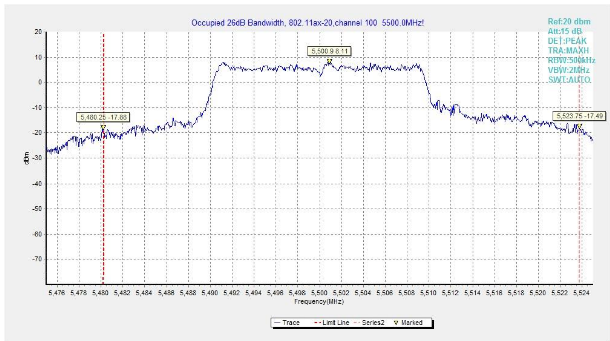
Fig.100 Occupied 26dB Bandwidth (802.11ax-HE20, 5500MHz)
