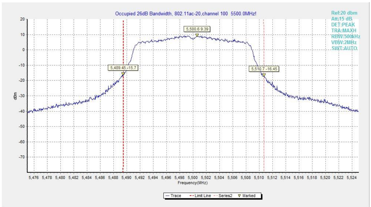
Fig.77 Occupied 26dB Bandwidth (802.11ac-VHT20, 5500MHz)
