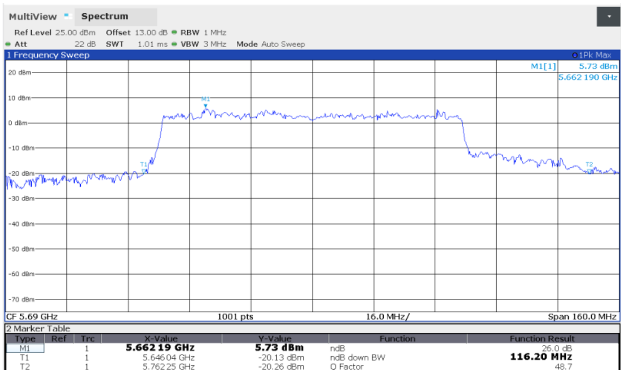
Fig.56 Occupied 26dB Bandwidth (802.11ax-HE80, 5690MHz)
