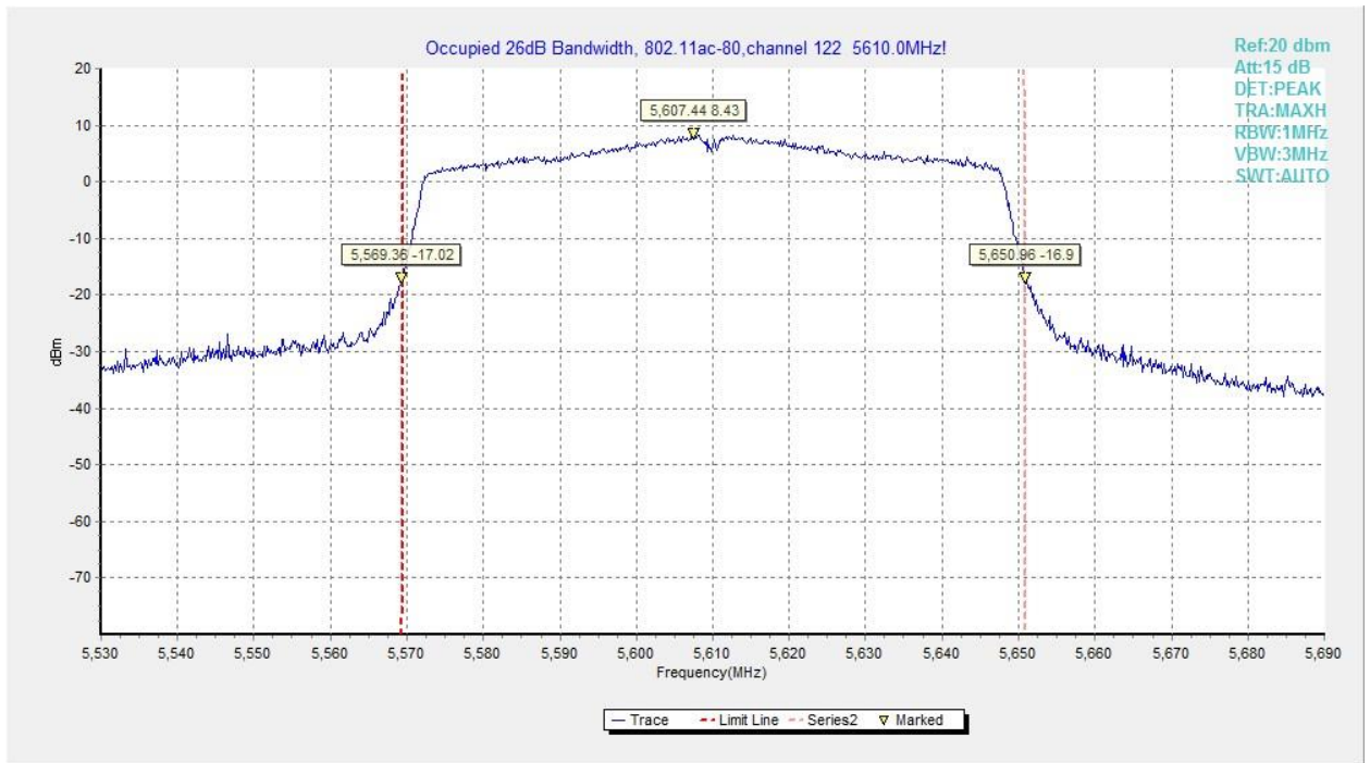
Fig.32 Occupied 26dB Bandwidth (802. 11ac-VHT80, 5610MHz)
