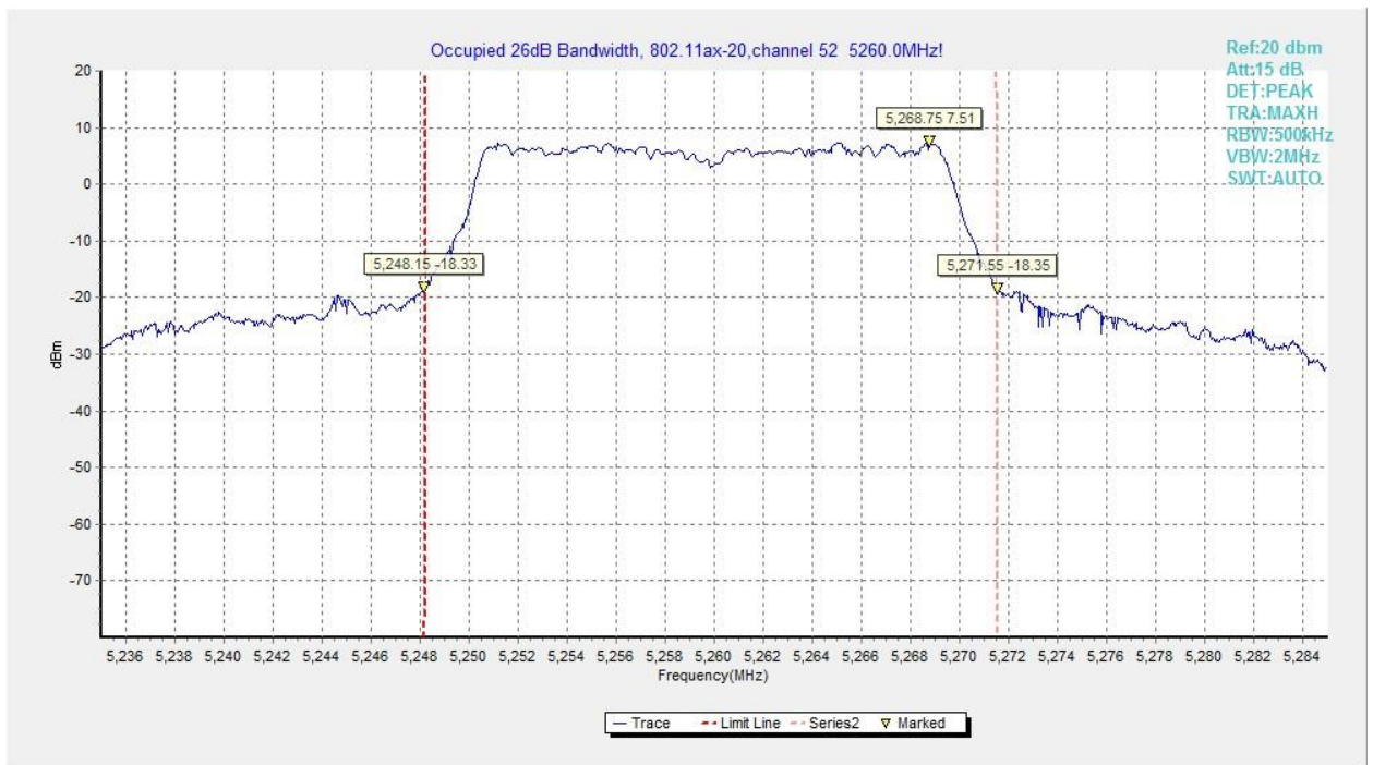
Fig.37 Occupied 26dB Bandwidth (802.11ax-HE20, 5260MHz)
