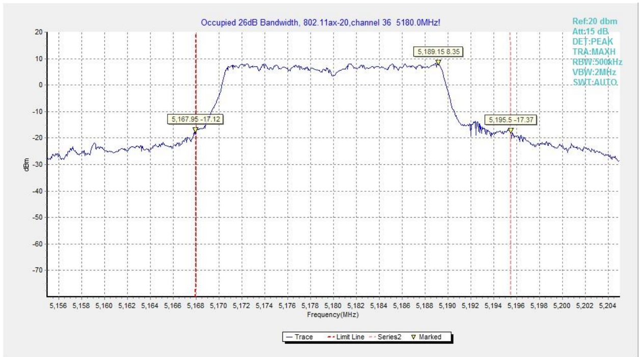
Fig.34 Occupied 26dB Bandwidth (802.11ax-HE20, 5180MHz)
