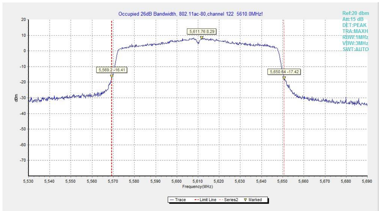
Fig.92 Occupied 26dB Bandwidth (802. 11ac-VHT80, 5610MHz)
