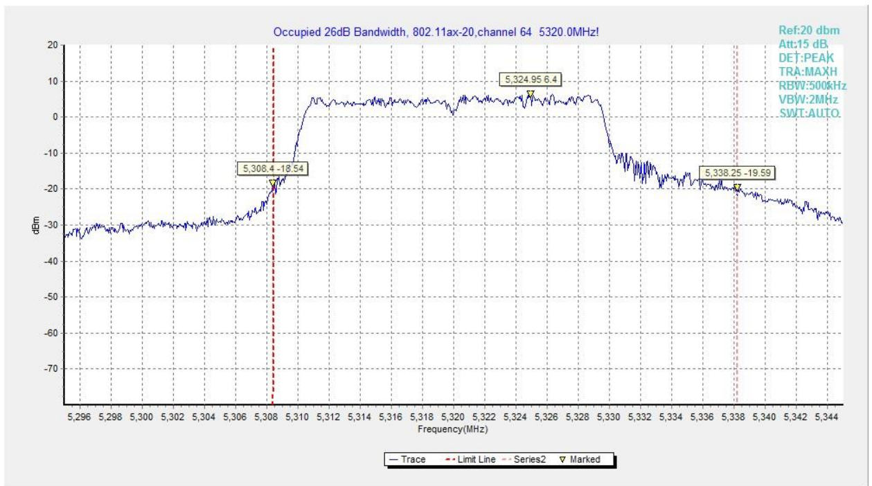
Fig.99 Occupied 26dB Bandwidth (802.11ax-HE20, 5320MHz)
