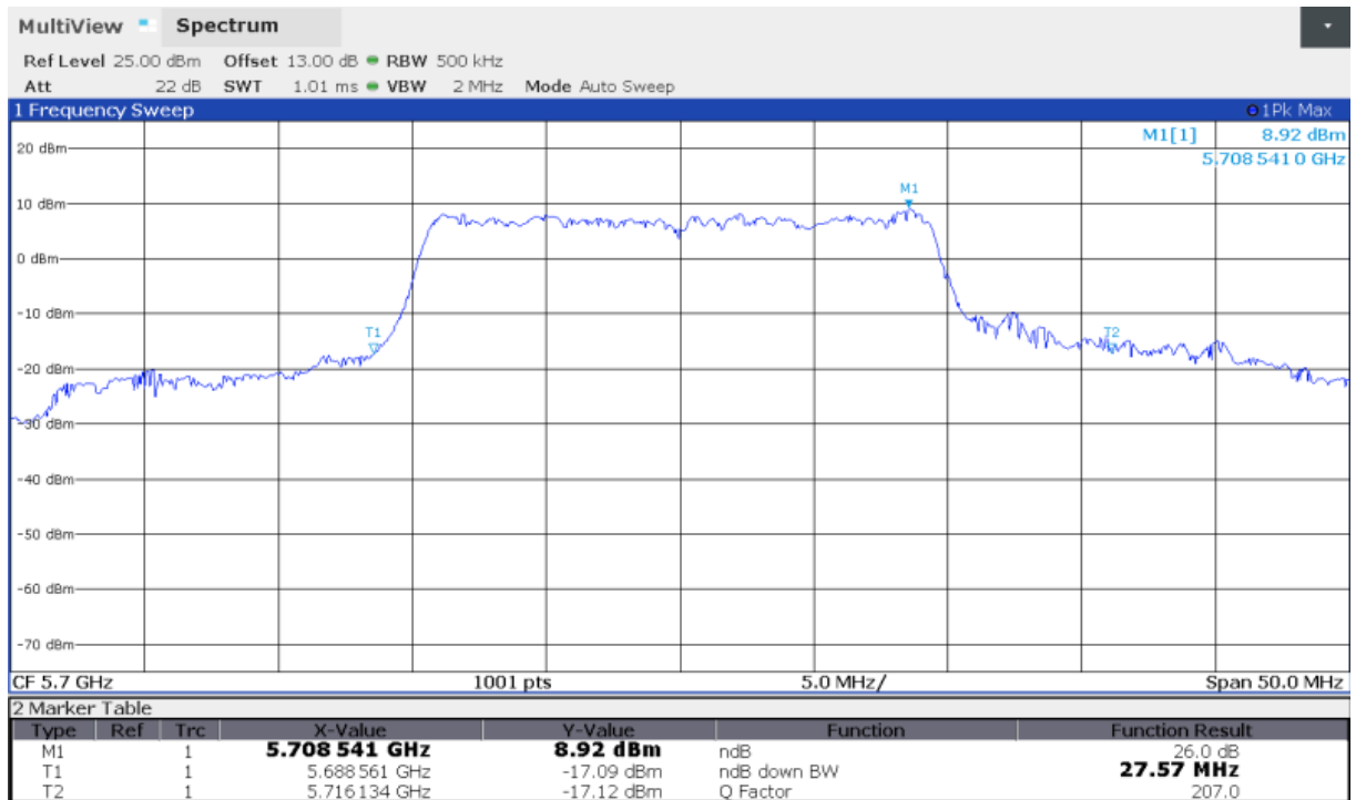
Fig.42 Occupied 26dB Bandwidth (802.11ax-HE20, 5700MHz)
