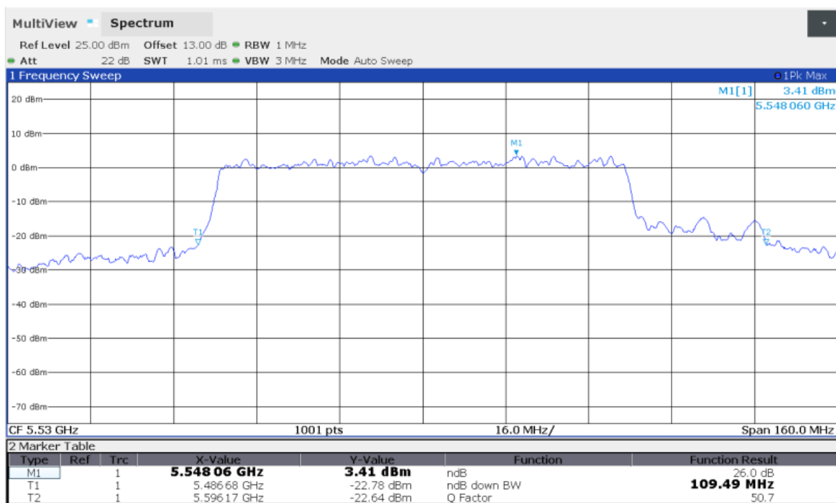
Fig.54 Occupied 26dB Bandwidth (802.11ax-HE80, 5530MHz)
