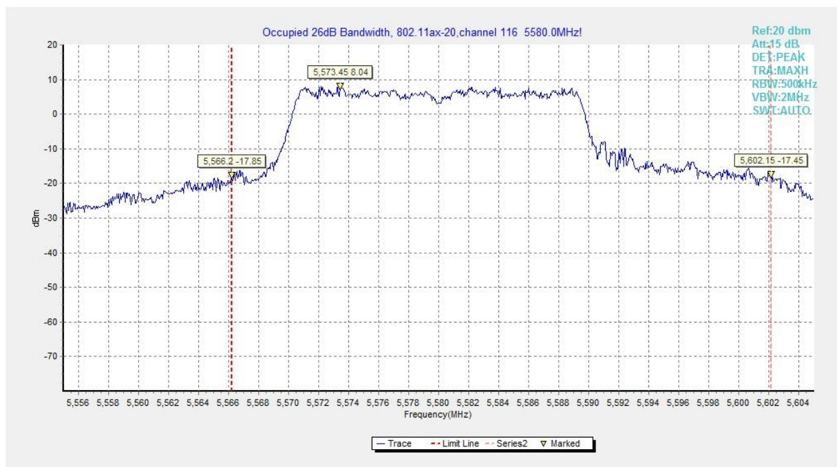
Fig.101 Occupied 26dB Bandwidth (802.11ax-HE20, 5580MHz)
