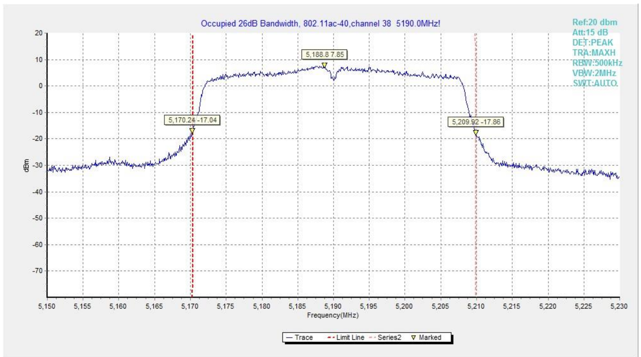
Fig.81 Occupied 26dB Bandwidth (802.11ac-VHT40, 5190MHz)
