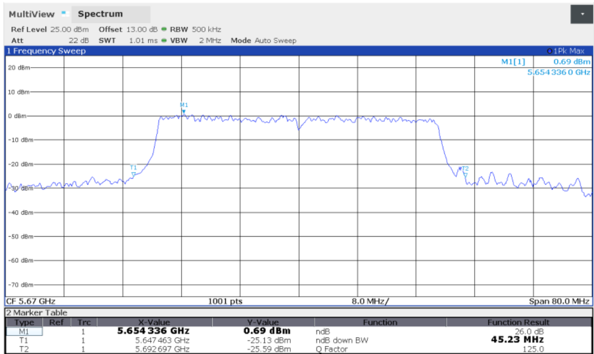
Fig.50 Occupied 26dB Bandwidth (802.11ax-HE40, 5670MHz)
