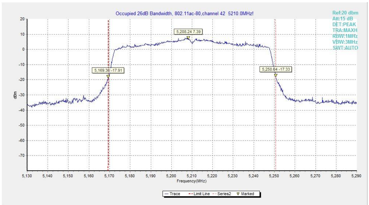
Fig.89 Occupied 26dB Bandwidth (802.11ac-VHT80, 5210MHz)
