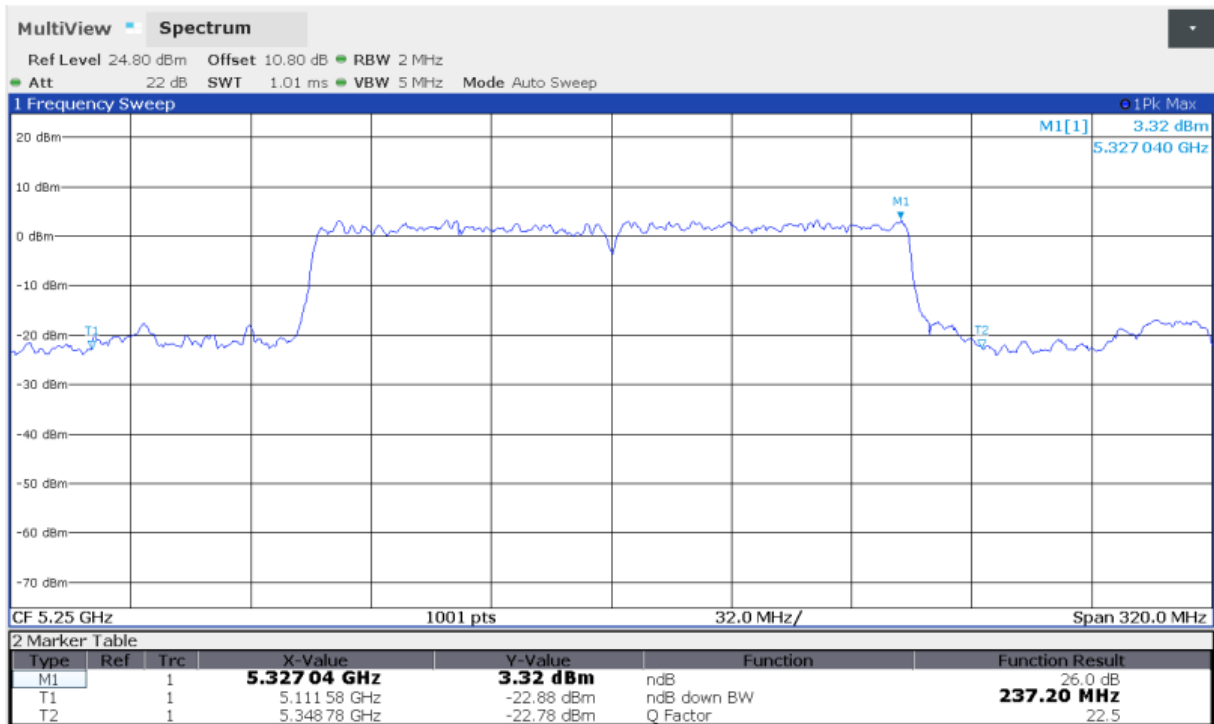
Fig.59 Occupied 26dB Bandwidth (802.11ax-HE160, 5250MHz)
