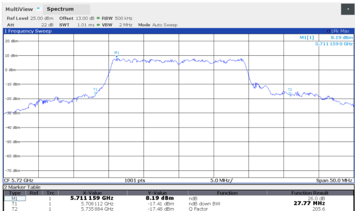
Fig.103 Occupied 26dB Bandwidth (802.11ax-HE20, 5720MHz)
