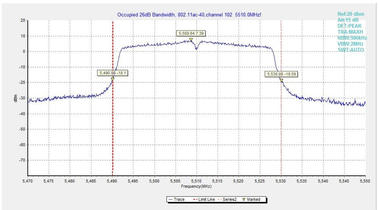
Fig.85 Occupied 26dB Bandwidth (802.11ac-VHT40, 5510MHz)
