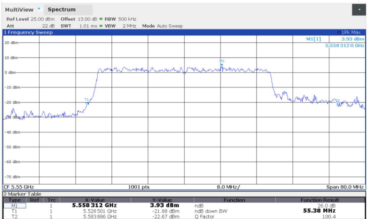
Fig.49 Occupied 26dB Bandwidth (802.11ax-HE40, 5550MHz)
