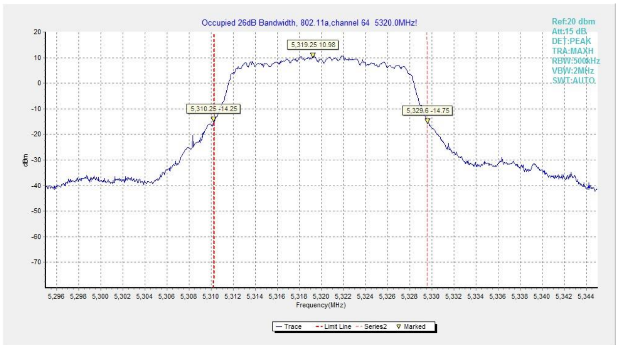
Fig.66 Occupied 26dB Bandwidth (802.11a, 5320MHz)
