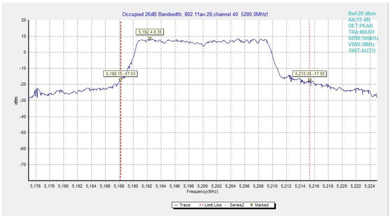
Fig.35 Occupied 26dB Bandwidth (802.11ax-HE20, 5200MHz)
