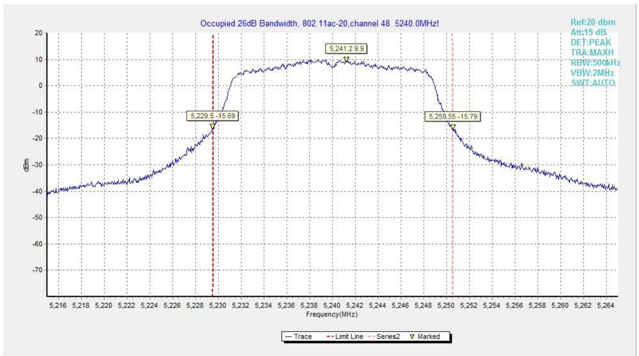
Fig.73 Occupied 26dB Bandwidth (802.11ac-VHT20, 5240MHz)
