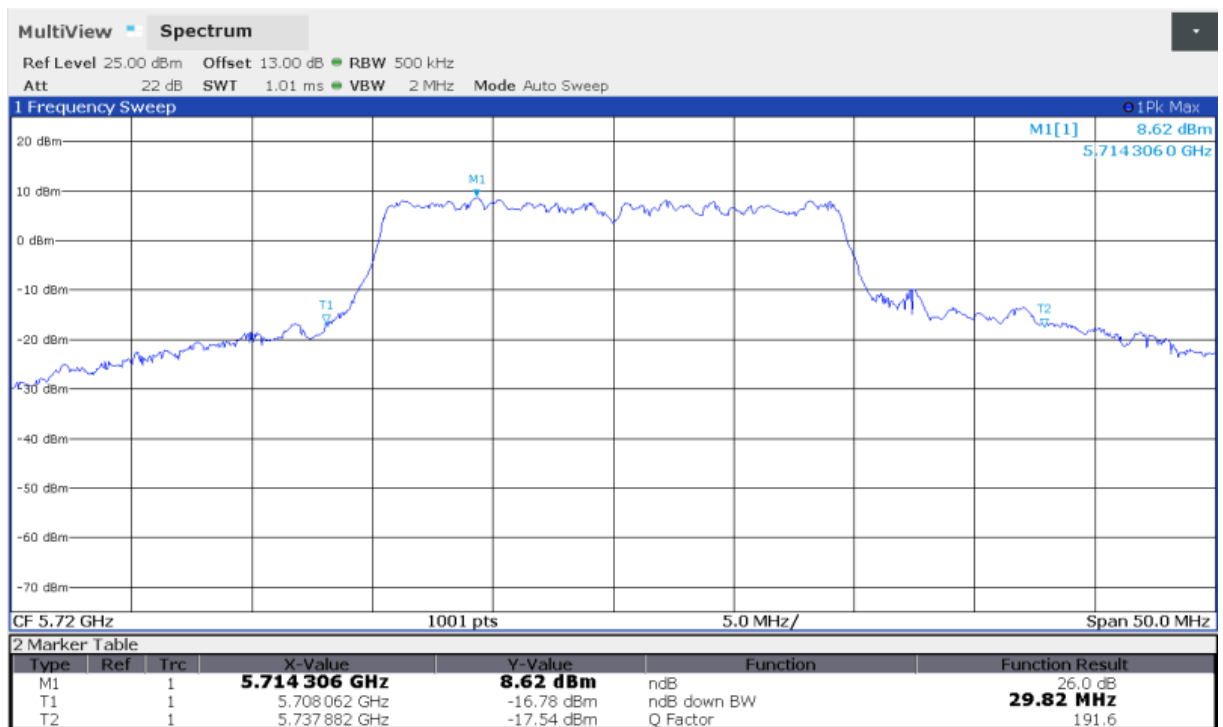
Fig.43 Occupied 26dB Bandwidth (802.11ax-HE20, 5720MHz)
