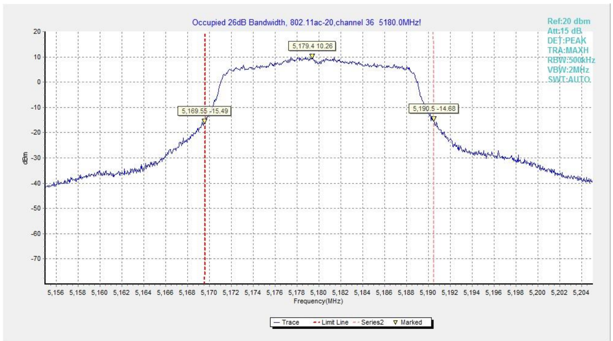
Fig.71 Occupied 26dB Bandwidth (802.11ac-VHT20, 5180MHz)
