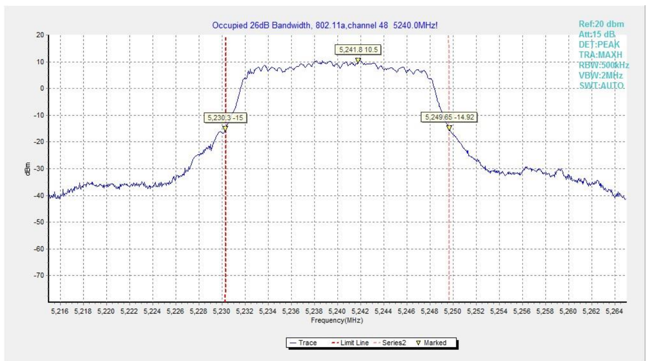
Fig.63 Occupied 26dB Bandwidth (802.11a, 5240MHz)
