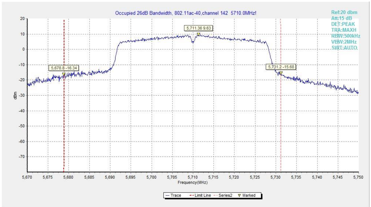
Fig.88 Occupied 26dB Bandwidth (802.11ac-VHT40, 5710MHz)
