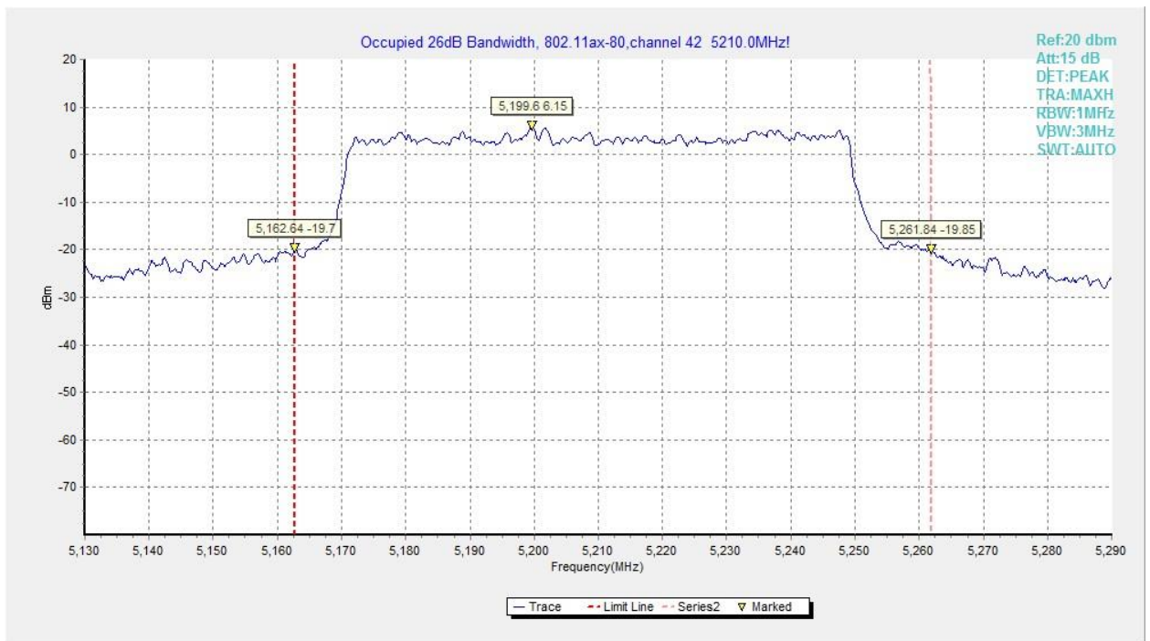
Fig.52 Occupied 26dB Bandwidth (802.11ax-HE80, 5210MHz)
