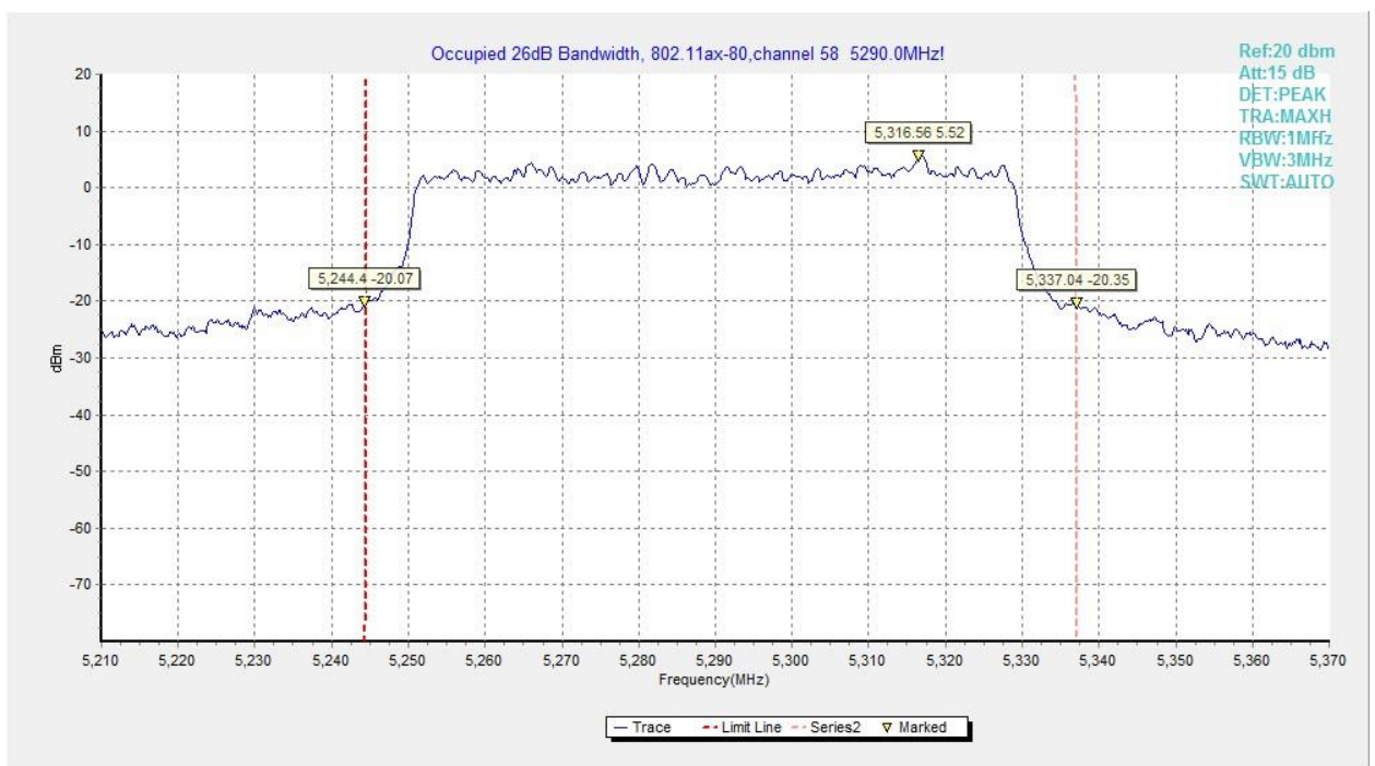
Fig.53 Occupied 26dB Bandwidth (802.11ax-HE80, 5290MHz)
