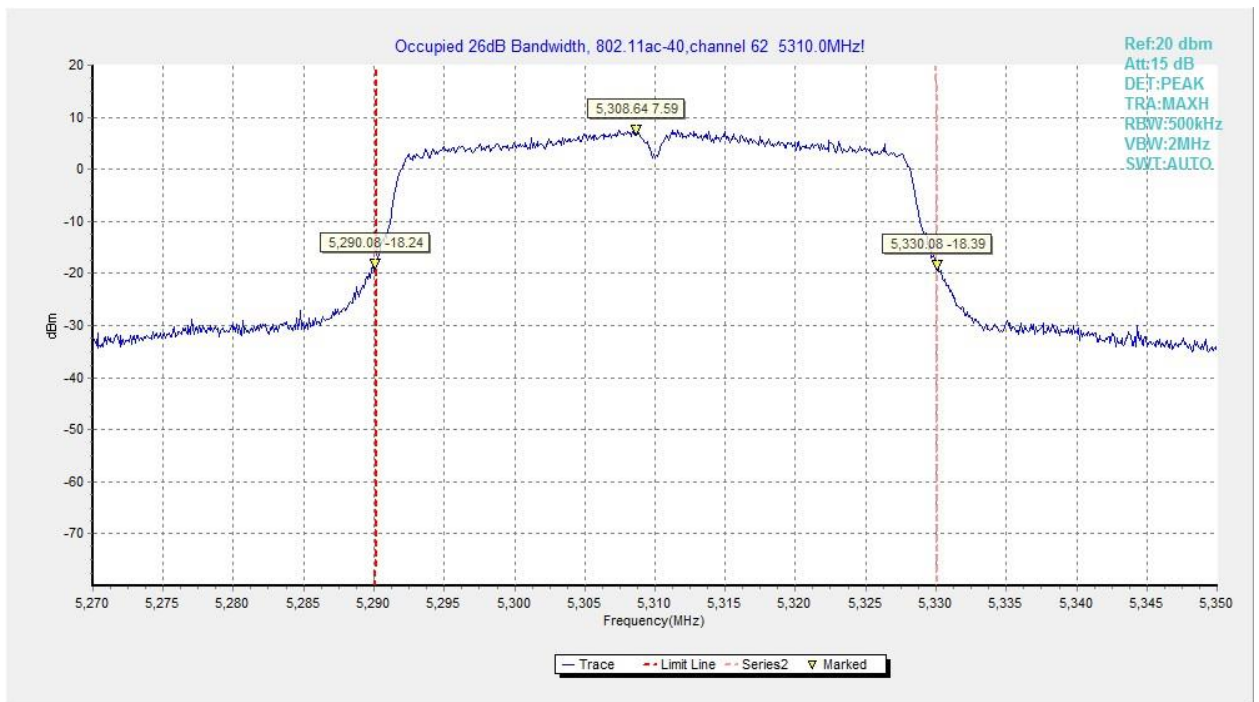
Fig.84 Occupied 26dB Bandwidth (802.11ac-VHT40, 5310MHz)
