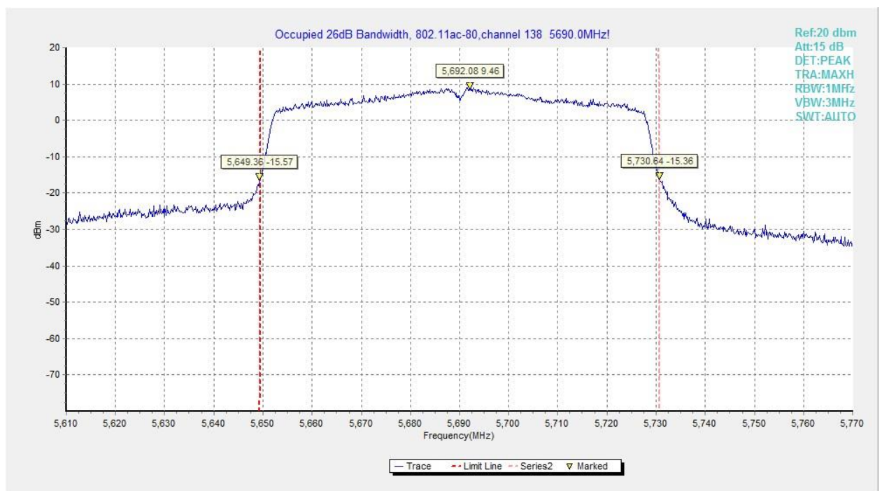
Fig.93 Occupied 26dB Bandwidth (802. 11ac-VHT80, 5690MHz)
