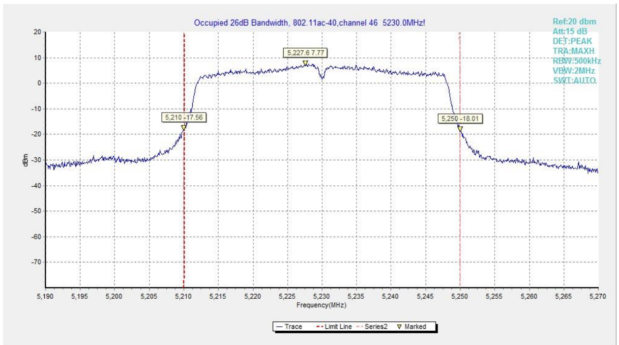
Fig.82 Occupied 26dB Bandwidth (802.11ac-VHT40, 5230MHz)
