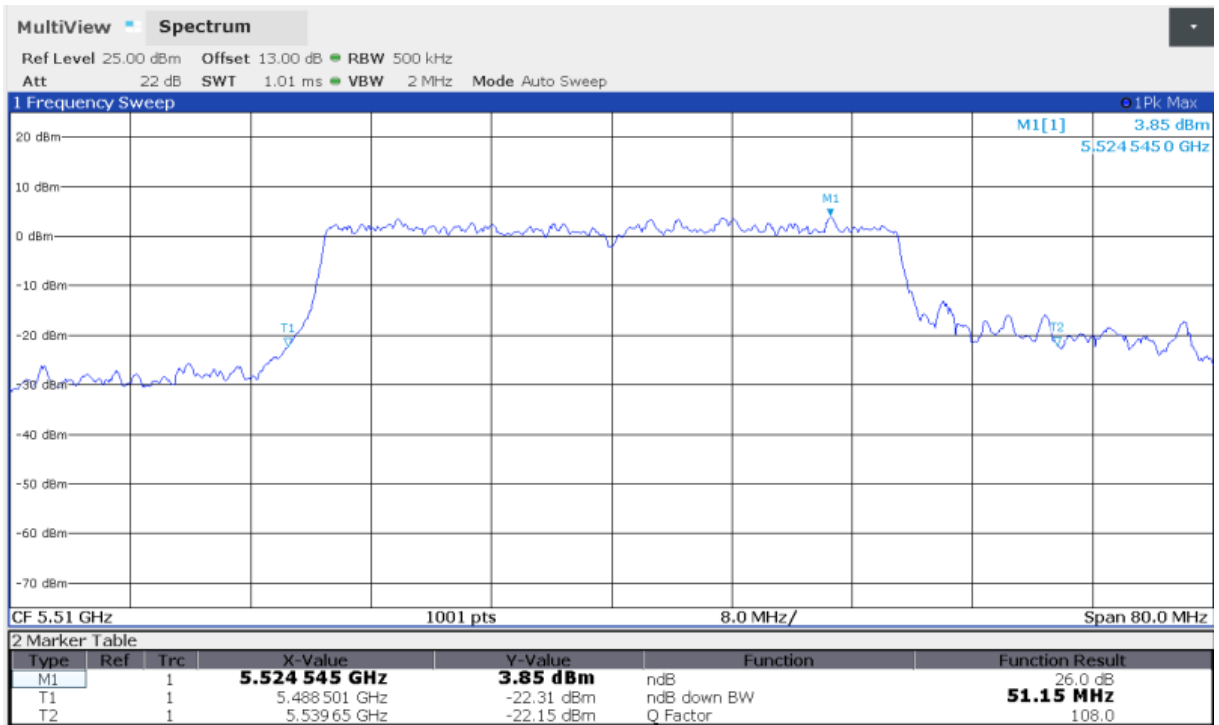
Fig.48 Occupied 26dB Bandwidth (802.11ax-HE40, 5510MHz)
