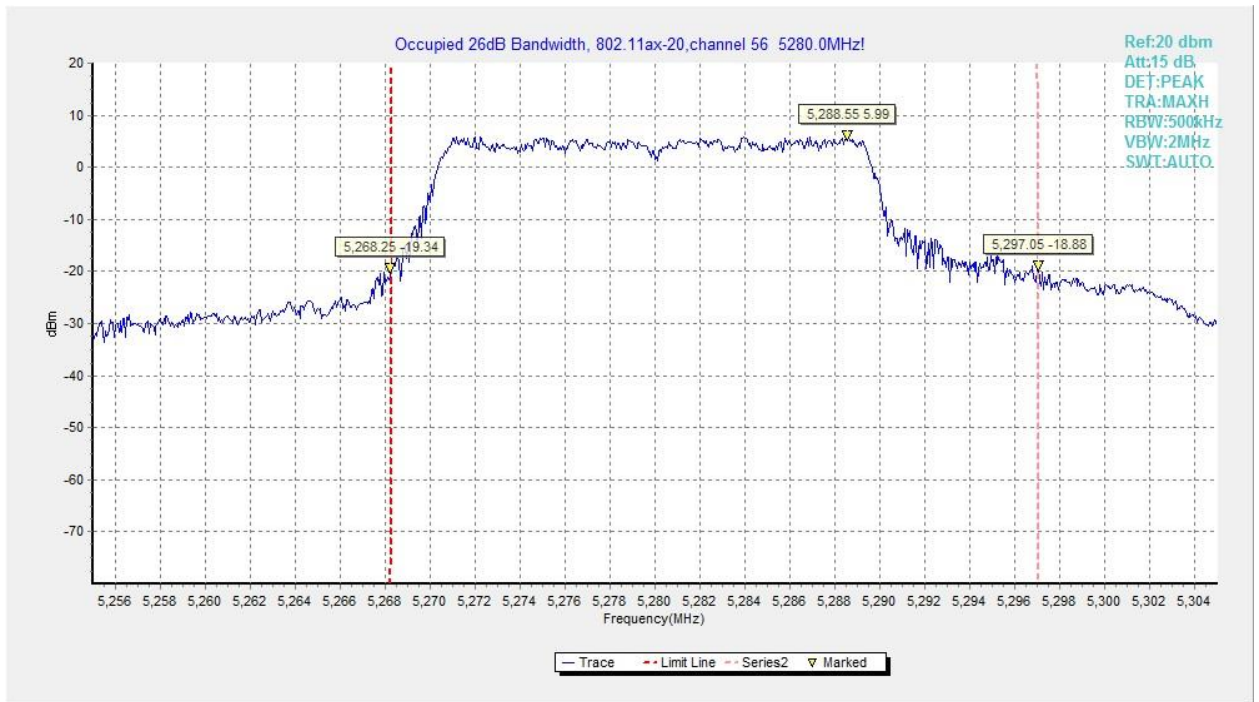
Fig.98 Occupied 26dB Bandwidth (802.11ax-HE20, 5280MHz)
