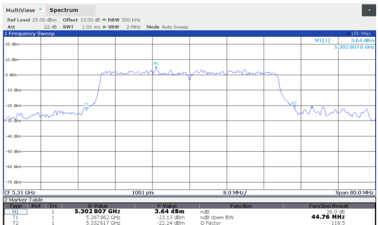
Fig.47 Occupied 26dB Bandwidth (802.11ax-HE40, 5310MHz)
