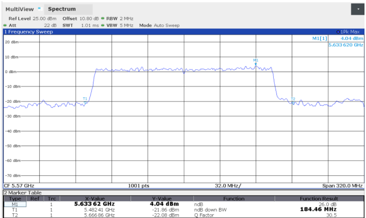
Fig.60 Occupied 26dB Bandwidth (802.11ax-HE160, 5570MHz)
