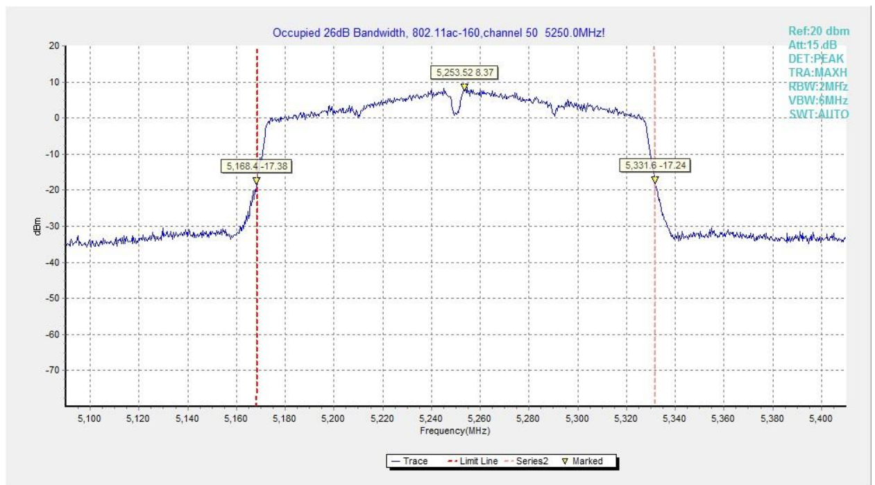
Fig.57 Occupied 26dB Bandwidth (802.11ac-VHT160, 5250MHz)
