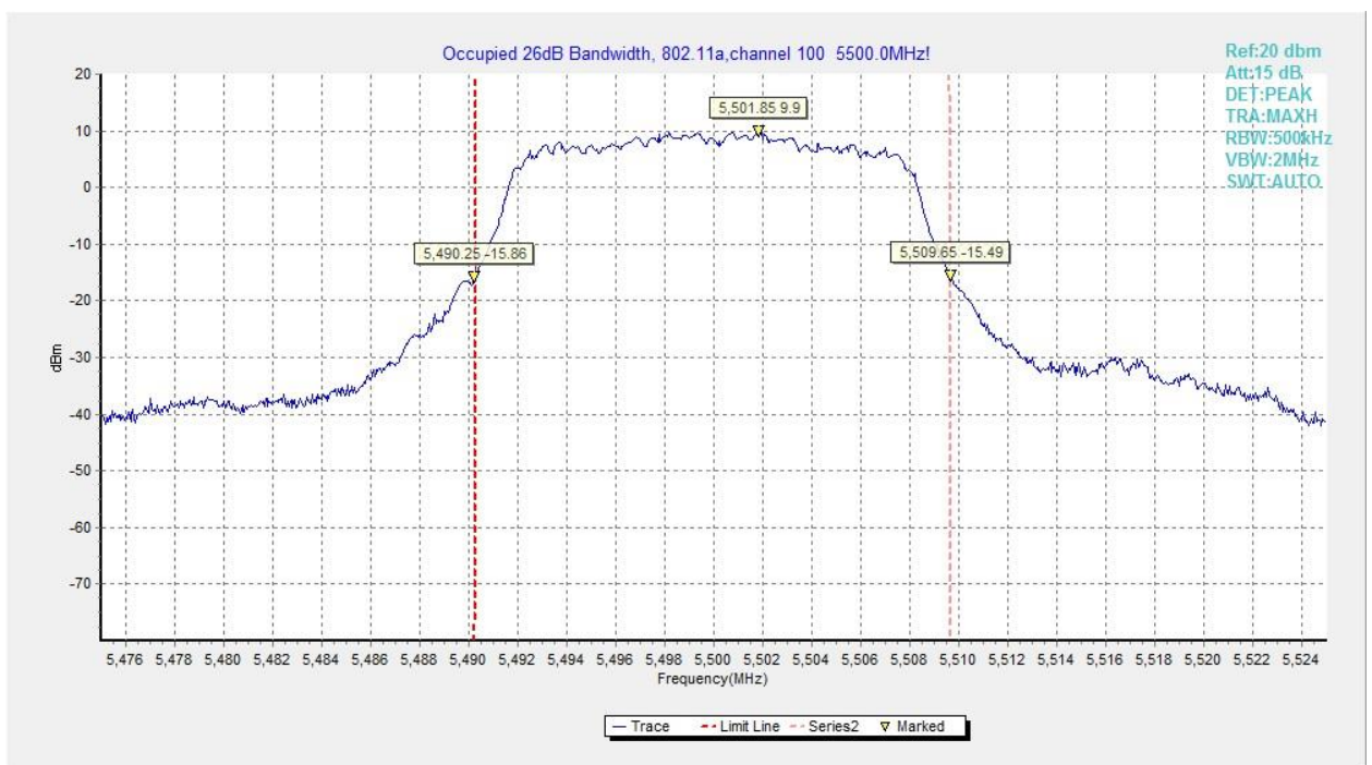
Fig.67 Occupied 26dB Bandwidth (802.11a, 5500MHz)
