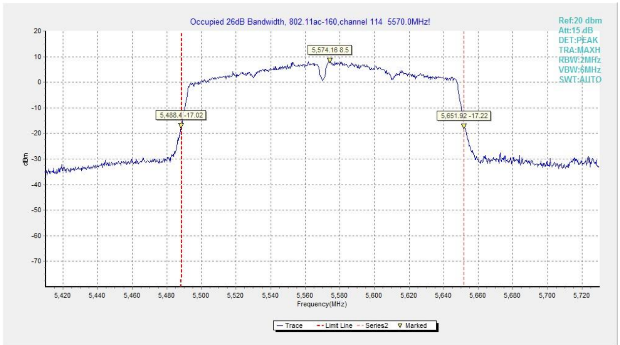
Fig.58 Occupied 26dB Bandwidth (802.11ac-VHT160, 5570MHz)
