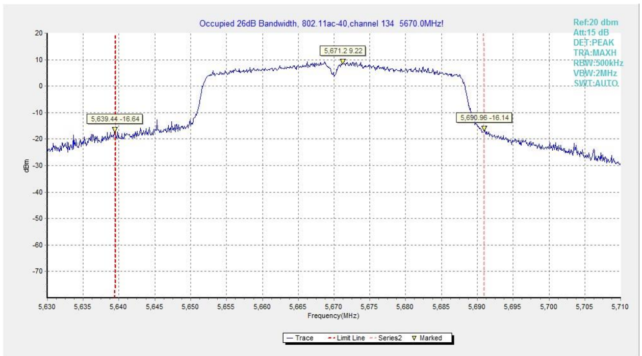
Fig.87 Occupied 26dB Bandwidth 802.11ac-VHT40, 5670MHz)
