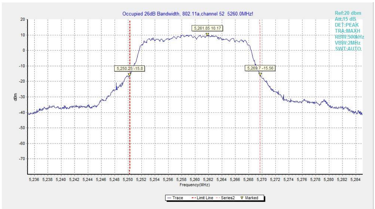
Fig.64 Occupied 26dB Bandwidth (802.11a, 5260MHz)
