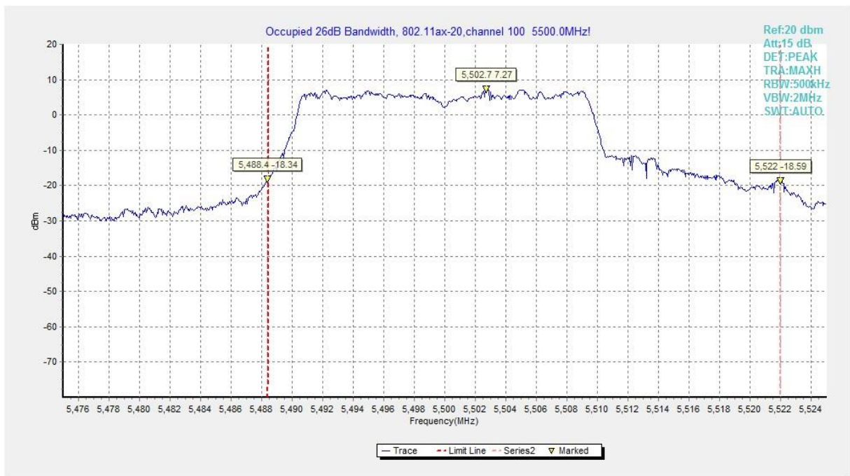
Fig.40 Occupied 26dB Bandwidth (802.11ax-HE20, 5500MHz)
