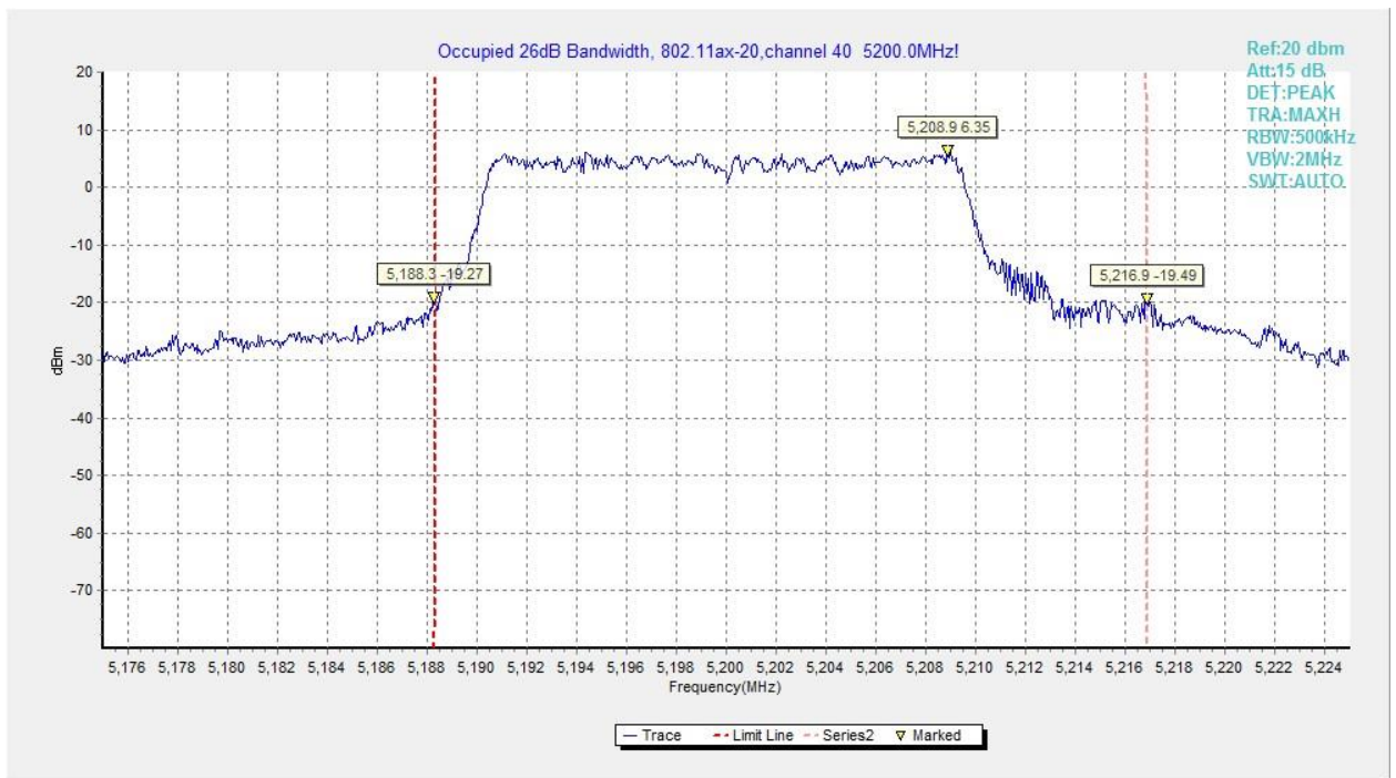
Fig.95 Occupied 26dB Bandwidth (802.11ax-HE20, 5200MHz)
