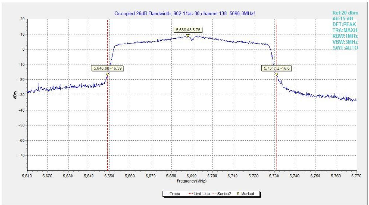
Fig.33 Occupied 26dB Bandwidth (802. 11ac-VHT80, 5690MHz)
