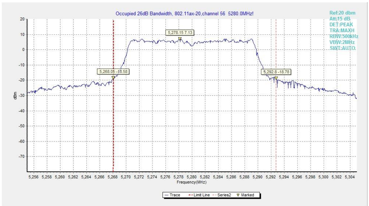
Fig.38 Occupied 26dB Bandwidth (802.11ax-HE20, 5280MHz)
