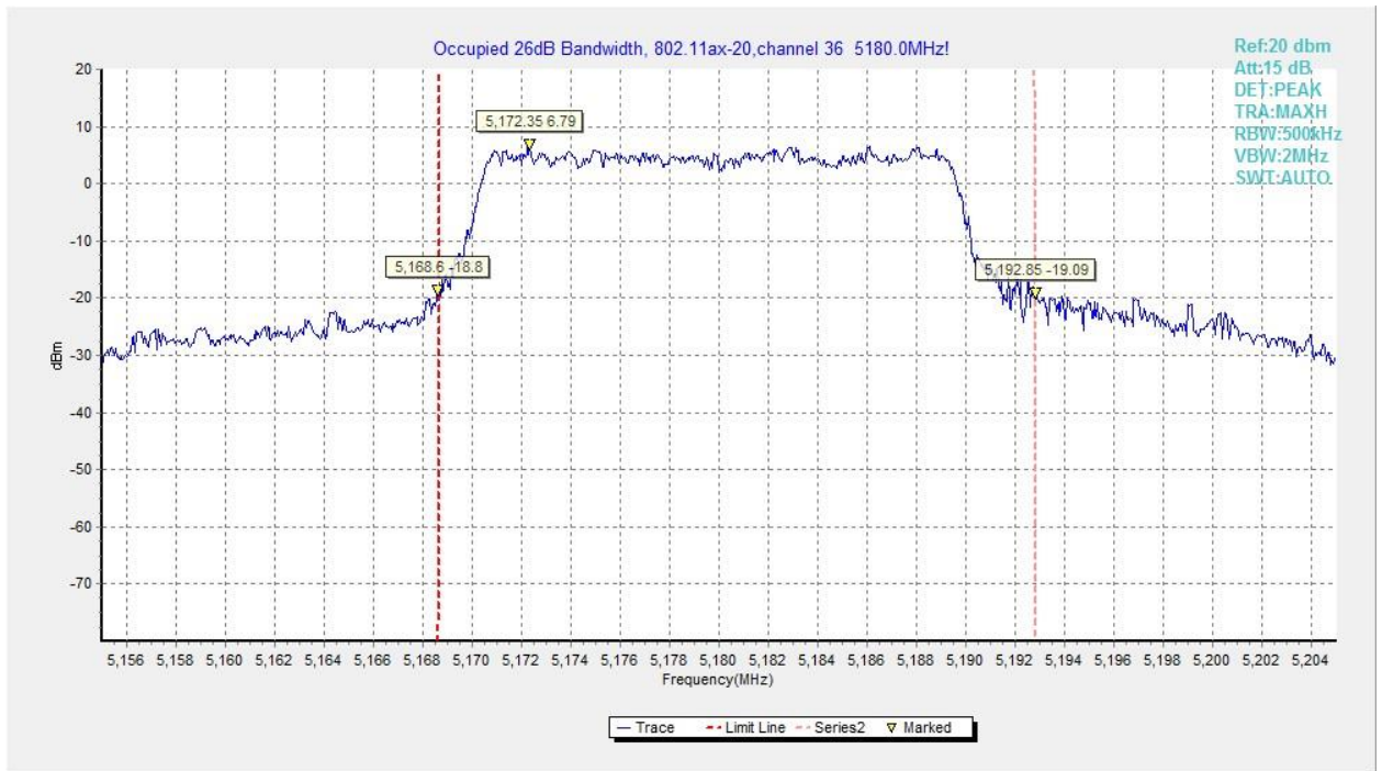
Fig.94 Occupied 26dB Bandwidth (802.11ax-HE20, 5180MHz)
