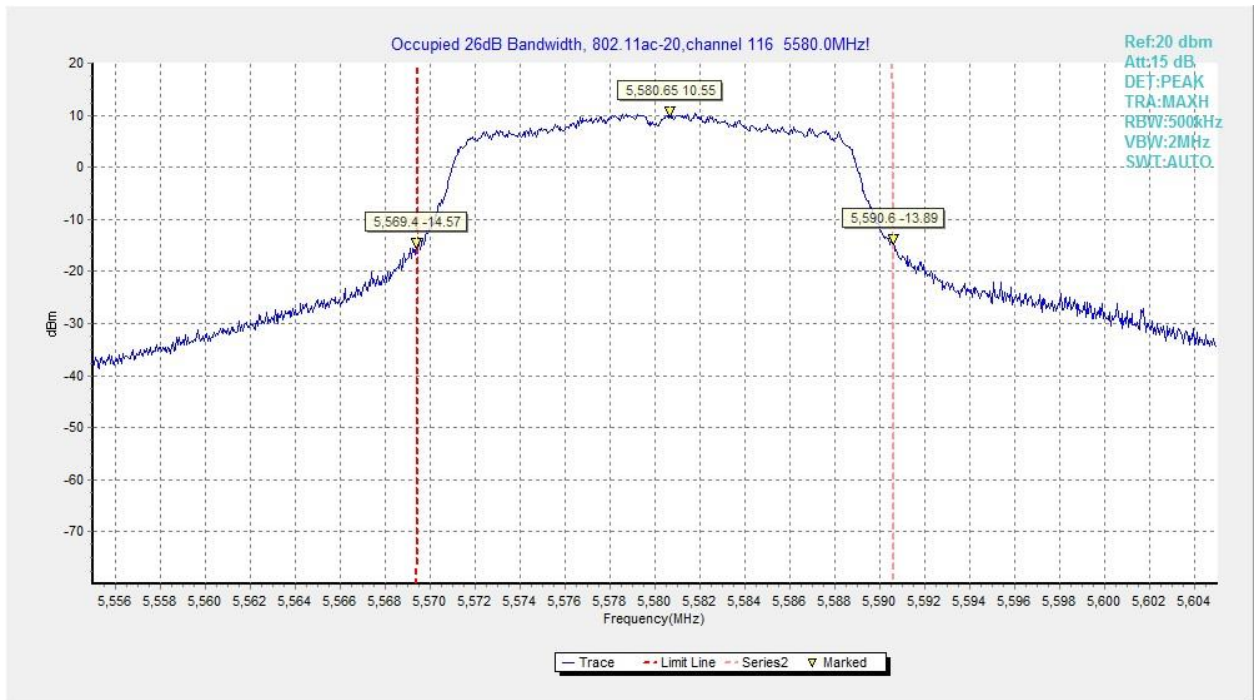
Fig.78 Occupied 26dB Bandwidth (802.11ac-VHT20, 5580MHz)
