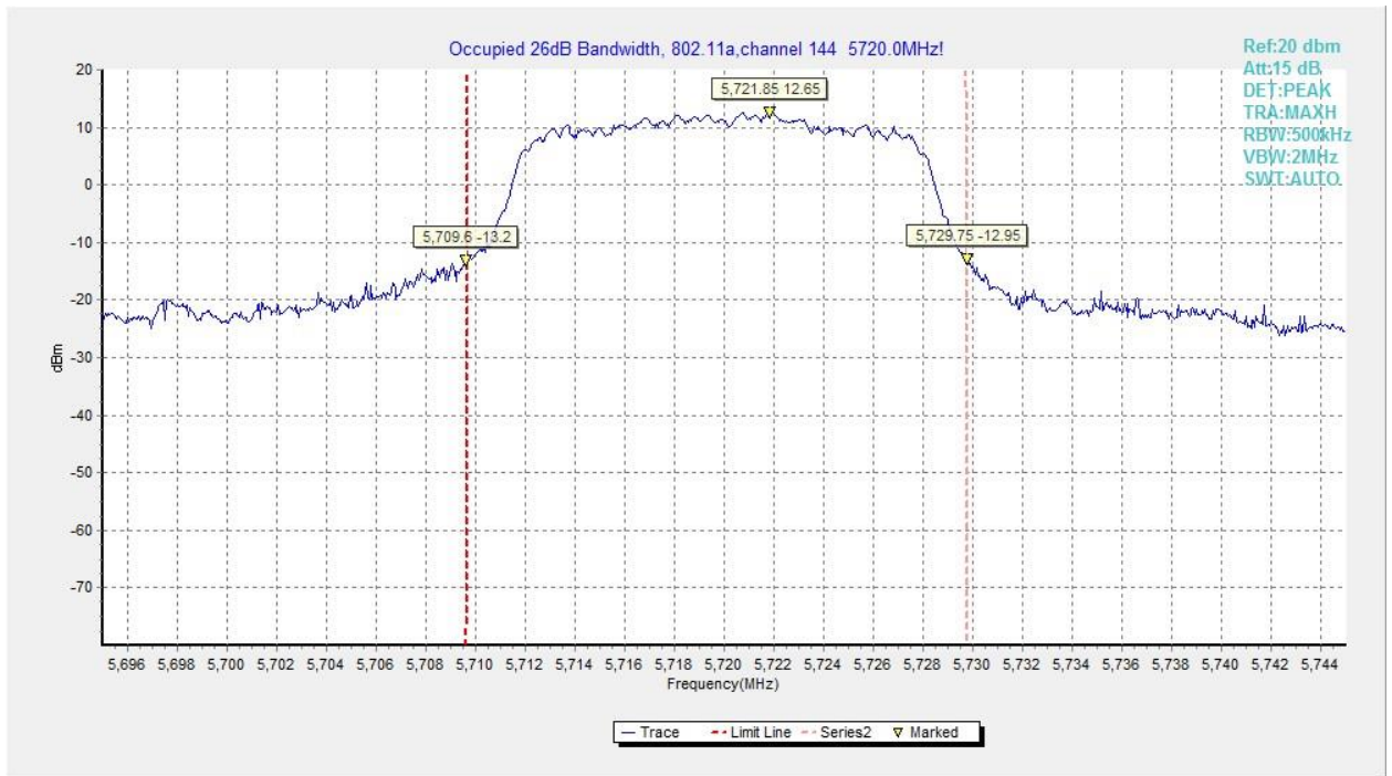
Fig.70 Occupied 26dB Bandwidth (802.11a, 5720MHz)
