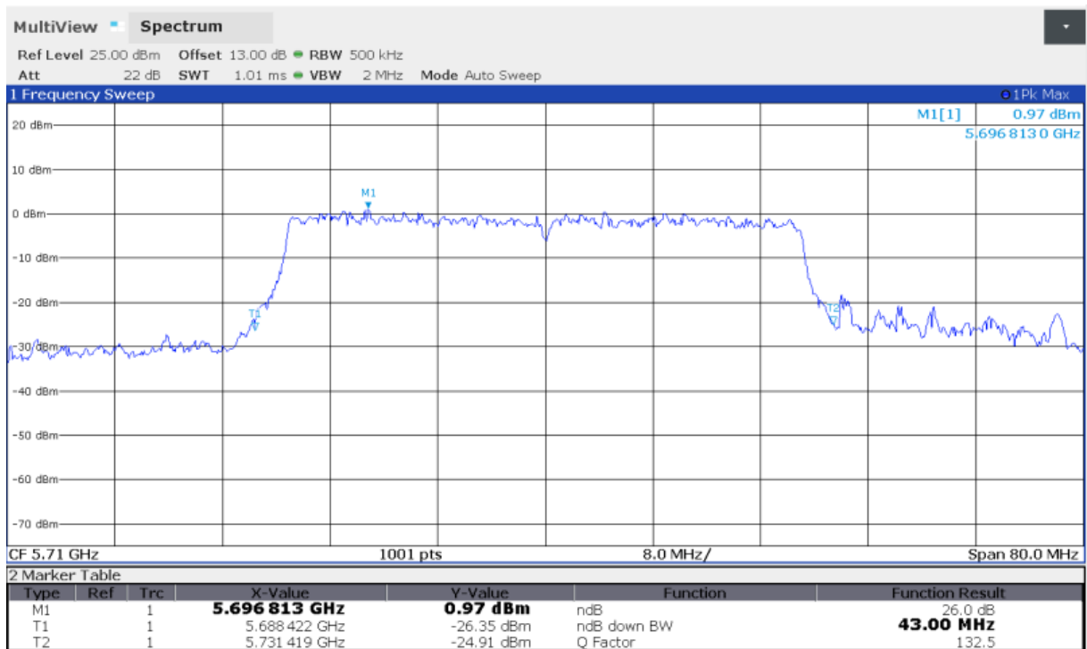
Fig.51 Occupied 26dB Bandwidth (802.11ax-HE40, 5710MHz)
