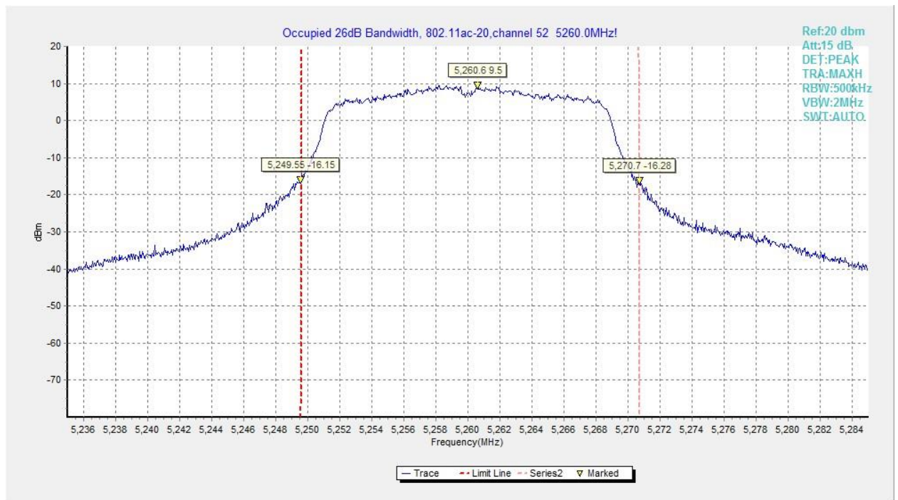
Fig.74 Occupied 26dB Bandwidth (802.11ac-VHT20, 5260MHz)
