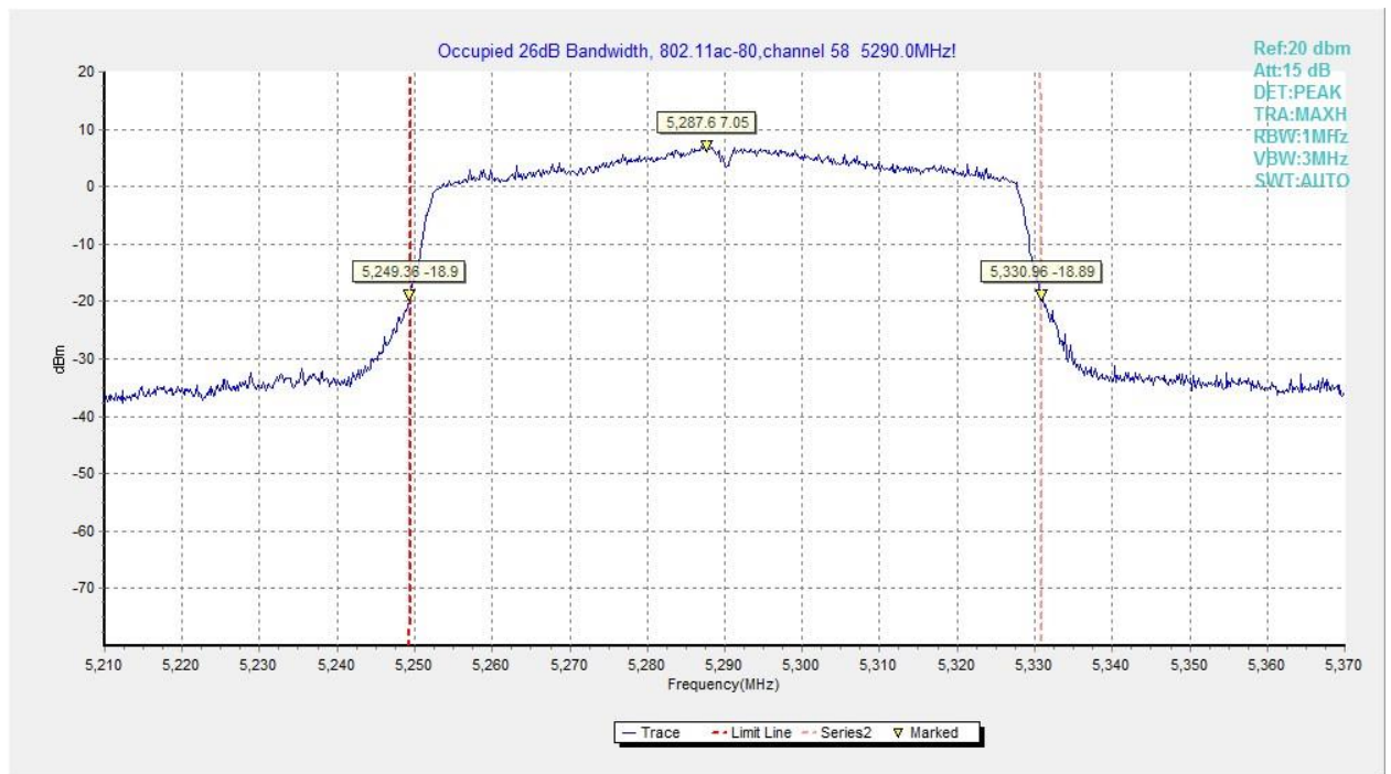
Fig.90 Occupied 26dB Bandwidth (802. 11ac-VHT80, 5290MHz)
