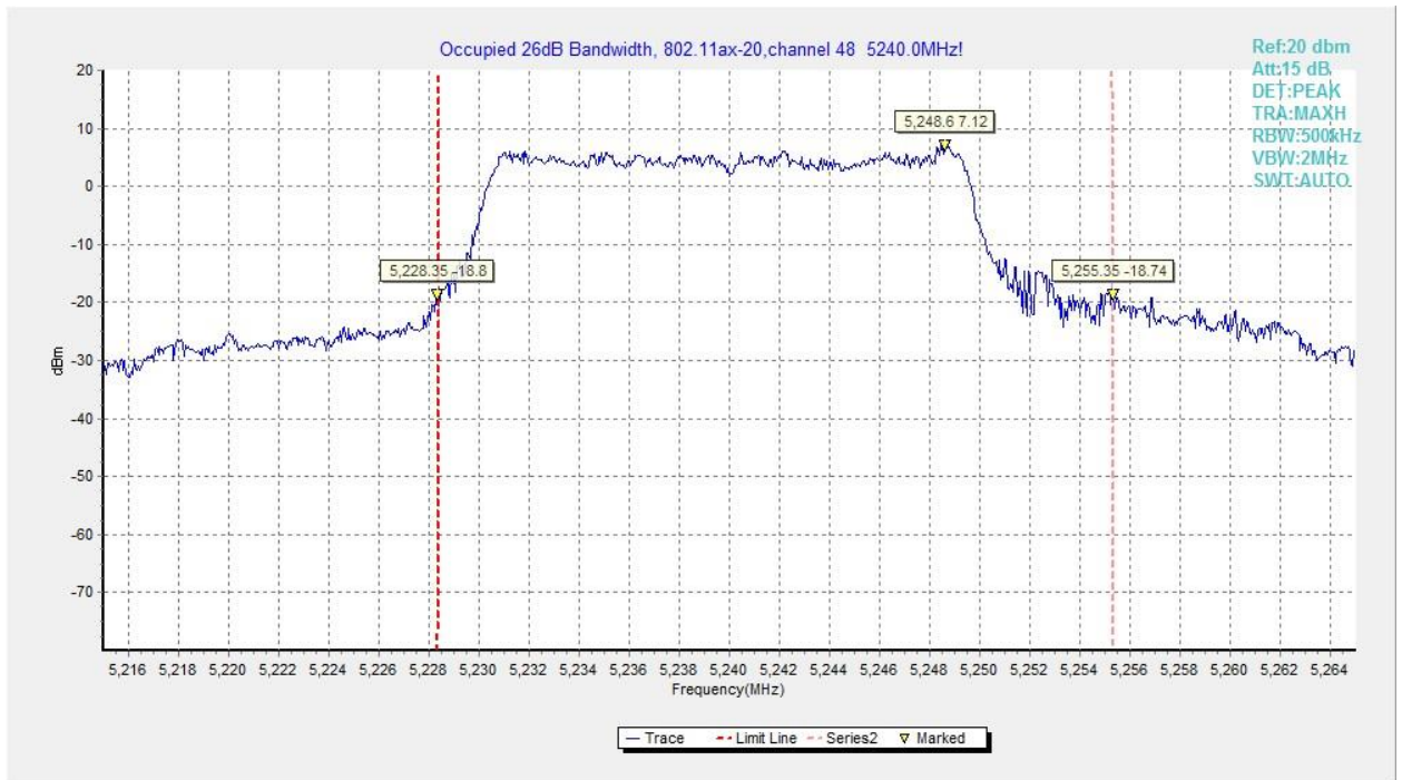
Fig.96 Occupied 26dB Bandwidth (802.11ax-HE20, 5240MHz)
