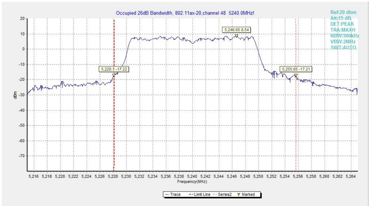
Fig.36 Occupied 26dB Bandwidth (802.11ax-HE20, 5240MHz)
