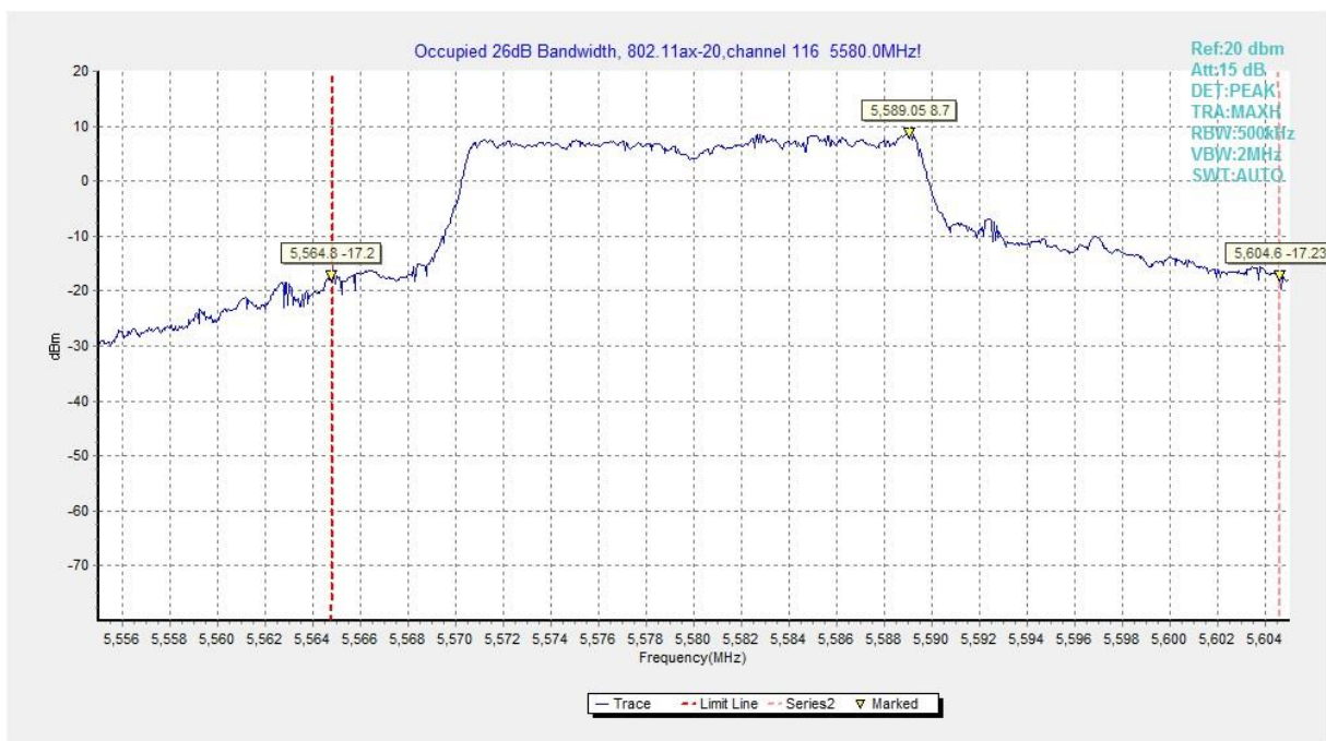
Fig.41 Occupied 26dB Bandwidth (802.11ax-HE20, 5580MHz)
