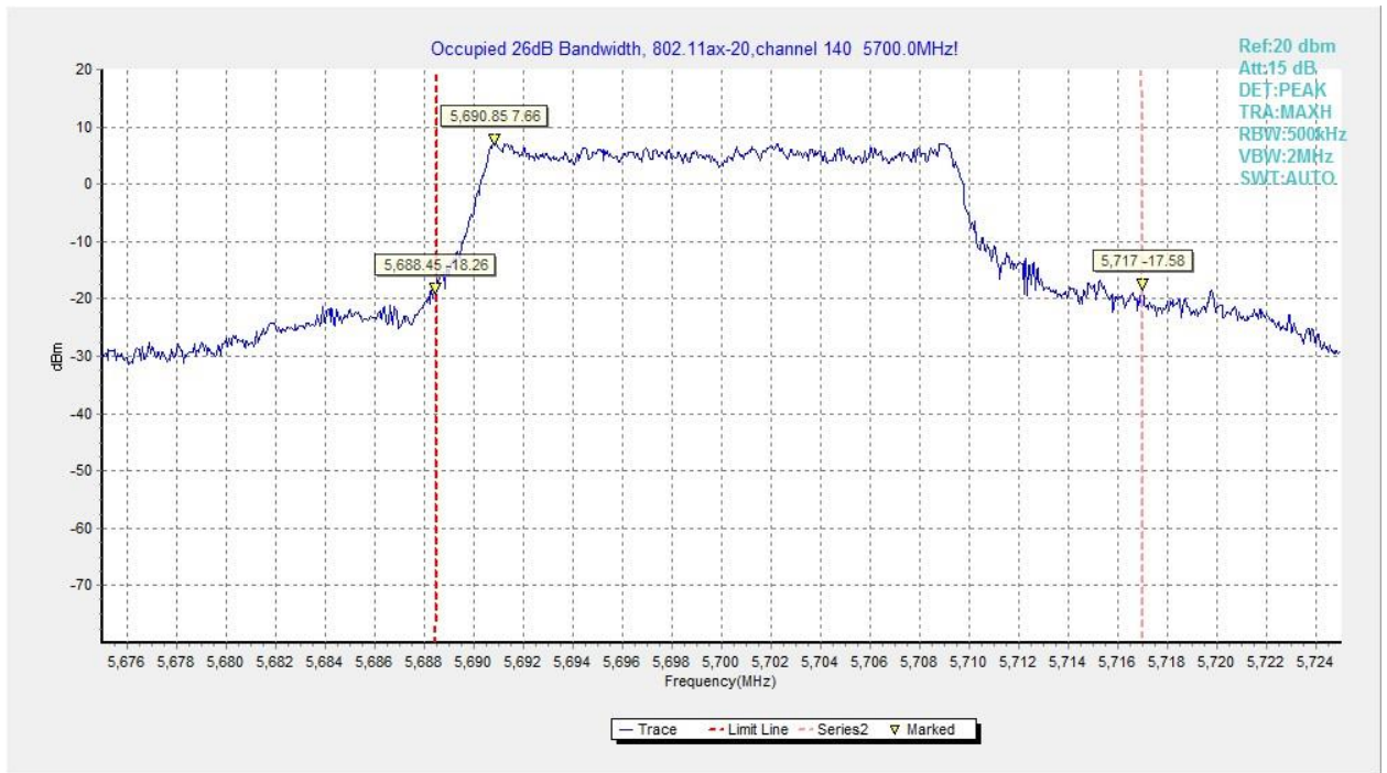
Fig.102 Occupied 26dB Bandwidth (802.11ax-HE20, 5700MHz)
