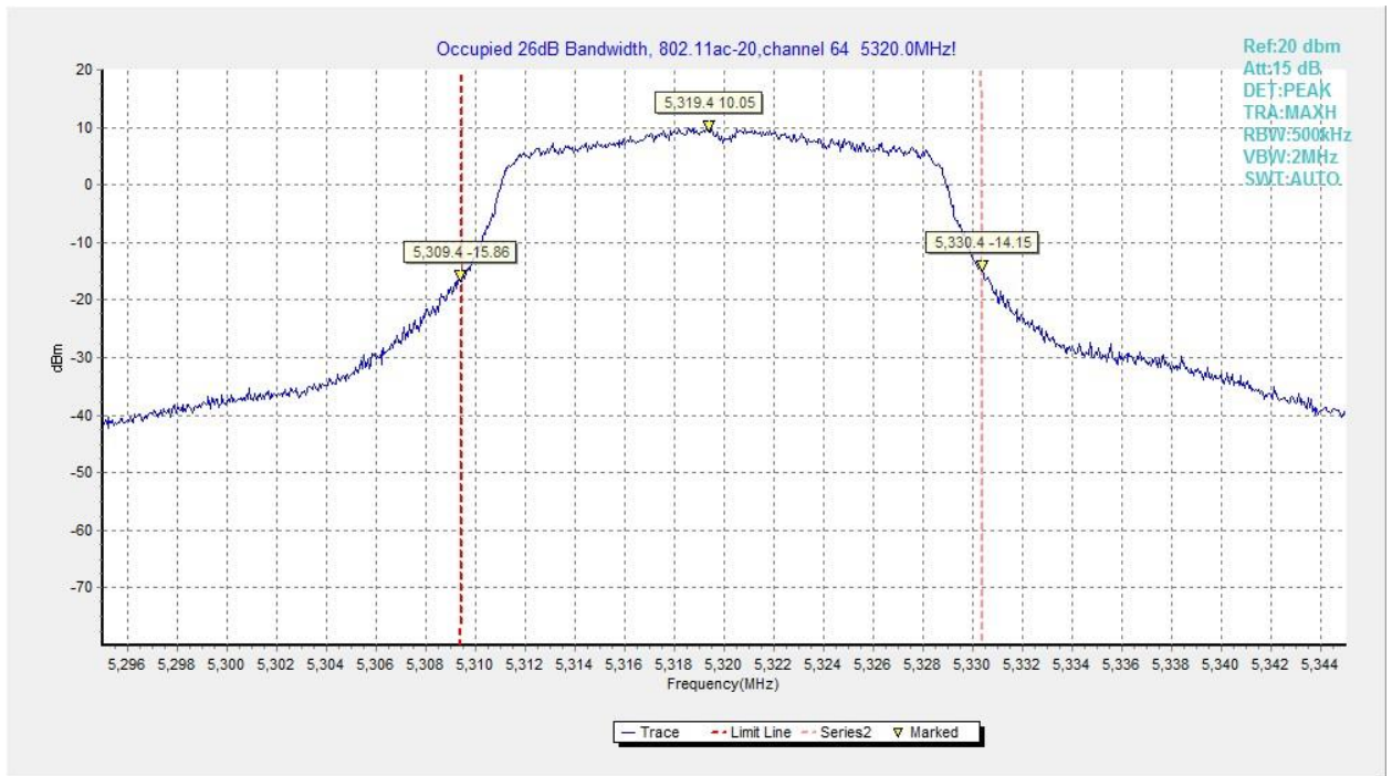
Fig.76 Occupied 26dB Bandwidth (802.11ac-VHT20, 5320MHz)
