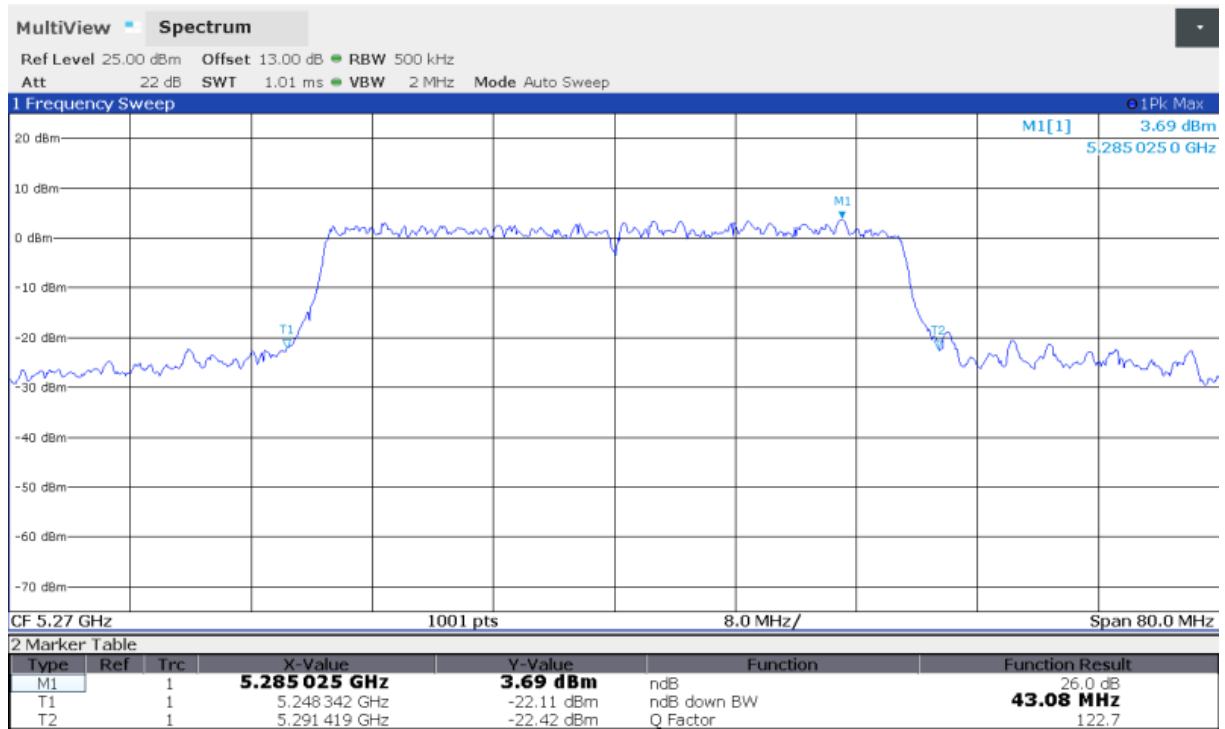
Fig.46 Occupied 26dB Bandwidth (802.11ax-HE40, 5270MHz)
