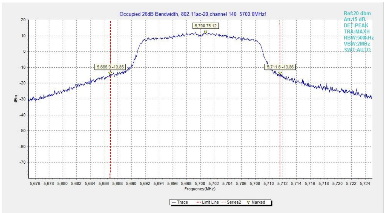
Fig.79 Occupied 26dB Bandwidth (802.11ac-VHT20, 5700MHz)
