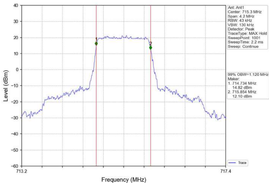
Band12_1.4MHz_QPSK_HCH_715.3MHz_RB_6_0_NTNV
