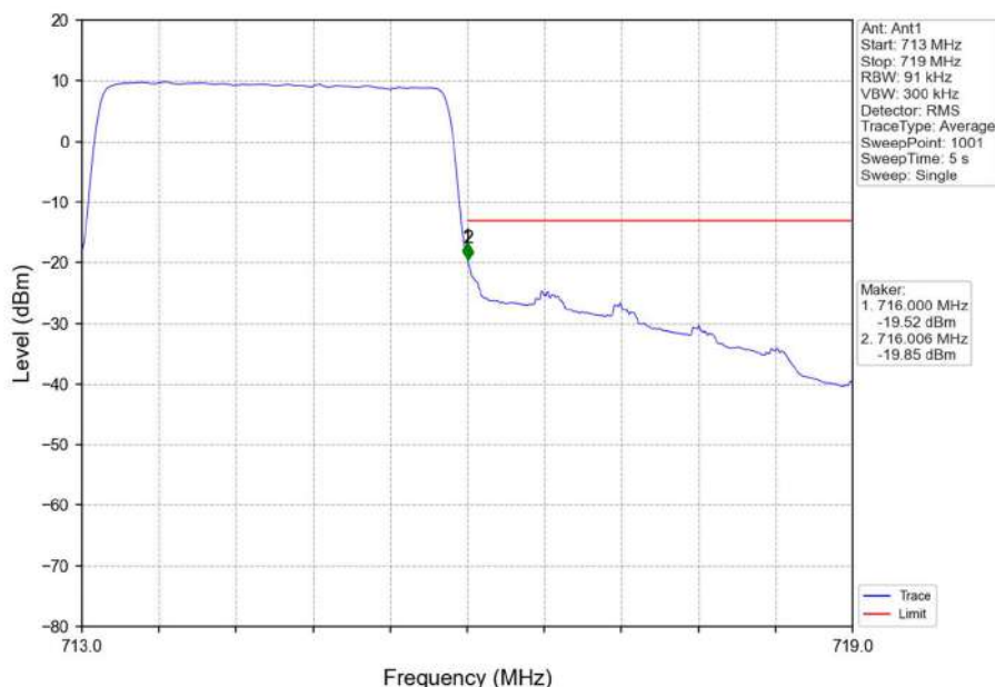
Band12_3MHz_16QAM_HCH_714.5MHz_RB_15_0_NTNV
