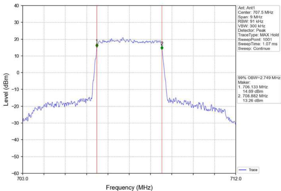
Band12_3MHz_QPSK_MCH_707.5MHz_RB_15_0_NTNV
