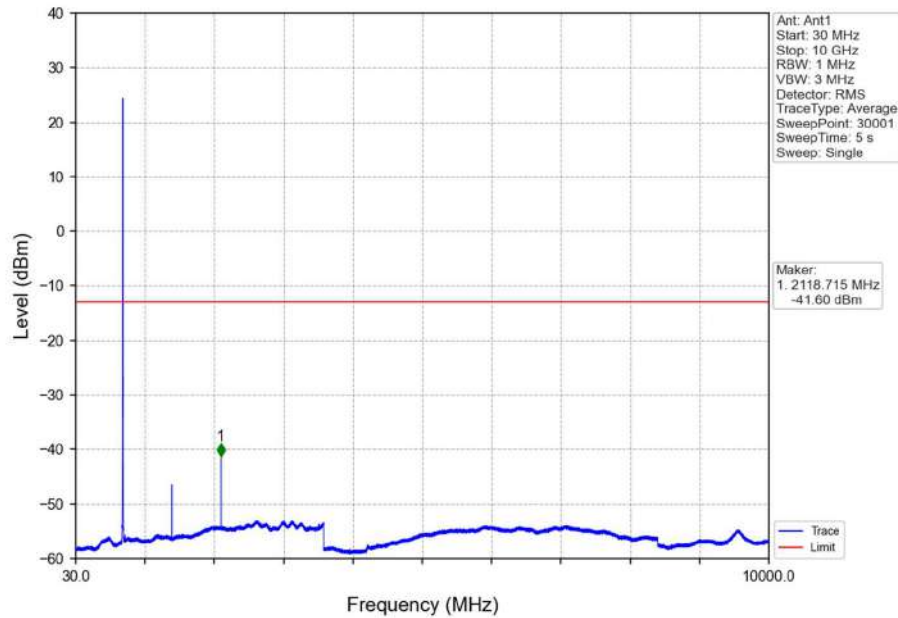
Band12_3MHz_16QAM_MCH_707.5MHz_RB_1_0_NTNV
