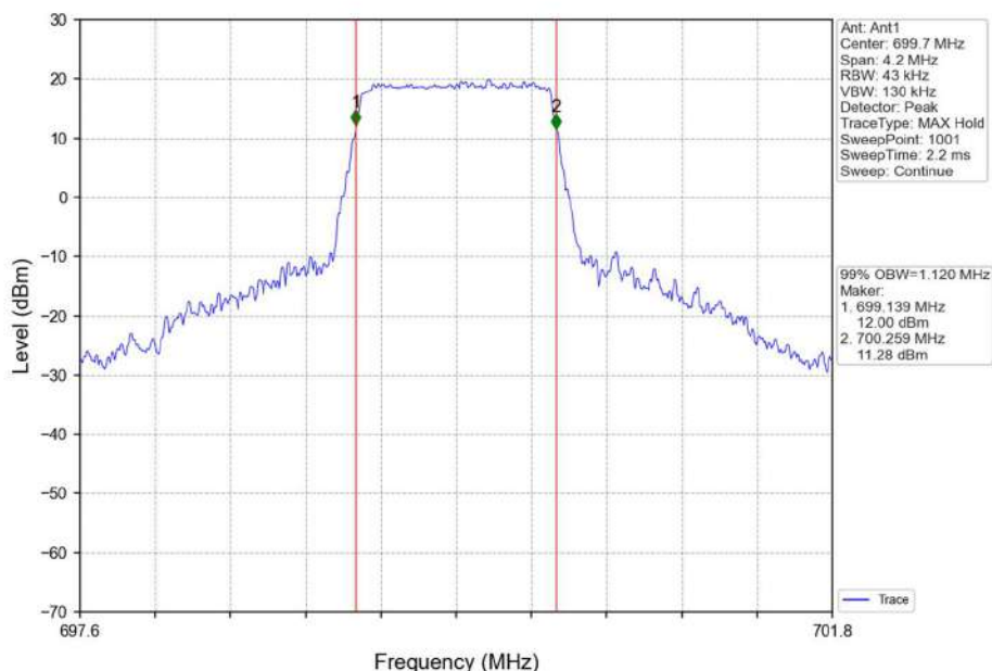
Band12_1.4MHz_16QAM_LCH_699.7MHz_RB_6_0_NTNV
