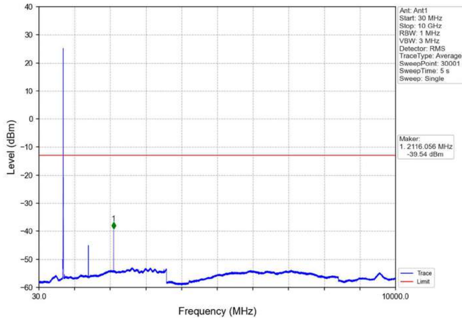
Band12_5MHz_QPSK_MCH_707.5MHz_RB_1_0_NTNV
