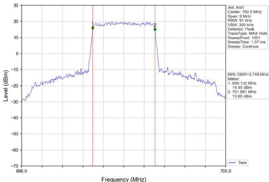
Band12_3MHz_QPSK_LCH_700.5MHz_RB_15_0_NTNV
