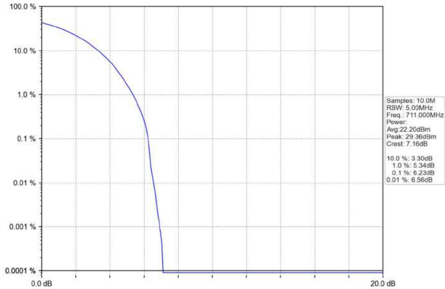
Band12_10MHz_QPSK_HCH_711MHz_RB_50_0_NTNV
