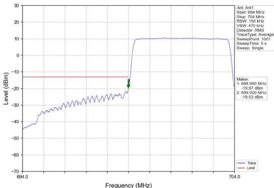
Band12_5MHz_QPSK_LCH_701.5MHz_RB_25_0_NTNV
