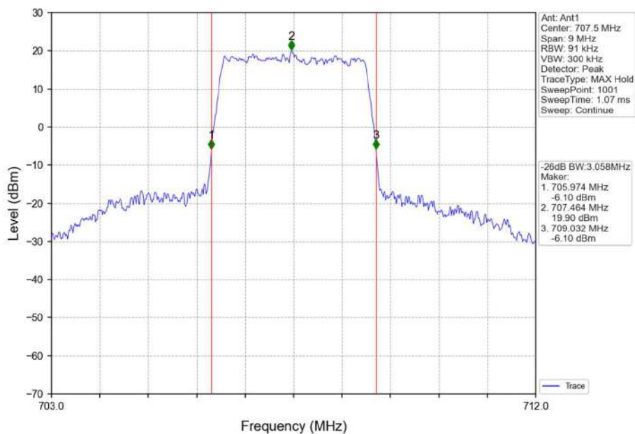
Band12_3MHz_16QAM_MCH_707.5MHz_RB_15_0_NTNV
