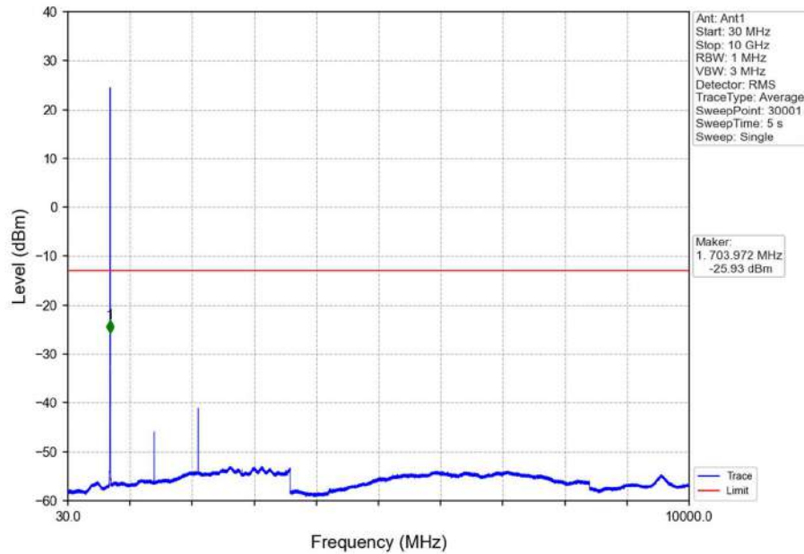
Band12_1.4MHz_16QAM_MCH_707.5MHz_RB_1_0_NTNV
