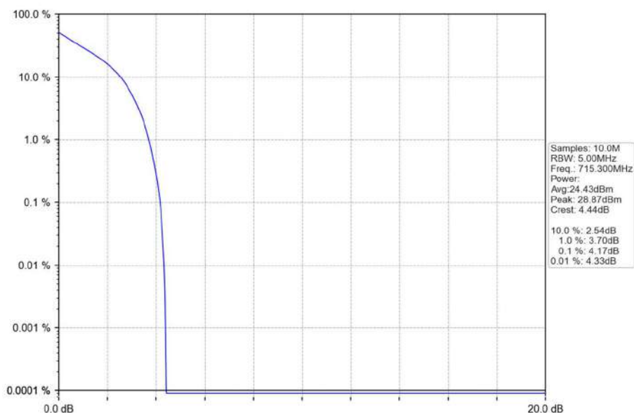
Band12_1.4MHz_QPSK_HCH_715.3MHz_RB_6_0_NTNV
