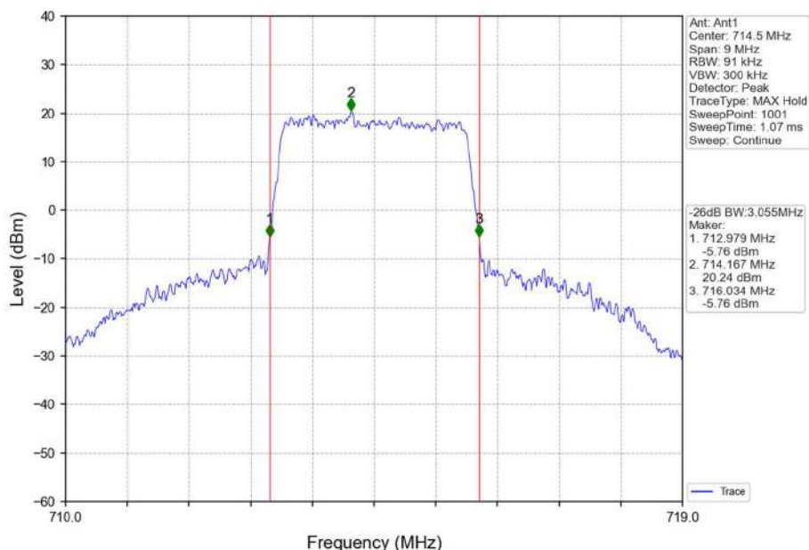
Band12_3MHz_16QAM_HCH_714.5MHz_RB_15_0_NTNV
