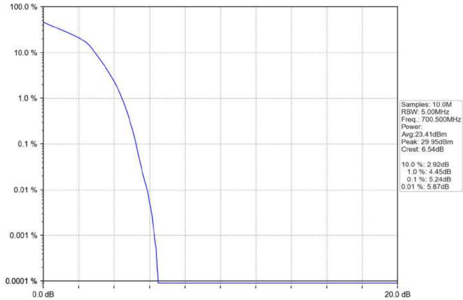
Band12_3MHz_16QAM_LCH_700.5MHz_RB_15_0_NTNV
