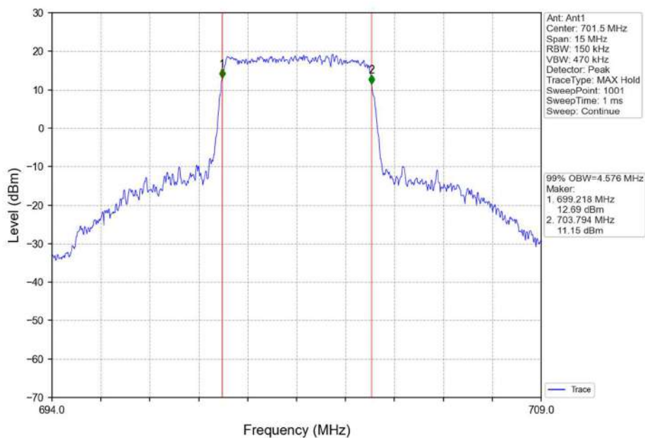
Band12_5MHz_16QAM_LCH_701.5MHz_RB_25_0_NTNV
