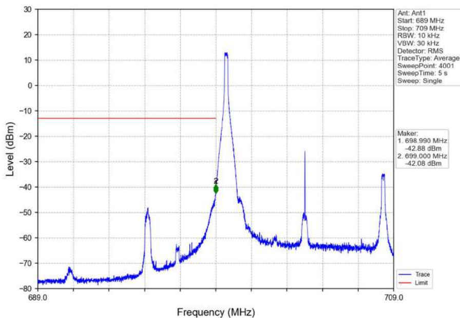
Band12_10MHz_16QAM_LCH_704MHz_RB_1_0_NTNV
