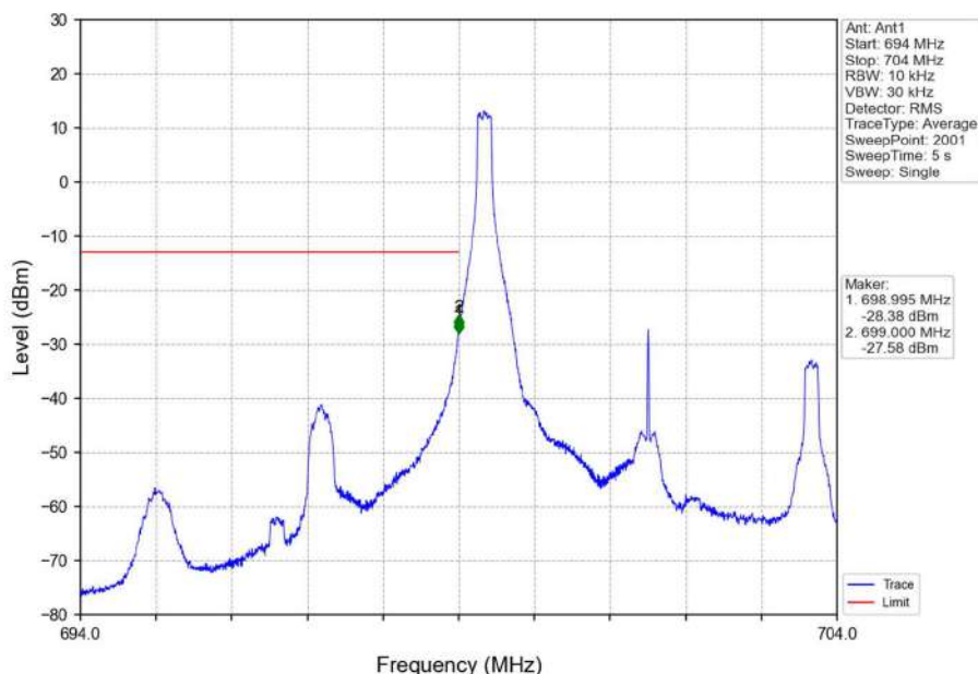
Band12_5MHz_16QAM_LCH_701.5MHz_RB_1_0_NTNV
