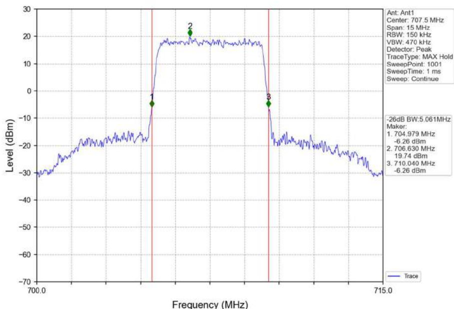
Band12_5MHz_16QAM_MCH_707.5MHz_RB_25_0_NTNV
