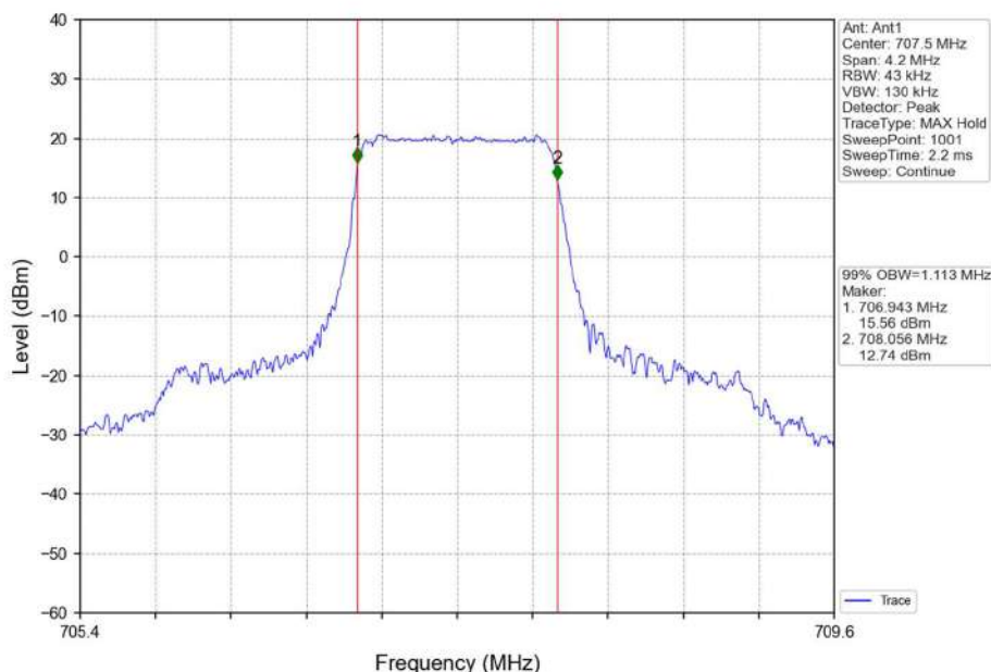
Band12_1.4MHz_QPSK_MCH_707.5MHz_RB_6_0_NTNV
