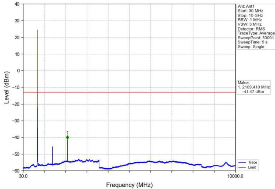
Band12_10MHz_16QAM_MCH_707.5MHz_RB_1_0_NTNV
