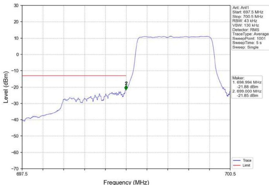
Band12_1.4MHz_QPSK_LCH_699.7MHz_RB_6_0_NTNV
