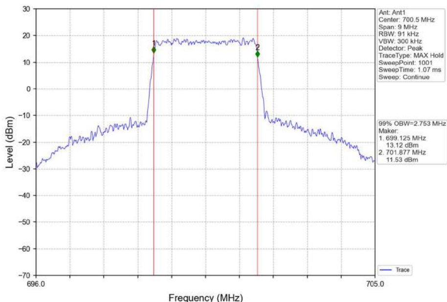
Band12_3MHz_16QAM_LCH_700.5MHz_RB_15_0_NTNV
