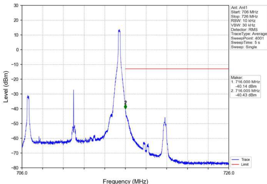
Band12_10MHz_QPSK_HCH_711MHz_RB_1_49_NTNV
