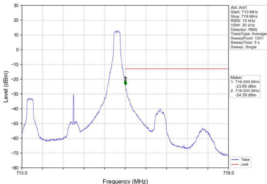
Band12_3MHz_16QAM_HCH_714.5MHz_RB_1_14_NTNV
