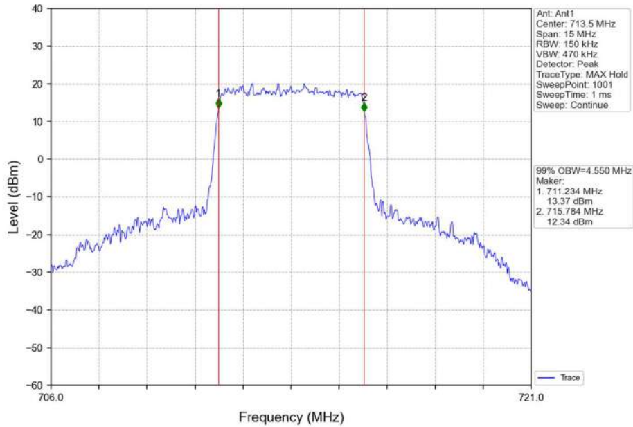
Band12_5MHz_16QAM_HCH_713.5MHz_RB_25_0_NTNV
