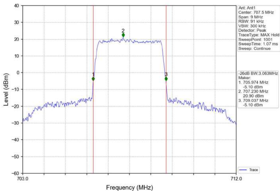
Band12_3MHz_QPSK_MCH_707.5MHz_RB_15_0_NTNV
