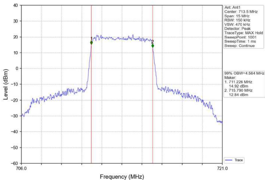
Band12_5MHz_QPSK_HCH_713.5MHz_RB_25_0_NTNV
