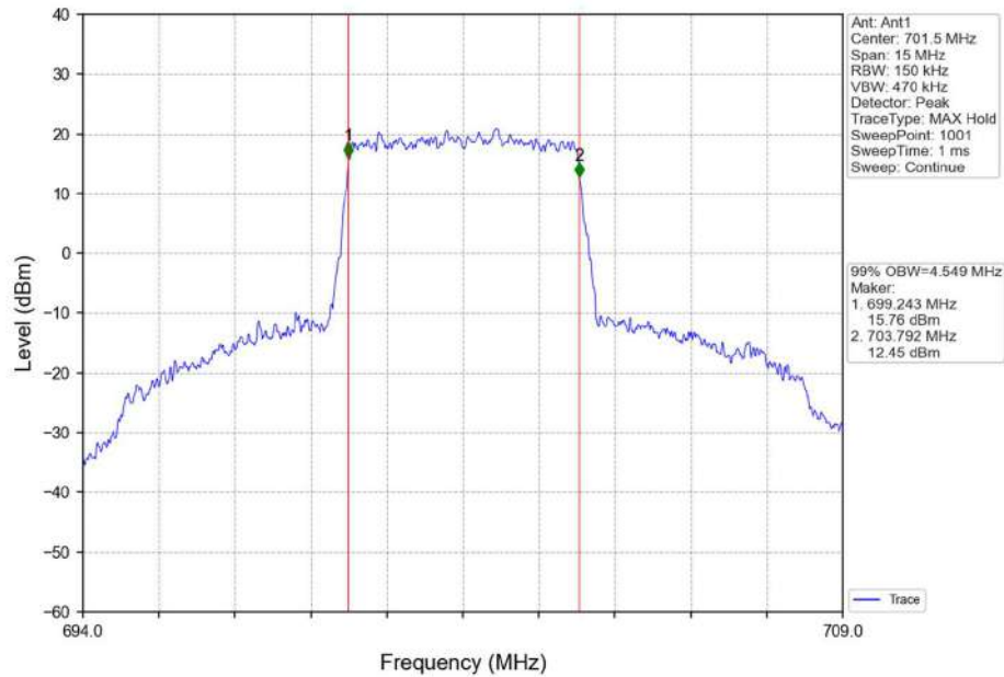
Band12_5MHz_QPSK_LCH_701.5MHz_RB_25_0_NTNV
