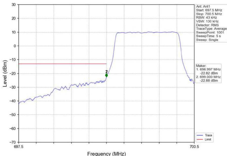
Band12_1.4MHz_16QAM_LCH_699.7MHz_RB_6_0_NTNV
