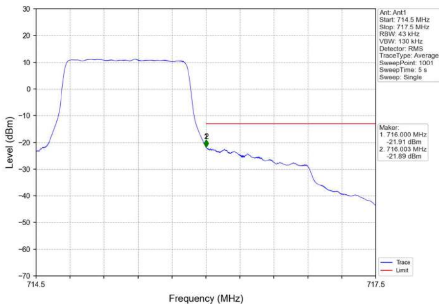
Band12_1.4MHz_QPSK_HCH_715.3MHz_RB_6_0_NTNV
