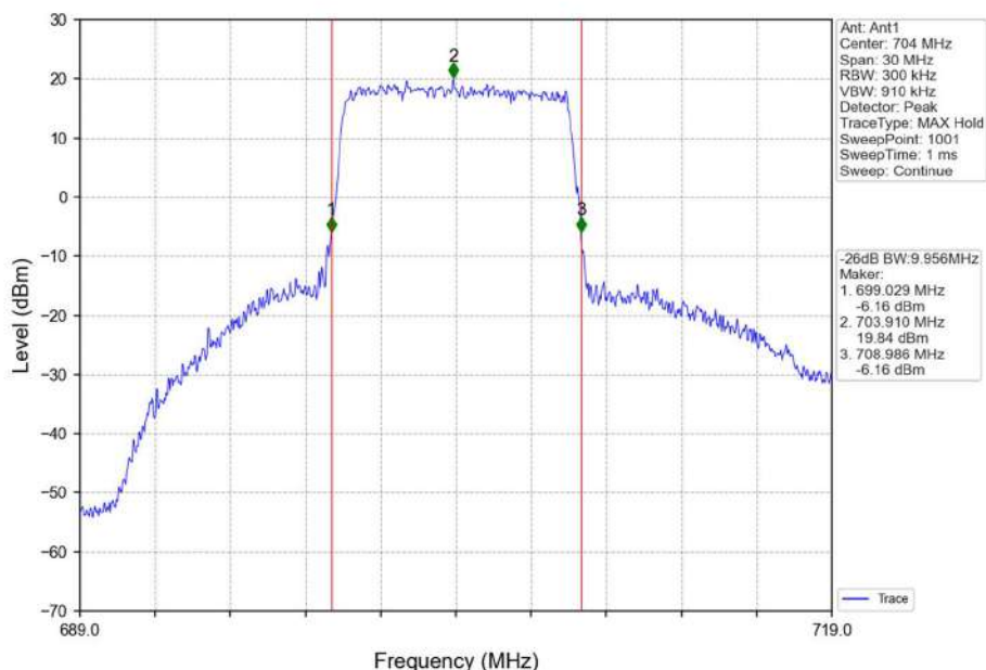
Band12_10MHz_16QAM_LCH_704MHz_RB_50_0_NTNV
