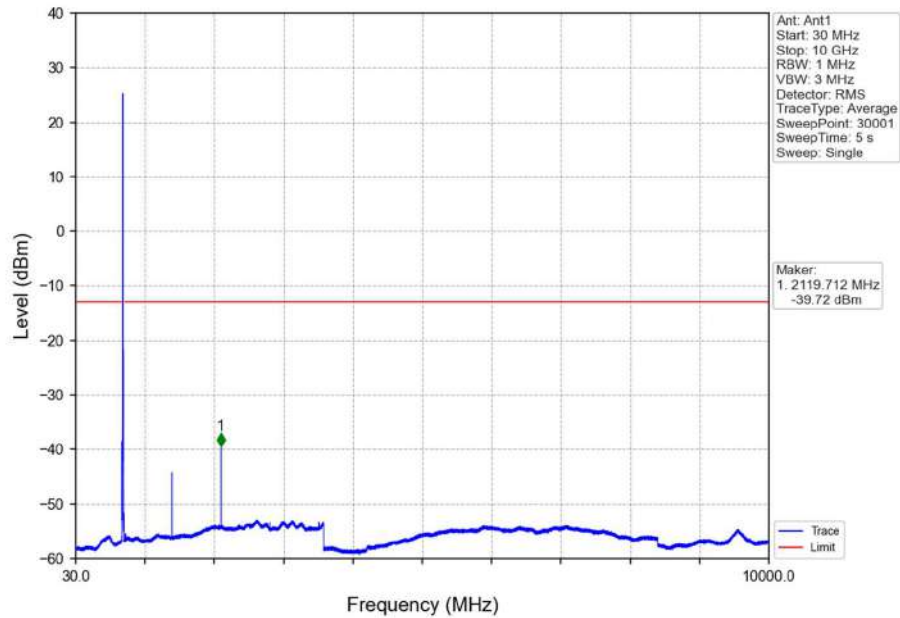
Band12_10MHz_QPSK_HCH_711MHz_RB_1_0_NTNV
