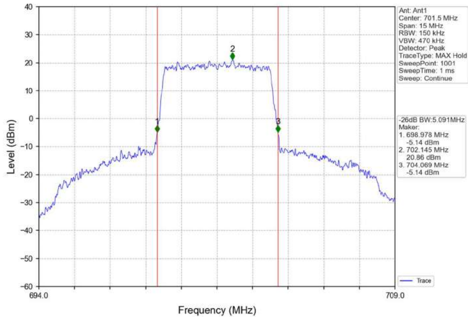
Band12_5MHz_QPSK_LCH_701.5MHz_RB_25_0_NTNV
