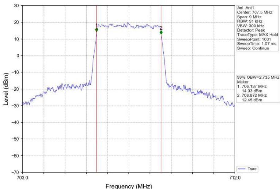
Band12_3MHz_16QAM_MCH_707.5MHz_RB_15_0_NTNV
