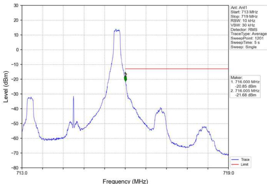
Band12_3MHz_QPSK_HCH_714.5MHz_RB_1_14_NTNV
