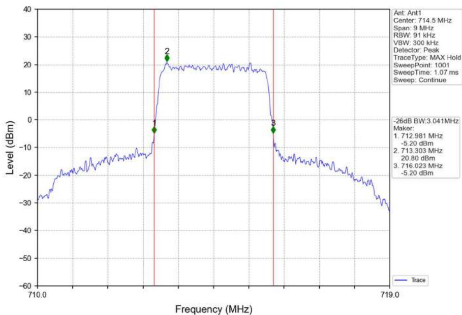
Band12_3MHz_QPSK_HCH_714.5MHz_RB_15_0_NTNV
