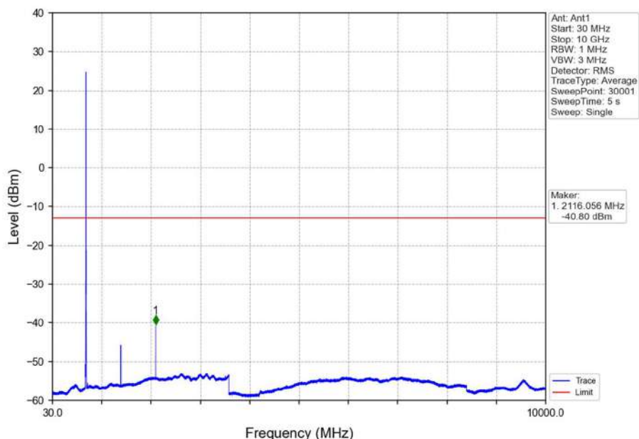
Band12_5MHz_16QAM_MCH_707.5MHz_RB_1_0_NTNV
