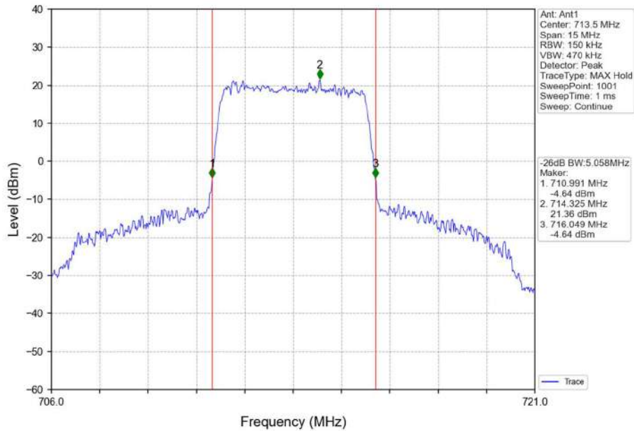
Band12_5MHz_QPSK_HCH_713.5MHz_RB_25_0_NTNV
