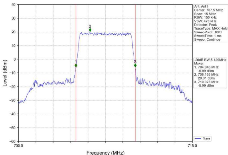
Band12_5MHz_QPSK_MCH_707.5MHz_RB_25_0_NTNV
