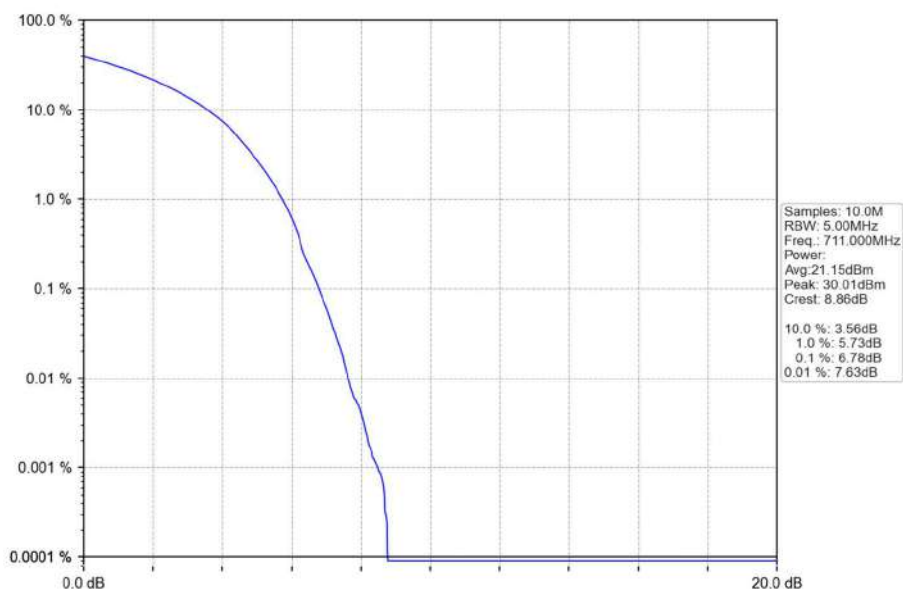
Band12_10MHz_16QAM_HCH_711MHz_RB_50_0_NTNV
