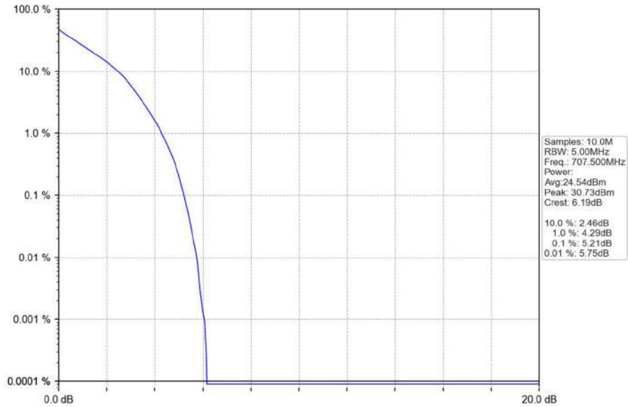
Band12_3MHz_QPSK_MCH_707.5MHz_RB_15_0_NTNV
