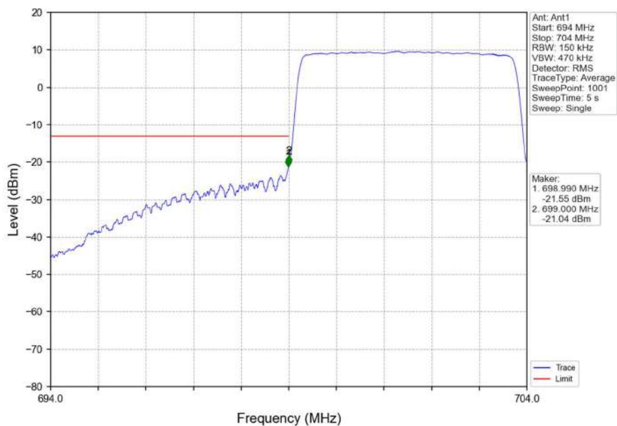
Band12_5MHz_16QAM_LCH_701.5MHz_RB_25_0_NTNV
