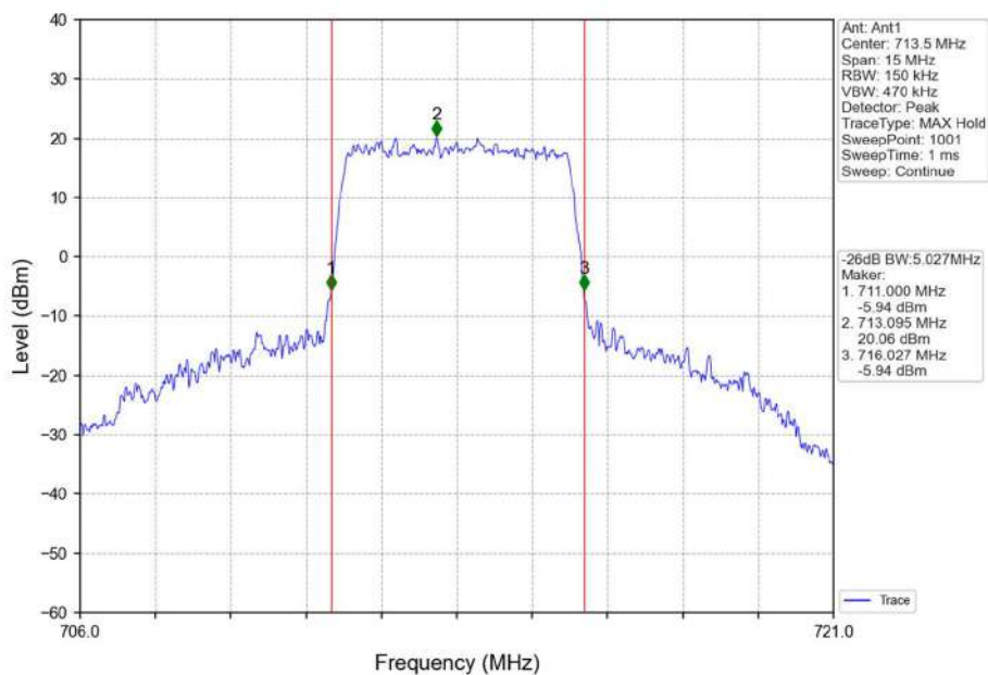
Band12_5MHz_16QAM_HCH_713.5MHz_RB_25_0_NTNV
