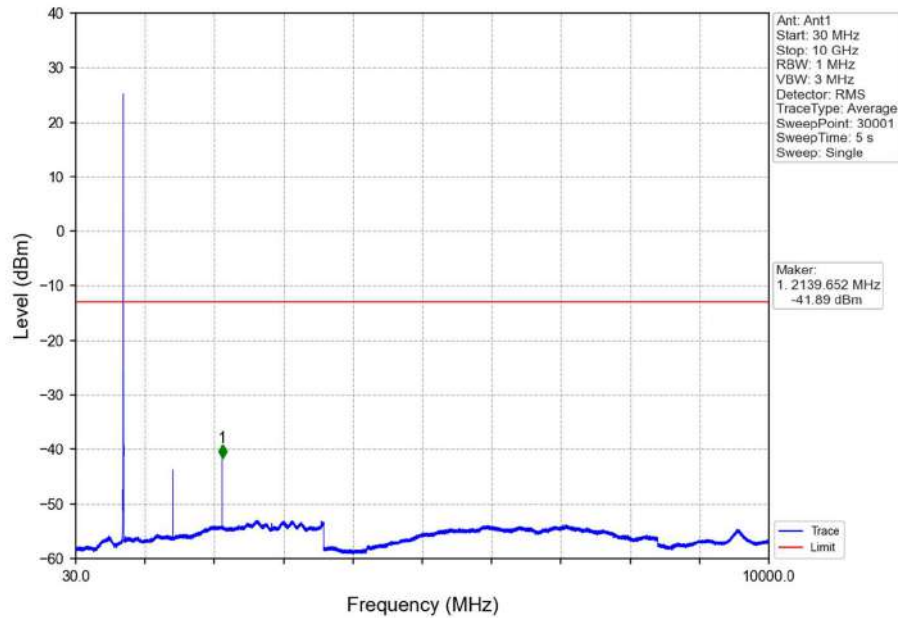
Band12_3MHz_16QAM_HCH_714.5MHz_RB_1_0_NTNV
