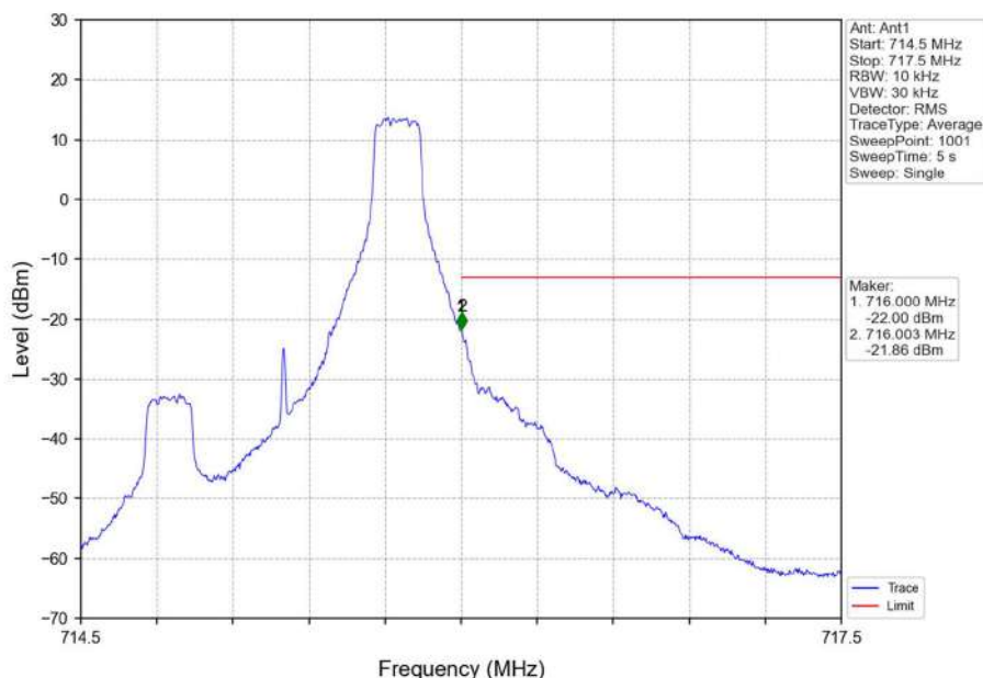
Band12_1.4MHz_QPSK_HCH_715.3MHz_RB_1_5_NTNV
