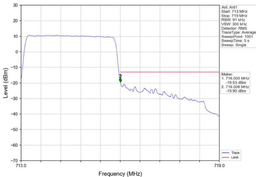
Band12_3MHz_QPSK_HCH_714.5MHz_RB_15_0_NTNV
