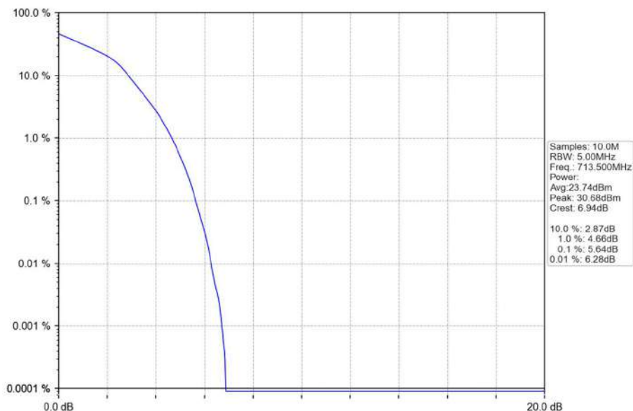
Band12_5MHz_16QAM_HCH_713.5MHz_RB_25_0_NTNV
