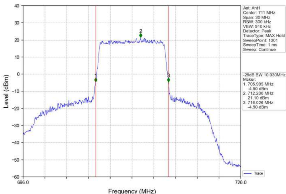
Band12_10MHz_QPSK_HCH_711MHz_RB_50_0_NTNV
