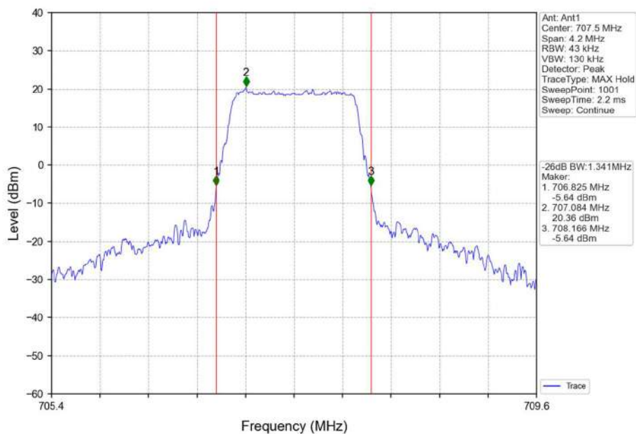
Band12_1.4MHz_16QAM_MCH_707.5MHz_RB_6_0_NTNV
