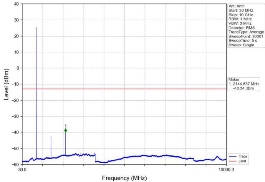
Band12_1.4MHz_QPSK_HCH_715.3MHz_RB_1_0_NTNV
