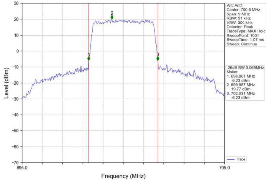
Band12_3MHz_QPSK_LCH_700.5MHz_RB_15_0_NTNV
