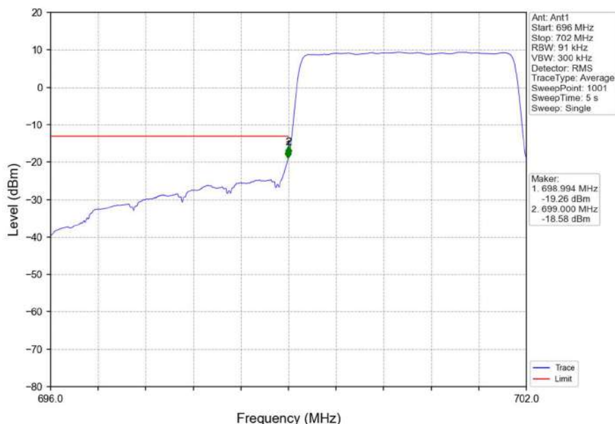
Band12_3MHz_16QAM_LCH_700.5MHz_RB_15_0_NTNV
