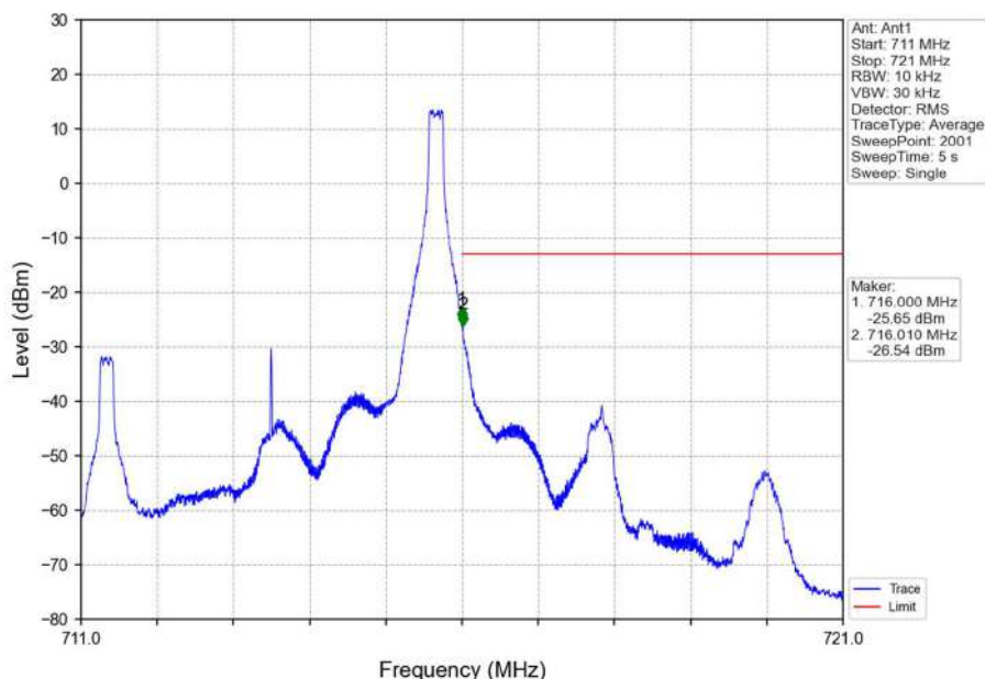
Band12_5MHz_QPSK_HCH_713.5MHz_RB_1_24_NTNV
