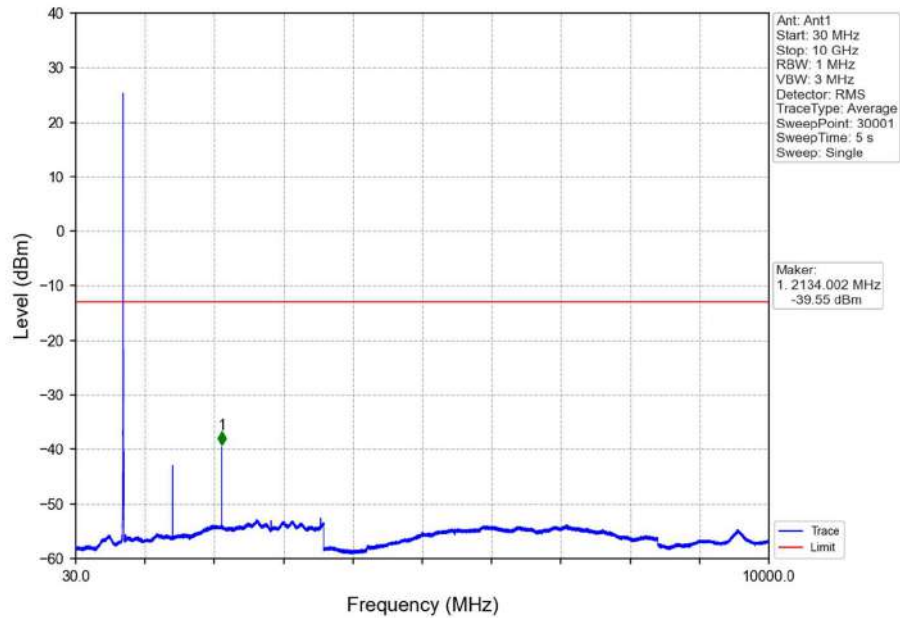
Band12_5MHz_QPSK_HCH_713.5MHz_RB_1_0_NTNV
