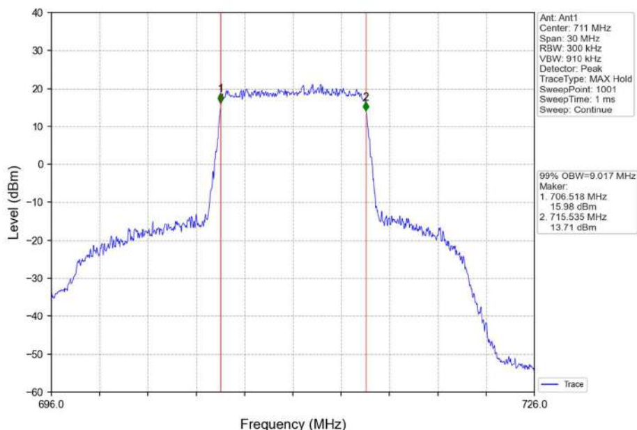
Band12_10MHz_QPSK_HCH_711MHz_RB_50_0_NTNV
