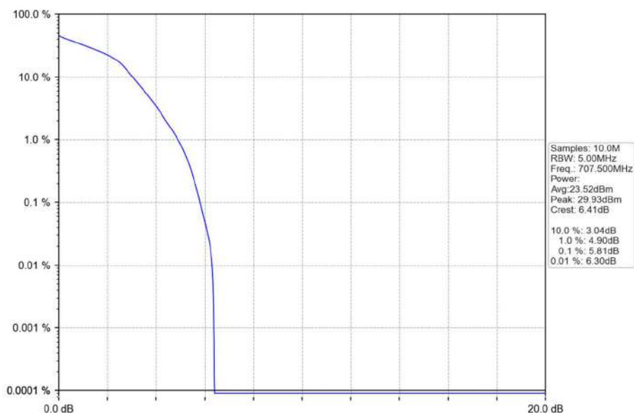
Band12_1.4MHz_16QAM_MCH_707.5MHz_RB_6_0_NTNV
