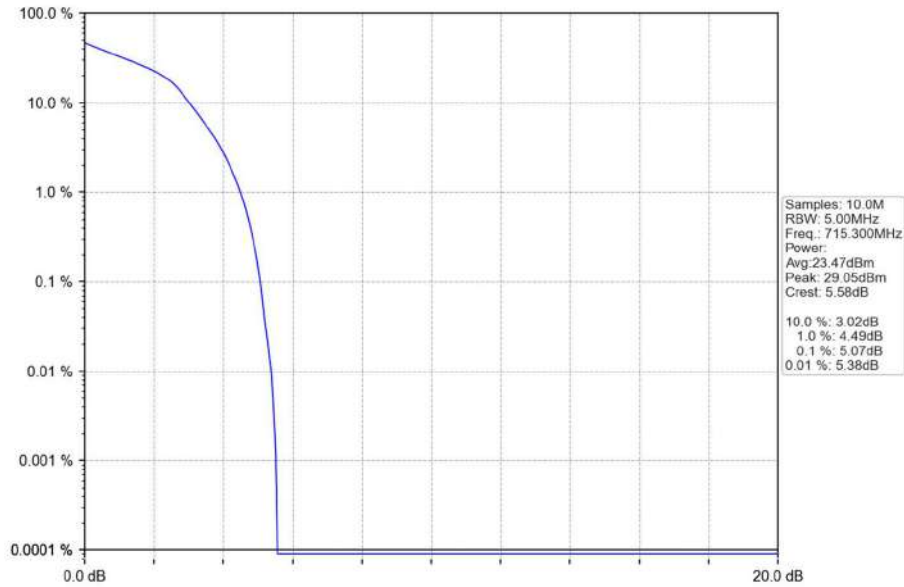
Band12_1.4MHz_16QAM_HCH_715.3MHz_RB_6_0_NTNV
