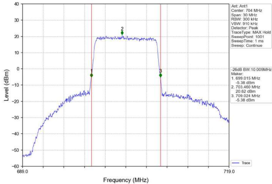
Band12_10MHz_QPSK_LCH_704MHz_RB_50_0_NTNV
