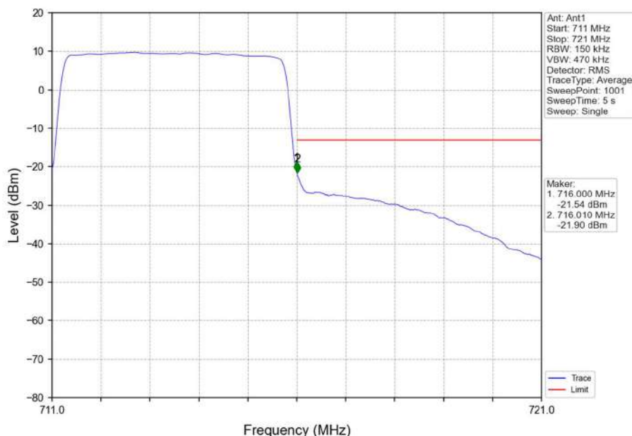
Band12_5MHz_16QAM_HCH_713.5MHz_RB_25_0_NTNV
