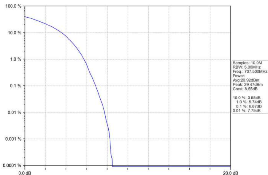
Band12_10MHz_16QAM_MCH_707.5MHz_RB_50_0_NTNV
