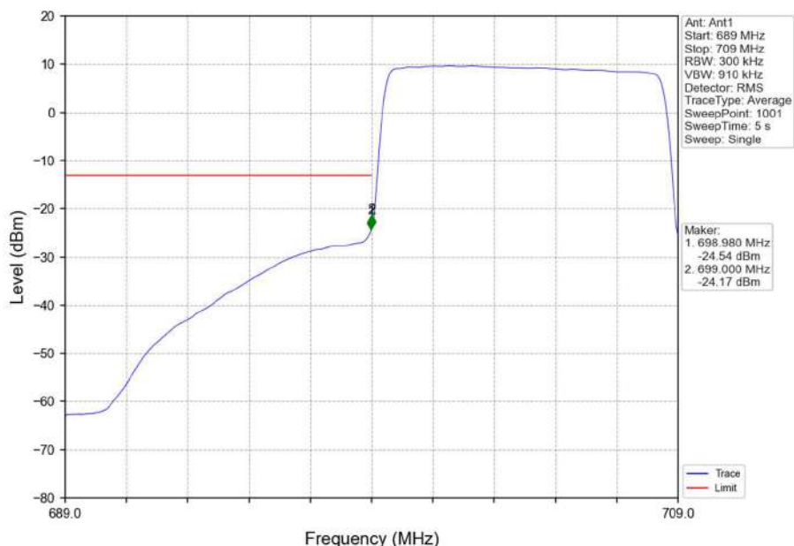
Band12_10MHz_16QAM_LCH_704MHz_RB_50_0_NTNV
