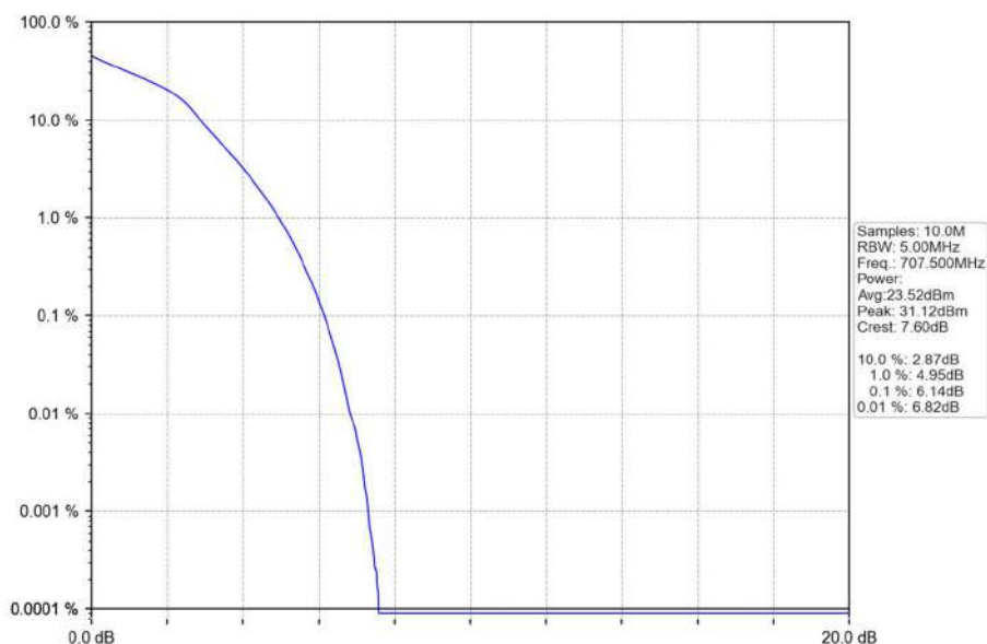
Band12_5MHz_16QAM_MCH_707.5MHz_RB_25_0_NTNV
