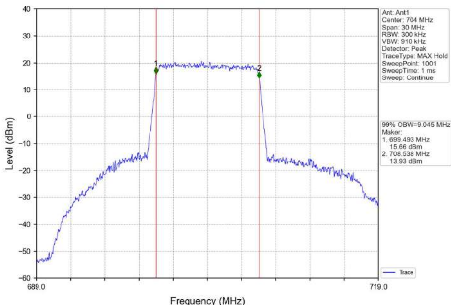
Band12_10MHz_QPSK_LCH_704MHz_RB_50_0_NTNV
