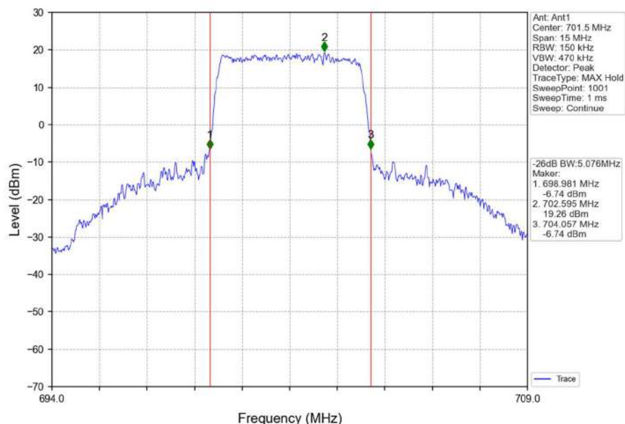
Band12_5MHz_16QAM_LCH_701.5MHz_RB_25_0_NTNV
