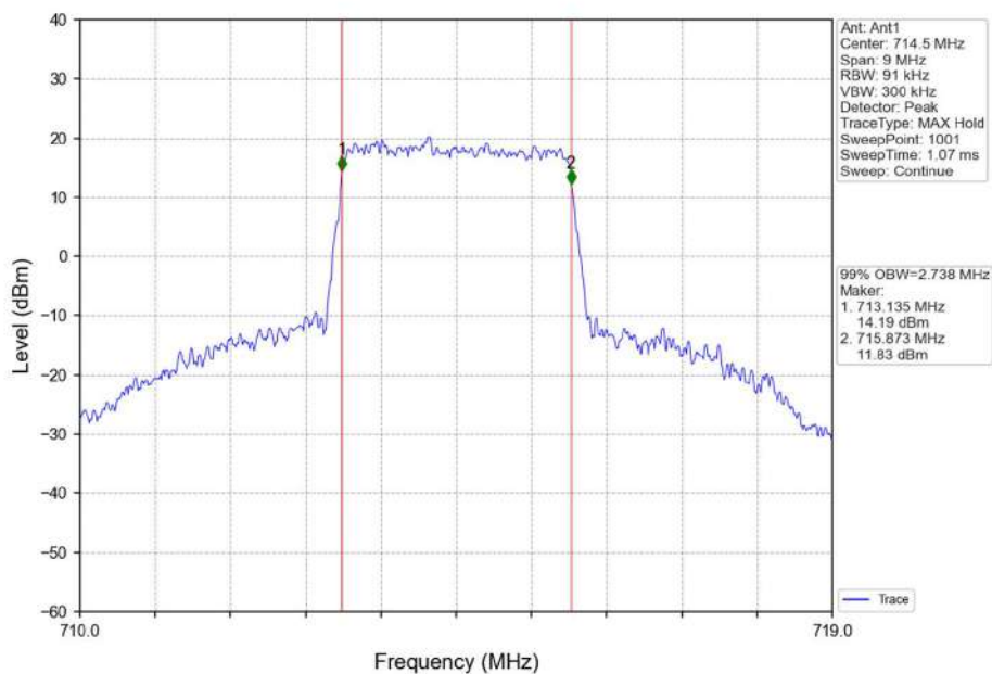
Band12_3MHz_16QAM_HCH_714.5MHz_RB_15_0_NTNV
