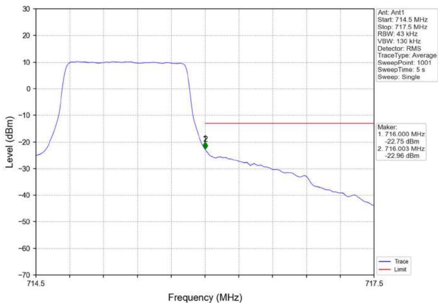
Band12_1.4MHz_16QAM_HCH_715.3MHz_RB_6_0_NTNV
