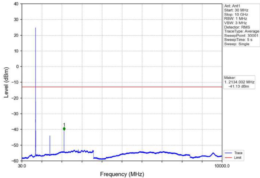
Band12_5MHz_16QAM_HCH_713.5MHz_RB_1_0_NTNV
