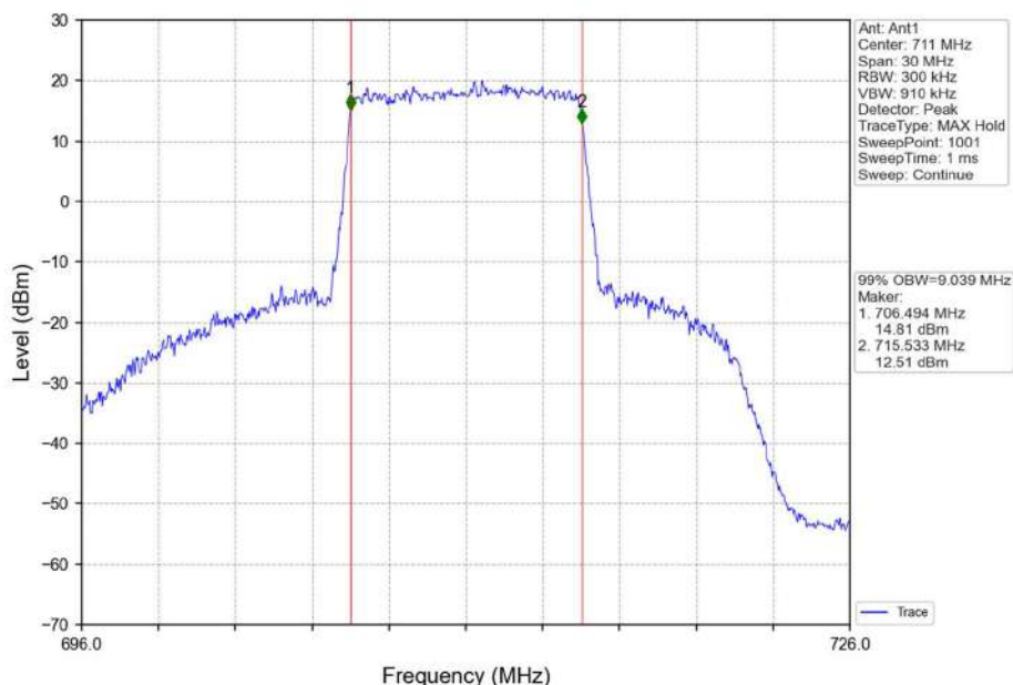
Band12_10MHz_16QAM_HCH_711MHz_RB_50_0_NTNV
