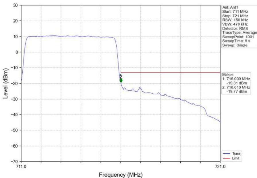
Band12_5MHz_QPSK_HCH_713.5MHz_RB_25_0_NTNV
