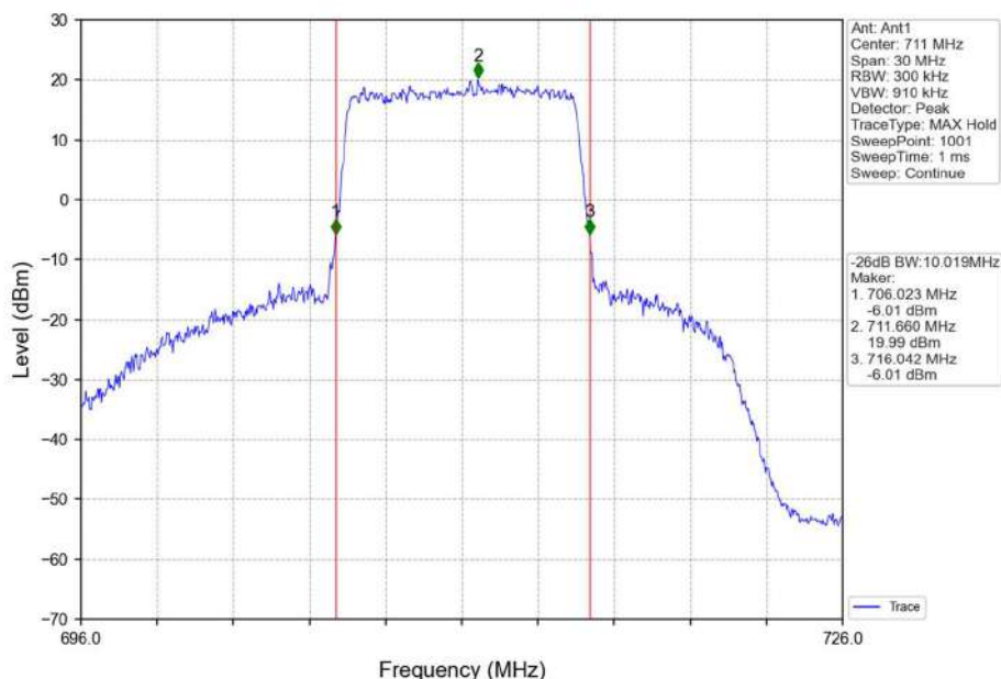
Band12_10MHz_16QAM_HCH_711MHz_RB_50_0_NTNV
