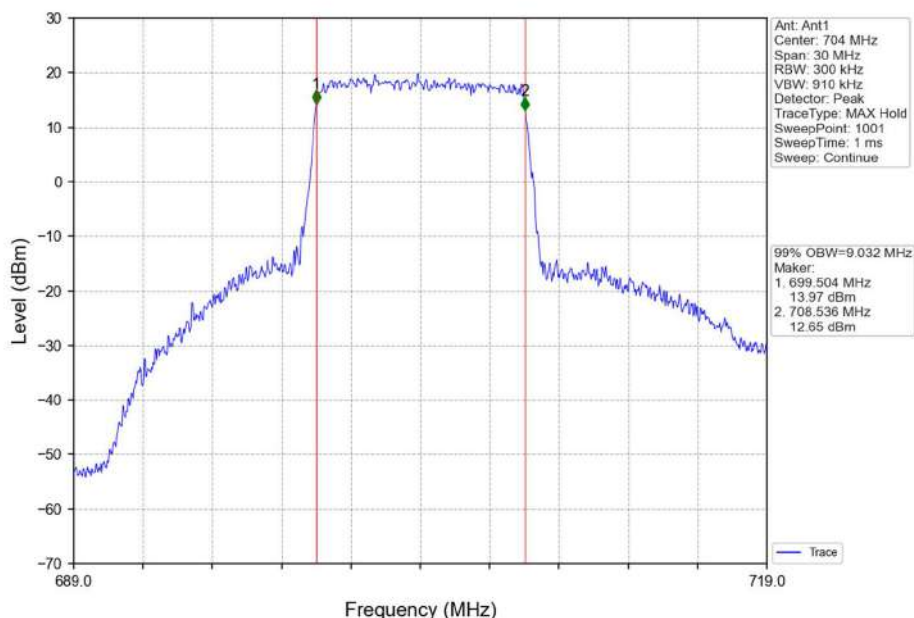
Band12_10MHz_16QAM_LCH_704MHz_RB_50_0_NTNV
