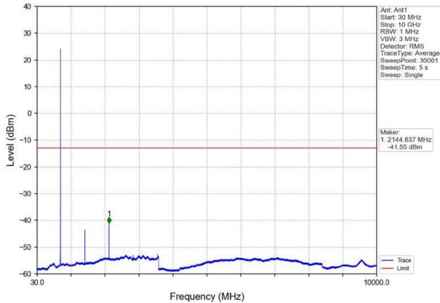
Band12_1.4MHz_16QAM_HCH_715.3MHz_RB_1_0_NTNV
