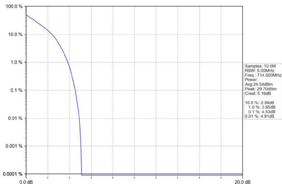
Band12_3MHz_QPSK_HCH_714.5MHz_RB_15_0_NTNV
