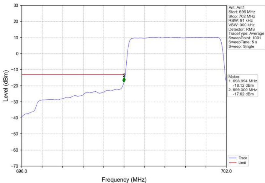
Band12_3MHz_QPSK_LCH_700.5MHz_RB_15_0_NTNV
