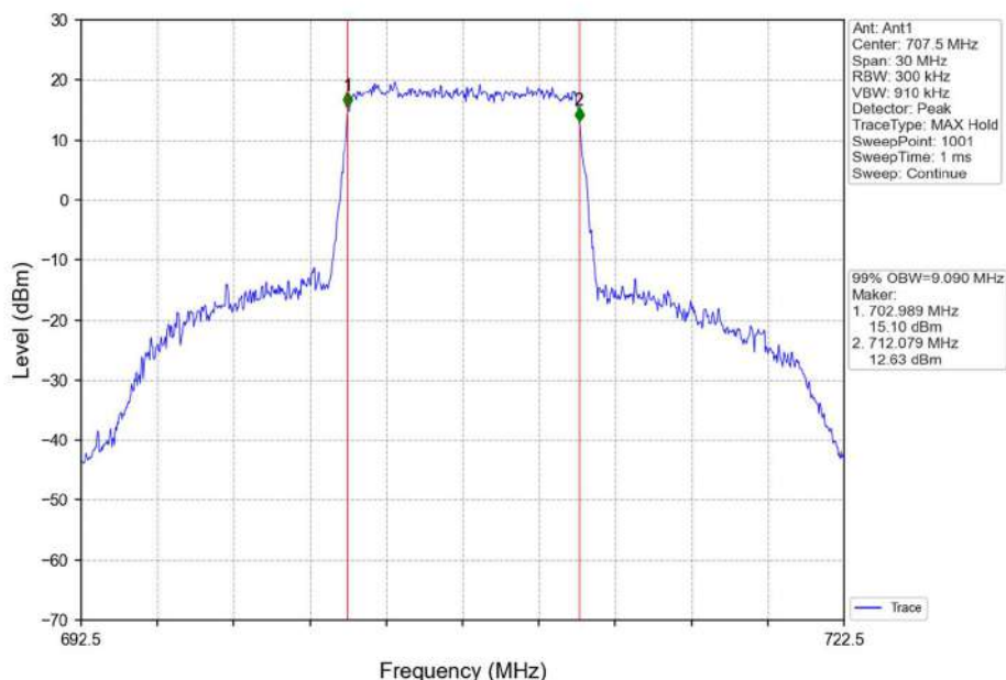
Band12_10MHz_16QAM_MCH_707.5MHz_RB_50_0_NTNV
