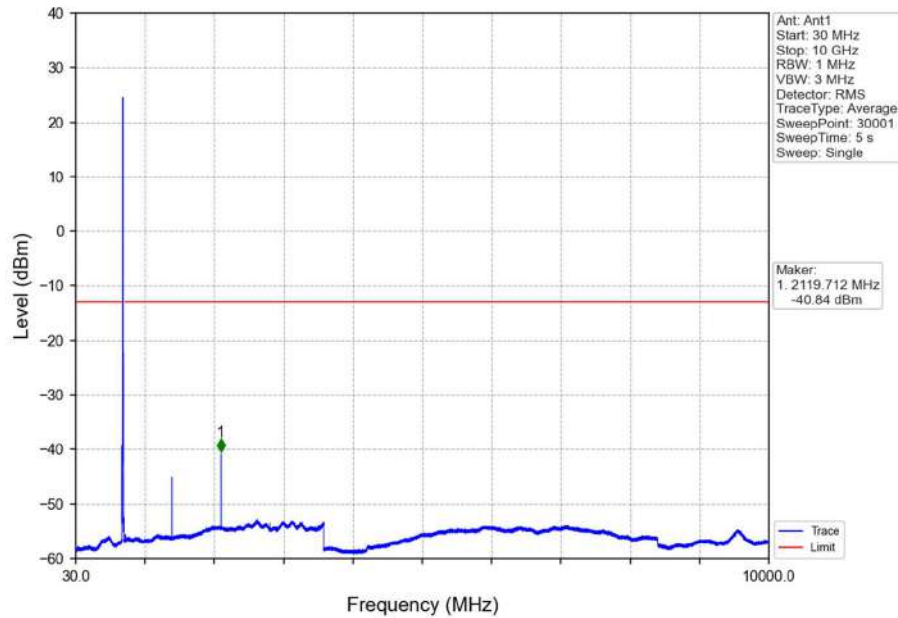
Band12_10MHz_16QAM_HCH_711MHz_RB_1_0_NTNV
