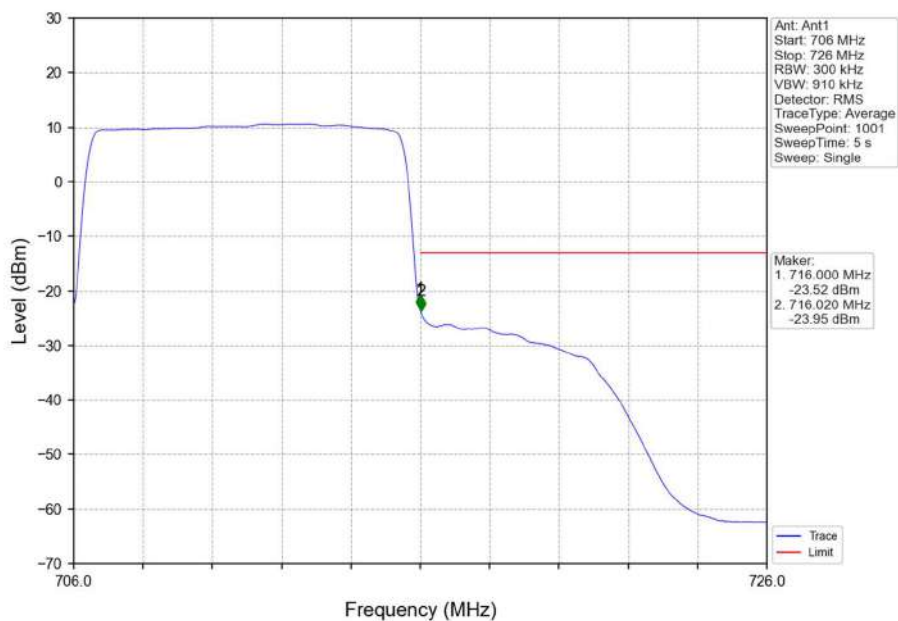
Band12_10MHz_QPSK_HCH_711MHz_RB_50_0_NTNV
