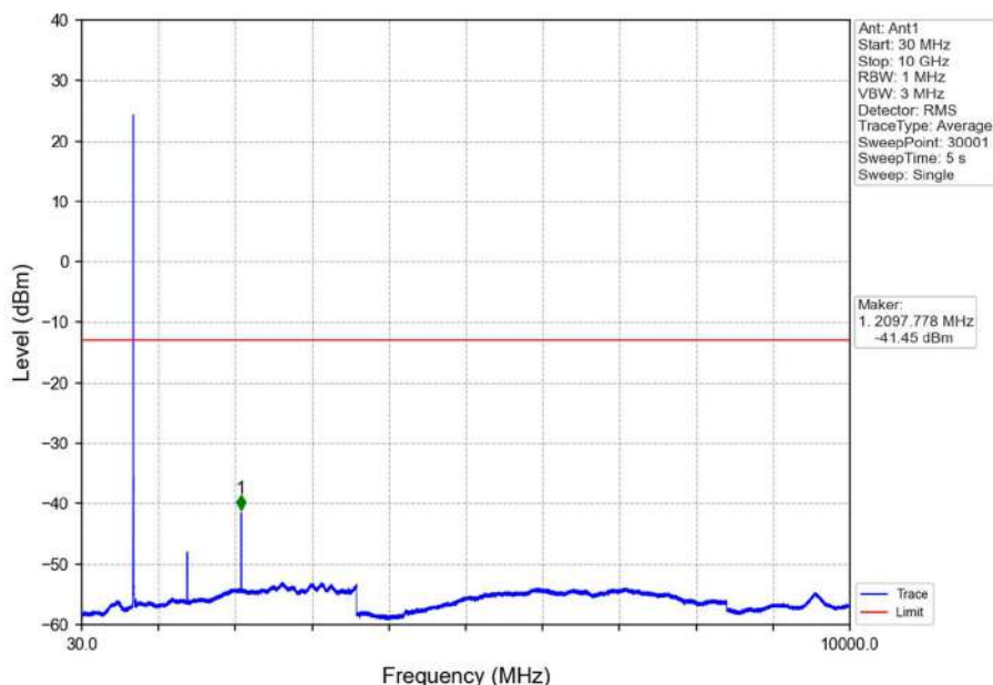
Band12_3MHz_16QAM_LCH_700.5MHz_RB_1_0_NTNV
