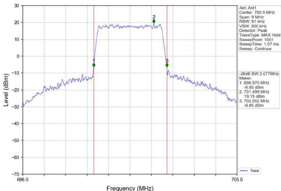
Band12_3MHz_16QAM_LCH_700.5MHz_RB_15_0_NTNV
