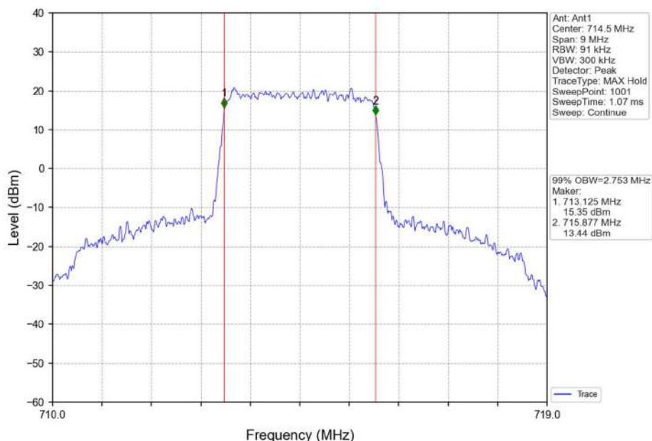
Band12_3MHz_QPSK_HCH_714.5MHz_RB_15_0_NTNV
