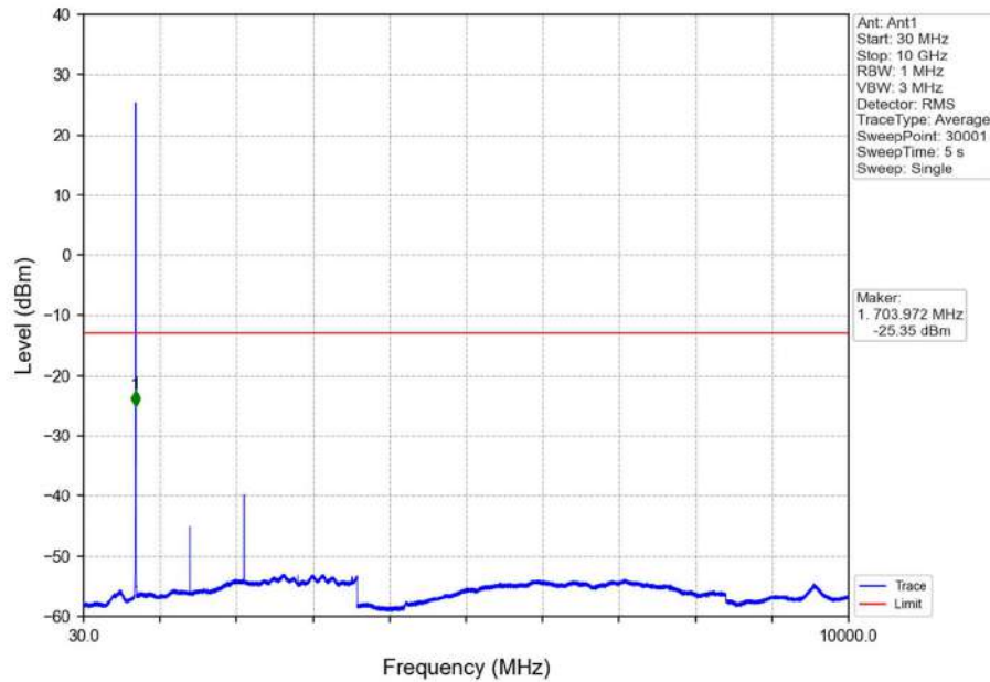
Band12_1.4MHz_QPSK_MCH_707.5MHz_RB_1_0_NTNV
