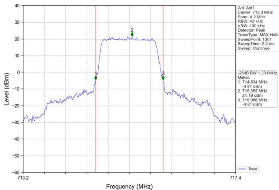
Band12_1.4MHz_QPSK_HCH_715.3MHz_RB_6_0_NTNV
