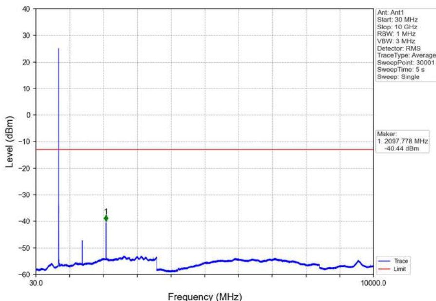
Band12_3MHz_QPSK_LCH_700.5MHz_RB_1_0_NTNV
