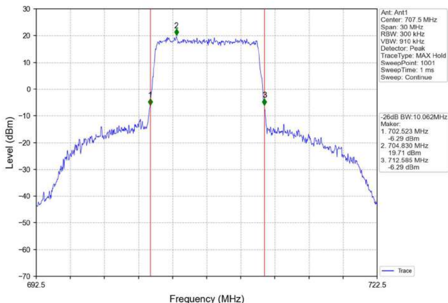
Band12_10MHz_16QAM_MCH_707.5MHz_RB_50_0_NTNV
