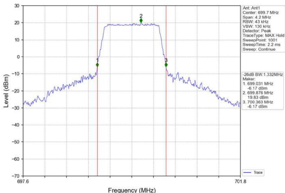
Band12_1.4MHz_16QAM_LCH_699.7MHz_RB_6_0_NTNV
