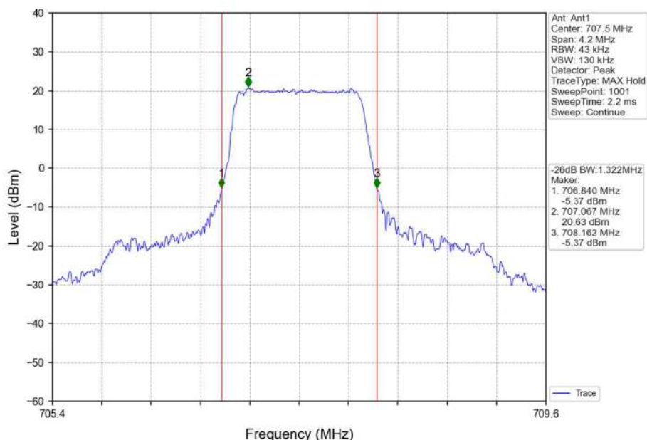
Band12_1.4MHz_QPSK_MCH_707.5MHz_RB_6_0_NTNV
