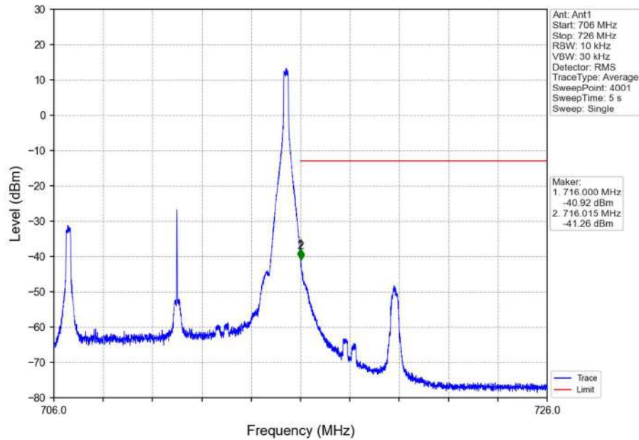
Band12_10MHz_16QAM_HCH_711MHz_RB_1_49_NTNV
