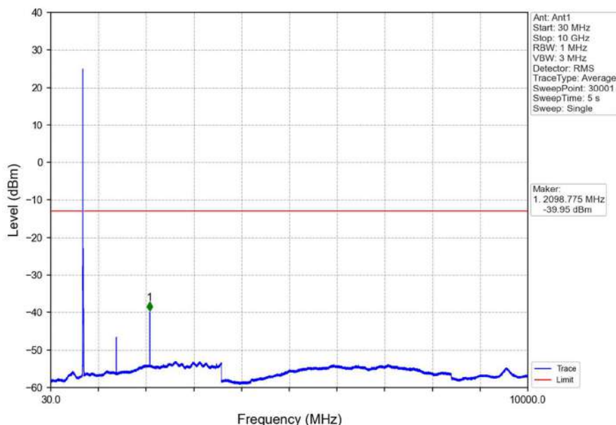
Band12_10MHz_QPSK_LCH_704MHz_RB_1_0_NTNV
