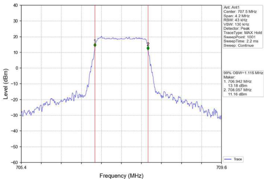
Band12_1.4MHz_16QAM_MCH_707.5MHz_RB_6_0_NTNV
