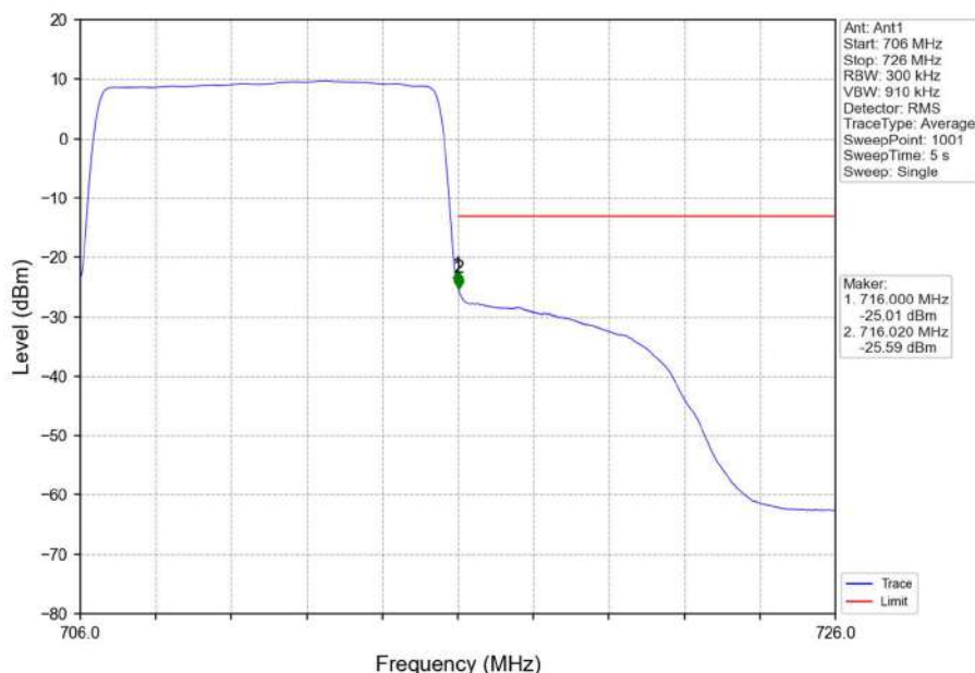
Band12_10MHz_16QAM_HCH_711MHz_RB_50_0_NTNV
