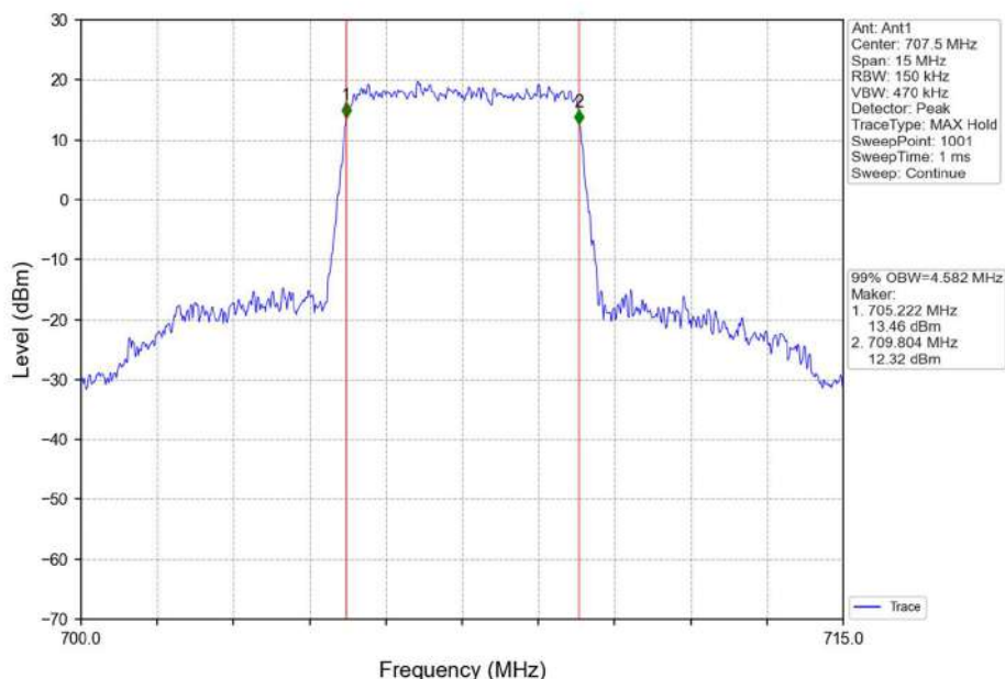
Band12_5MHz_16QAM_MCH_707.5MHz_RB_25_0_NTNV
