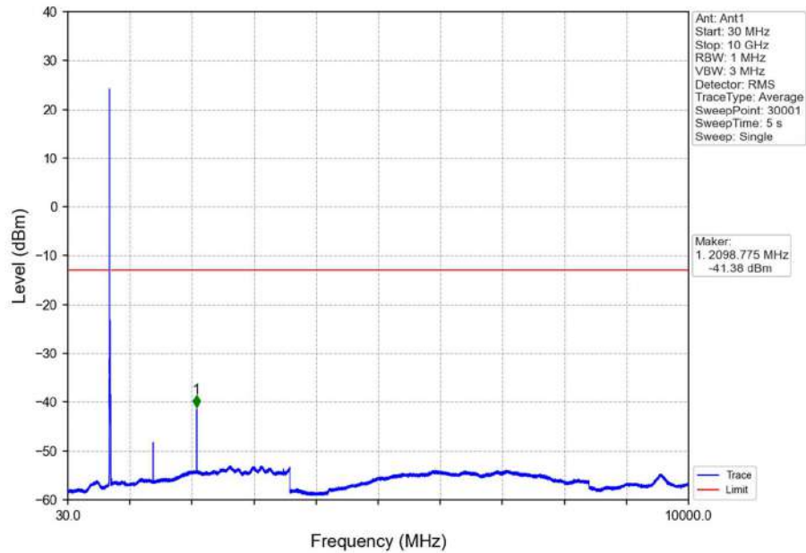
Band12_10MHz_16QAM_LCH_704MHz_RB_1_0_NTNV
