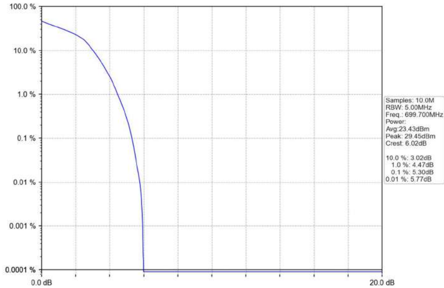
Band12_1.4MHz_16QAM_LCH_699.7MHz_RB_6_0_NTNV
