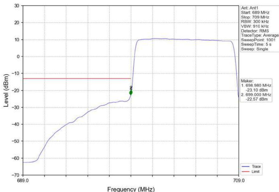
Band12_10MHz_QPSK_LCH_704MHz_RB_50_0_NTNV
