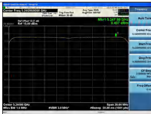
Test Mode:802.11ax HE20 5240MHz Chain1
