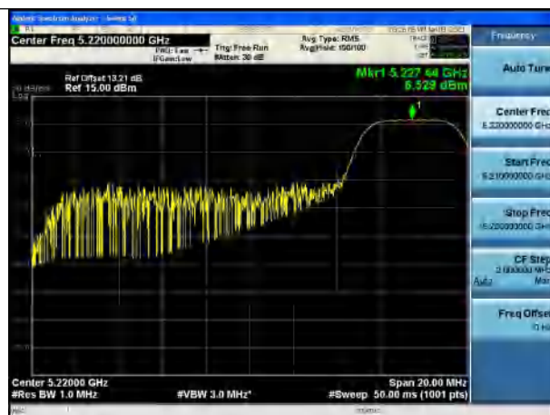
Test Mode:802.11ax HE20 5220MHz Chain0
