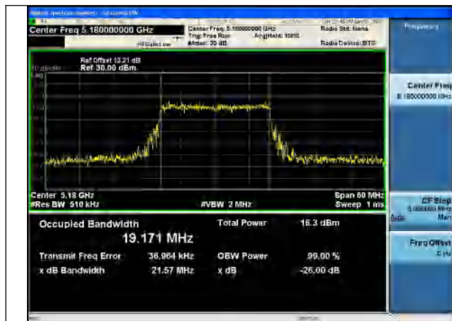
Test Mode:802.11ax HE20 5180MHz Chain0
