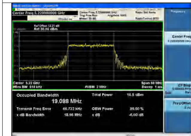
Test Mode:802.11ax HE20 5220MHz Chain1
