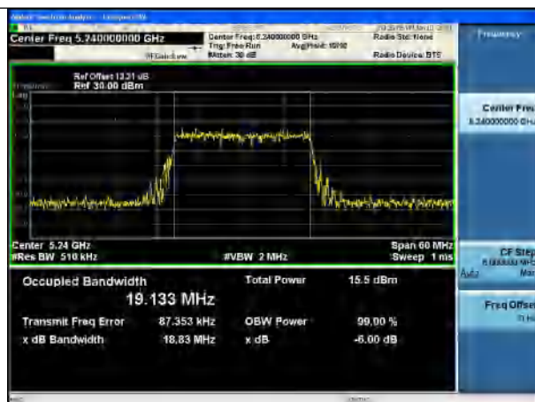
Test Mode:802.11be EHT20 5240MHz Chain1
