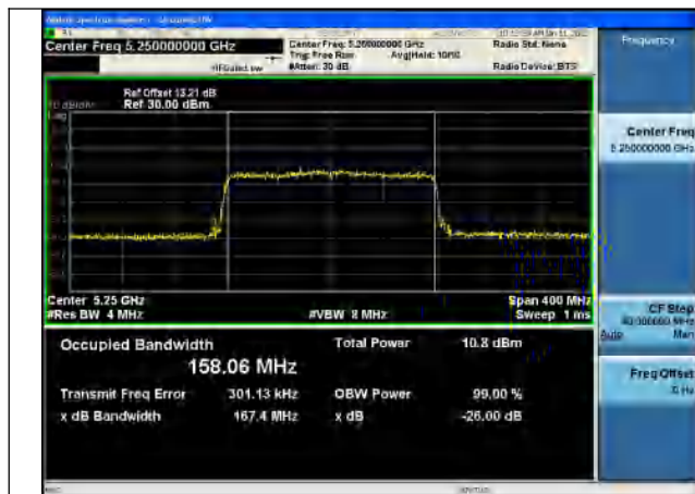
Test Mode:802.11be EHT160 5250MHz Chain0
