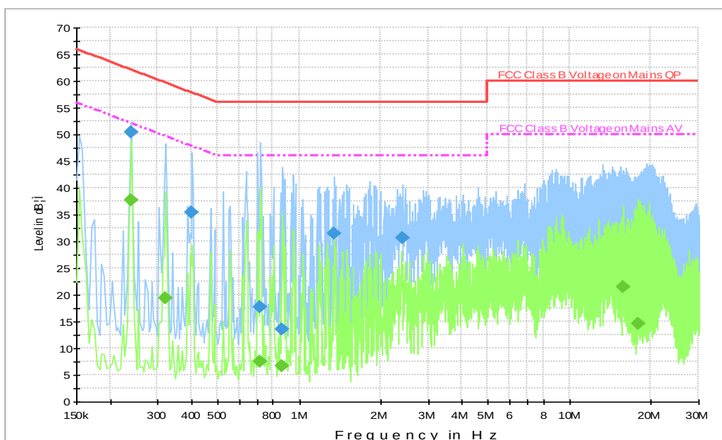
Fig. 50 Conducted Emission(802.11a, IDLE)
