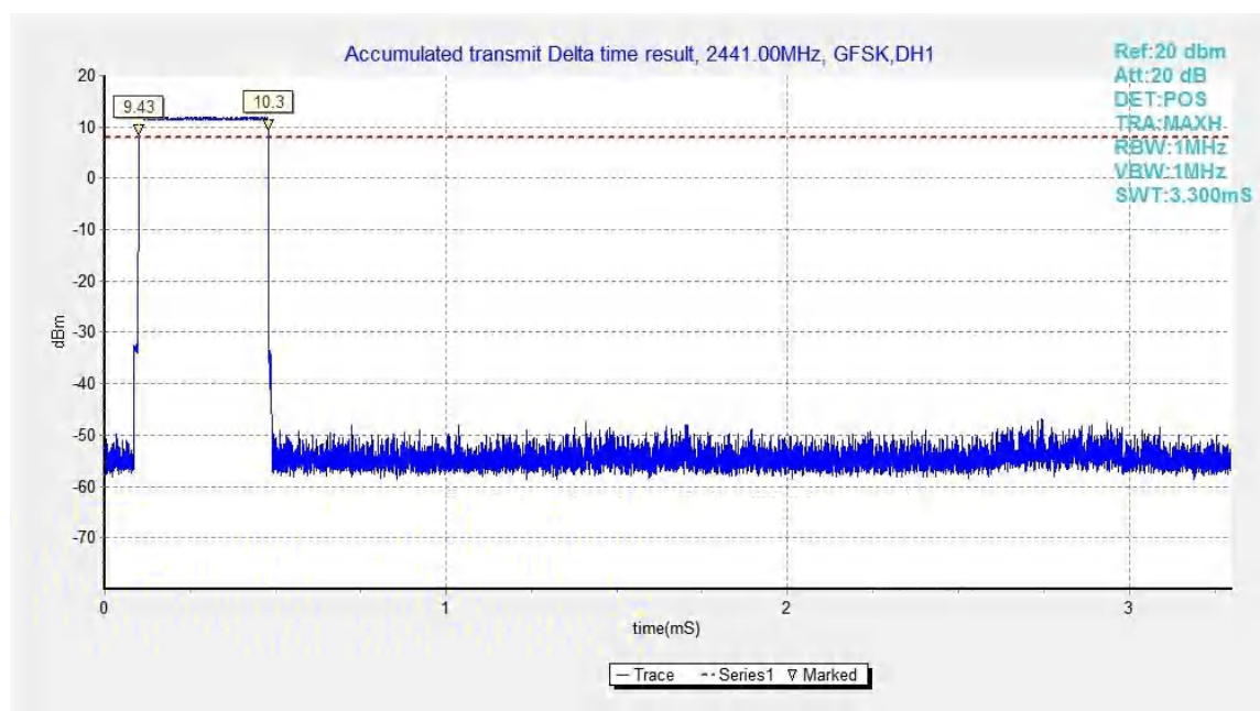
Fig.58. Time of occupancy (Dwell Time): Channel 39, Packet DH1
