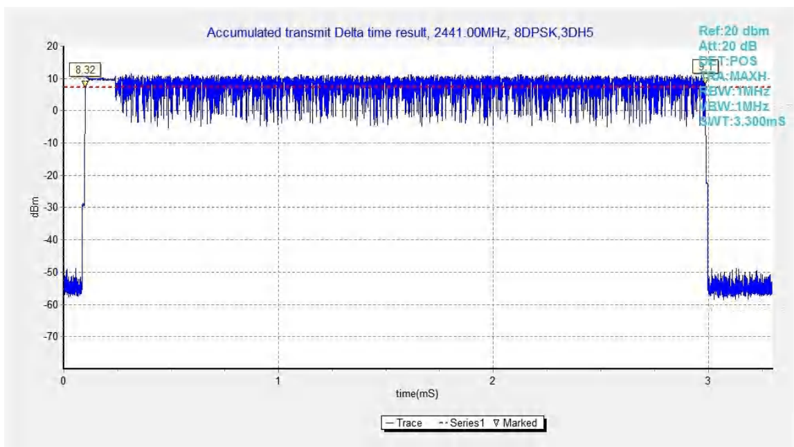
Fig.74. Time of occupancy (Dwell Time): Channel 39, Packet 3-DH5
