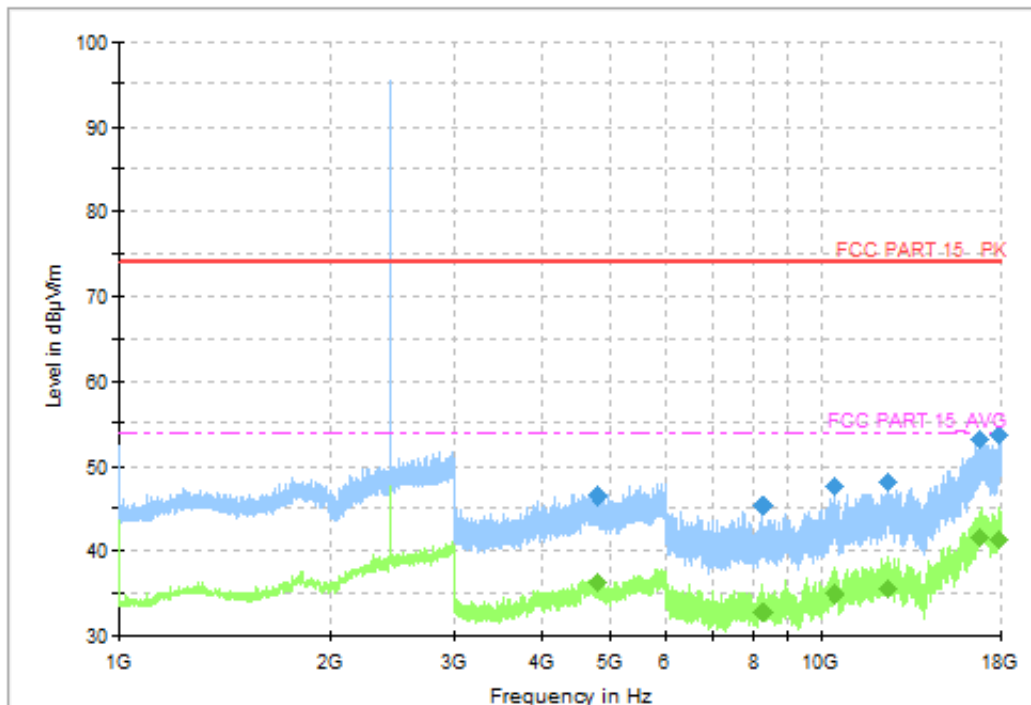
Fig. 2 Radiated Spurious Emission (GFSK, CH39, 1GHz ~18GHz)
