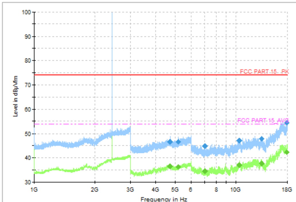
Fig. 12 Radiated Spurious Emission (8DPSK, CH39, 1GHz ~18GHz)
