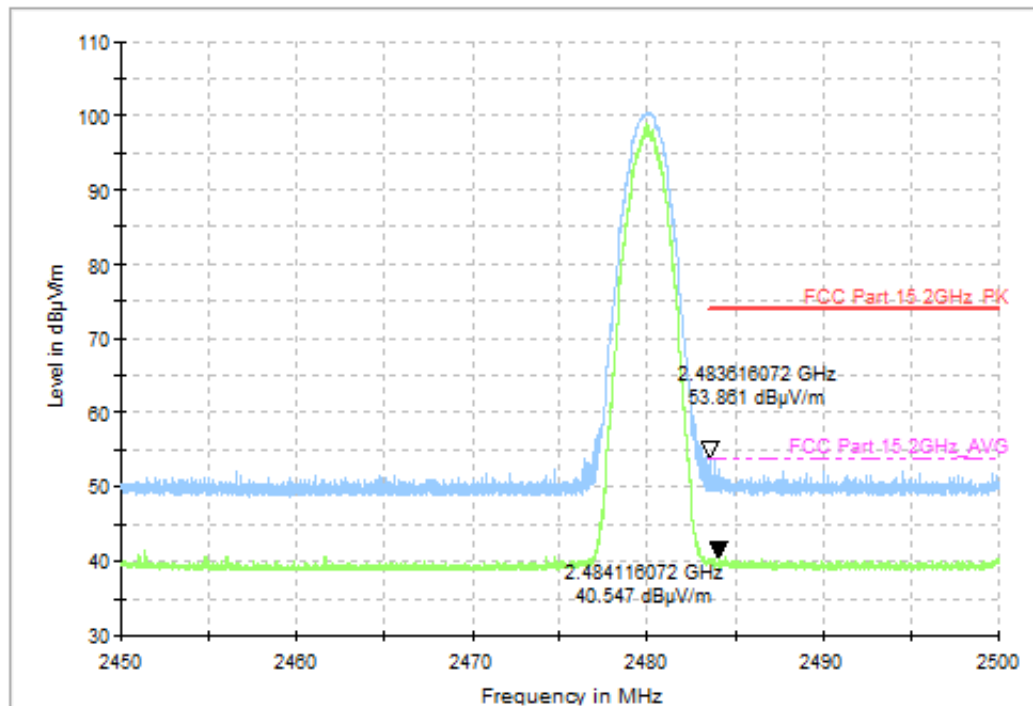
Fig. 15 Radiated Band Edges (8DPSK, CH78, 2.45GHz~2.50GHz)
