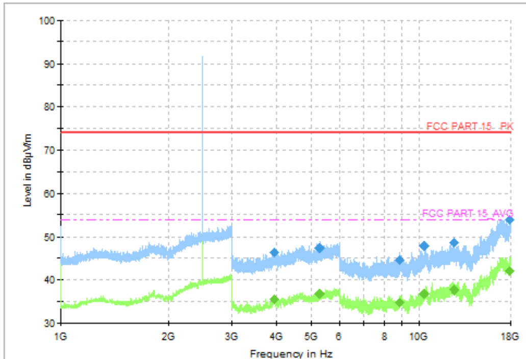
Fig. 3 Radiated Spurious Emission (GFSK, CH78, 1GHz ~18GHz)
