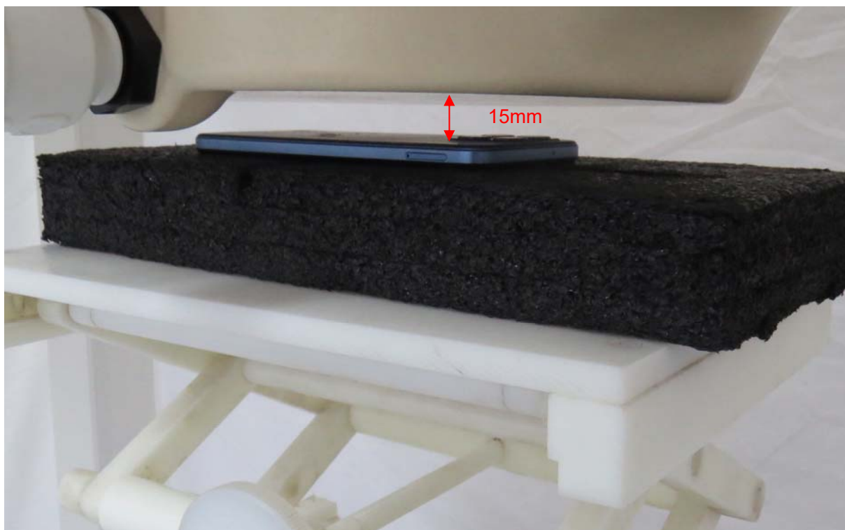
Picture 5: Back Side, the distance from handset to the bottom of the Phantom is 15mm
