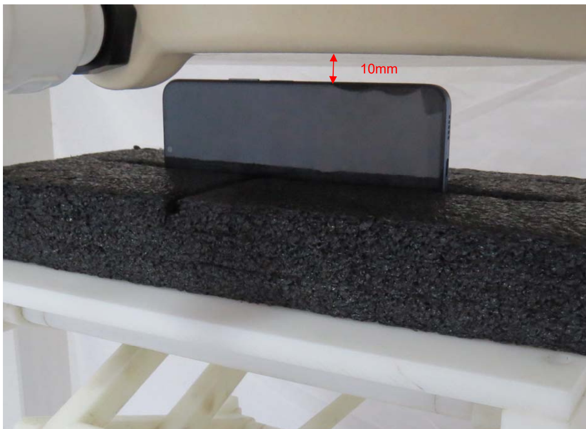
Picture 10: Right Edge, the distance from handset to the bottom of the Phantom is 10mm
