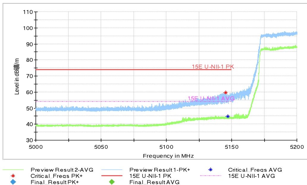
Fig.63 Band Edges (802.11ac-HT80, CH42, 5210MHz)
