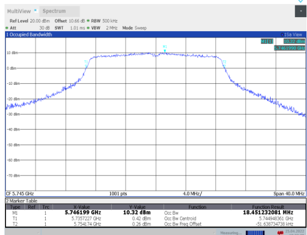
11AC20SISO_Ant1_5745
