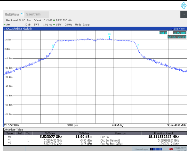
11AC20SISO_Ant1_5520
