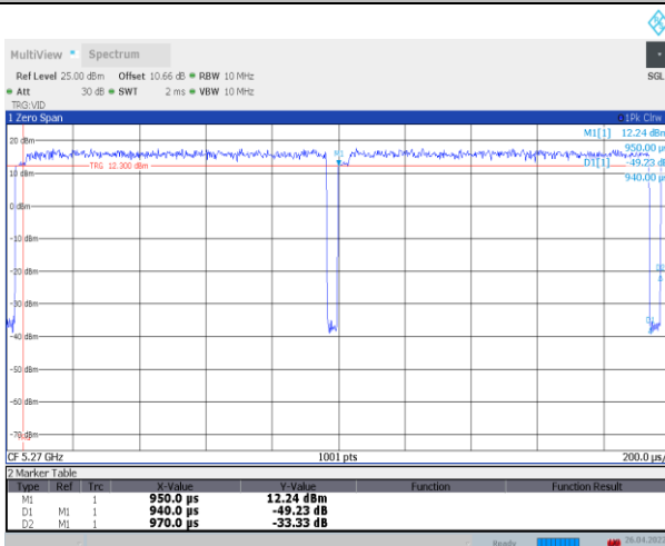
11AC40SISO_Ant1_5270
