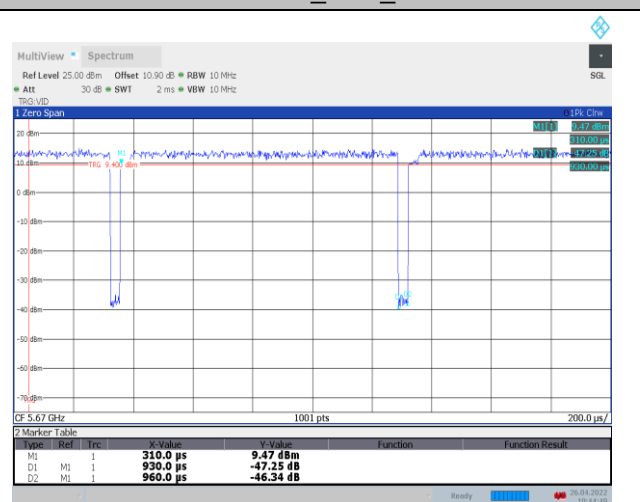
11N40SISO_Ant1_5670
