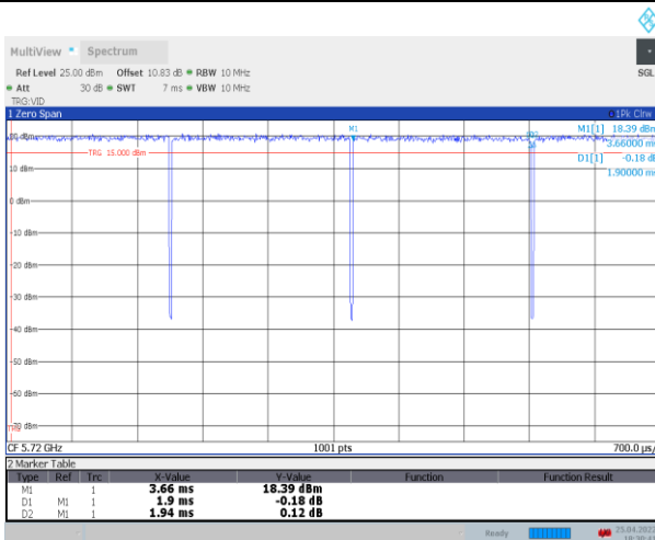
11AC20SISO_Ant1_5720
