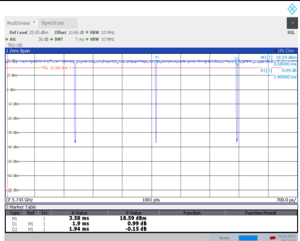
11AC20SISO_Ant1_5745
