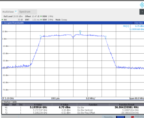
11N40SISO_Ant1_5190
