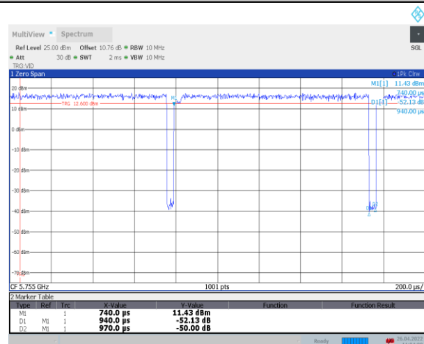
11AC40SISO_Ant1_5755
