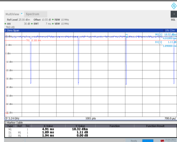
11AC20SISO_Ant1_5240
