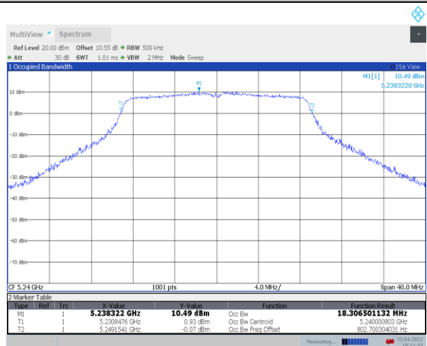
11AC20SISO_Ant1_5240
