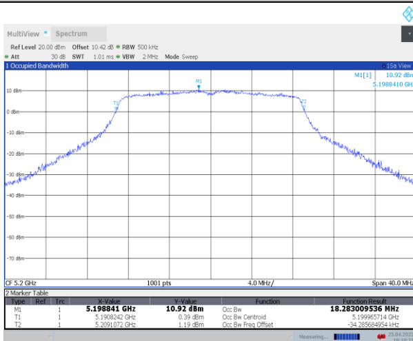
11AC20SISO_Ant1_5200
