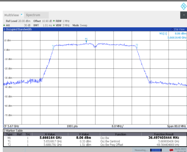
11N40SISO_Ant1_5670
