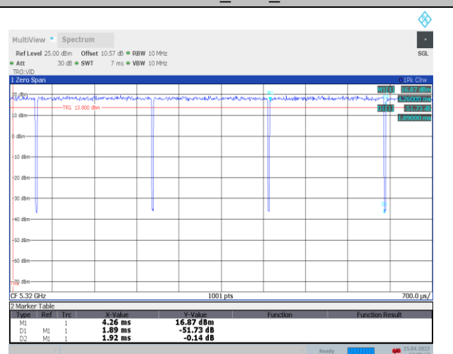
11N20SISO_Ant1_5320
