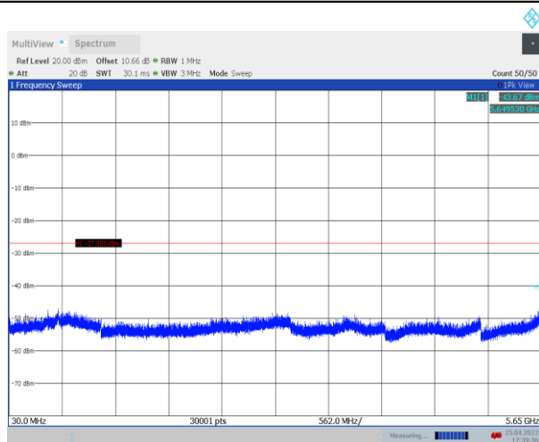
11N20SISO_Ant1_5785_30~5650
