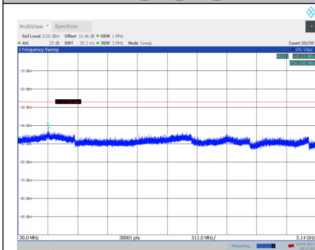
11AC20SISO_Ant1_5300_30~5140
