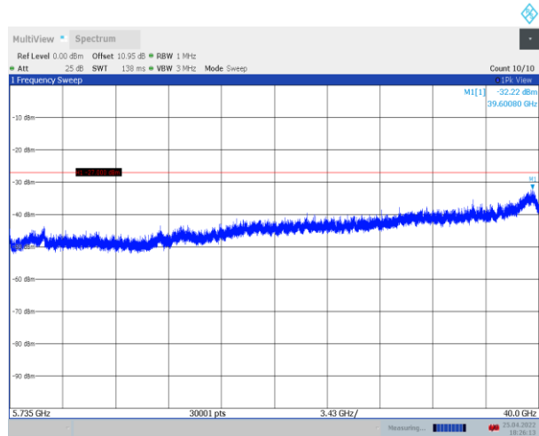
11AC20SISO_Ant1_5680_5735~40000
