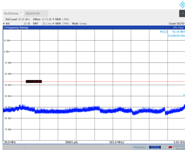
11N40SISO_Ant1_5795_30~5650
