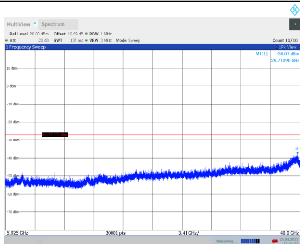
11N20SISO_Ant1_5785_5925~40000
