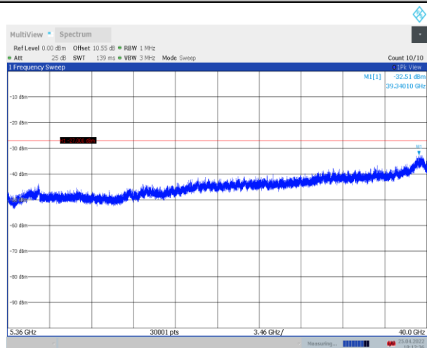
11AC20SISO_Ant1_5240_5360~40000
