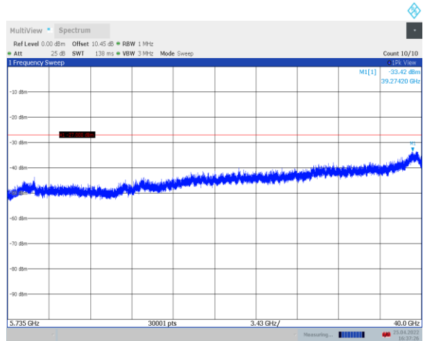
11A_Ant1_5660_5735~40000
