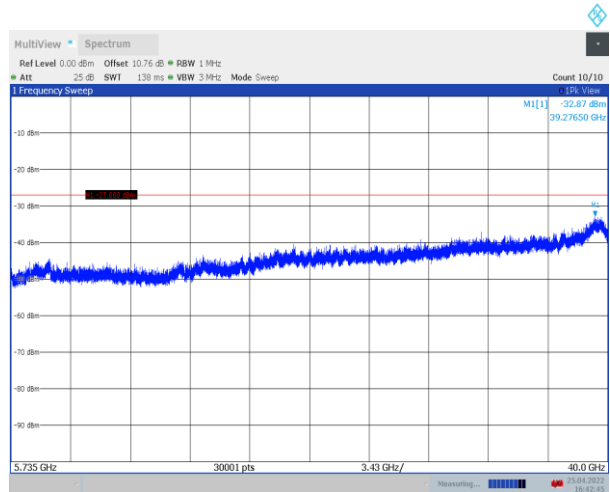
11A_Ant1_5680_5735~40000
