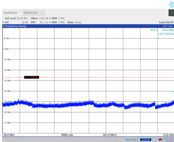
11A_Ant1_5745_30~5650
