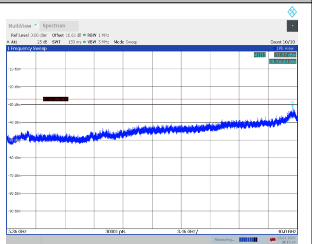
11AC20SISO_Ant1_5300_5360~40000
