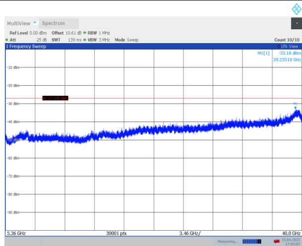
11N20SISO_Ant1_5300_5360~40000
