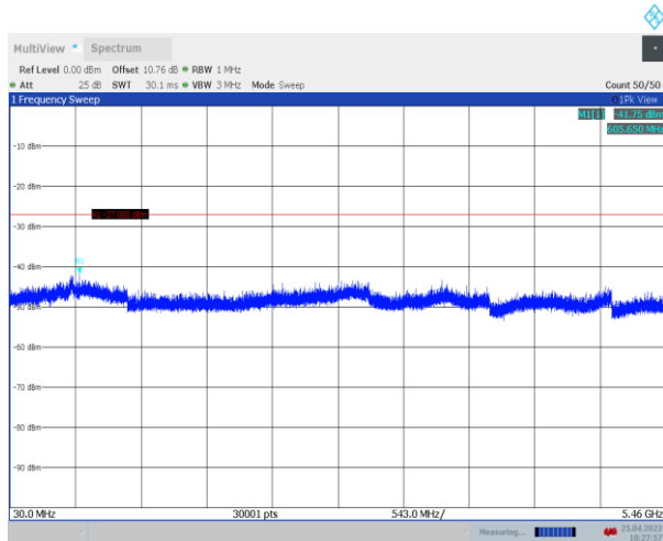
11AC20SISO_Ant1_5680_30~5460
