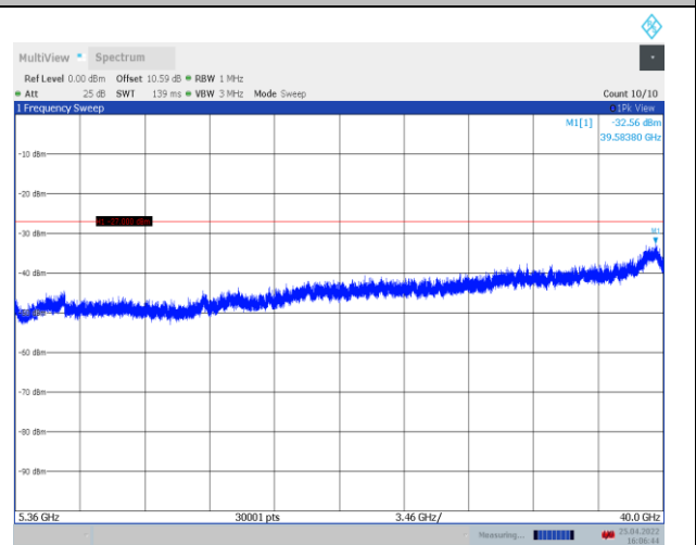
11A_Ant1_5280_5360~40000
