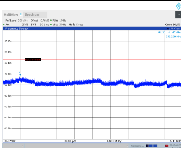
11N20SISO_Ant1_5700_30~5460
