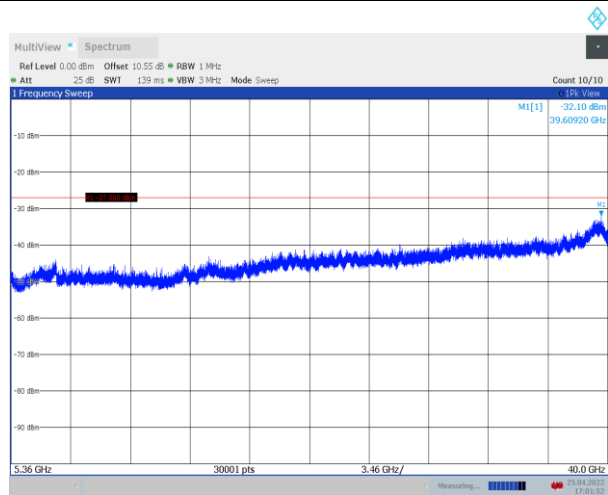
11N20SISO_Ant1_5260_5360~40000
