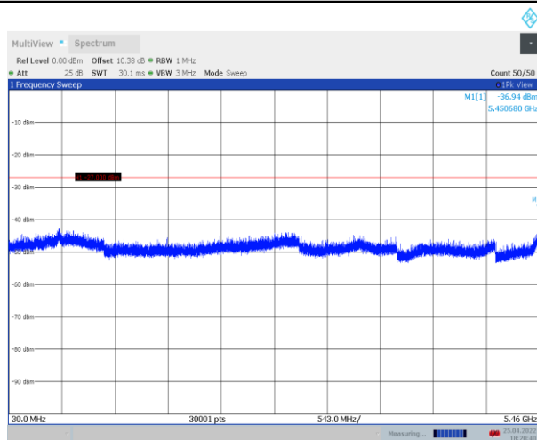
11AC20SISO_Ant1_5520_30~5460
