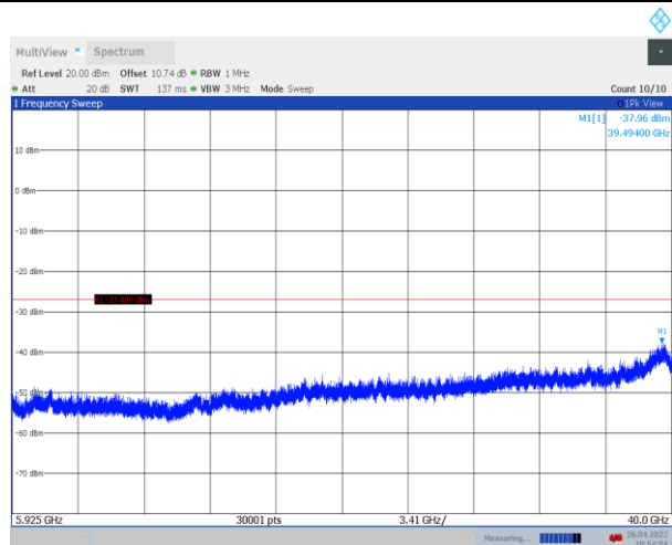
11N40SISO_Ant1_5795_5925~40000
