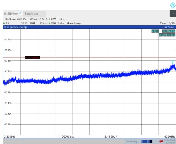
11AC20SISO_Ant1_5200_5360~40000
