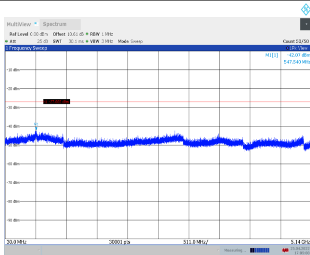
11N20SISO_Ant1_5300_30~5140
