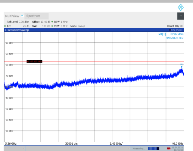
11A_Ant1_5300_5360~40000
