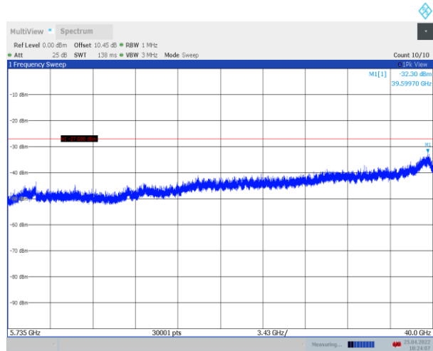
11AC20SISO_Ant1_5660_5735~40000
