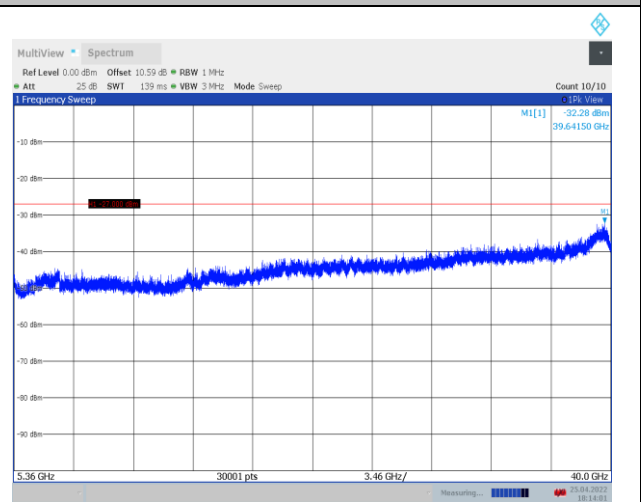
11AC20SISO_Ant1_5280_5360~40000
