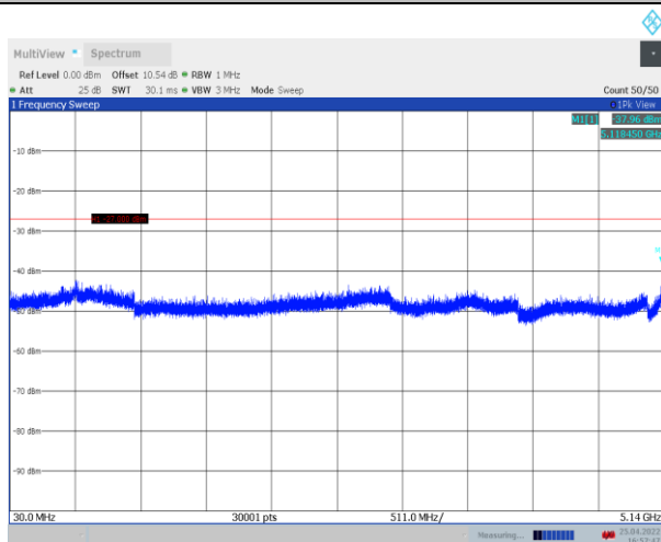
11N20SISO_Ant1_5180_30~5140
