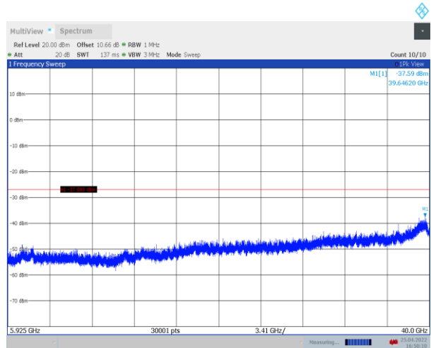
11A_Ant1_5745_5925~40000
