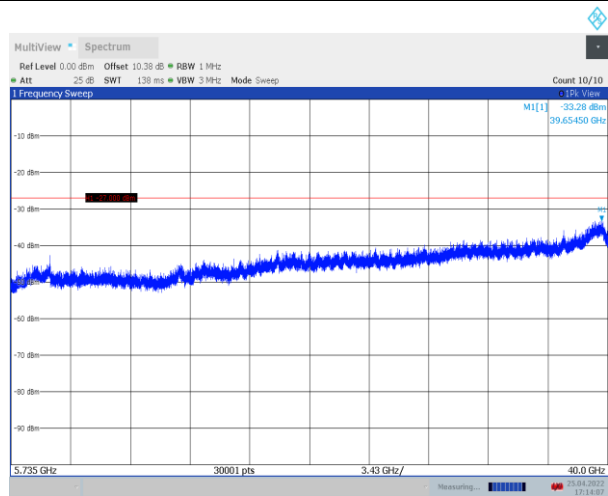
11N20SISO_Ant1_5520_5735~40000
