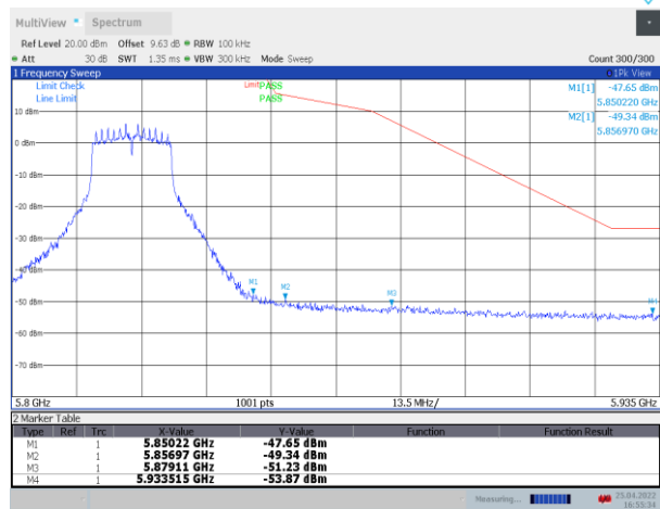
11N20SISO_Ant1_High_5825
