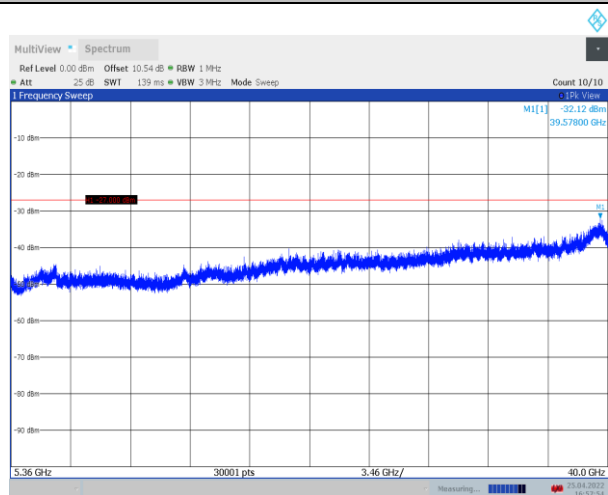
11N20SISO_Ant1_5180_5360~40000
