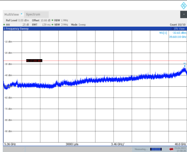
11N40SISO_Ant1_5310_5360~40000
