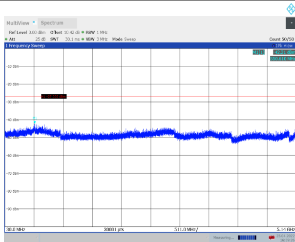
11N20SISO_Ant1_5240_30~5140
