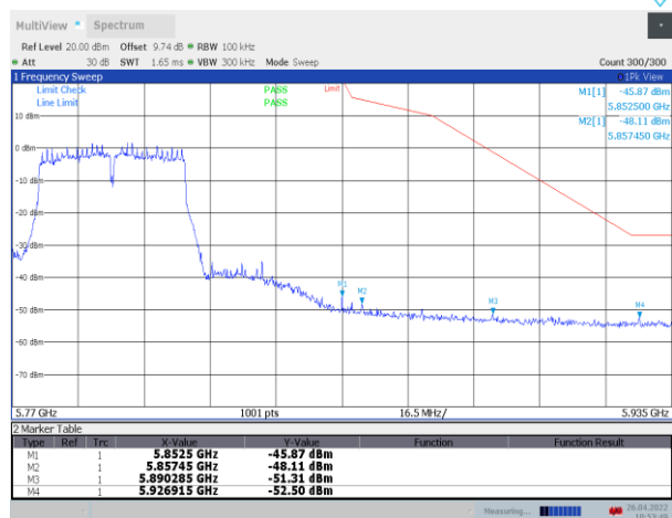
11N40SISO_Ant1_High_5795
