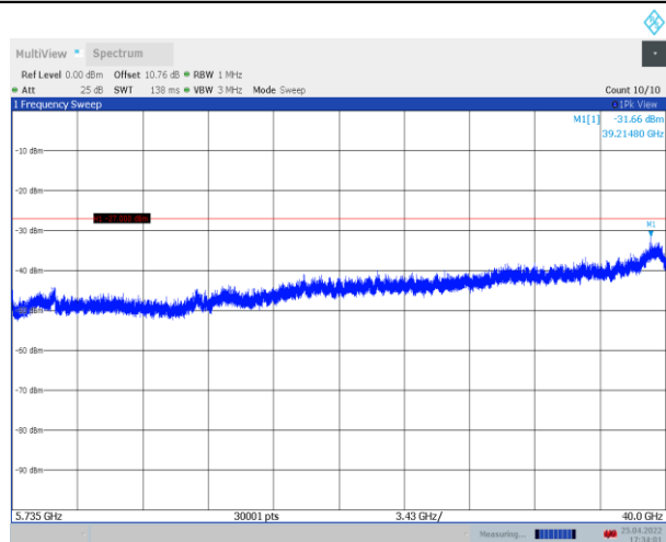
11N20SISO_Ant1_5700_5735~40000
