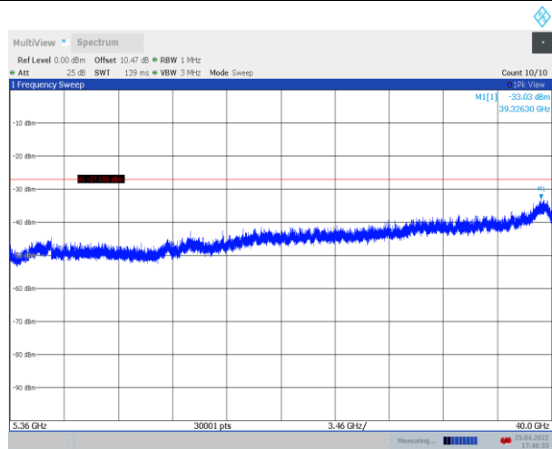
11N40SISO_Ant1_5230_5360~40000
