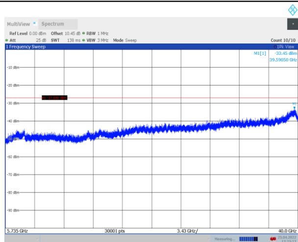
11N20SISO_Ant1_5580_5735~40000
