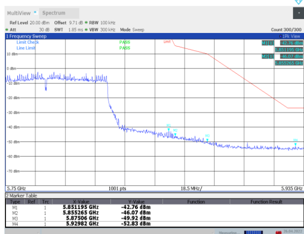
11AC80SISO_Ant1_High_5775
