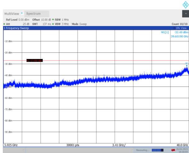
11N40SISO_Ant1_5755_5925~40000
