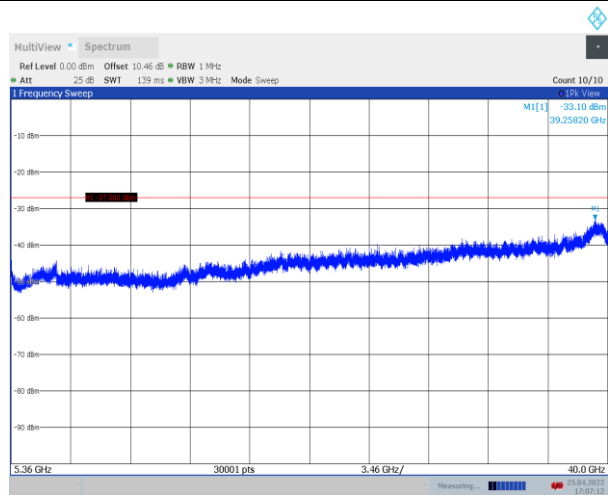
11N20SISO_Ant1_5320_5360~40000
