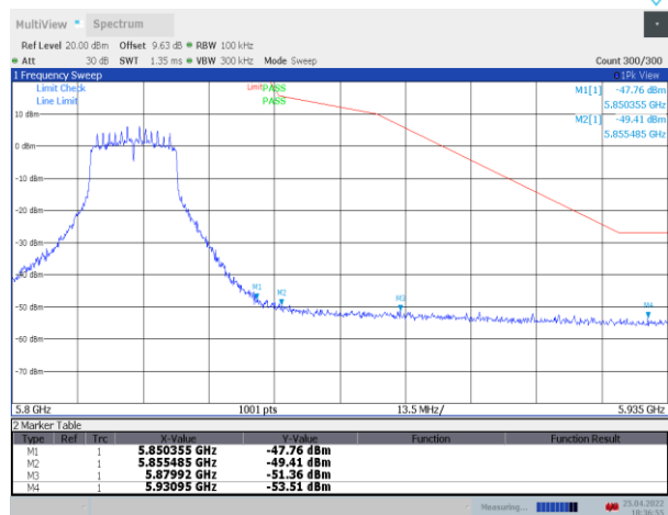
11AC40SISO_Ant1_High_5795
