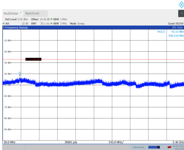
11AC20SISO_Ant1_5660_30~5460
