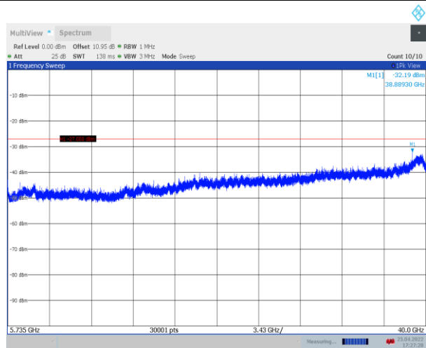
11N20SISO_Ant1_5680_5735~40000
