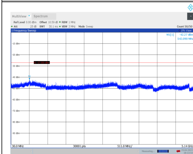
11AC20SISO_Ant1_5280_30~5140
