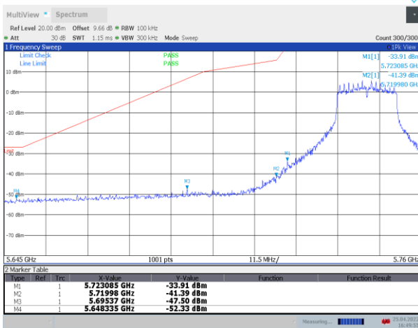
11N20SISO_Ant1_Low_5745
