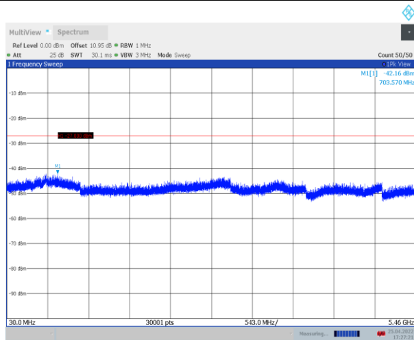
11N20SISO_Ant1_5680_30~5460
