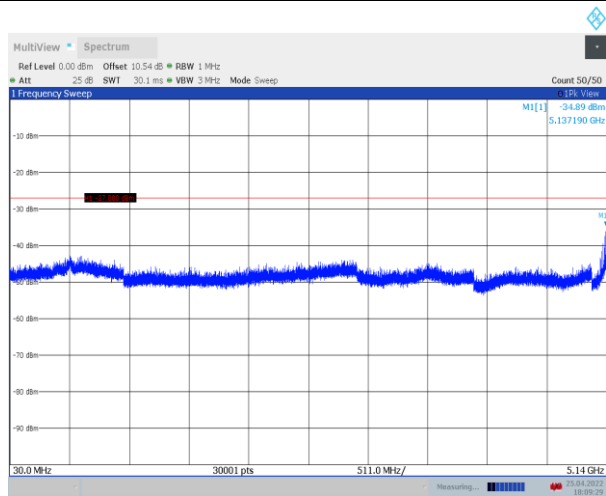
11AC20SISO_Ant1_5200_30~5140
