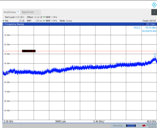
11N20SISO_Ant1_5240_5360~40000
