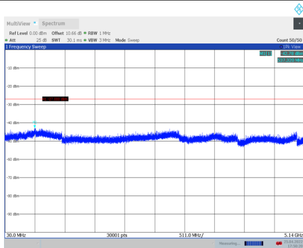
11N40SISO_Ant1_5310_30~5140
