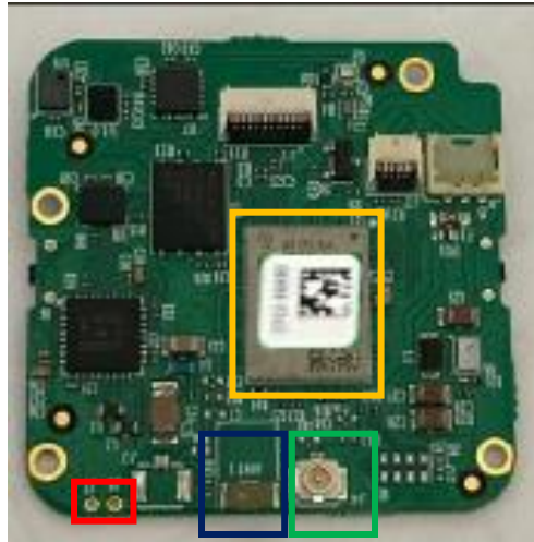
R-Link Watch PCB Assembly
