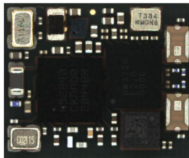
View inside Murata Module (taken from Murata report)
