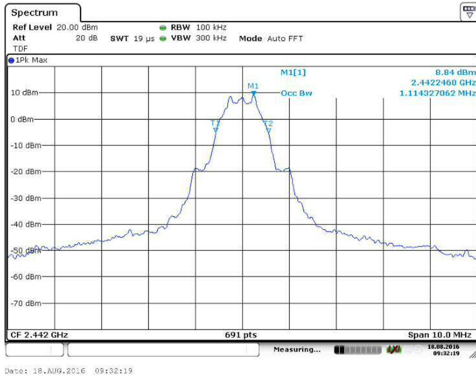
Figure 24: 99% OBW channel mid, BGM121
