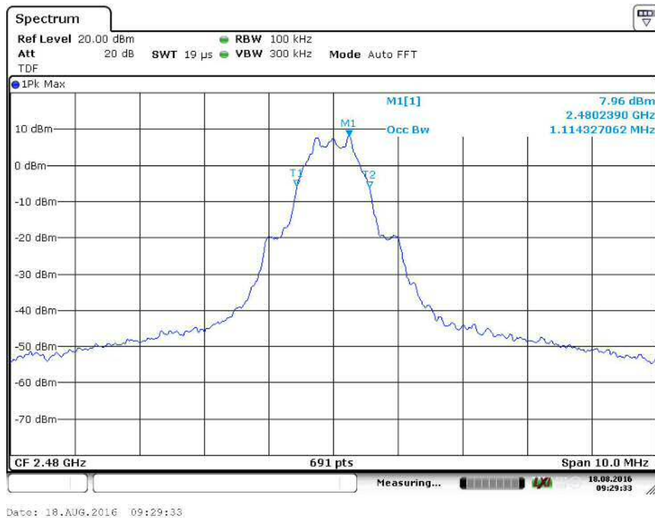
Figure 25: 99% OBW channel high, BGM121
