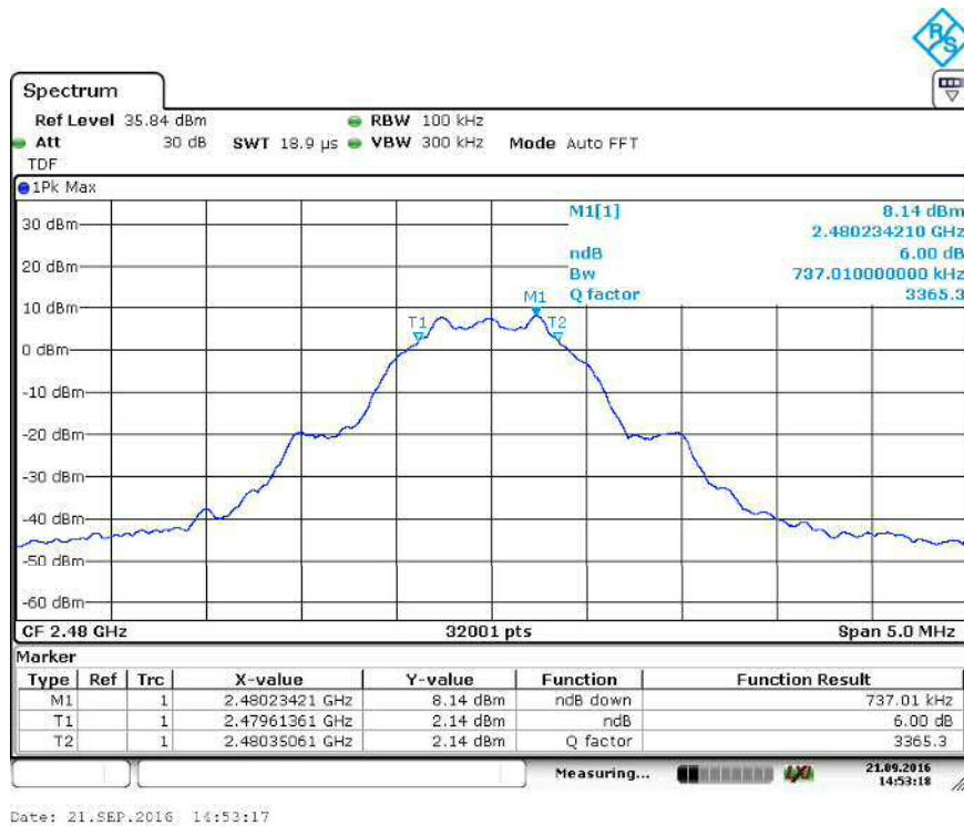
Figure 19: 6 dB bandwidth channel high
