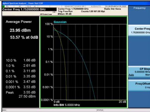
Channel 1513 / 1752.6 MHz
