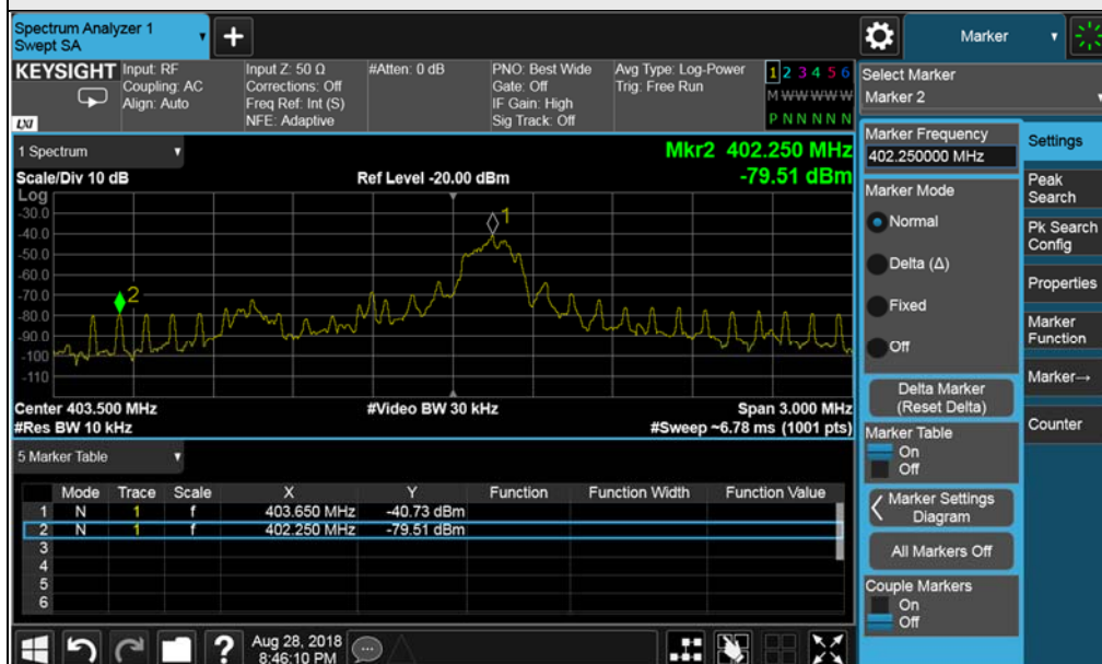
Interferer level on fc= -3dB below the calculated access threshold
