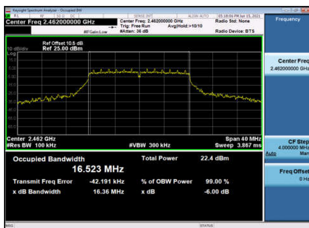
6dB Bandwidth-802.11g,2462MHz
