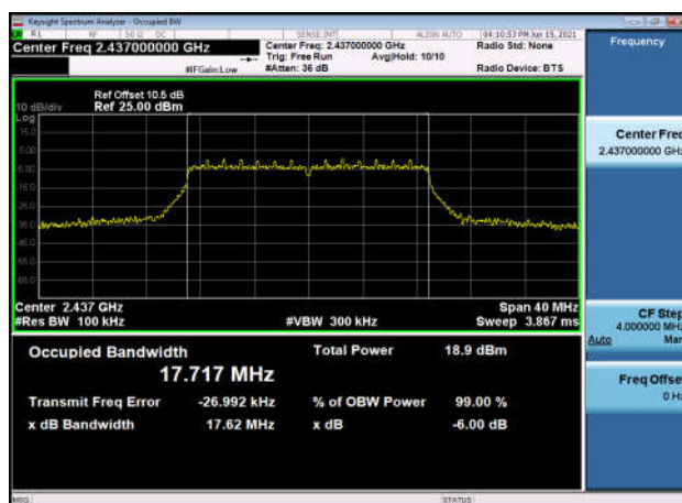
6dB Bandwidth-802.11n(HT20),2437MHz
