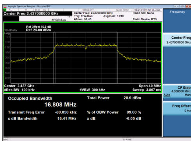
6dB Bandwidth-802.11g,2437MHz
