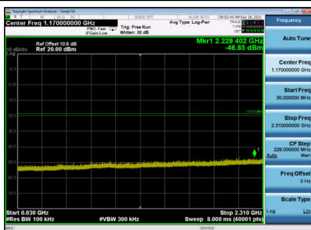
,Plot 3,30MHz~2310MHz-802.11g,2462MHz
