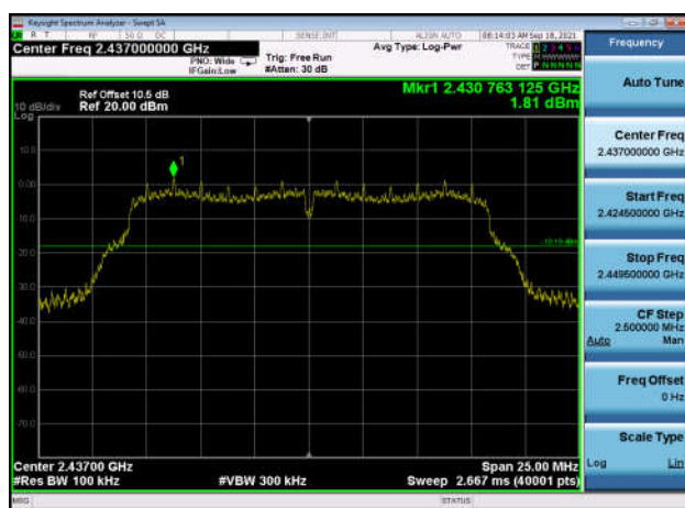
,Plot 1,Reference Level-802.11g ,2437MHz,Ant0
