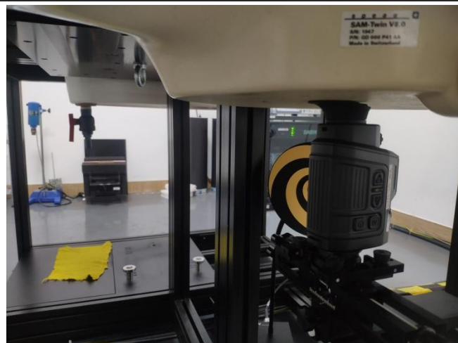
Front (0mm)
