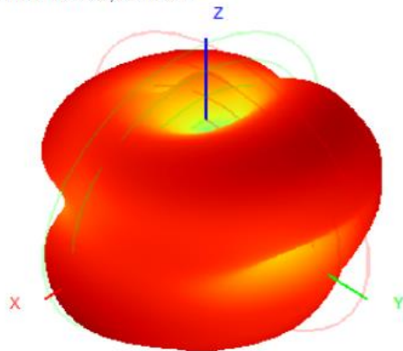
2400.0MHz H+V, Eff 62.3%
