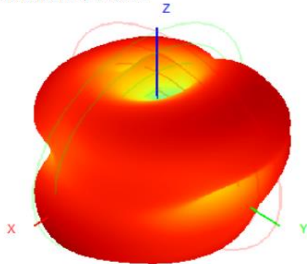
2410.0MHz H+V, Eff 61.0%
