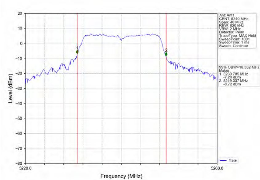
802.11a_HCH_5240MHz_Ant1_NTNV
