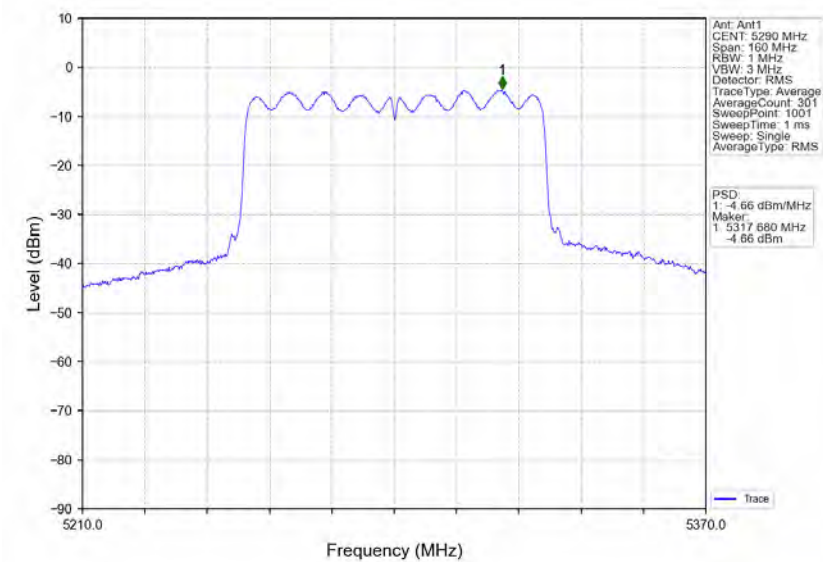
802.11ac(VHT80)_MCH_5290MHz_Ant1_NTNV
