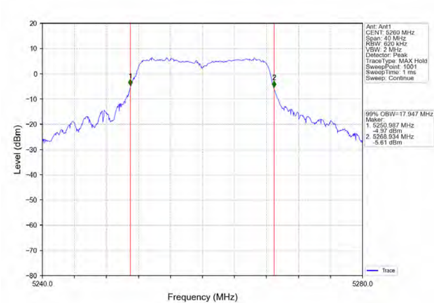
802.11a_LCH_5260MHz_Ant1_NTNV
