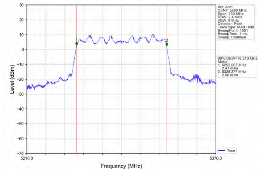
802.11ac(VHT80)_MCH_5290MHz_Ant1_NTNV
