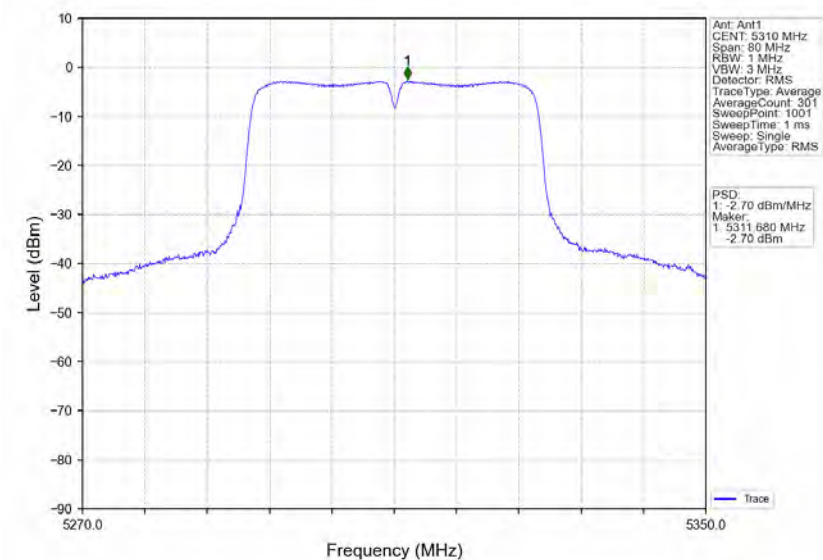
802.11ac(VHT40)_HCH_5310MHz_Ant1_NTNV
