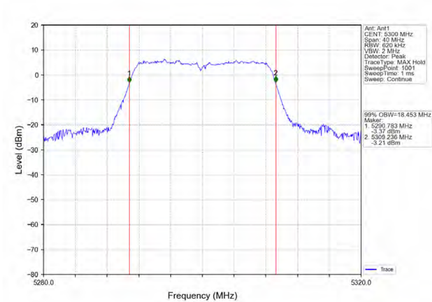
802.11n(HT20)_MCH_5300MHz_Ant1_NTNV
