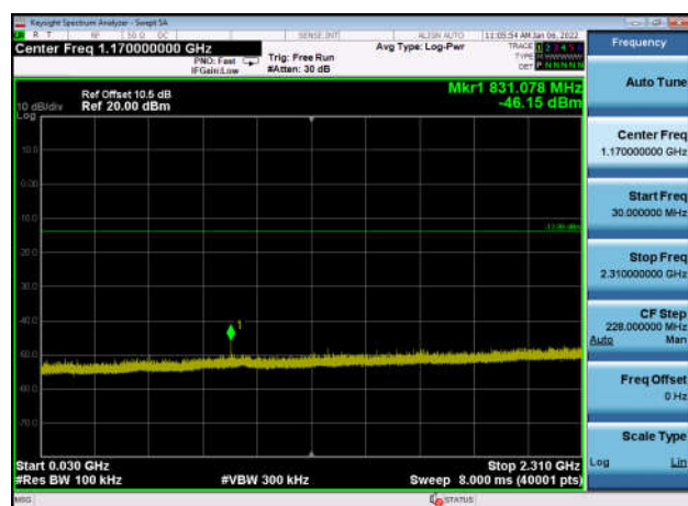
,Plot 3,30MHz~2310MHz-802.11g,2462MHz
