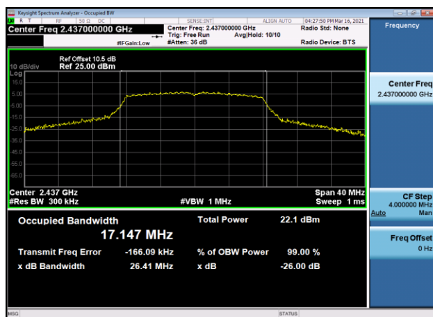
99% Bandwidth-802.11g,2437MHz
