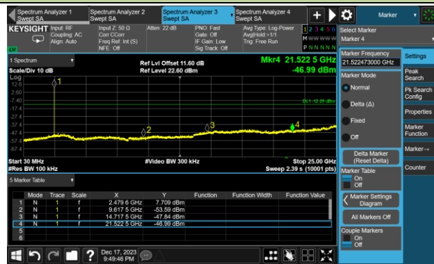
Channel 78 (2480MHz)
