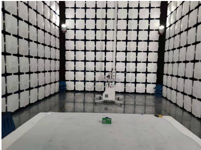
30MHZ- 1GHz for radiated emission test setup
