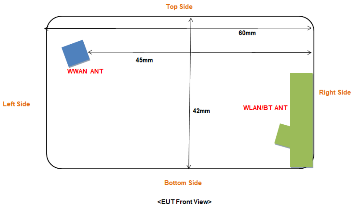
Block Diagram for EUT Antenna Position
