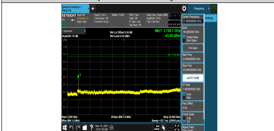
Band2-1.4MHz-QPSK-18900-1RB#0-Range5:2000~20000MHz
