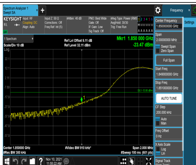
Band2-15MHz-16QAM-18675-1RB#0
