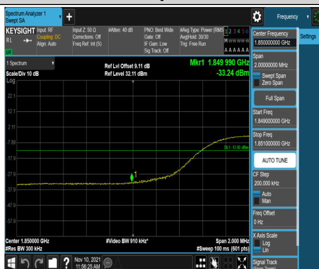
Band2-15MHz-16QAM-18675-75RB#0
