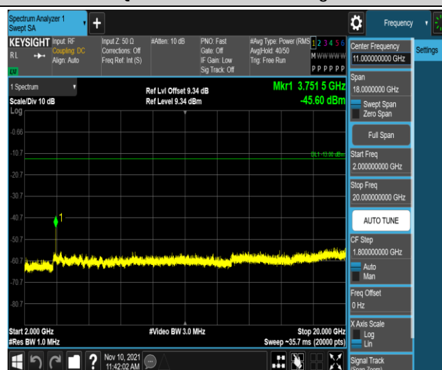
Band2-10MHz-16QAM-18900-1RB#0-Range5:2000~20000MHz
