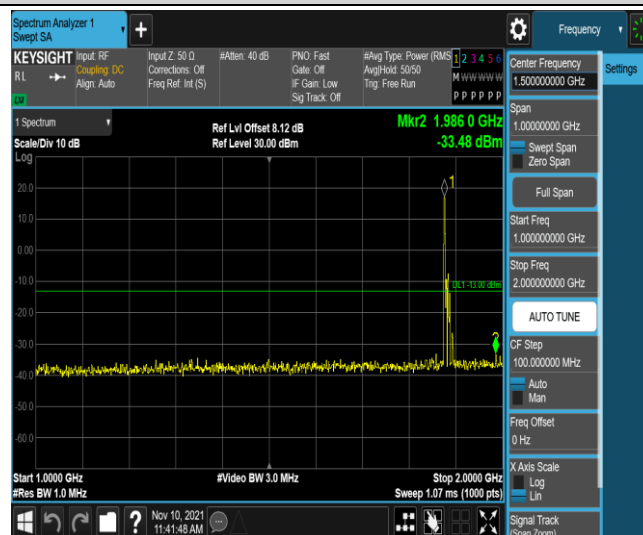
Band2-10MHz-16QAM-18900-1RB#0-Range4:1000~2000MHz
