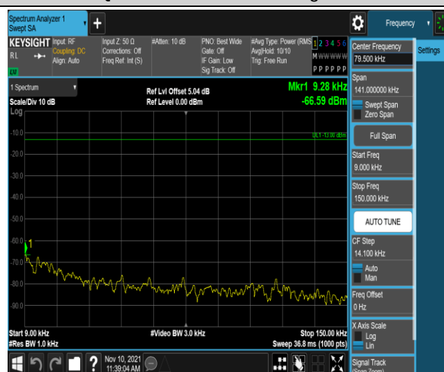
Band2-10MHz-16QAM-18650-1RB#0-Range1:0.009~0.15MHz
