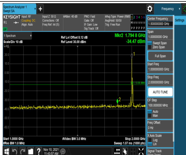
Band2-10MHz-16QAM-19150-1RB#0-Range4:1000~2000MHz
