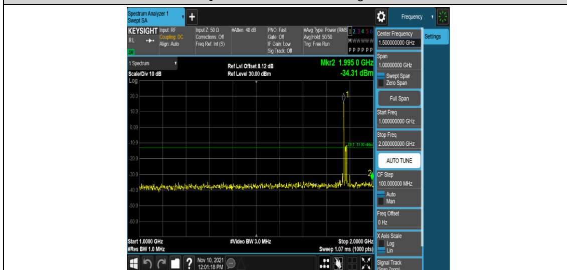
Band2-15MHz-QPSK-18900-1RB#0-Range4:1000~2000MHz
