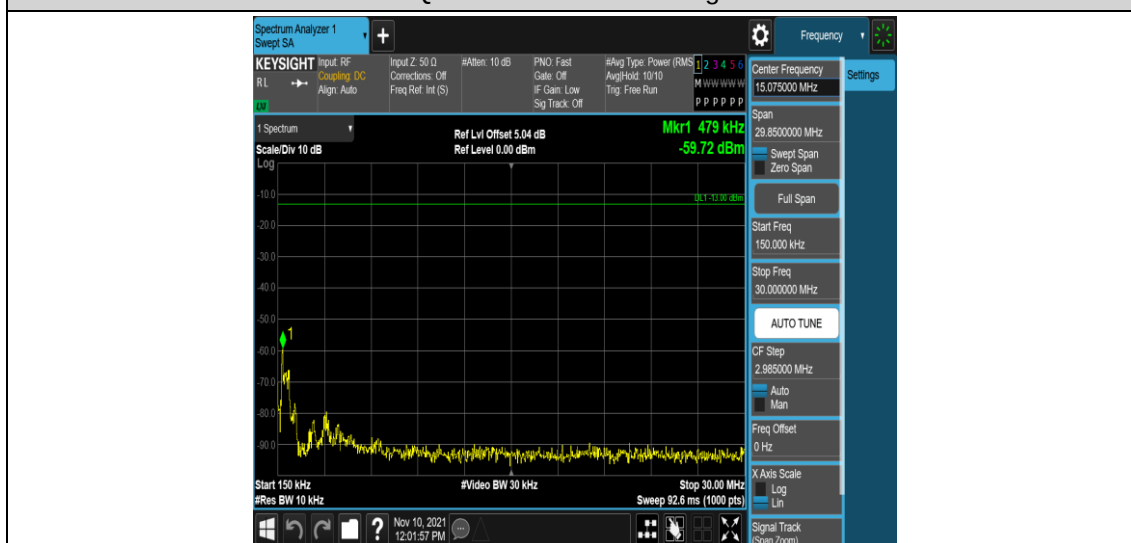
Band2-15MHz-16QAM-18900-1RB#0-Range2:0.15~30MHz
