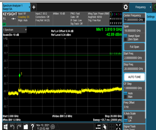
Band2-5MHz-16QAM-19175-1RB#0-Range5:2000~20000MHz
