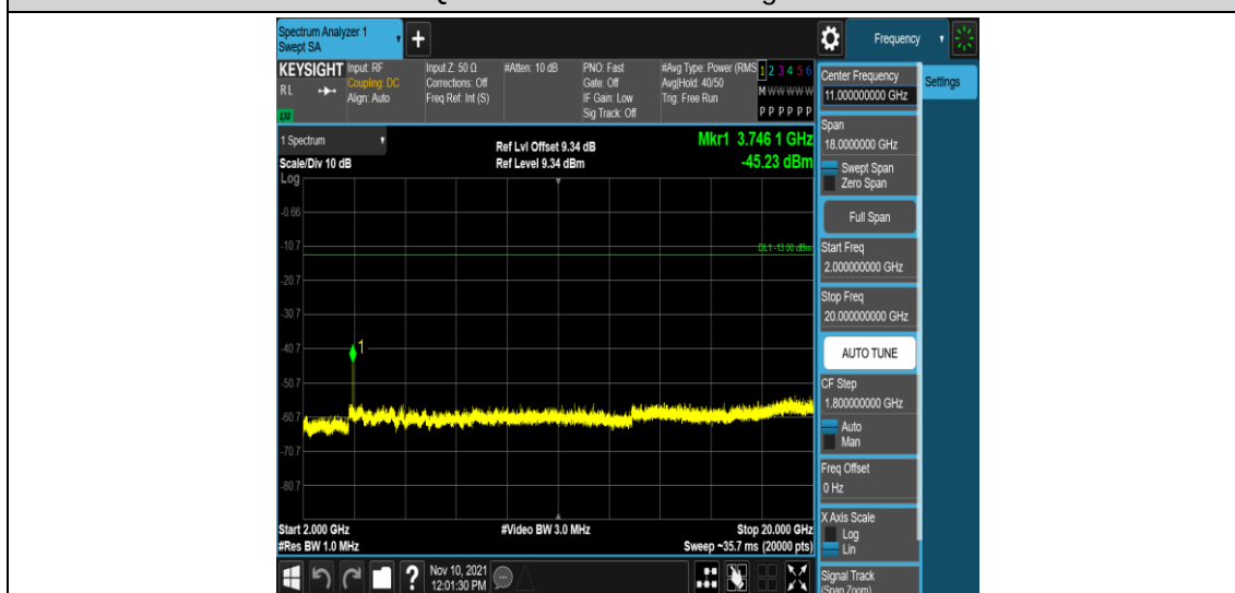
Band2-15MHz-QPSK-18900-1RB#0-Range5:2000~20000MHz
