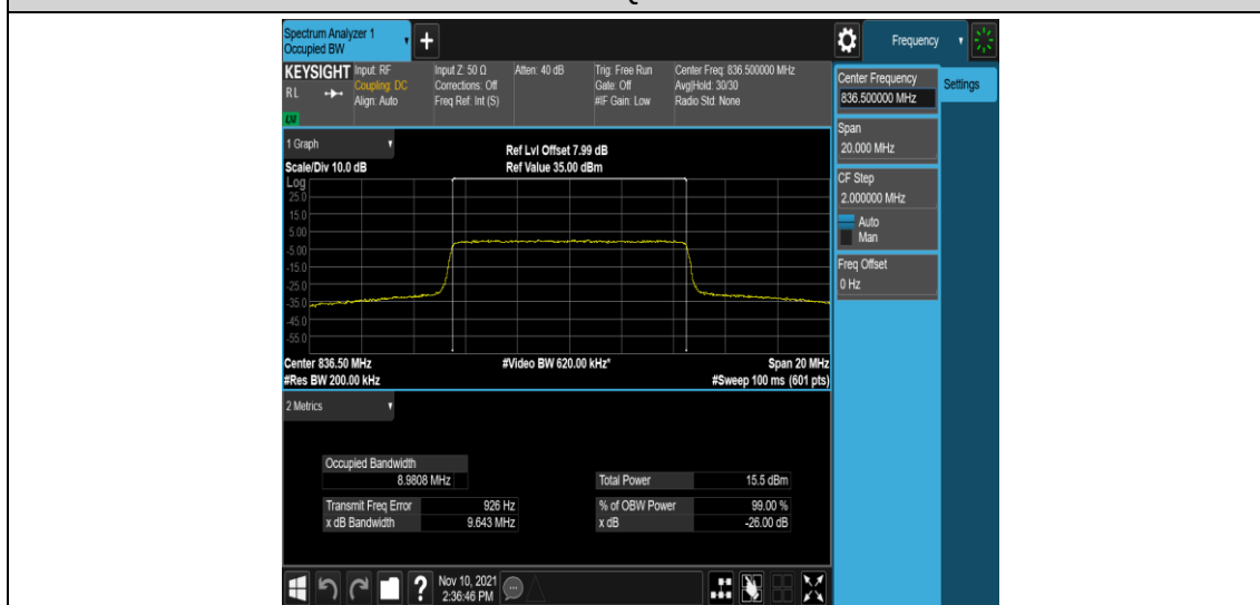
Band5-10MHz-16QAM-20525-50RB#0
