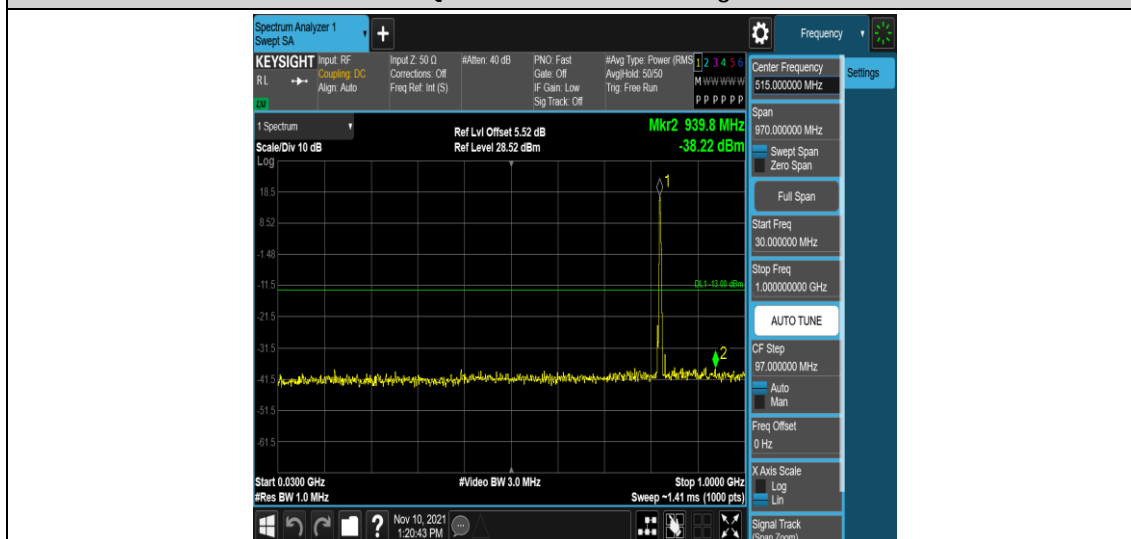
Band5-3MHz-16QAM-20415-1RB#0-Range3:30~1000MHz
