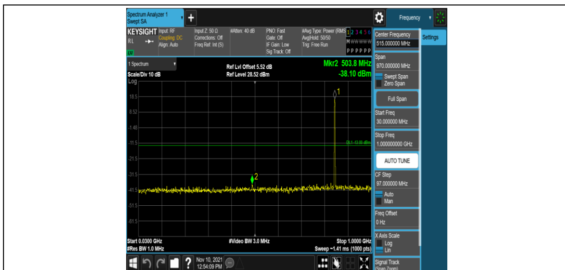
Band5-1.4MHz-16QAM-20643-1RB#0-Range3:30~1000MHz
