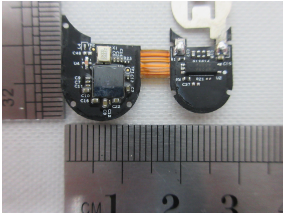
Main board_Rear
