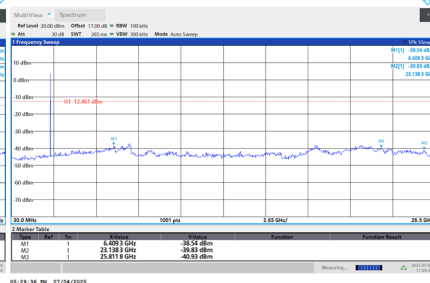
Harmonic-CH39
