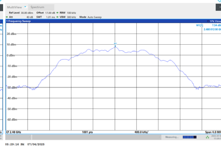
Bandedge-CH39
