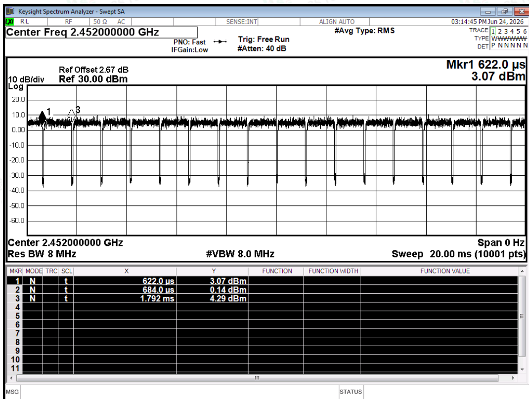
Duty Cycle NVNT n40 2452MHz Ant1
