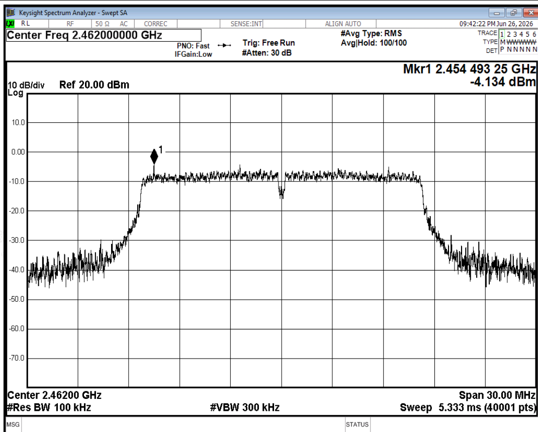
Tx. Spurious NVNT g 2462MHz Ant2 Ref
