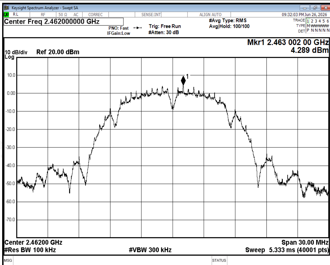
Tx. Spurious NVNT b 2462MHz Ant2 Ref
