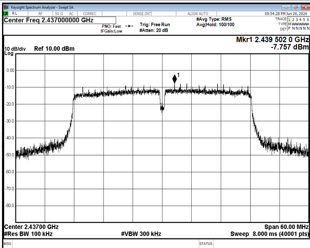
Tx. Spurious NVNT n40 2437MHz Ant2 Ref
