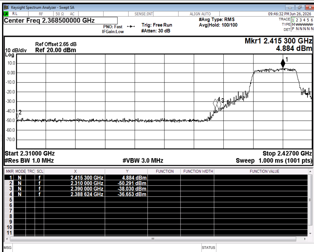
Restrict Band NVNT n20 2412MHz Ant2 Peak
