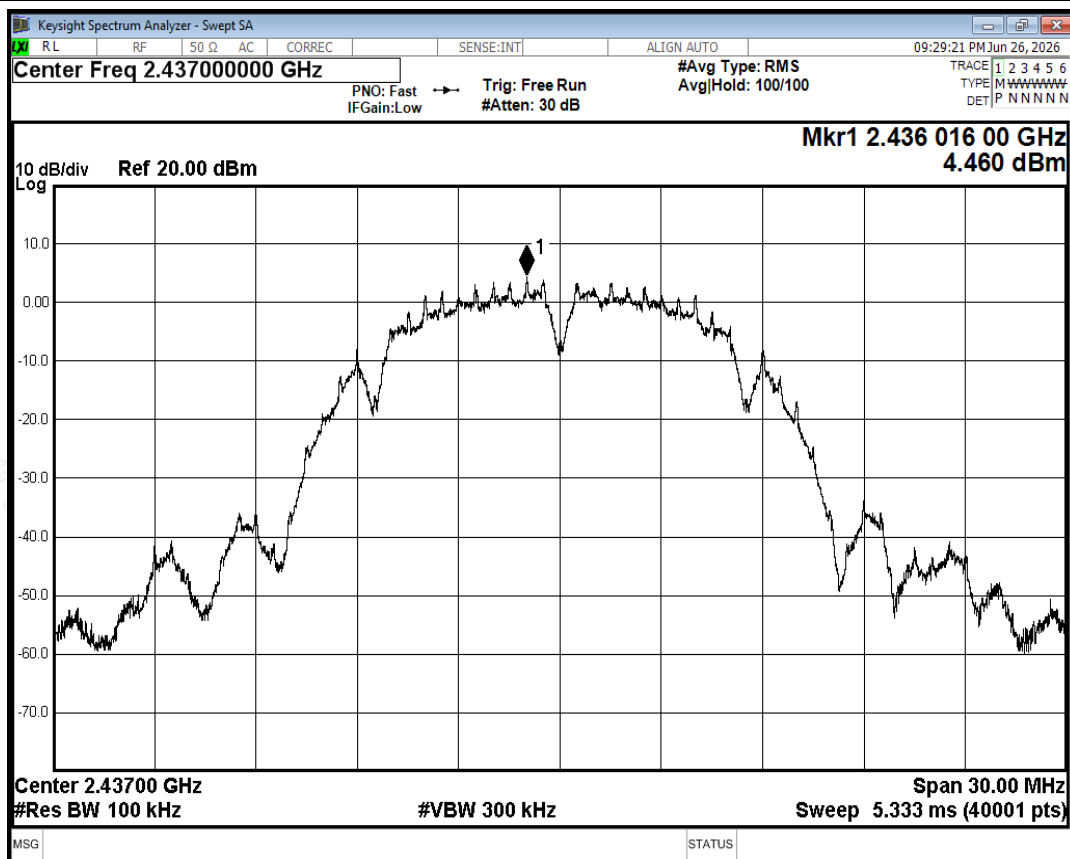
Tx. Spurious NVNT b 2437MHz Ant2 Ref
