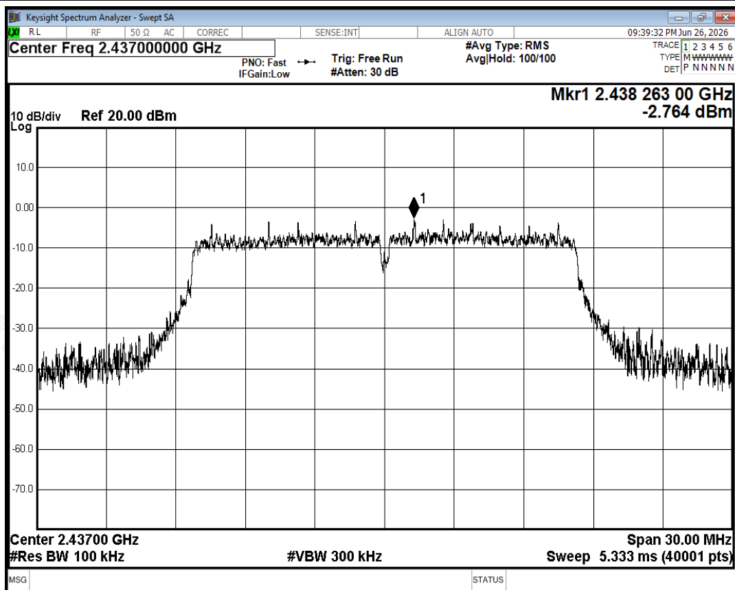
Tx. Spurious NVNT g 2437MHz Ant2 Ref
