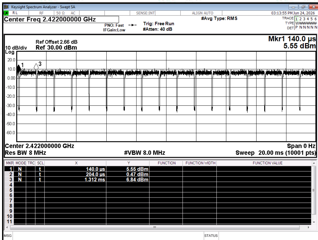
Duty Cycle NVNT n40 2422MHz Ant1
