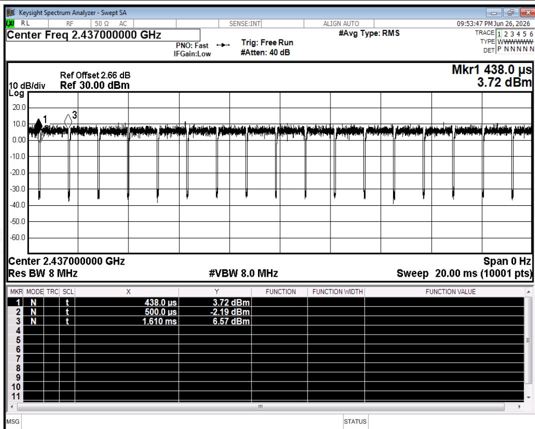
Duty Cycle NVNT n40 2437MHz Ant2
