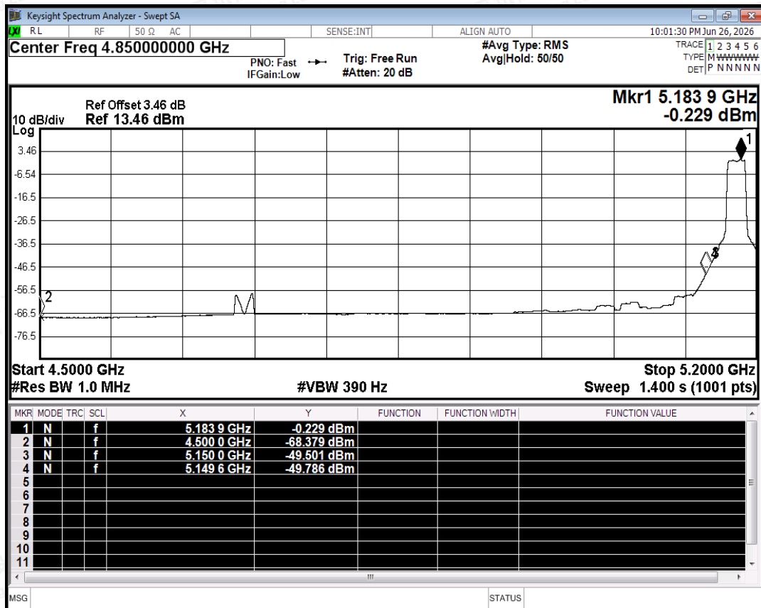
Restrict Band NVNT a 5180MHz Ant2 Average
