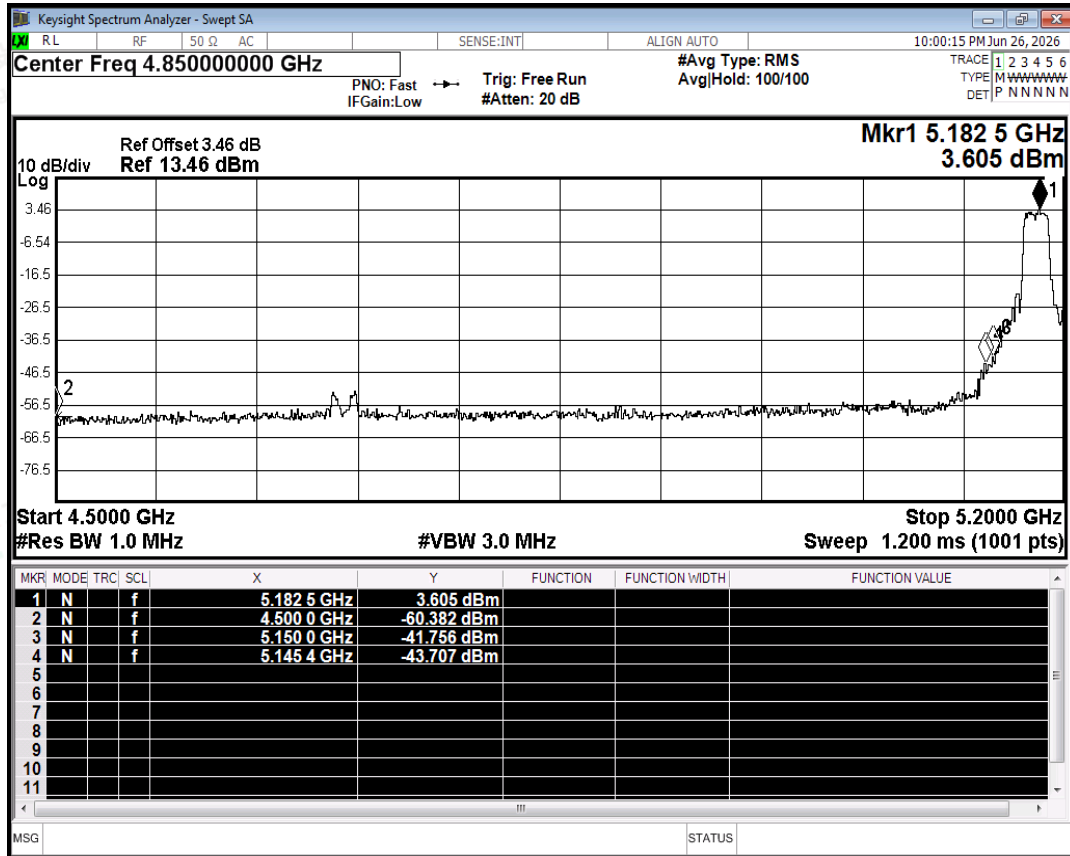
Restrict Band NVNT a 5180MHz Ant2 Peak
