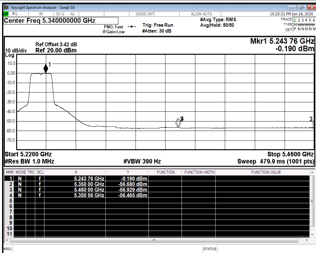
Restrict Band NVNT a 5240MHz Ant2 Average
