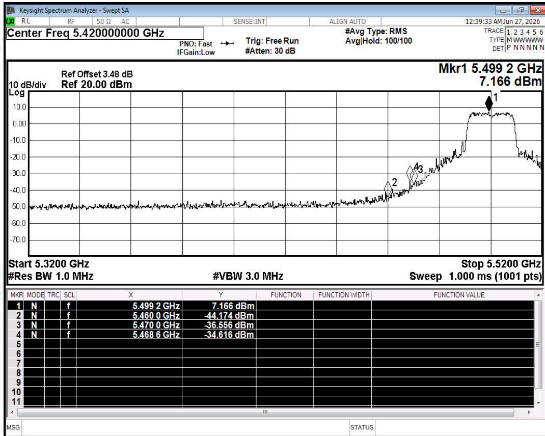
Restrict Band NVNT ac20 5500MHz Ant2 Peak
