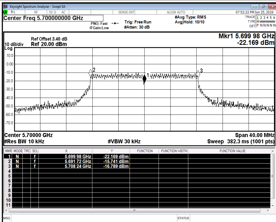
Freq. Stability NVNT a 5700MHz Ant1
