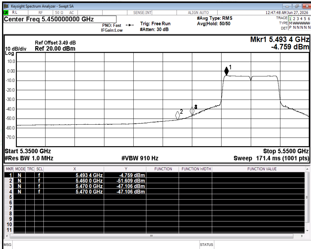
Restrict Band NVNT n40 5510MHz Ant2 Average
