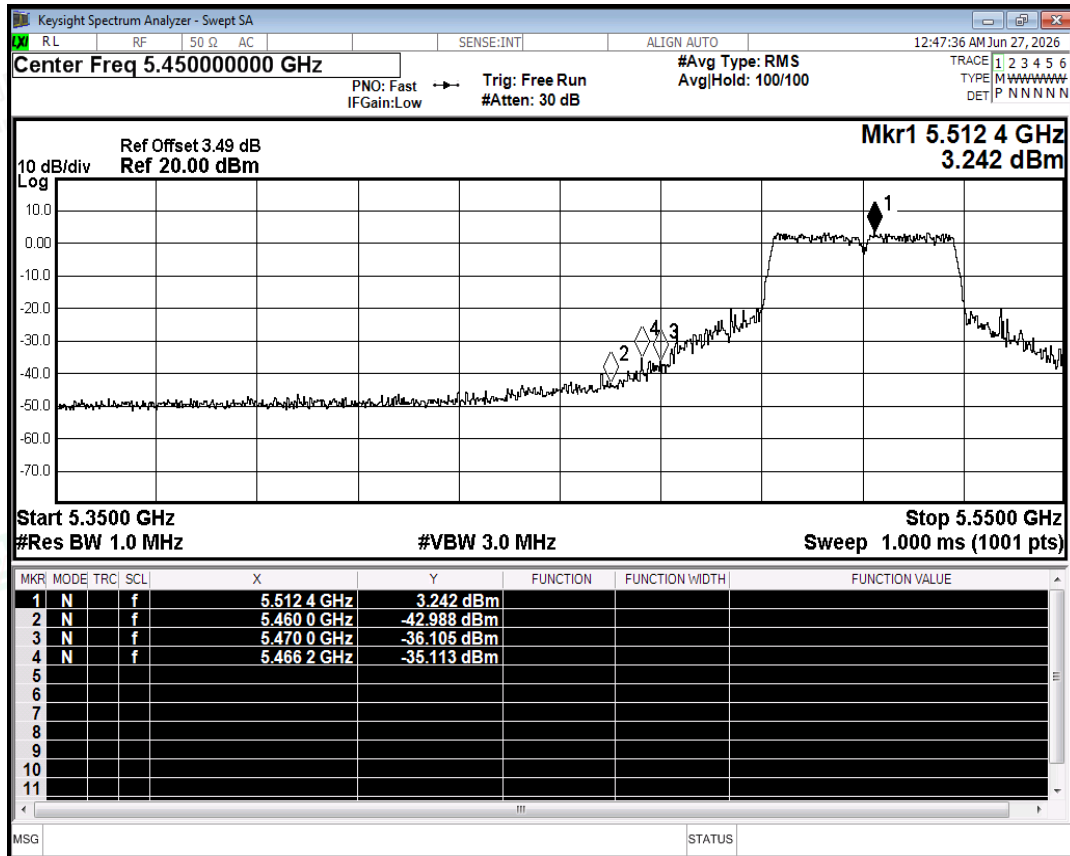
Restrict Band NVNT n40 5510MHz Ant2 Peak
