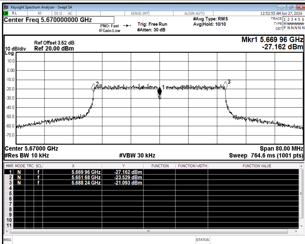
Freq. Stability NVNT n40 5670MHz Ant2
