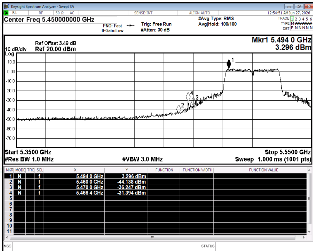
Restrict Band NVNT ac40 5510MHz Ant2 Peak
