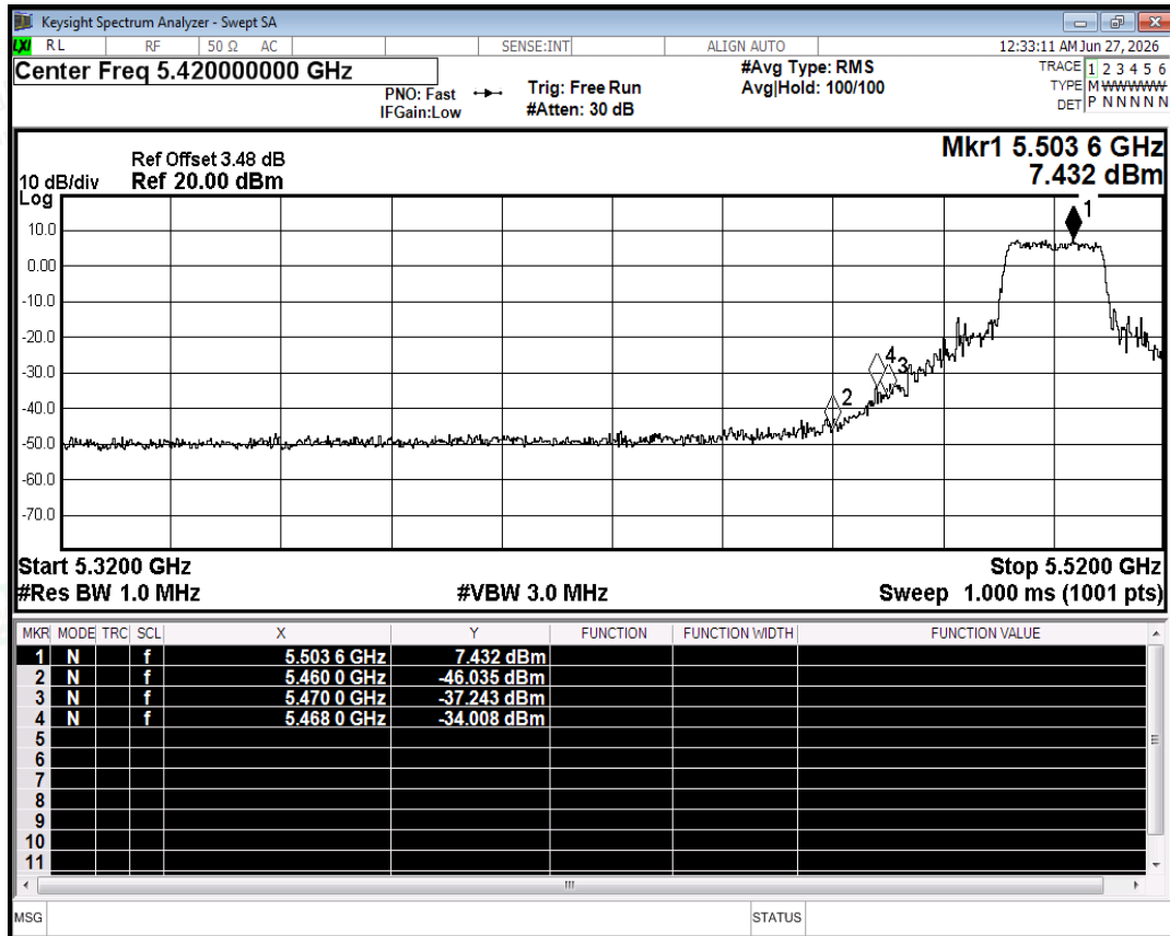
Restrict Band NVNT n20 5500MHz Ant2 Peak
