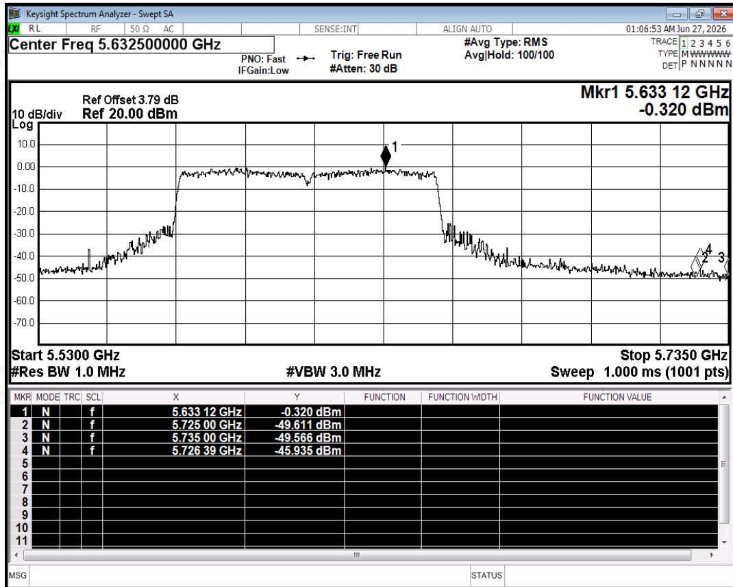
Restrict Band NVNT ac80 5610MHz Ant2 Peak
