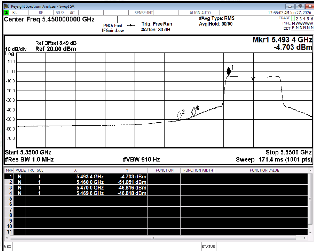
Restrict Band NVNT ac40 5510MHz Ant2 Average
