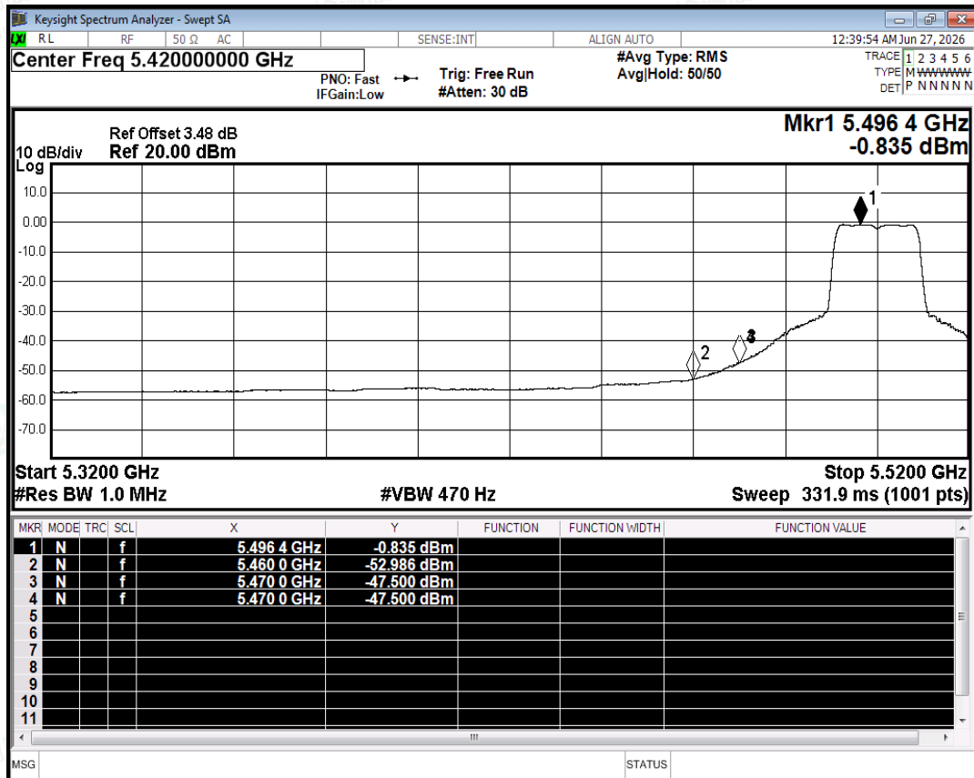
Restrict Band NVNT ac20 5500MHz Ant2 Average
