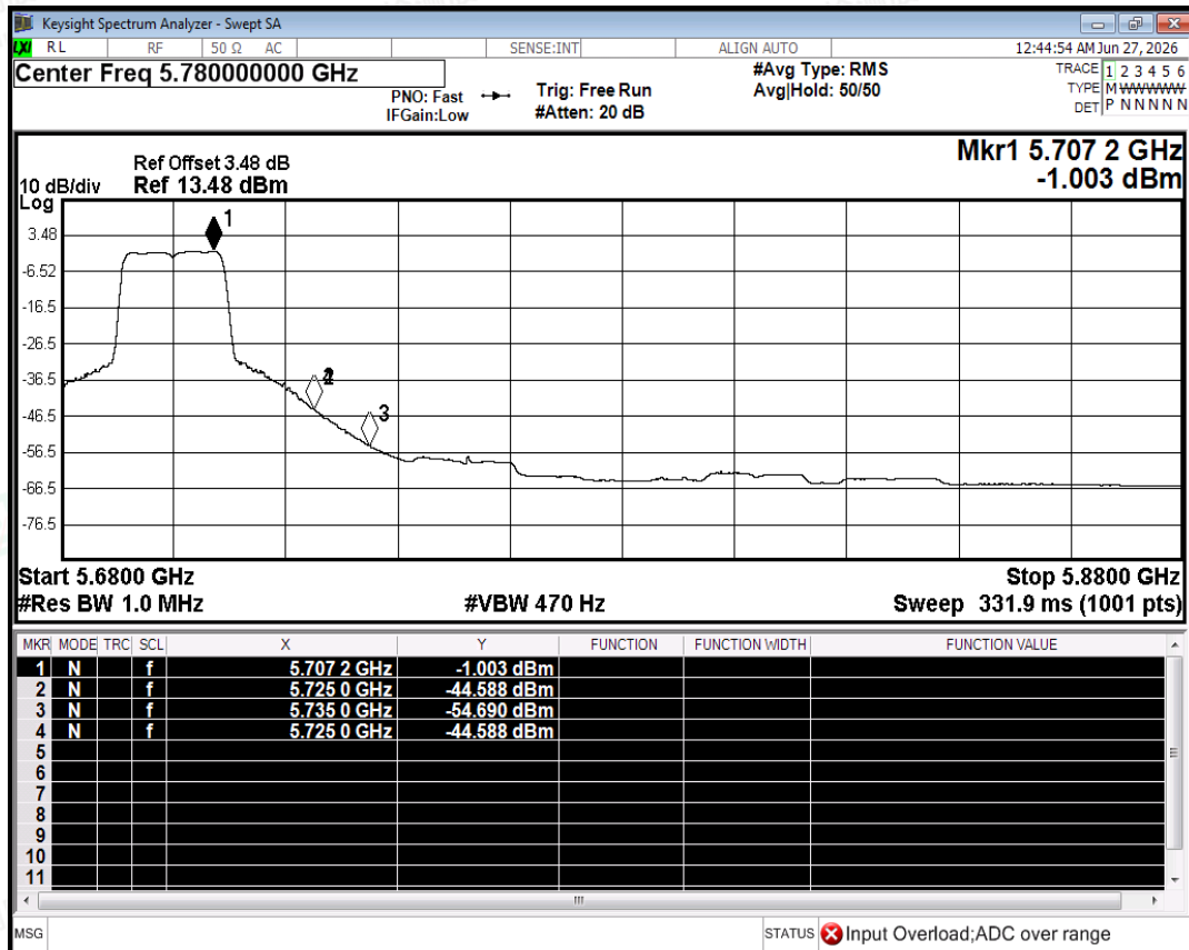
Restrict Band NVNT ac20 5700MHz Ant2 Average
