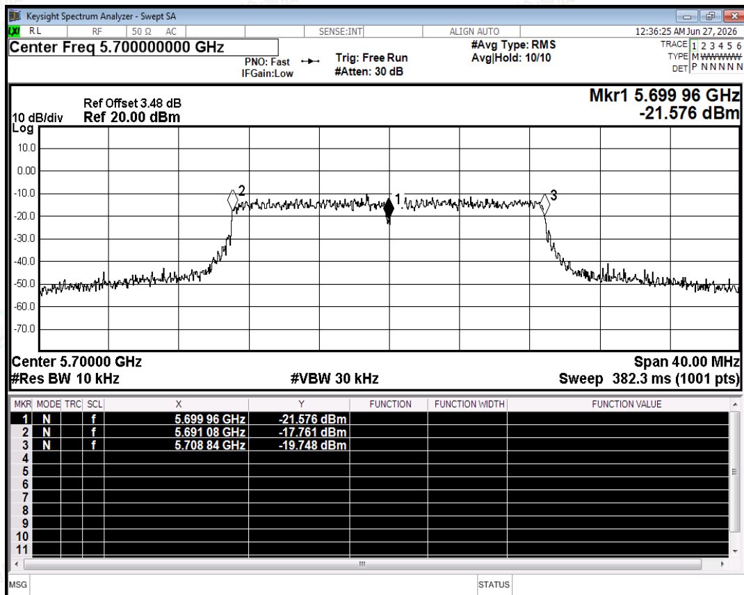
Freq. Stability NVNT n20 5700MHz Ant2
