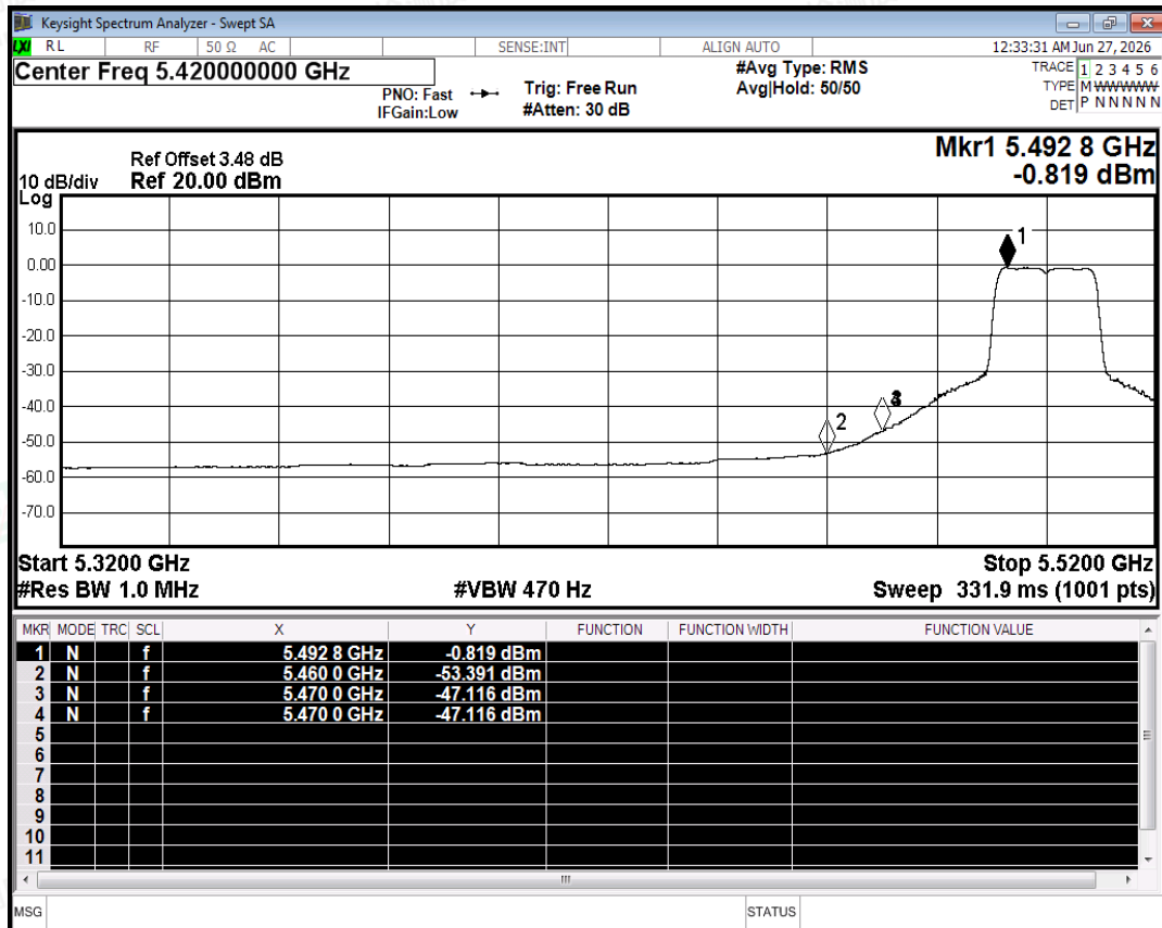
Restrict Band NVNT n20 5500MHz Ant2 Average
