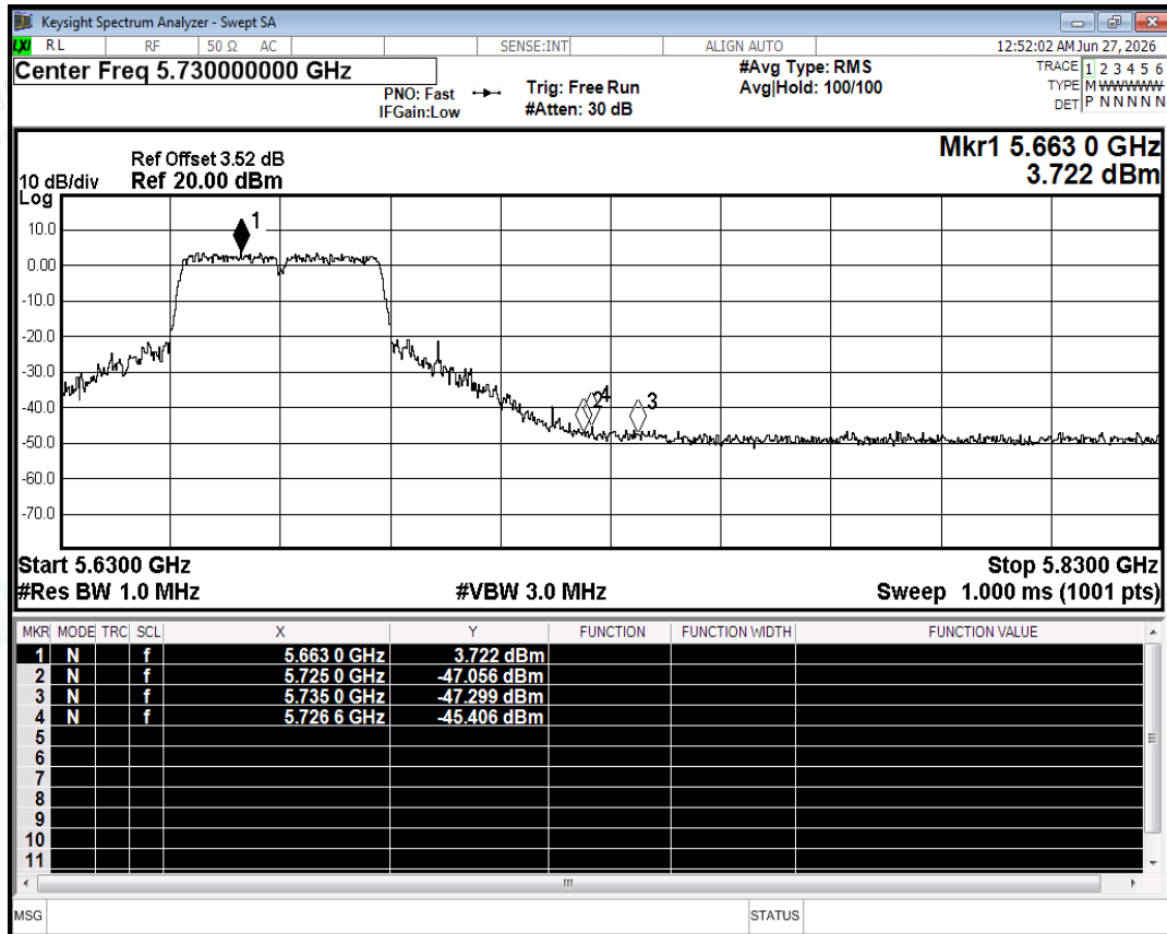
Restrict Band NVNT n40 5670MHz Ant2 Peak
