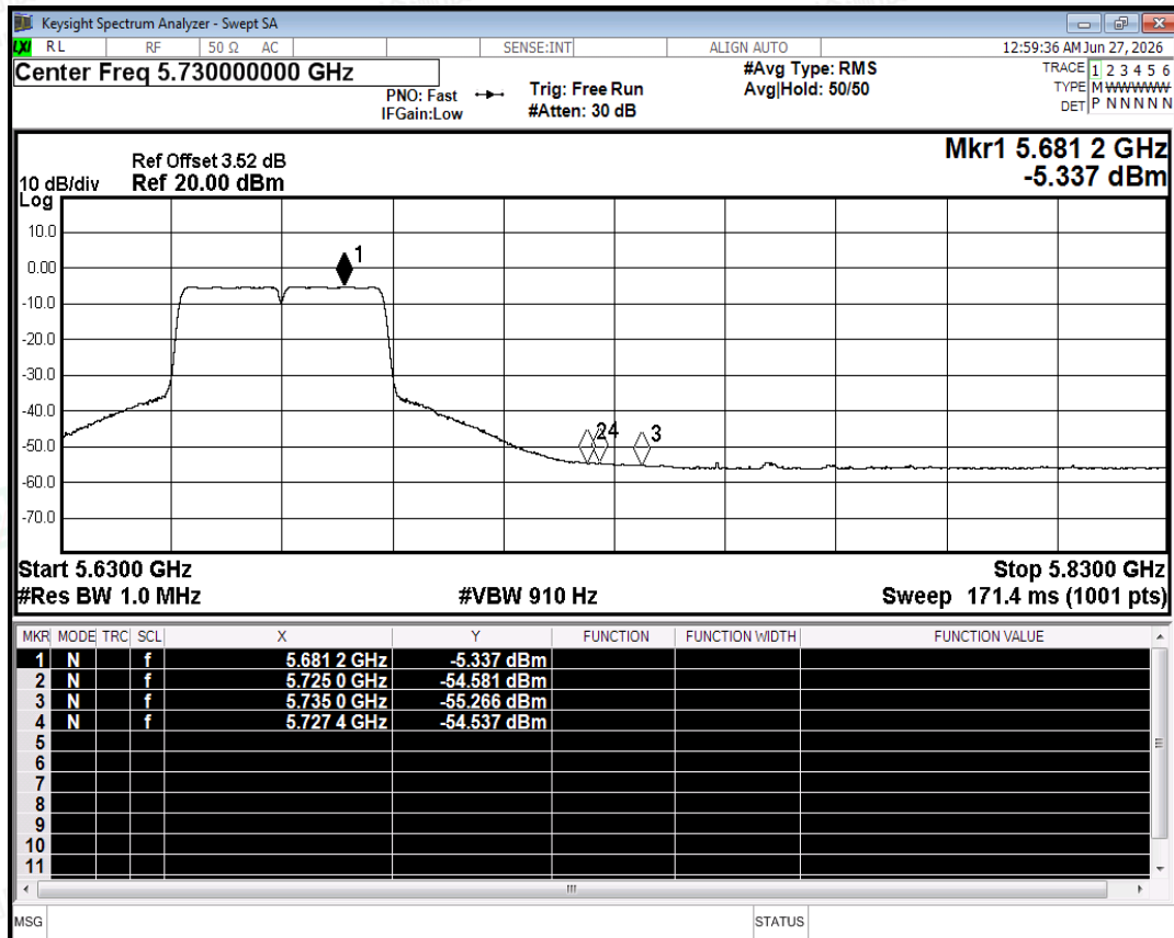
Restrict Band NVNT ac40 5670MHz Ant2 Average
