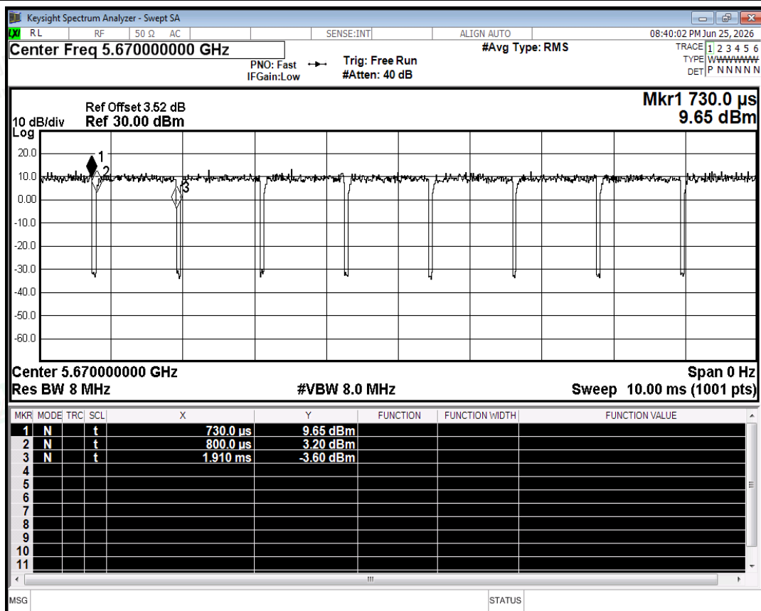
Duty Cycle NVNT n40 5670MHz Ant1
