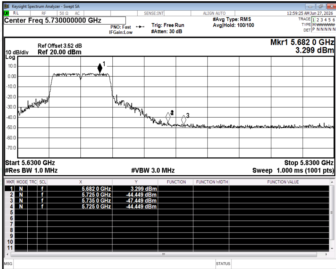
Restrict Band NVNT ac40 5670MHz Ant2 Peak
