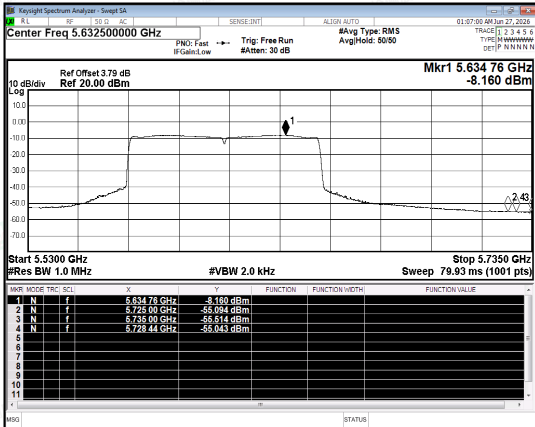
Restrict Band NVNT ac80 5610MHz Ant2 Average
