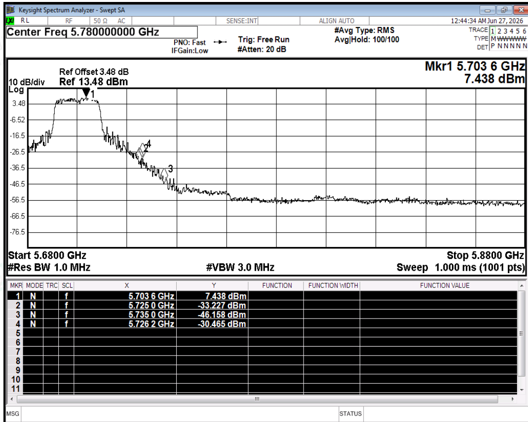
Restrict Band NVNT ac20 5700MHz Ant2 Peak
