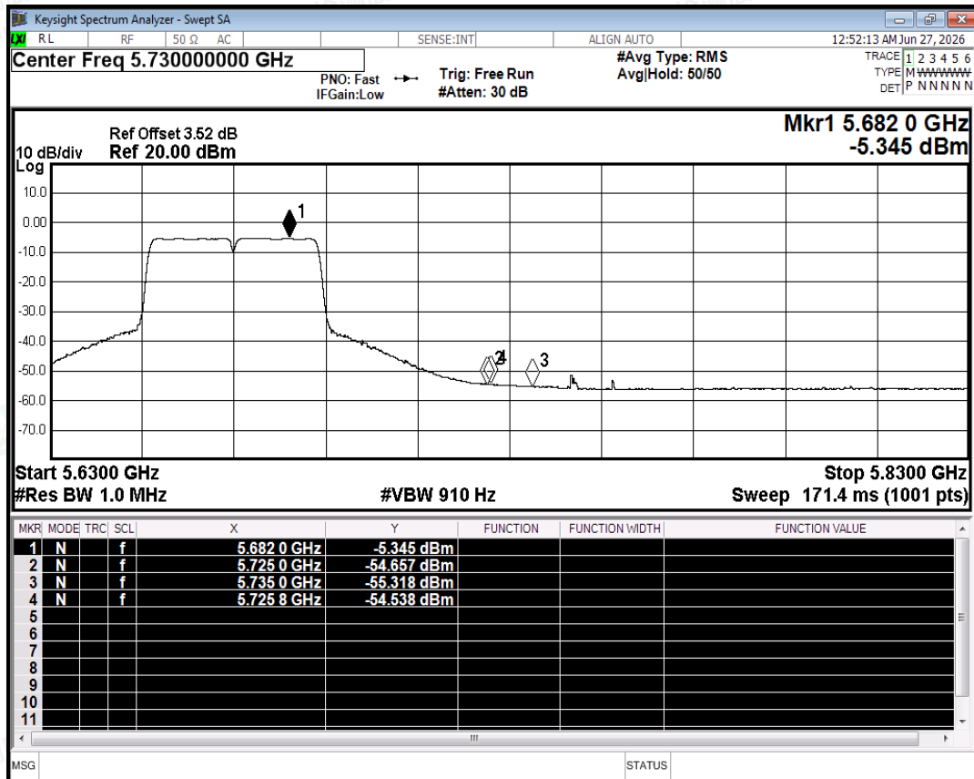
Restrict Band NVNT n40 5670MHz Ant2 Average
