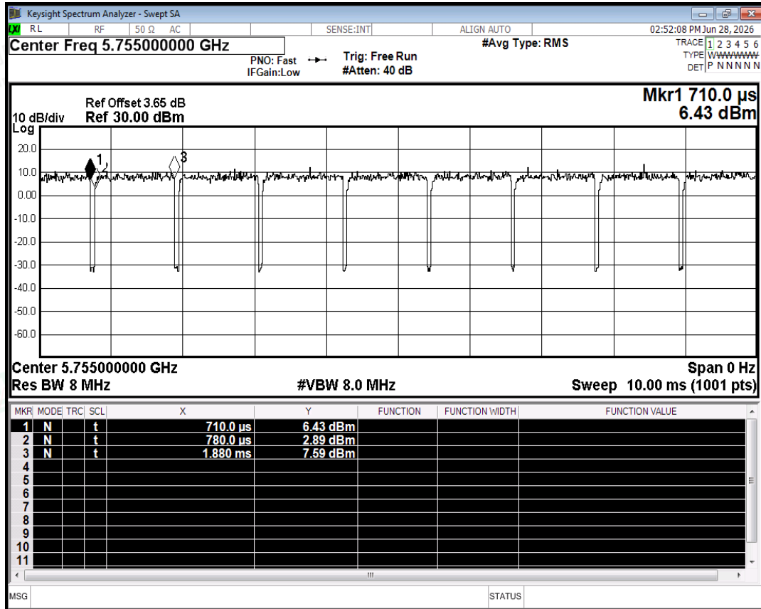
Duty Cycle NVNT n40 5755MHz Ant2
