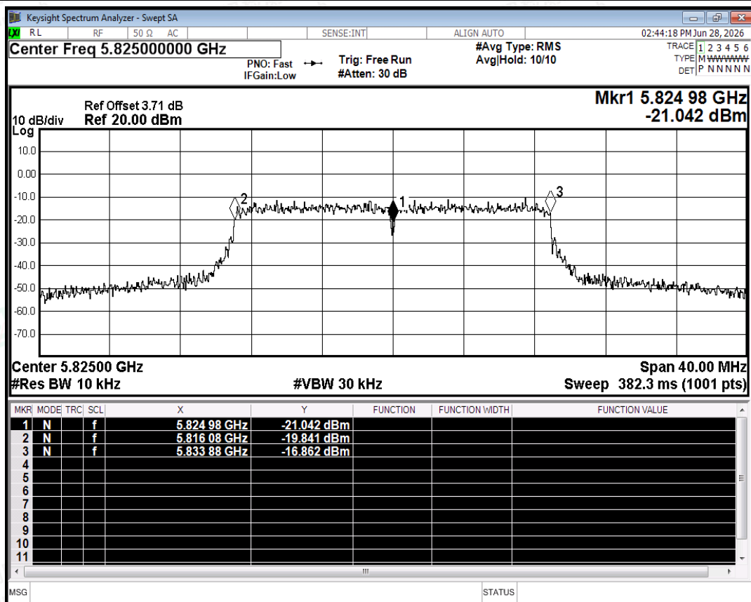
Freq. Stability NVNT n20 5825MHz Ant2
