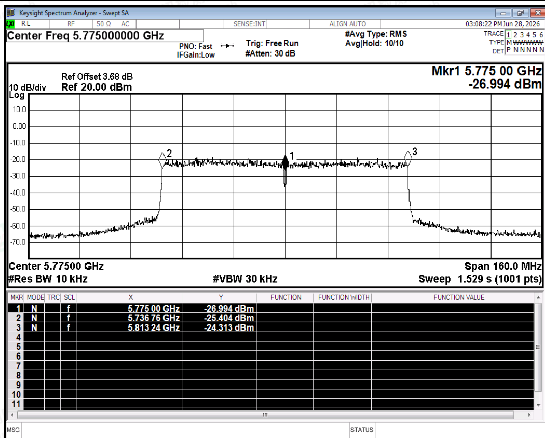
Freq. Stability NVNT ac80 5775MHz Ant2
