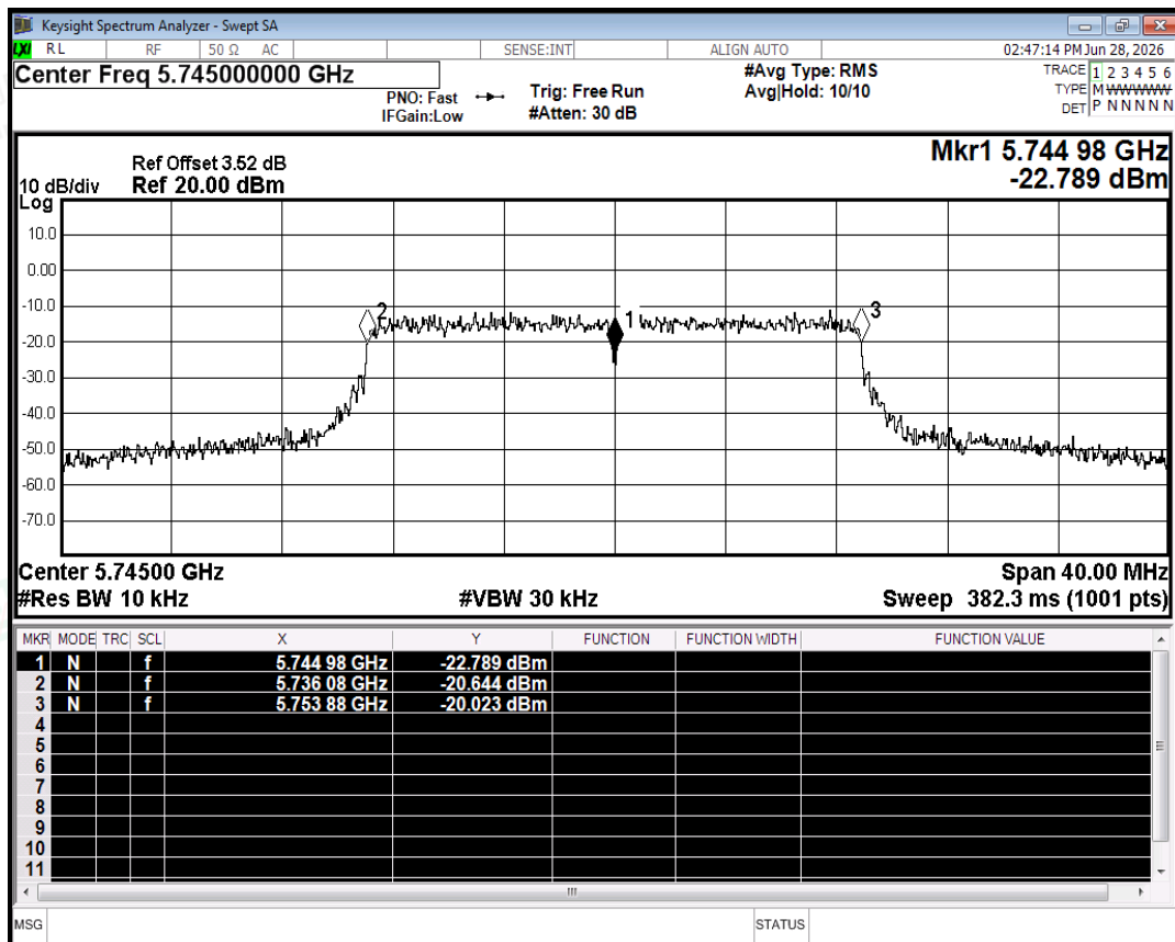
Freq. Stability NVNT ac20 5745MHz Ant2
