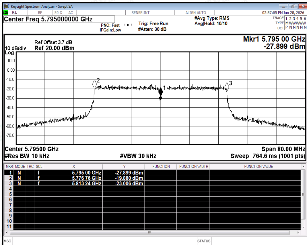
Freq. Stability NVNT n40 5795MHz Ant2
