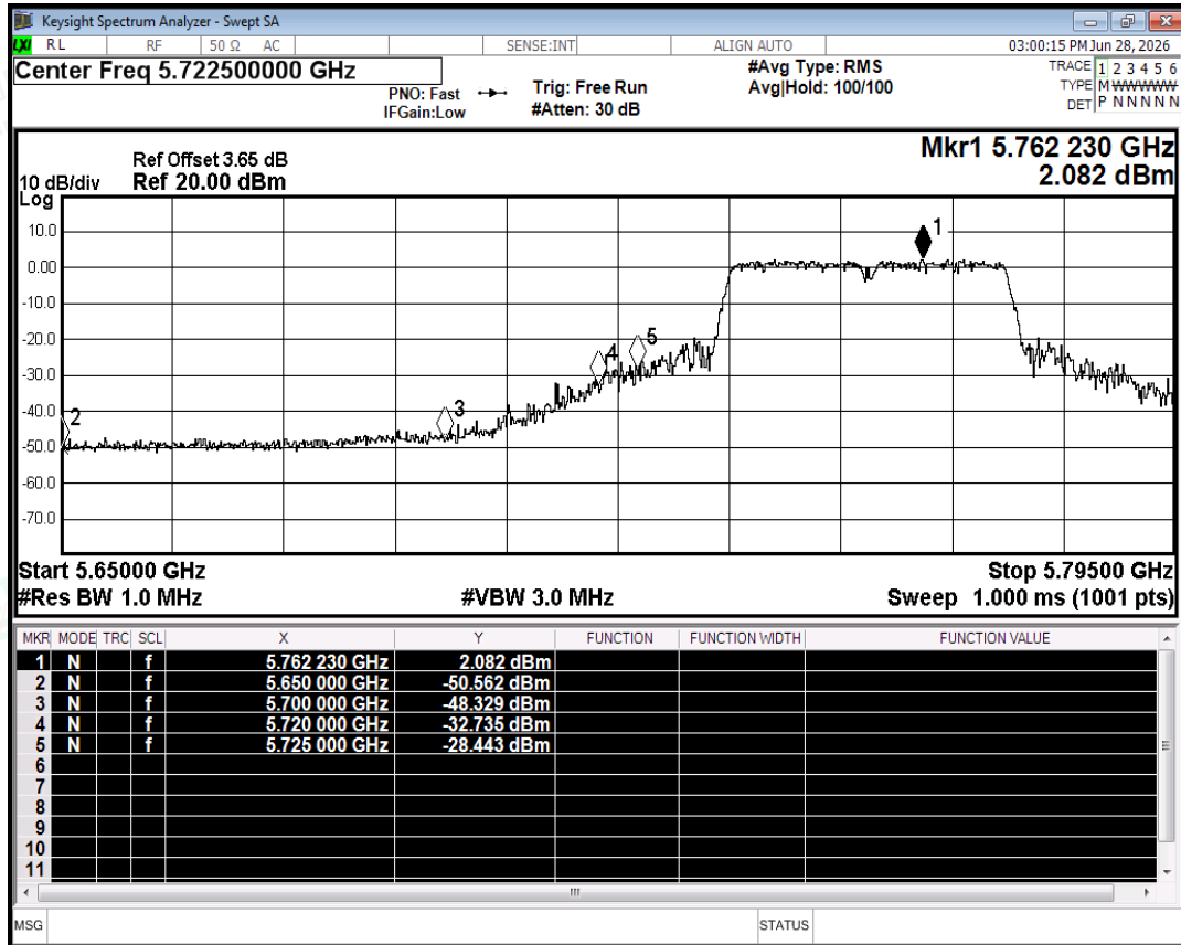
Restrict Band NVNT ac40 5755MHz Ant2 Peak
