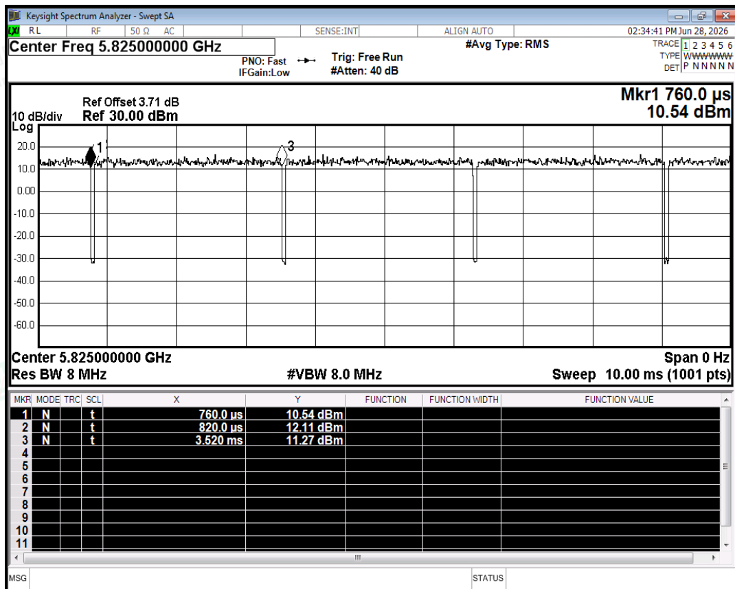
Duty Cycle NVNT a 5825MHz Ant2
