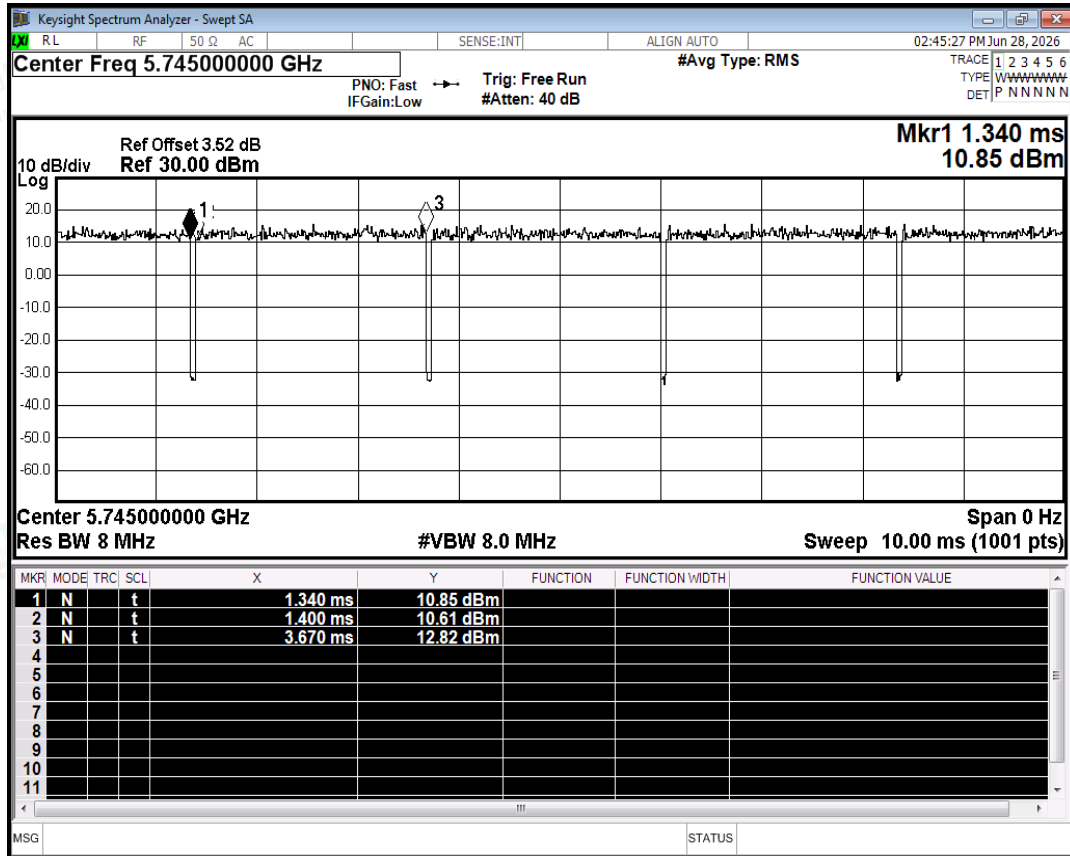
Duty Cycle NVNT ac20 5745MHz Ant2
