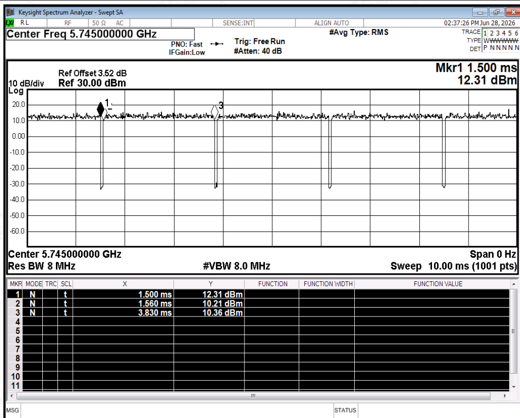
Duty Cycle NVNT n20 5745MHz Ant2
