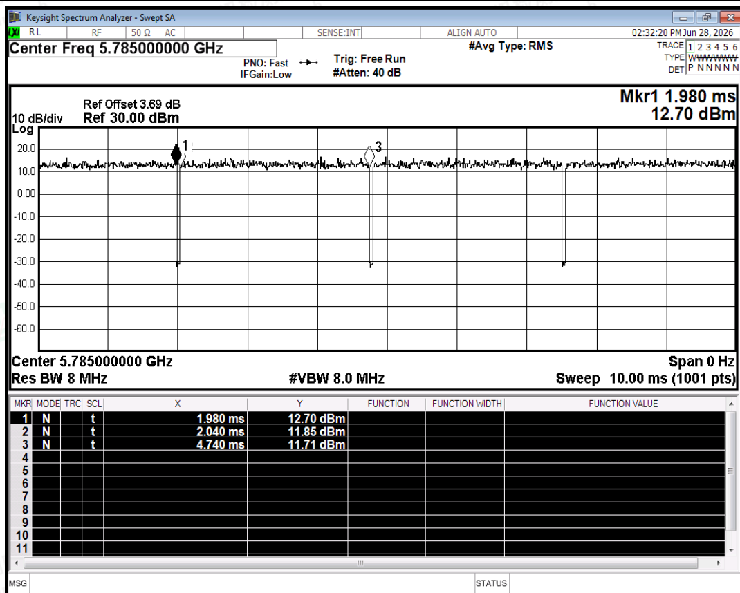
Duty Cycle NVNT a 5785MHz Ant2
