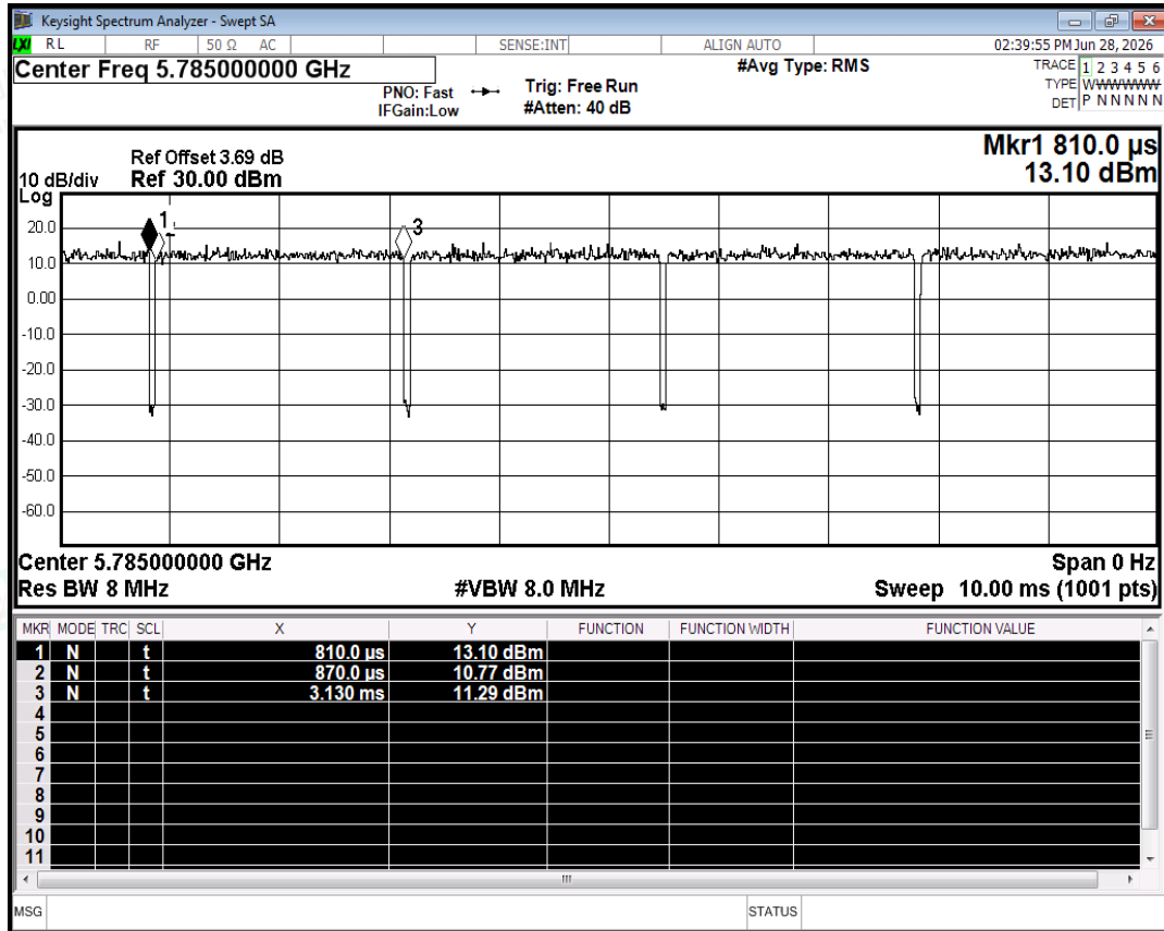
Duty Cycle NVNT n20 5785MHz Ant2
