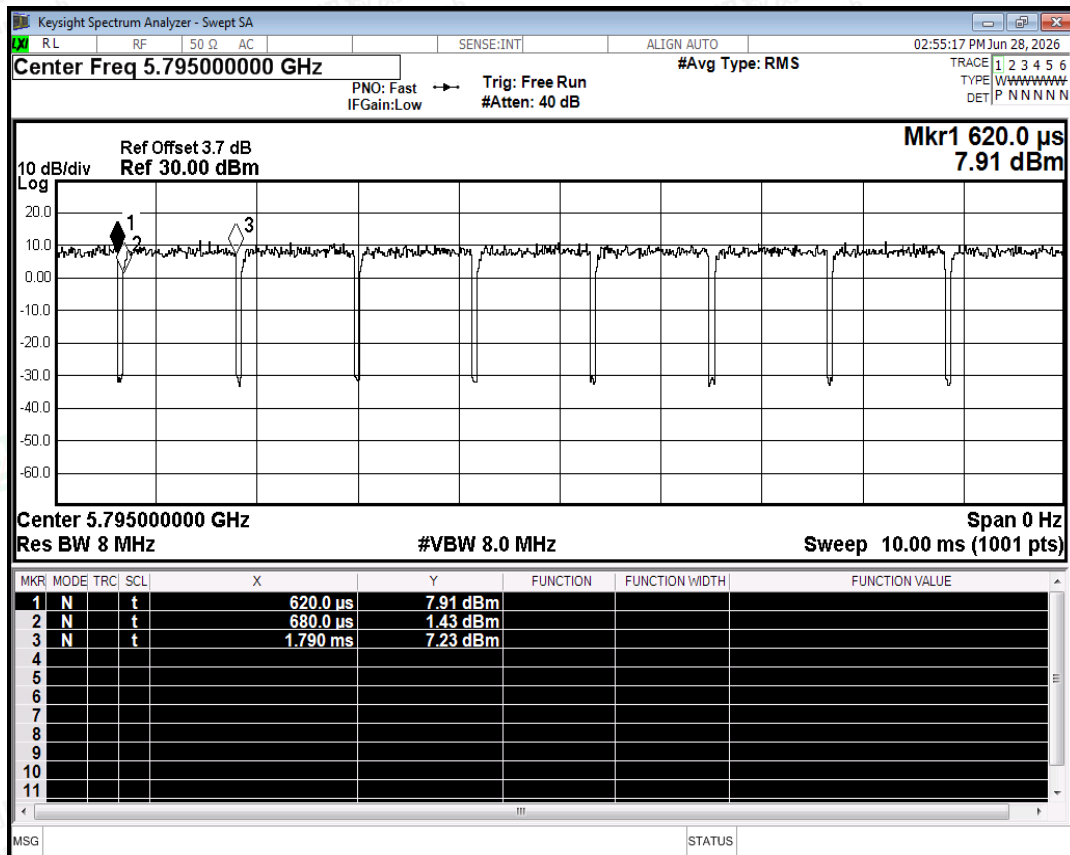
Duty Cycle NVNT n40 5795MHz Ant2
