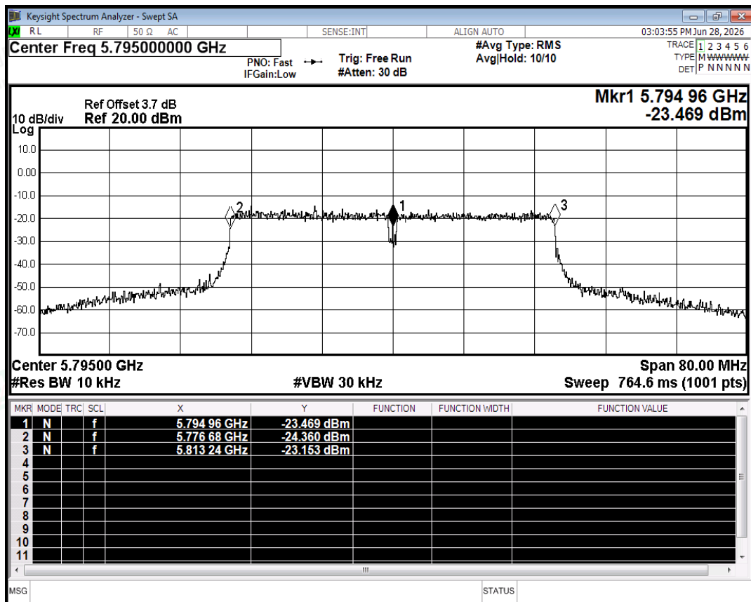
Freq. Stability NVNT ac40 5795MHz Ant2
