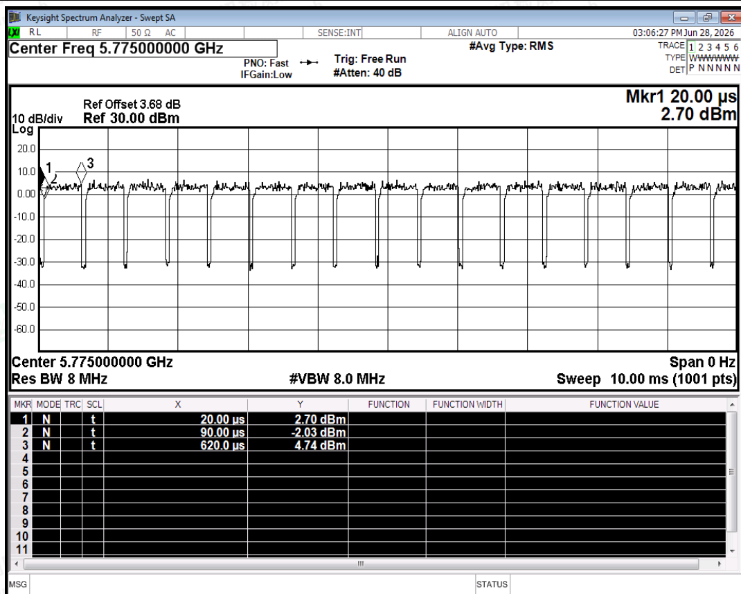
Duty Cycle NVNT ac80 5775MHz Ant2
