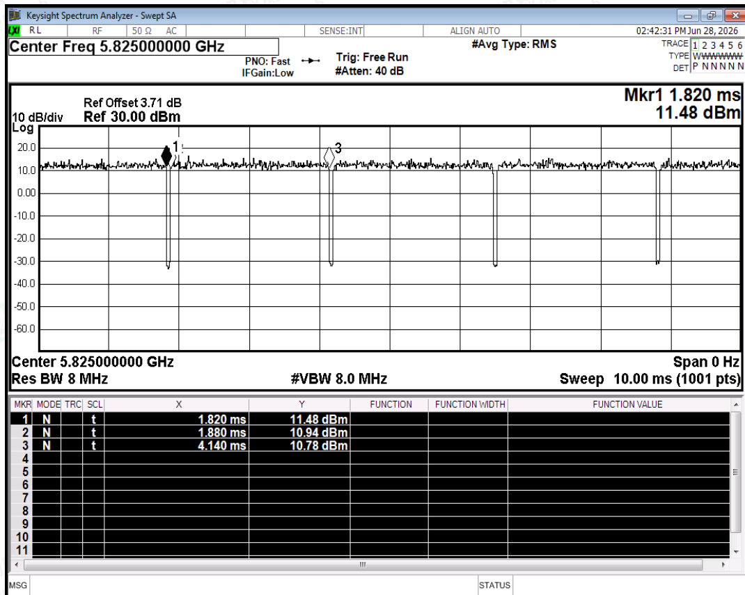
Duty Cycle NVNT n20 5825MHz Ant2
