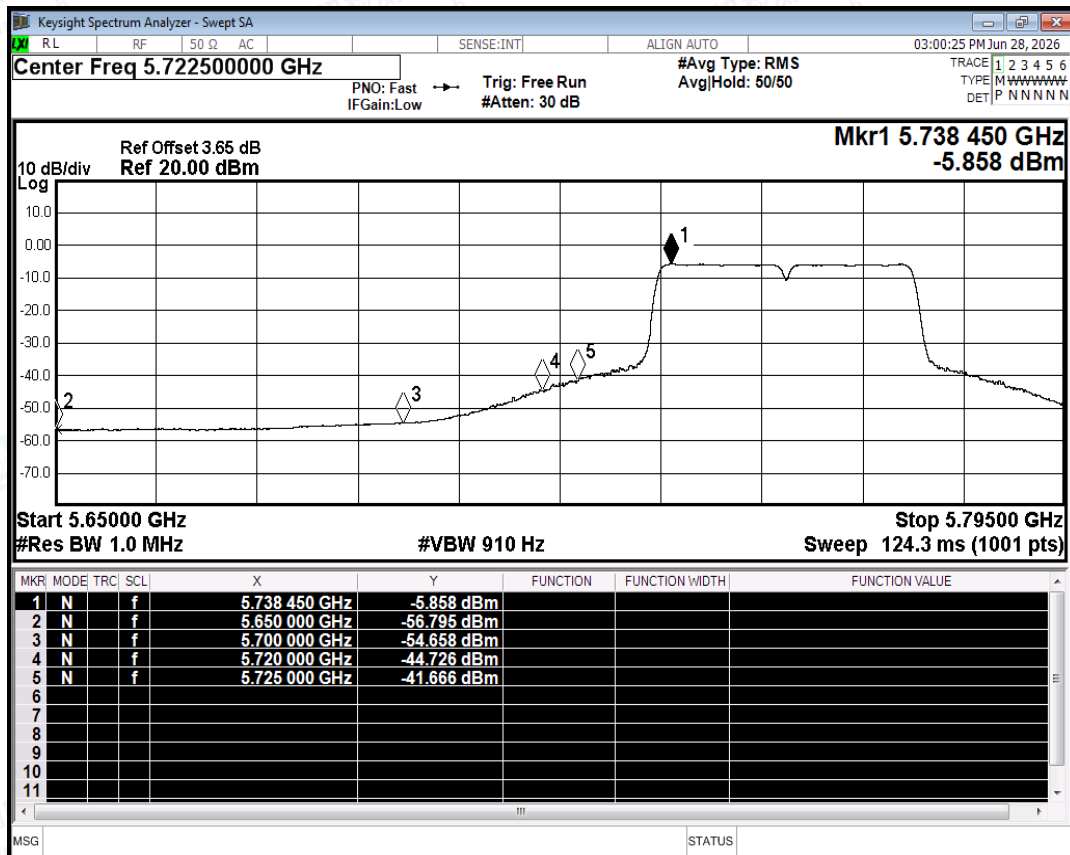
Restrict Band NVNT ac40 5755MHz Ant2 Average
