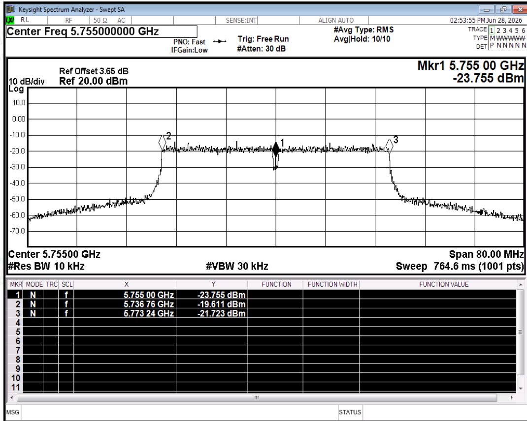
Freq. Stability NVNT n40 5755MHz Ant2
