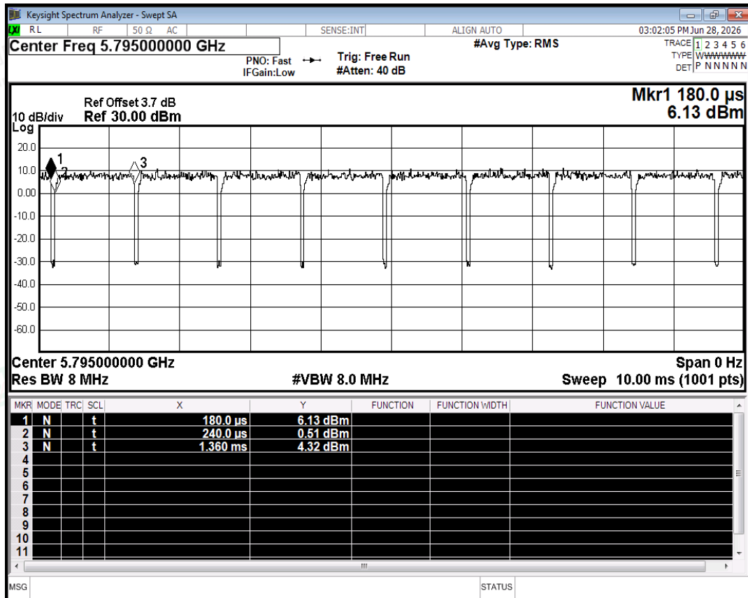
Duty Cycle NVNT ac40 5795MHz Ant2
