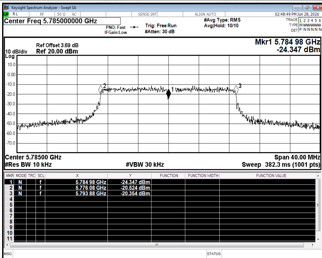
Freq. Stability NVNT ac20 5785MHz Ant2
