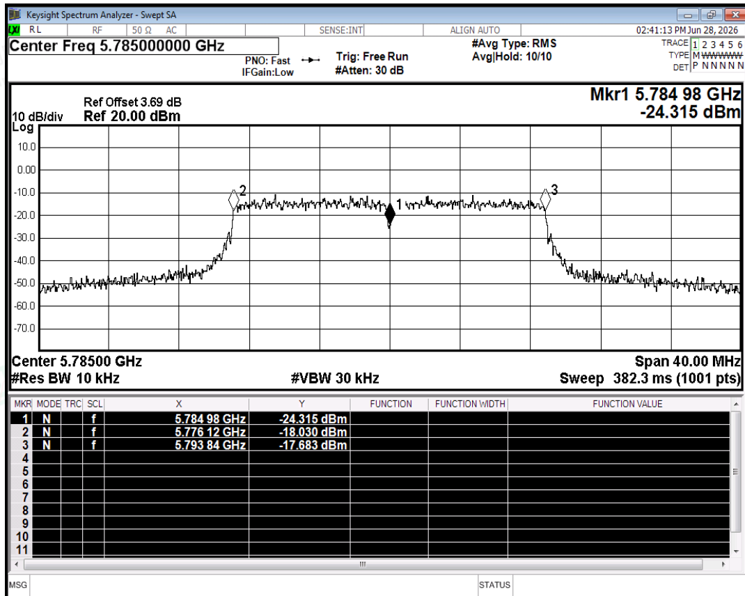
Freq. Stability NVNT n20 5785MHz Ant2
