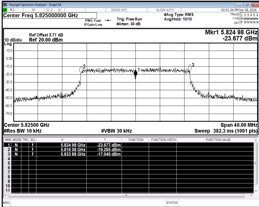
Freq. Stability NVNT ac20 5825MHz Ant2
