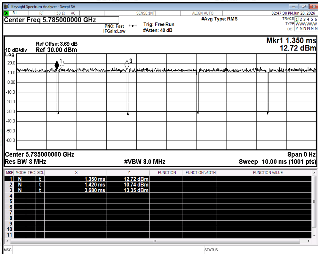
Duty Cycle NVNT ac20 5785MHz Ant2
