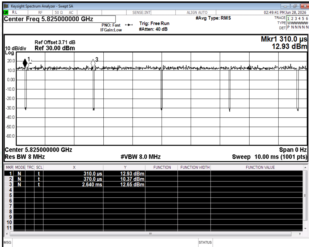
Duty Cycle NVNT ac20 5825MHz Ant2
