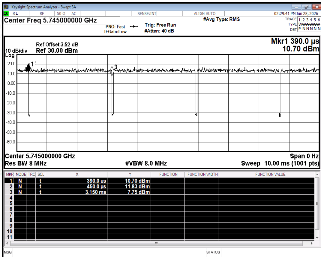
Duty Cycle NVNT a 5745MHz Ant2
