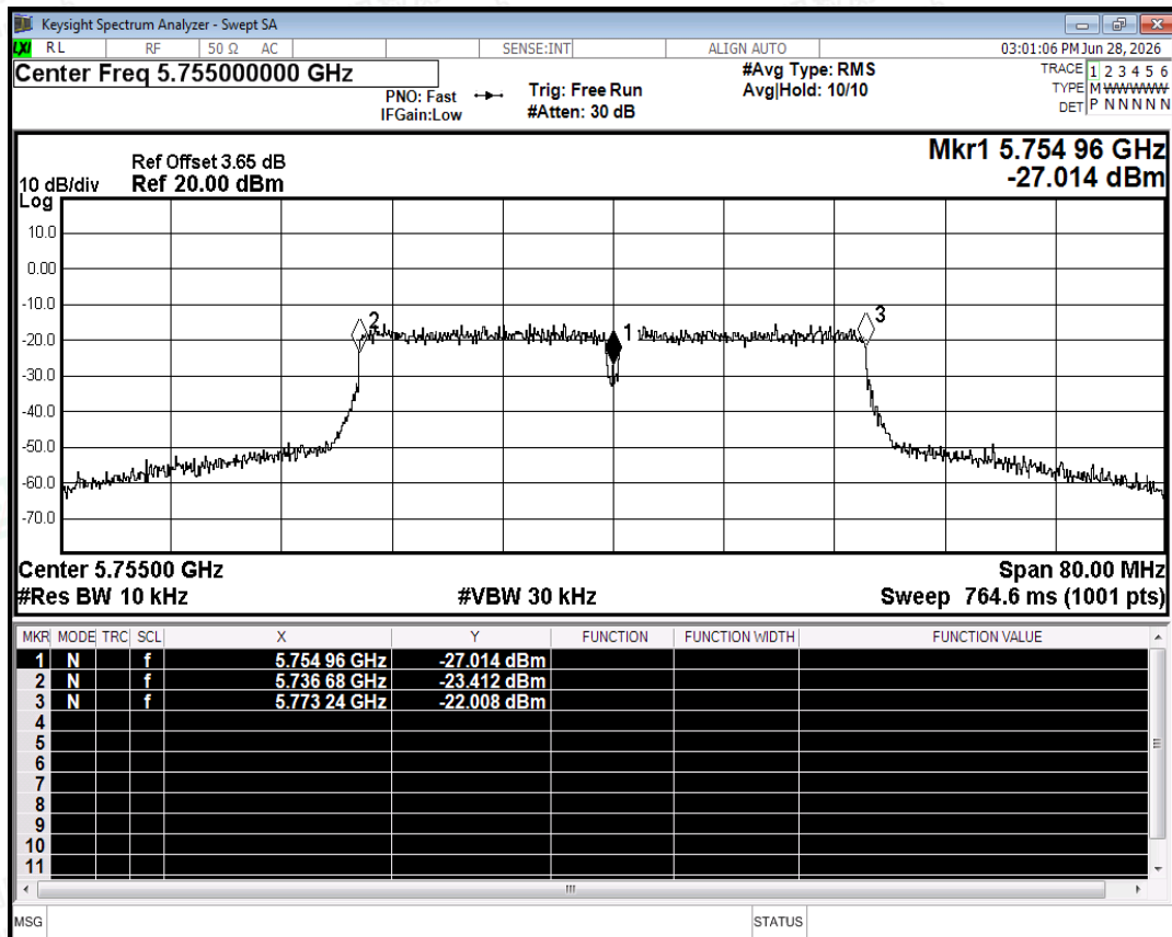
Freq. Stability NVNT ac40 5755MHz Ant2
