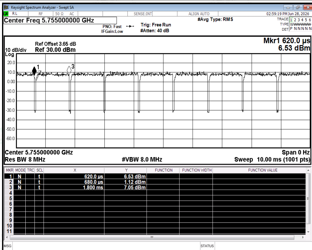
Duty Cycle NVNT ac40 5755MHz Ant2
