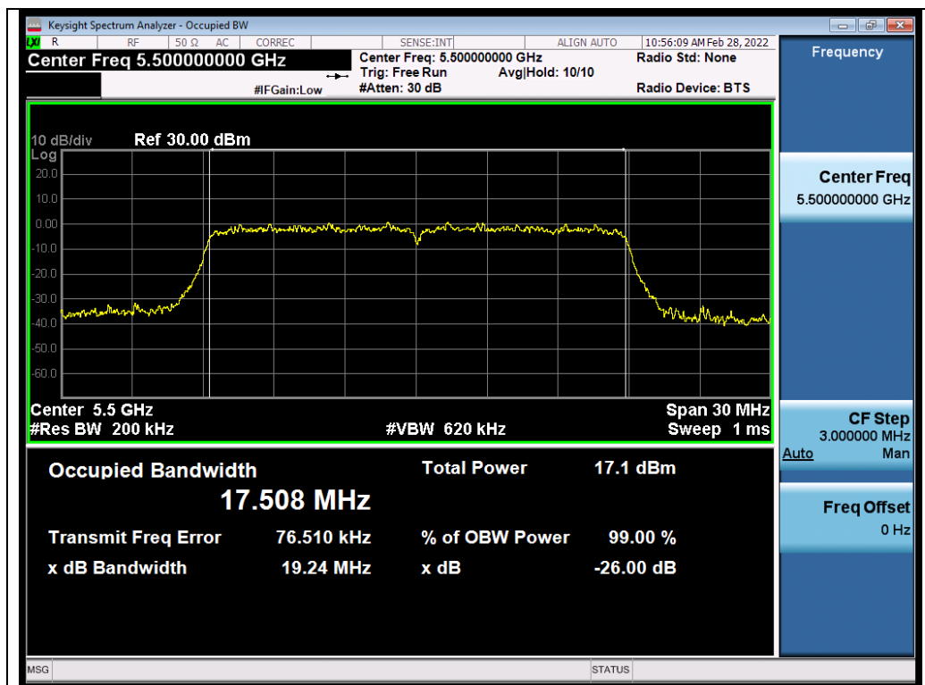
Test_Graph_802.11n20_ANT2_5500_MCS0_OBW
