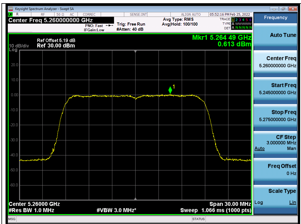
Test_Graph_802.11ac20_ANT1_5260_MCS0_PSD
