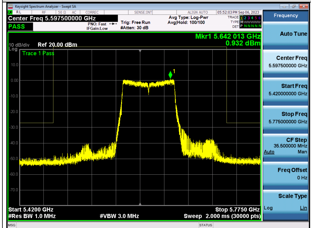
Test_Graph_802.11ac80_ANT2_5610_MCS9_Frequency Band 3
