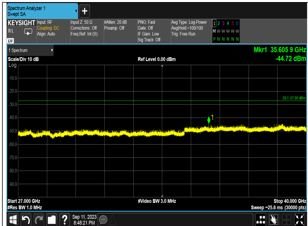
Test_Graph_802.11ac80_ANT1_5610_MCS9_Frequency Band 5
