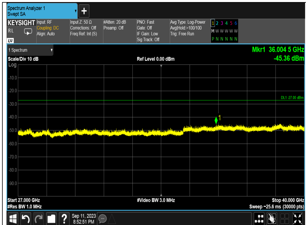
Test_Graph_802.11n40_ANT2_5590_MCS0_Frequency Band 5
